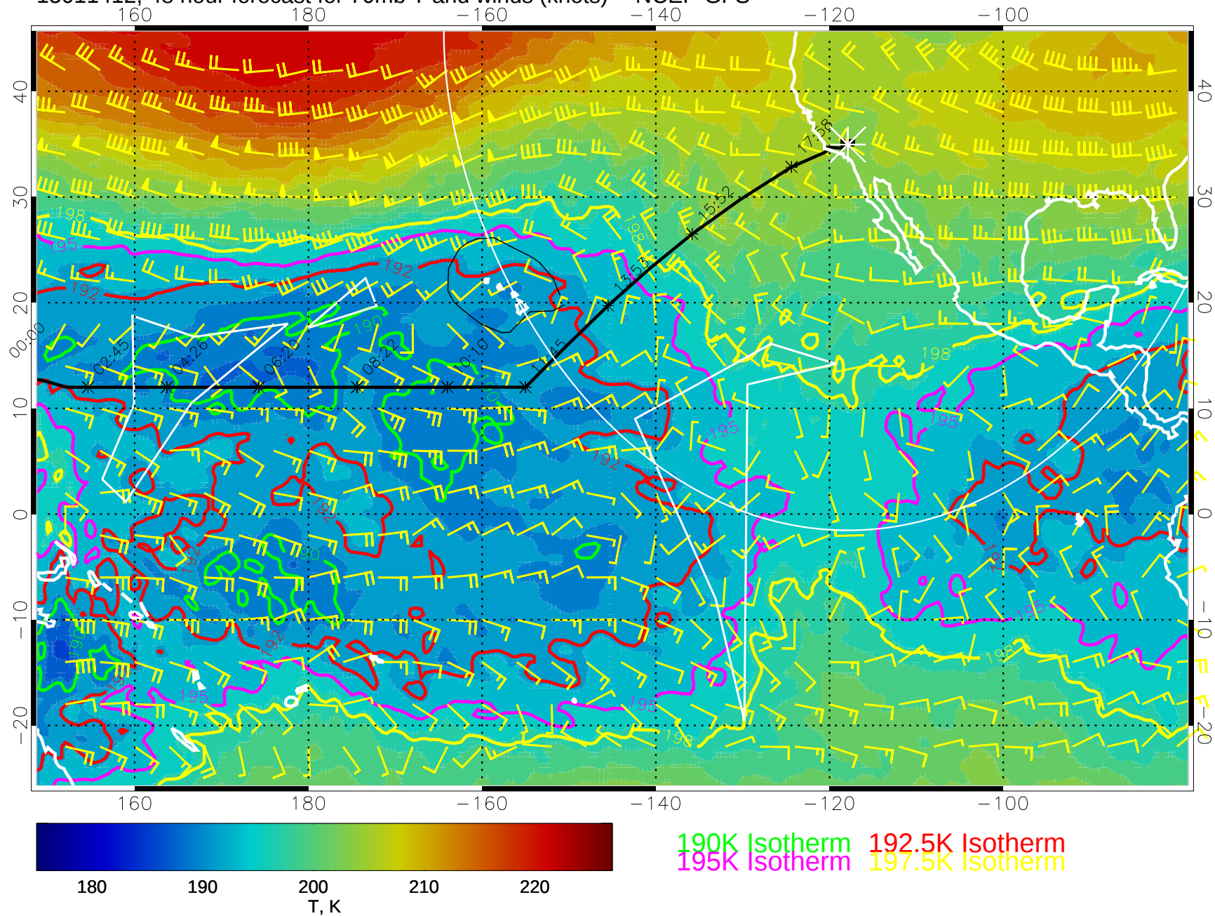
15011412, 48 hour forecast for 70mb T and winds (knots) -- NCEP GFS
