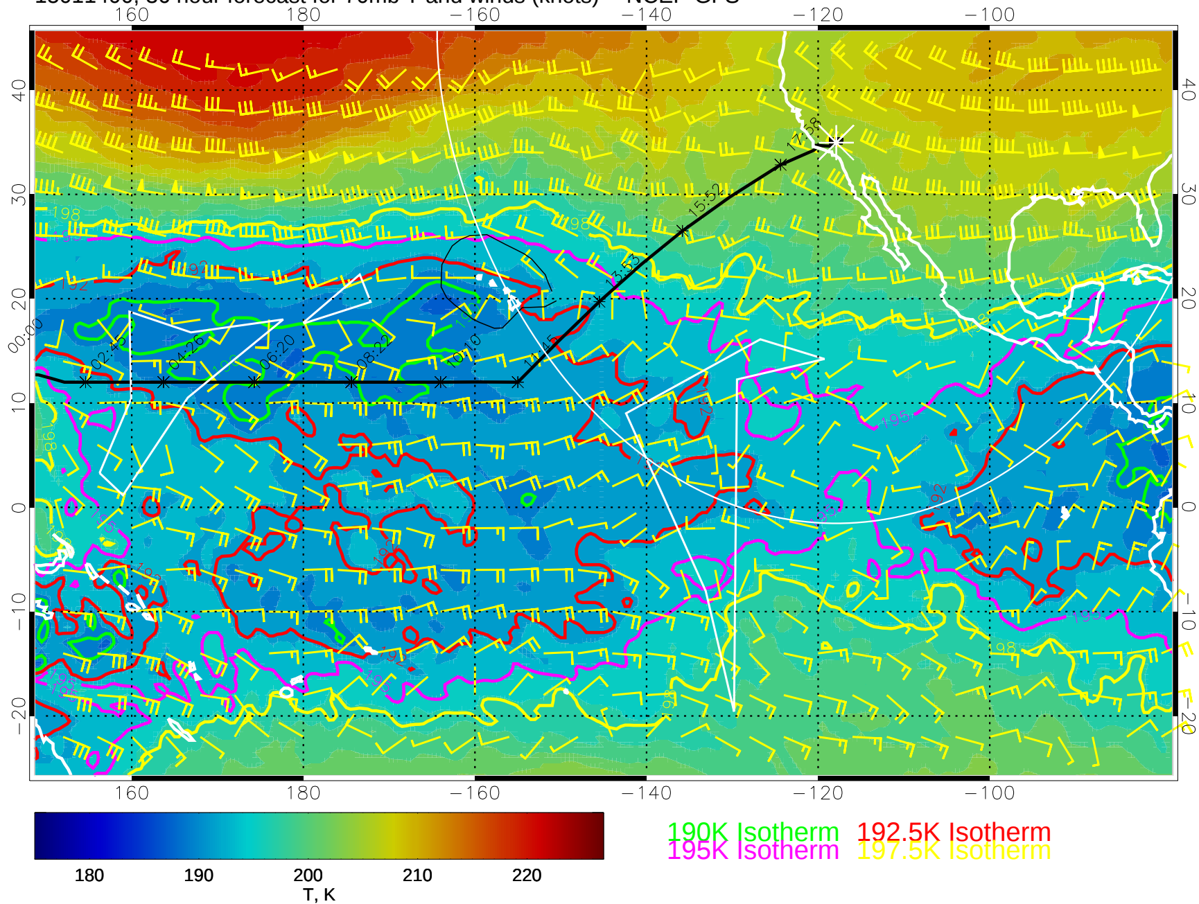
15011400, 36 hour forecast for 70mb T and winds (knots) -- NCEP GFS
