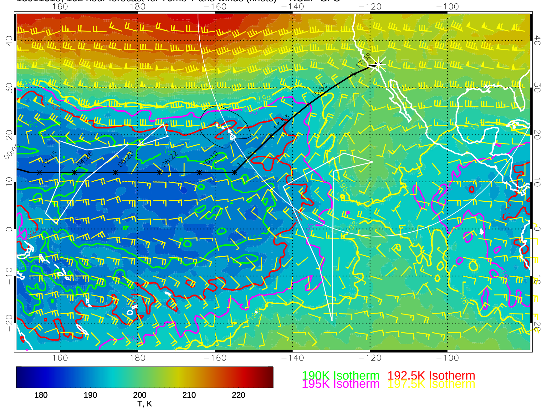
15011618, 102 hour forecast for 70mb T and winds (knots) -- NCEP GFS
