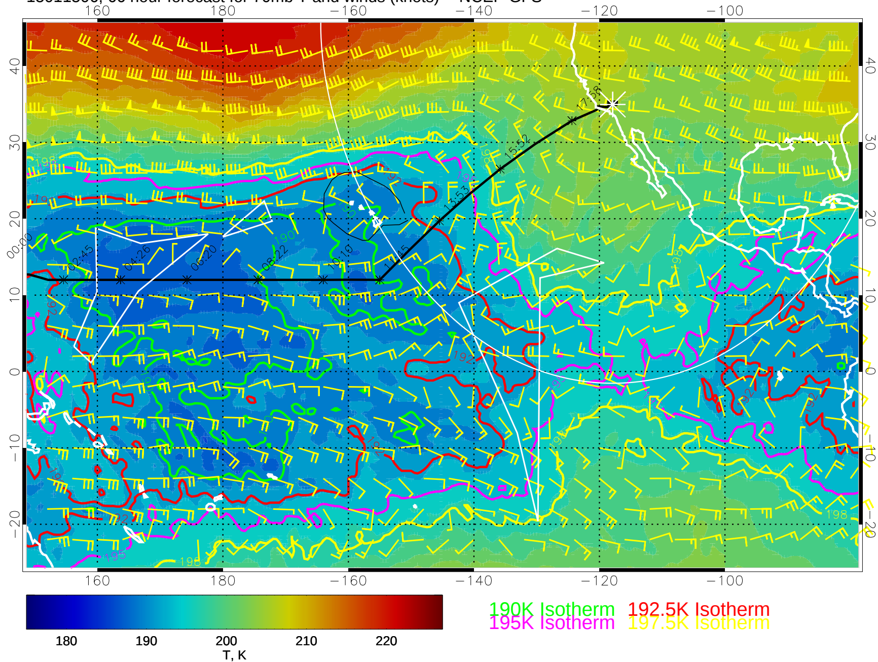
15011506, 66 hour forecast for 70mb T and winds (knots) -- NCEP GFS
