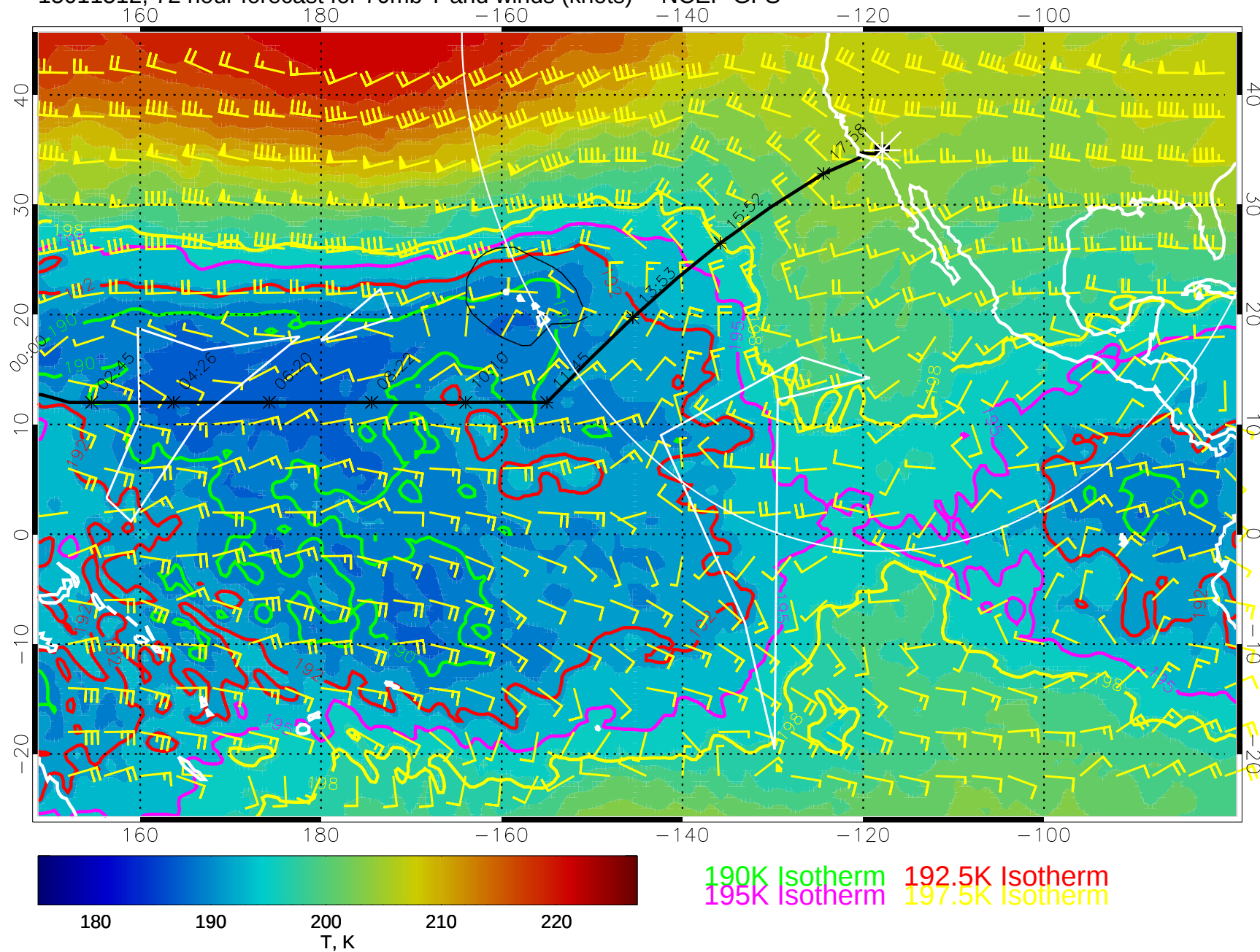
15011512, 72 hour forecast for 70mb T and winds (knots) -- NCEP GFS
