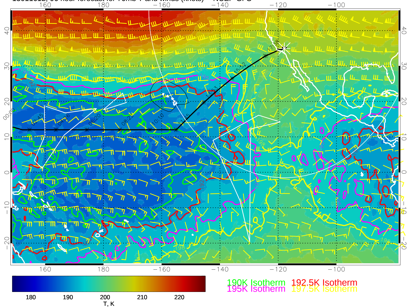
15011612, 96 hour forecast for 70mb T and winds (knots) -- NCEP GFS
