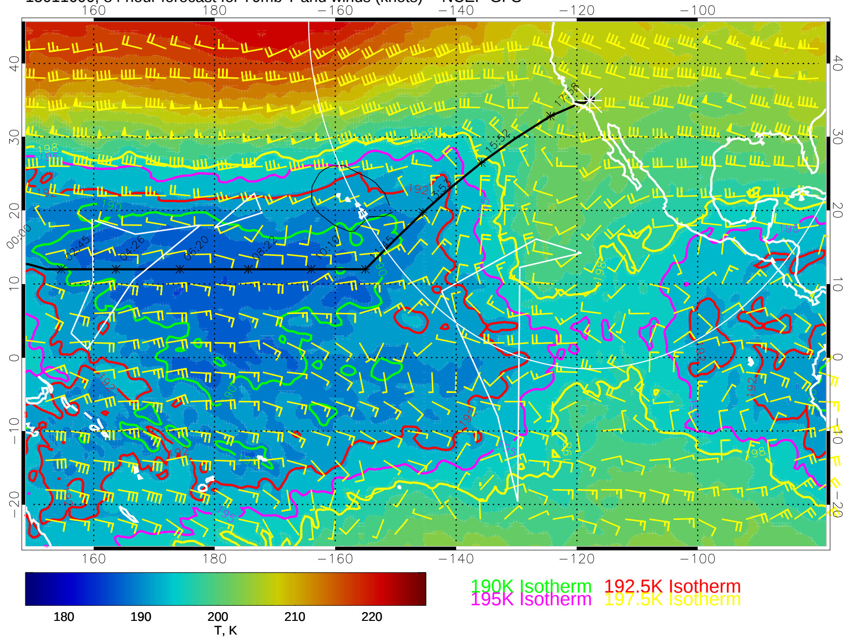
15011600, 84 hour forecast for 70mb T and winds (knots) -- NCEP GFS
