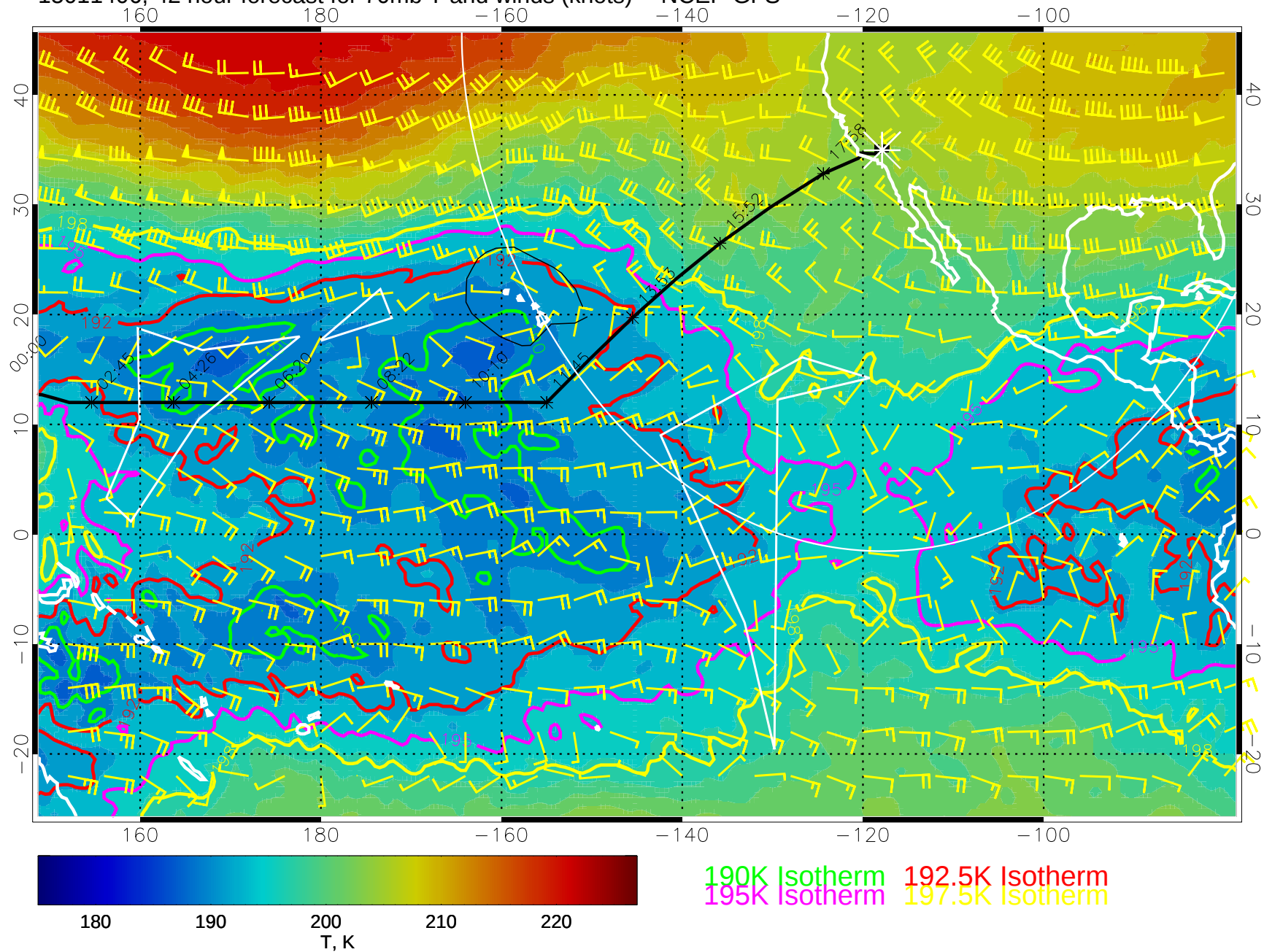
15011406, 42 hour forecast for 70mb T and winds (knots) -- NCEP GFS
