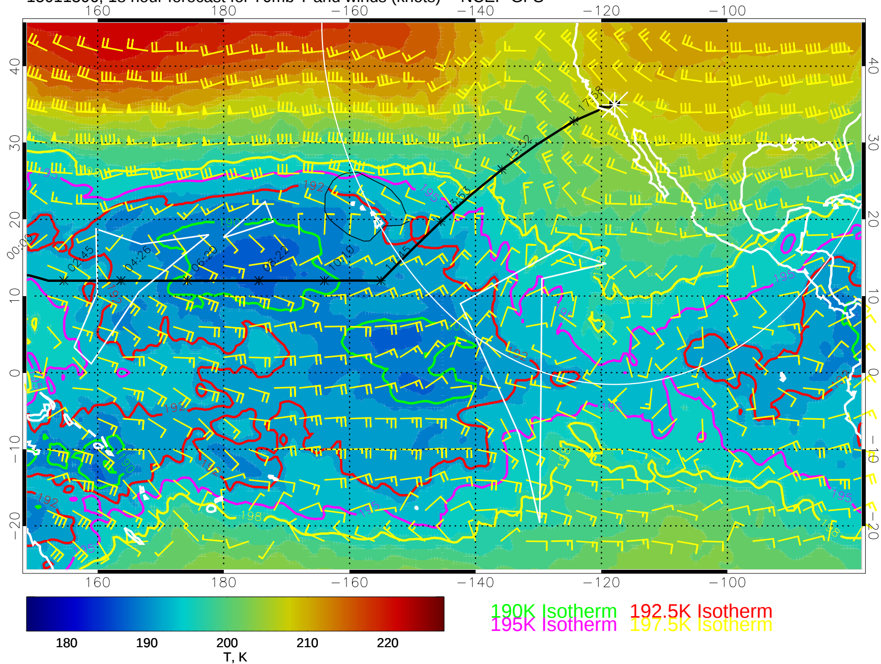
15011306, 18 hour forecast for 70mb T and winds (knots) -- NCEP GFS
