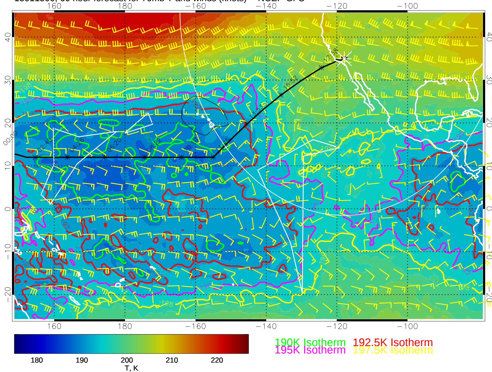
15011500, 60 hour forecast for 70mb T and winds (knots) -- NCEP GFS
