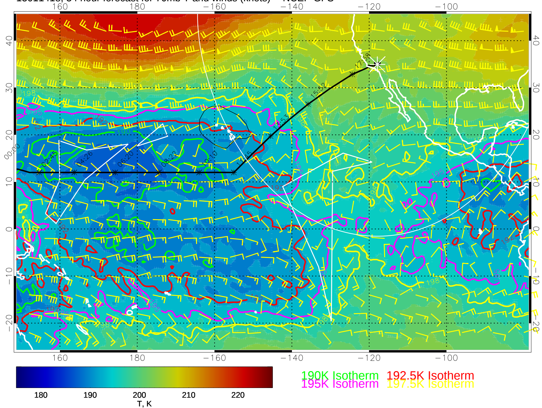
15011418, 54 hour forecast for 70mb T and winds (knots) -- NCEP GFS
