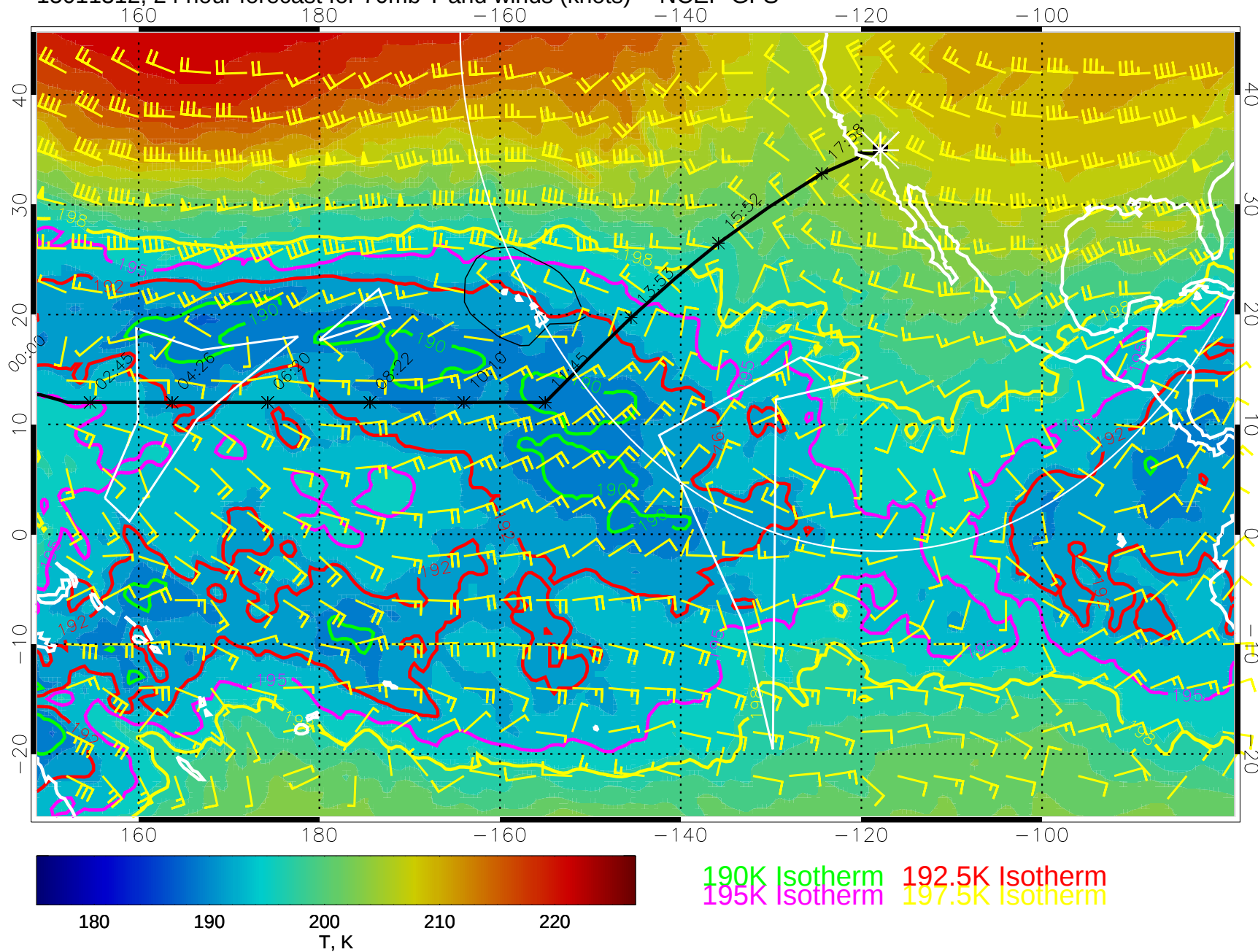
15011312, 24 hour forecast for 70mb T and winds (knots) -- NCEP GFS
