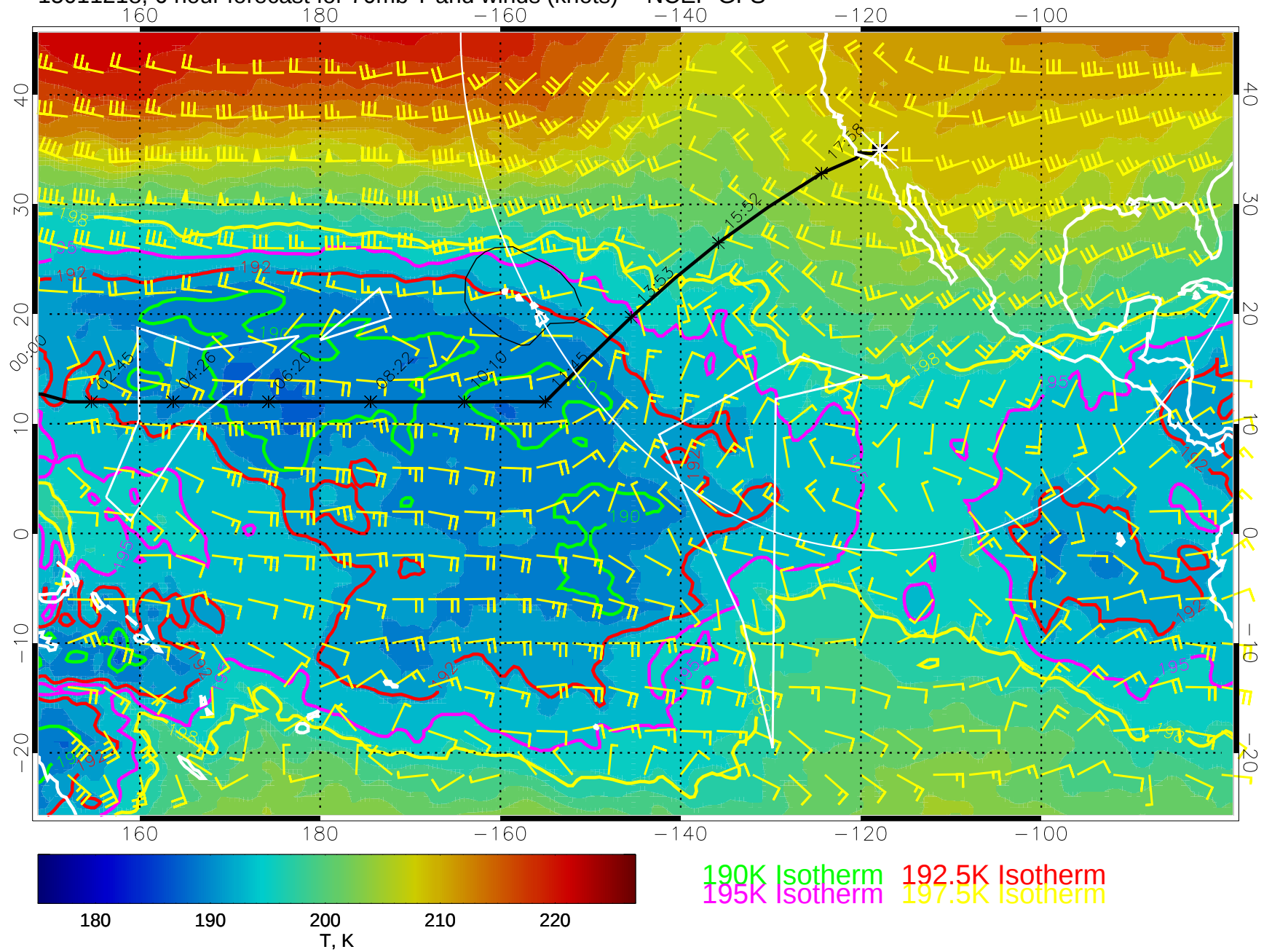
15011218, 6 hour forecast for 70mb T and winds (knots) -- NCEP GFS
