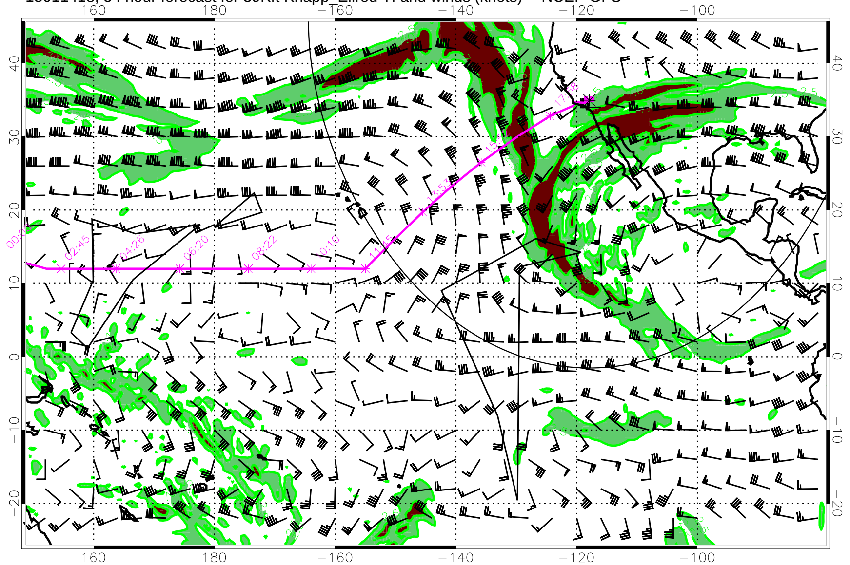
15011418, 54 hour forecast for 39Kft Knapp_Ellrod TI and winds (knots) -- NCEP GFS
