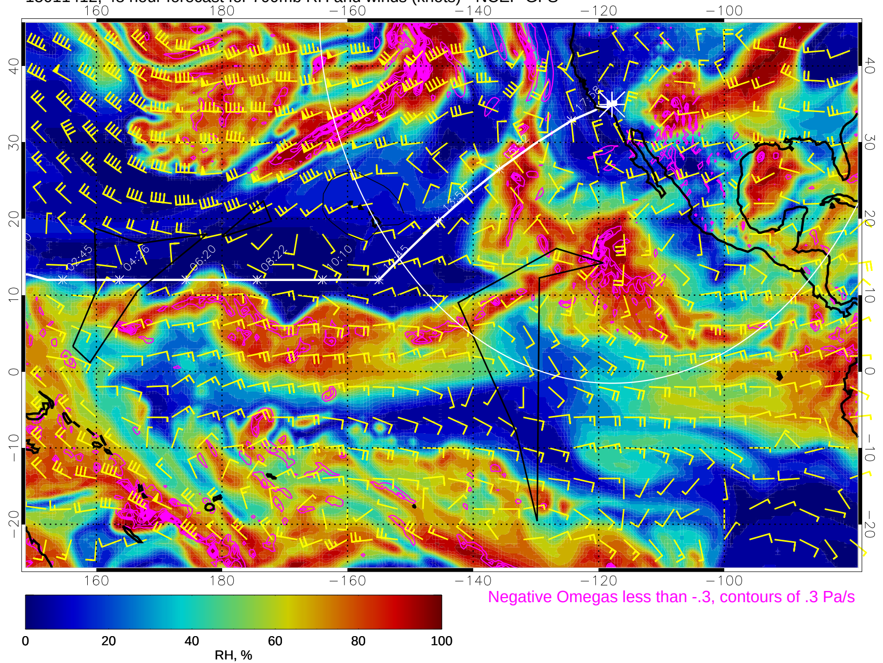
15011412, 48 hour forecast for 700mb RH and winds (knots) - NCEP GFS
