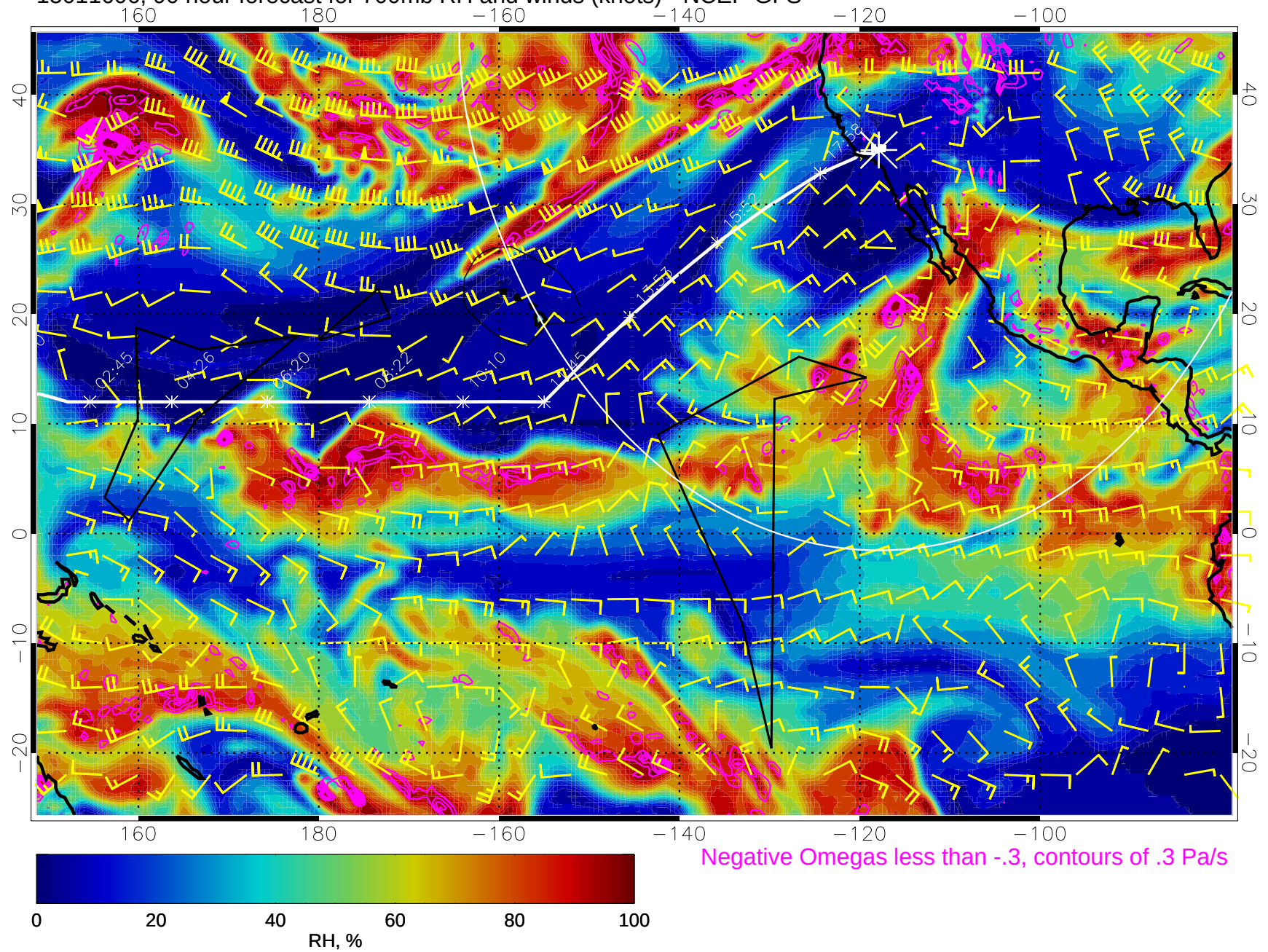
15011606, 90 hour forecast for 700mb RH and winds (knots) - NCEP GFS
