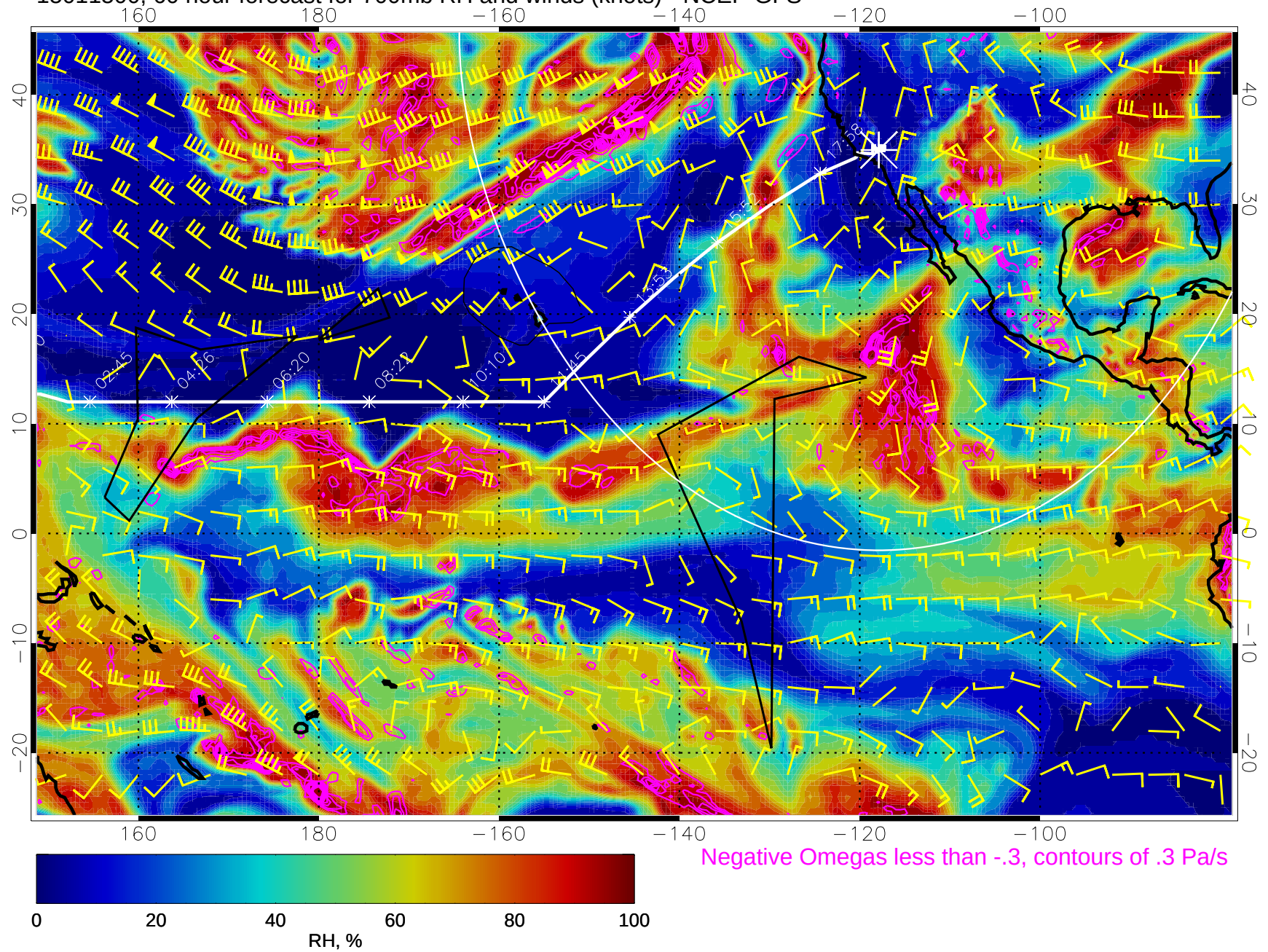
15011500, 60 hour forecast for 700mb RH and winds (knots) - NCEP GFS
