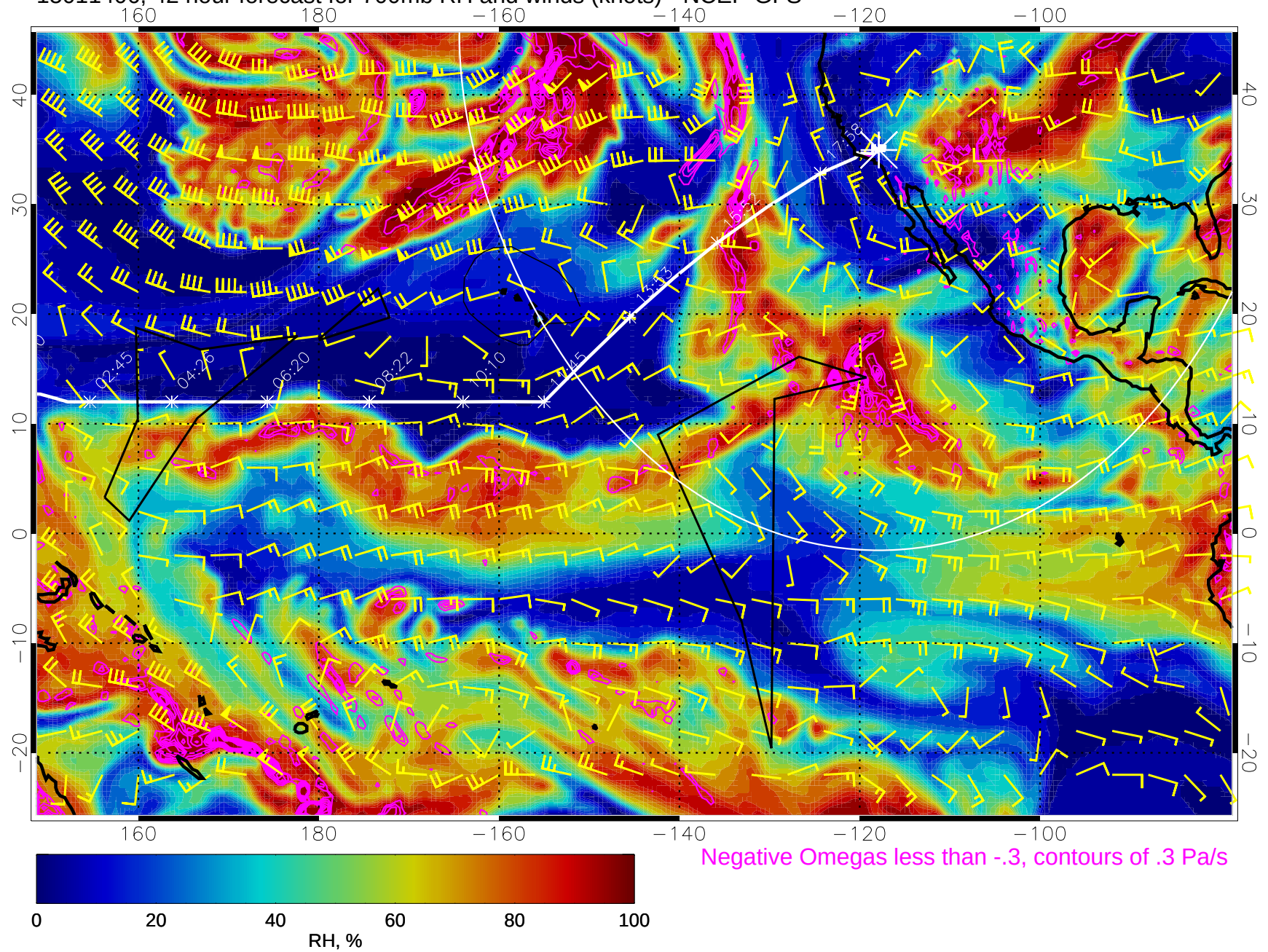
15011406, 42 hour forecast for 700mb RH and winds (knots) - NCEP GFS
