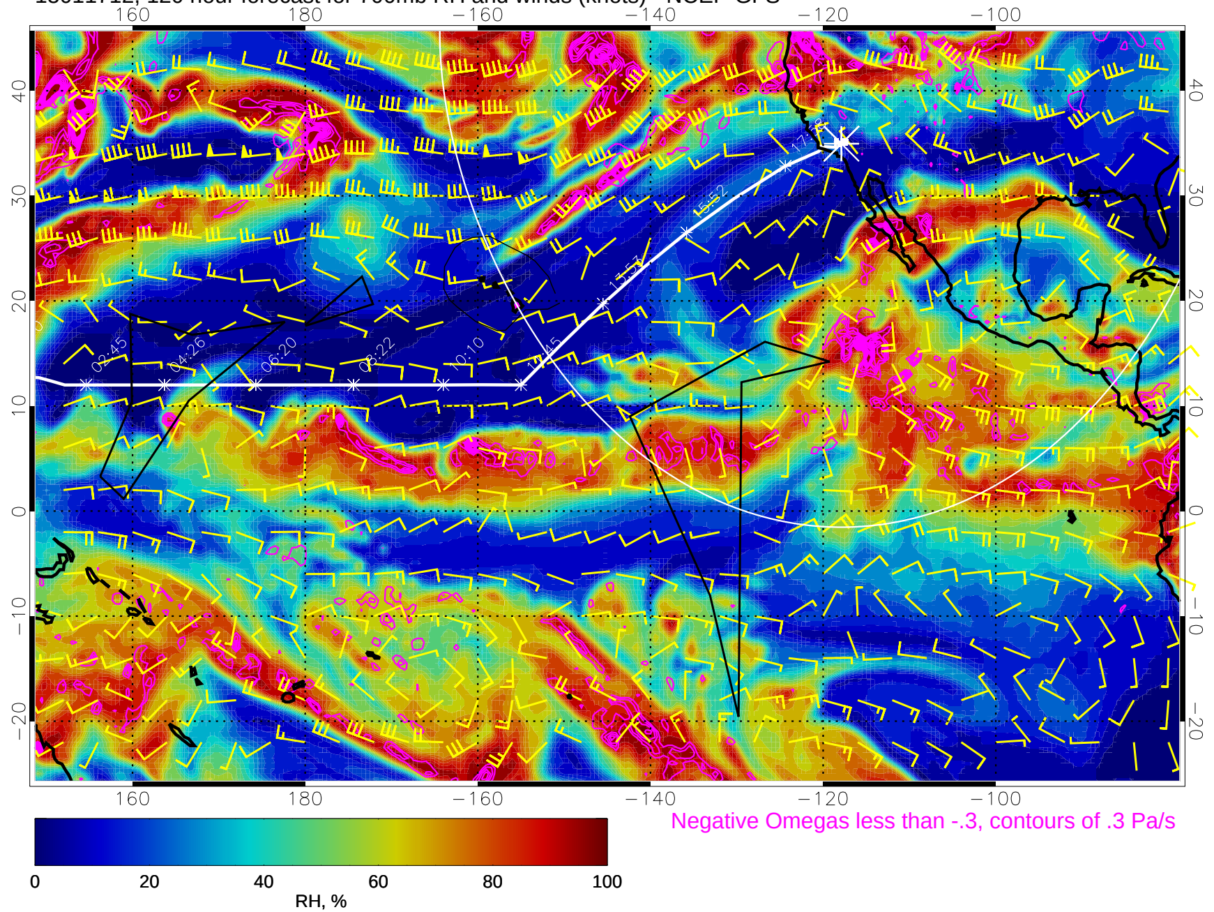
15011712, 120 hour forecast for 700mb RH and winds (knots) - NCEP GFS
