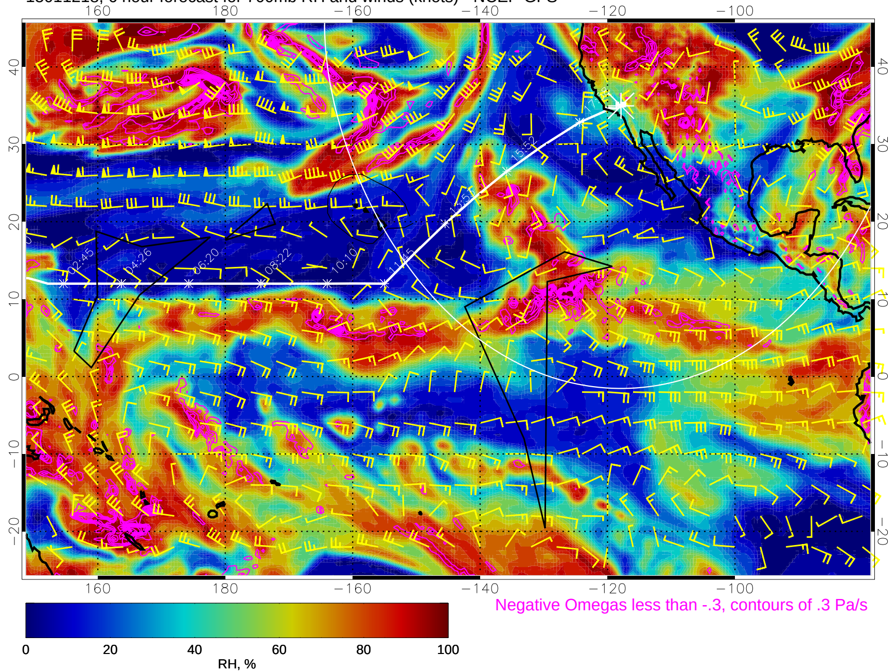
15011218, 6 hour forecast for 700mb RH and winds (knots) - NCEP GFS
