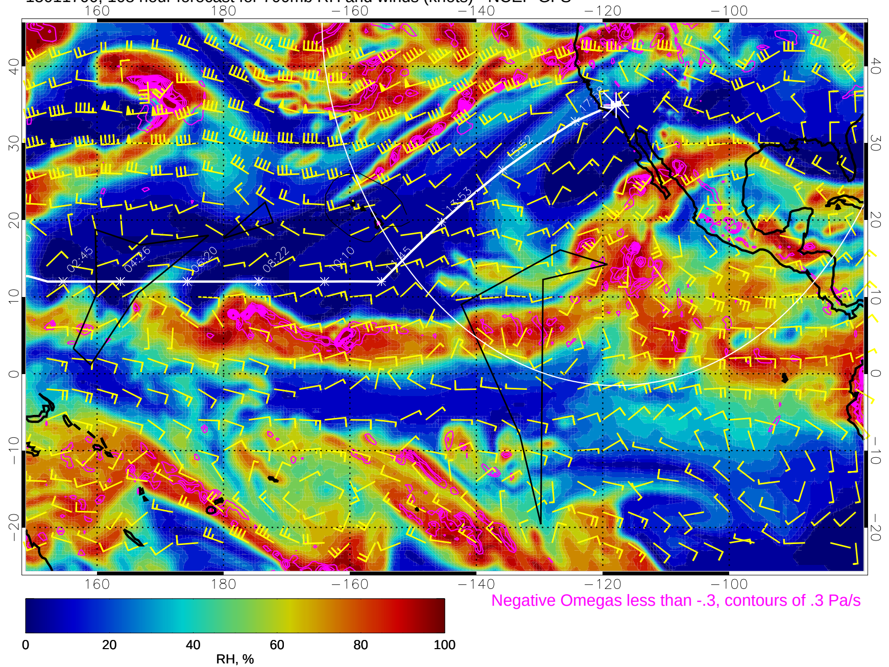
15011700, 108 hour forecast for 700mb RH and winds (knots) - NCEP GFS
