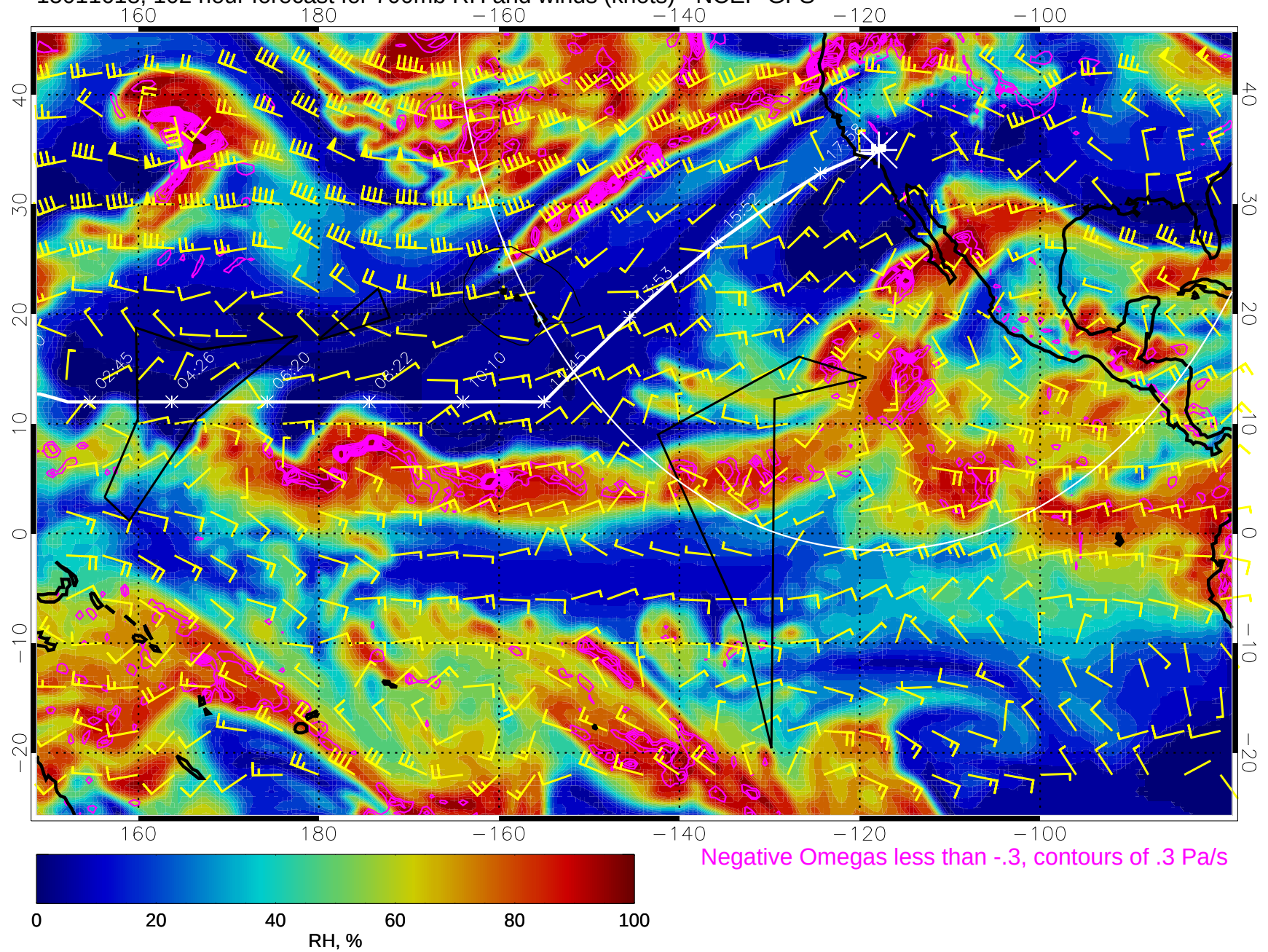
15011618, 102 hour forecast for 700mb RH and winds (knots) - NCEP GFS
