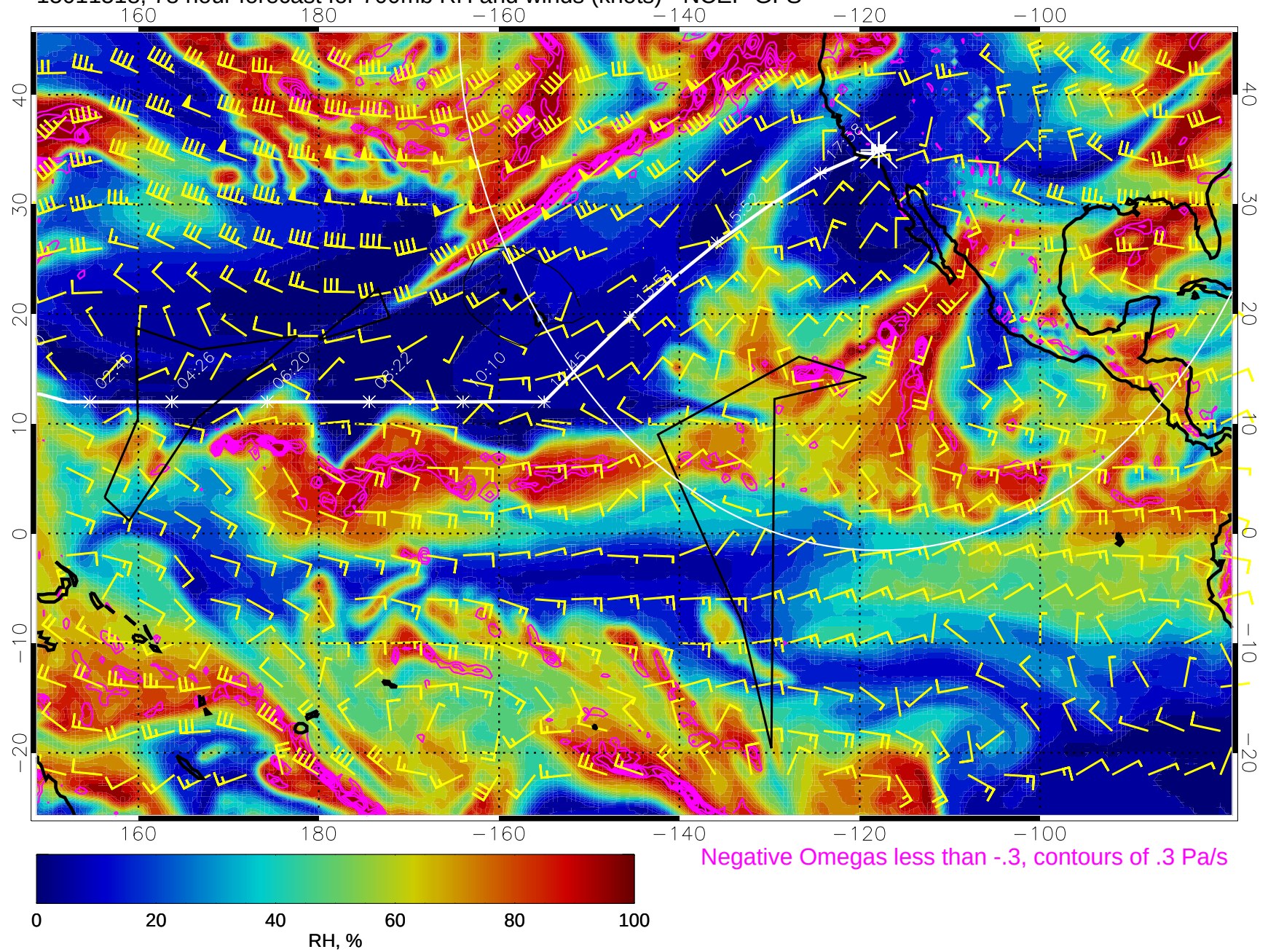
15011518, 78 hour forecast for 700mb RH and winds (knots) - NCEP GFS
