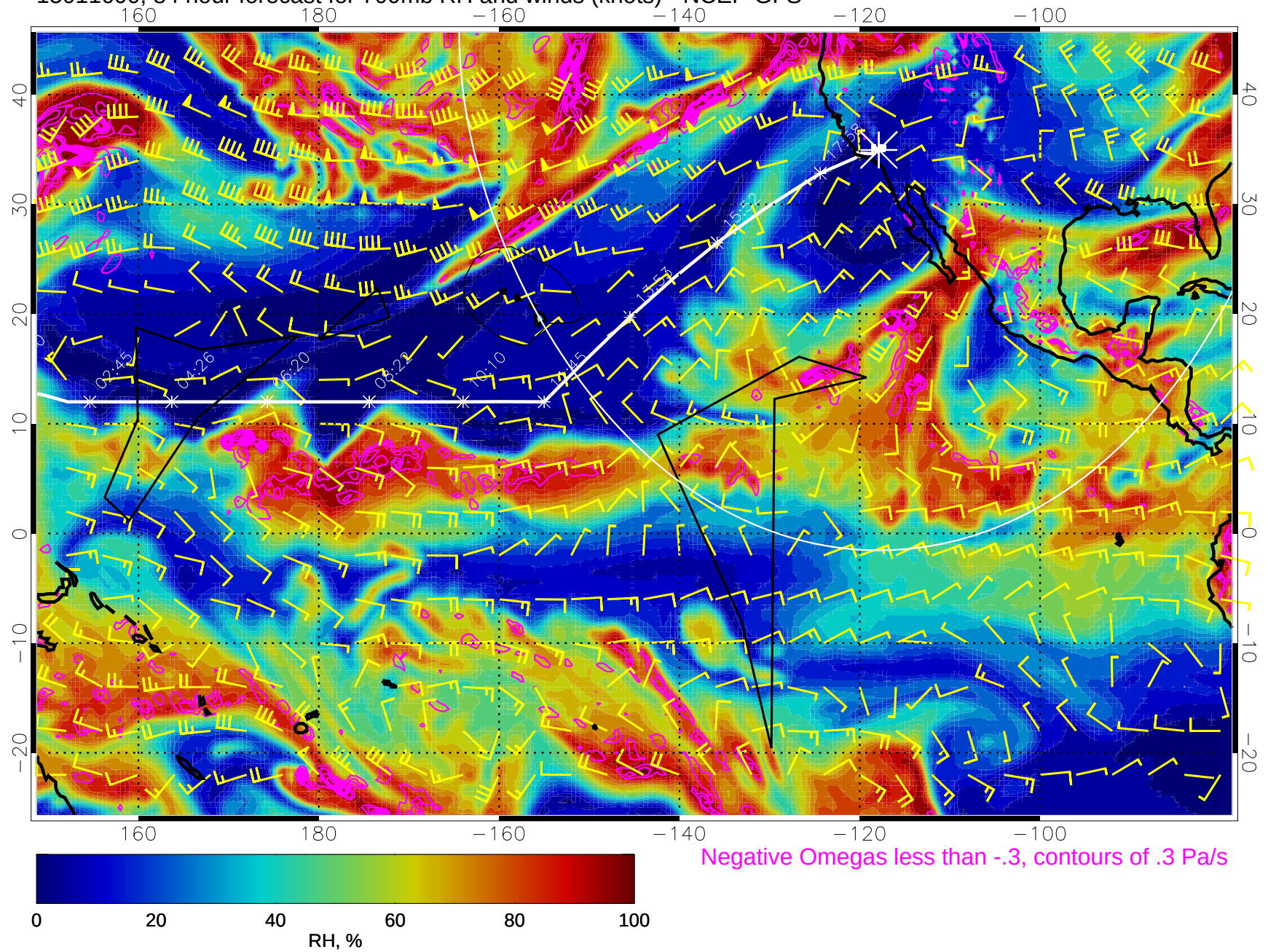
15011600, 84 hour forecast for 700mb RH and winds (knots) - NCEP GFS
