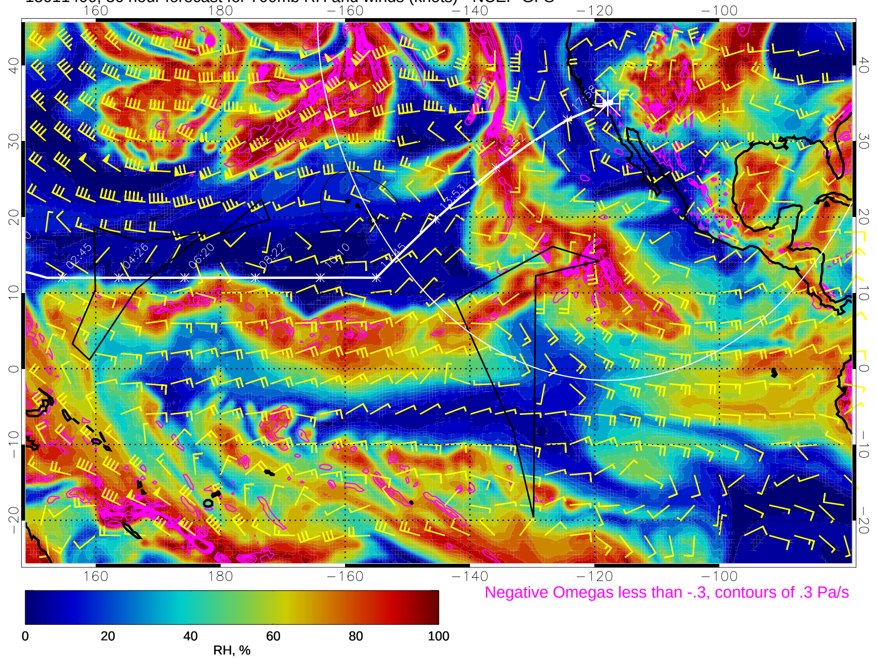
15011400, 36 hour forecast for 700mb RH and winds (knots) - NCEP GFS
