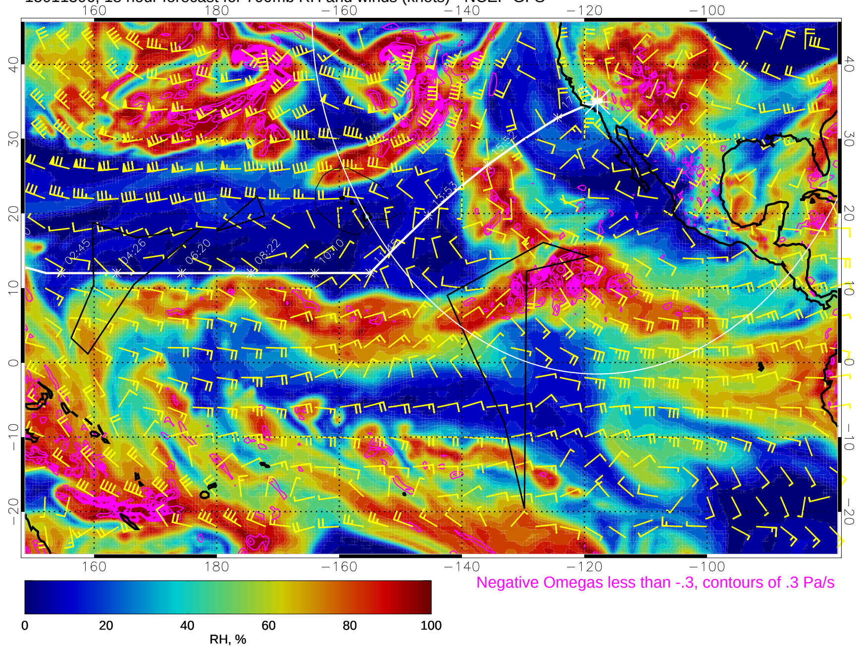
15011306, 18 hour forecast for 700mb RH and winds (knots) - NCEP GFS
