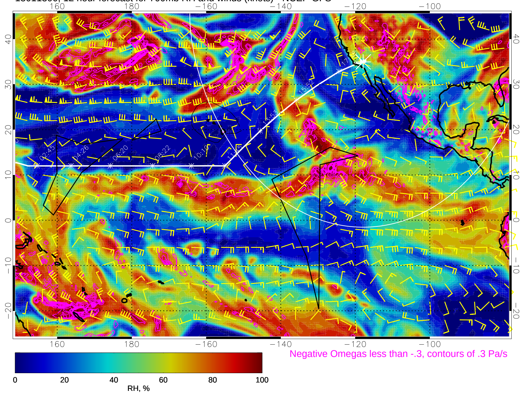
15011300, 12 hour forecast for 700mb RH and winds (knots) - NCEP GFS
