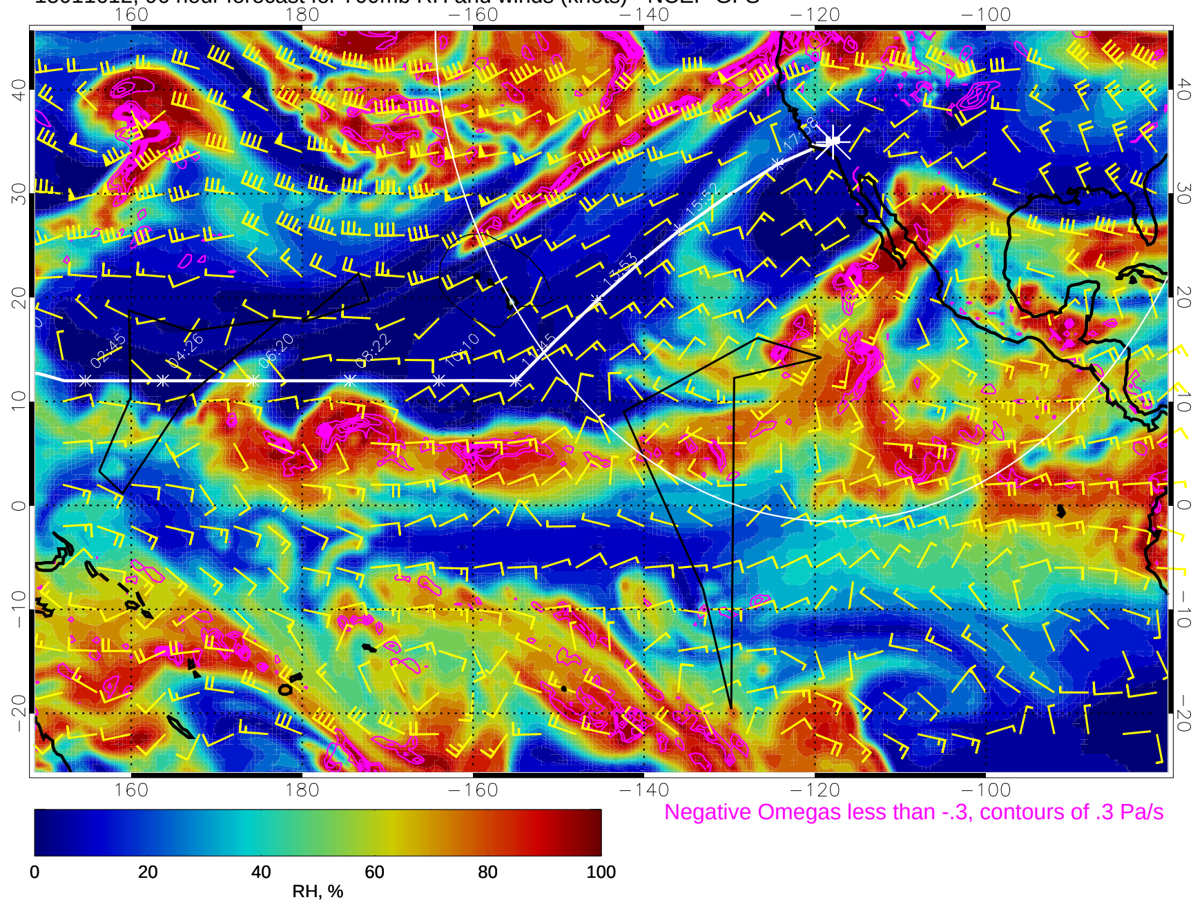
15011612, 96 hour forecast for 700mb RH and winds (knots) - NCEP GFS
