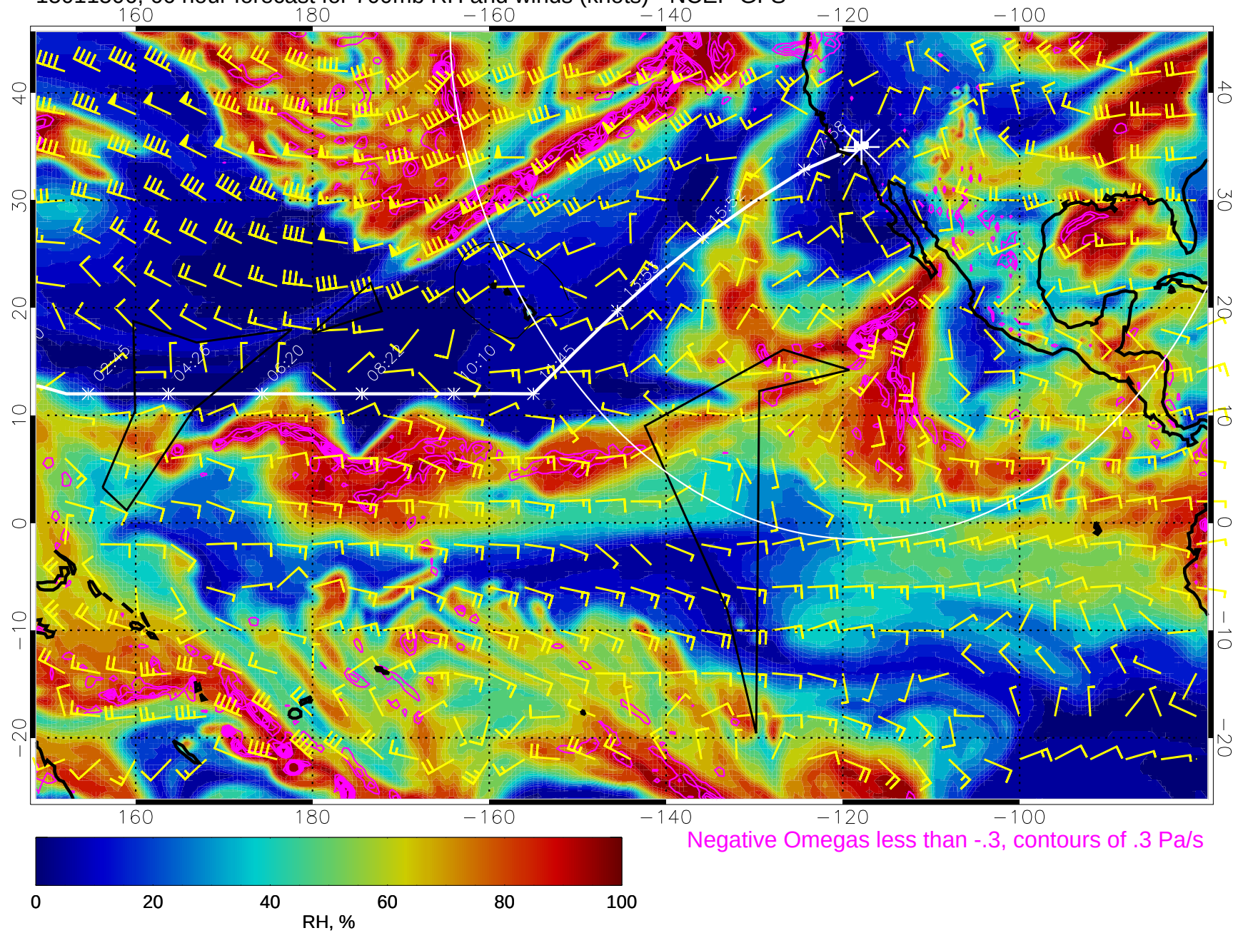
15011506, 66 hour forecast for 700mb RH and winds (knots) - NCEP GFS
