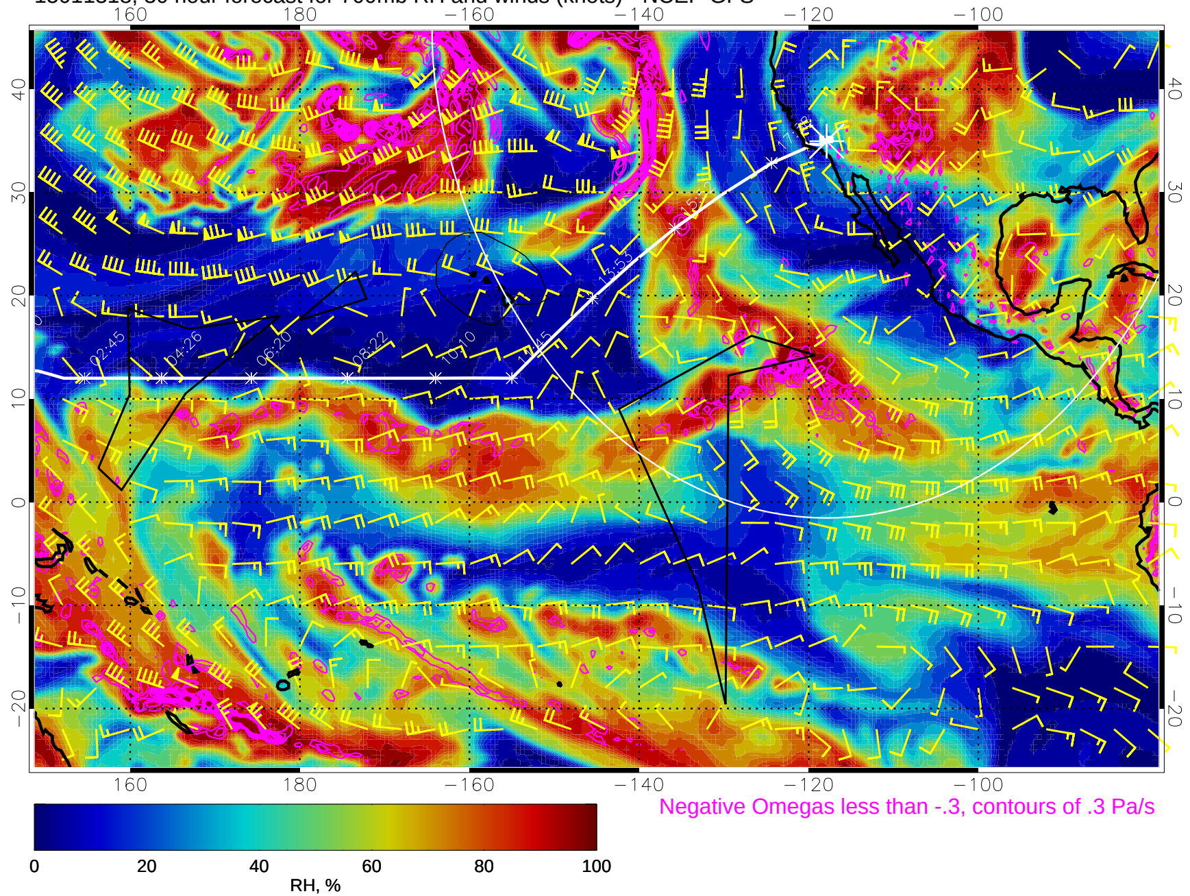
15011318, 30 hour forecast for 700mb RH and winds (knots) - NCEP GFS
