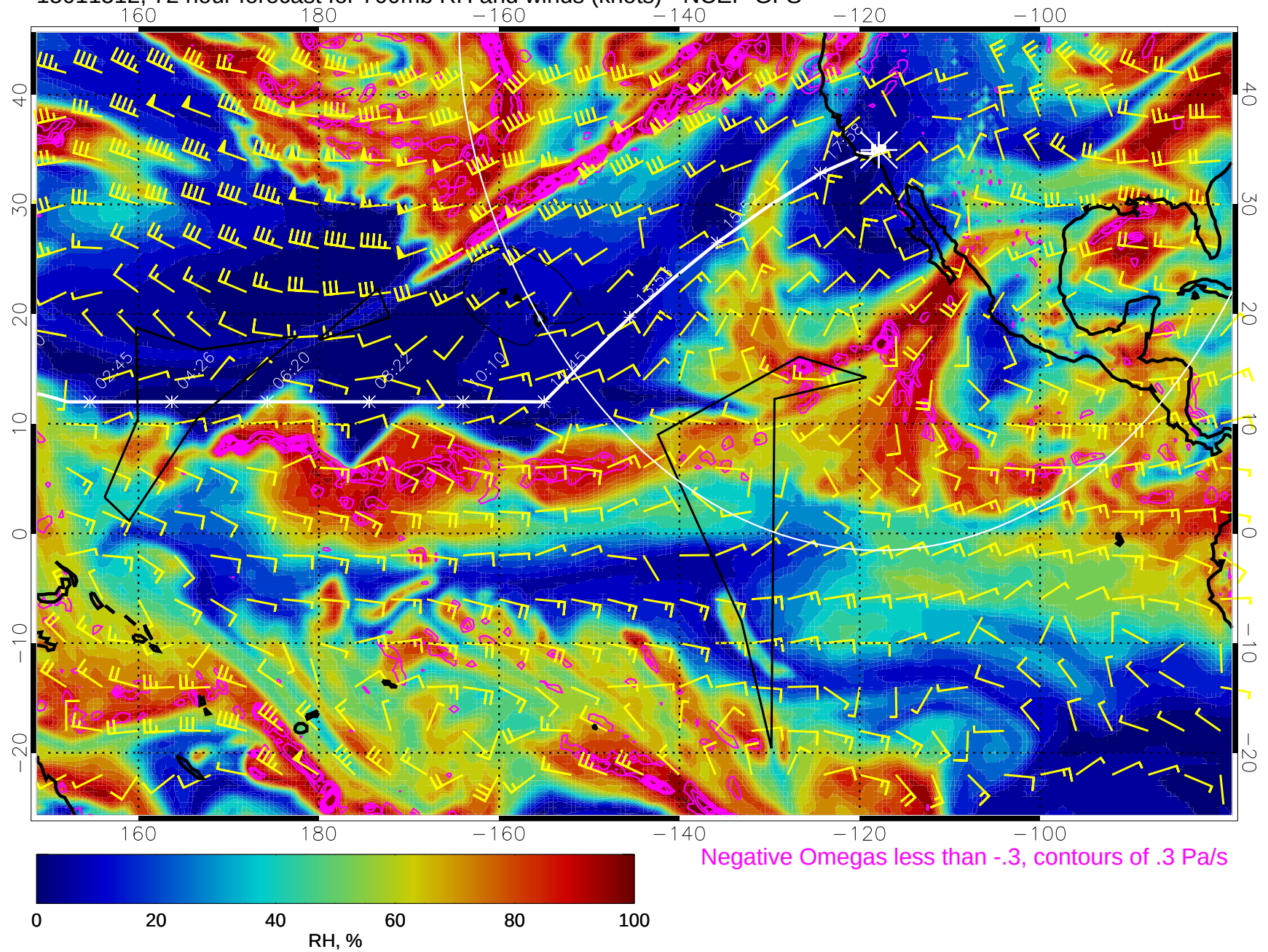
15011512, 72 hour forecast for 700mb RH and winds (knots) - NCEP GFS
