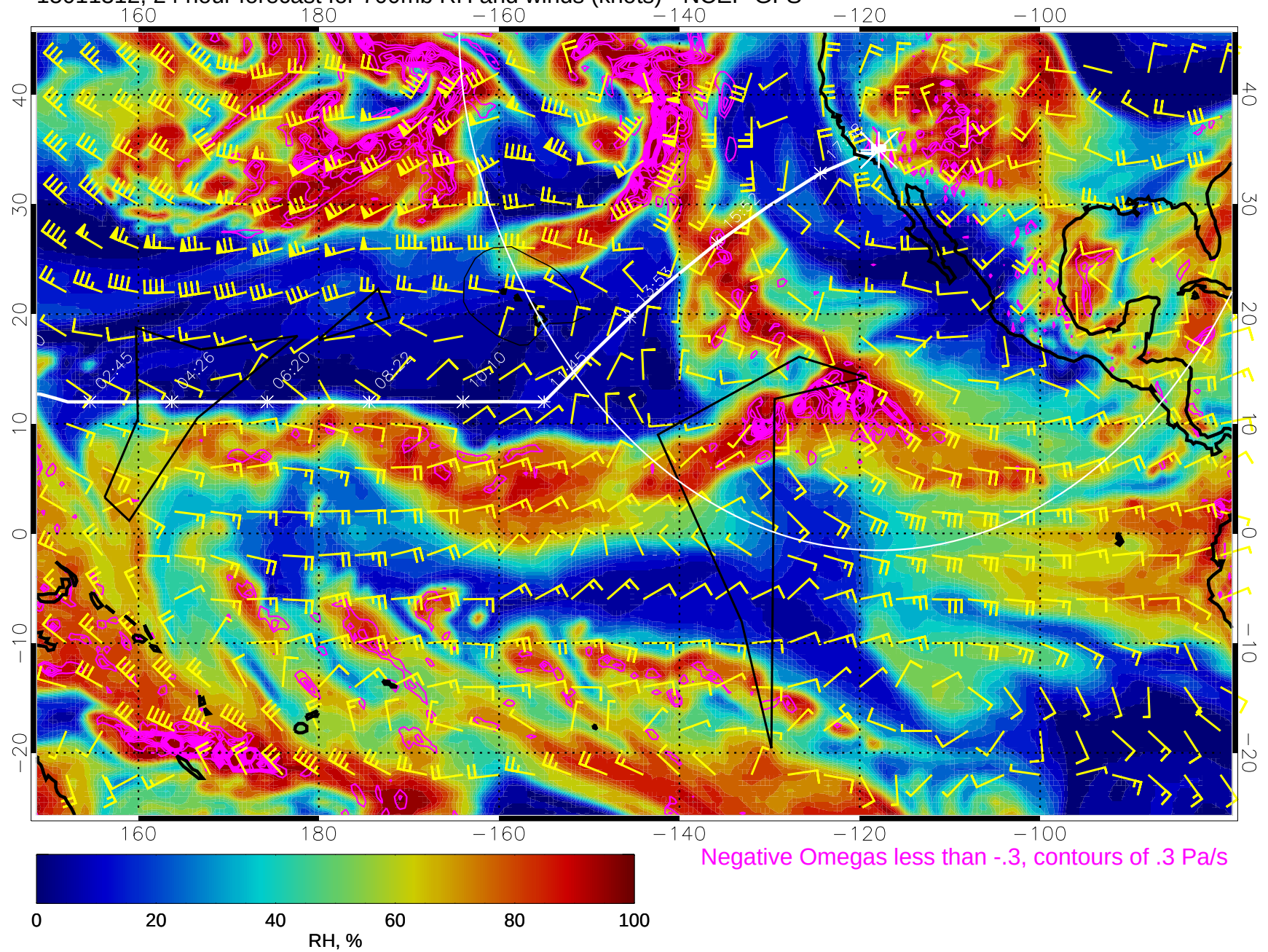
15011312, 24 hour forecast for 700mb RH and winds (knots) - NCEP GFS
