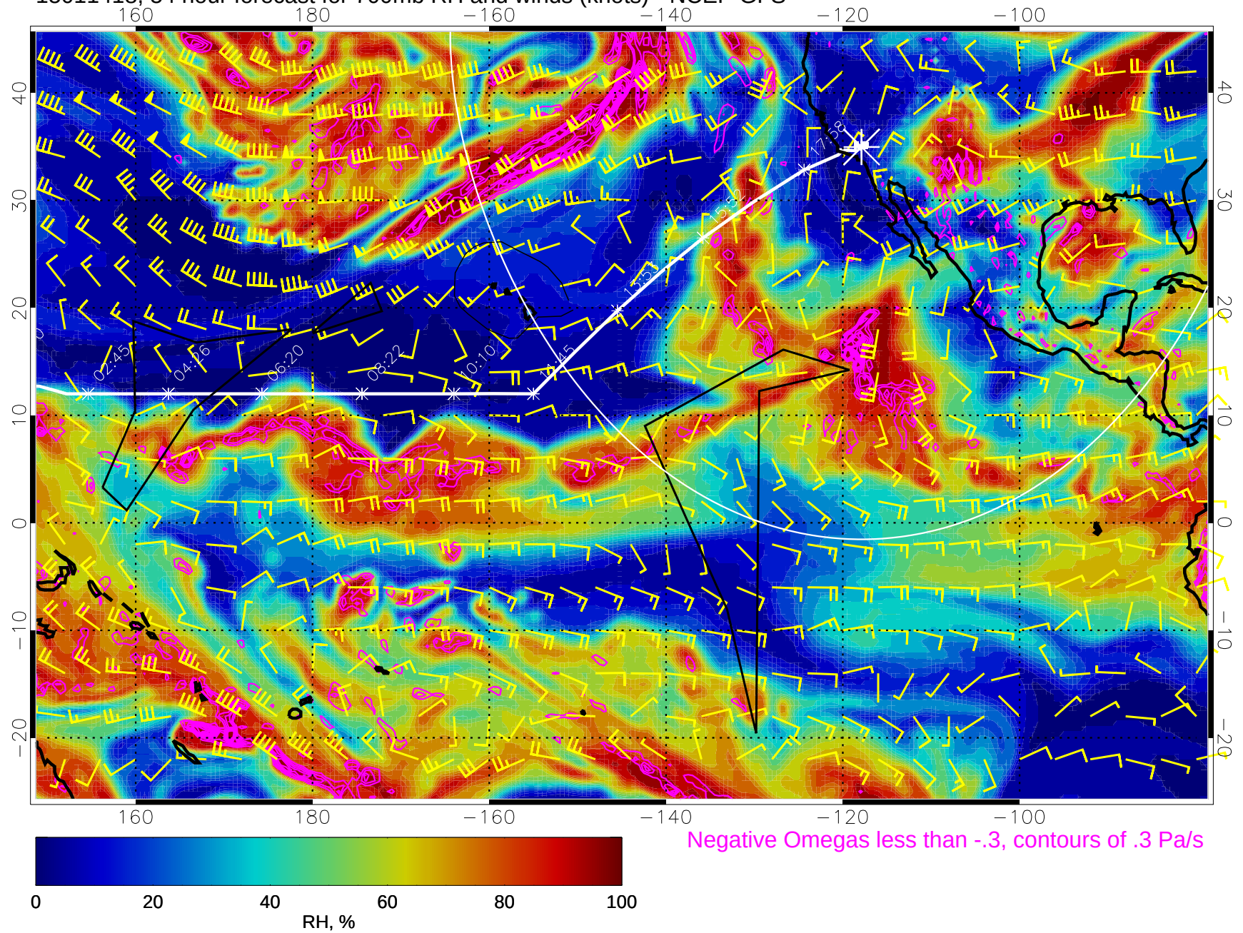
15011418, 54 hour forecast for 700mb RH and winds (knots) - NCEP GFS
