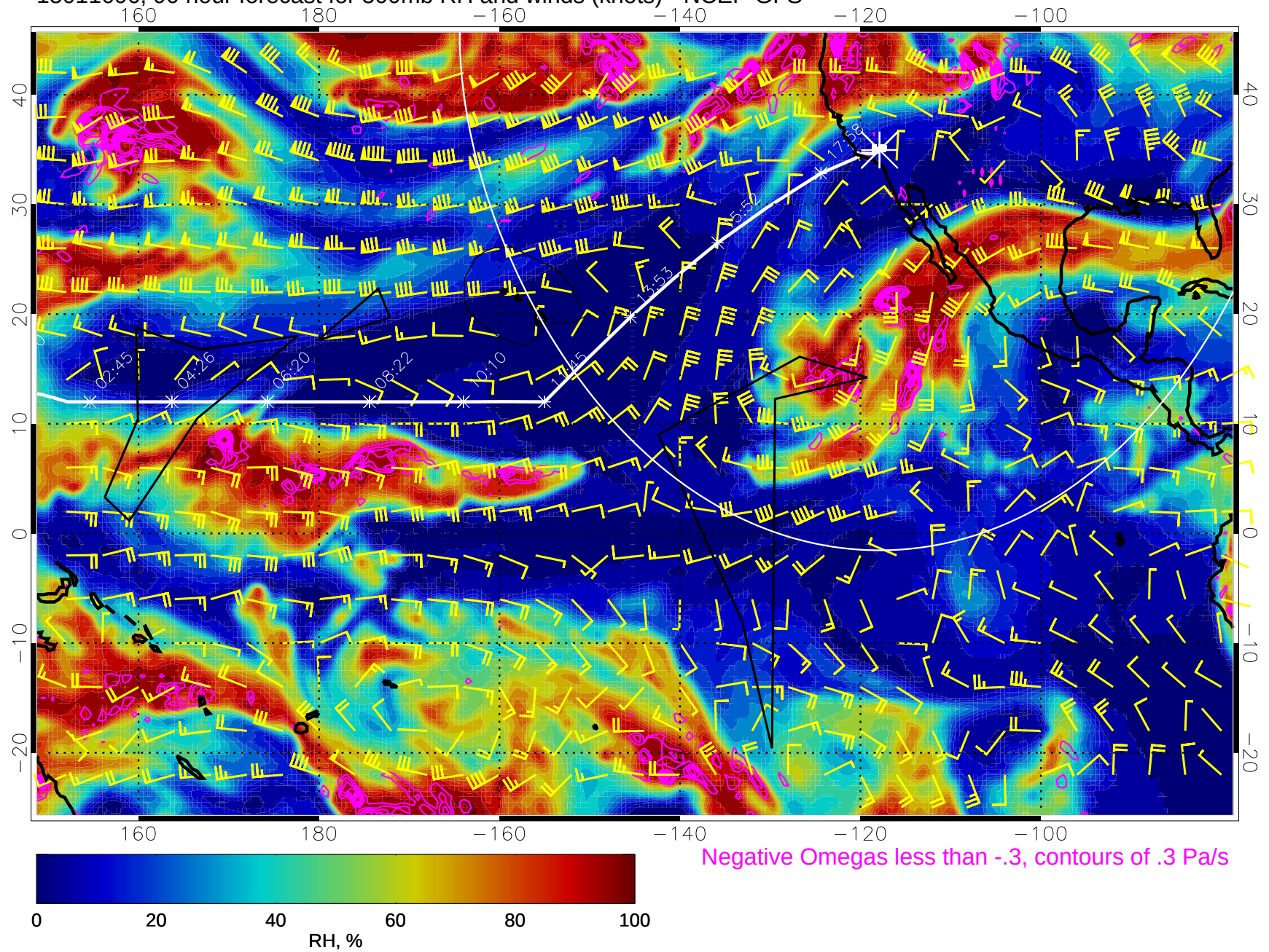
15011606, 90 hour forecast for 500mb RH and winds (knots) - NCEP GFS
