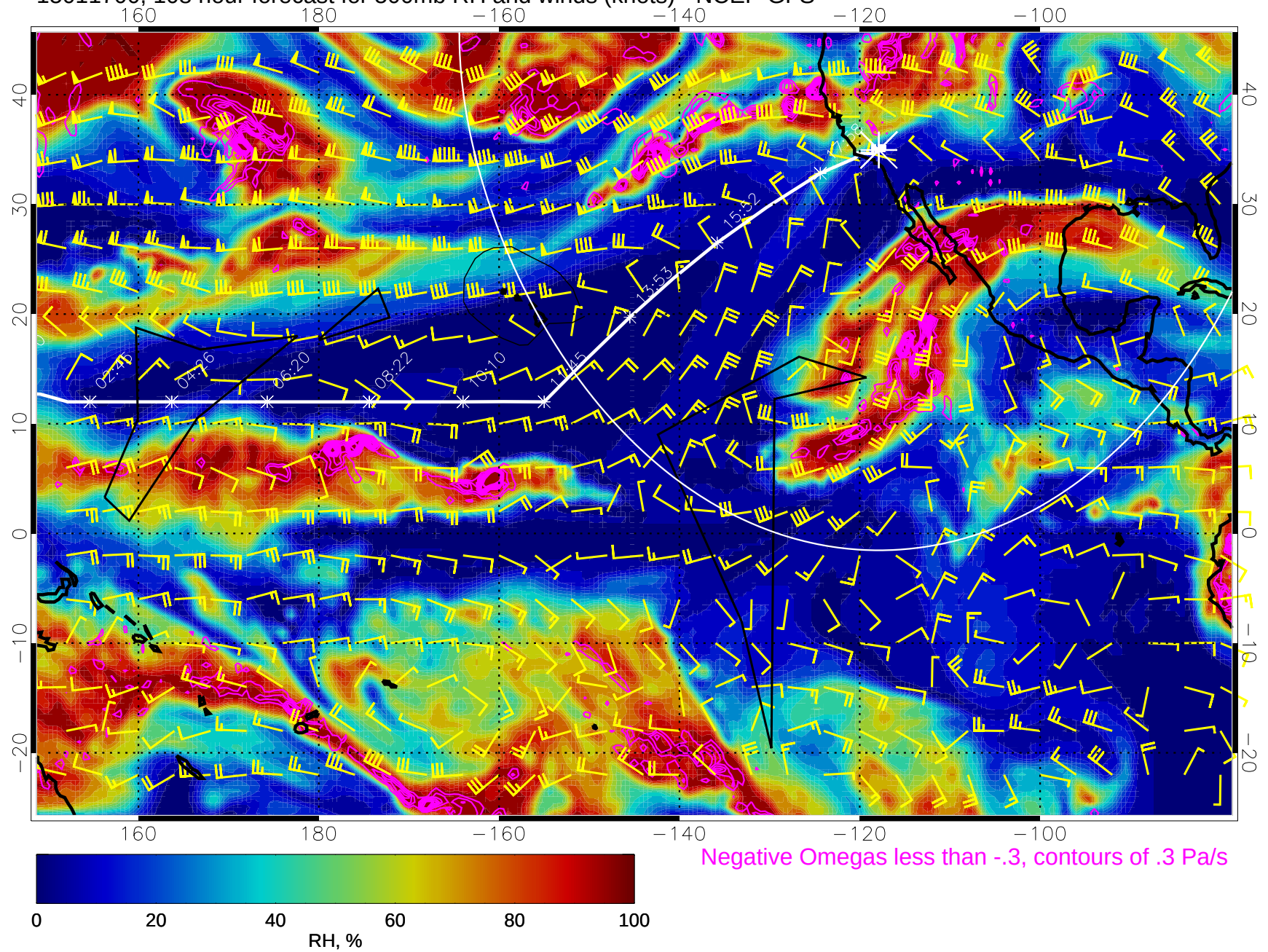
15011700, 108 hour forecast for 500mb RH and winds (knots) - NCEP GFS
