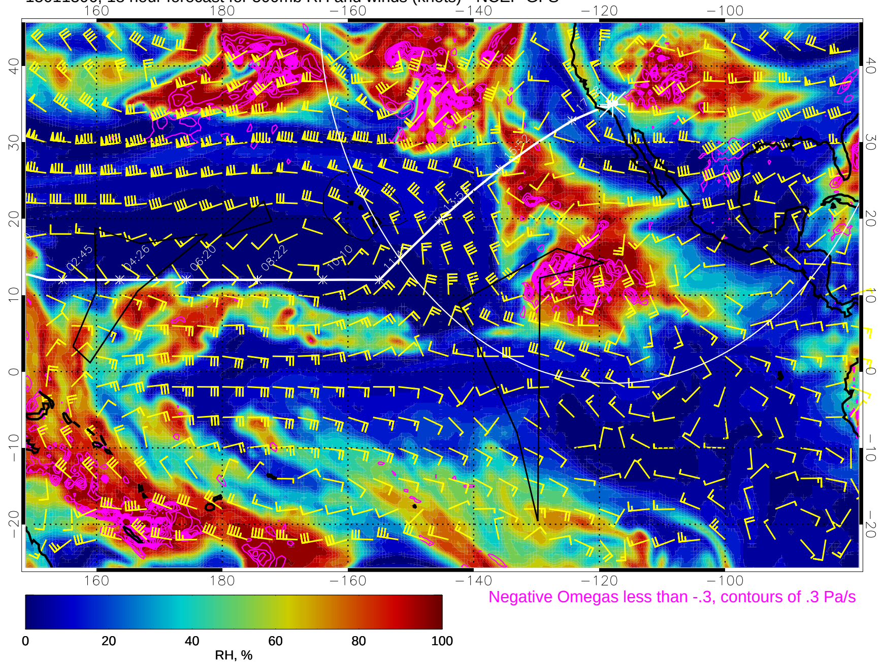
15011306, 18 hour forecast for 500mb RH and winds (knots) - NCEP GFS
