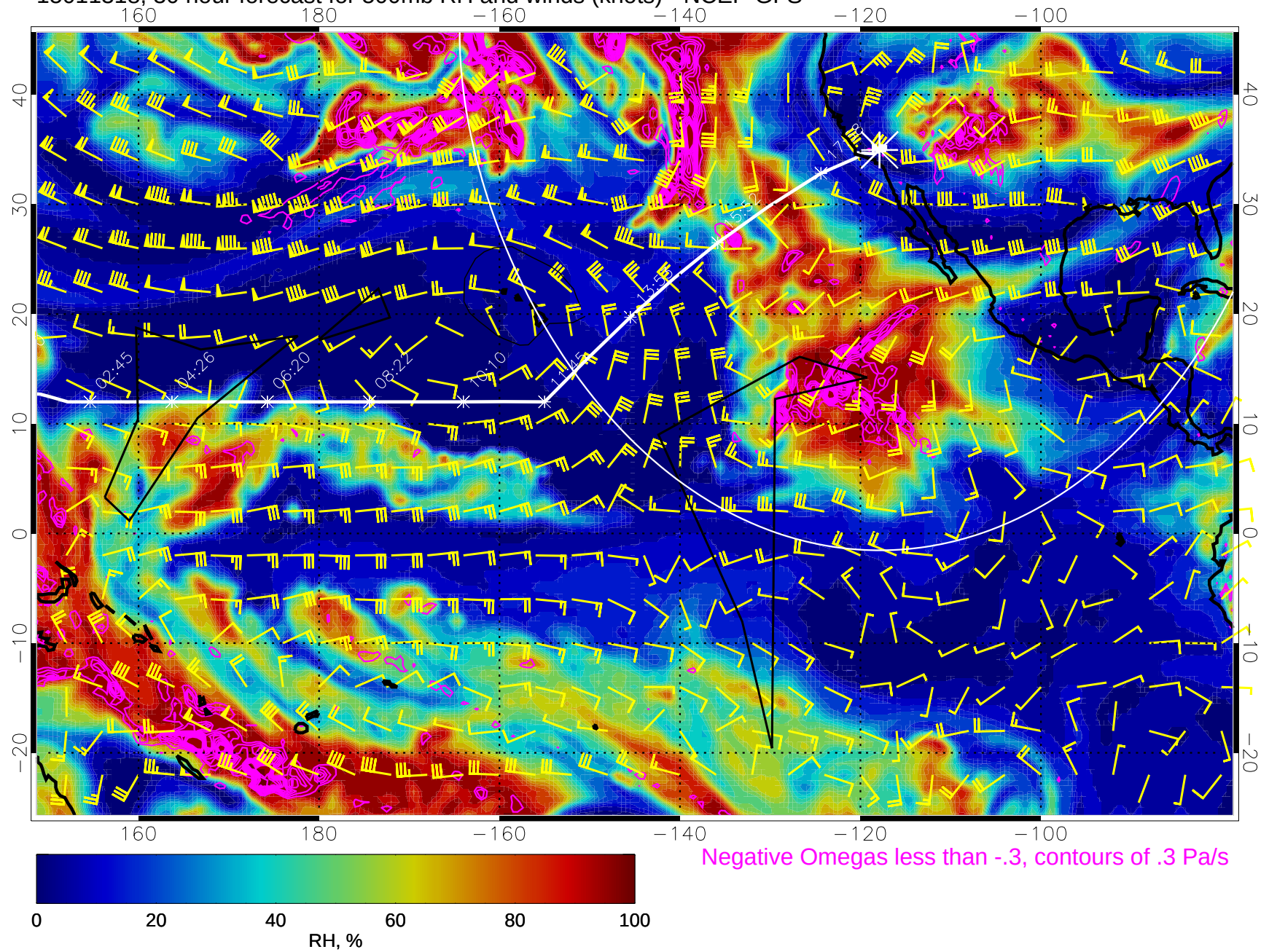
15011318, 30 hour forecast for 500mb RH and winds (knots) - NCEP GFS
