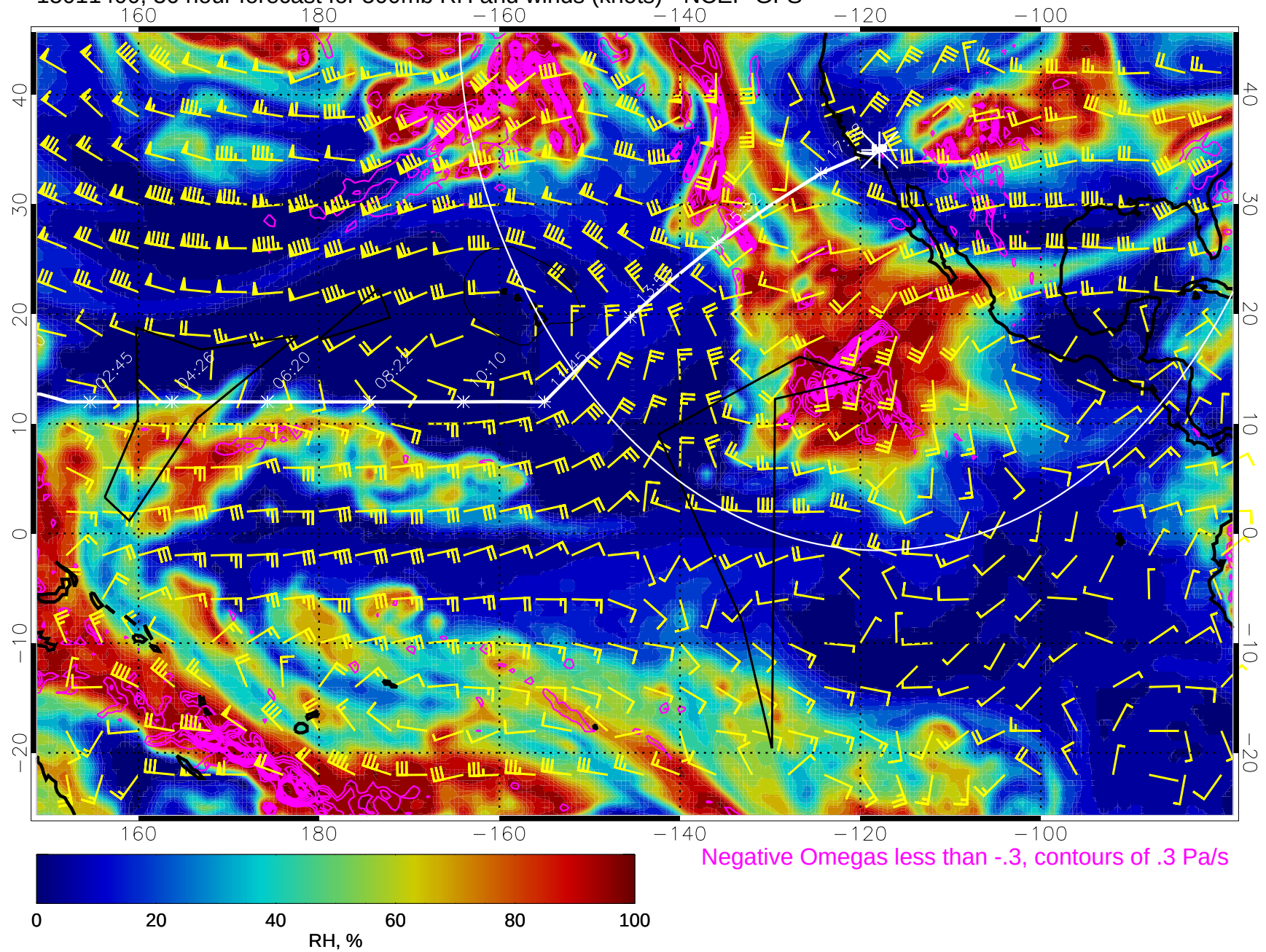
15011400, 36 hour forecast for 500mb RH and winds (knots) - NCEP GFS
