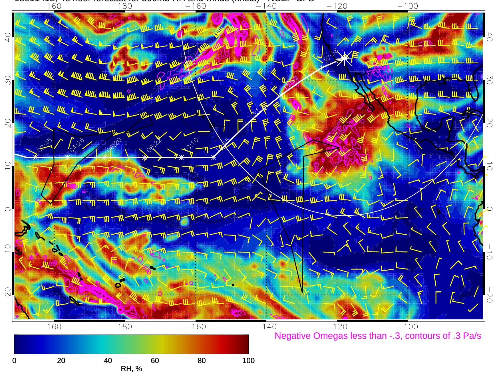
15011412, 48 hour forecast for 500mb RH and winds (knots) - NCEP GFS
