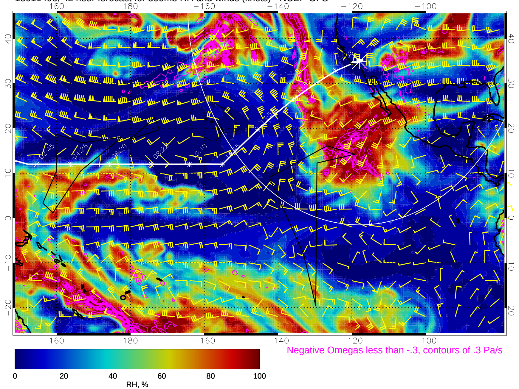
15011406, 42 hour forecast for 500mb RH and winds (knots) - NCEP GFS
