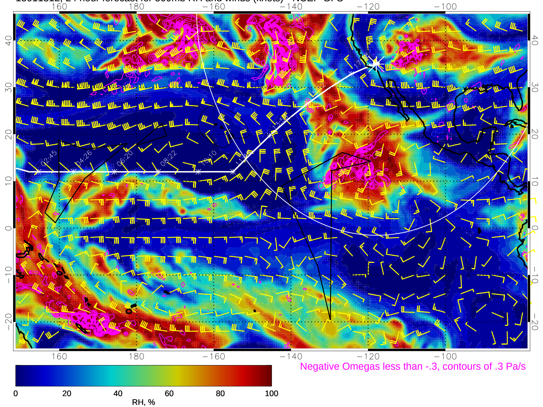
15011312, 24 hour forecast for 500mb RH and winds (knots) - NCEP GFS
