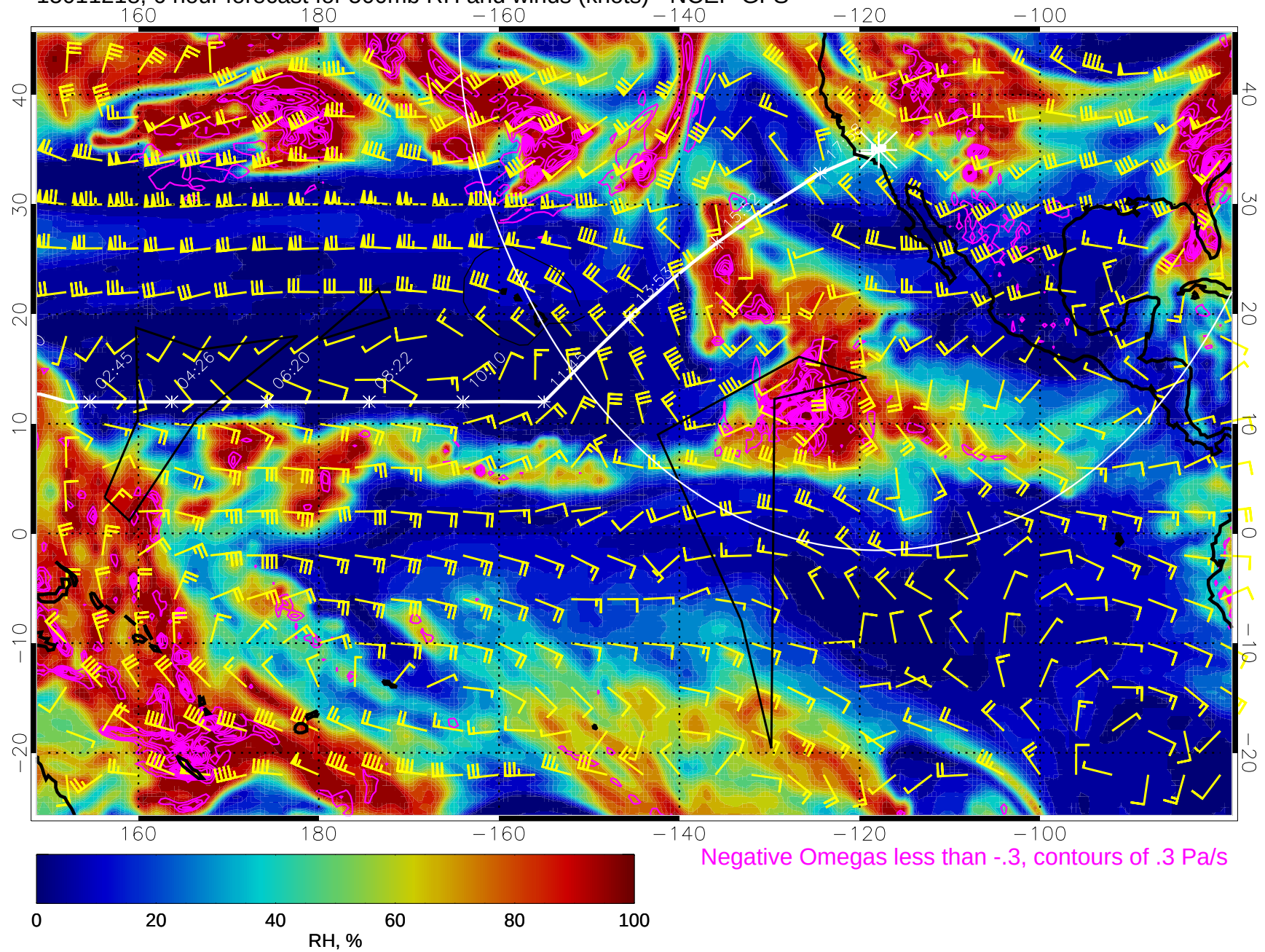
15011218, 6 hour forecast for 500mb RH and winds (knots) - NCEP GFS
