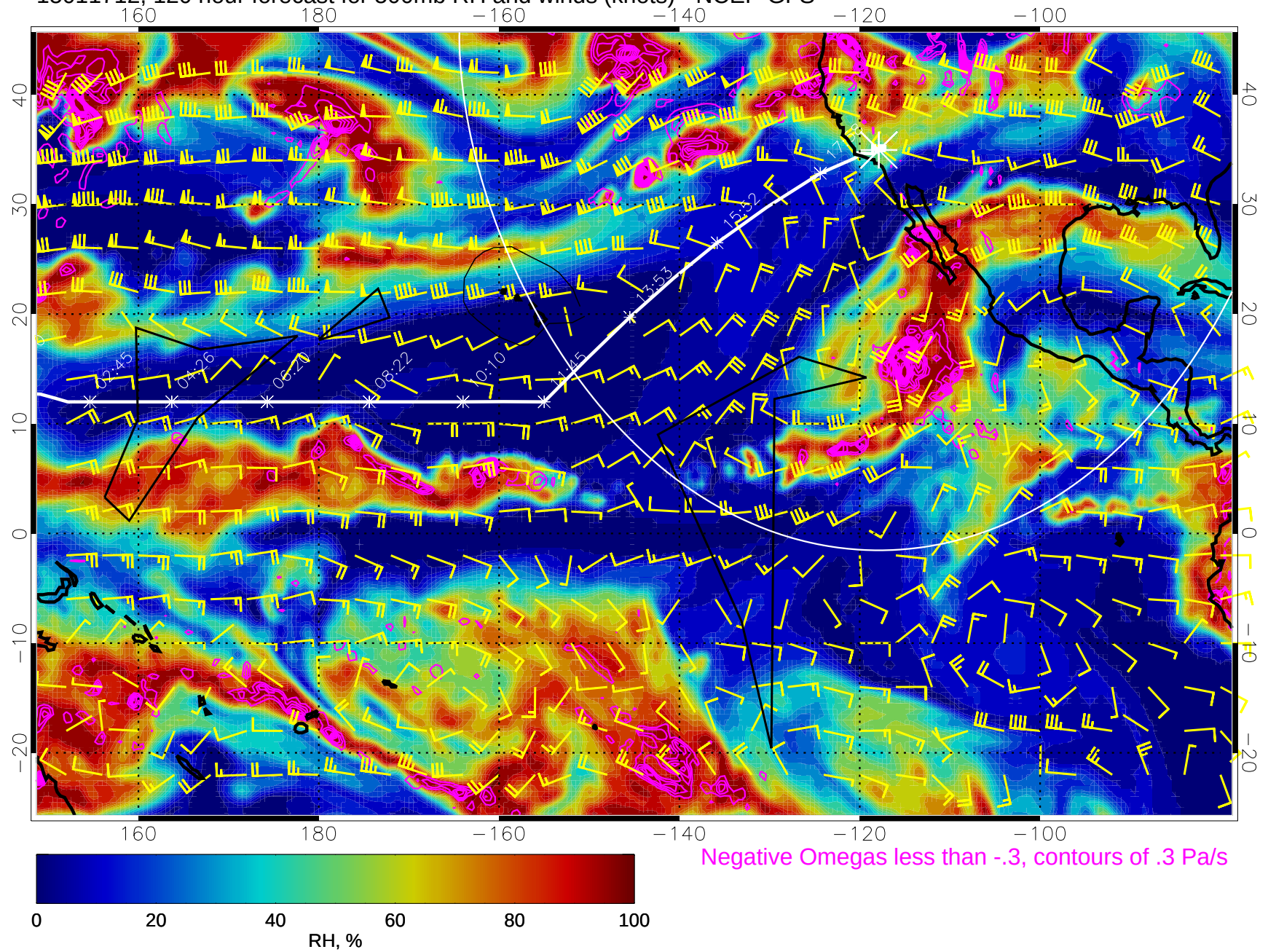
15011712, 120 hour forecast for 500mb RH and winds (knots) - NCEP GFS
