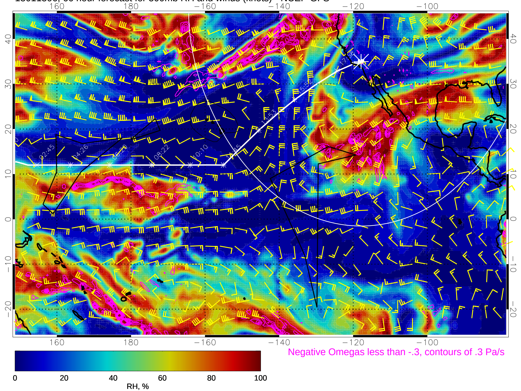
15011506, 66 hour forecast for 500mb RH and winds (knots) - NCEP GFS
