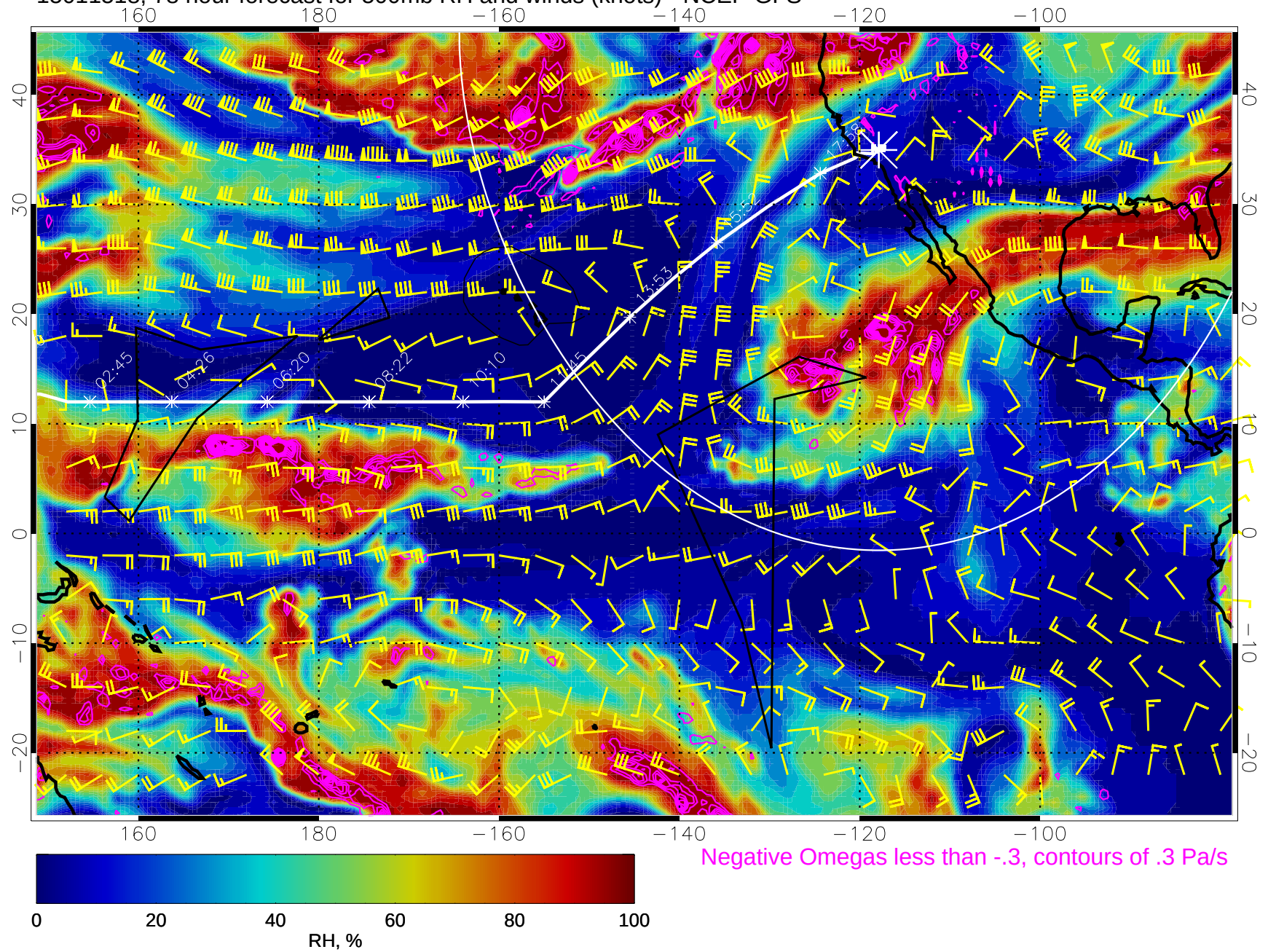
15011518, 78 hour forecast for 500mb RH and winds (knots) - NCEP GFS
