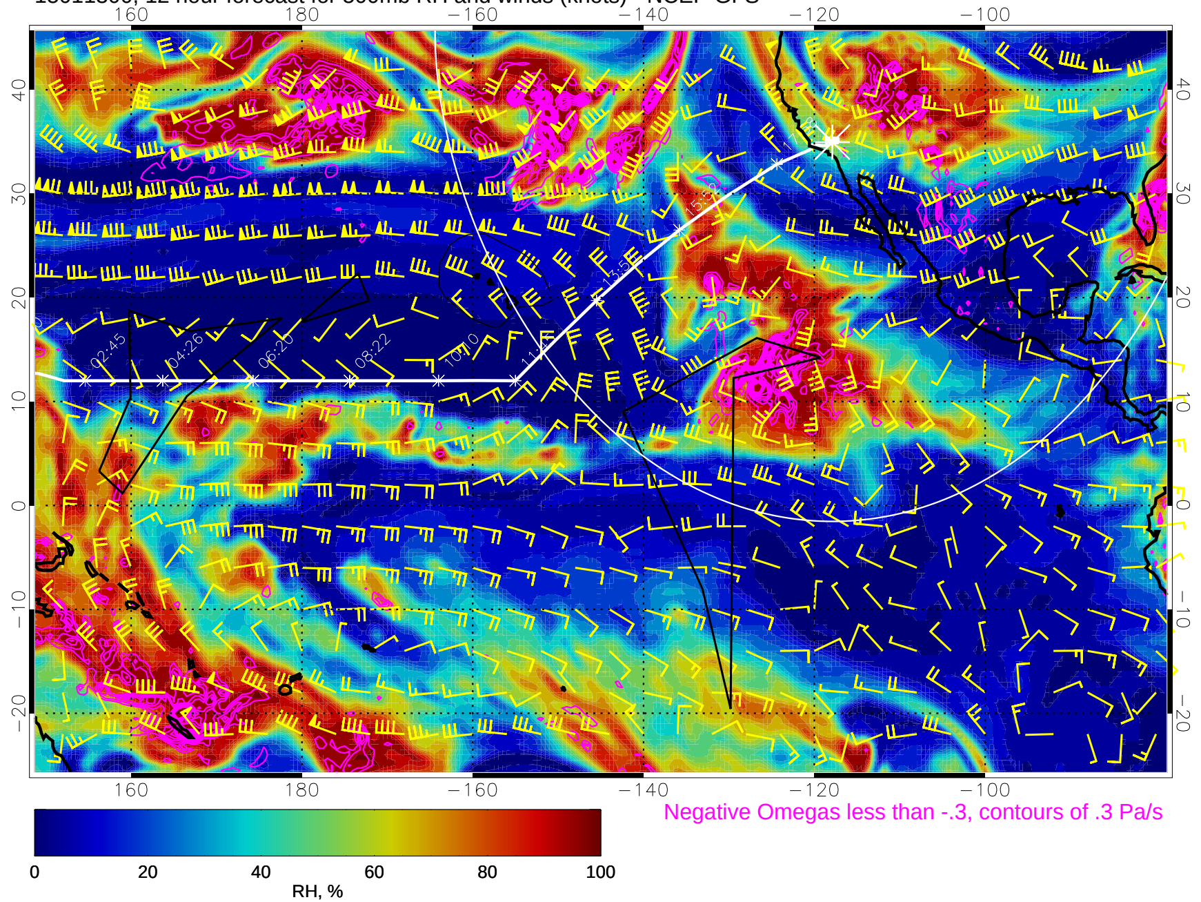
15011300, 12 hour forecast for 500mb RH and winds (knots) - NCEP GFS
