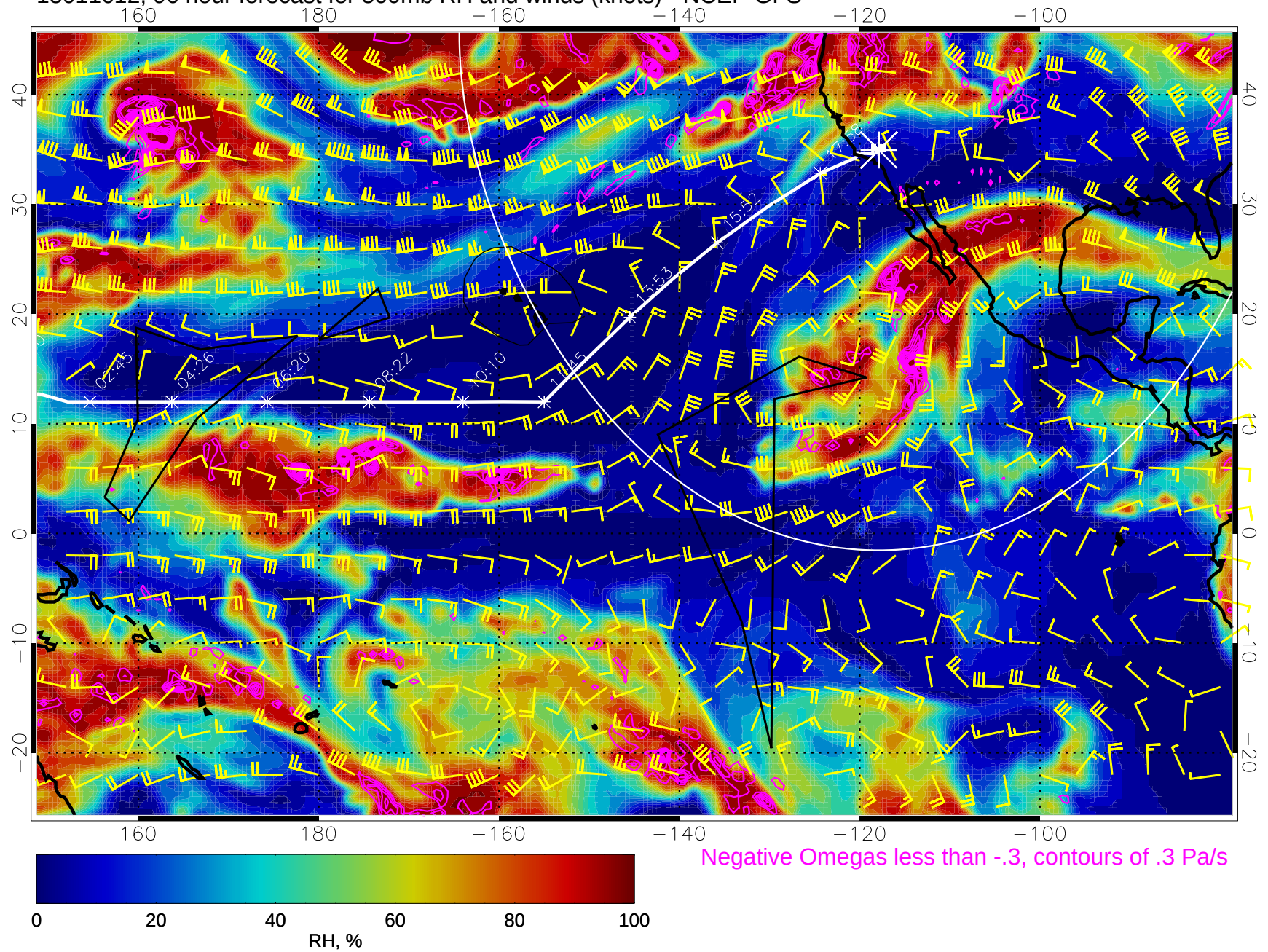
15011612, 96 hour forecast for 500mb RH and winds (knots) - NCEP GFS
