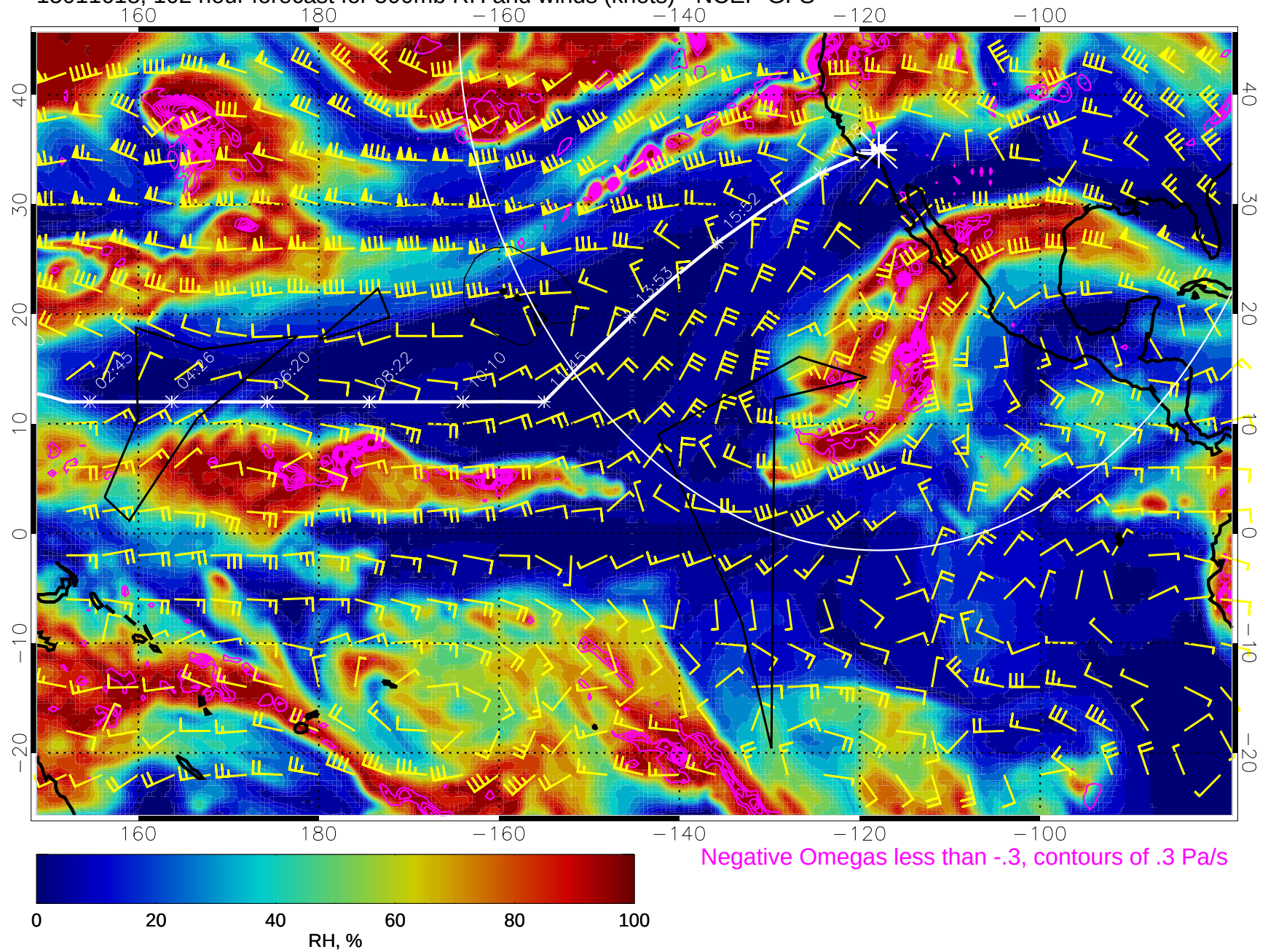
15011618, 102 hour forecast for 500mb RH and winds (knots) - NCEP GFS
