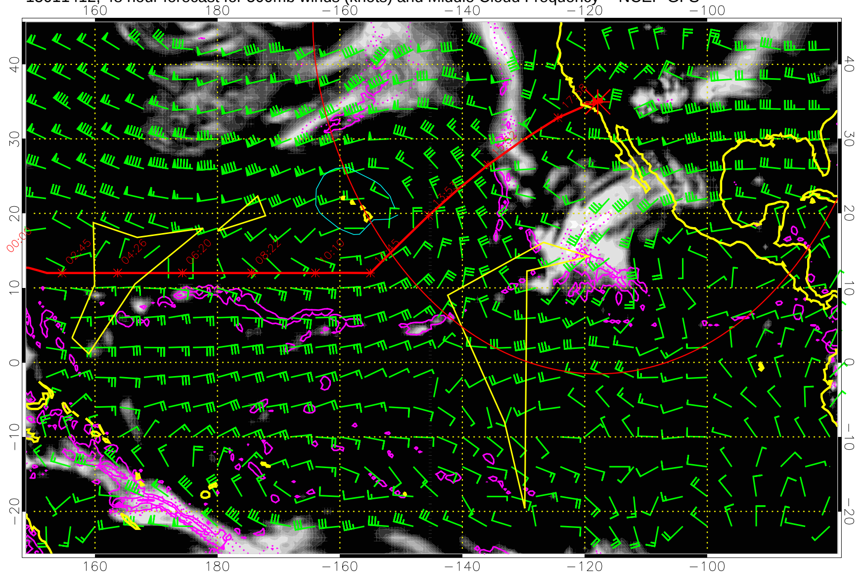
15011412, 48 hour forecast for 500mb winds (knots) and Middle Cloud Frequency -- NCEP GFS
