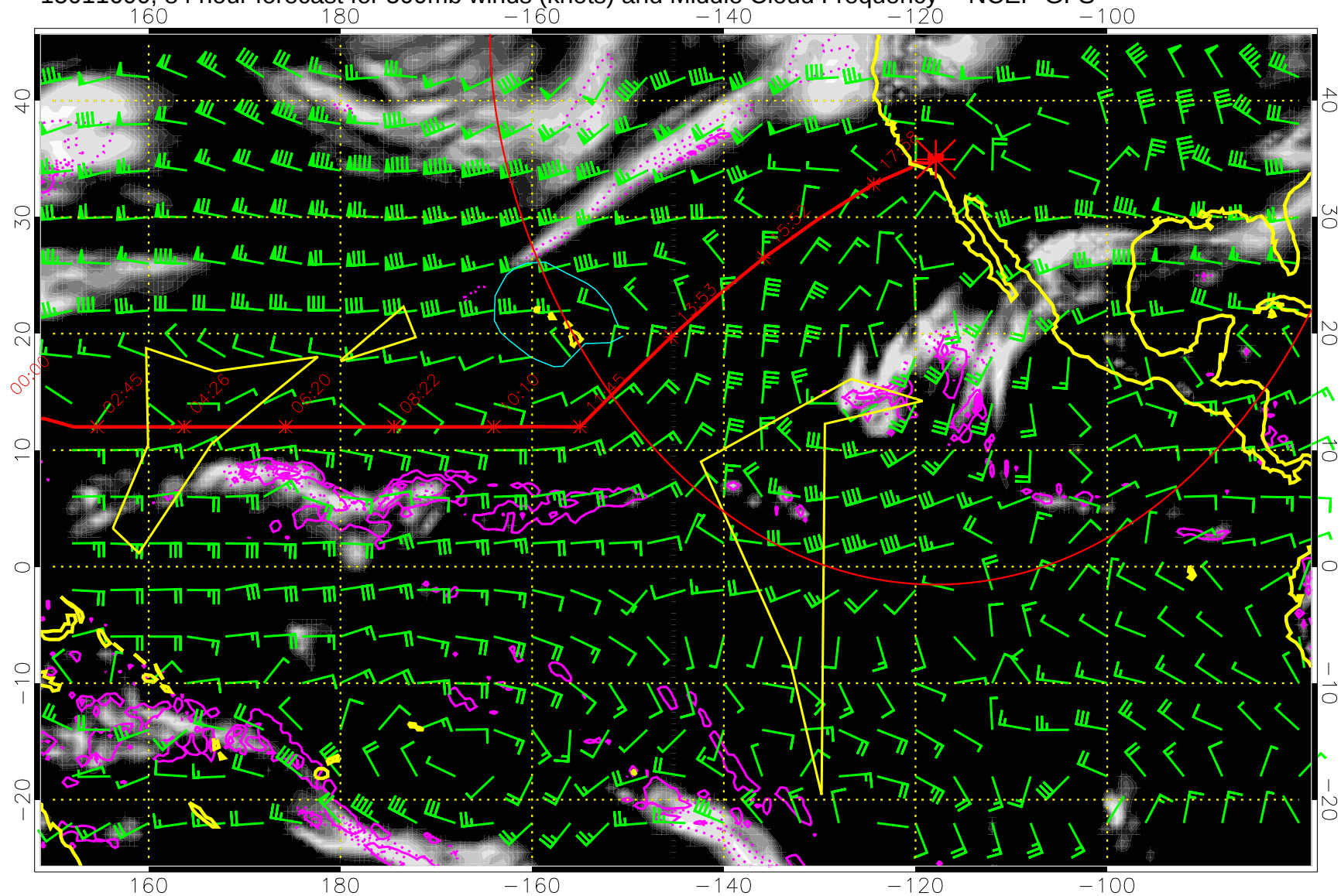
15011600, 84 hour forecast for 500mb winds (knots) and Middle Cloud Frequency -- NCEP GFS
