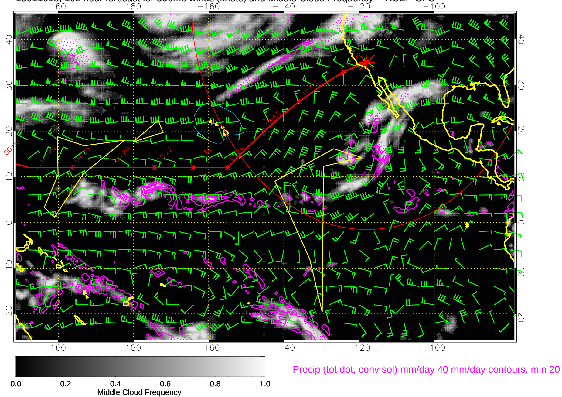
15011618, 102 hour forecast for 500mb winds (knots) and Middle Cloud Frequency -- NCEP GFS
