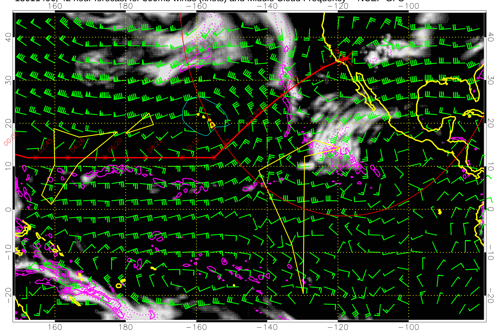
15011406, 42 hour forecast for 500mb winds (knots) and Middle Cloud Frequency -- NCEP GFS
