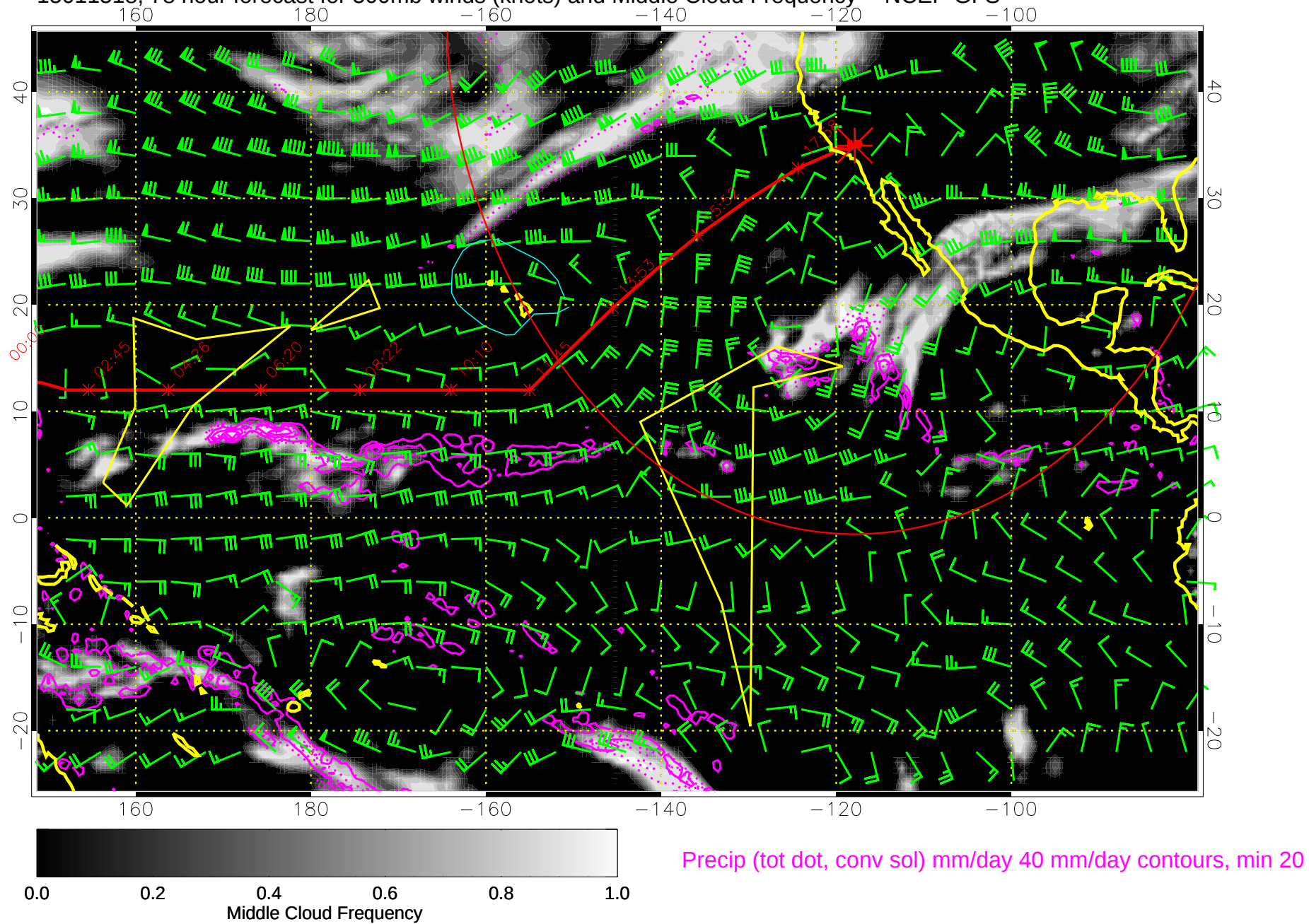
15011518, 78 hour forecast for 500mb winds (knots) and Middle Cloud Frequency -- NCEP GFS
