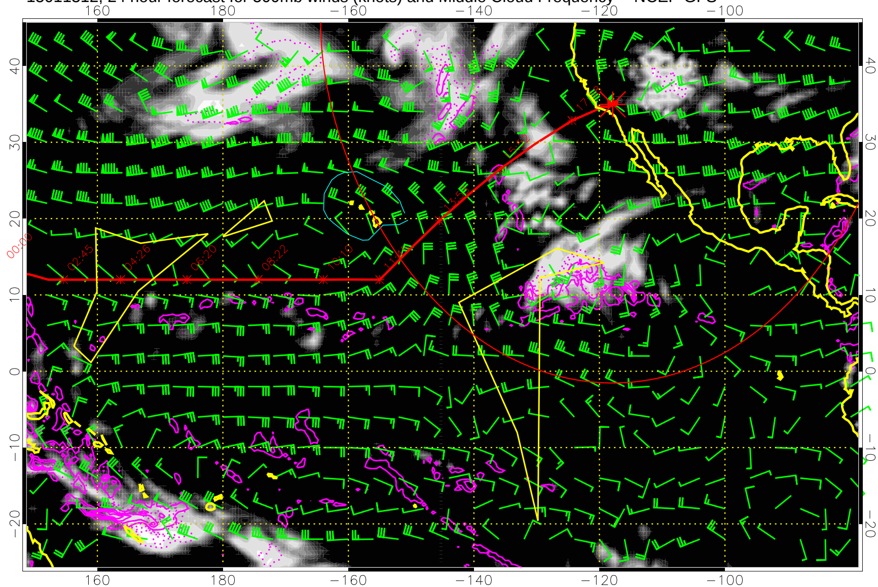
15011312, 24 hour forecast for 500mb winds (knots) and Middle Cloud Frequency -- NCEP GFS
