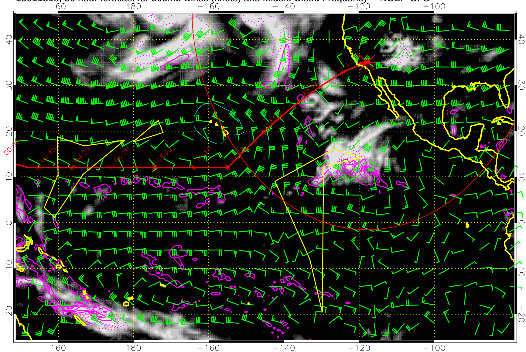
15011318, 30 hour forecast for 500mb winds (knots) and Middle Cloud Frequency -- NCEP GFS
