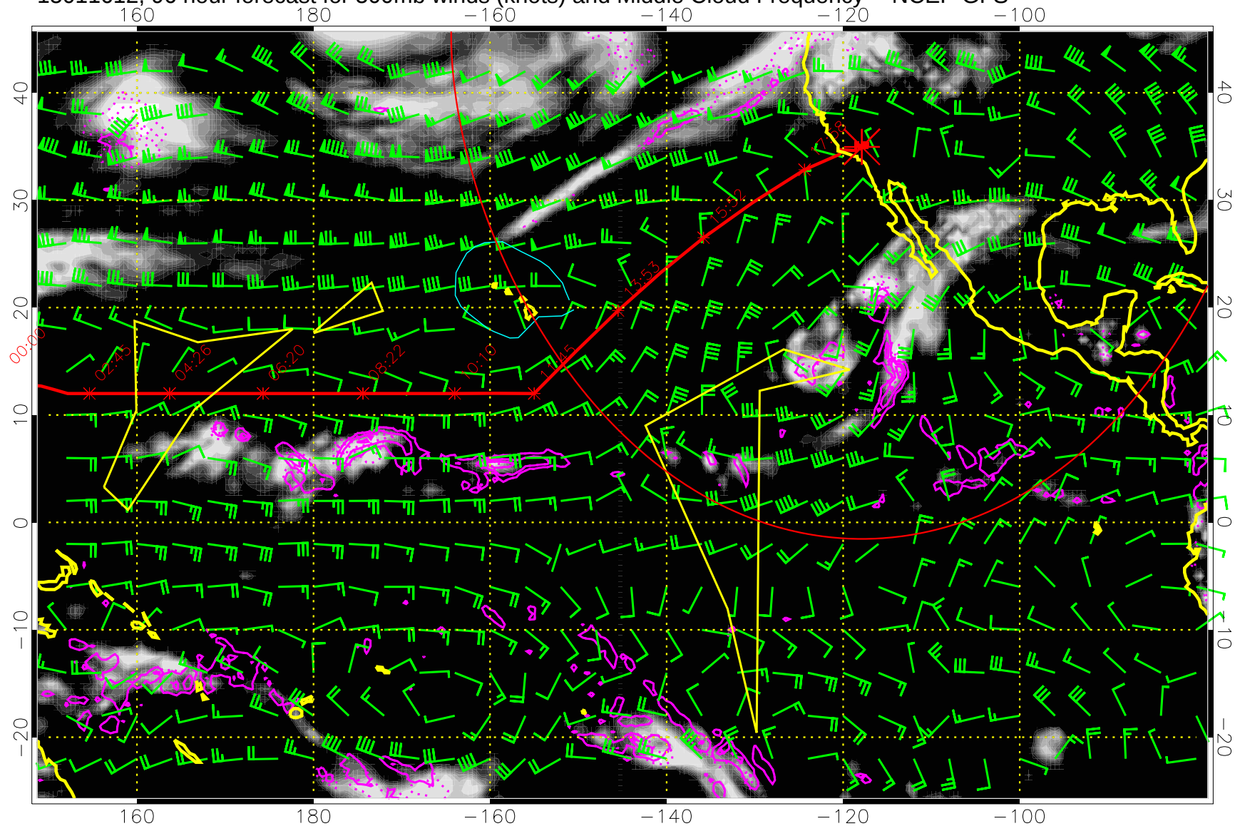
15011612, 96 hour forecast for 500mb winds (knots) and Middle Cloud Frequency -- NCEP GFS
