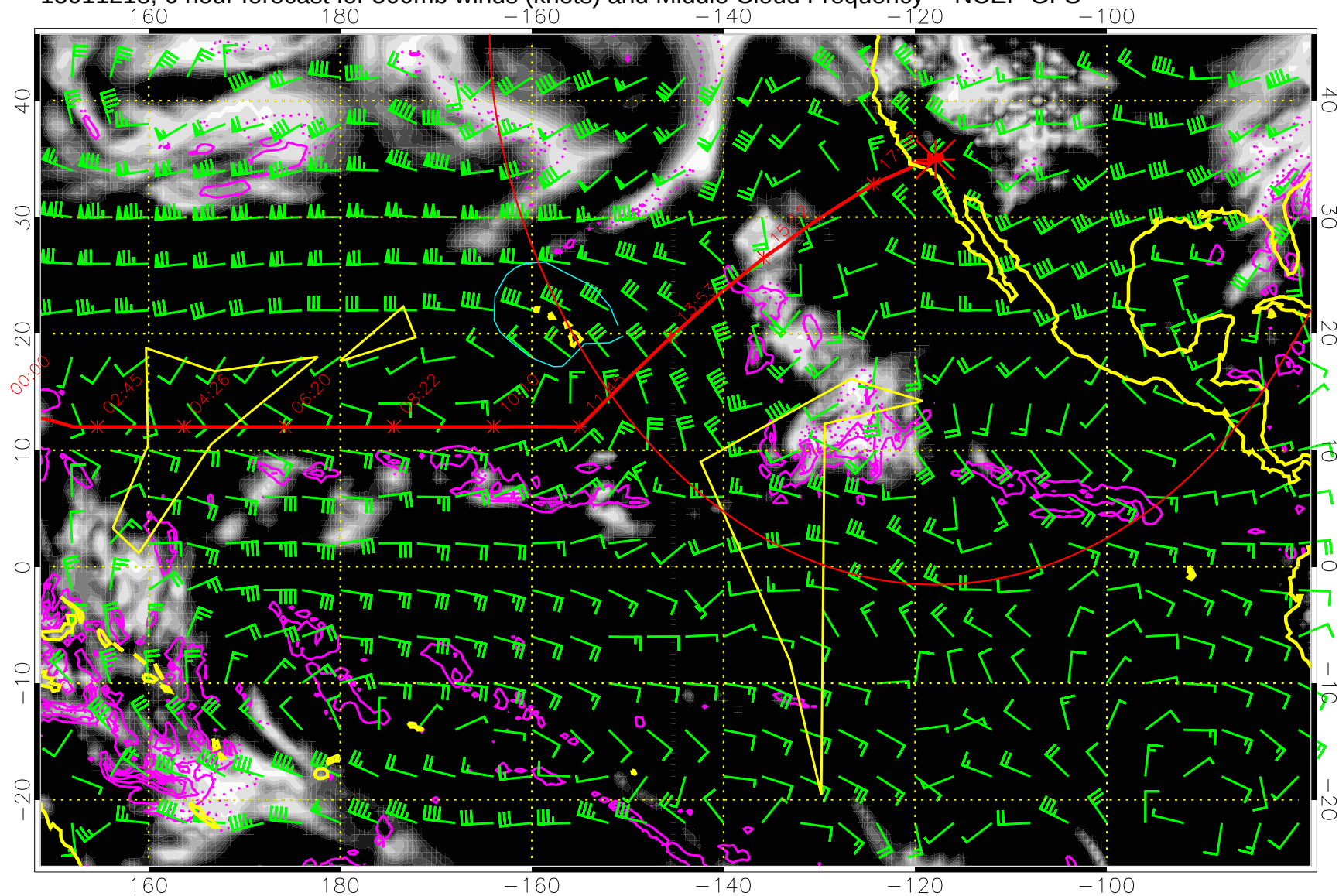
15011218, 6 hour forecast for 500mb winds (knots) and Middle Cloud Frequency -- NCEP GFS
