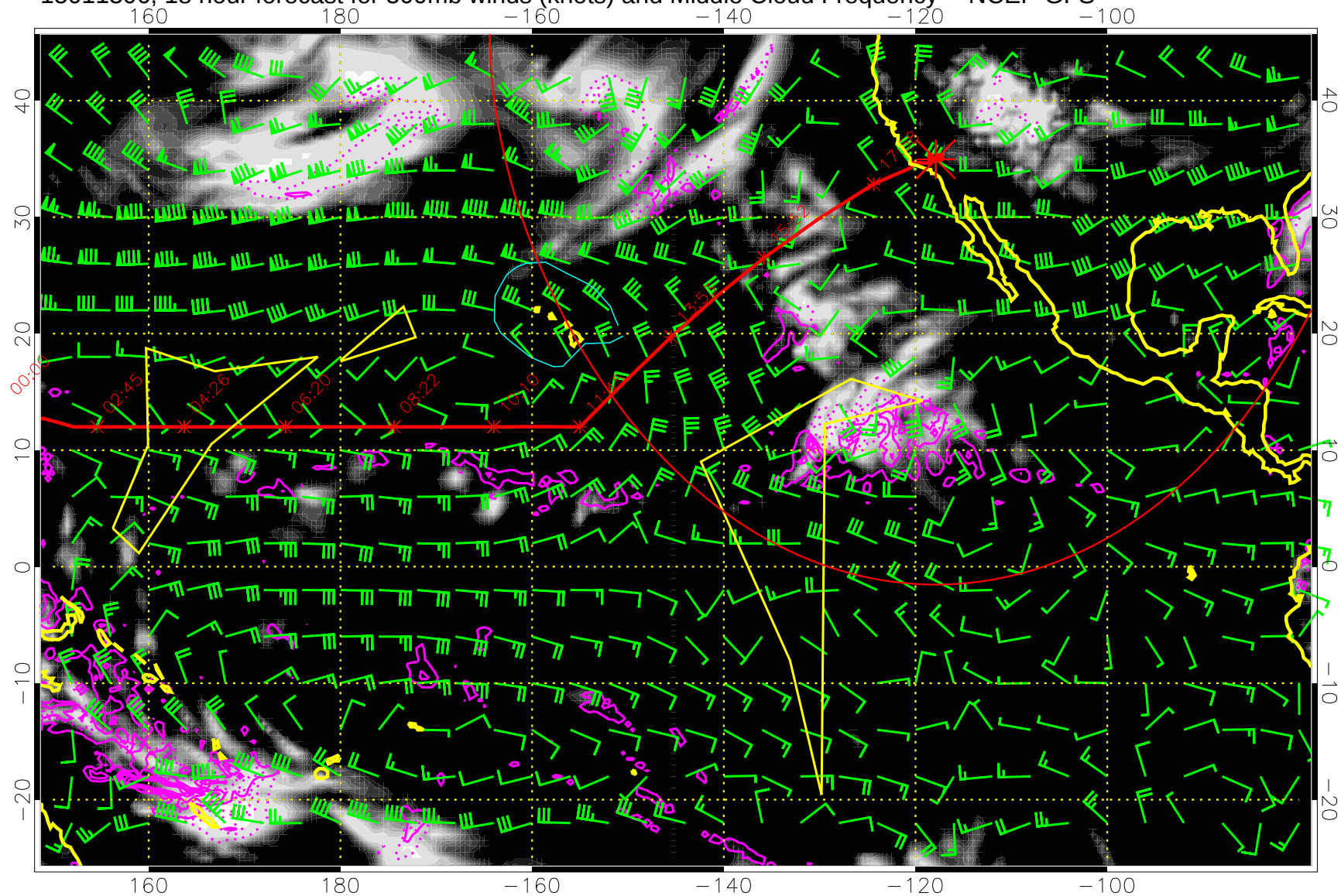
15011306, 18 hour forecast for 500mb winds (knots) and Middle Cloud Frequency -- NCEP GFS
