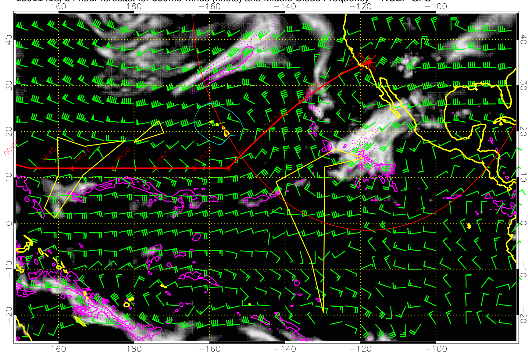
15011418, 54 hour forecast for 500mb winds (knots) and Middle Cloud Frequency -- NCEP GFS
