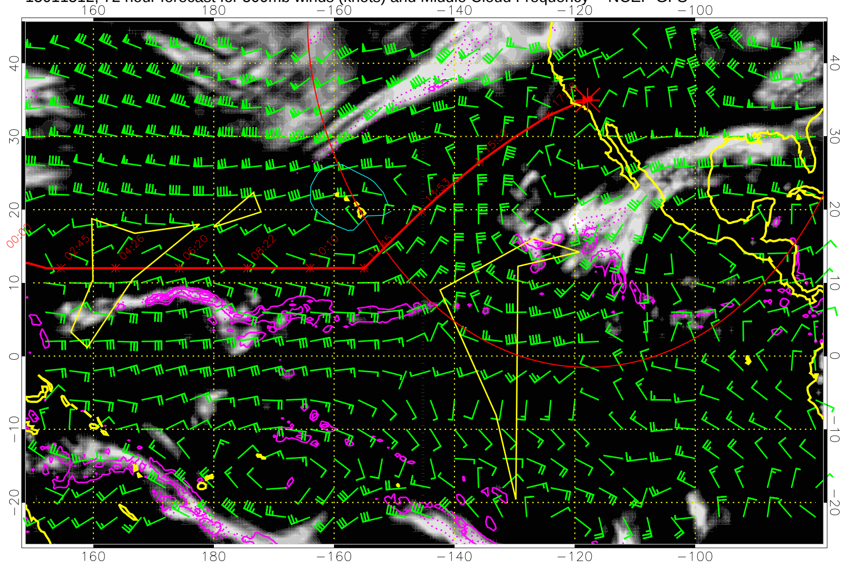
15011512, 72 hour forecast for 500mb winds (knots) and Middle Cloud Frequency -- NCEP GFS
