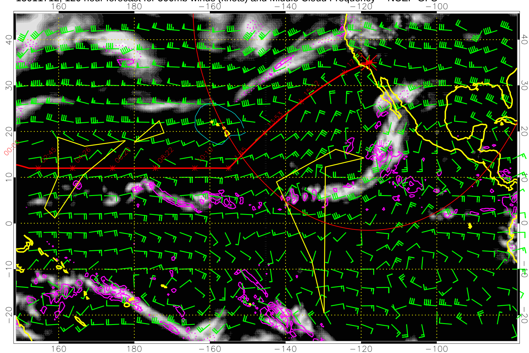
15011712, 120 hour forecast for 500mb winds (knots) and Middle Cloud Frequency -- NCEP GFS
