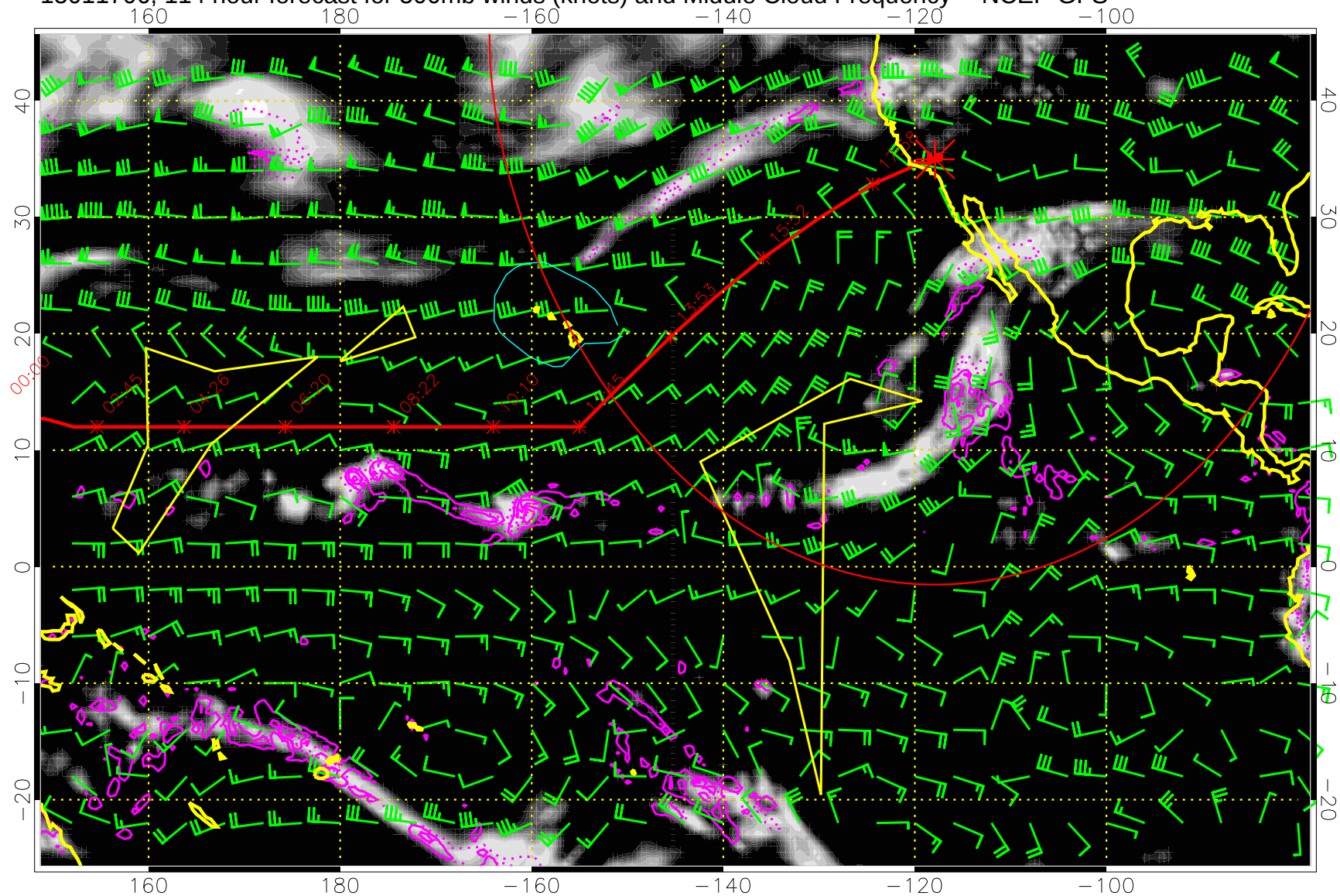
15011706, 114 hour forecast for 500mb winds (knots) and Middle Cloud Frequency -- NCEP GFS
