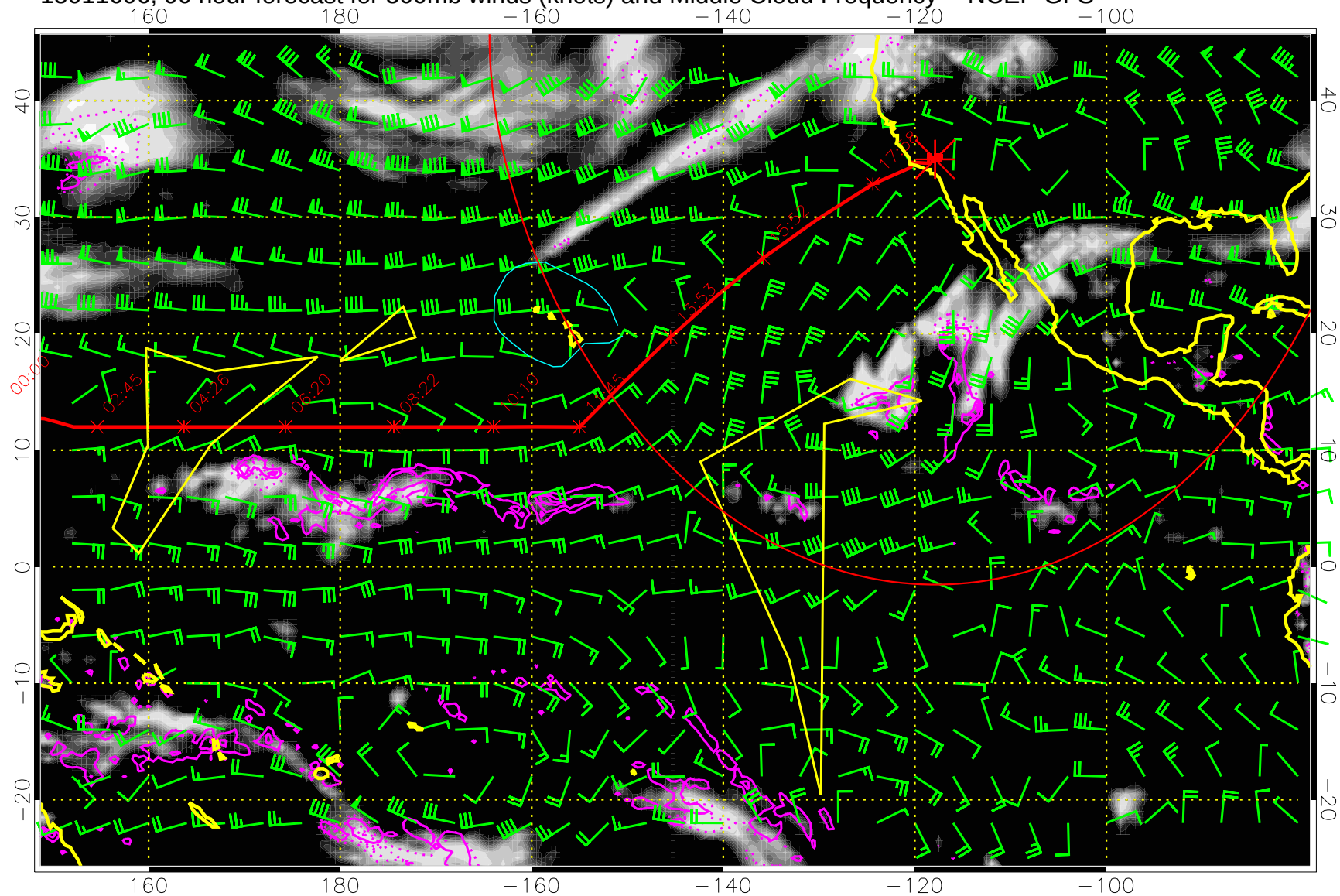
15011606, 90 hour forecast for 500mb winds (knots) and Middle Cloud Frequency -- NCEP GFS
