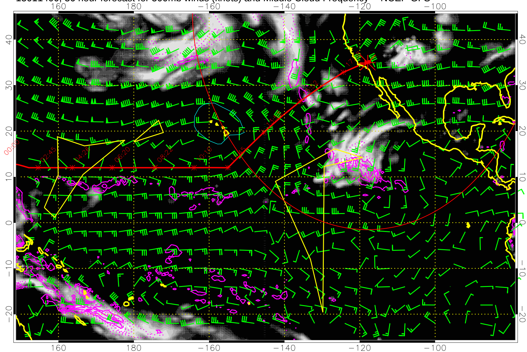
15011400, 36 hour forecast for 500mb winds (knots) and Middle Cloud Frequency -- NCEP GFS
