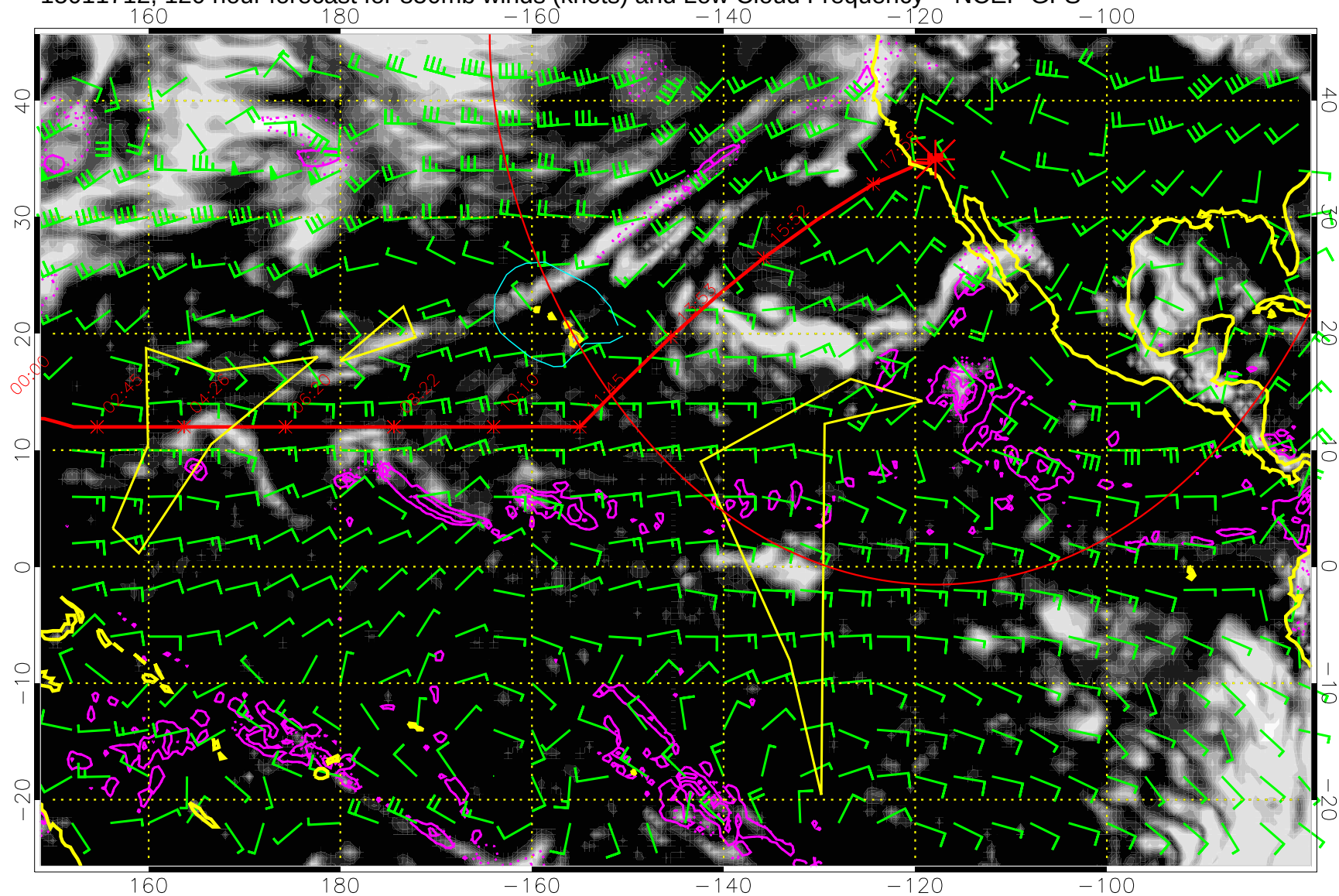
15011712, 120 hour forecast for 850mb winds (knots) and Low Cloud Frequency -- NCEP GFS
