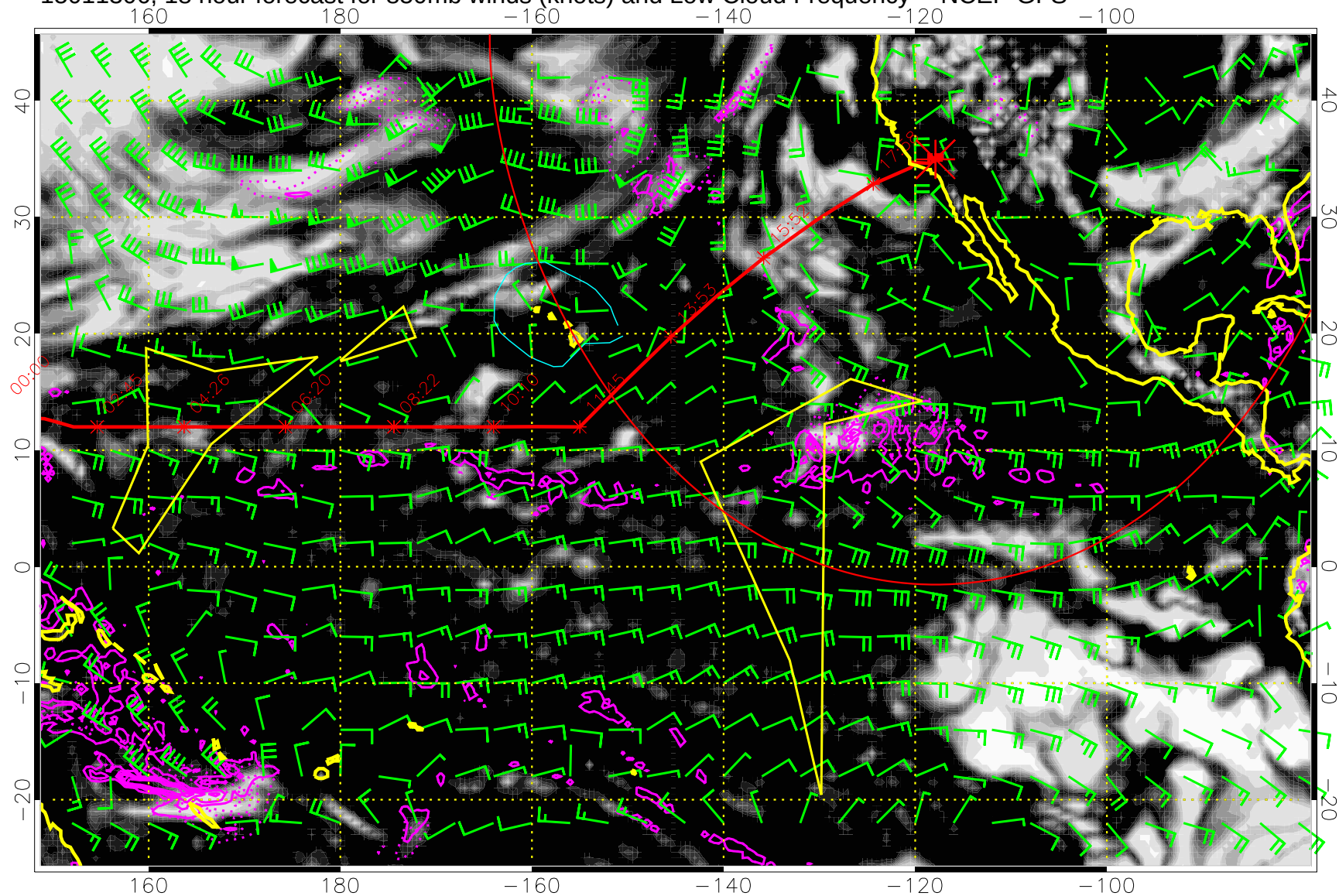
15011306, 18 hour forecast for 850mb winds (knots) and Low Cloud Frequency -- NCEP GFS
