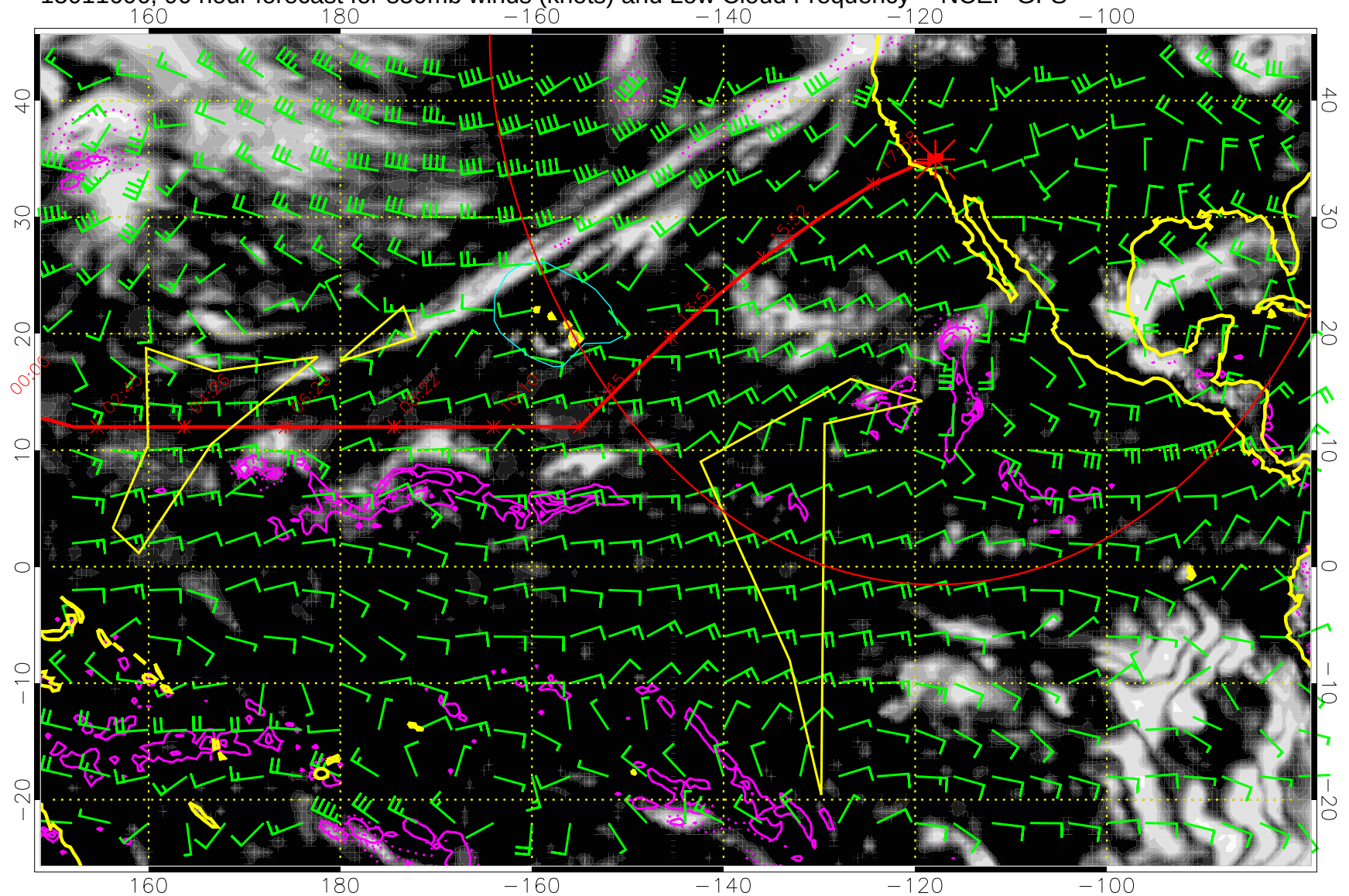
15011606, 90 hour forecast for 850mb winds (knots) and Low Cloud Frequency -- NCEP GFS
