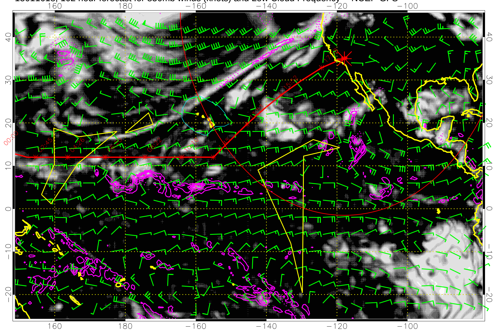
15011618, 102 hour forecast for 850mb winds (knots) and Low Cloud Frequency -- NCEP GFS
