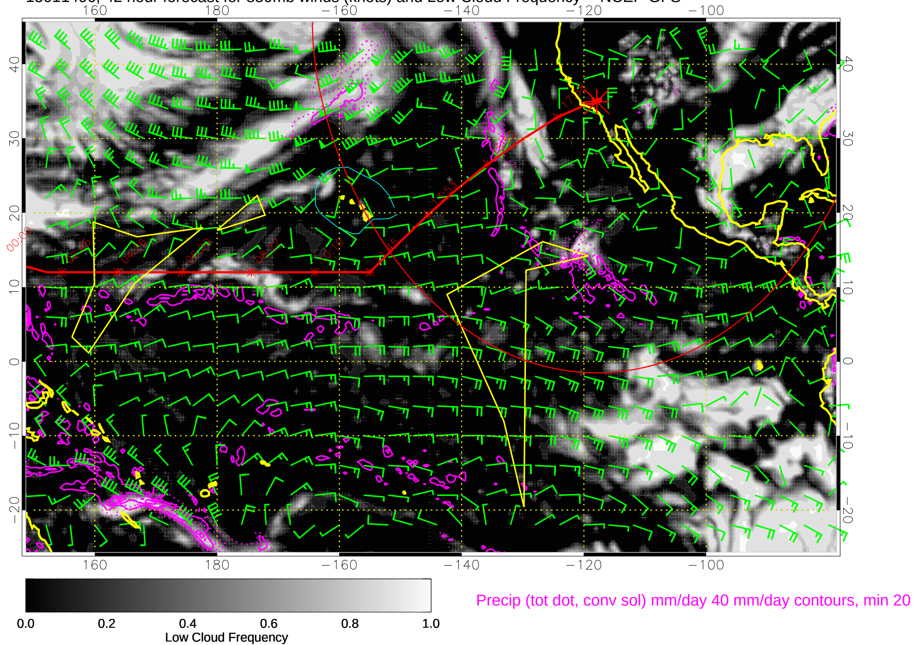
15011406, 42 hour forecast for 850mb winds (knots) and Low Cloud Frequency -- NCEP GFS
