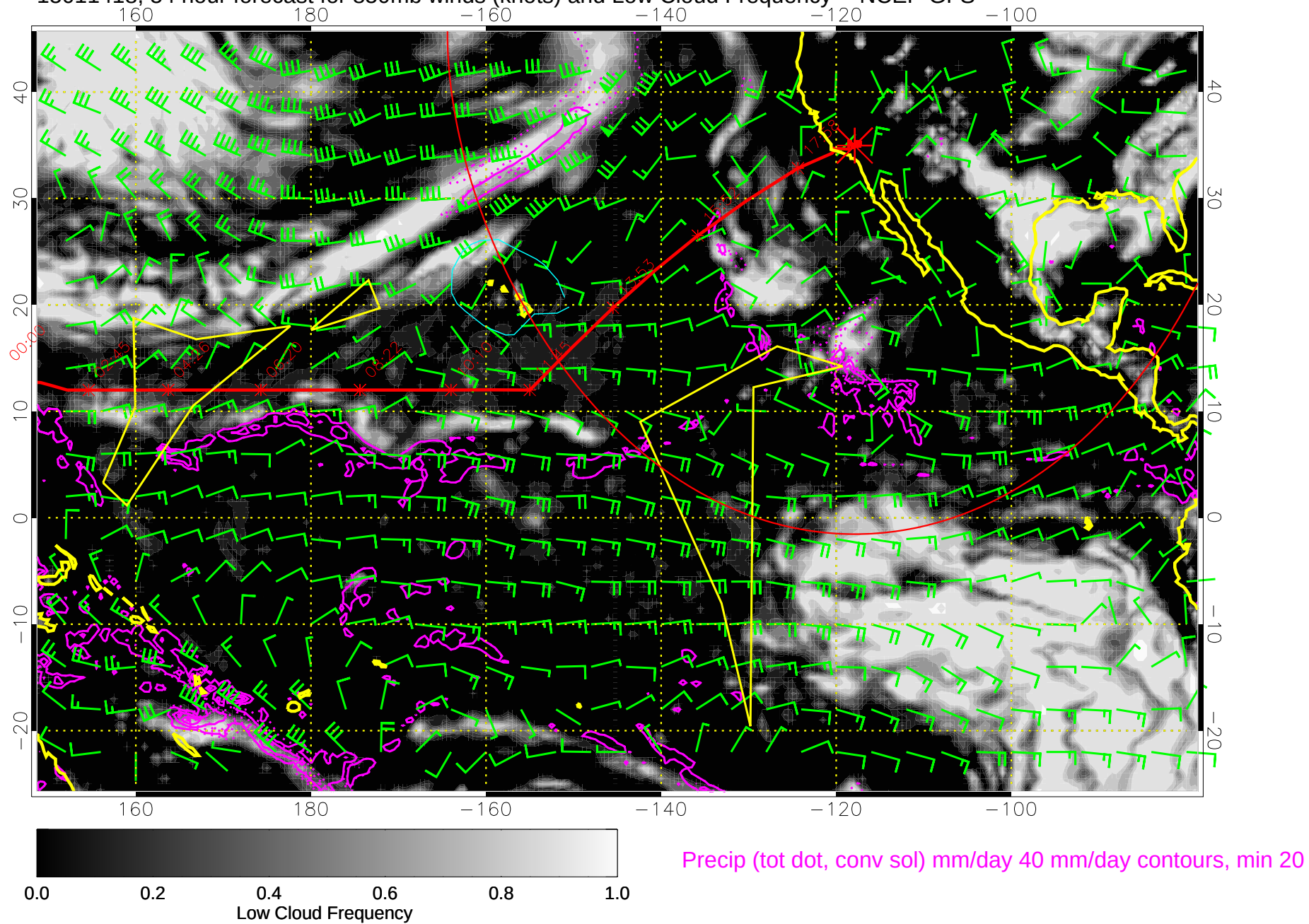
15011418, 54 hour forecast for 850mb winds (knots) and Low Cloud Frequency -- NCEP GFS
