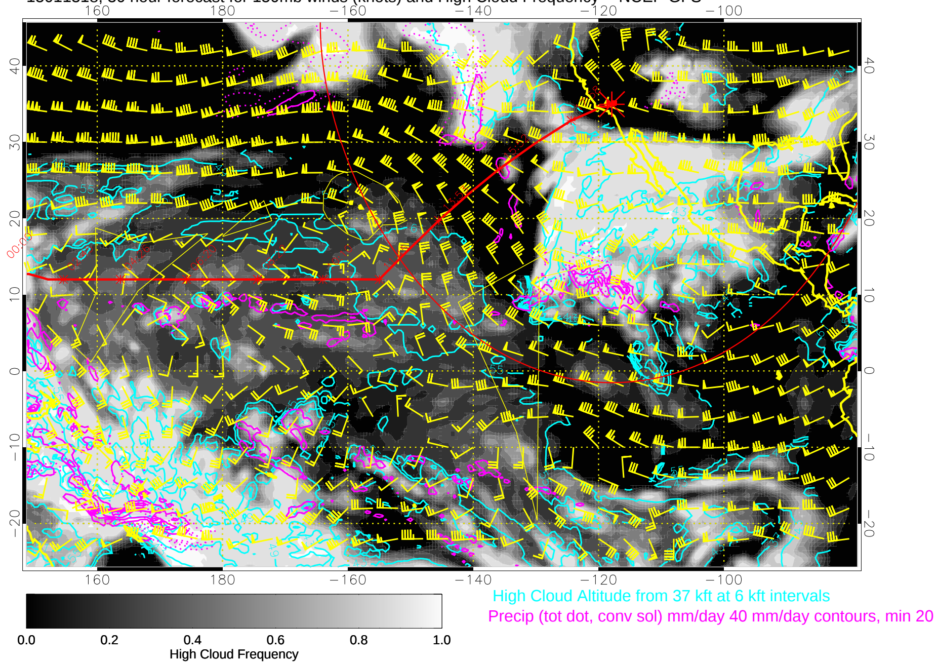
15011318, 30 hour forecast for 150mb winds (knots) and High Cloud Frequency -- NCEP GFS
