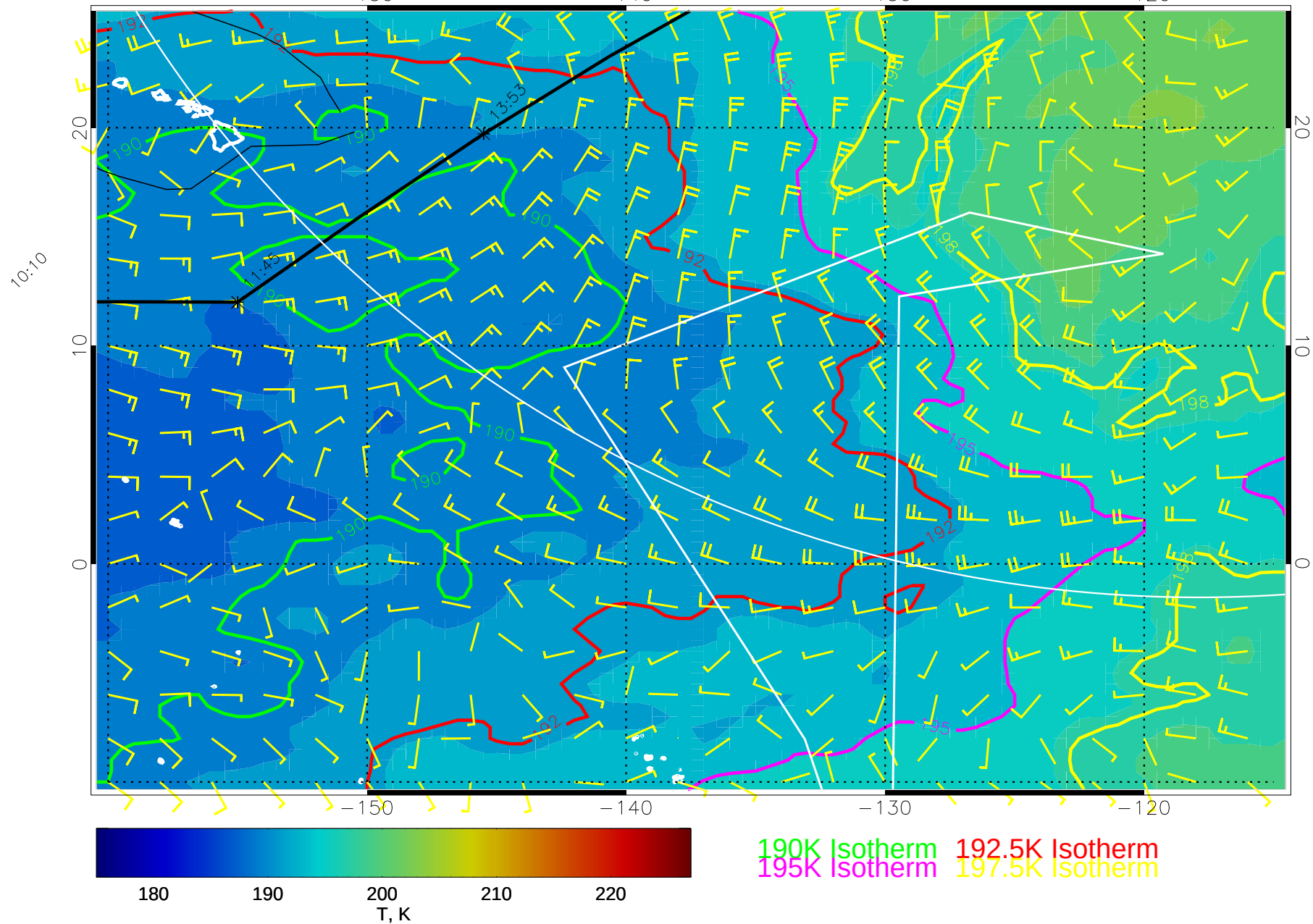
15011612, 108 hour forecast for 70mb T and winds (knots) -- NCEP GFS
