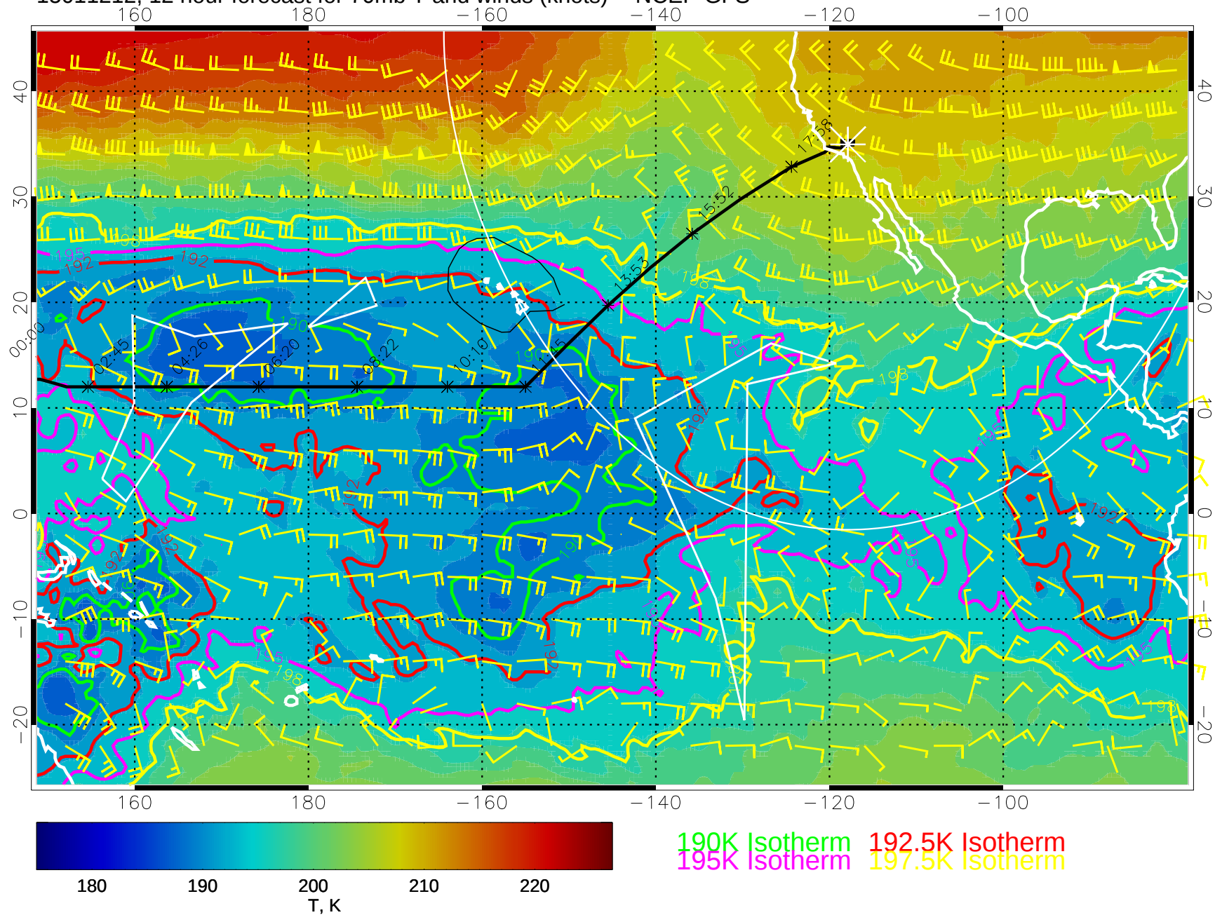
15011212, 12 hour forecast for 70mb T and winds (knots) -- NCEP GFS
