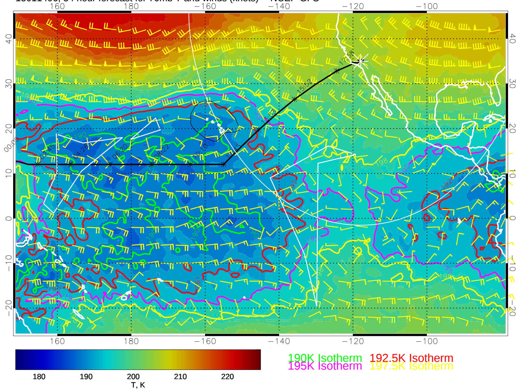
15011406, 54 hour forecast for 70mb T and winds (knots) -- NCEP GFS
