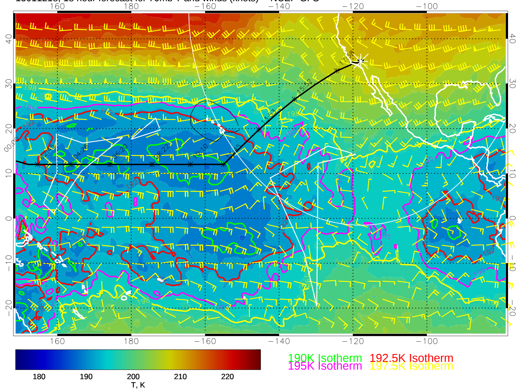
15011218, 18 hour forecast for 70mb T and winds (knots) -- NCEP GFS
