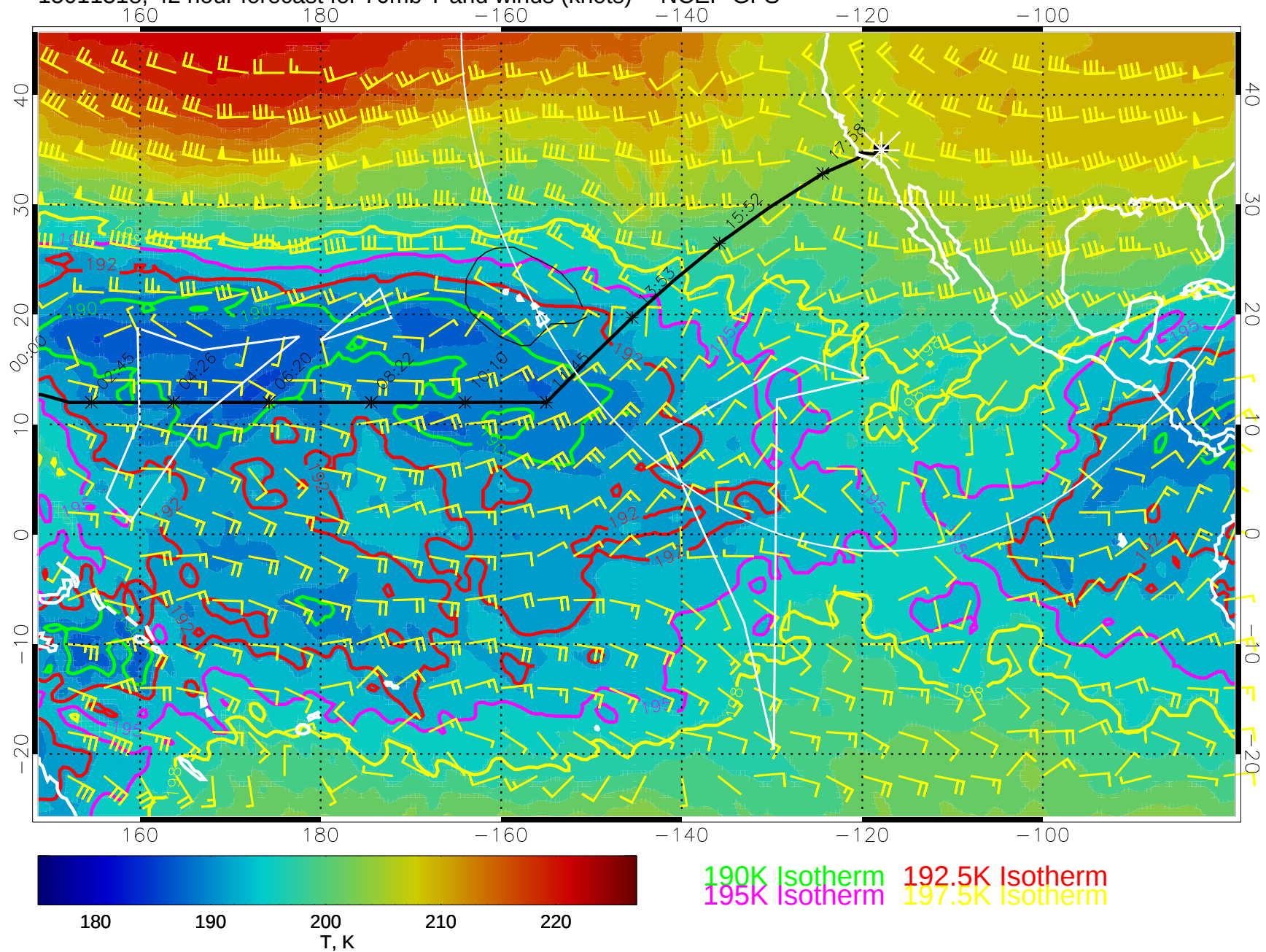
15011318, 42 hour forecast for 70mb T and winds (knots) -- NCEP GFS
