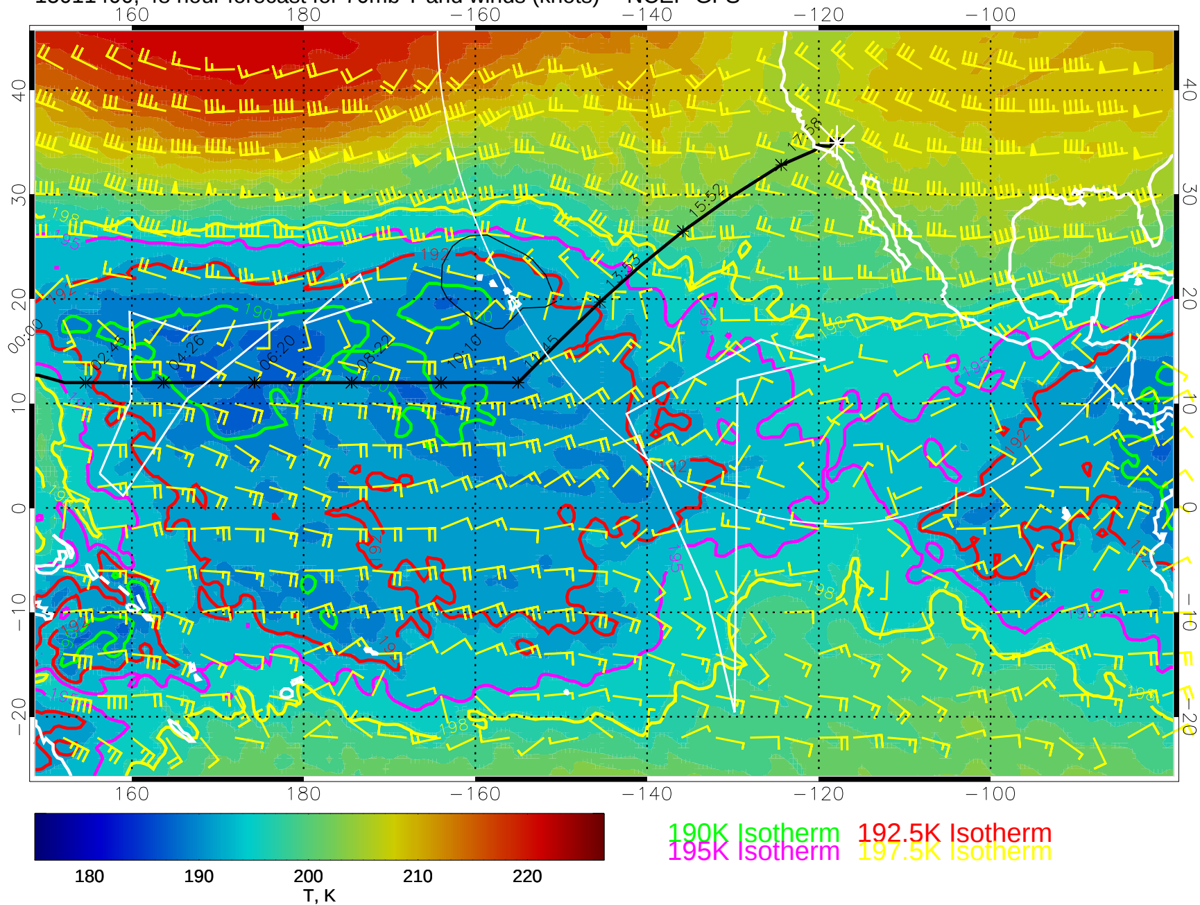
15011400, 48 hour forecast for 70mb T and winds (knots) -- NCEP GFS
