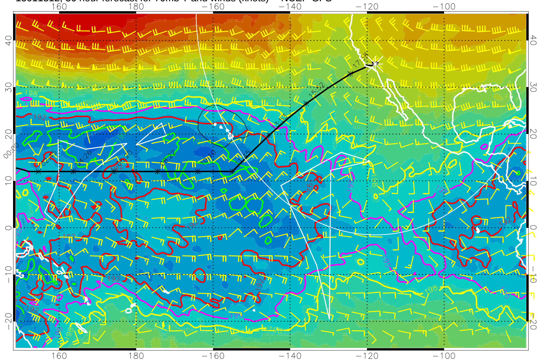
15011312, 36 hour forecast for 70mb T and winds (knots) -- NCEP GFS
