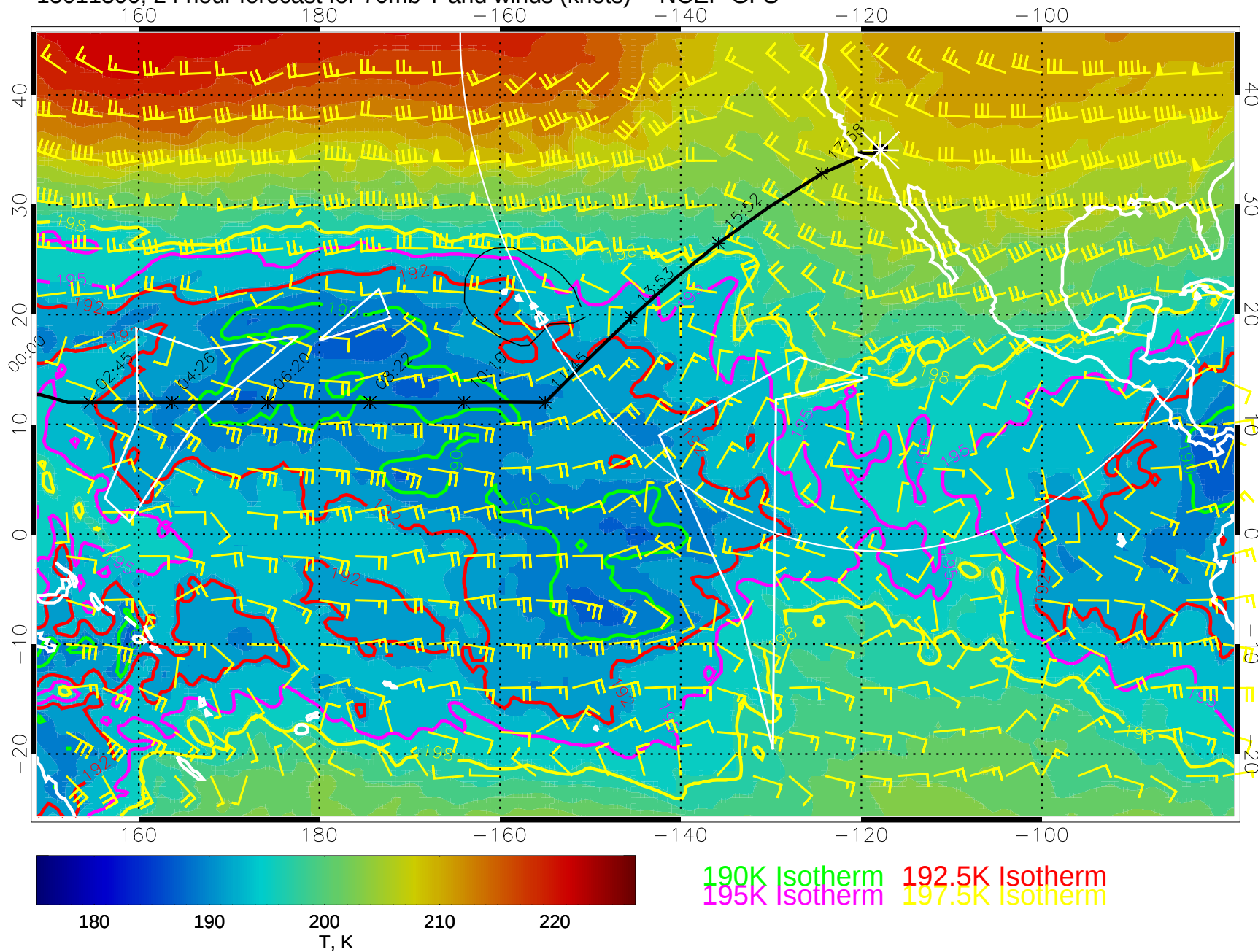
15011300, 24 hour forecast for 70mb T and winds (knots) -- NCEP GFS
