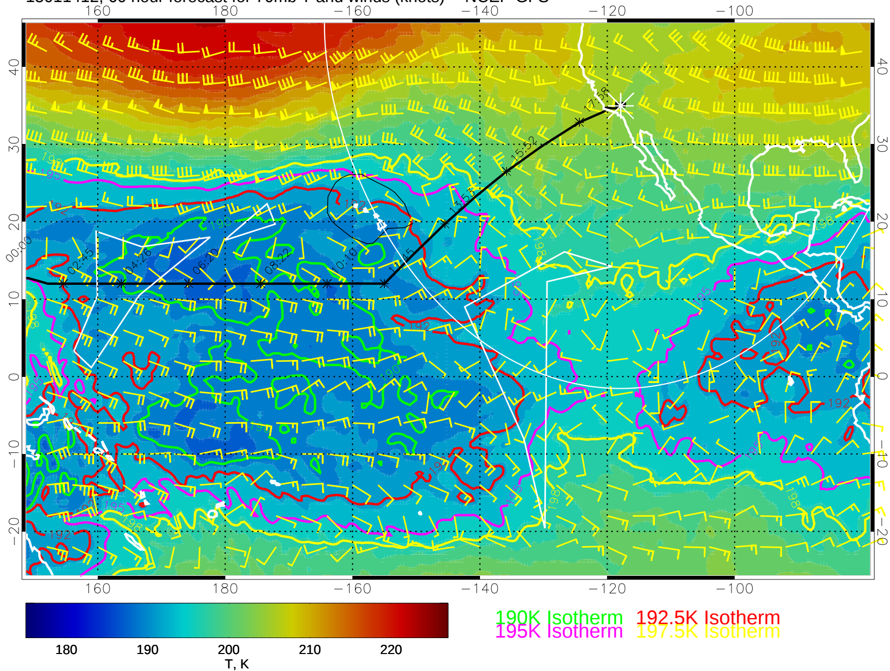
15011412, 60 hour forecast for 70mb T and winds (knots) -- NCEP GFS
