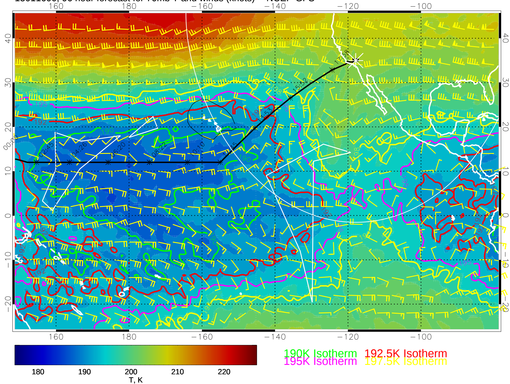
15011600, 96 hour forecast for 70mb T and winds (knots) -- NCEP GFS
