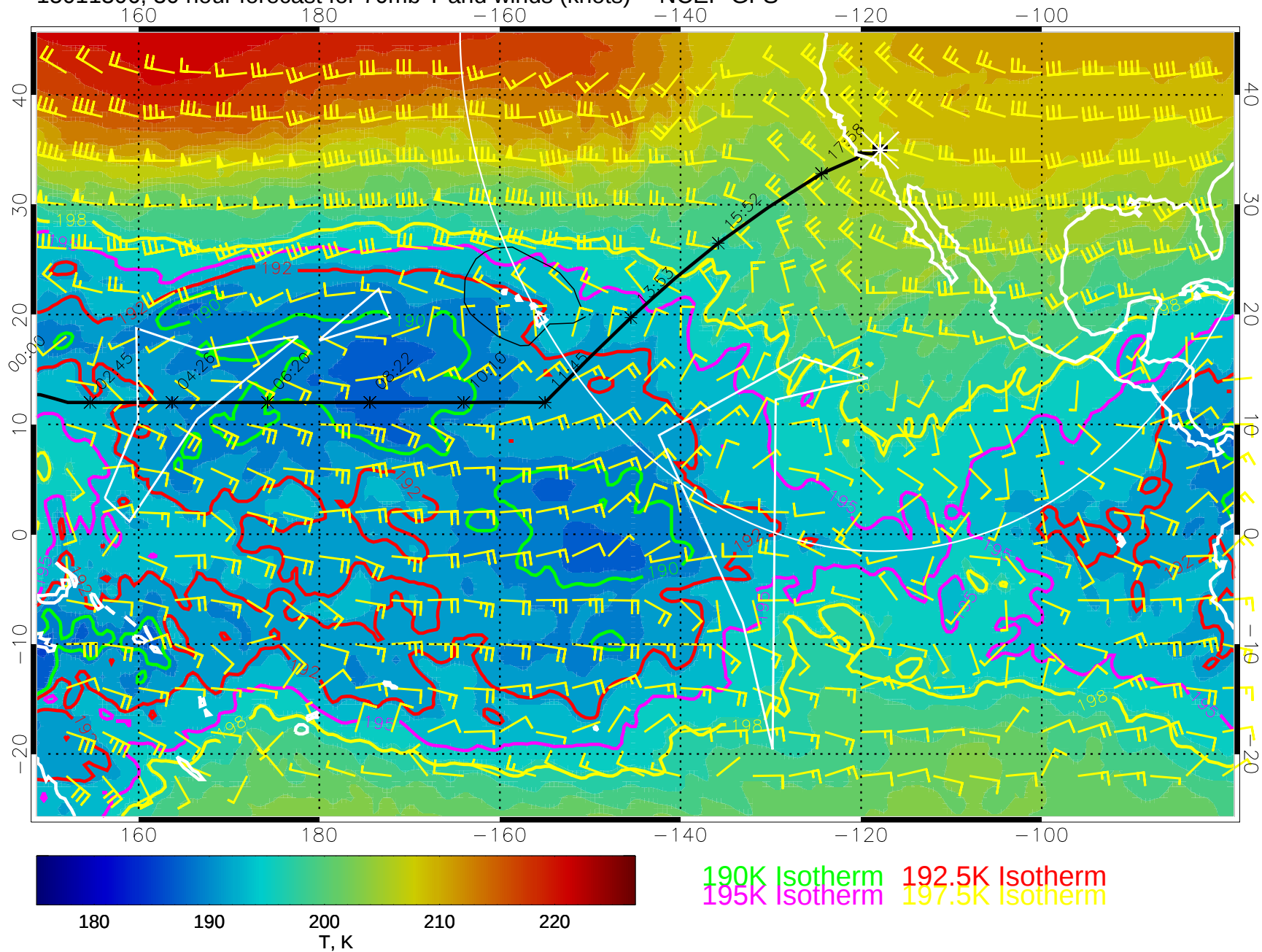
15011306, 30 hour forecast for 70mb T and winds (knots) -- NCEP GFS
