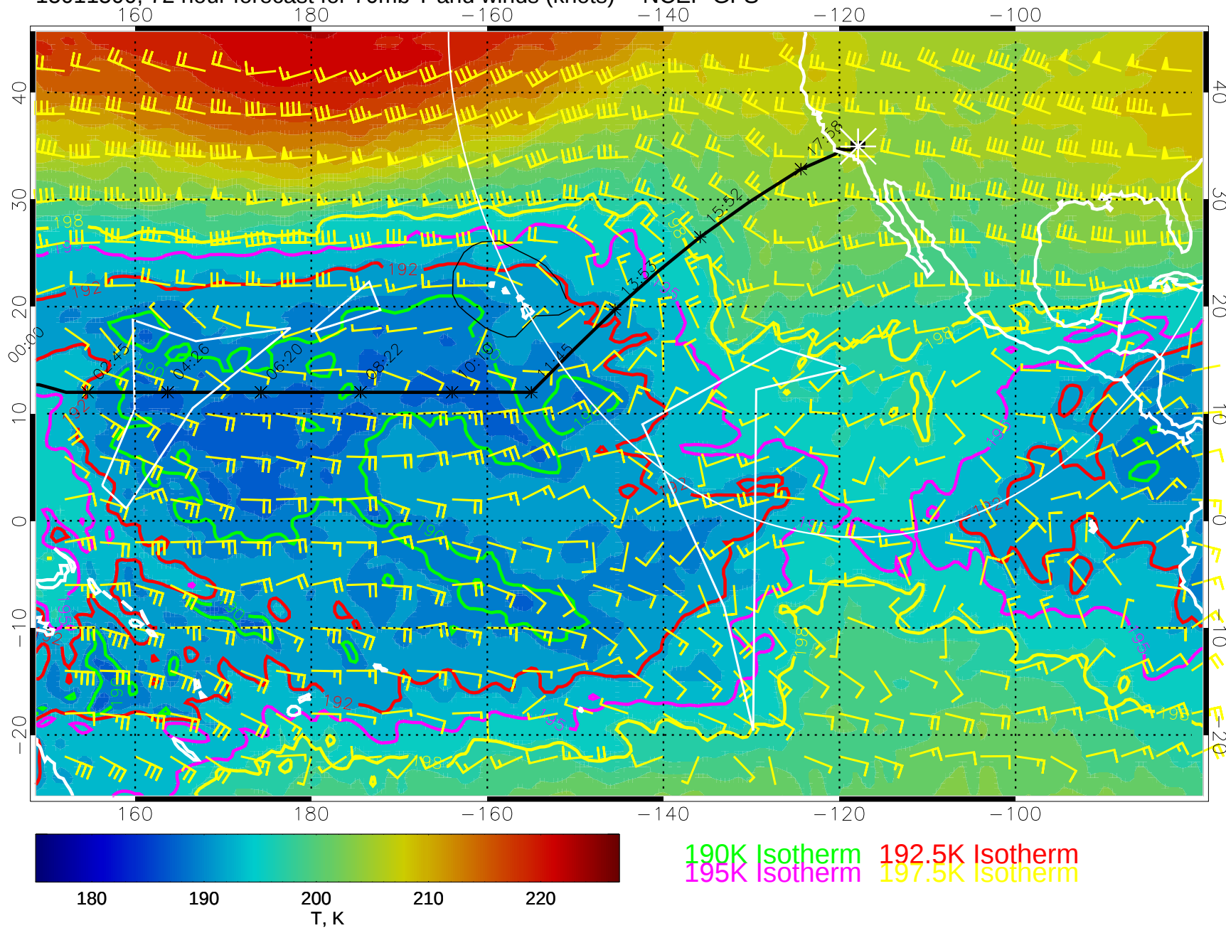
15011500, 72 hour forecast for 70mb T and winds (knots) -- NCEP GFS
