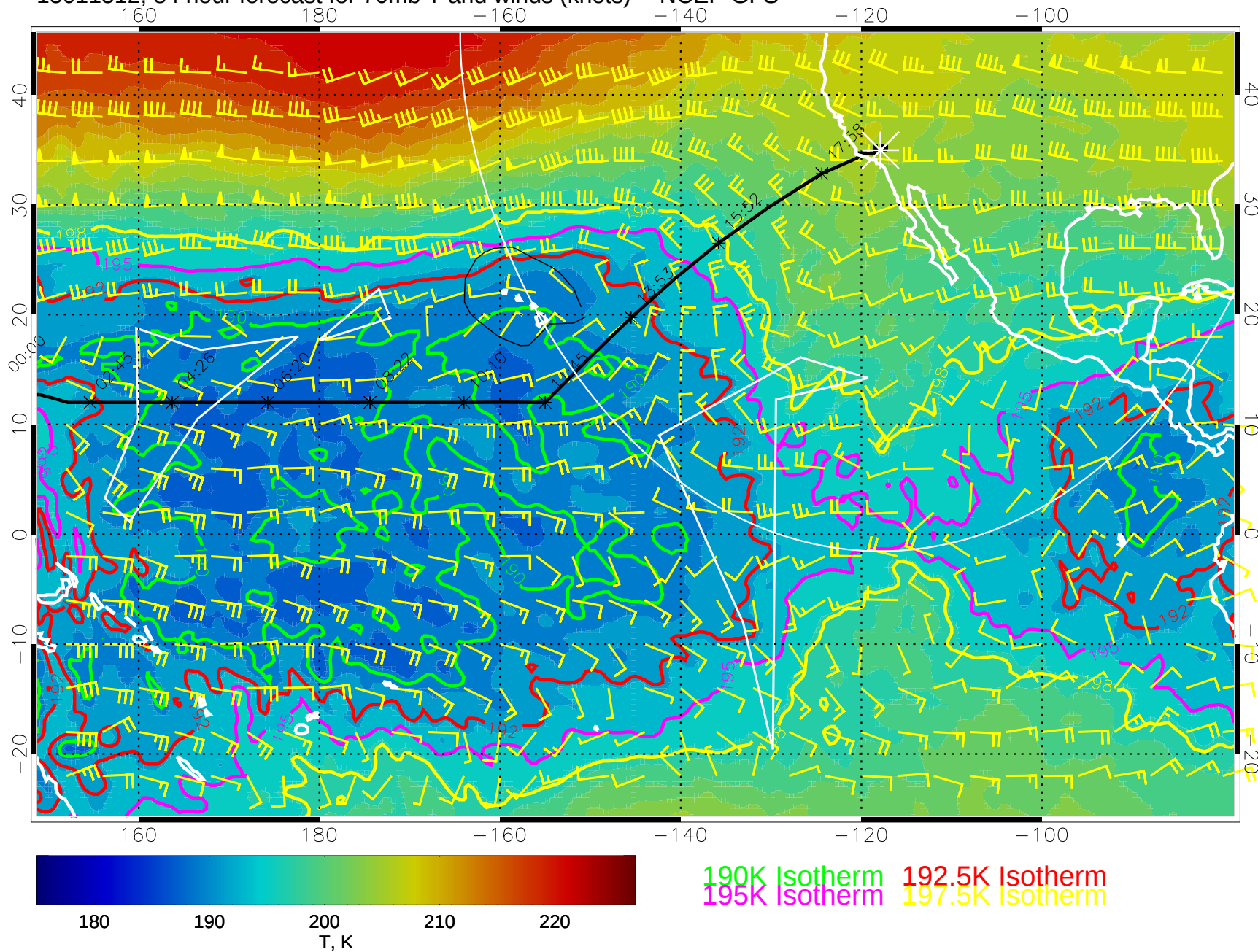
15011512, 84 hour forecast for 70mb T and winds (knots) -- NCEP GFS
