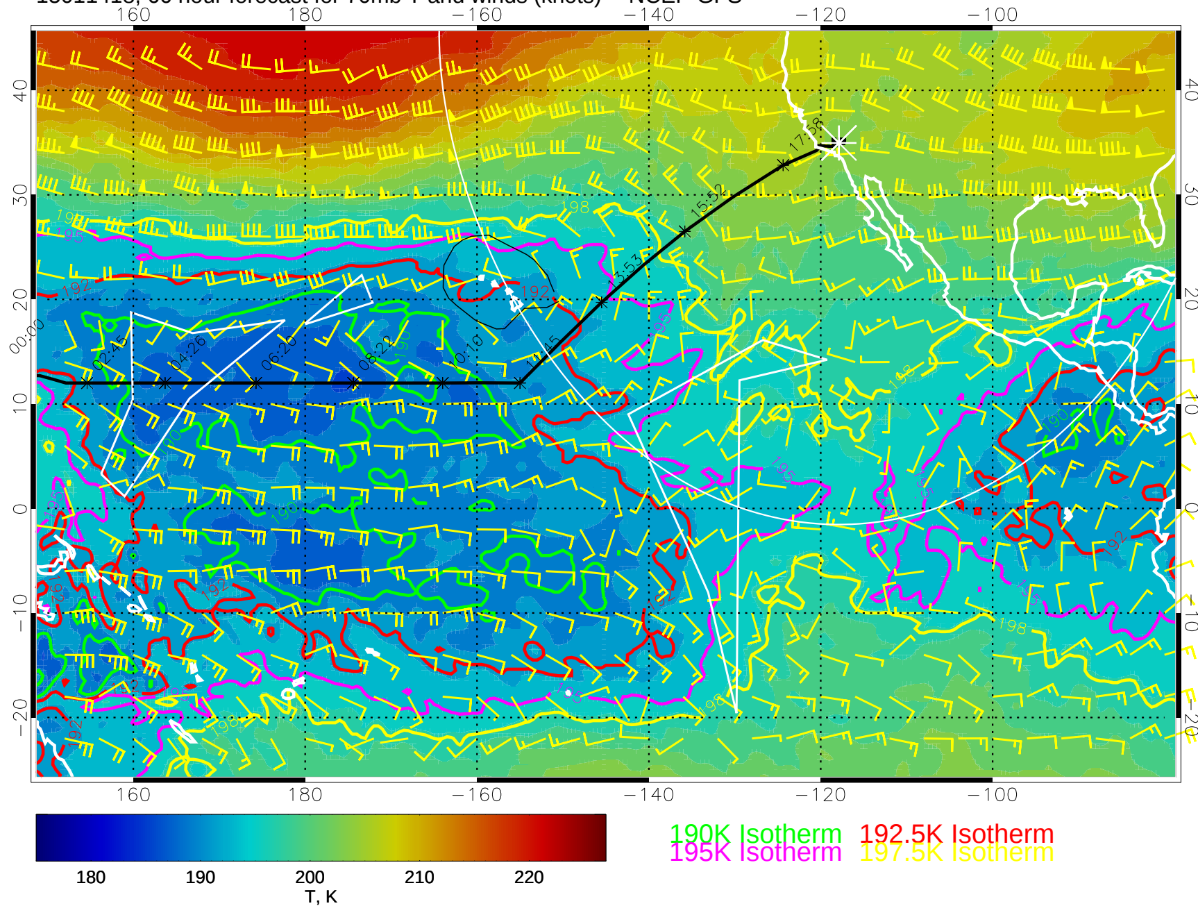
15011418, 66 hour forecast for 70mb T and winds (knots) -- NCEP GFS
