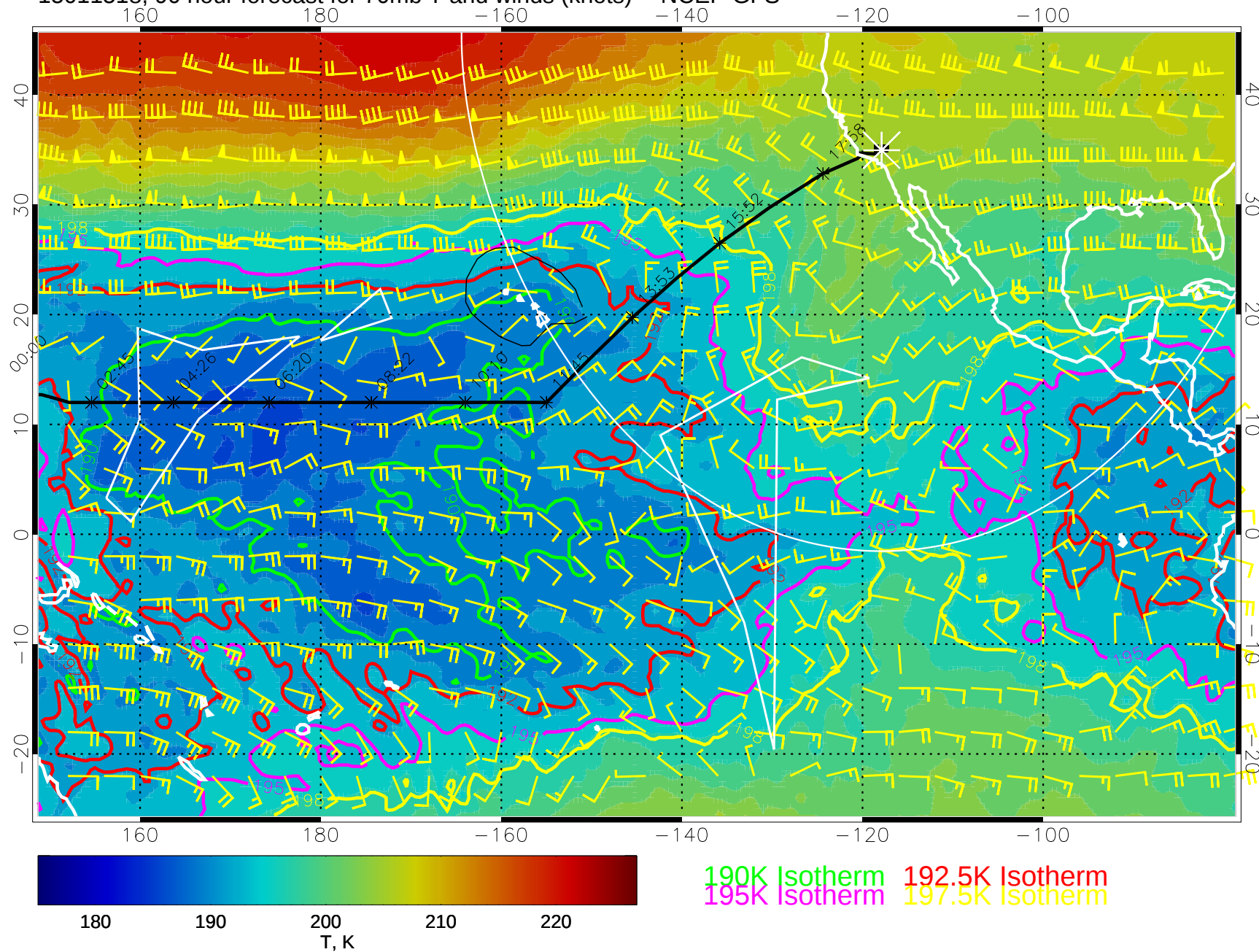
15011518, 90 hour forecast for 70mb T and winds (knots) -- NCEP GFS
