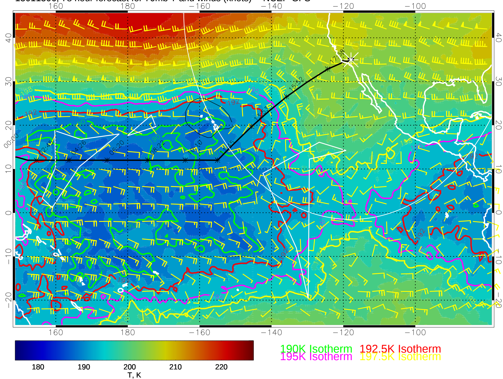
15011506, 78 hour forecast for 70mb T and winds (knots) -- NCEP GFS
