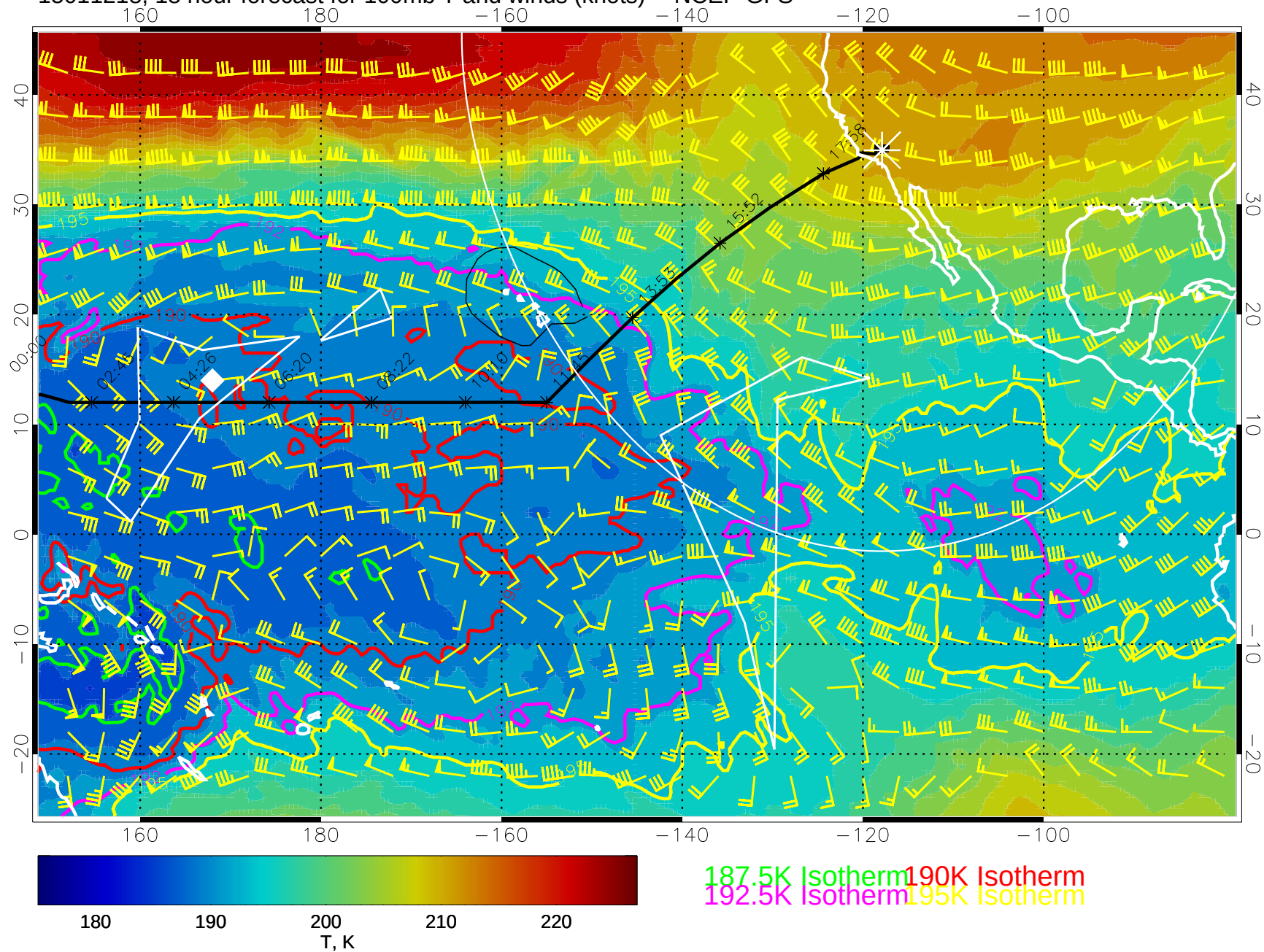
15011218, 18 hour forecast for 100mb T and winds (knots) -- NCEP GFS
