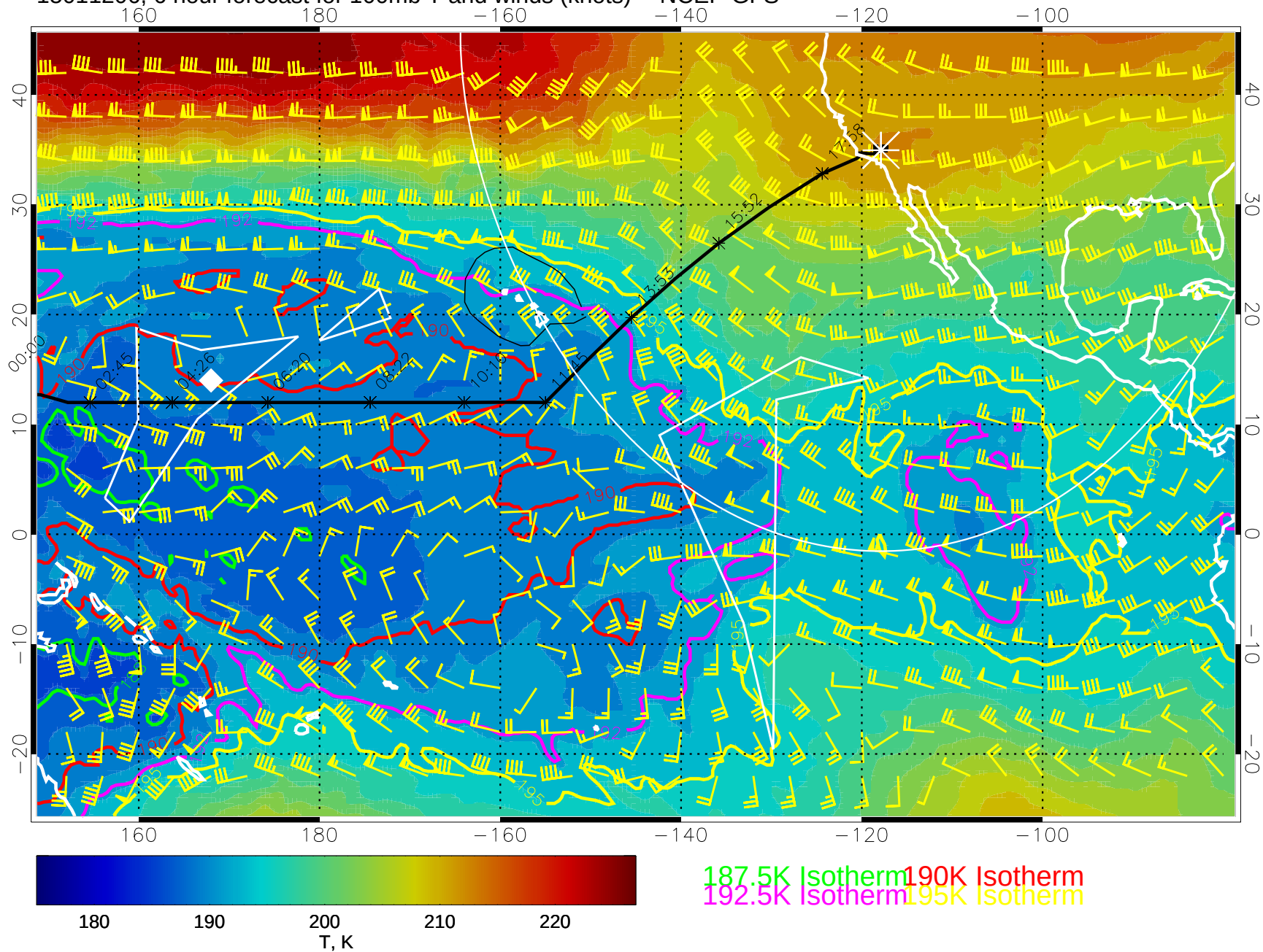
15011206, 6 hour forecast for 100mb T and winds (knots) -- NCEP GFS
