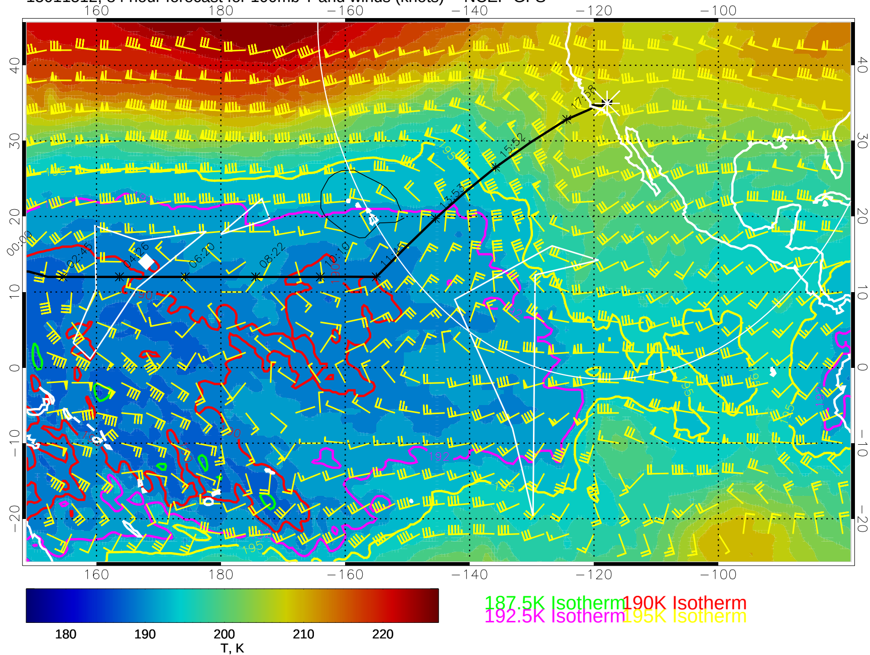
15011512, 84 hour forecast for 100mb T and winds (knots) -- NCEP GFS
