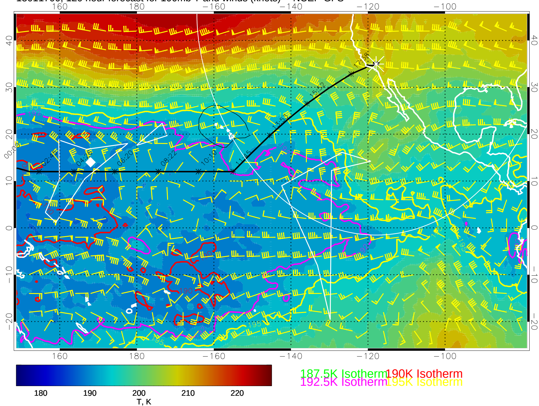
15011700, 120 hour forecast for 100mb T and winds (knots) -- NCEP GFS
