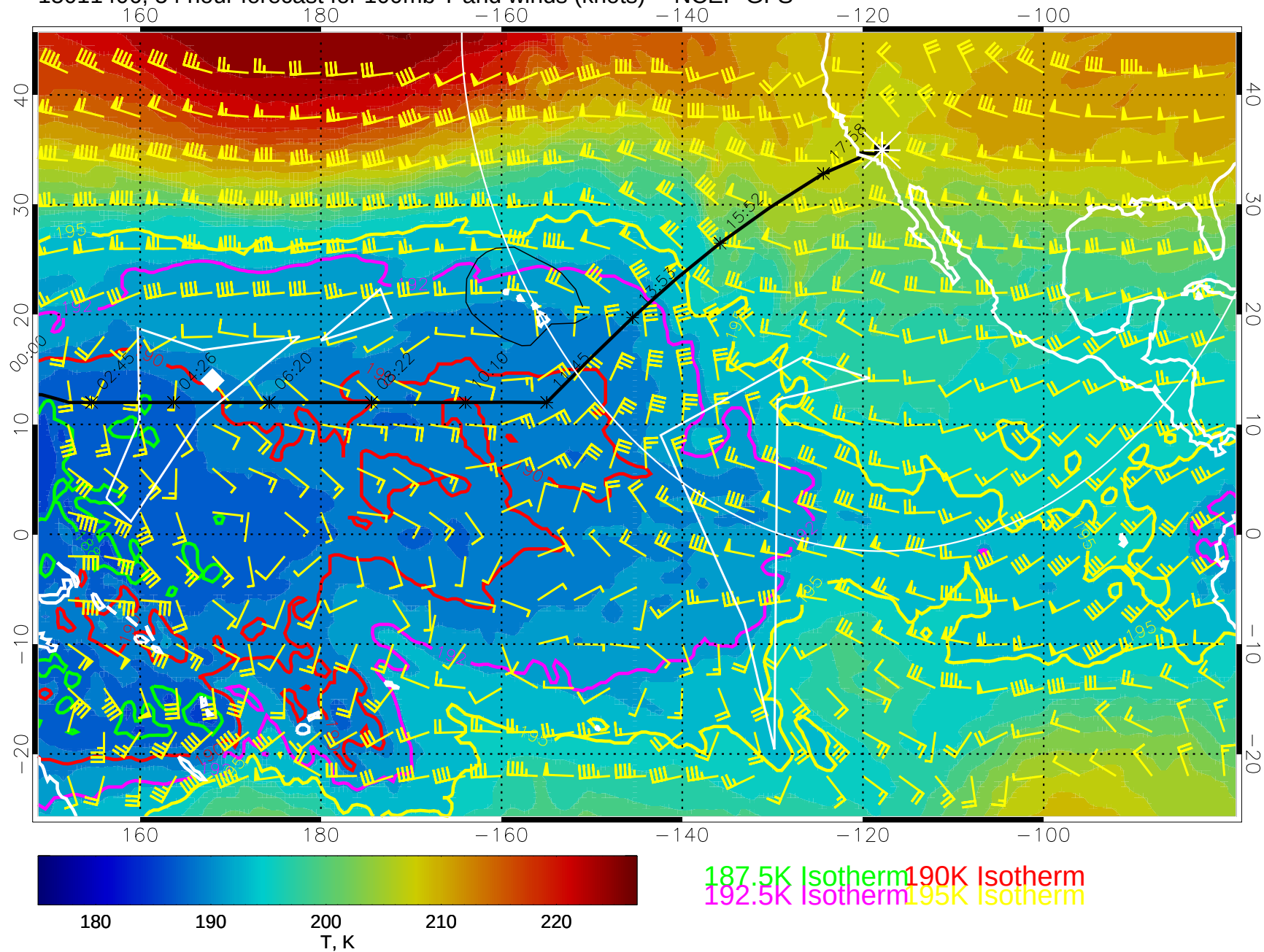
15011406, 54 hour forecast for 100mb T and winds (knots) -- NCEP GFS
