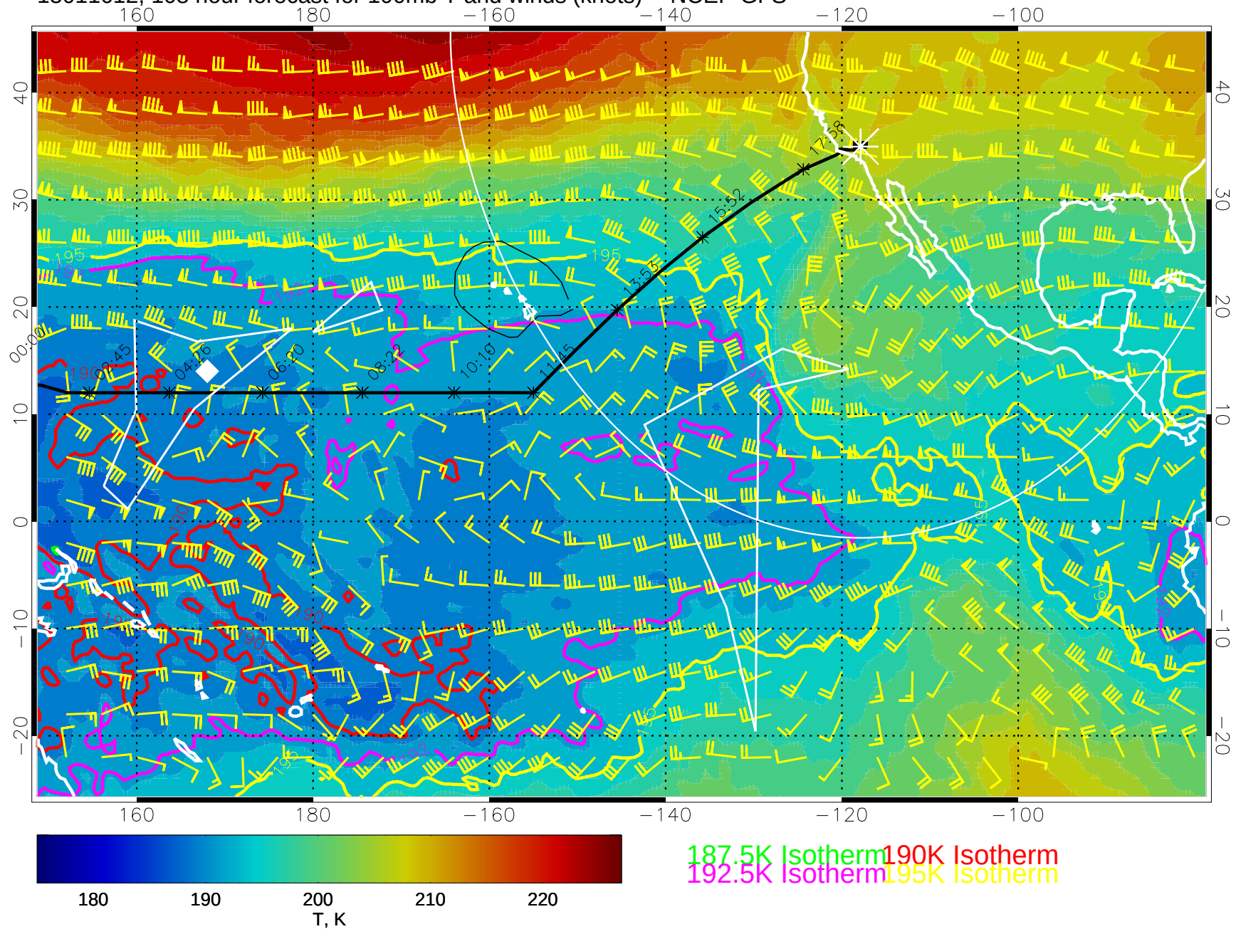
15011612, 108 hour forecast for 100mb T and winds (knots) -- NCEP GFS
