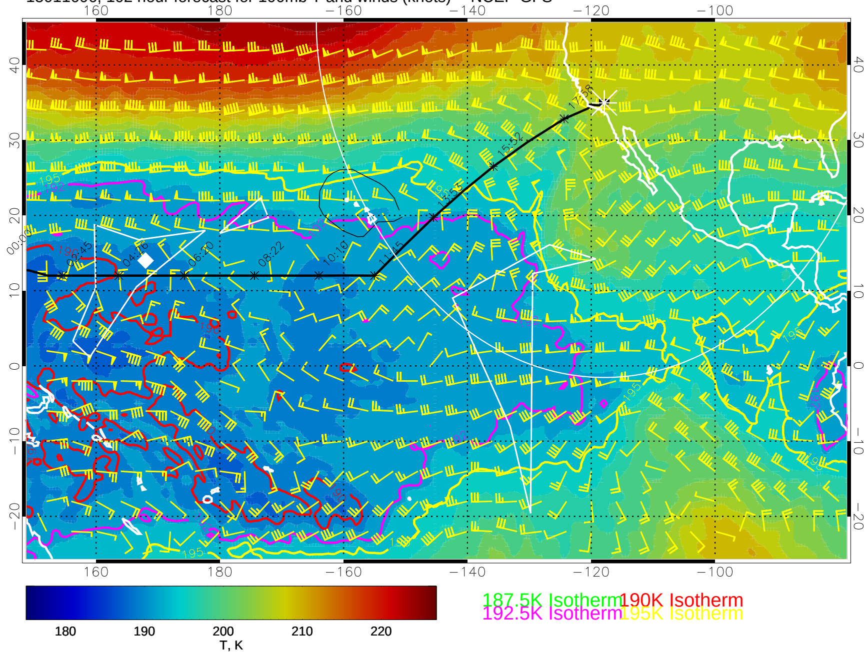
15011606, 102 hour forecast for 100mb T and winds (knots) -- NCEP GFS
