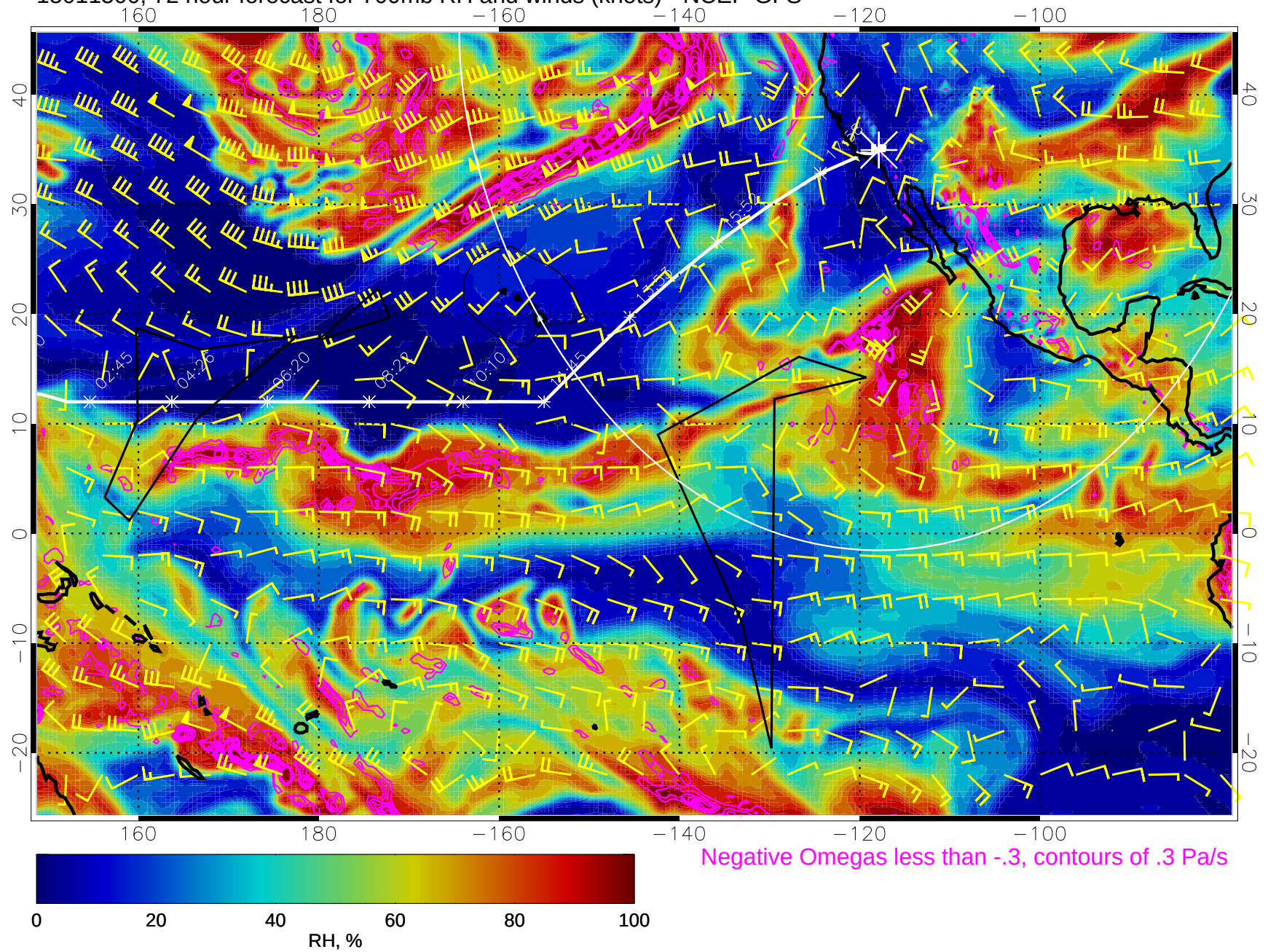
15011500, 72 hour forecast for 700mb RH and winds (knots) - NCEP GFS
