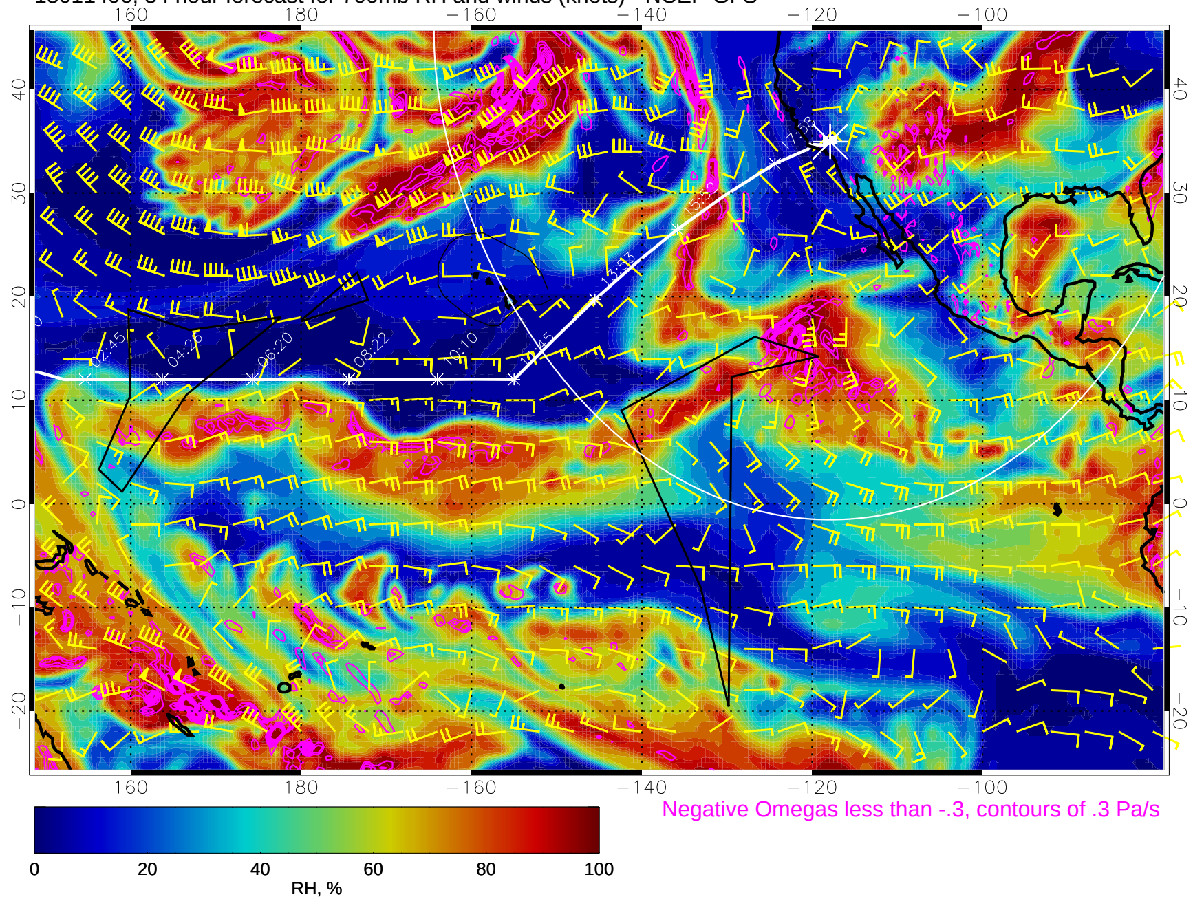
15011406, 54 hour forecast for 700mb RH and winds (knots) - NCEP GFS
