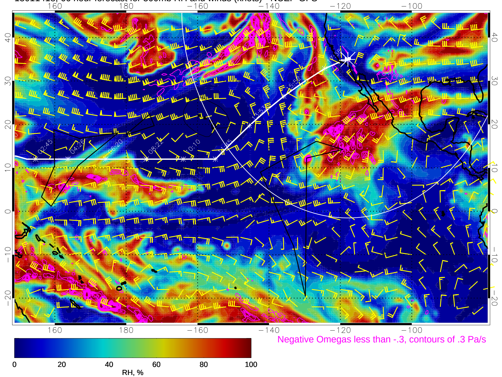
15011418, 66 hour forecast for 500mb RH and winds (knots) - NCEP GFS
