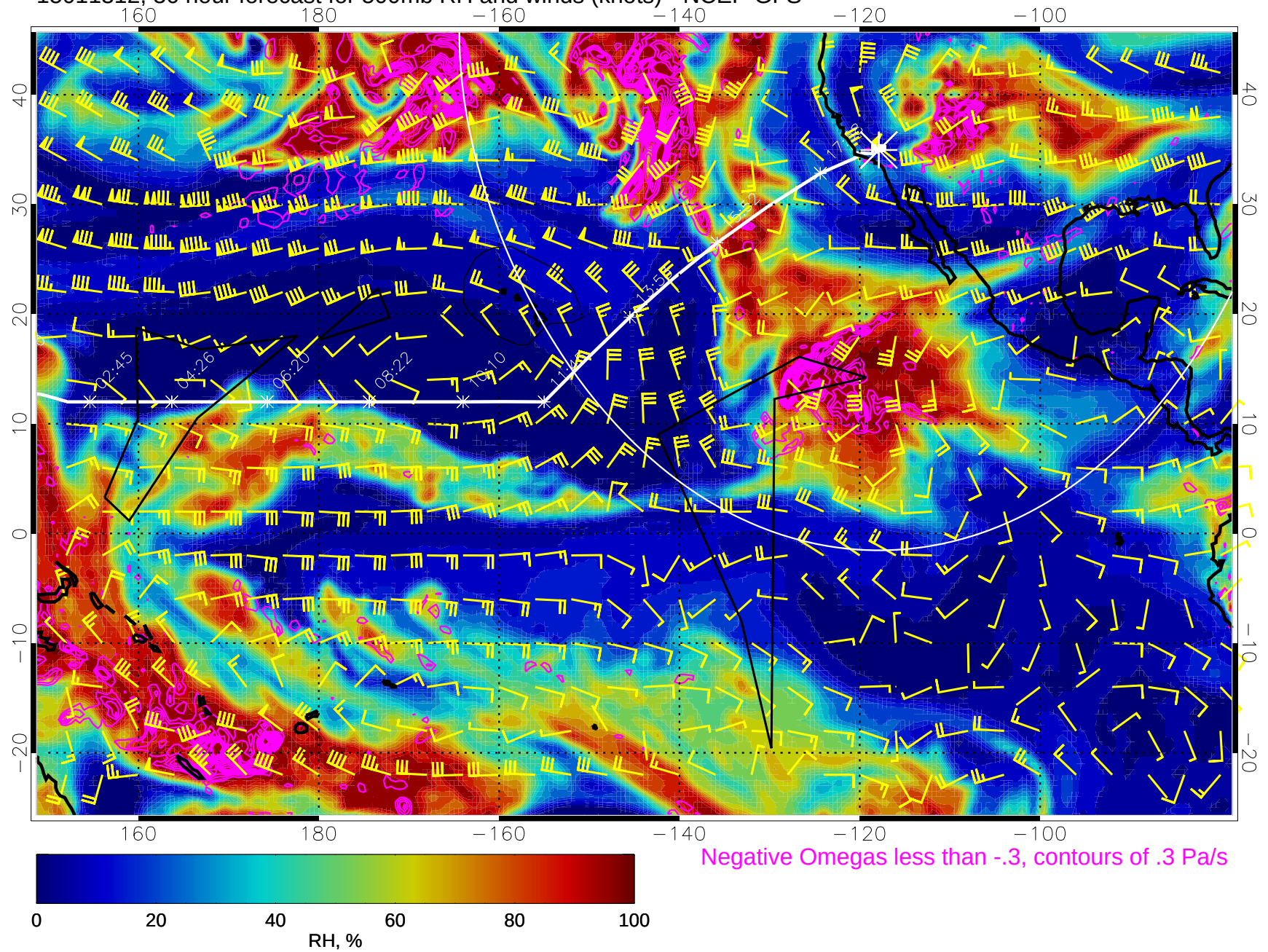
15011312, 36 hour forecast for 500mb RH and winds (knots) - NCEP GFS
