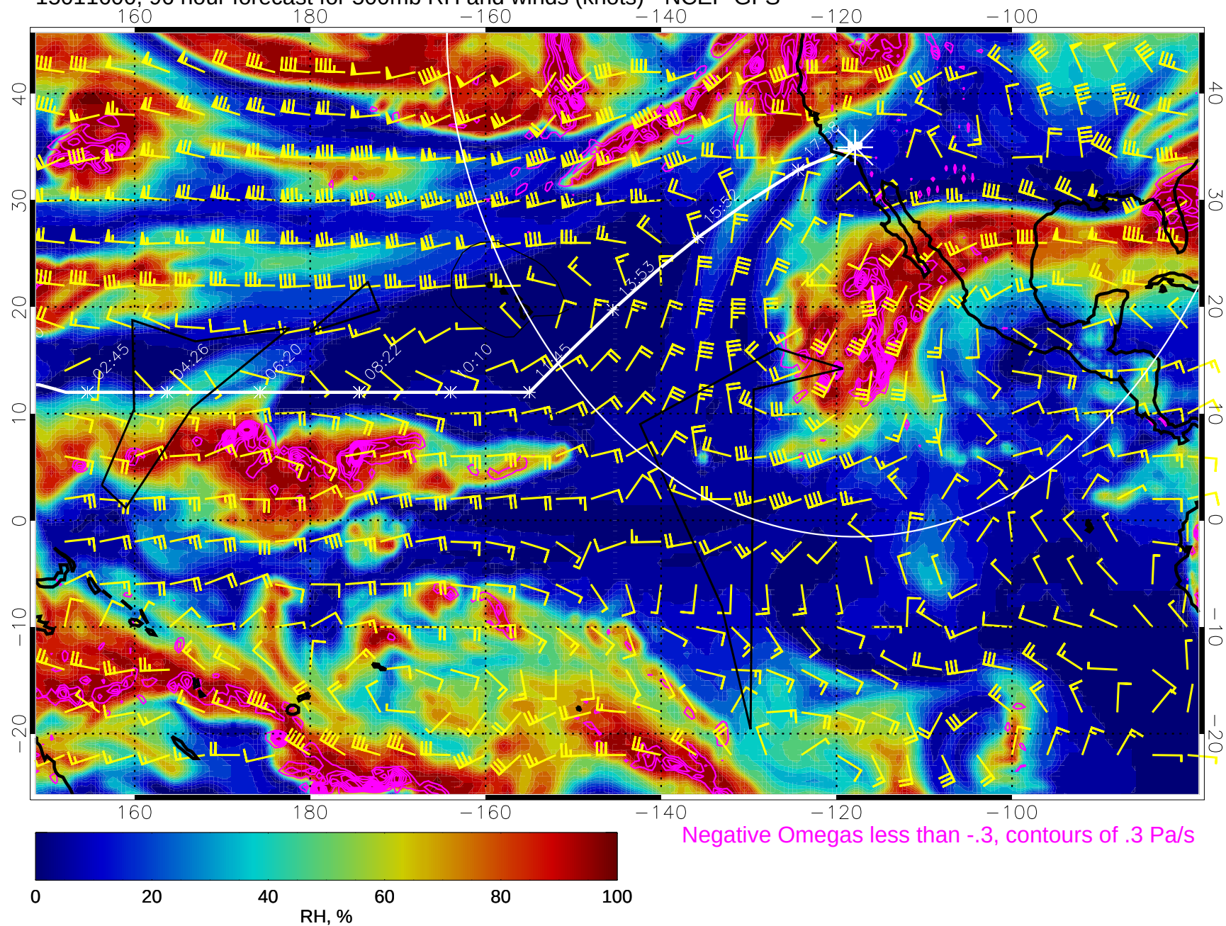
15011600, 96 hour forecast for 500mb RH and winds (knots) - NCEP GFS
