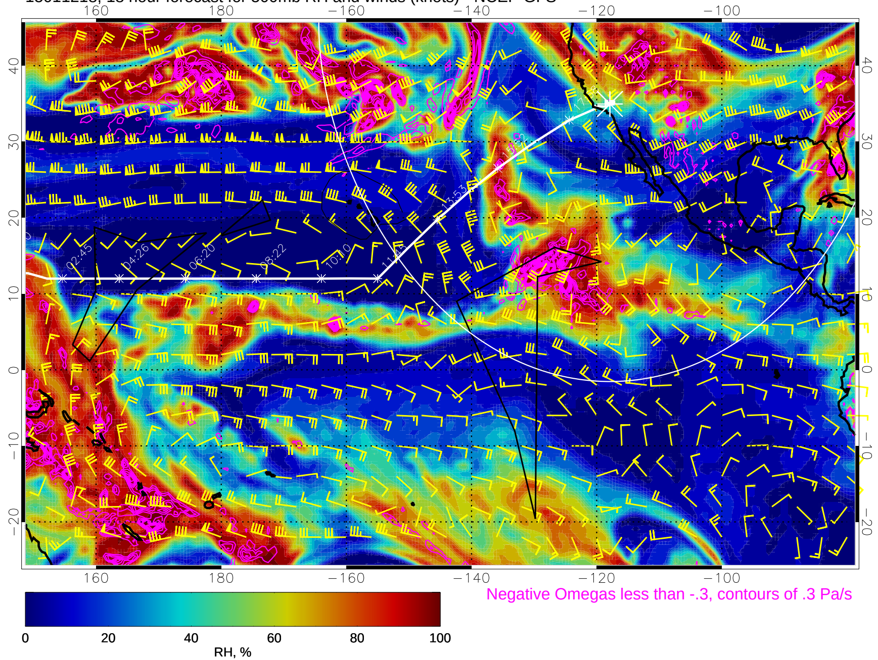
15011218, 18 hour forecast for 500mb RH and winds (knots) - NCEP GFS
