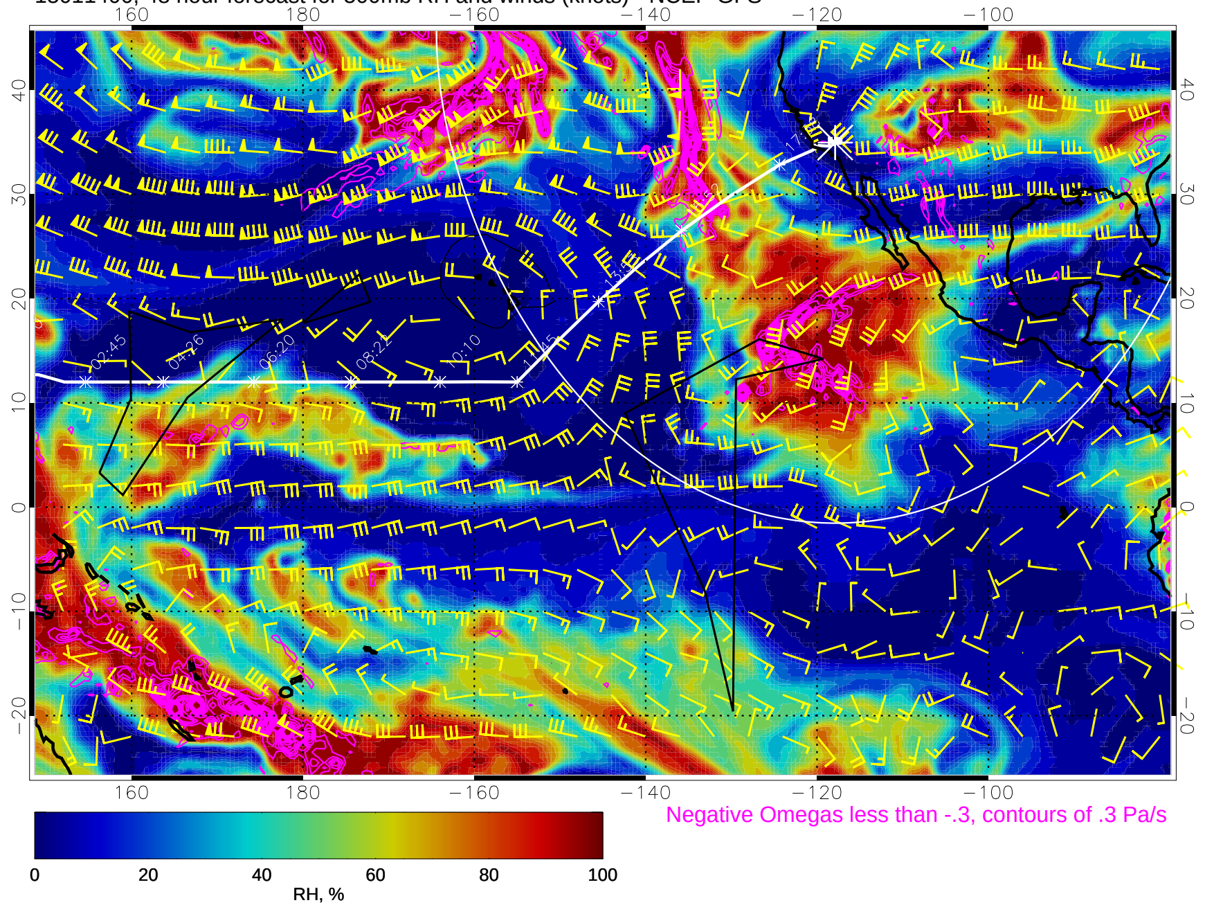
15011400, 48 hour forecast for 500mb RH and winds (knots) - NCEP GFS
