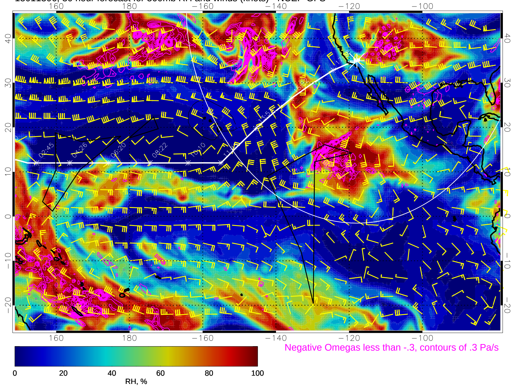
15011306, 30 hour forecast for 500mb RH and winds (knots) - NCEP GFS
