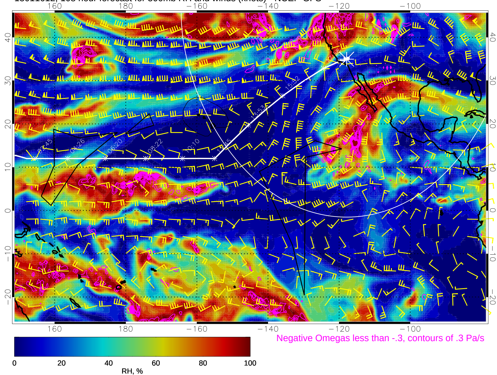
15011612, 108 hour forecast for 500mb RH and winds (knots) - NCEP GFS
