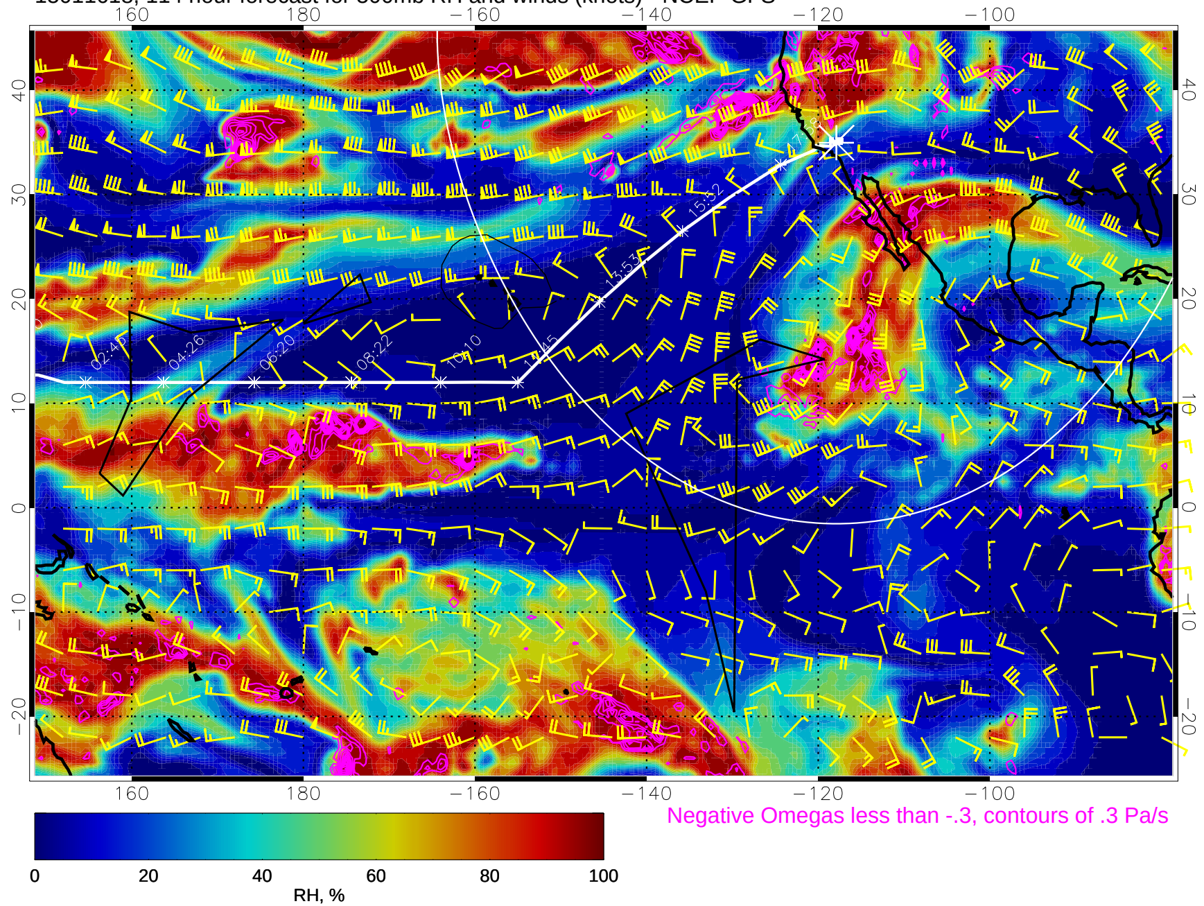
15011618, 114 hour forecast for 500mb RH and winds (knots) - NCEP GFS
