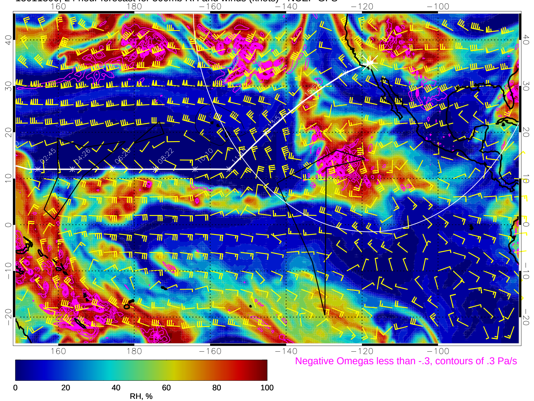
15011300, 24 hour forecast for 500mb RH and winds (knots) - NCEP GFS
