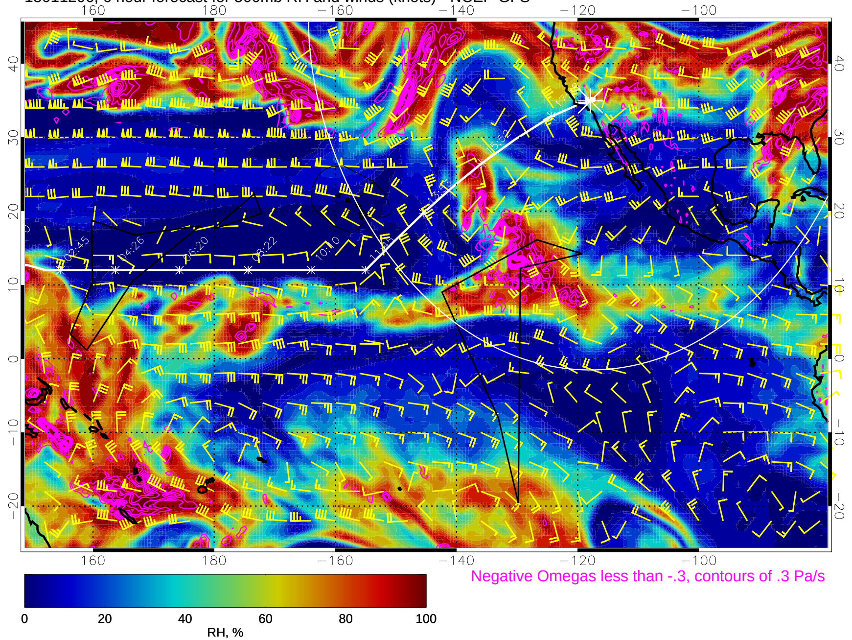
15011206, 6 hour forecast for 500mb RH and winds (knots) - NCEP GFS
