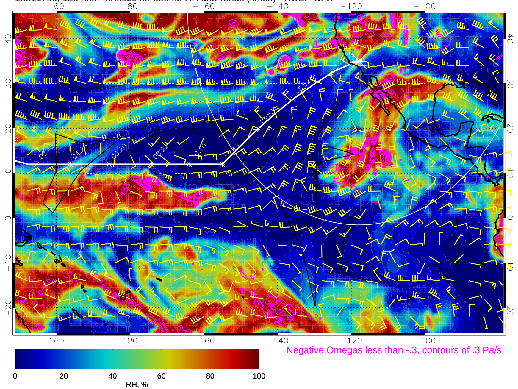
15011700, 120 hour forecast for 500mb RH and winds (knots) - NCEP GFS
