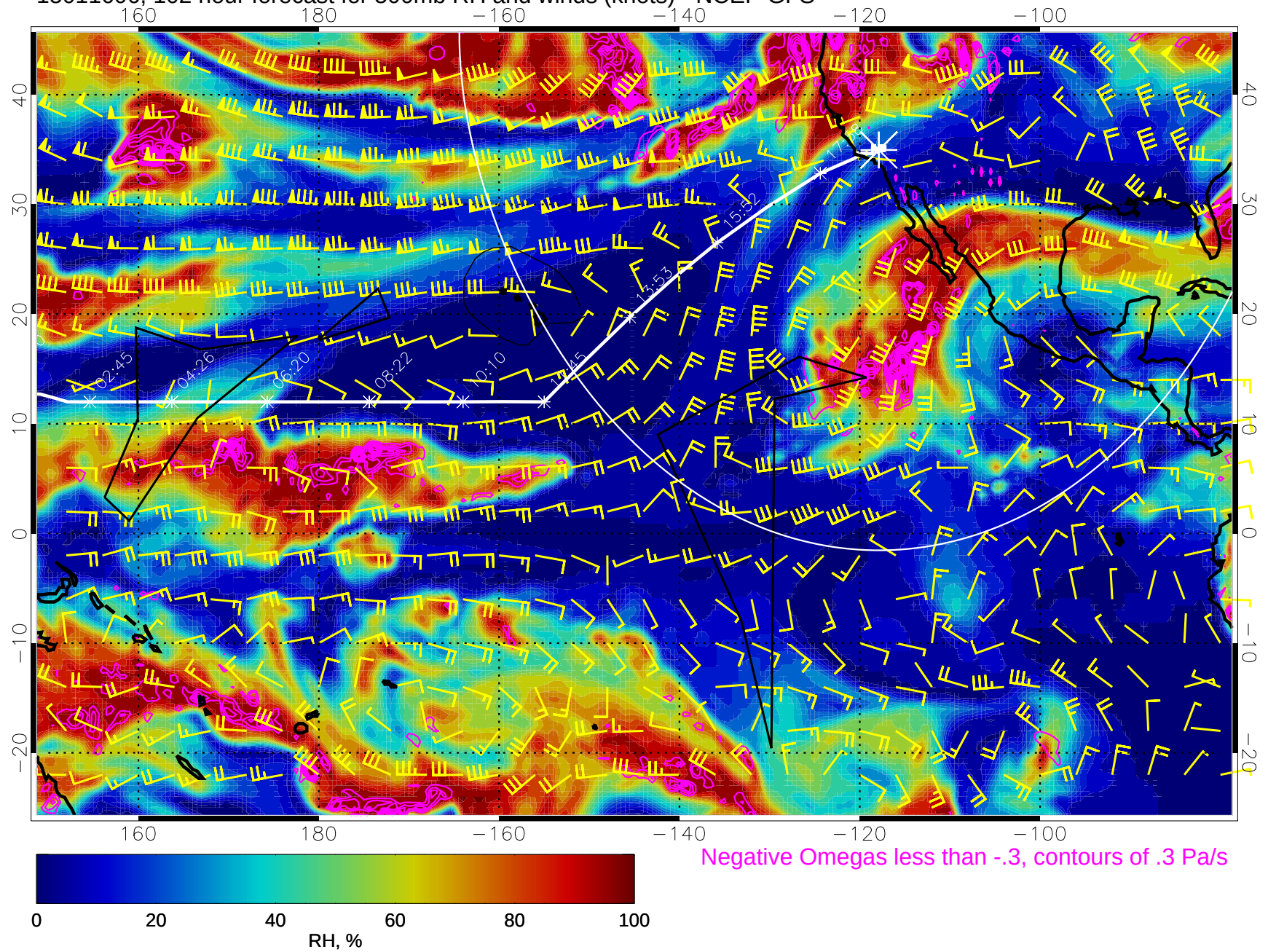
15011606, 102 hour forecast for 500mb RH and winds (knots) - NCEP GFS
