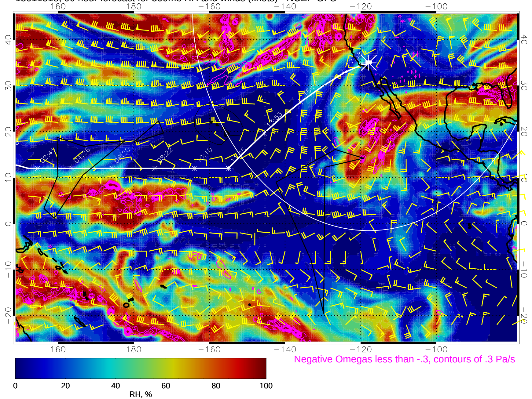
15011518, 90 hour forecast for 500mb RH and winds (knots) - NCEP GFS
