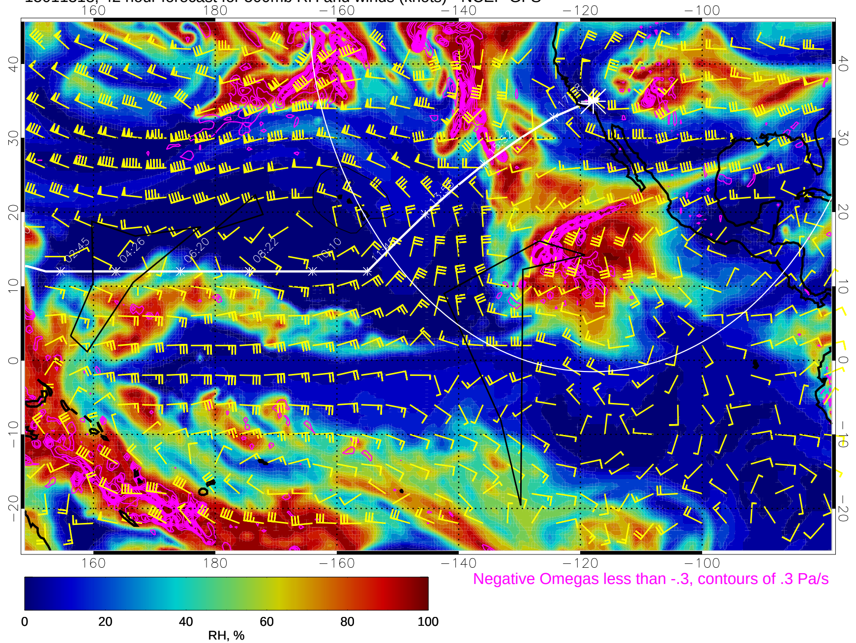
15011318, 42 hour forecast for 500mb RH and winds (knots) - NCEP GFS
