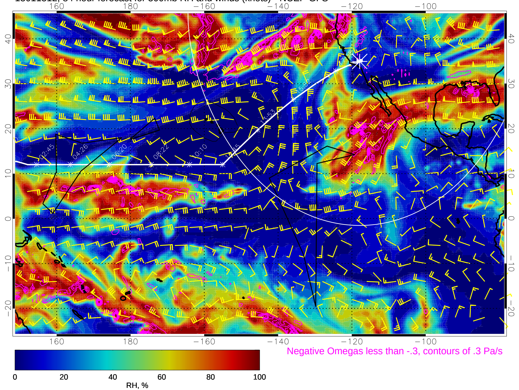
15011512, 84 hour forecast for 500mb RH and winds (knots) - NCEP GFS
