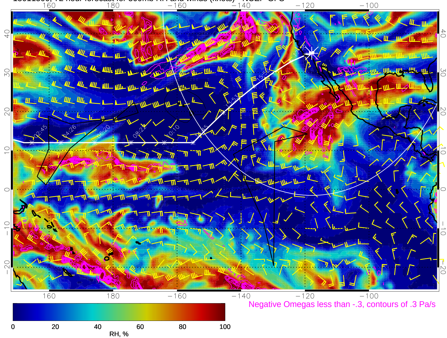
15011500, 72 hour forecast for 500mb RH and winds (knots) - NCEP GFS
