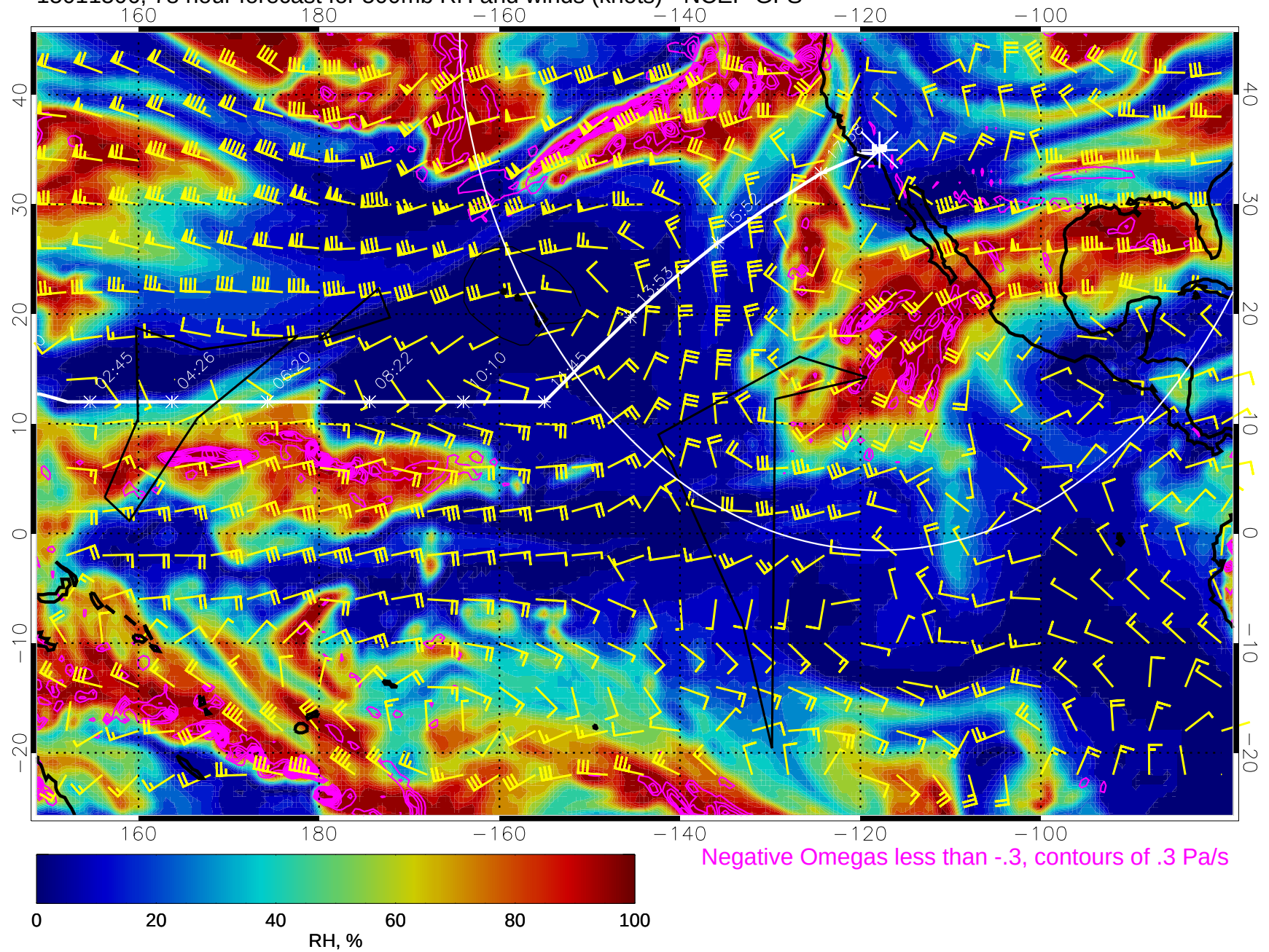
15011506, 78 hour forecast for 500mb RH and winds (knots) - NCEP GFS
