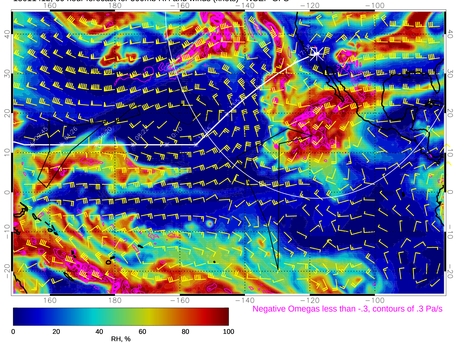
15011412, 60 hour forecast for 500mb RH and winds (knots) - NCEP GFS
