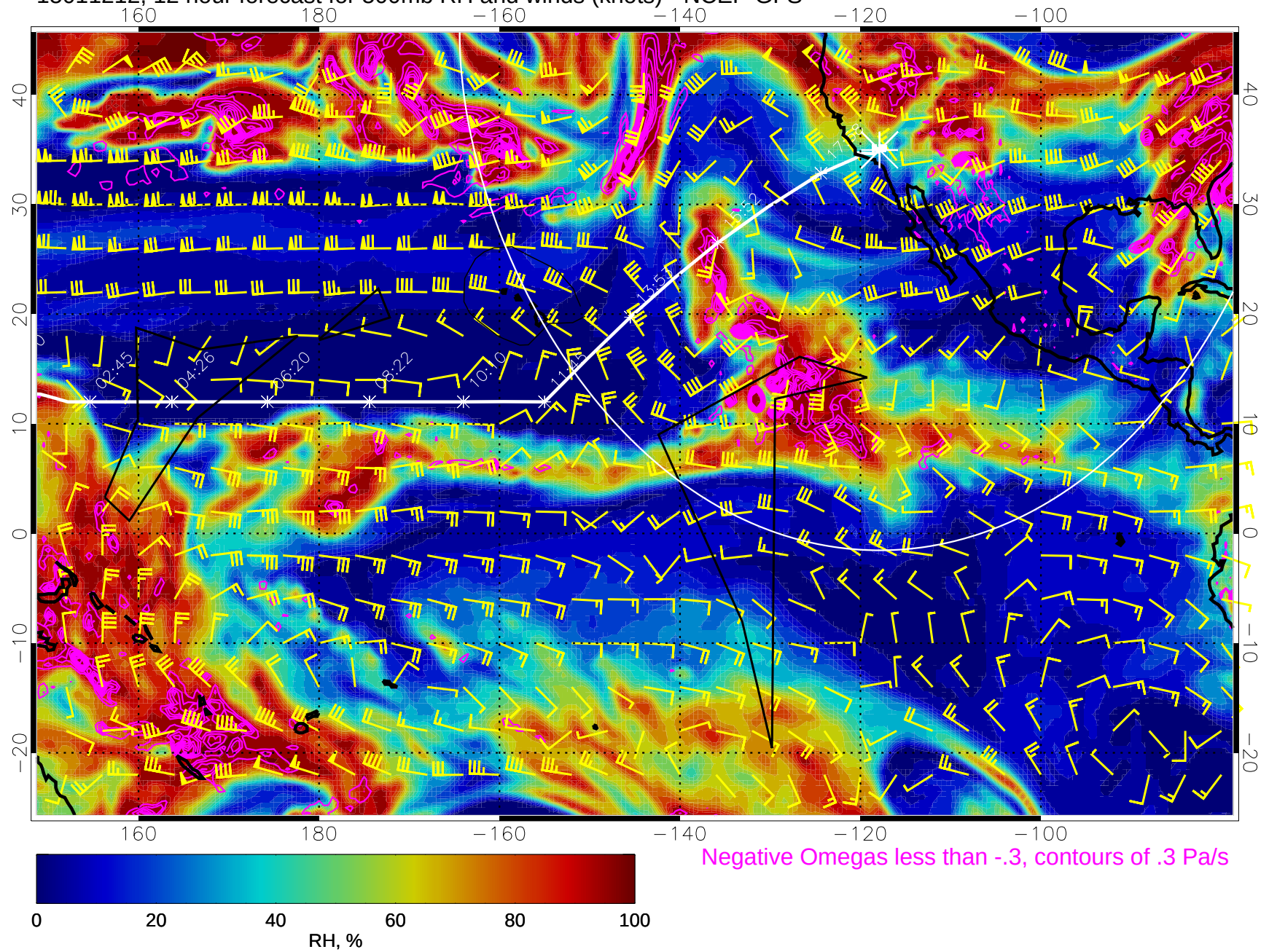
15011212, 12 hour forecast for 500mb RH and winds (knots) - NCEP GFS
