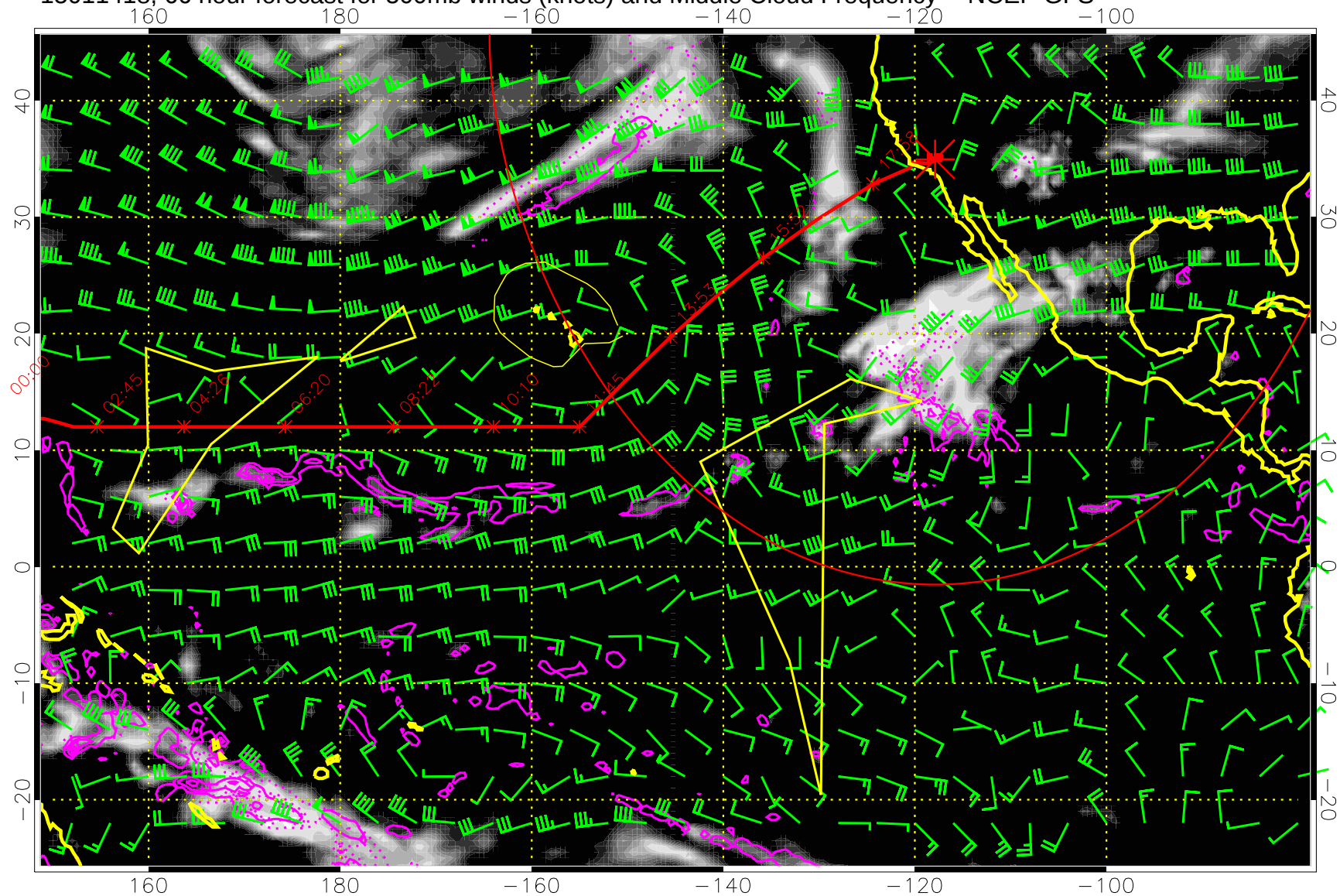
15011418, 66 hour forecast for 500mb winds (knots) and Middle Cloud Frequency -- NCEP GFS
