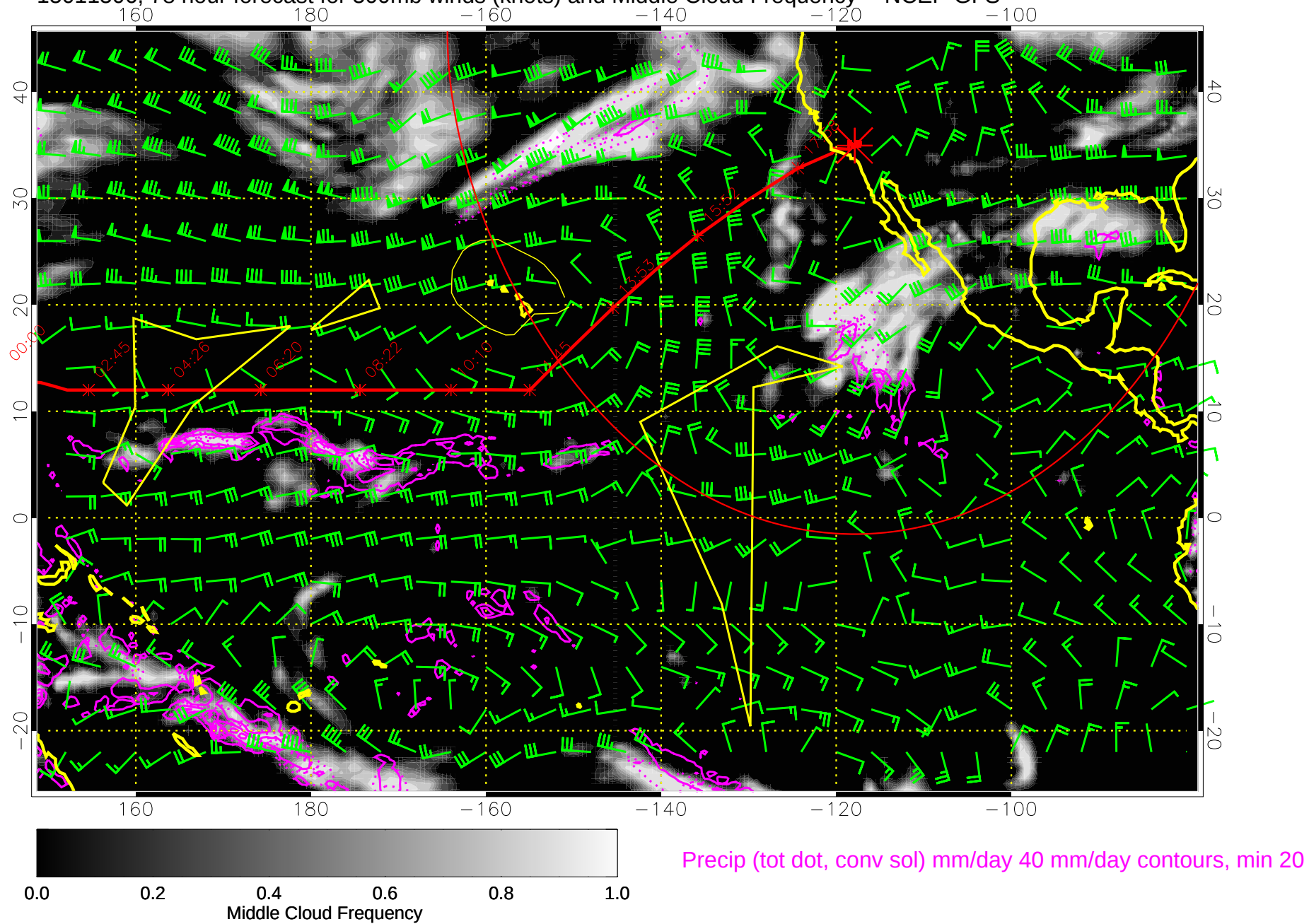
15011506, 78 hour forecast for 500mb winds (knots) and Middle Cloud Frequency -- NCEP GFS
