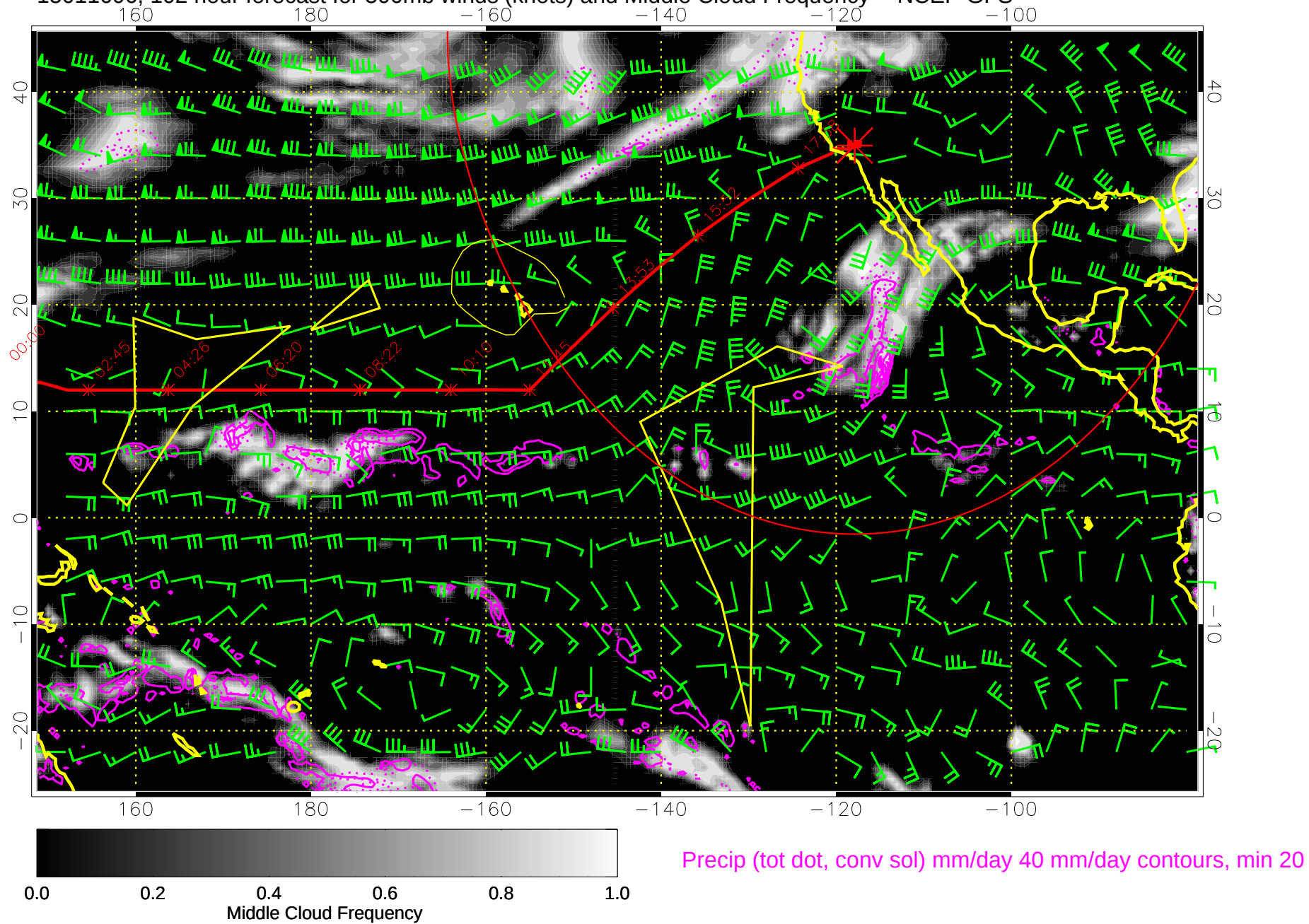
15011606, 102 hour forecast for 500mb winds (knots) and Middle Cloud Frequency -- NCEP GFS
