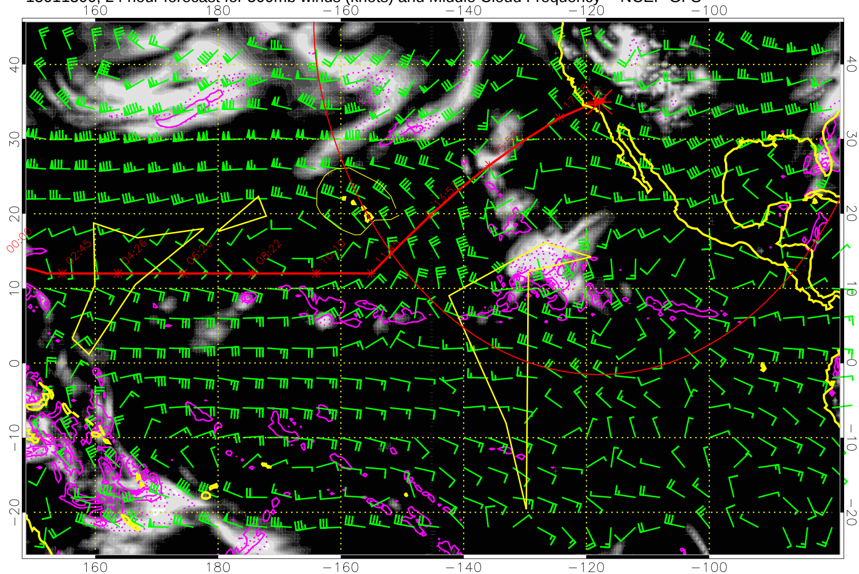
15011300, 24 hour forecast for 500mb winds (knots) and Middle Cloud Frequency -- NCEP GFS
