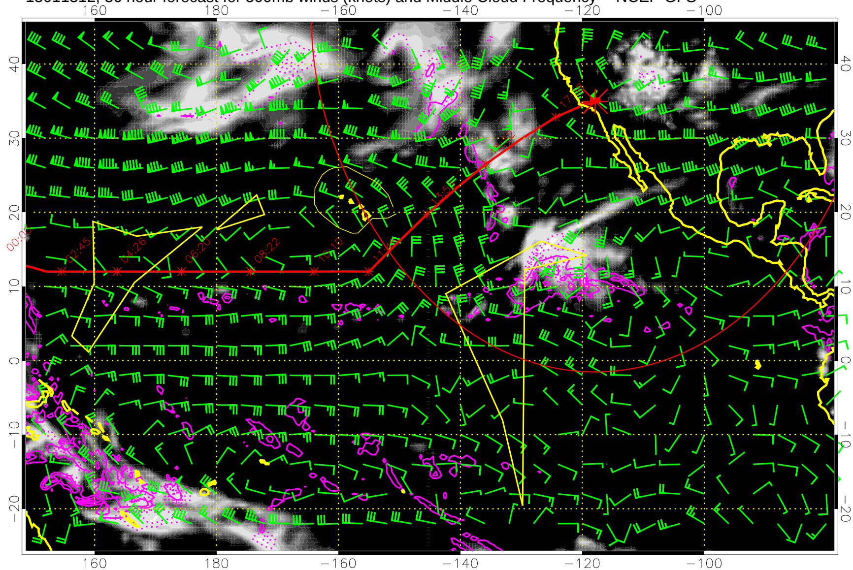
15011312, 36 hour forecast for 500mb winds (knots) and Middle Cloud Frequency -- NCEP GFS
