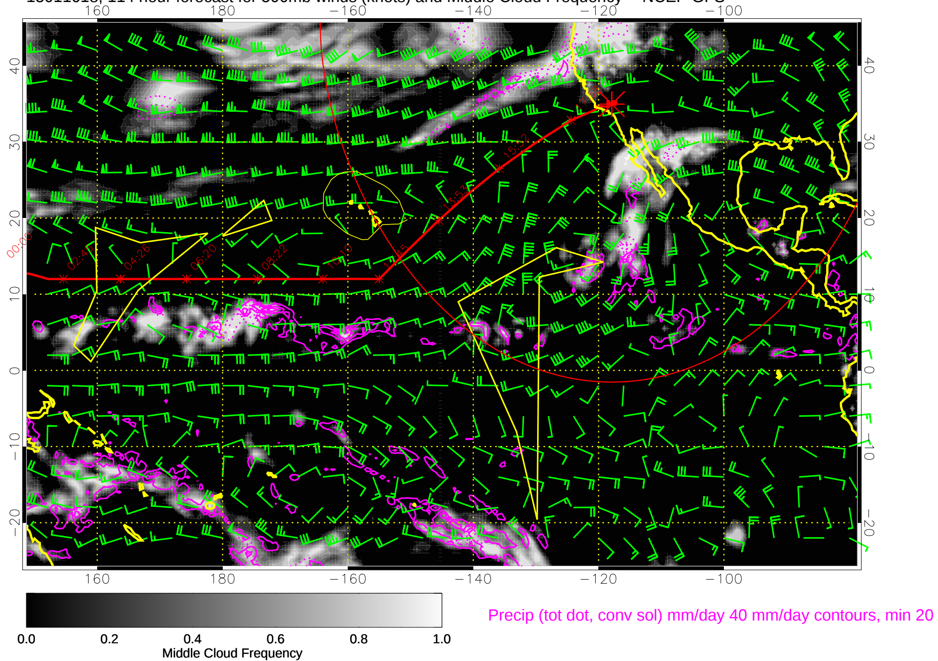
15011618, 114 hour forecast for 500mb winds (knots) and Middle Cloud Frequency -- NCEP GFS
