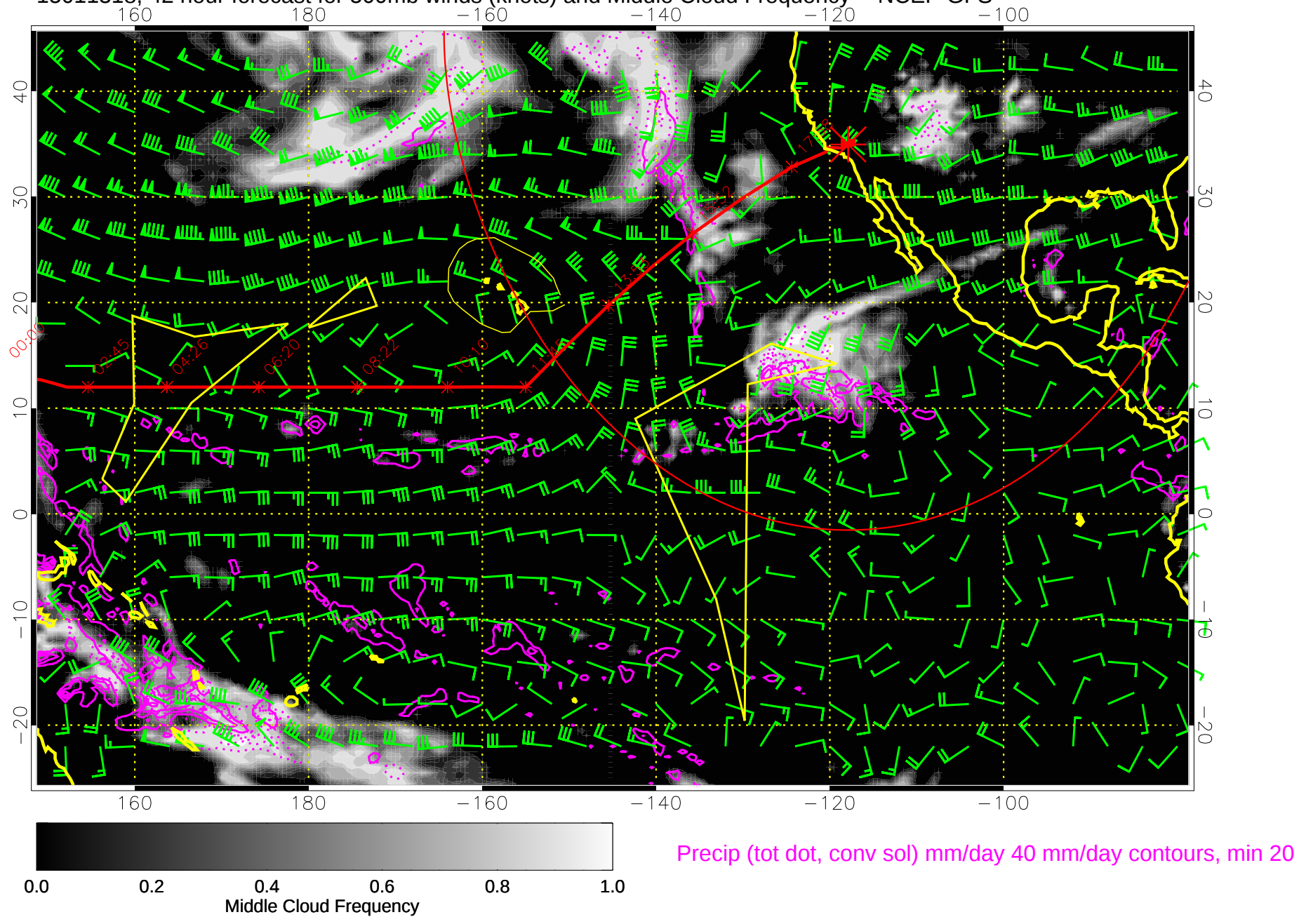
15011318, 42 hour forecast for 500mb winds (knots) and Middle Cloud Frequency -- NCEP GFS
