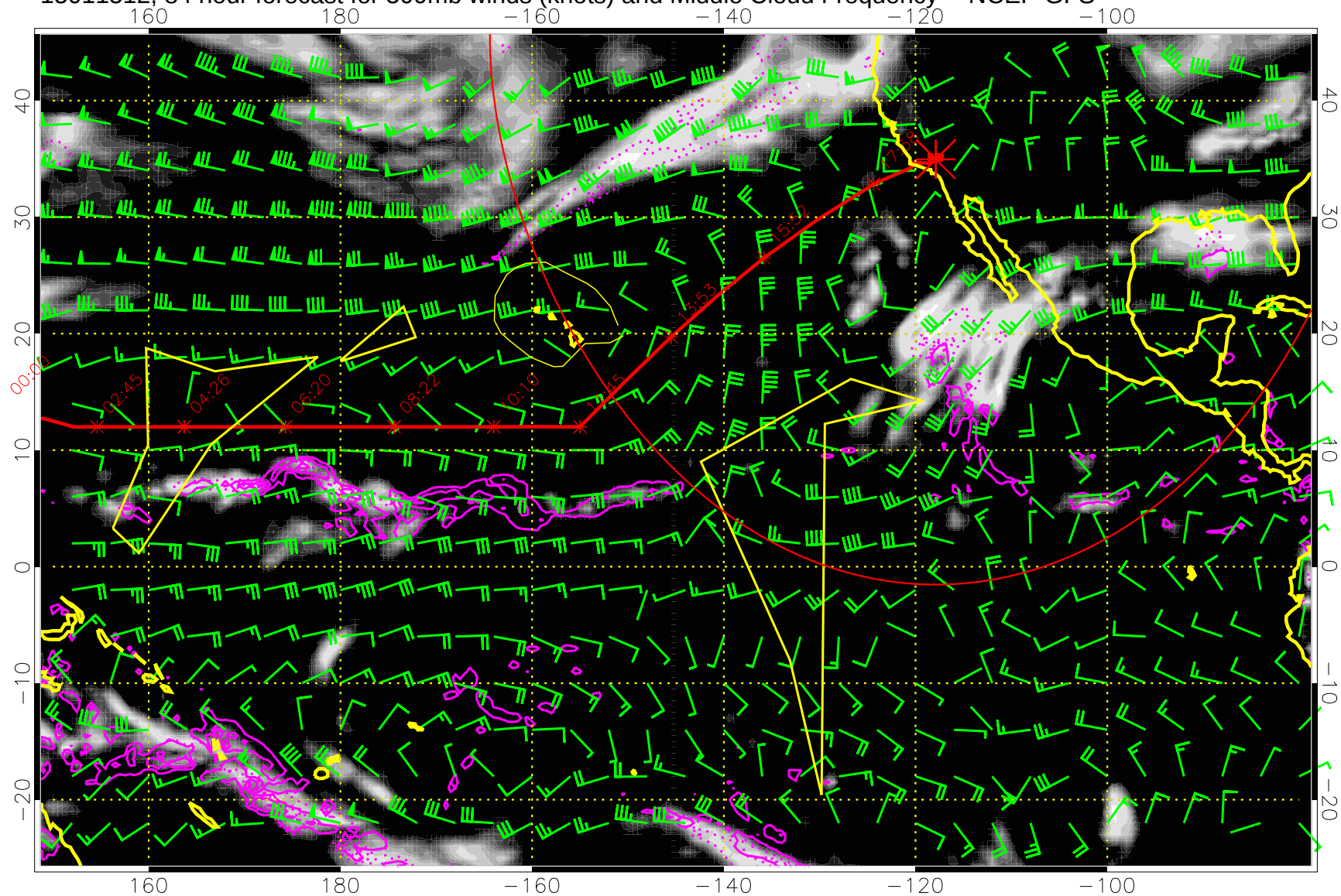
15011512, 84 hour forecast for 500mb winds (knots) and Middle Cloud Frequency -- NCEP GFS
