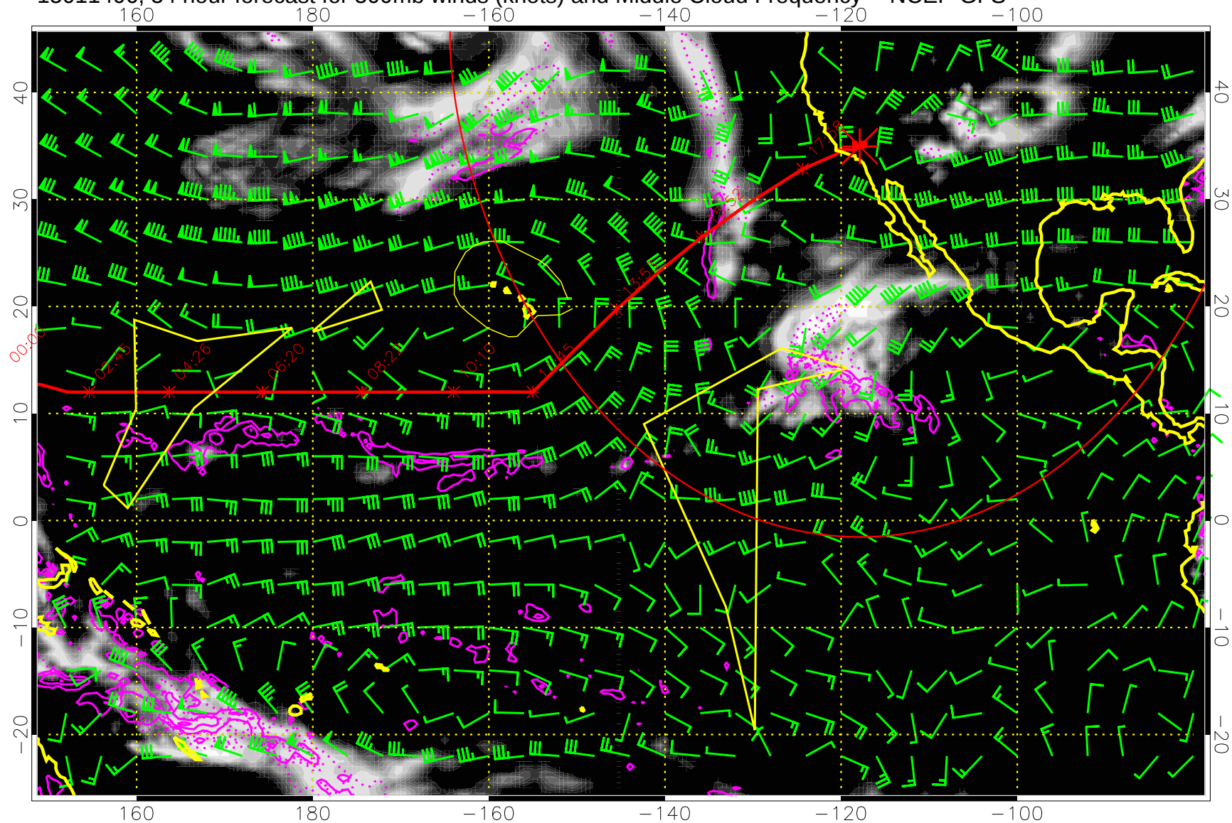
15011406, 54 hour forecast for 500mb winds (knots) and Middle Cloud Frequency -- NCEP GFS
