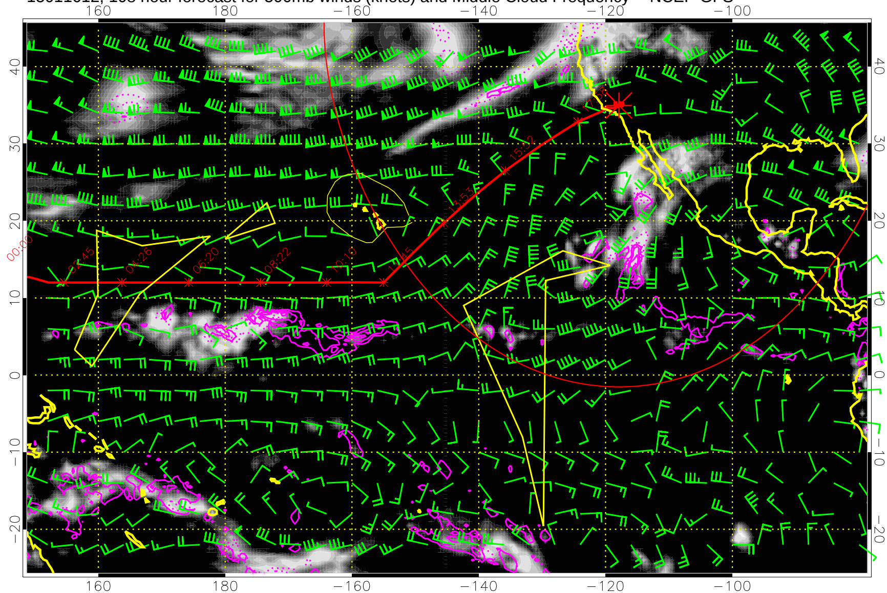
15011612, 108 hour forecast for 500mb winds (knots) and Middle Cloud Frequency -- NCEP GFS
