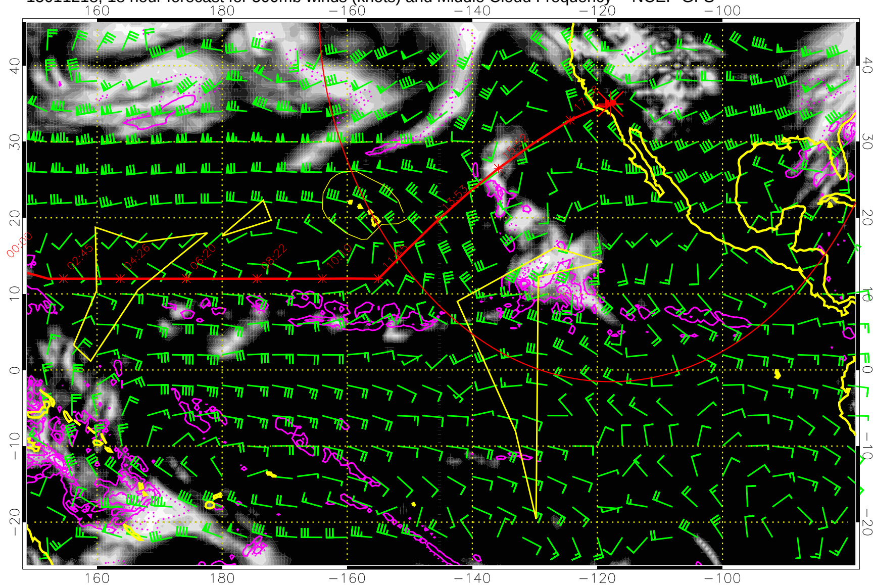
15011218, 18 hour forecast for 500mb winds (knots) and Middle Cloud Frequency -- NCEP GFS
