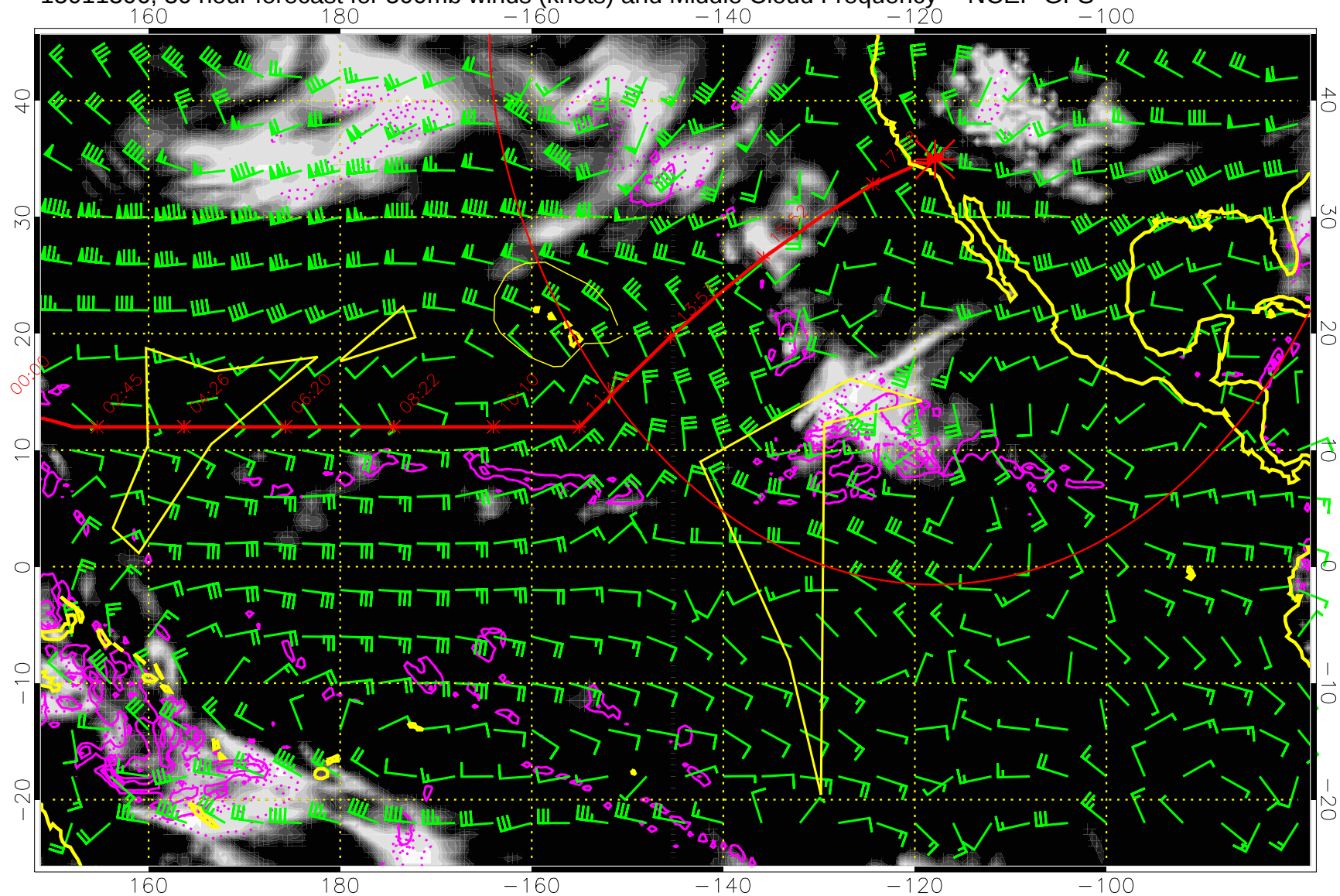
15011306, 30 hour forecast for 500mb winds (knots) and Middle Cloud Frequency -- NCEP GFS
