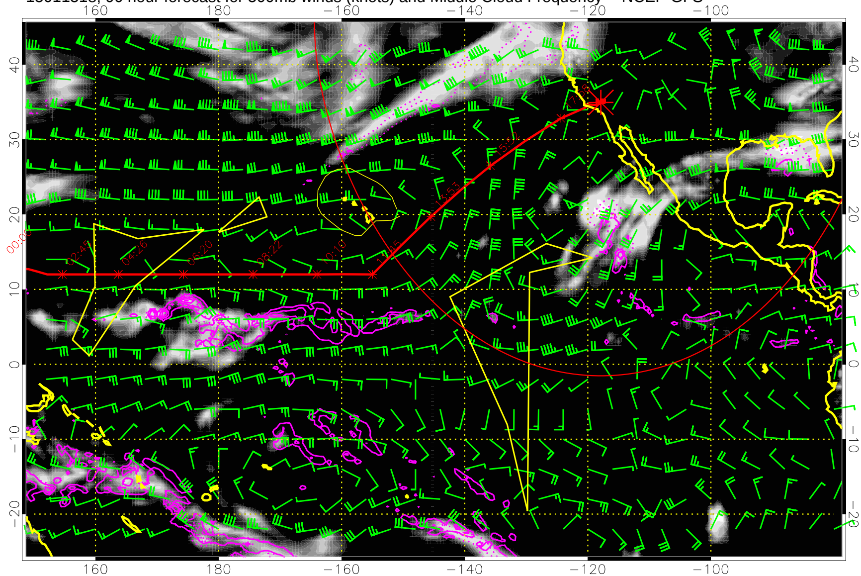
15011518, 90 hour forecast for 500mb winds (knots) and Middle Cloud Frequency -- NCEP GFS
