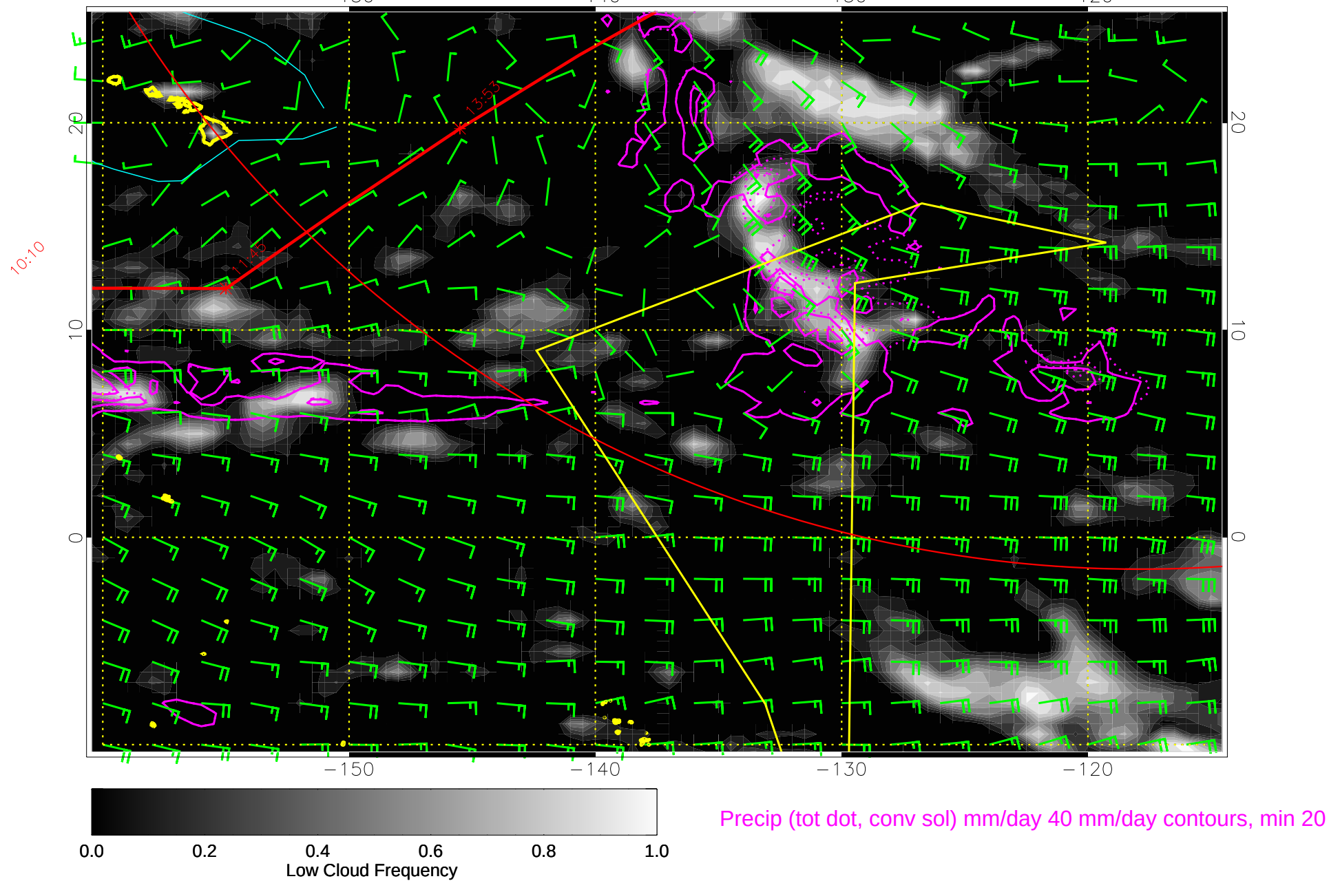
15011206, 6 hour forecast for 850mb winds (knots) and Low Cloud Frequency -- NCEP GFS
