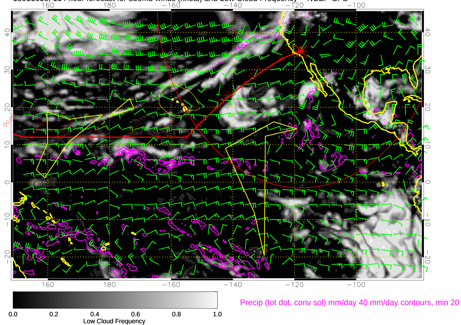
15011618, 114 hour forecast for 850mb winds (knots) and Low Cloud Frequency -- NCEP GFS
