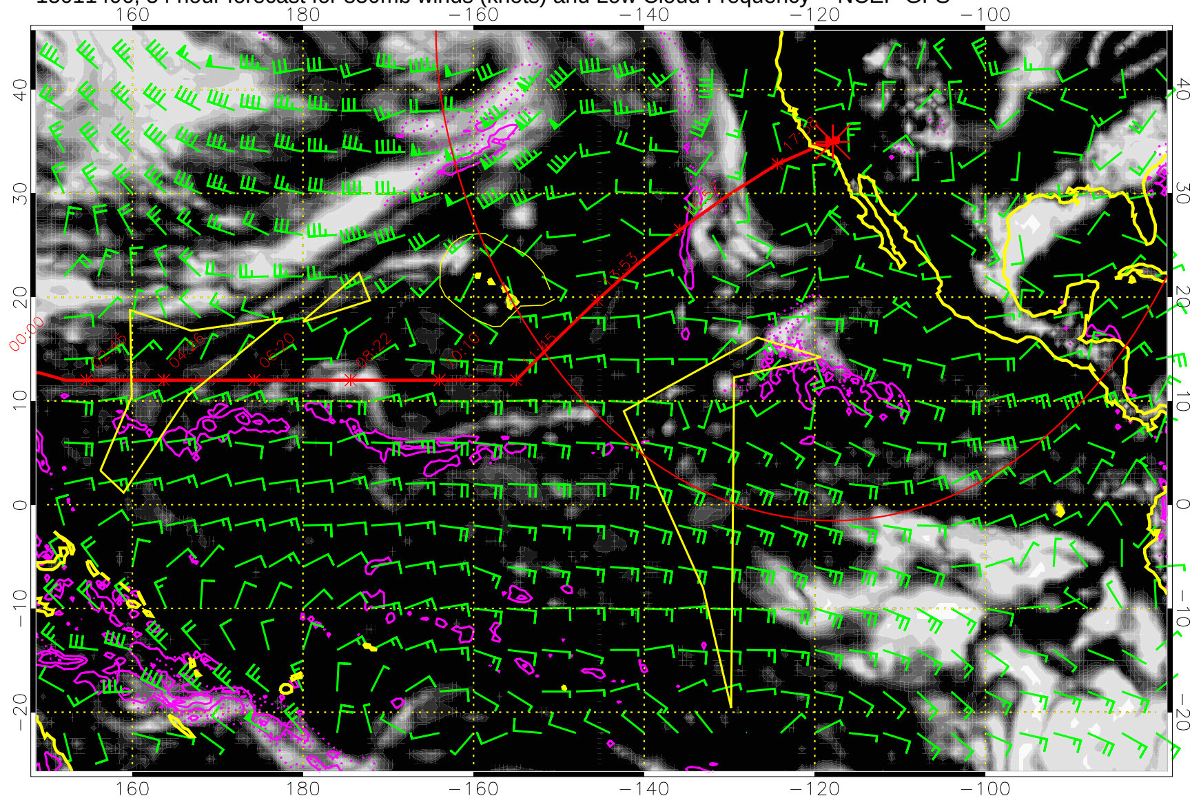
15011406, 54 hour forecast for 850mb winds (knots) and Low Cloud Frequency -- NCEP GFS
