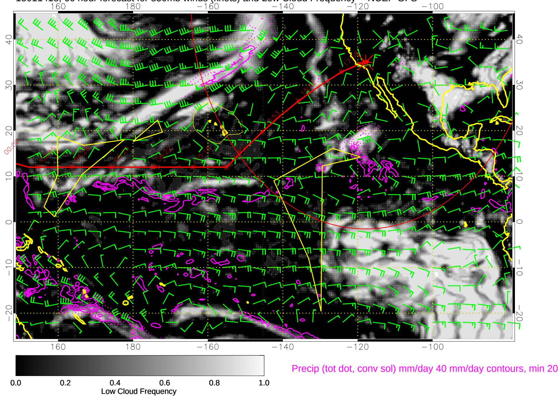
15011418, 66 hour forecast for 850mb winds (knots) and Low Cloud Frequency -- NCEP GFS
