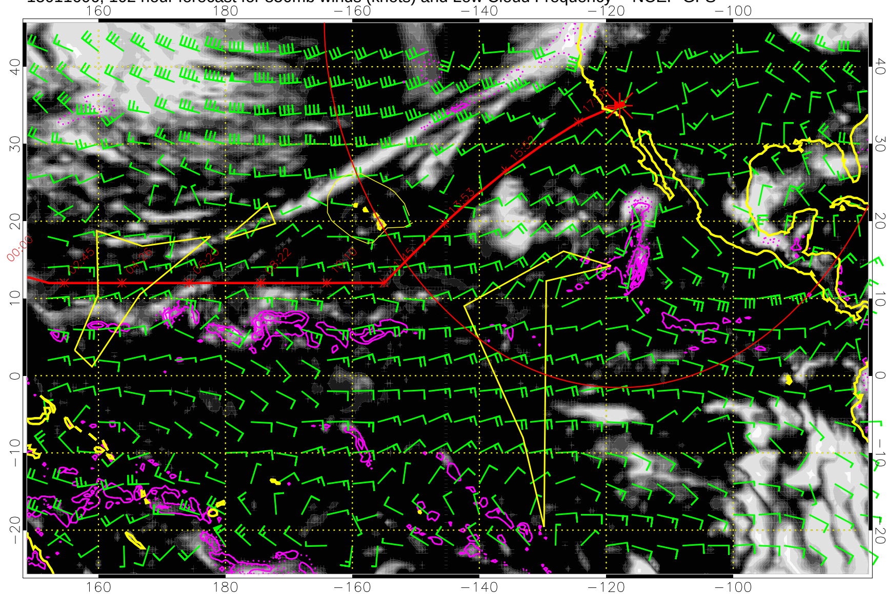
15011606, 102 hour forecast for 850mb winds (knots) and Low Cloud Frequency -- NCEP GFS
