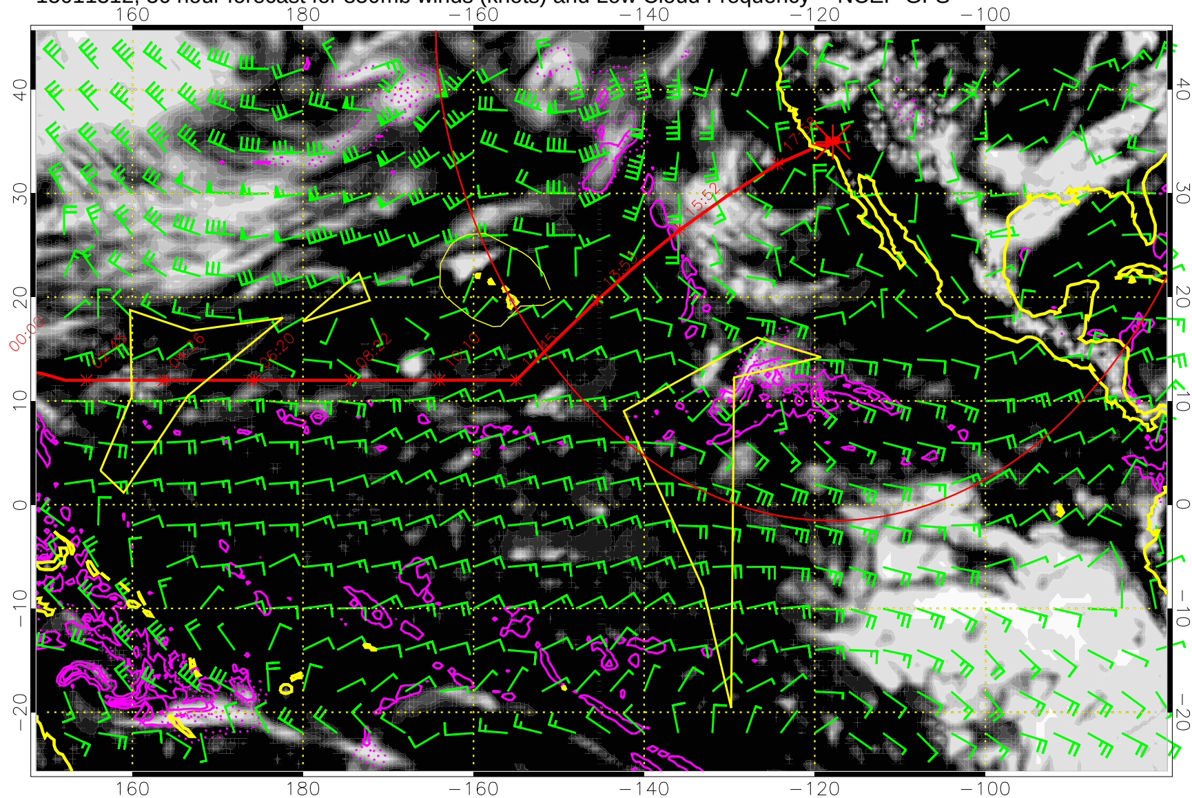
15011312, 36 hour forecast for 850mb winds (knots) and Low Cloud Frequency -- NCEP GFS
