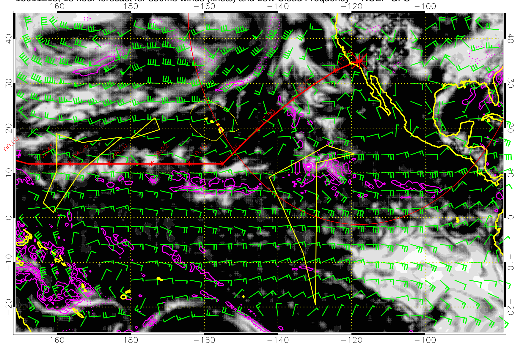
15011218, 18 hour forecast for 850mb winds (knots) and Low Cloud Frequency -- NCEP GFS
