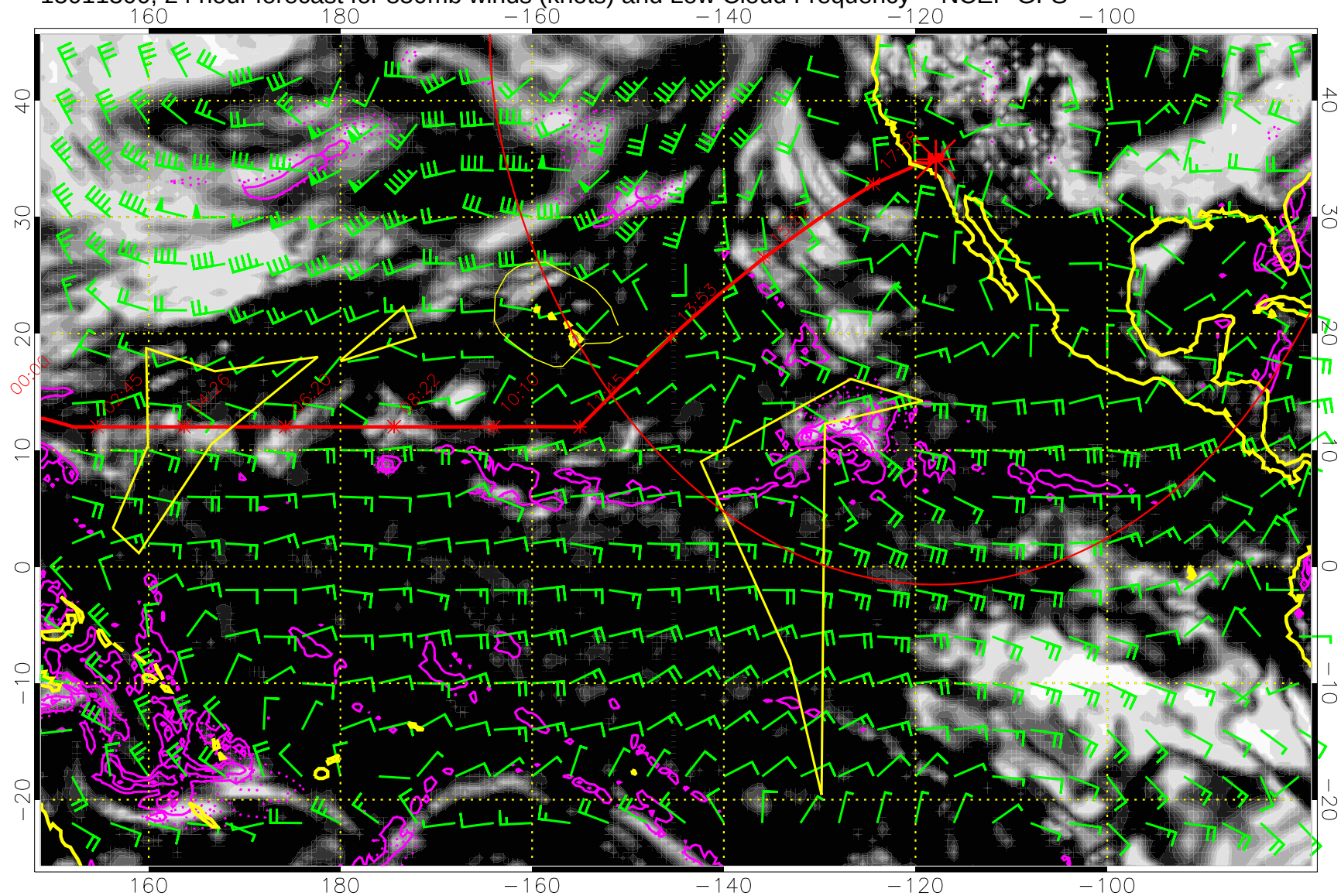
15011300, 24 hour forecast for 850mb winds (knots) and Low Cloud Frequency -- NCEP GFS
