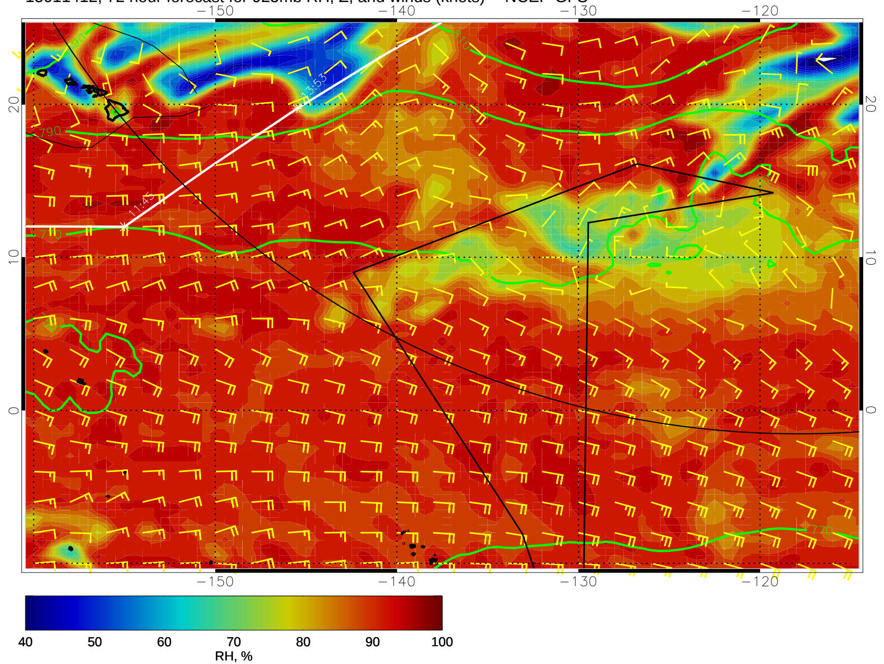
15011412, 72 hour forecast for 925mb RH, Z, and winds (knots) -- NCEP GFS
