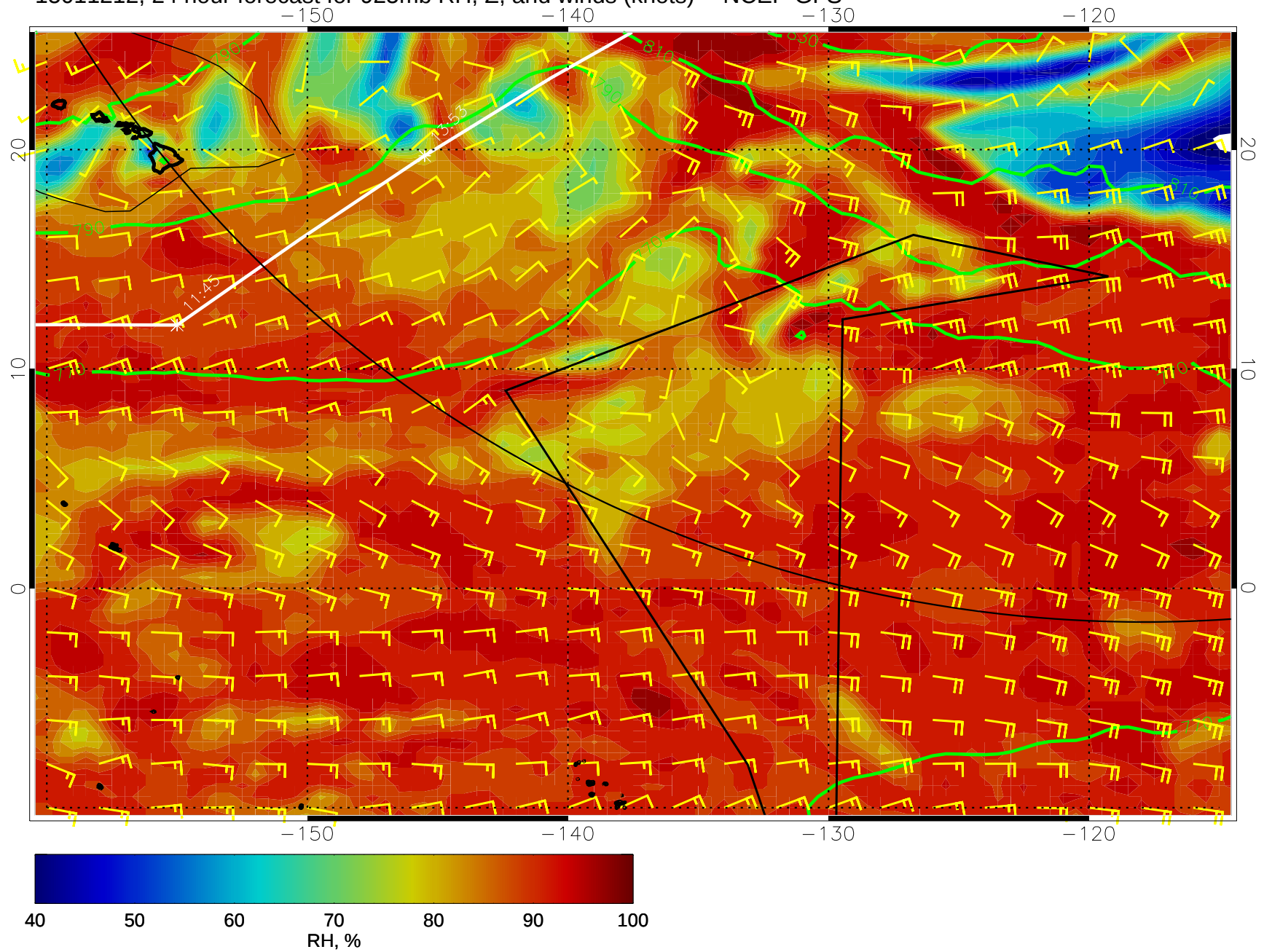
15011212, 24 hour forecast for 925mb RH, Z, and winds (knots) -- NCEP GFS
