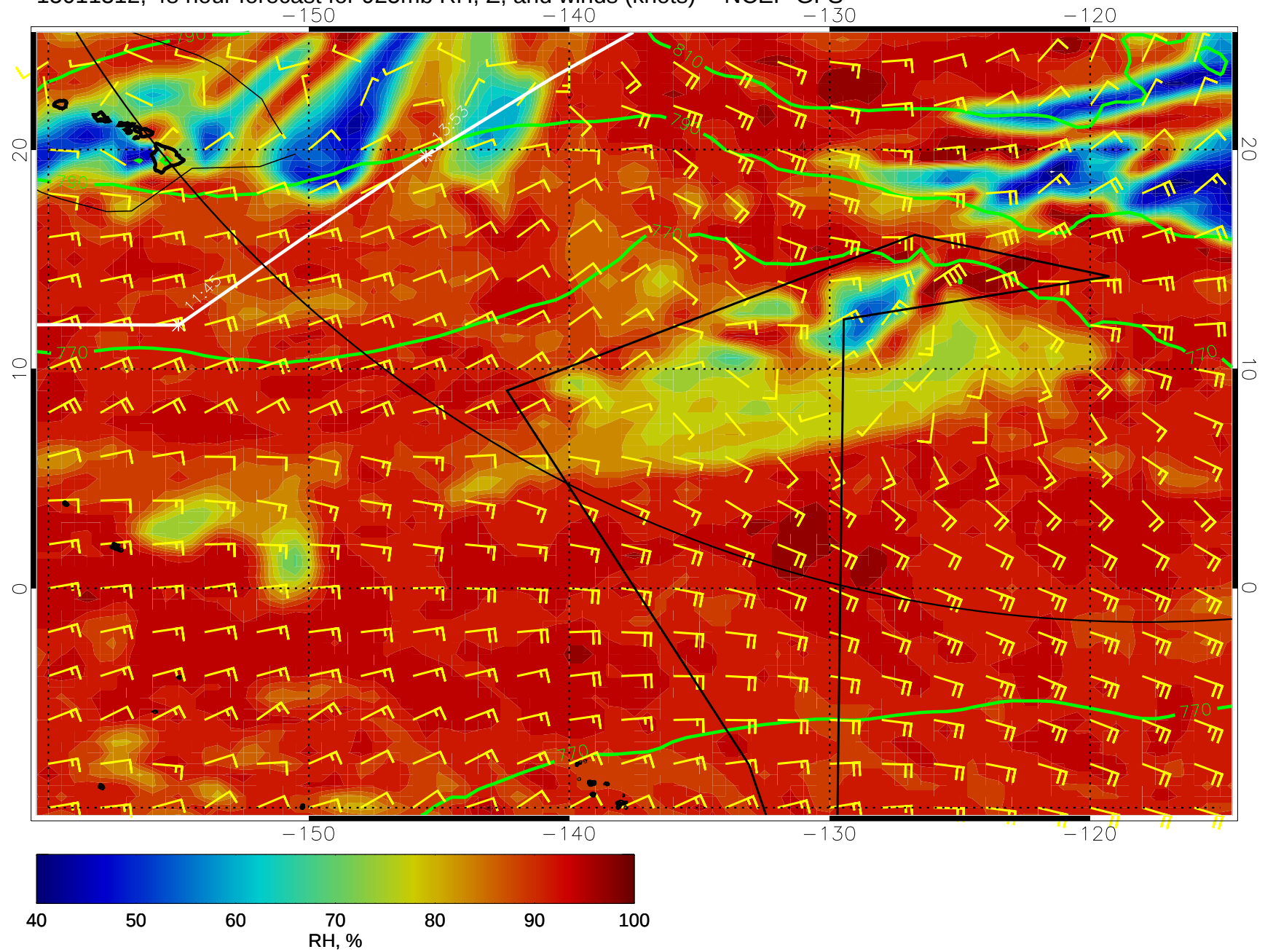
15011312, 48 hour forecast for 925mb RH, Z, and winds (knots) -- NCEP GFS
