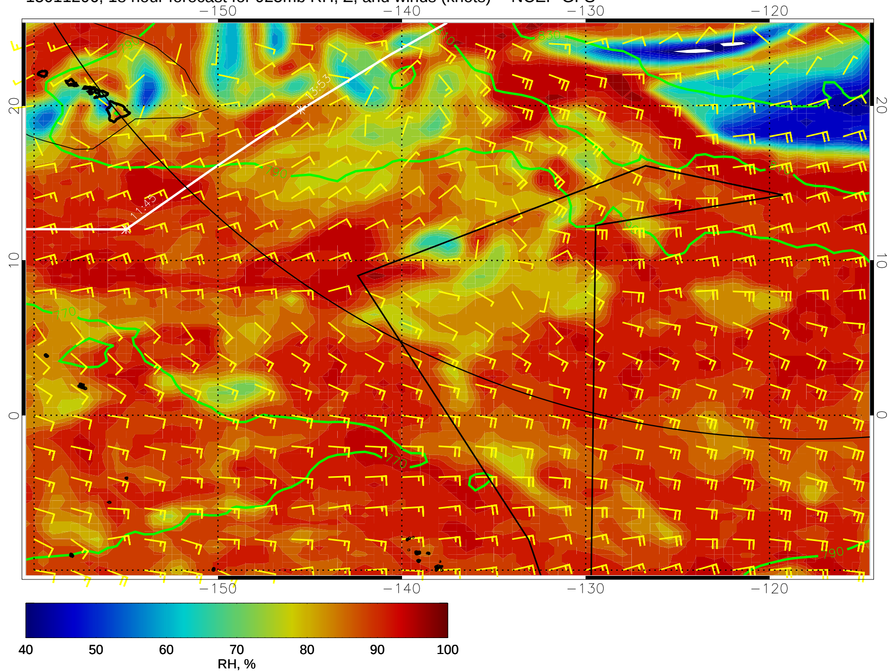
15011206, 18 hour forecast for 925mb RH, Z, and winds (knots) -- NCEP GFS
