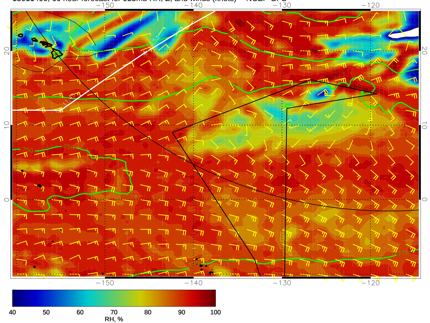
15011400, 60 hour forecast for 925mb RH, Z, and winds (knots) -- NCEP GFS
