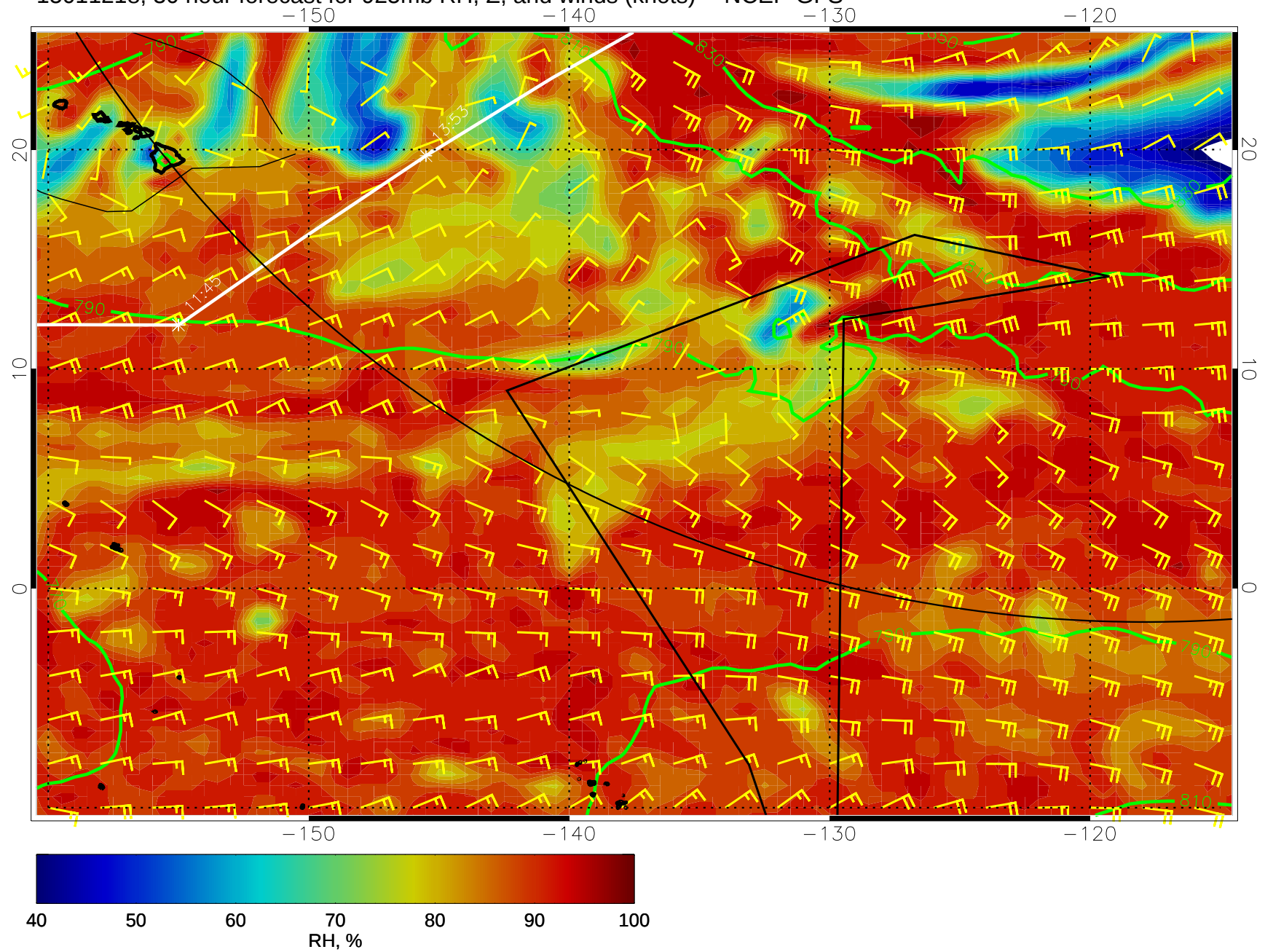
15011218, 30 hour forecast for 925mb RH, Z, and winds (knots) -- NCEP GFS
