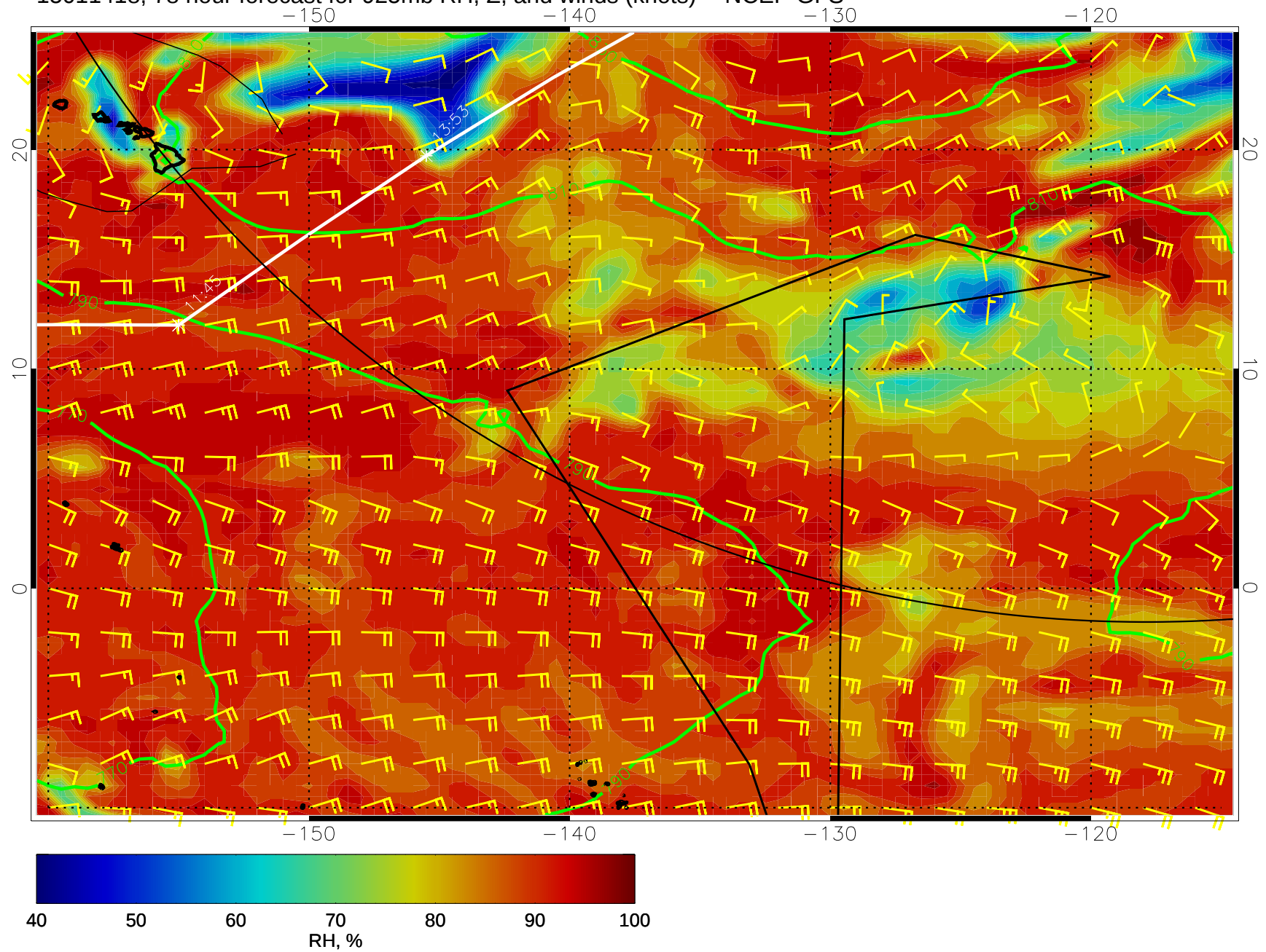
15011418, 78 hour forecast for 925mb RH, Z, and winds (knots) -- NCEP GFS
