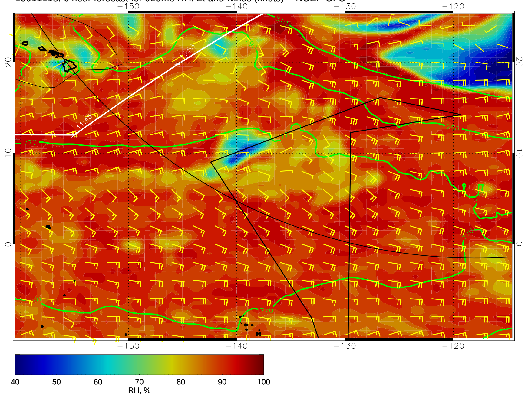
15011118, 6 hour forecast for 925mb RH, Z, and winds (knots) -- NCEP GFS
