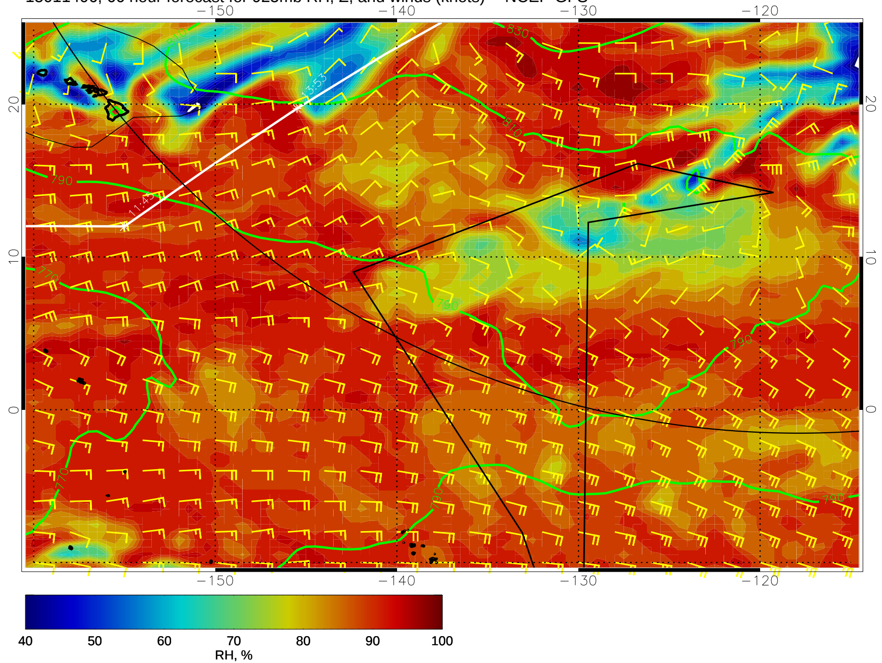
15011406, 66 hour forecast for 925mb RH, Z, and winds (knots) -- NCEP GFS
