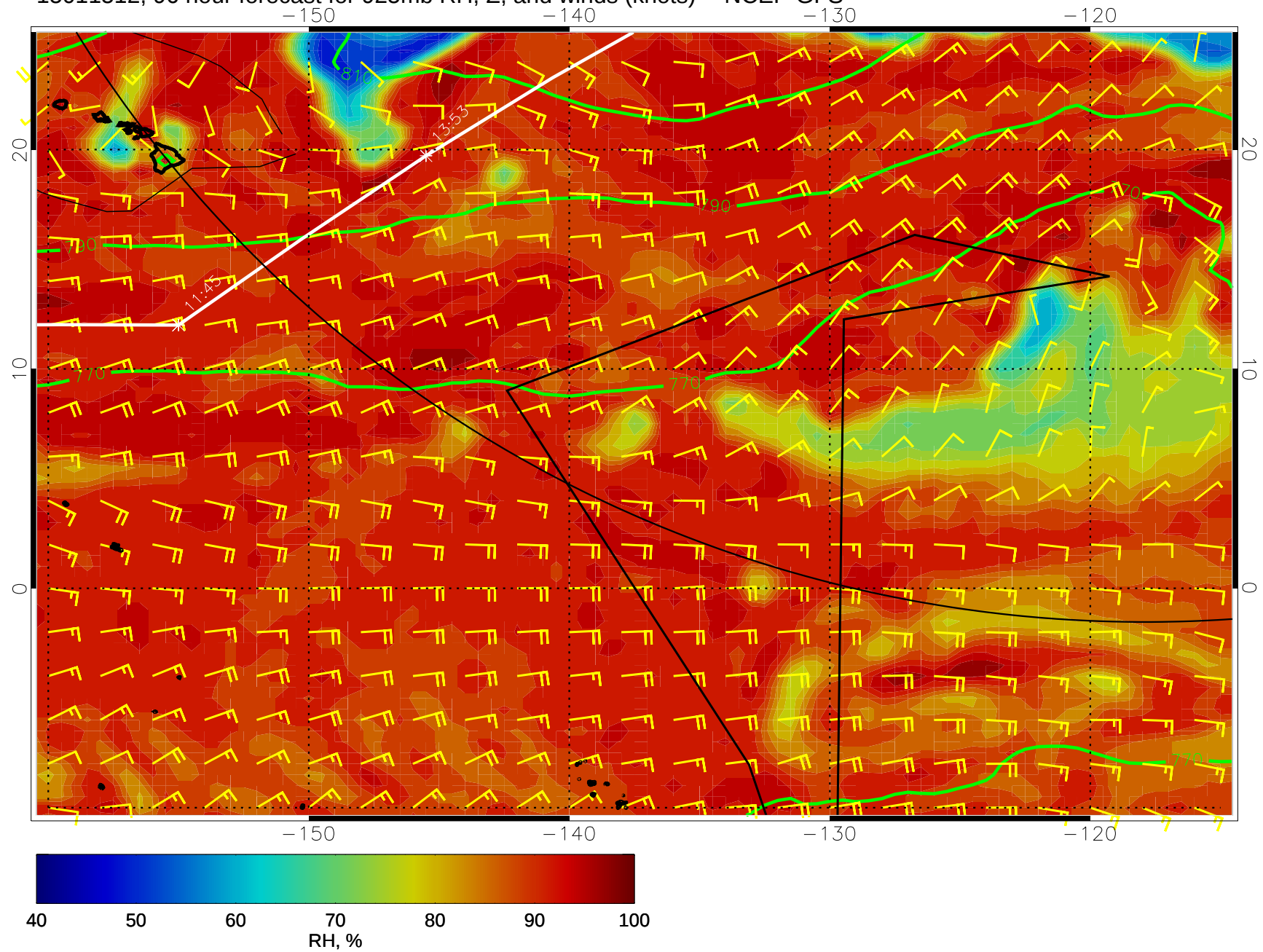
15011512, 96 hour forecast for 925mb RH, Z, and winds (knots) -- NCEP GFS
