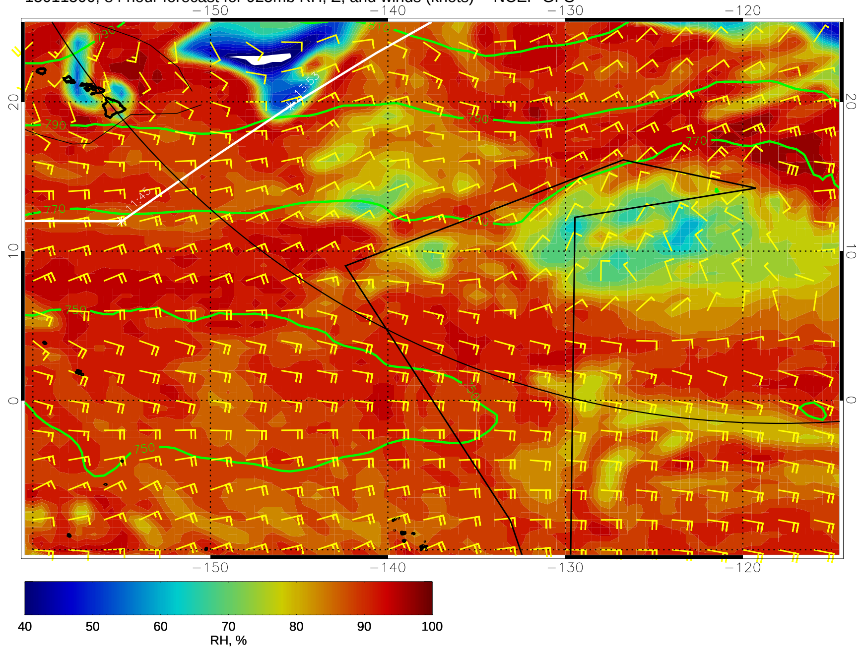
15011500, 84 hour forecast for 925mb RH, Z, and winds (knots) -- NCEP GFS
