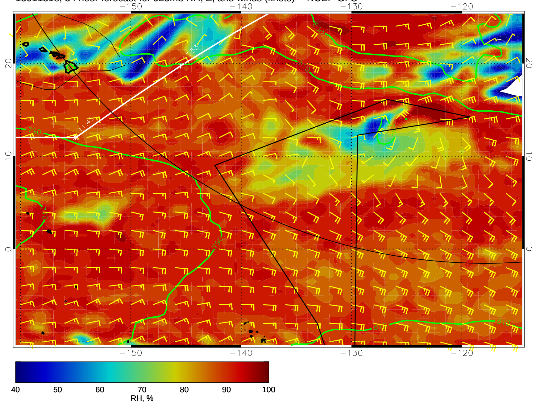
15011318, 54 hour forecast for 925mb RH, Z, and winds (knots) -- NCEP GFS
