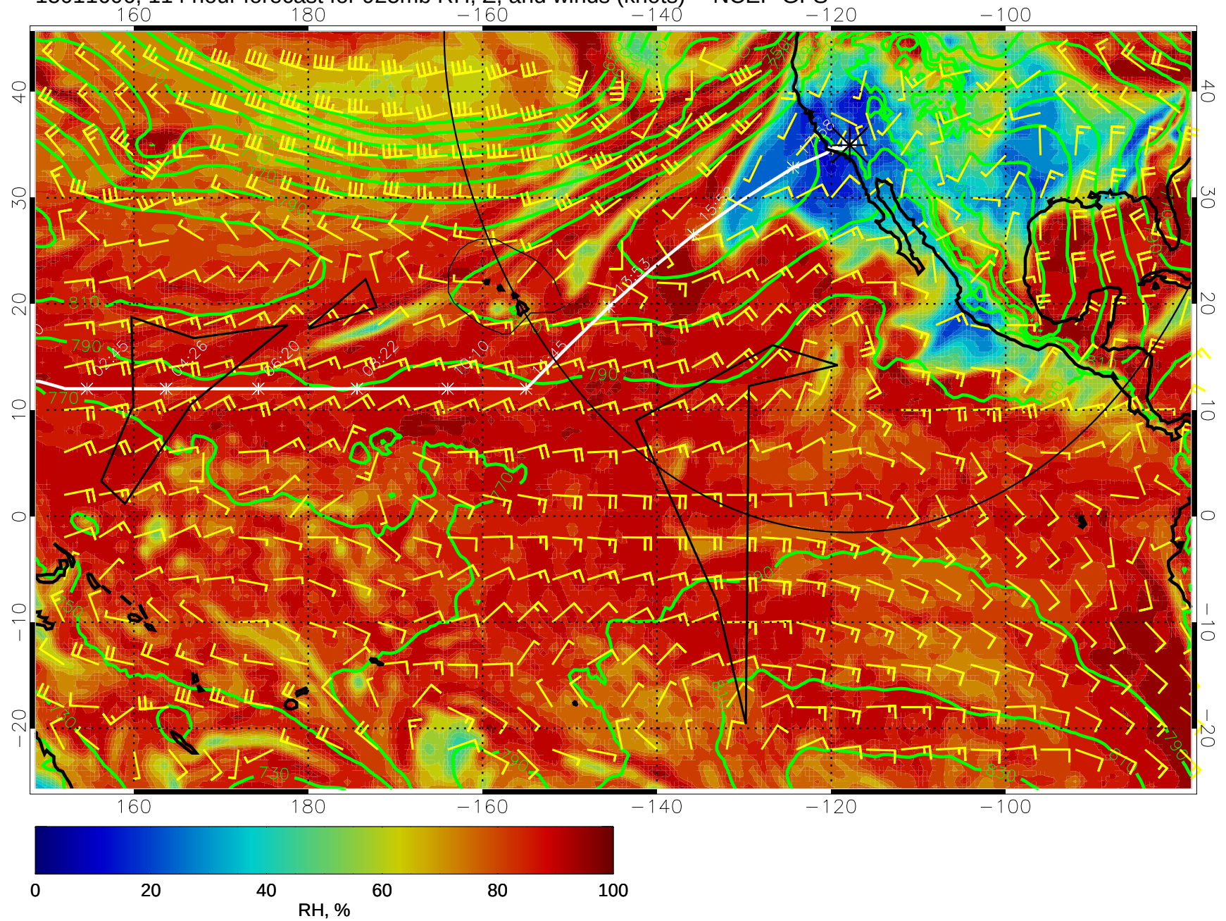
15011606, 114 hour forecast for 925mb RH, Z, and winds (knots) -- NCEP GFS
