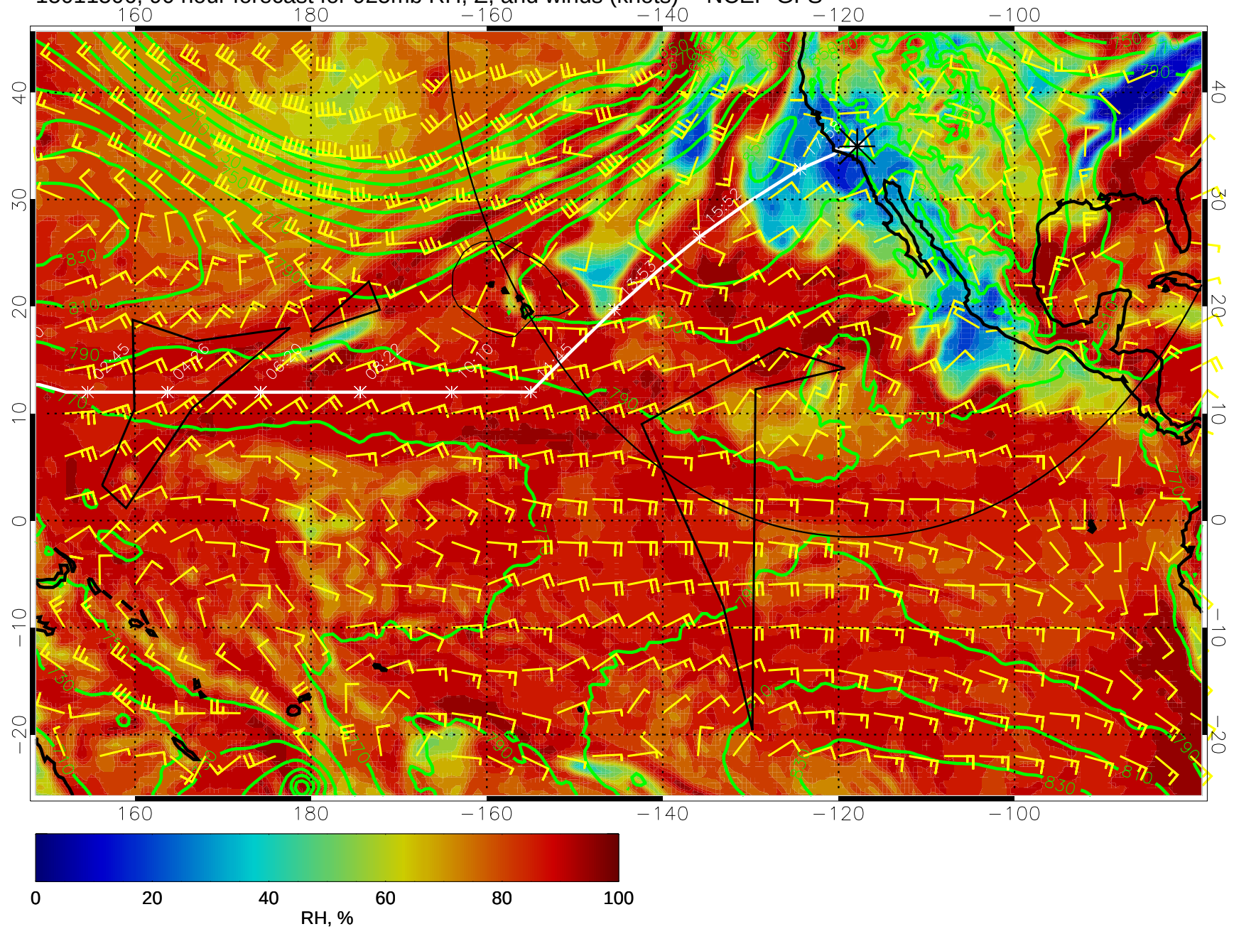
15011506, 90 hour forecast for 925mb RH, Z, and winds (knots) -- NCEP GFS
