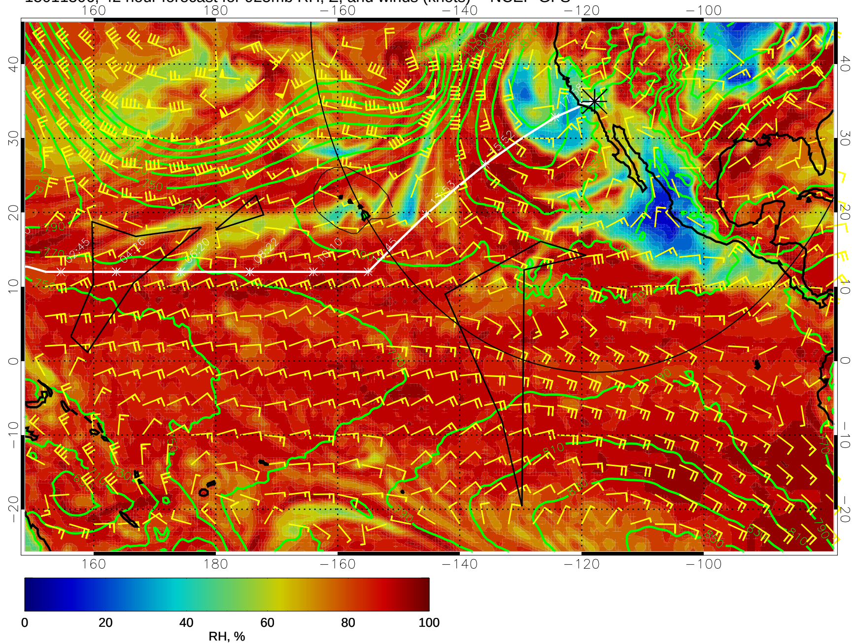
15011306, 42 hour forecast for 925mb RH, Z, and winds (knots) -- NCEP GFS
