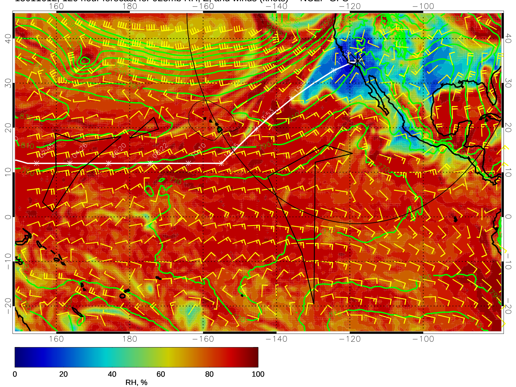
15011612, 120 hour forecast for 925mb RH, Z, and winds (knots) -- NCEP GFS
