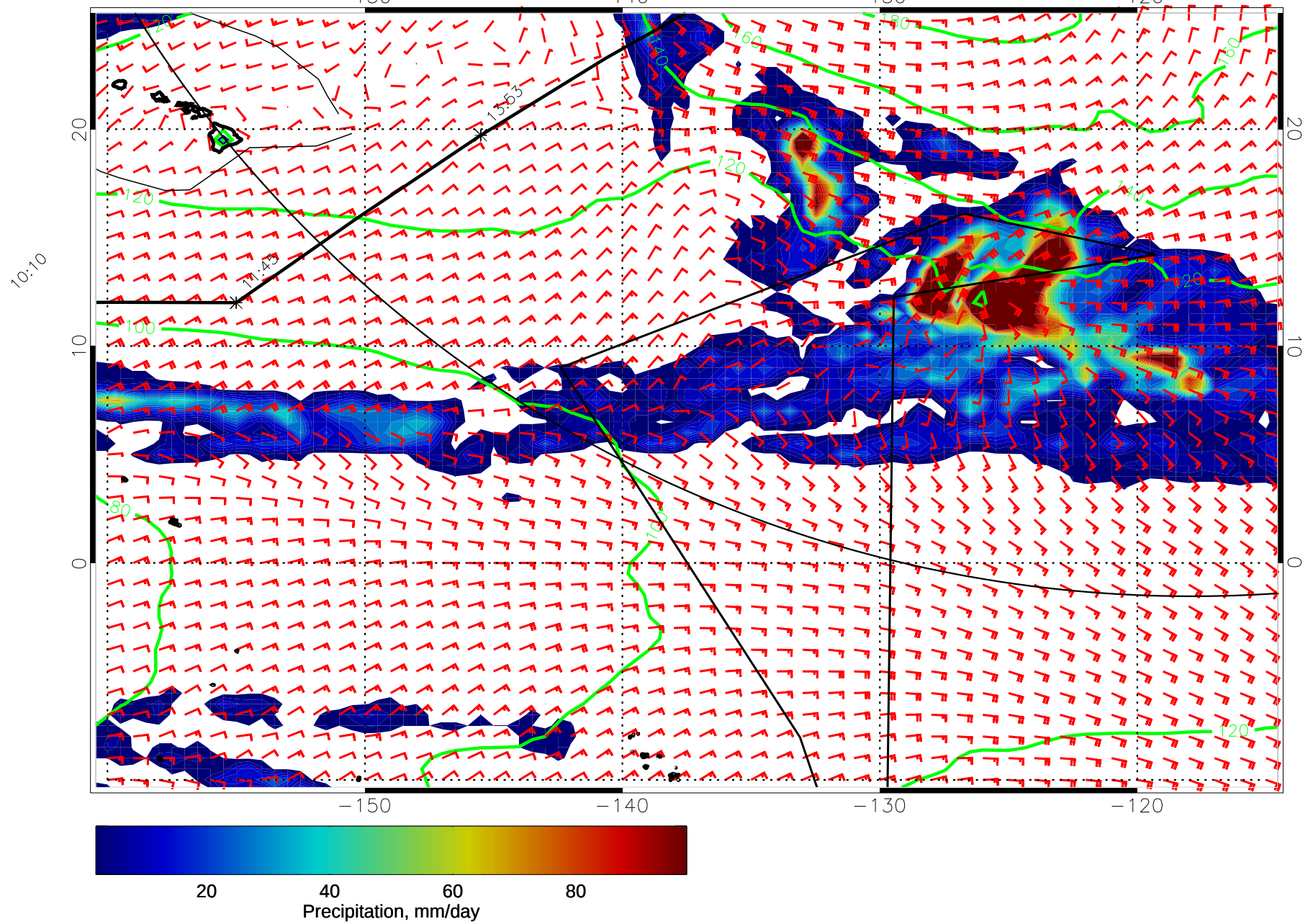
15011306, 42 hour forecast for precip, 1000mb Z, and winds (knots) -- NCEP GFS
