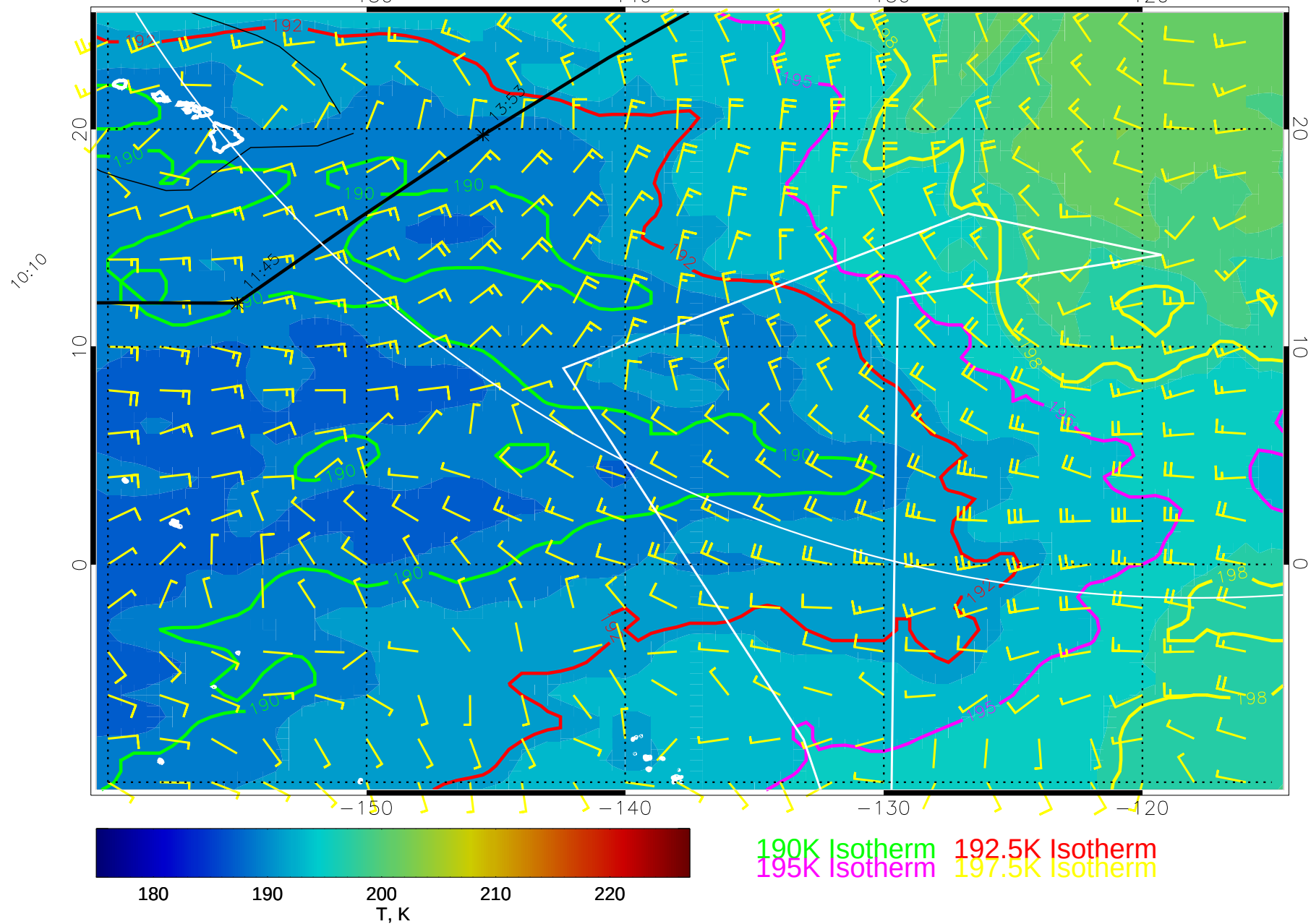
15011612, 120 hour forecast for 70mb T and winds (knots) -- NCEP GFS
