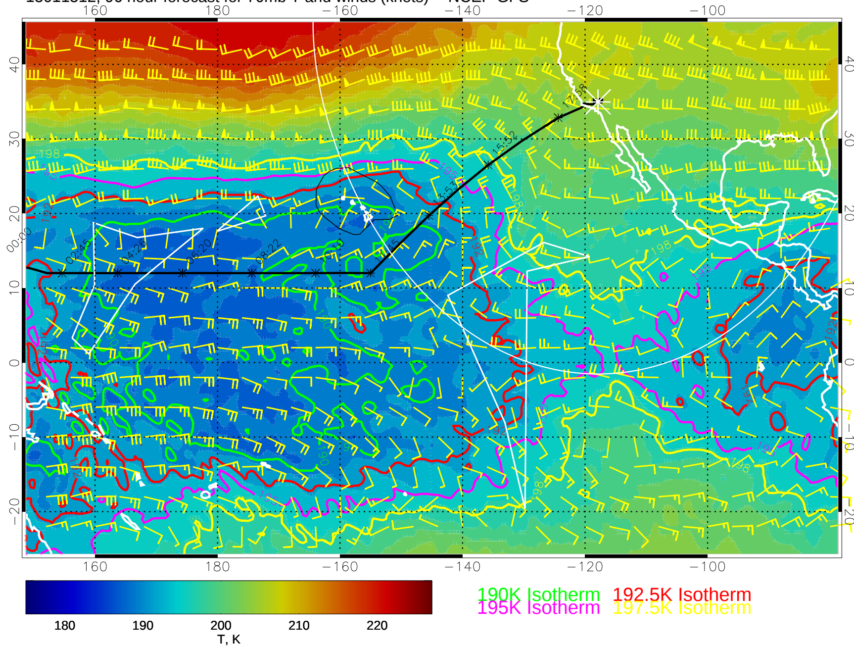
15011512, 96 hour forecast for 70mb T and winds (knots) -- NCEP GFS
