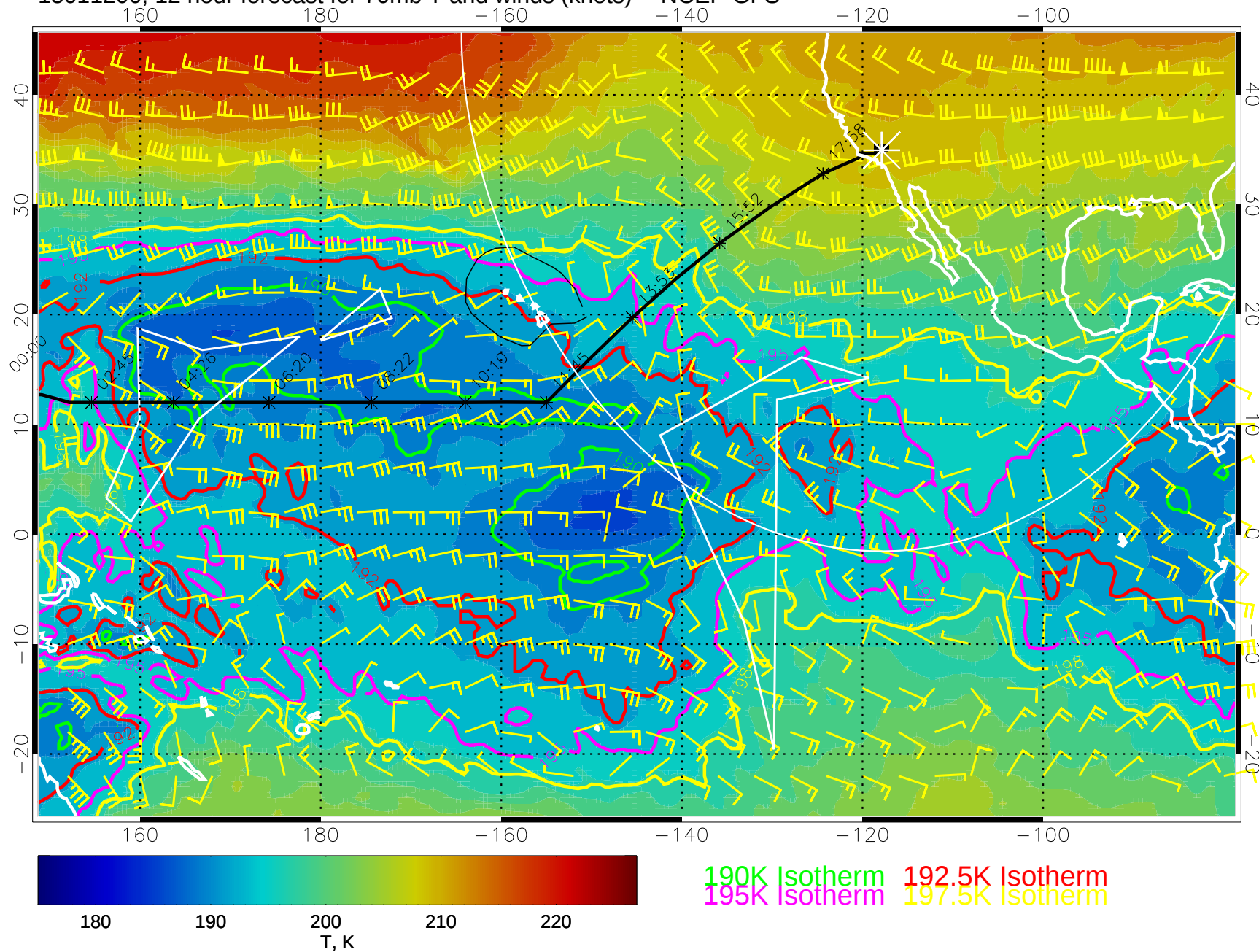
15011200, 12 hour forecast for 70mb T and winds (knots) -- NCEP GFS
