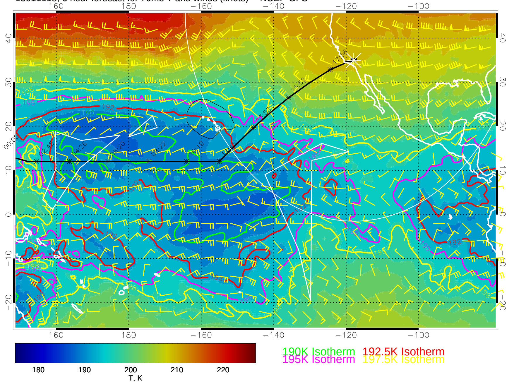
15011118, 6 hour forecast for 70mb T and winds (knots) -- NCEP GFS
