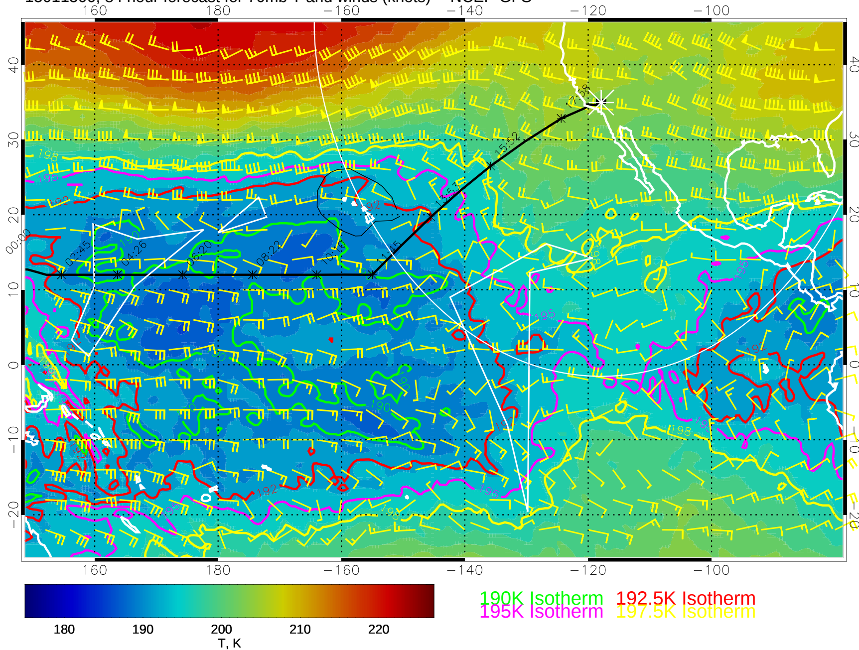
15011500, 84 hour forecast for 70mb T and winds (knots) -- NCEP GFS
