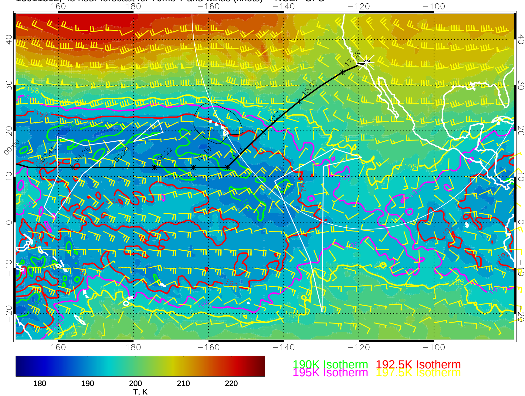
15011312, 48 hour forecast for 70mb T and winds (knots) -- NCEP GFS
