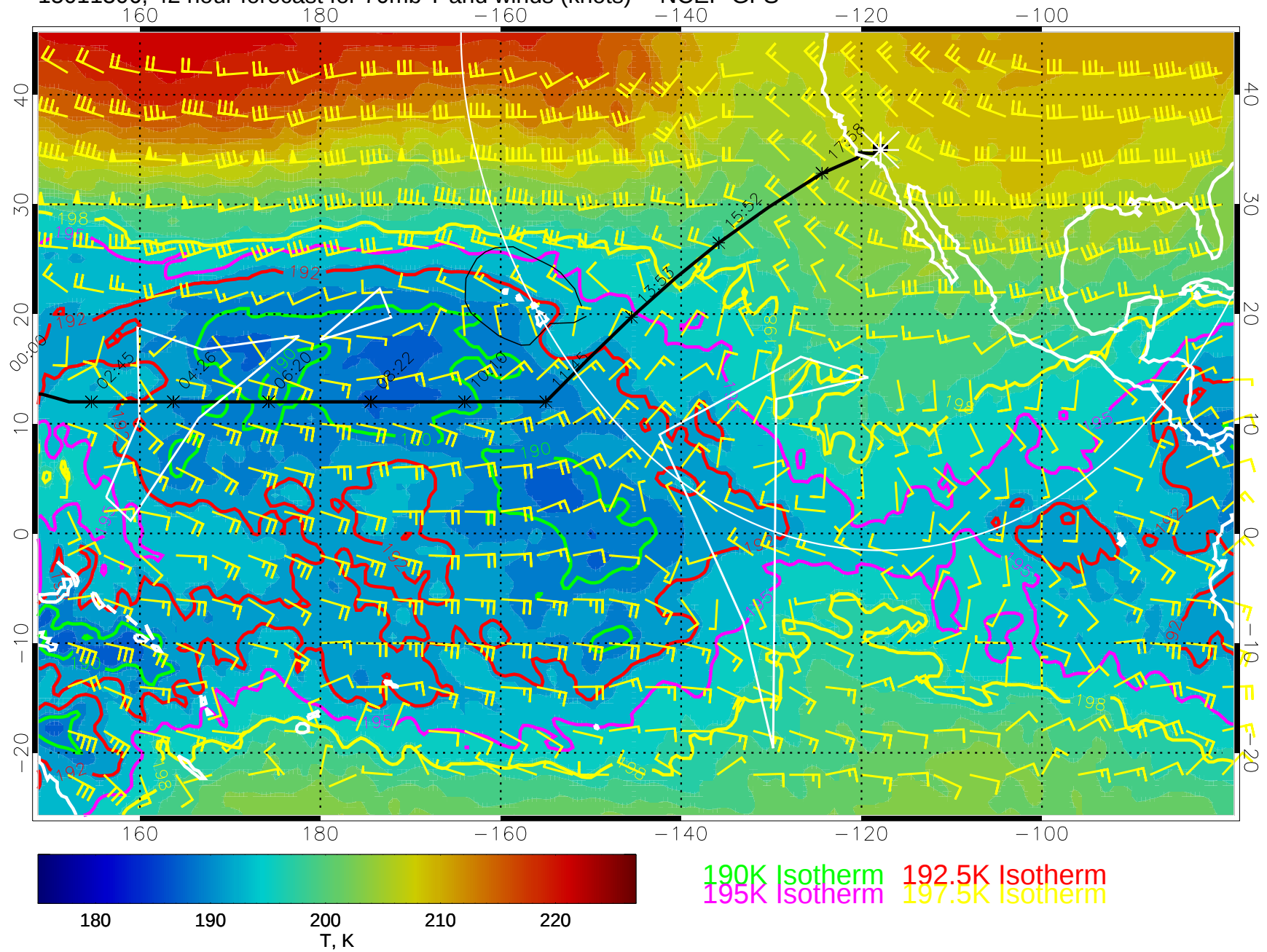
15011306, 42 hour forecast for 70mb T and winds (knots) -- NCEP GFS
