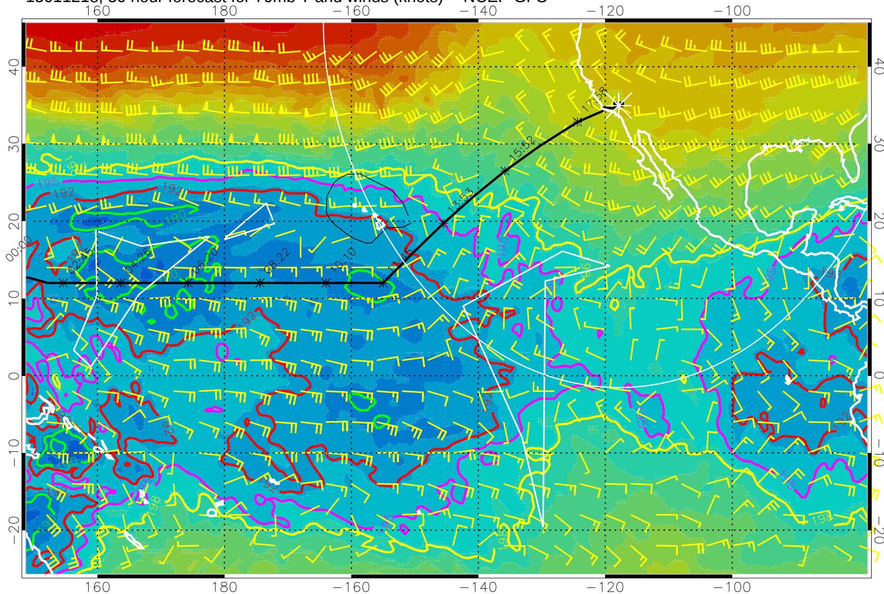
15011218, 30 hour forecast for 70mb T and winds (knots) -- NCEP GFS
