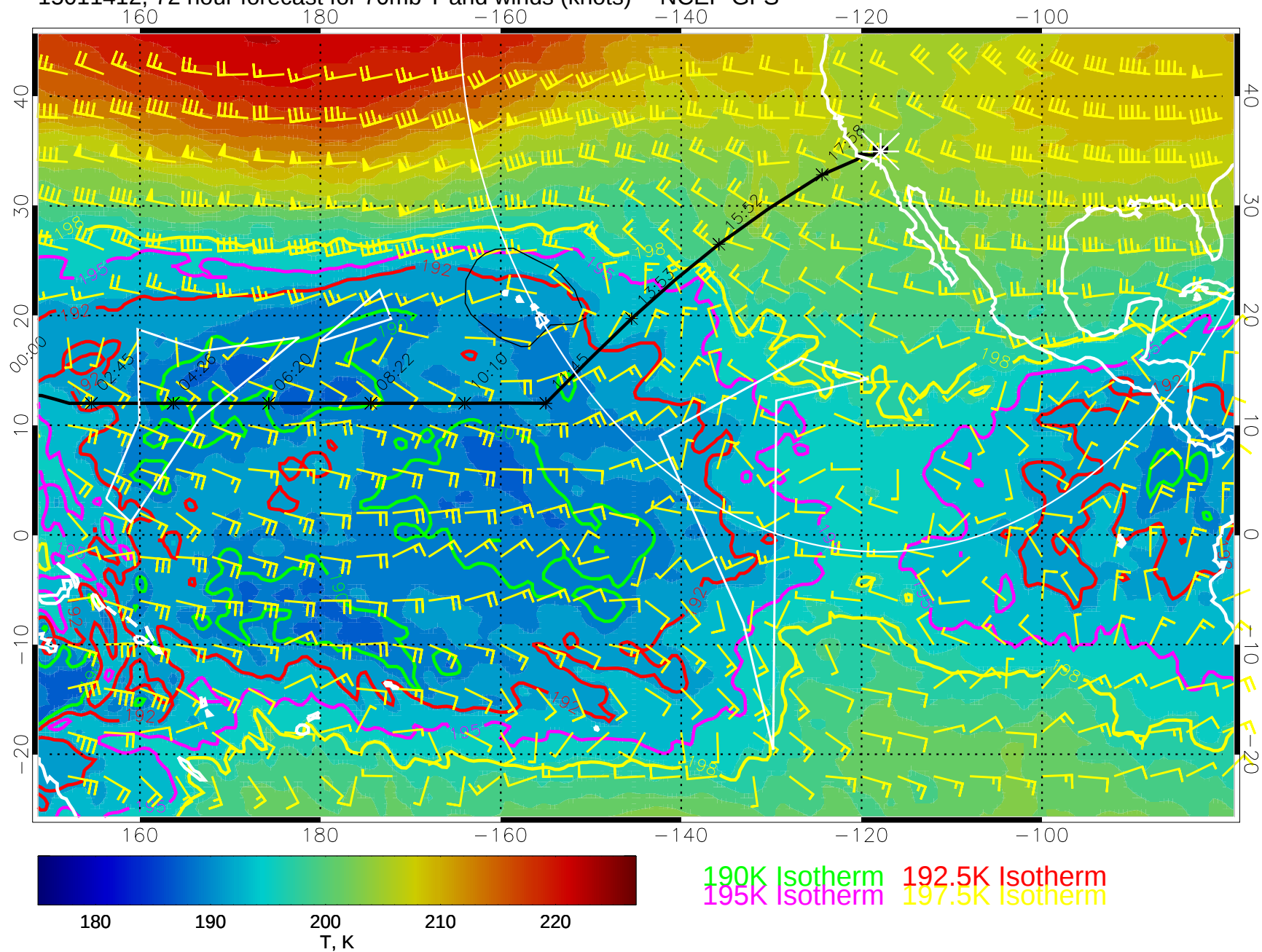
15011412, 72 hour forecast for 70mb T and winds (knots) -- NCEP GFS
