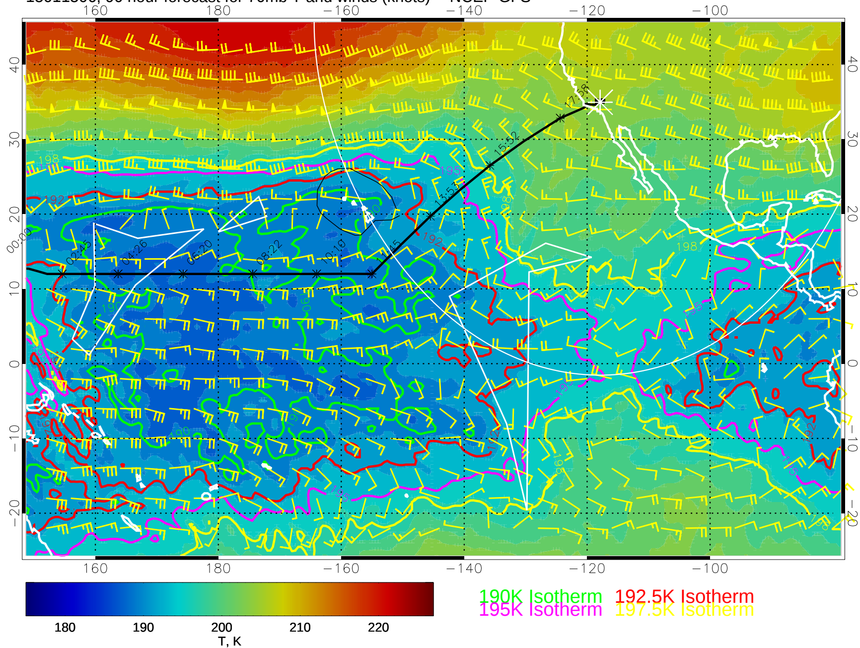
15011506, 90 hour forecast for 70mb T and winds (knots) -- NCEP GFS
