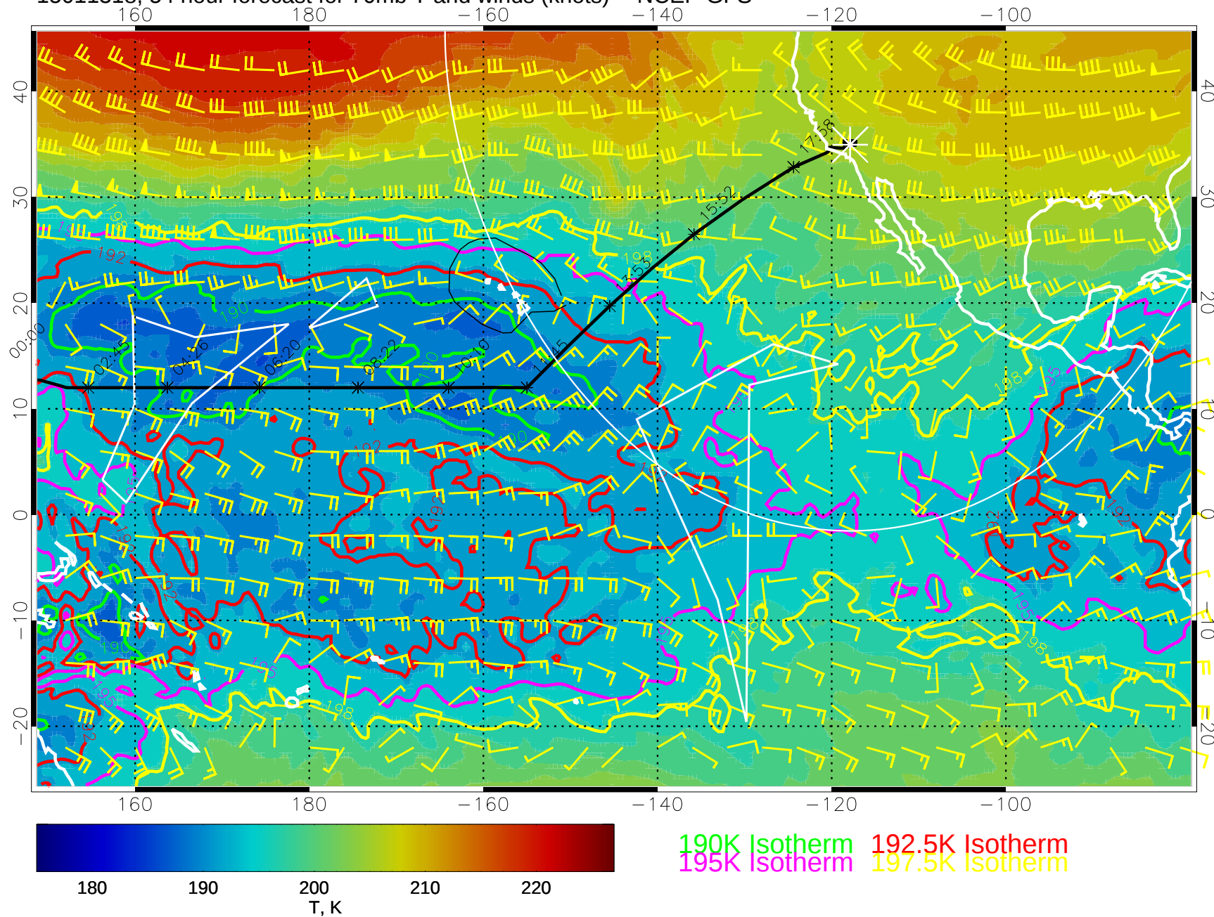
15011318, 54 hour forecast for 70mb T and winds (knots) -- NCEP GFS
