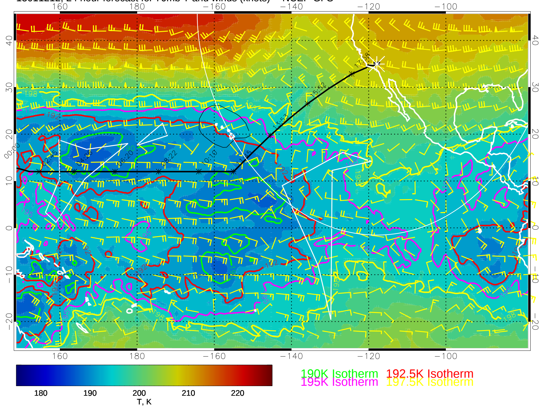
15011212, 24 hour forecast for 70mb T and winds (knots) -- NCEP GFS
