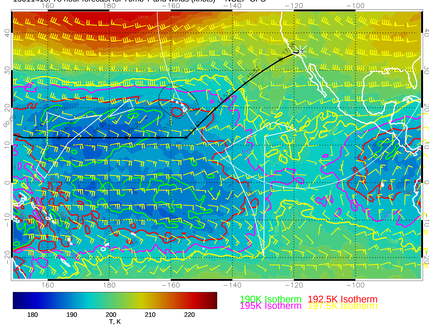
15011418, 78 hour forecast for 70mb T and winds (knots) -- NCEP GFS
