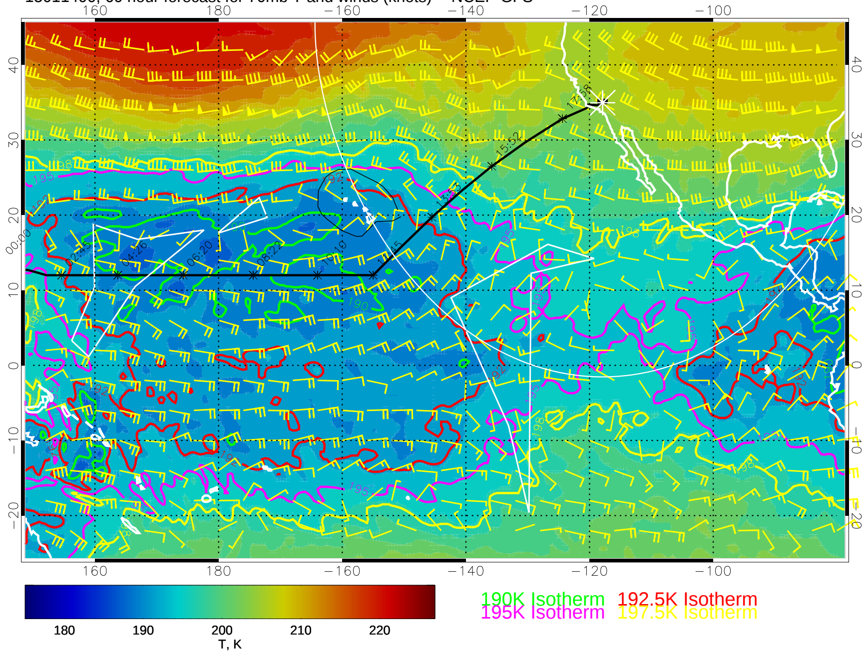
15011400, 60 hour forecast for 70mb T and winds (knots) -- NCEP GFS
