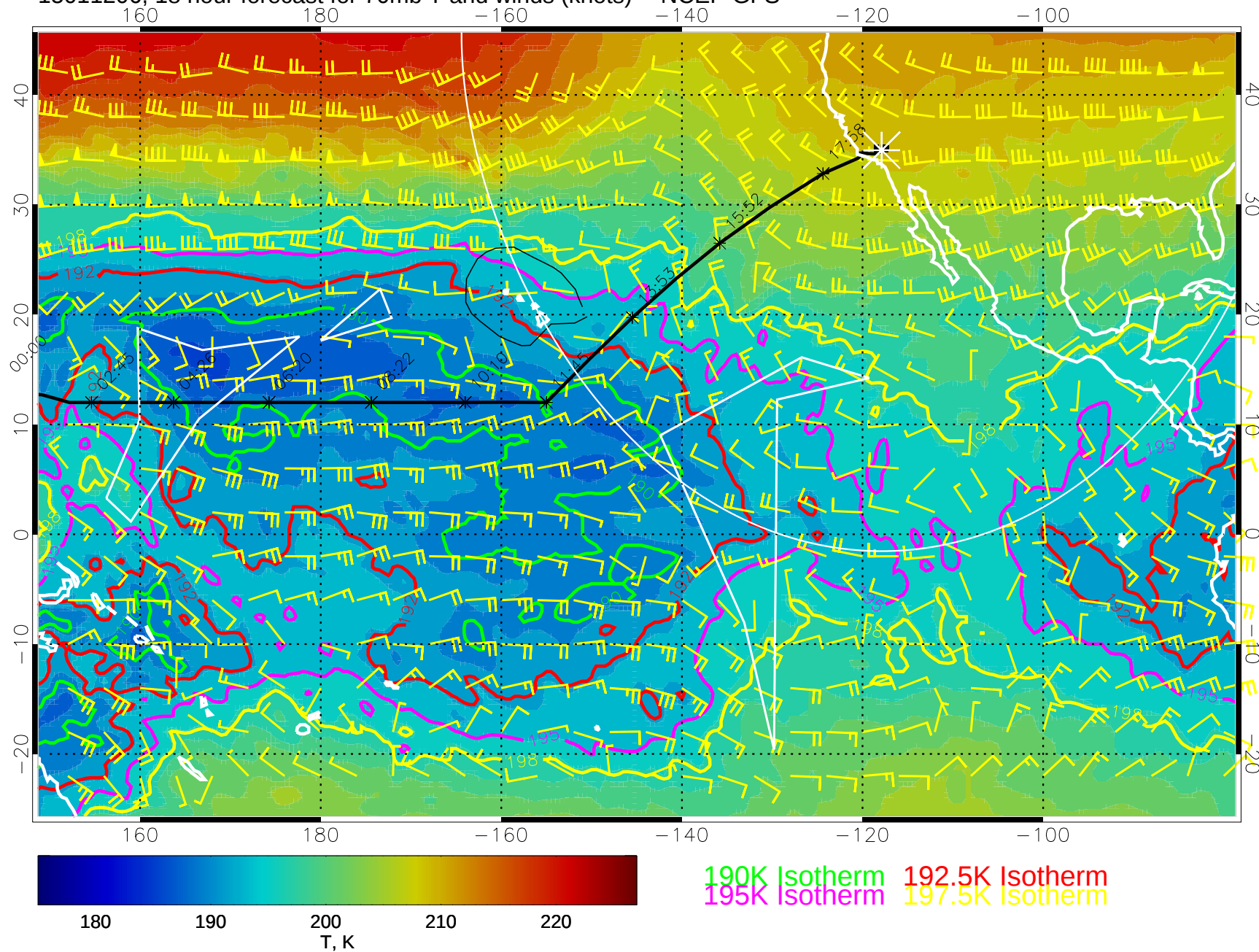
15011206, 18 hour forecast for 70mb T and winds (knots) -- NCEP GFS
