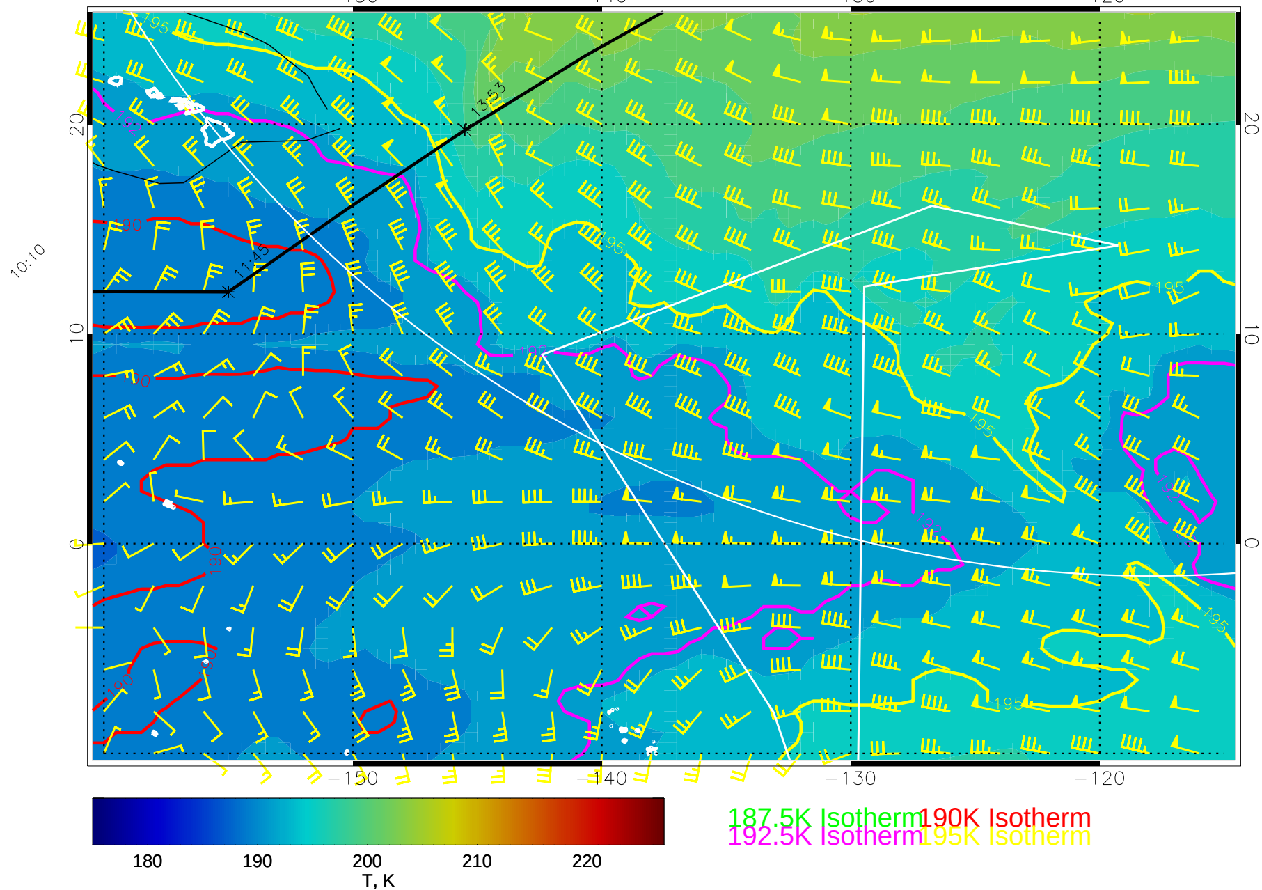
15011118, 6 hour forecast for 100mb T and winds (knots) -- NCEP GFS
