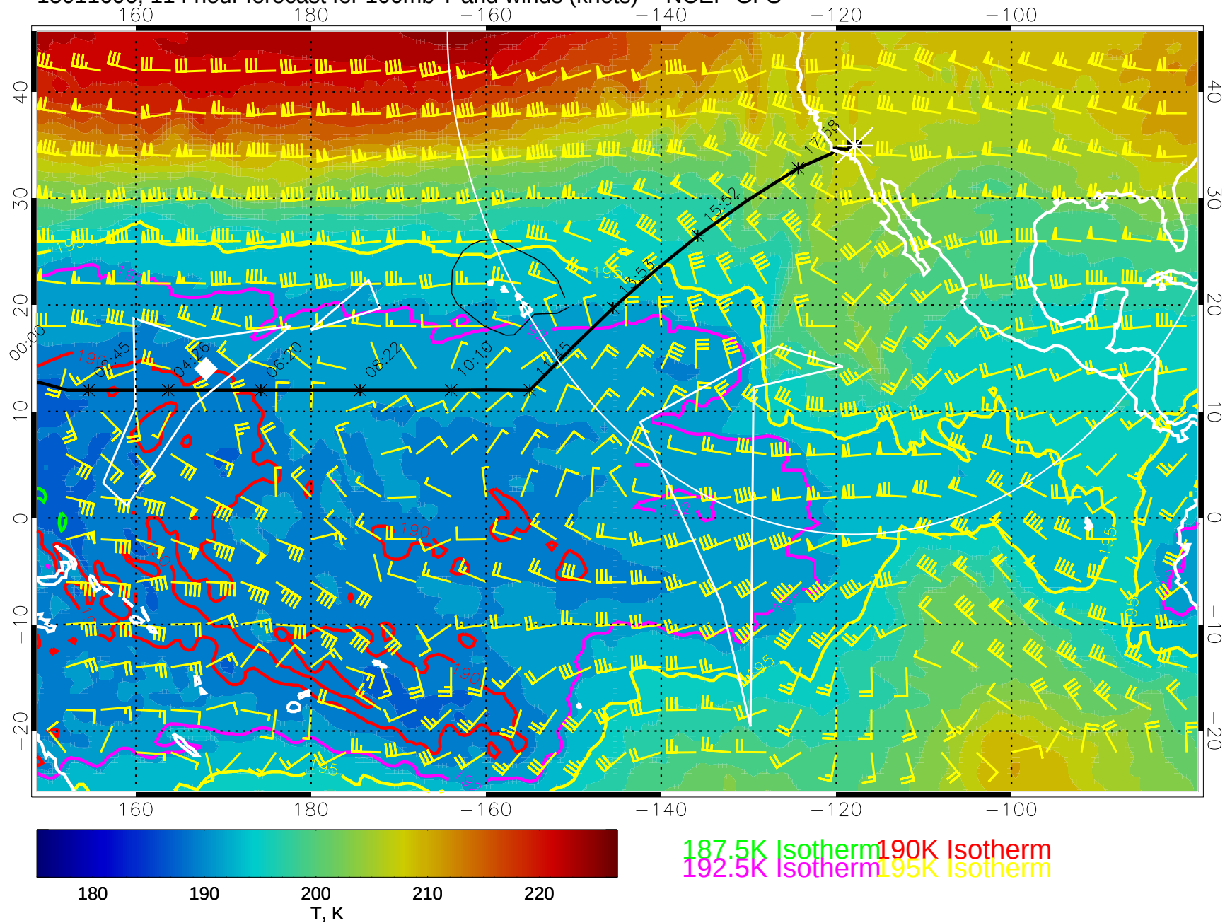
15011606, 114 hour forecast for 100mb T and winds (knots) -- NCEP GFS
