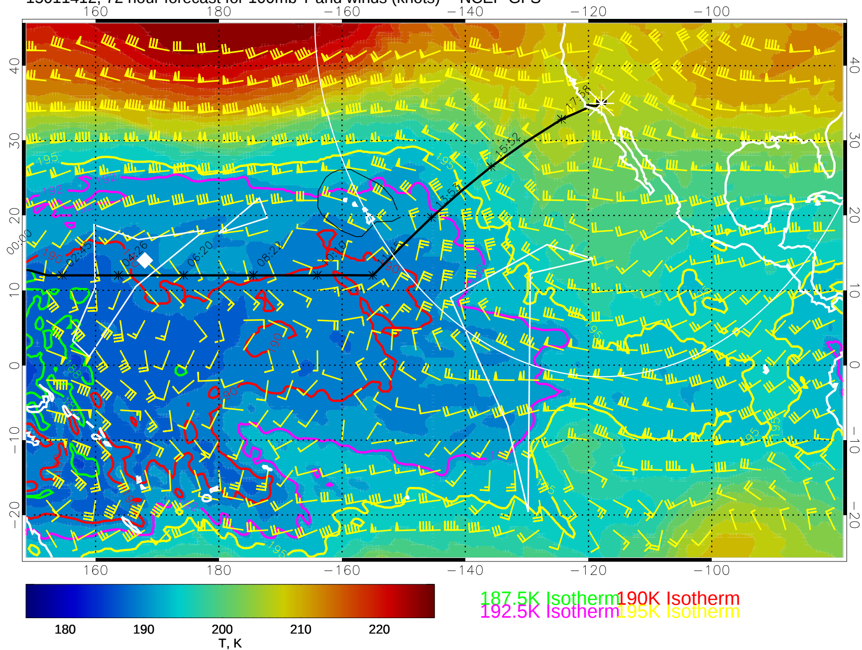
15011412, 72 hour forecast for 100mb T and winds (knots) -- NCEP GFS
