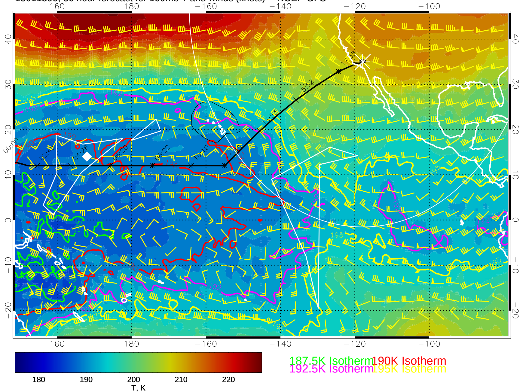
15011300, 36 hour forecast for 100mb T and winds (knots) -- NCEP GFS
