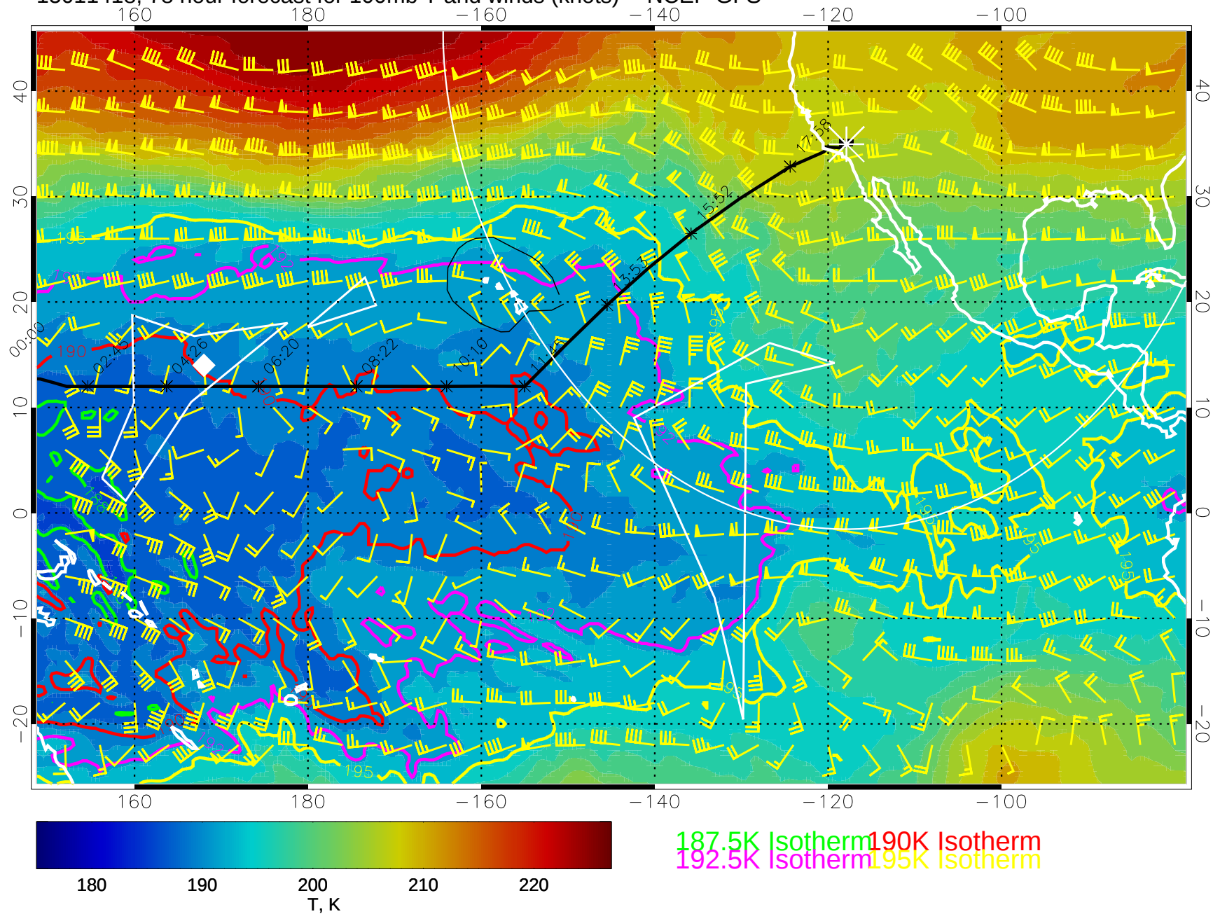
15011418, 78 hour forecast for 100mb T and winds (knots) -- NCEP GFS
