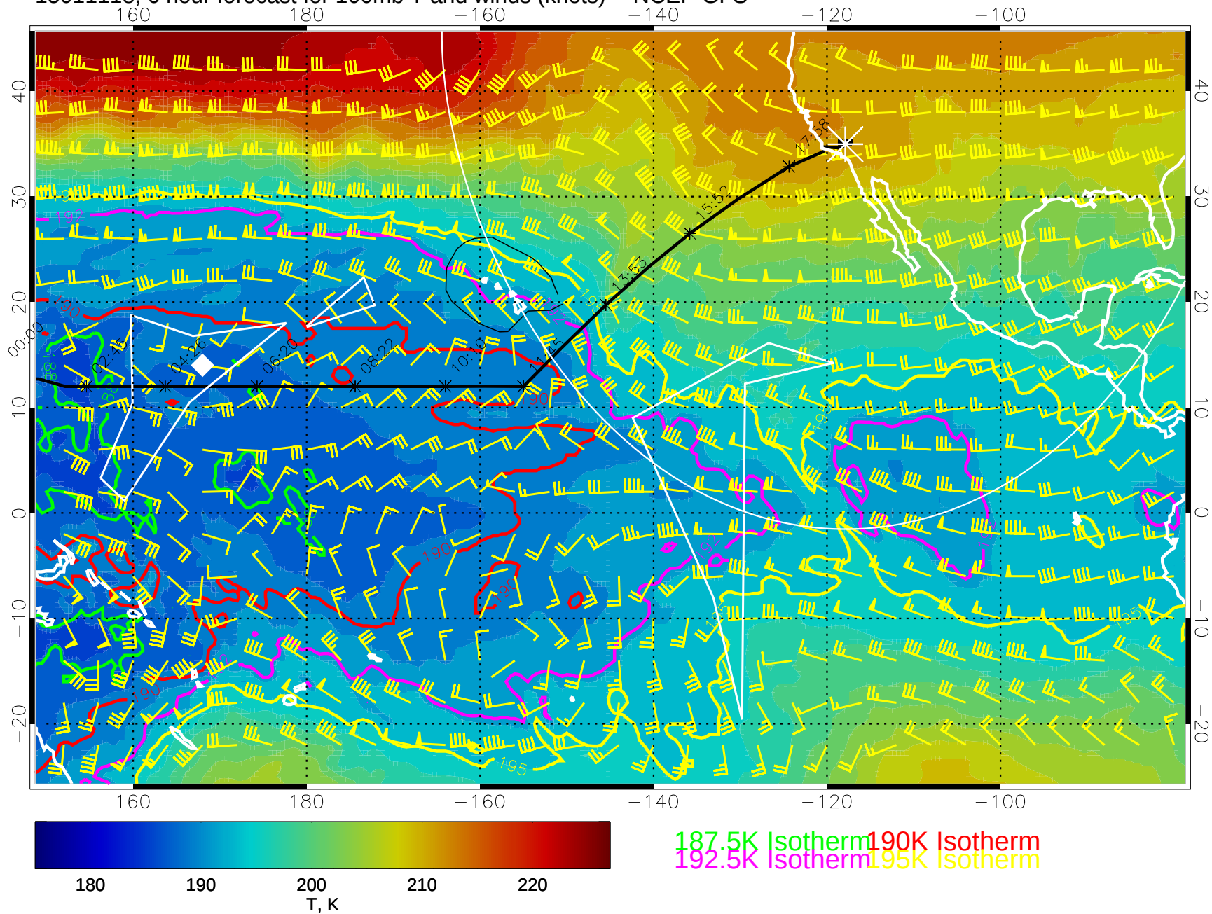
15011118, 6 hour forecast for 100mb T and winds (knots) -- NCEP GFS
