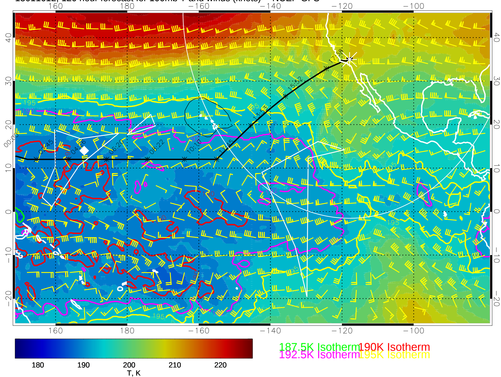
15011612, 120 hour forecast for 100mb T and winds (knots) -- NCEP GFS
