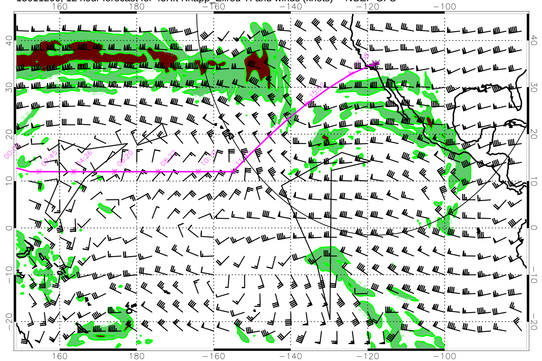
15011200, 12 hour forecast for 45Kft Knapp_Ellrod TI and winds (knots) -- NCEP GFS
