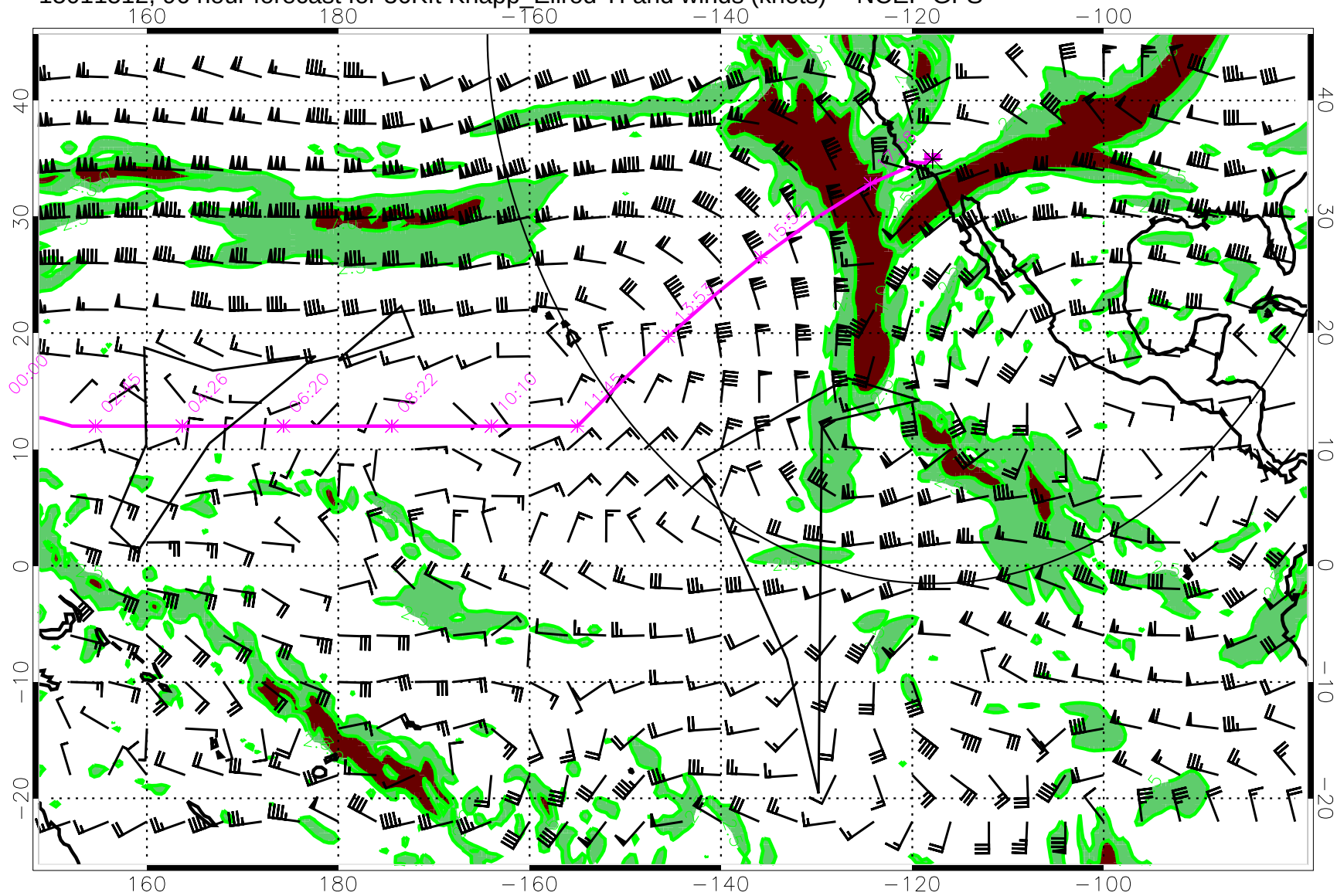
15011512, 96 hour forecast for 36Kft Knapp_Ellrod TI and winds (knots) -- NCEP GFS
