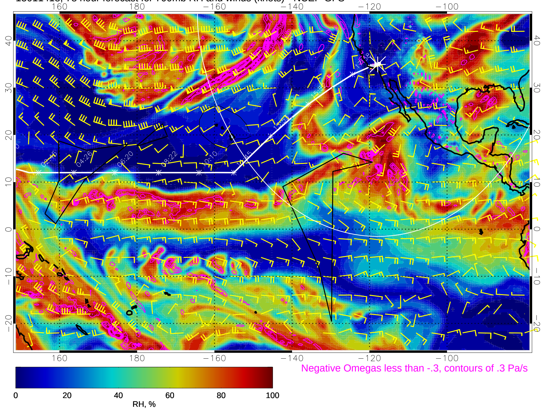
15011418, 78 hour forecast for 700mb RH and winds (knots) - NCEP GFS
