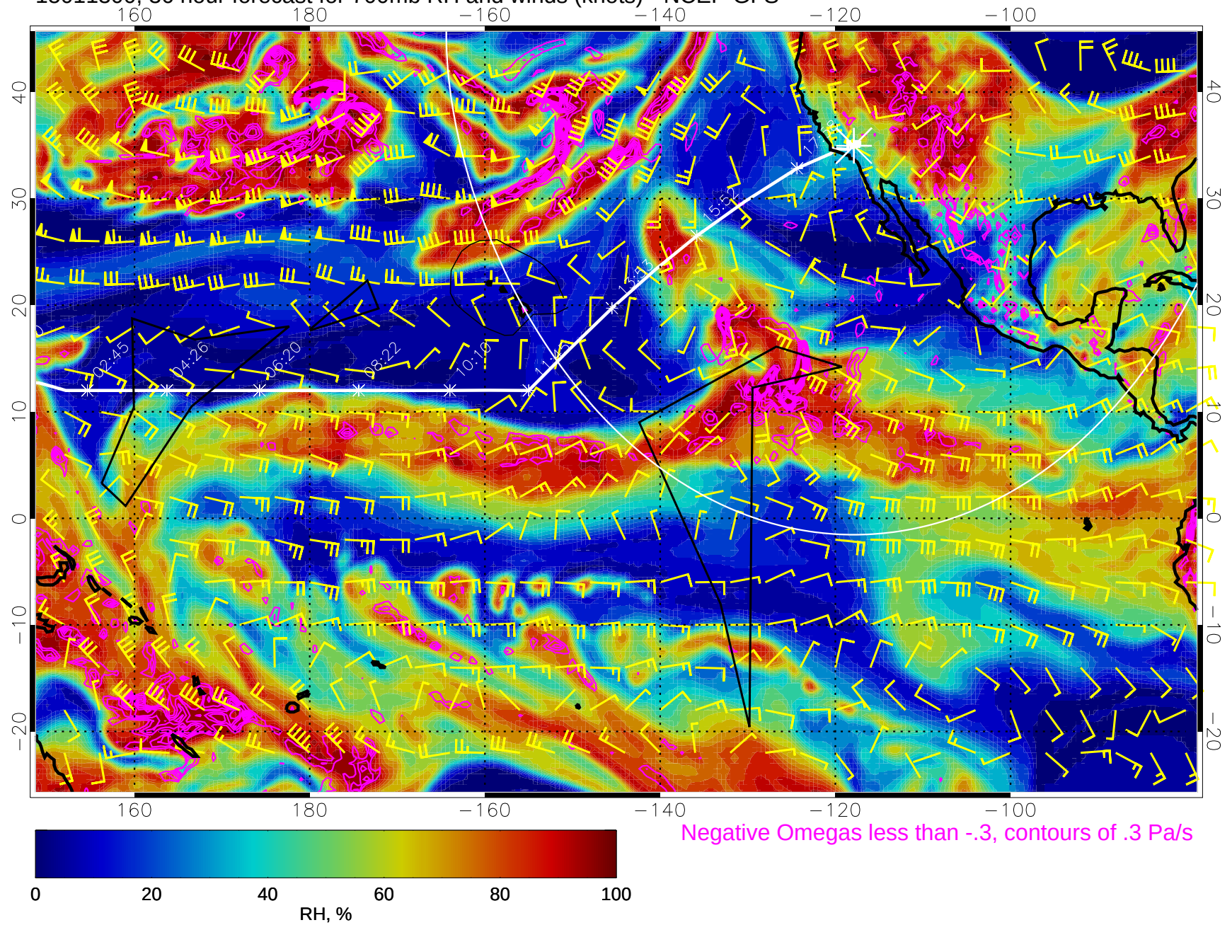
15011300, 36 hour forecast for 700mb RH and winds (knots) - NCEP GFS
