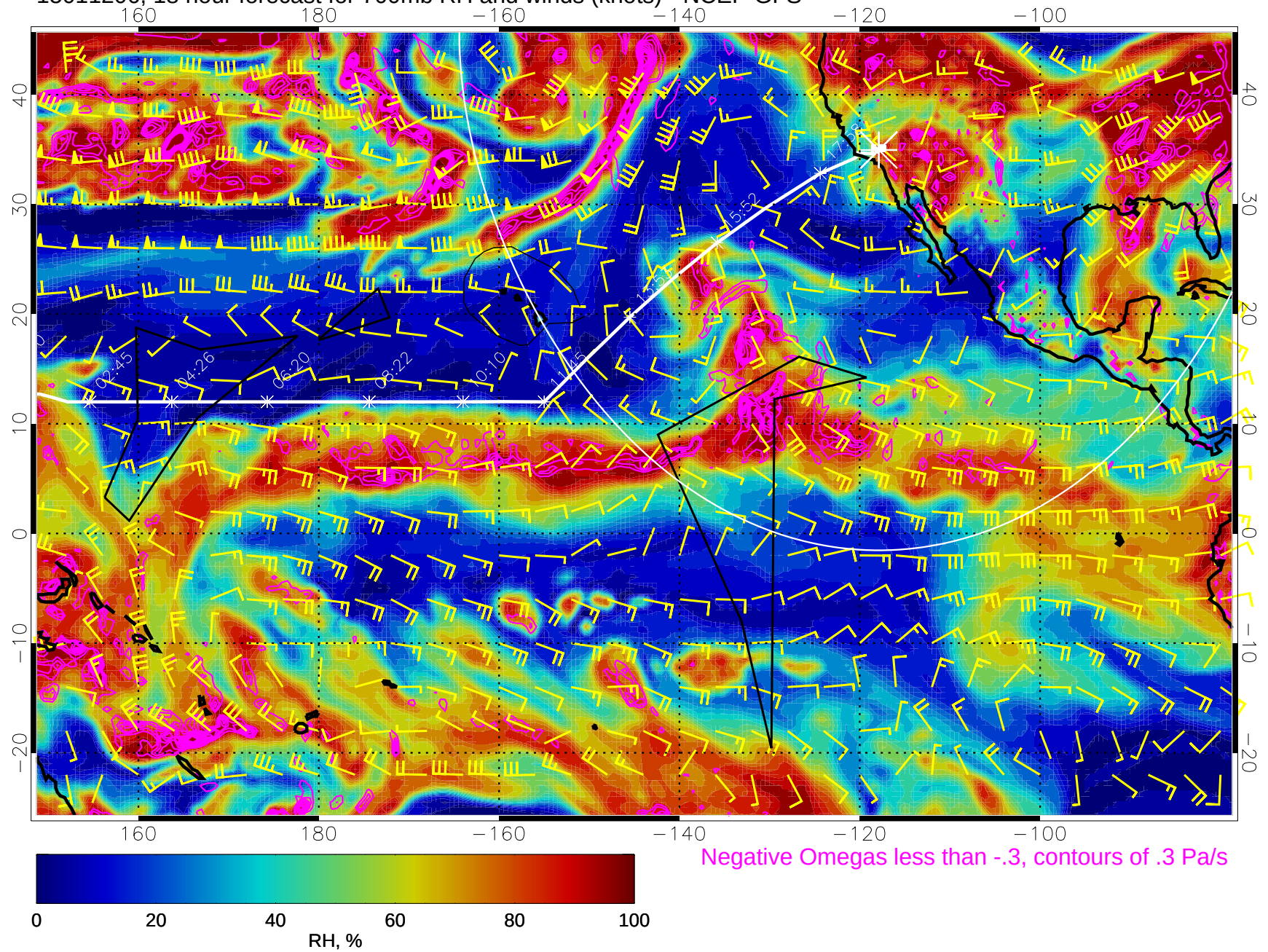
15011206, 18 hour forecast for 700mb RH and winds (knots) - NCEP GFS
