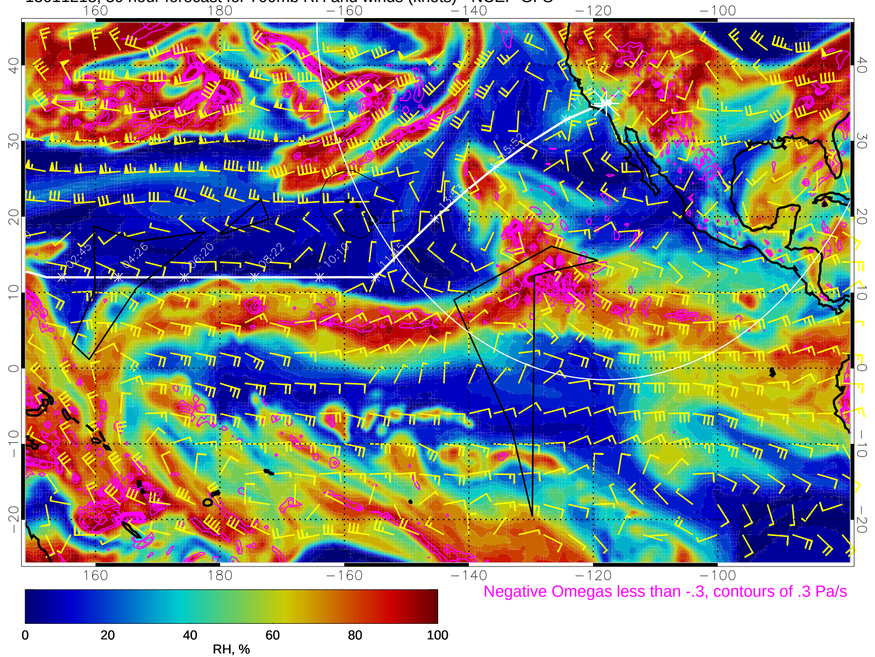
15011218, 30 hour forecast for 700mb RH and winds (knots) - NCEP GFS
