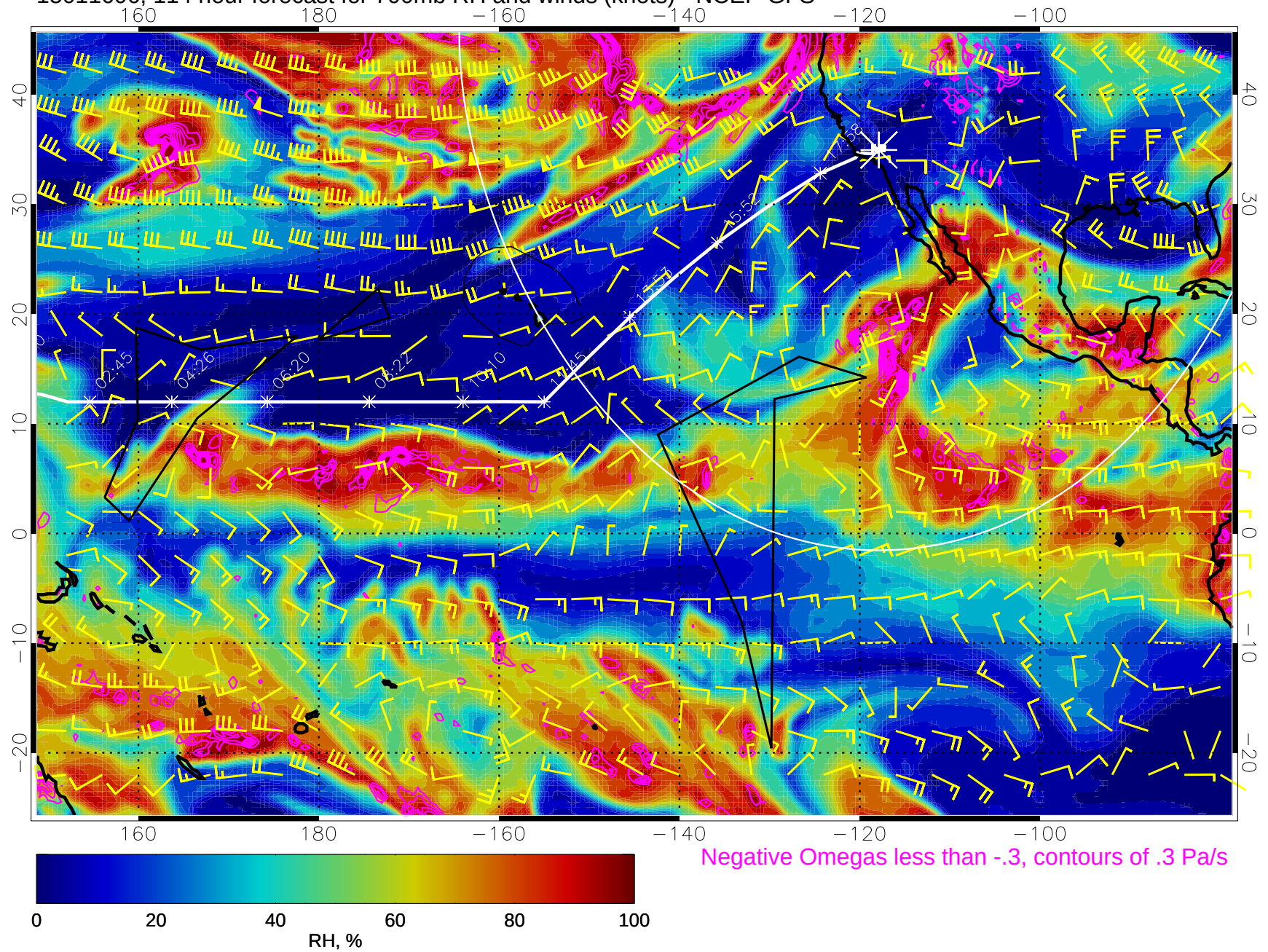
15011606, 114 hour forecast for 700mb RH and winds (knots) - NCEP GFS
