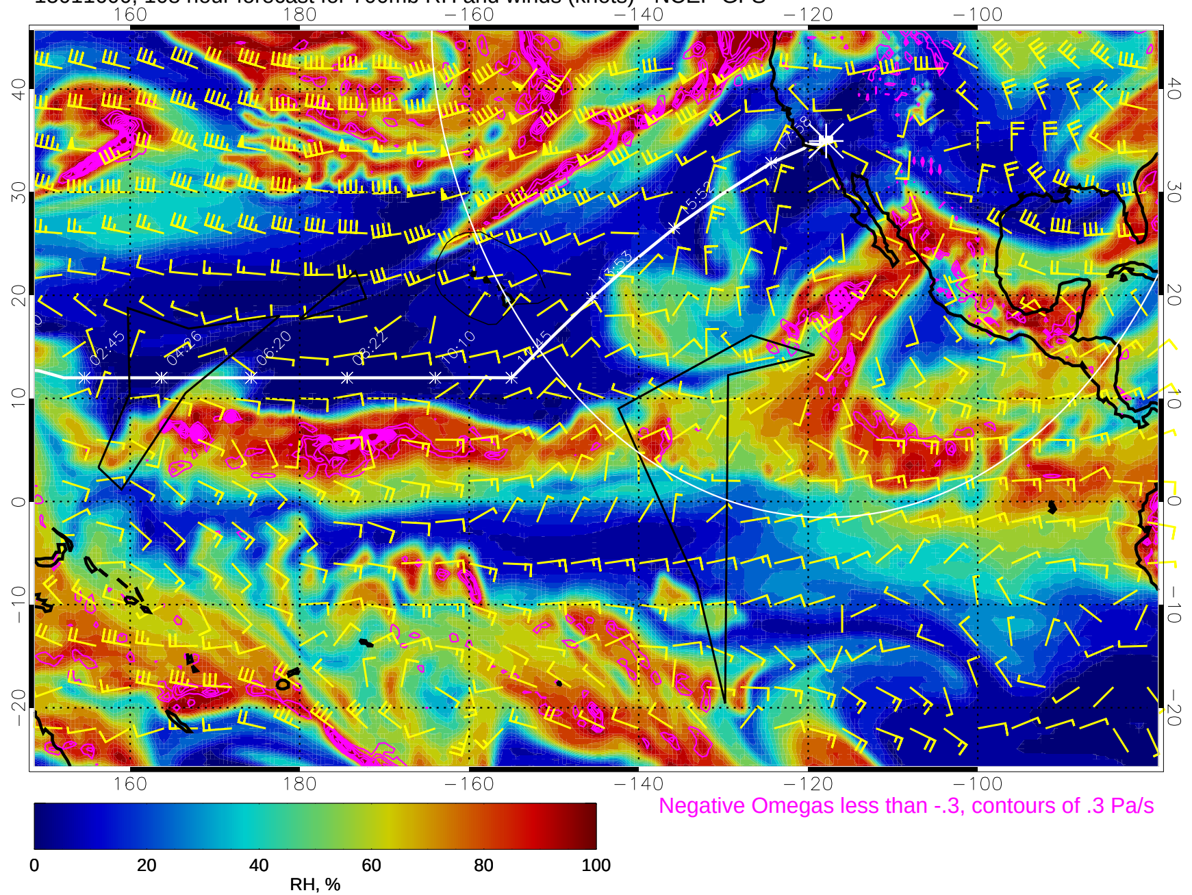
15011600, 108 hour forecast for 700mb RH and winds (knots) - NCEP GFS
