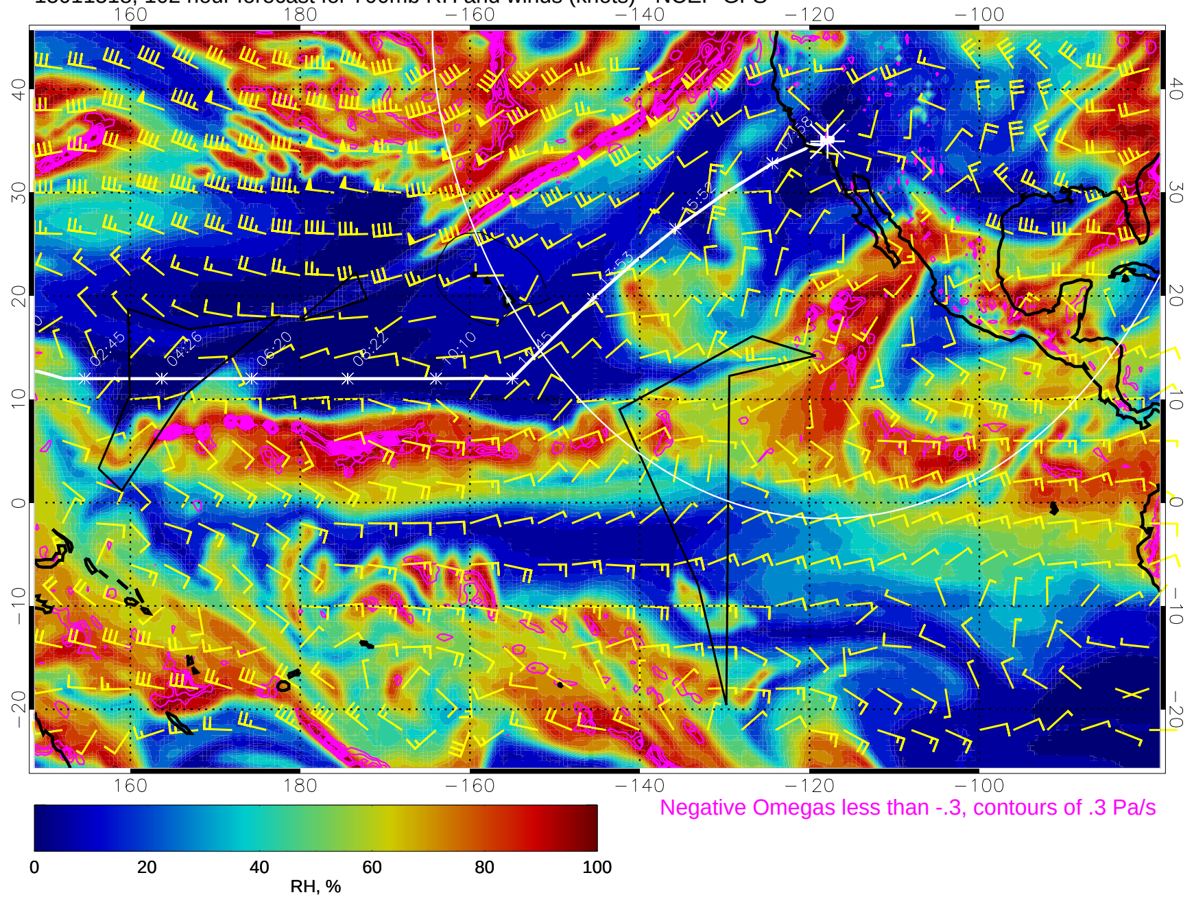
15011518, 102 hour forecast for 700mb RH and winds (knots) - NCEP GFS
