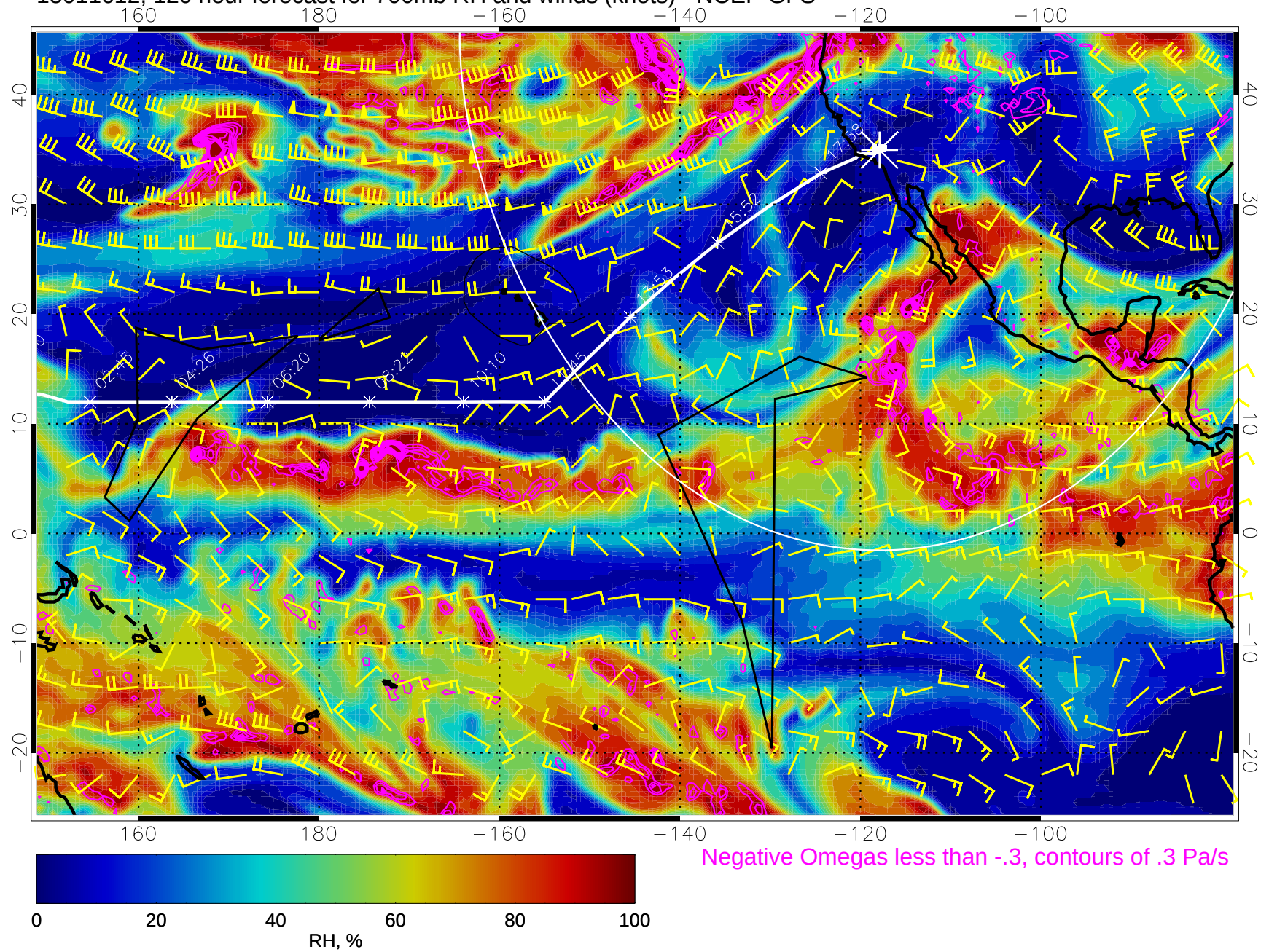
15011612, 120 hour forecast for 700mb RH and winds (knots) - NCEP GFS
