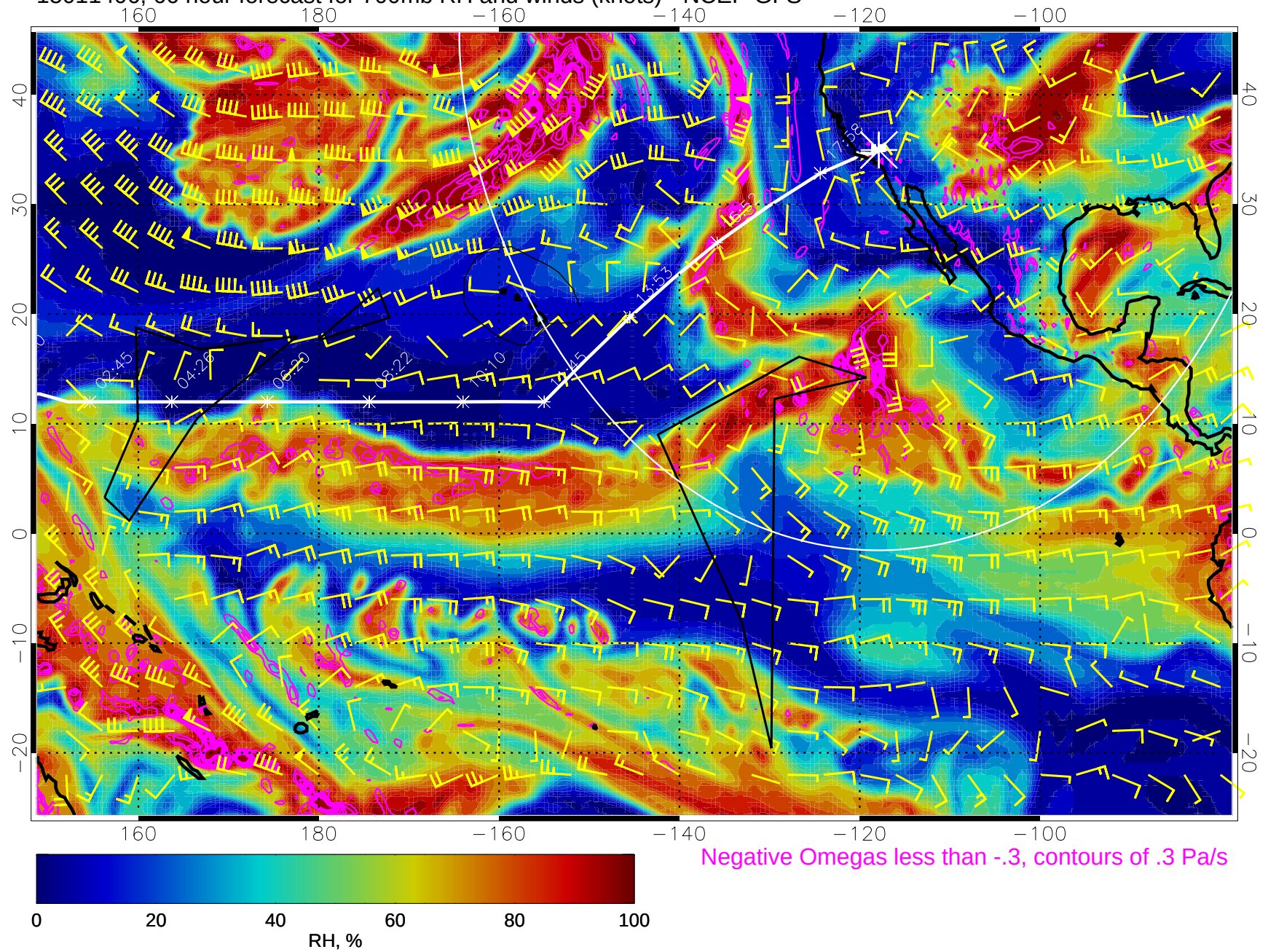
15011406, 66 hour forecast for 700mb RH and winds (knots) - NCEP GFS
