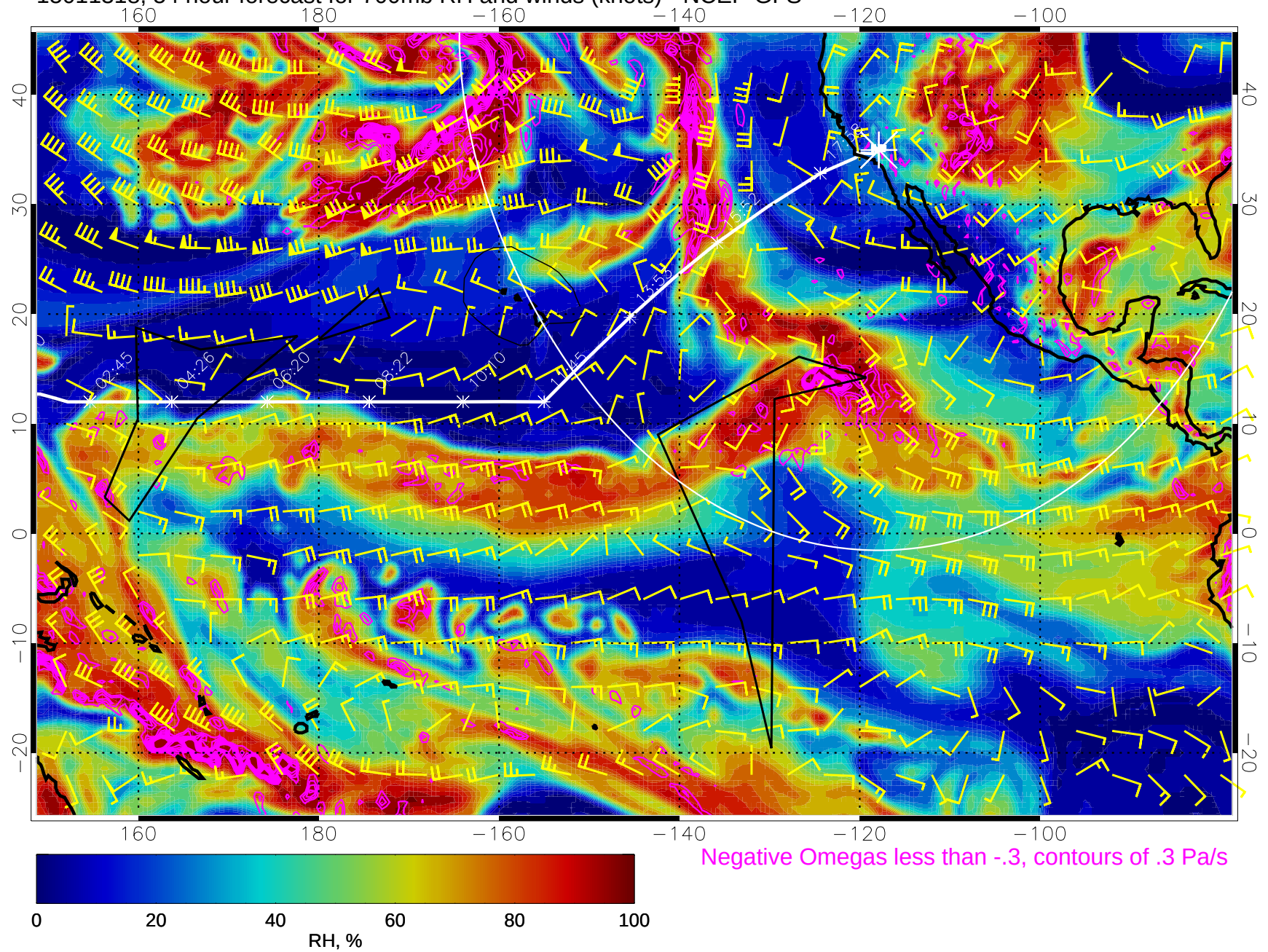
15011318, 54 hour forecast for 700mb RH and winds (knots) - NCEP GFS
