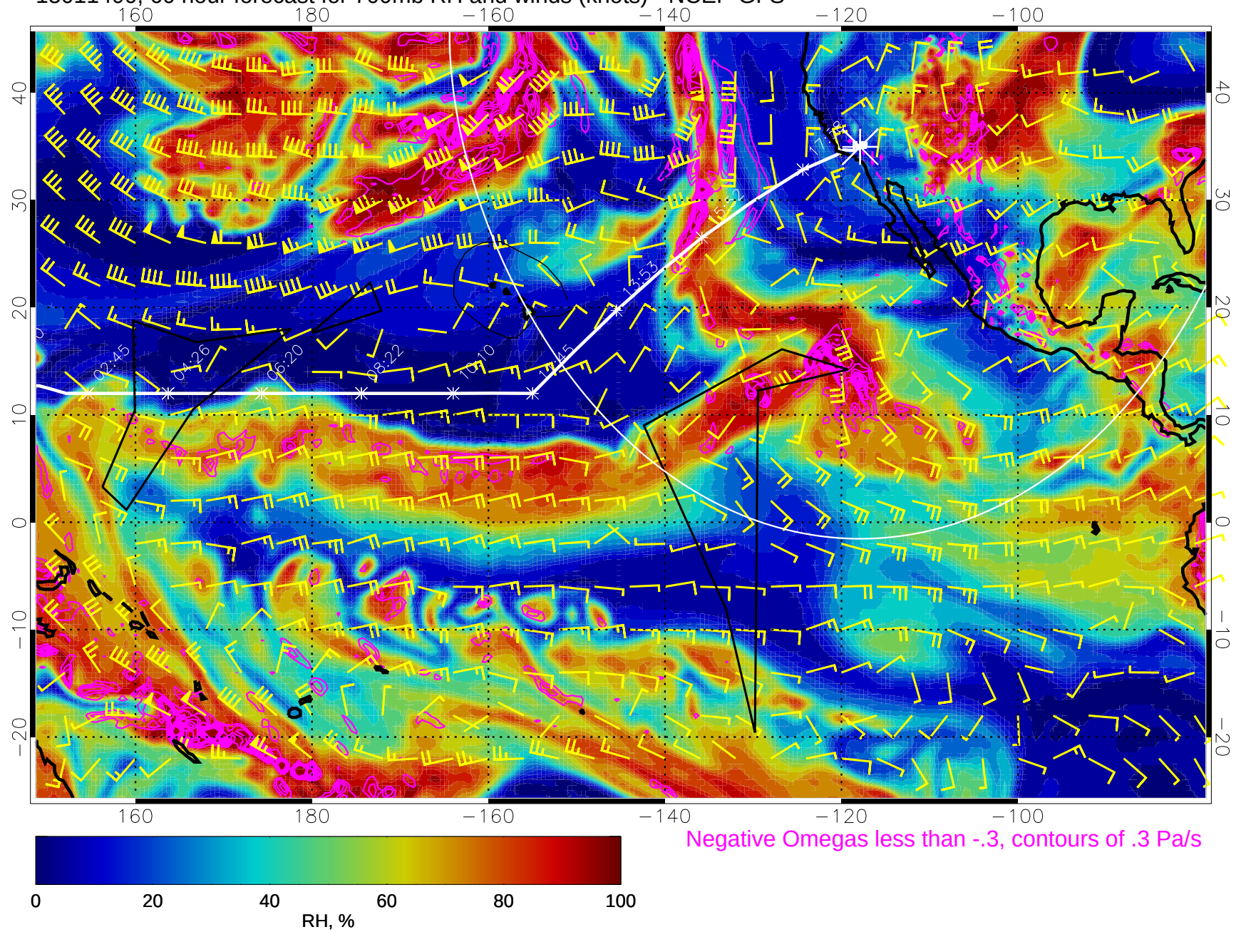
15011400, 60 hour forecast for 700mb RH and winds (knots) - NCEP GFS
