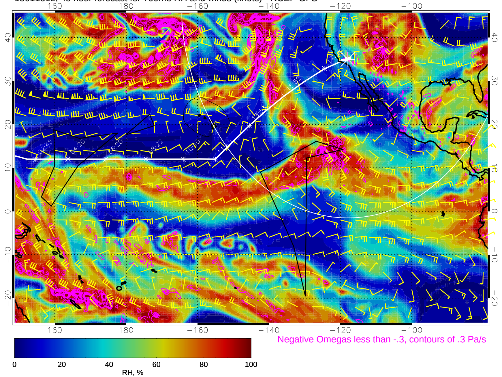
15011312, 48 hour forecast for 700mb RH and winds (knots) - NCEP GFS
