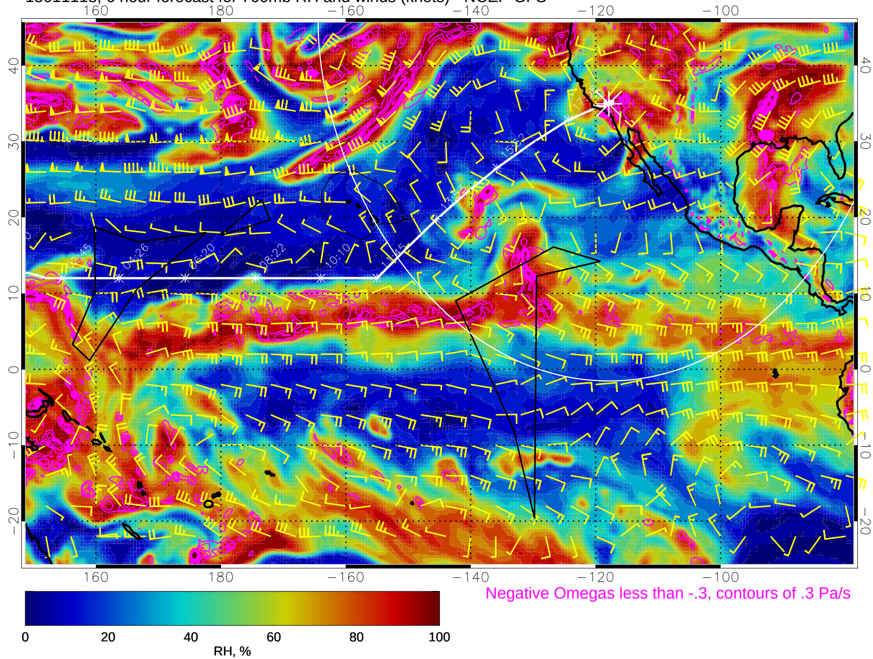
15011118, 6 hour forecast for 700mb RH and winds (knots) - NCEP GFS
