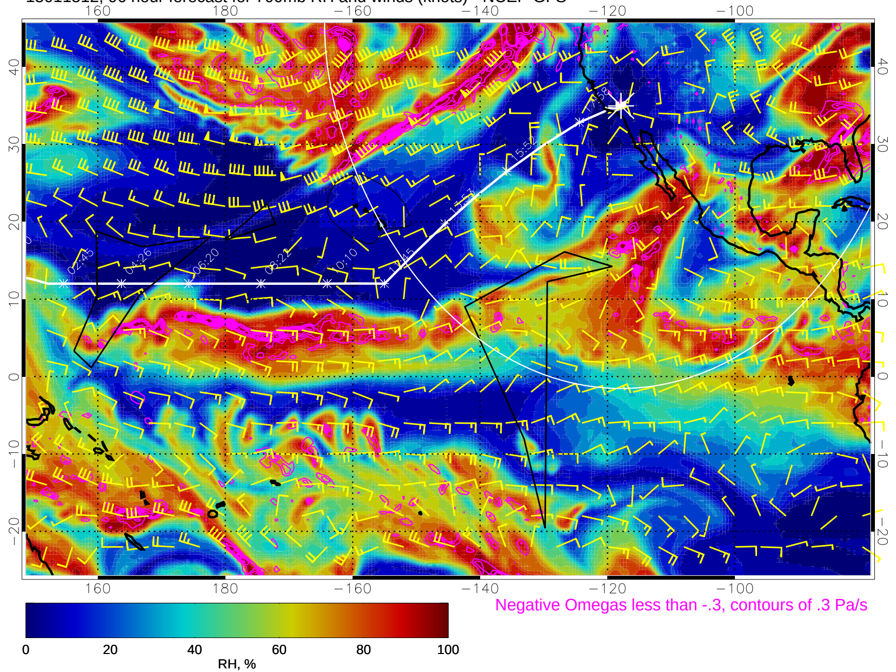
15011512, 96 hour forecast for 700mb RH and winds (knots) - NCEP GFS
