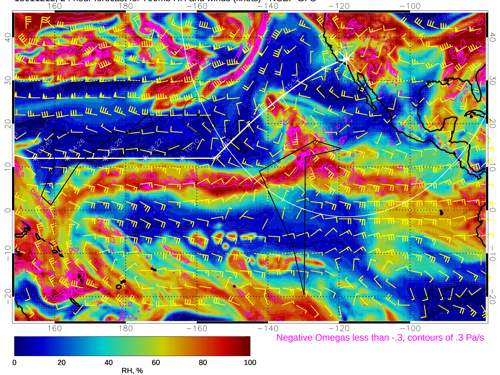
15011212, 24 hour forecast for 700mb RH and winds (knots) - NCEP GFS
