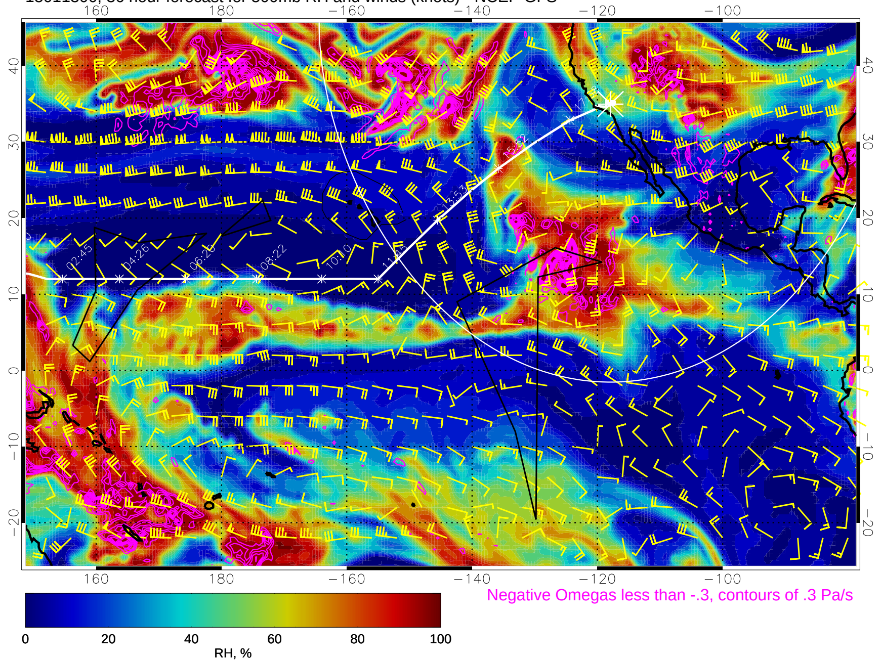
15011300, 36 hour forecast for 500mb RH and winds (knots) - NCEP GFS
