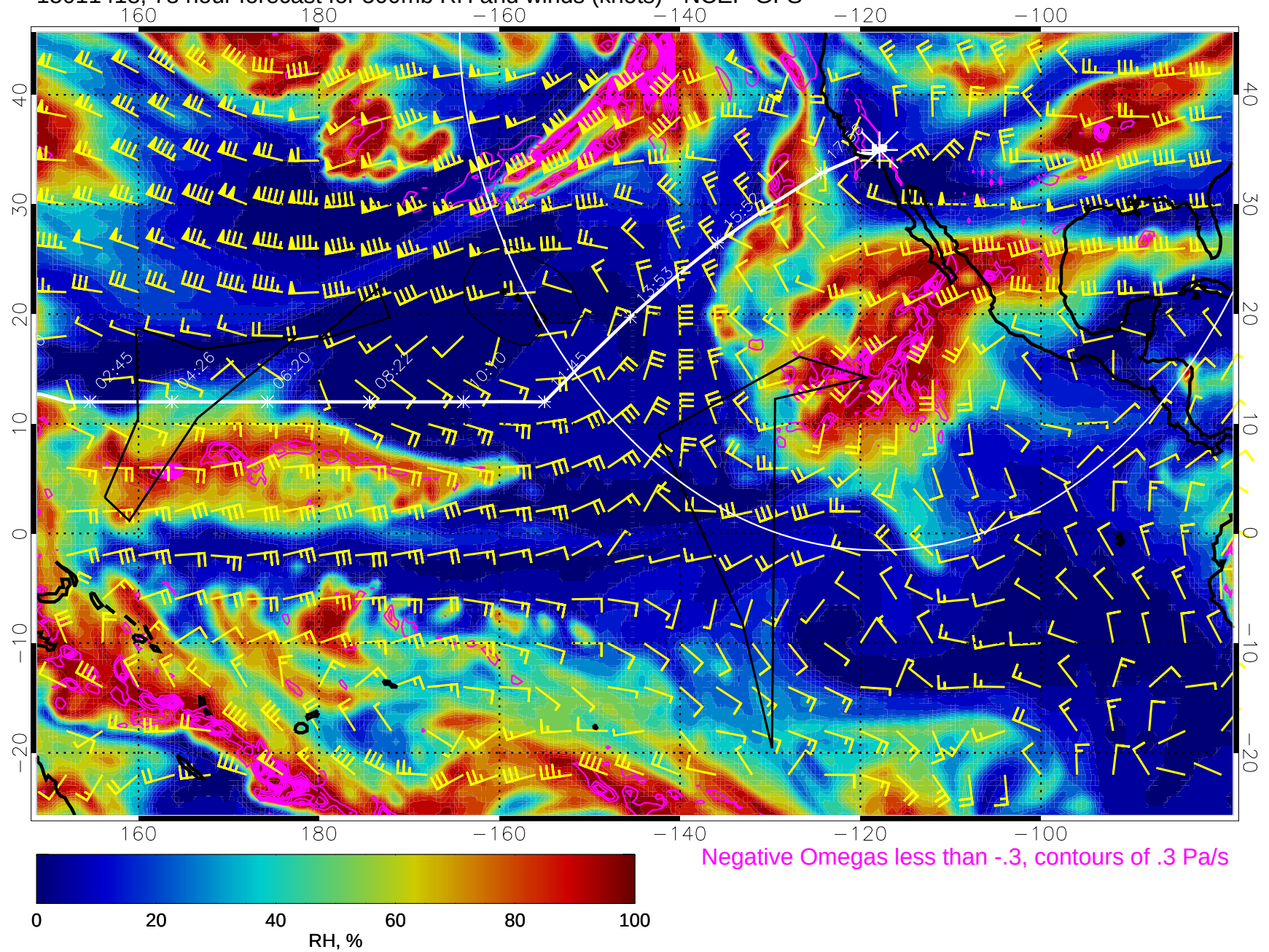
15011418, 78 hour forecast for 500mb RH and winds (knots) - NCEP GFS
