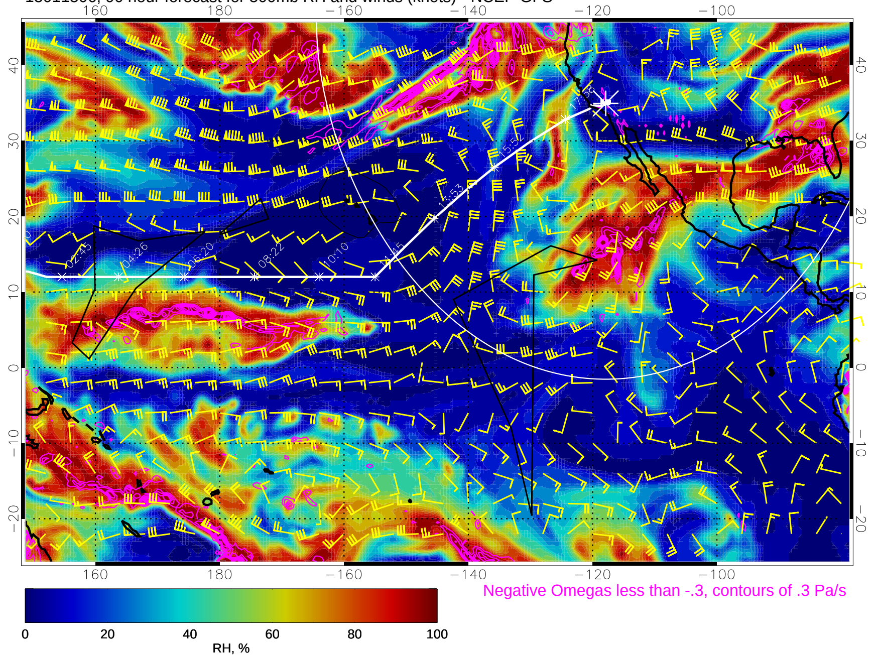
15011506, 90 hour forecast for 500mb RH and winds (knots) - NCEP GFS
