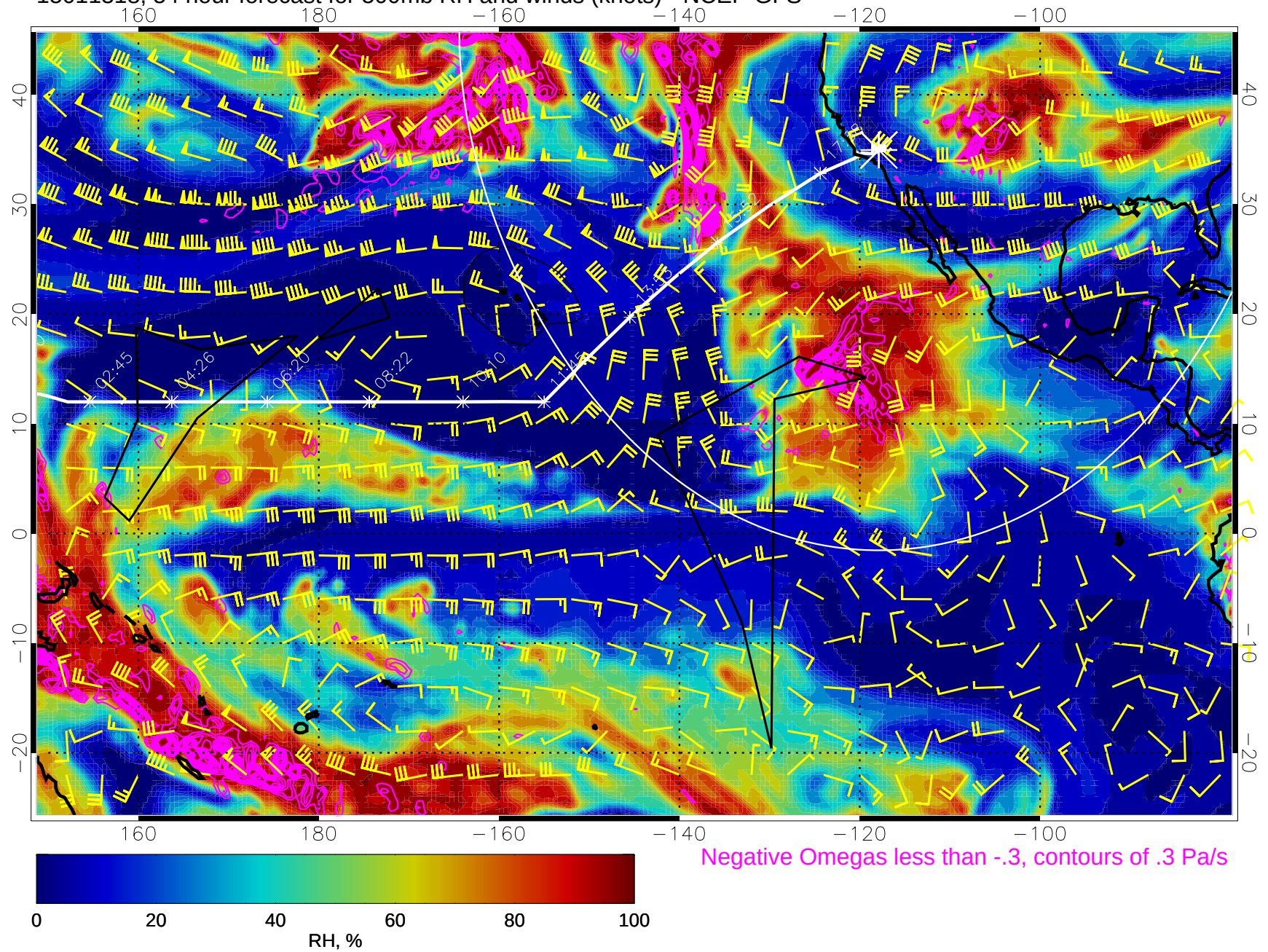
15011318, 54 hour forecast for 500mb RH and winds (knots) - NCEP GFS
