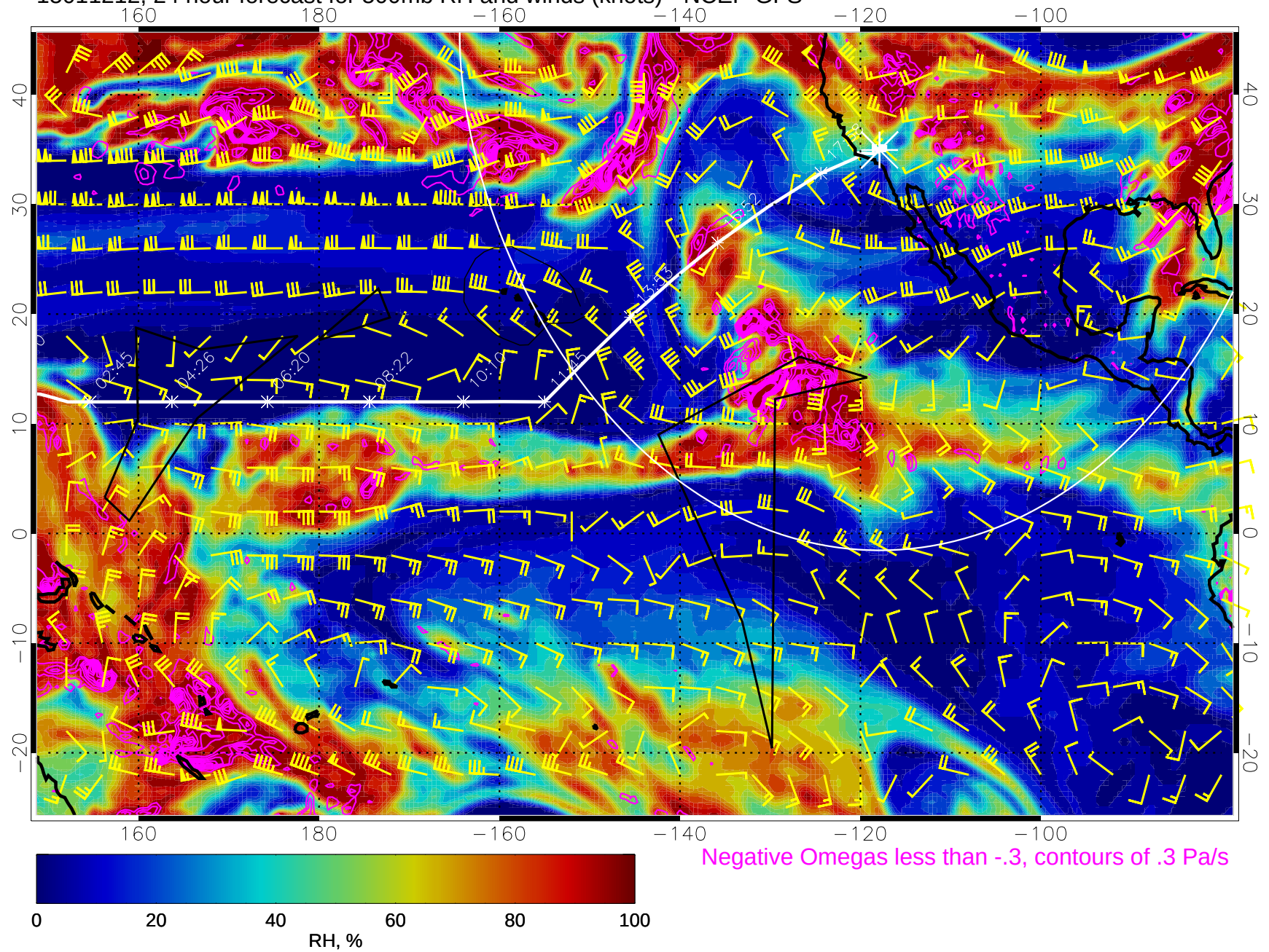
15011212, 24 hour forecast for 500mb RH and winds (knots) - NCEP GFS
