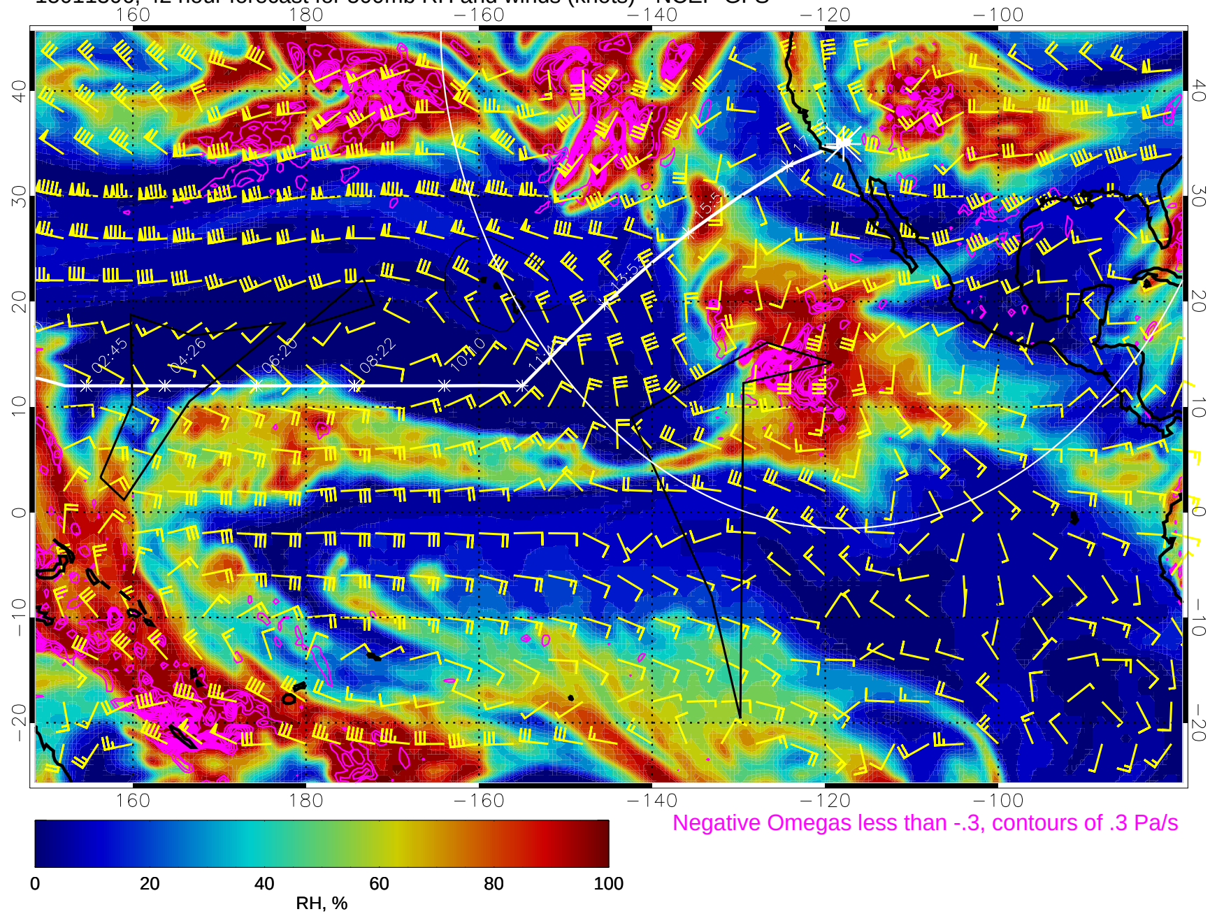
15011306, 42 hour forecast for 500mb RH and winds (knots) - NCEP GFS
