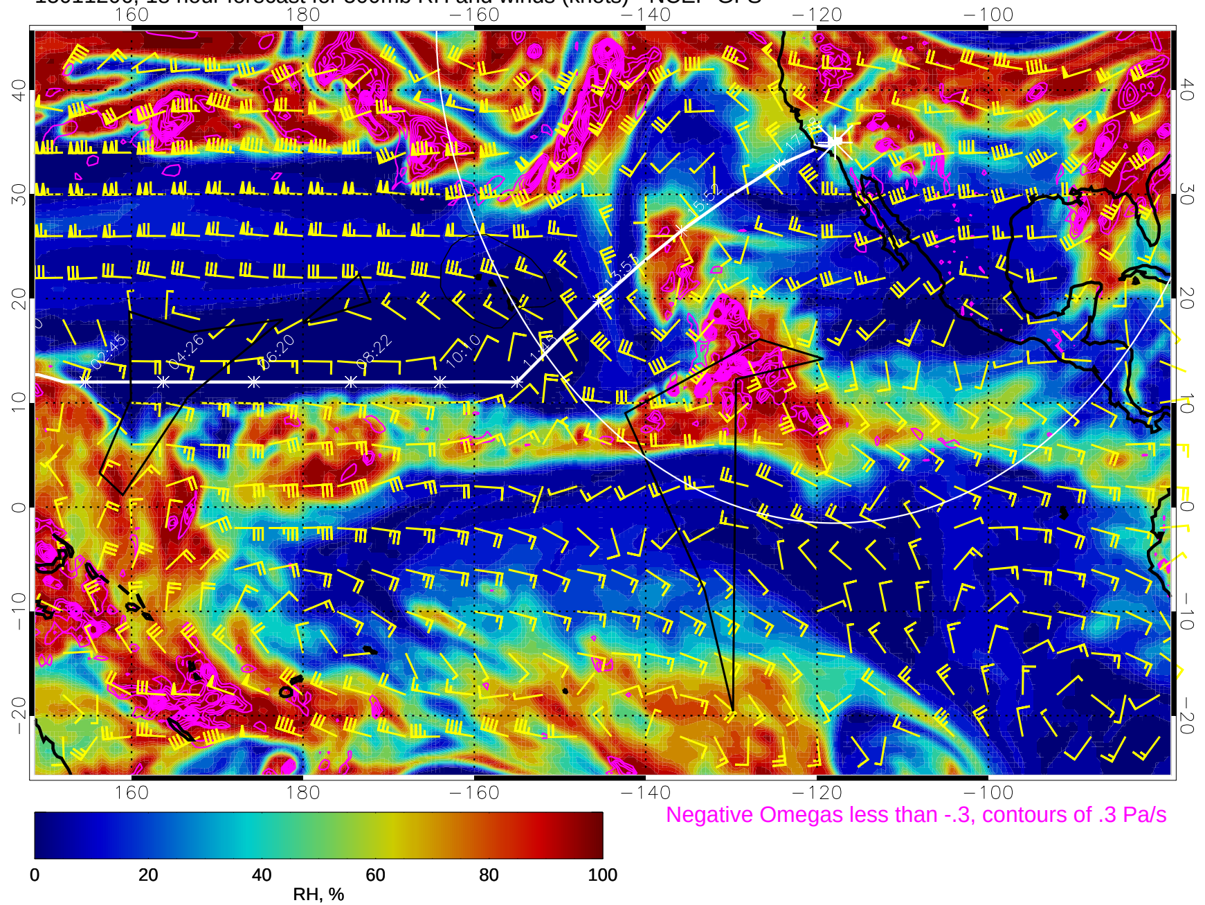
15011206, 18 hour forecast for 500mb RH and winds (knots) - NCEP GFS
