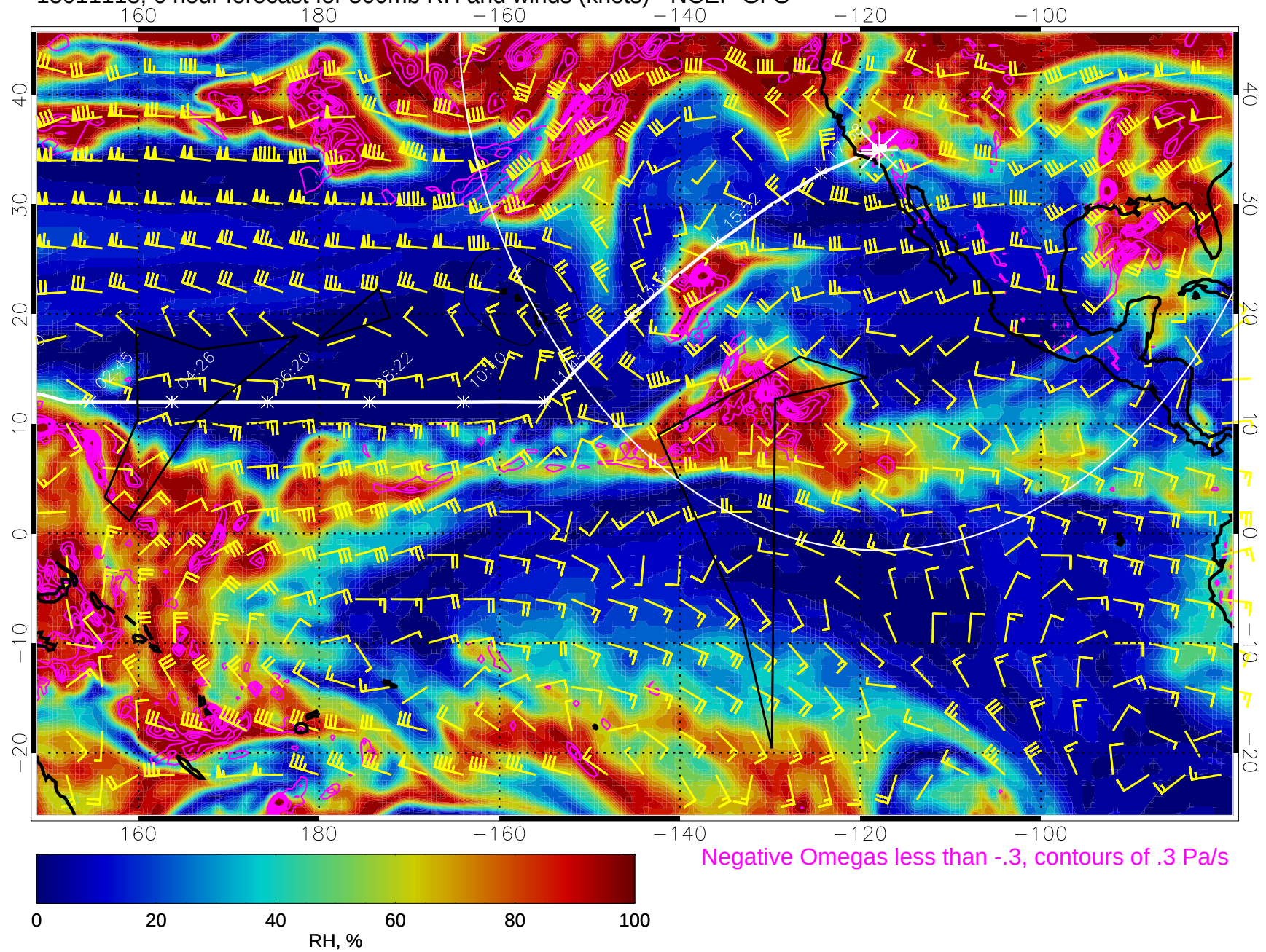
15011118, 6 hour forecast for 500mb RH and winds (knots) - NCEP GFS
