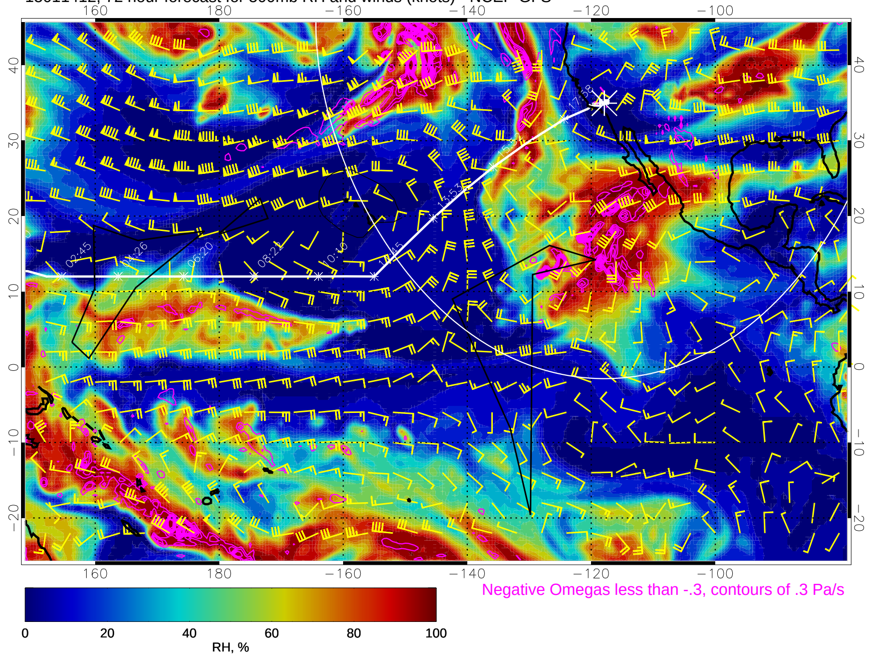
15011412, 72 hour forecast for 500mb RH and winds (knots) - NCEP GFS
