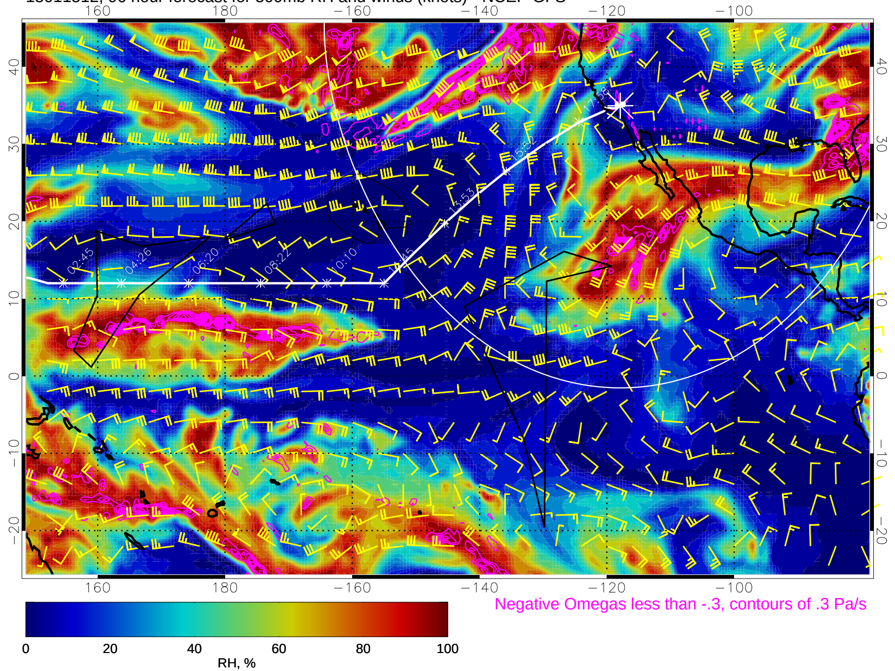
15011512, 96 hour forecast for 500mb RH and winds (knots) - NCEP GFS
