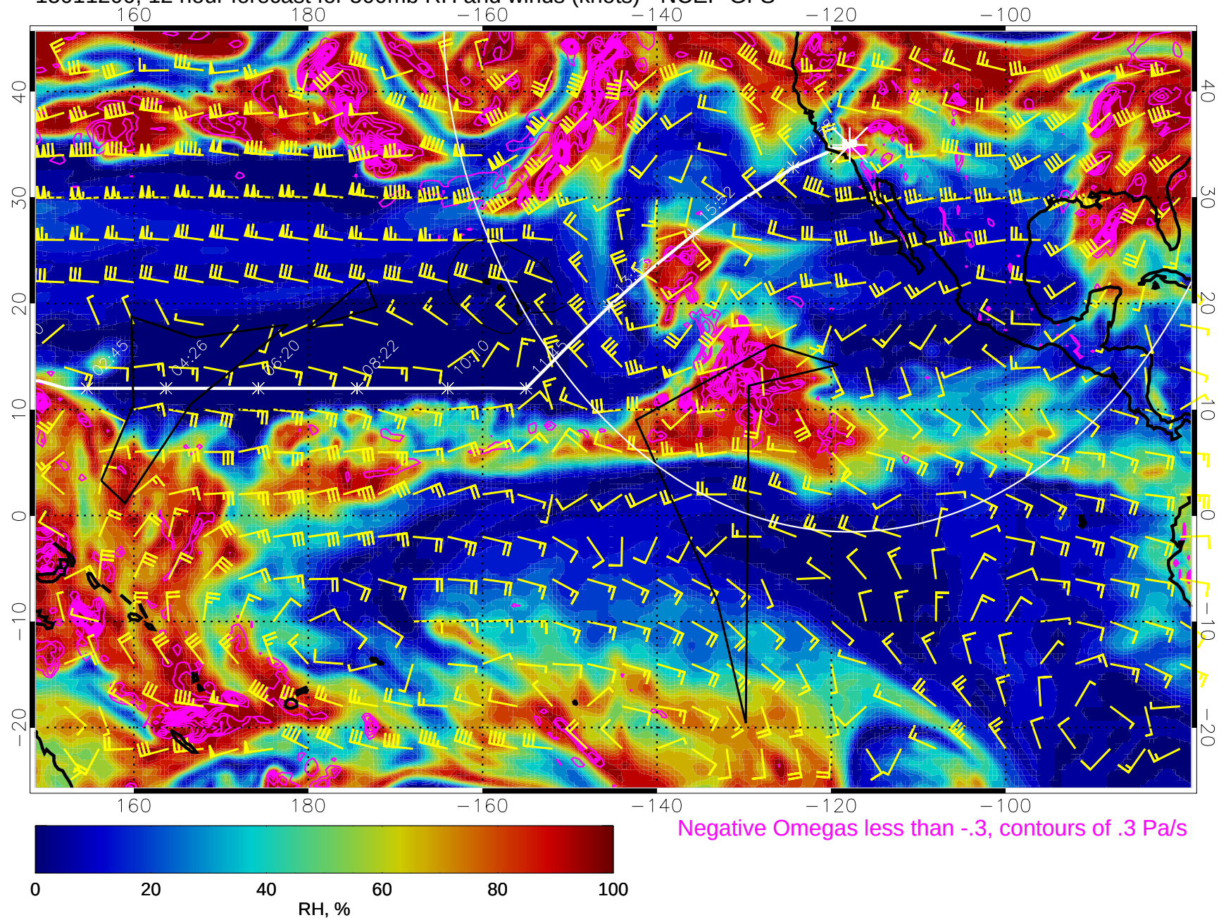
15011200, 12 hour forecast for 500mb RH and winds (knots) - NCEP GFS
