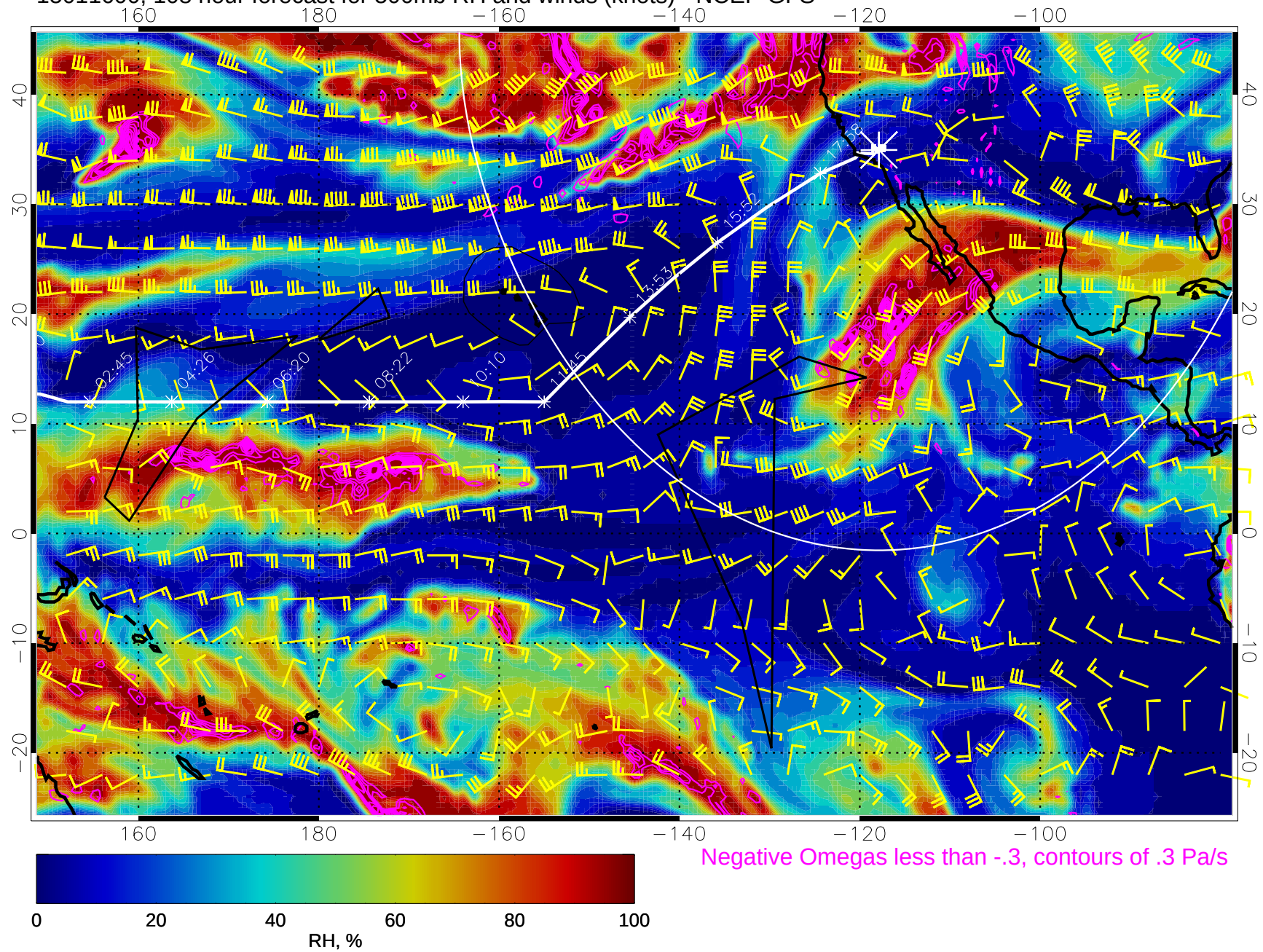
15011600, 108 hour forecast for 500mb RH and winds (knots) - NCEP GFS
