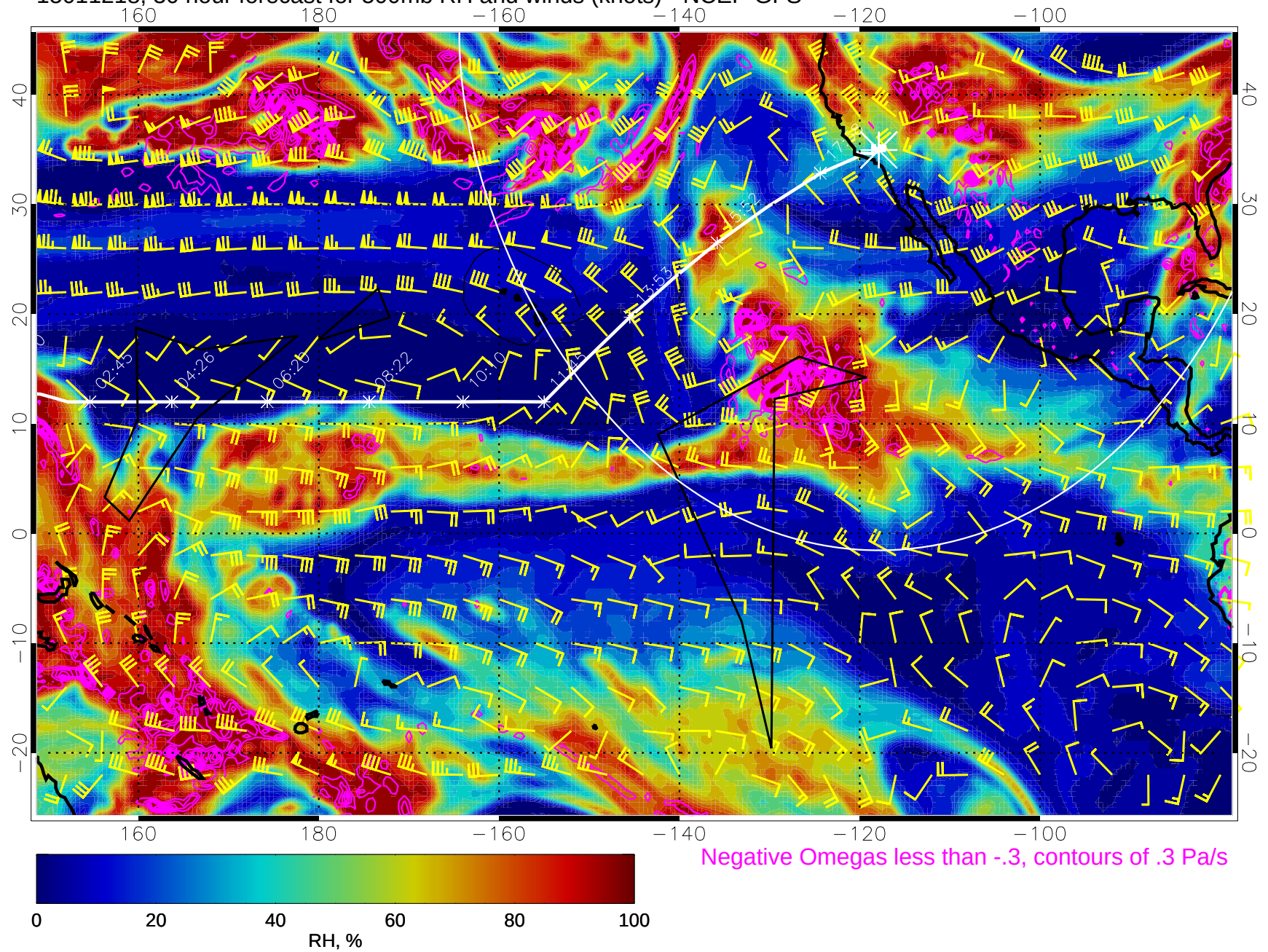
15011218, 30 hour forecast for 500mb RH and winds (knots) - NCEP GFS
