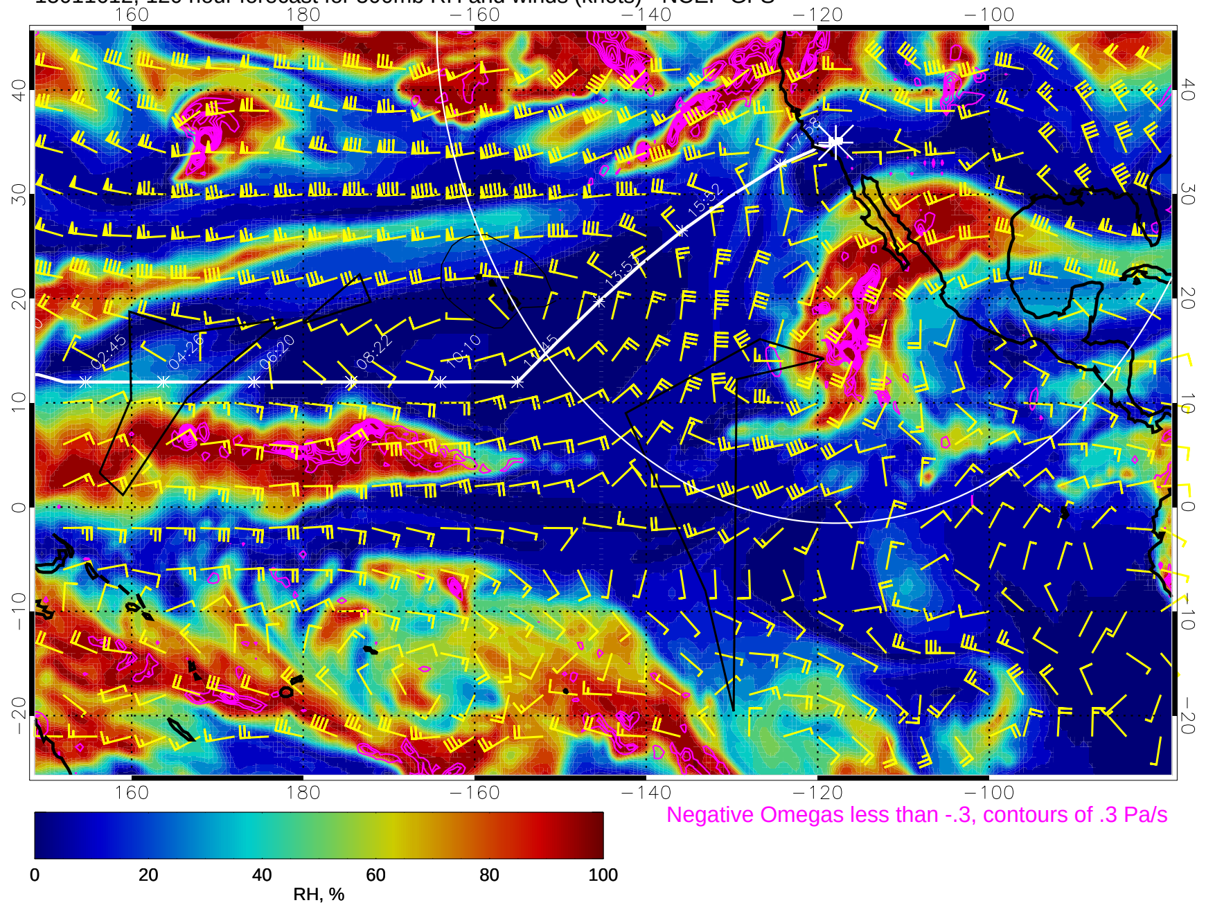
15011612, 120 hour forecast for 500mb RH and winds (knots) - NCEP GFS
