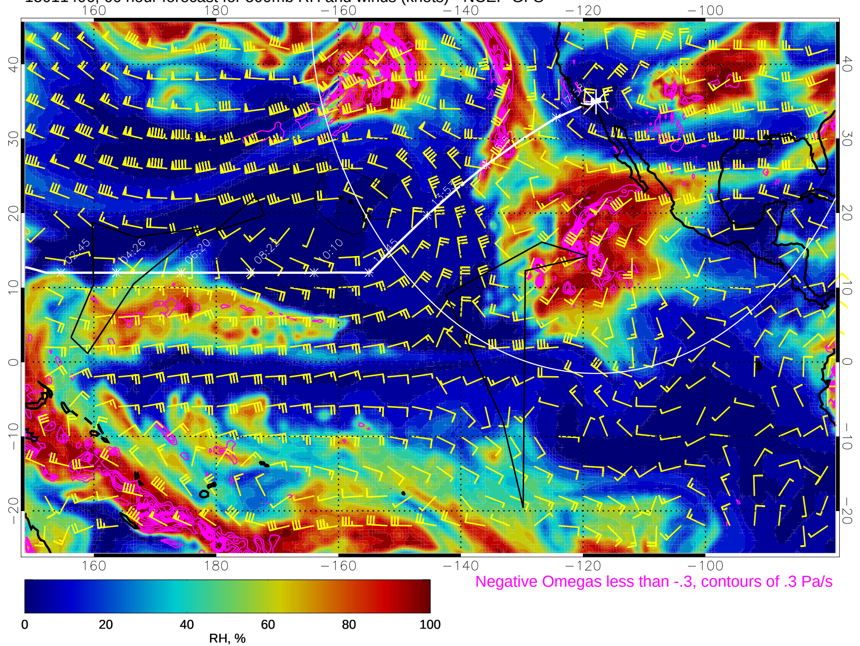
15011406, 66 hour forecast for 500mb RH and winds (knots) - NCEP GFS
