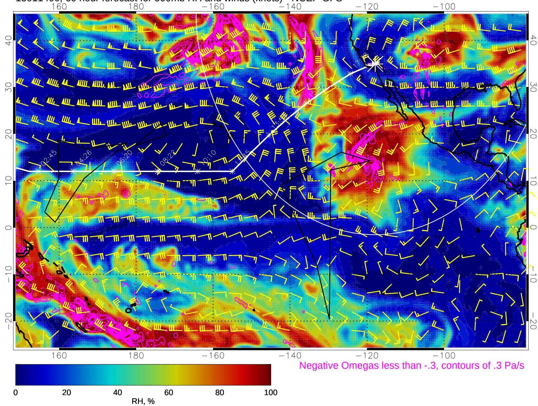
15011400, 60 hour forecast for 500mb RH and winds (knots) - NCEP GFS
