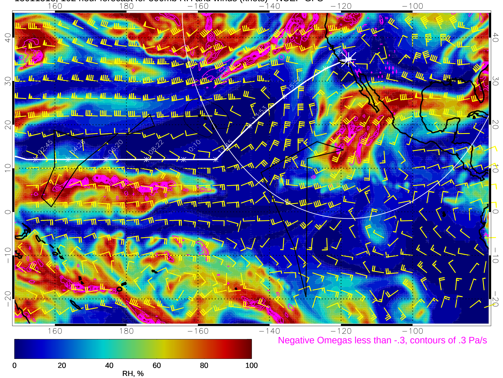
15011518, 102 hour forecast for 500mb RH and winds (knots) - NCEP GFS
