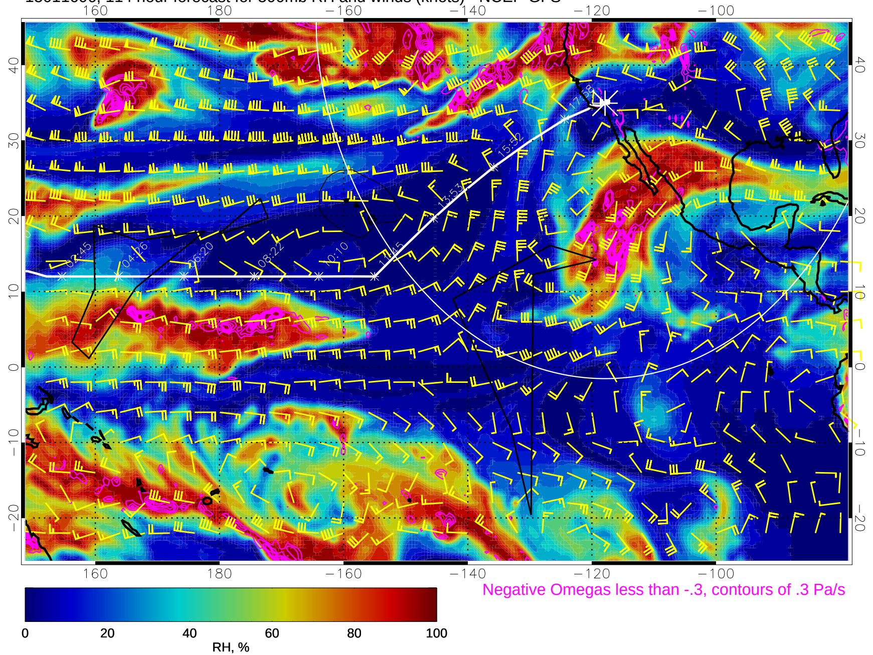
15011606, 114 hour forecast for 500mb RH and winds (knots) - NCEP GFS
