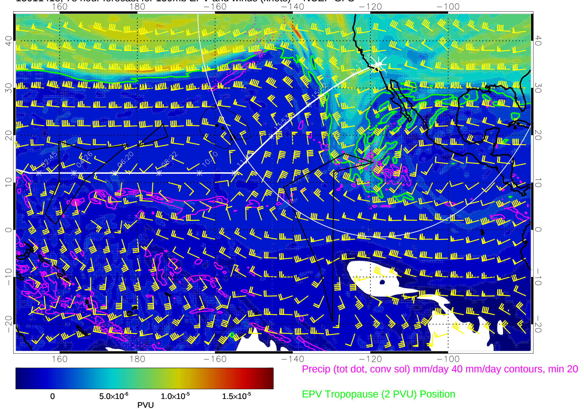
15011418, 78 hour forecast for 150mb EPV and winds (knots) -- NCEP GFS
