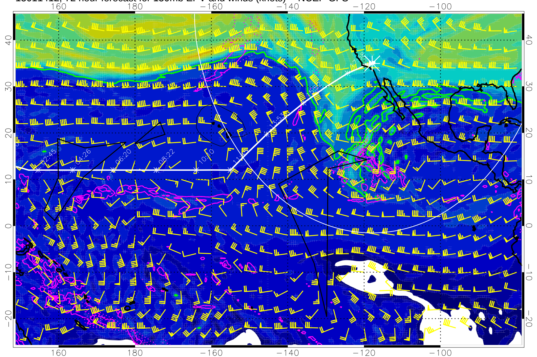
15011412, 72 hour forecast for 150mb EPV and winds (knots) -- NCEP GFS
