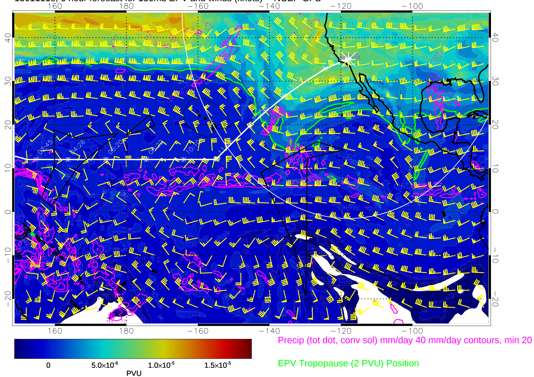
15011118, 6 hour forecast for 150mb EPV and winds (knots) -- NCEP GFS
