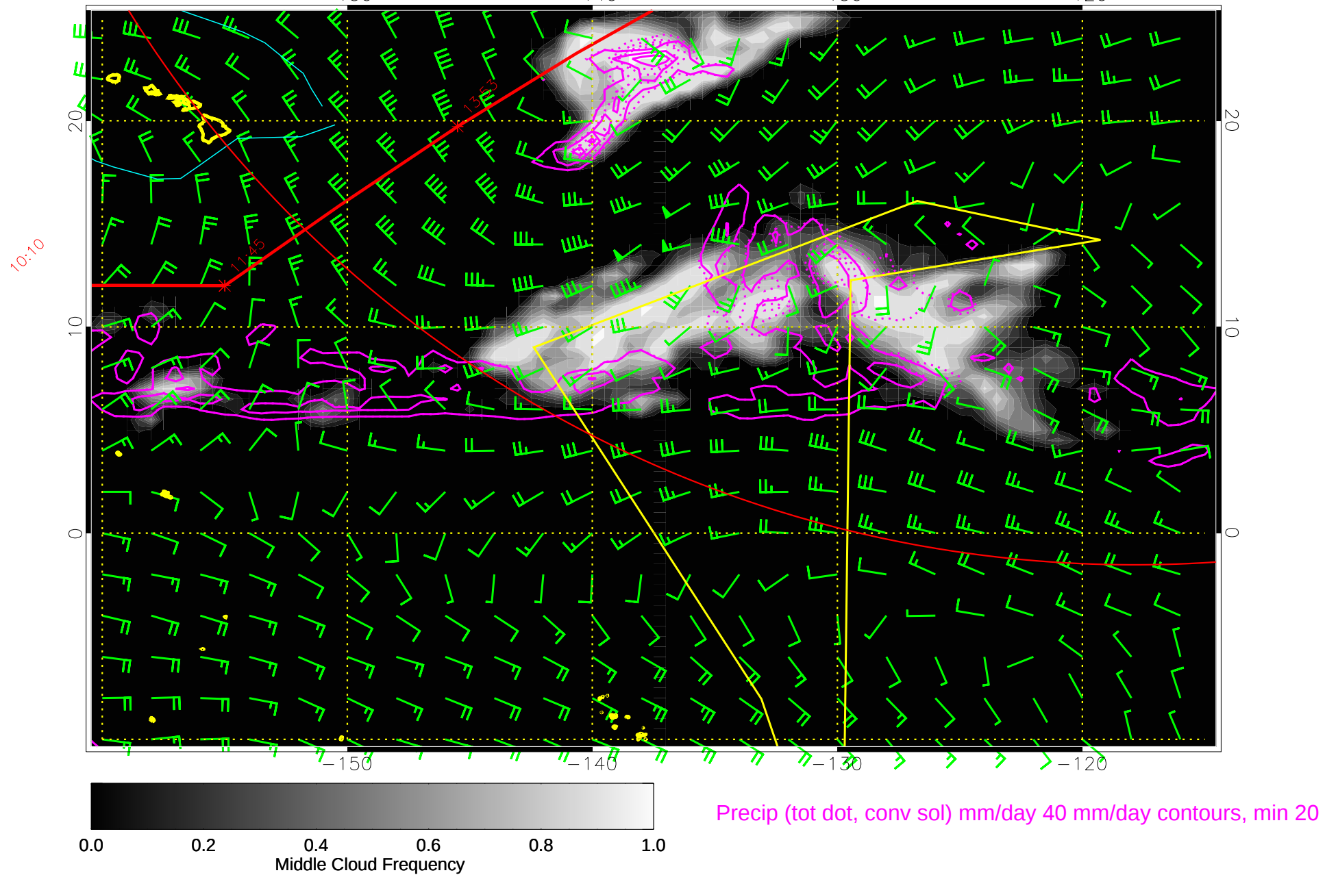
15011118, 6 hour forecast for 500mb winds (knots) and Middle Cloud Frequency -- NCEP GFS
