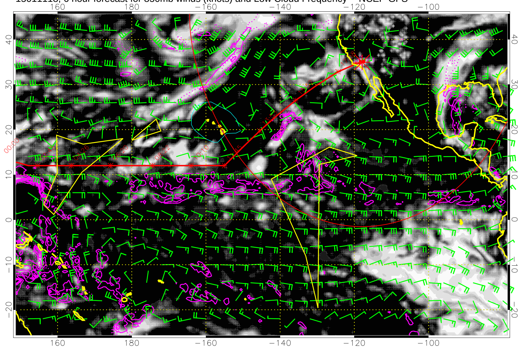
15011118, 6 hour forecast for 850mb winds (knots) and Low Cloud Frequency -- NCEP GFS
