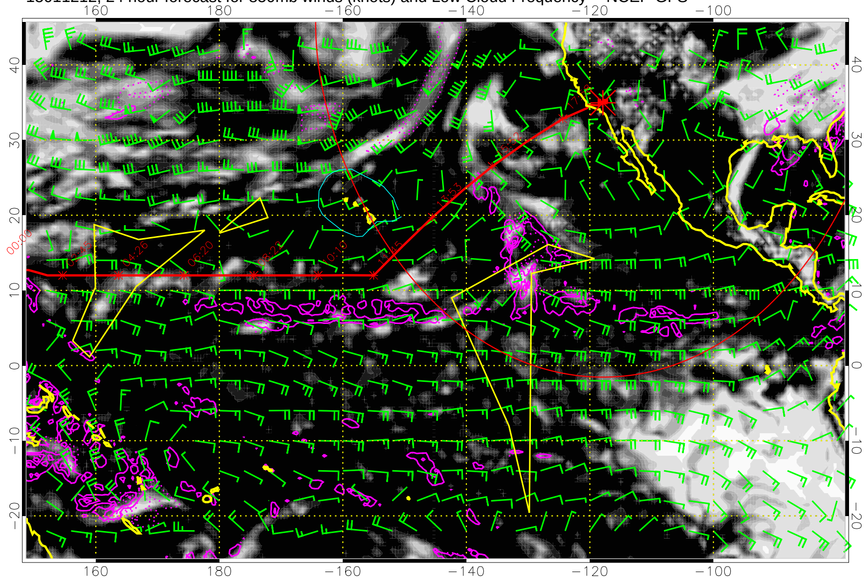
15011212, 24 hour forecast for 850mb winds (knots) and Low Cloud Frequency -- NCEP GFS
