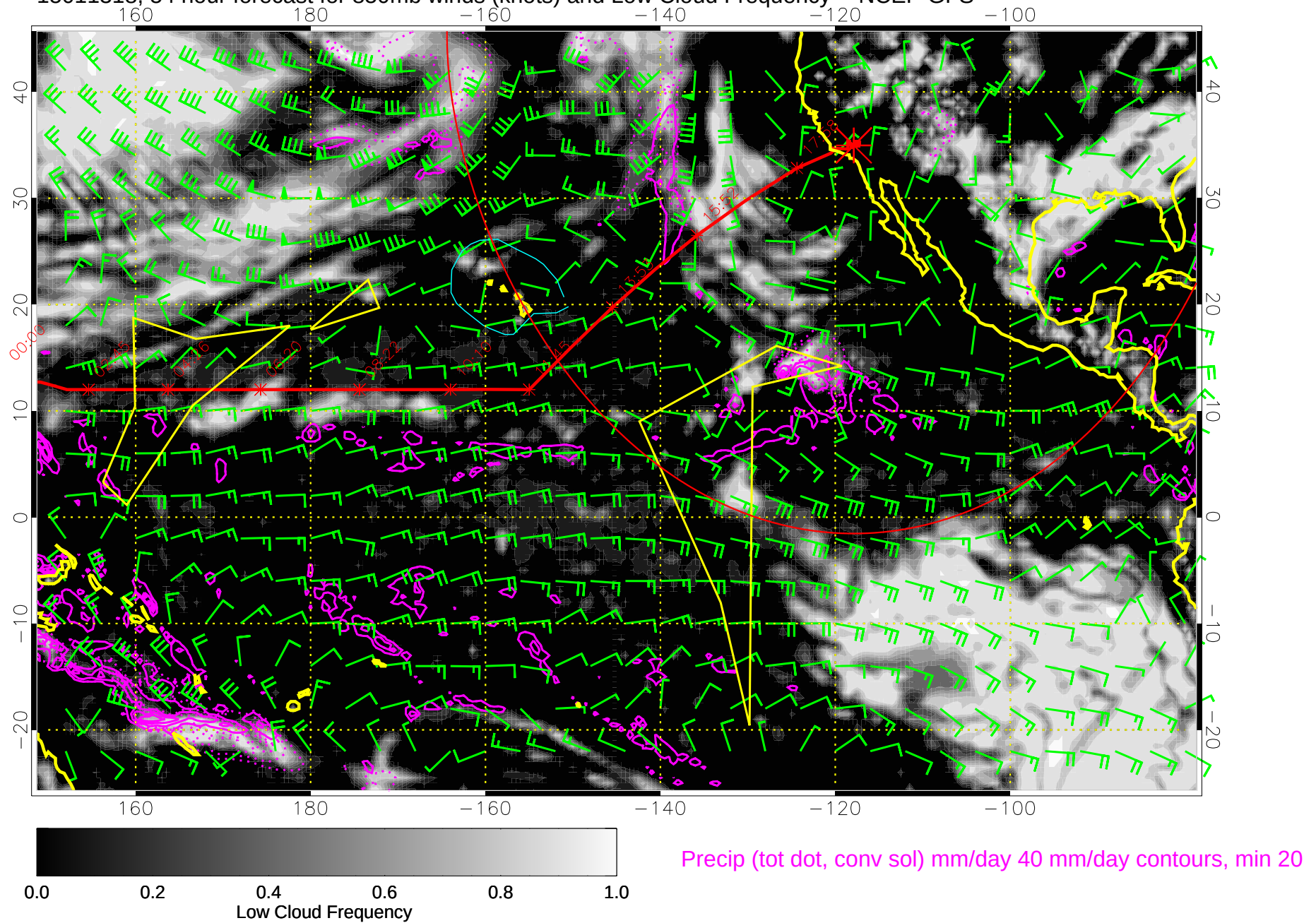
15011318, 54 hour forecast for 850mb winds (knots) and Low Cloud Frequency -- NCEP GFS
