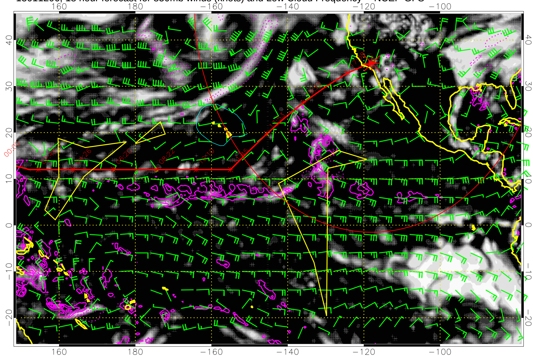
15011206, 18 hour forecast for 850mb winds (knots) and Low Cloud Frequency -- NCEP GFS
