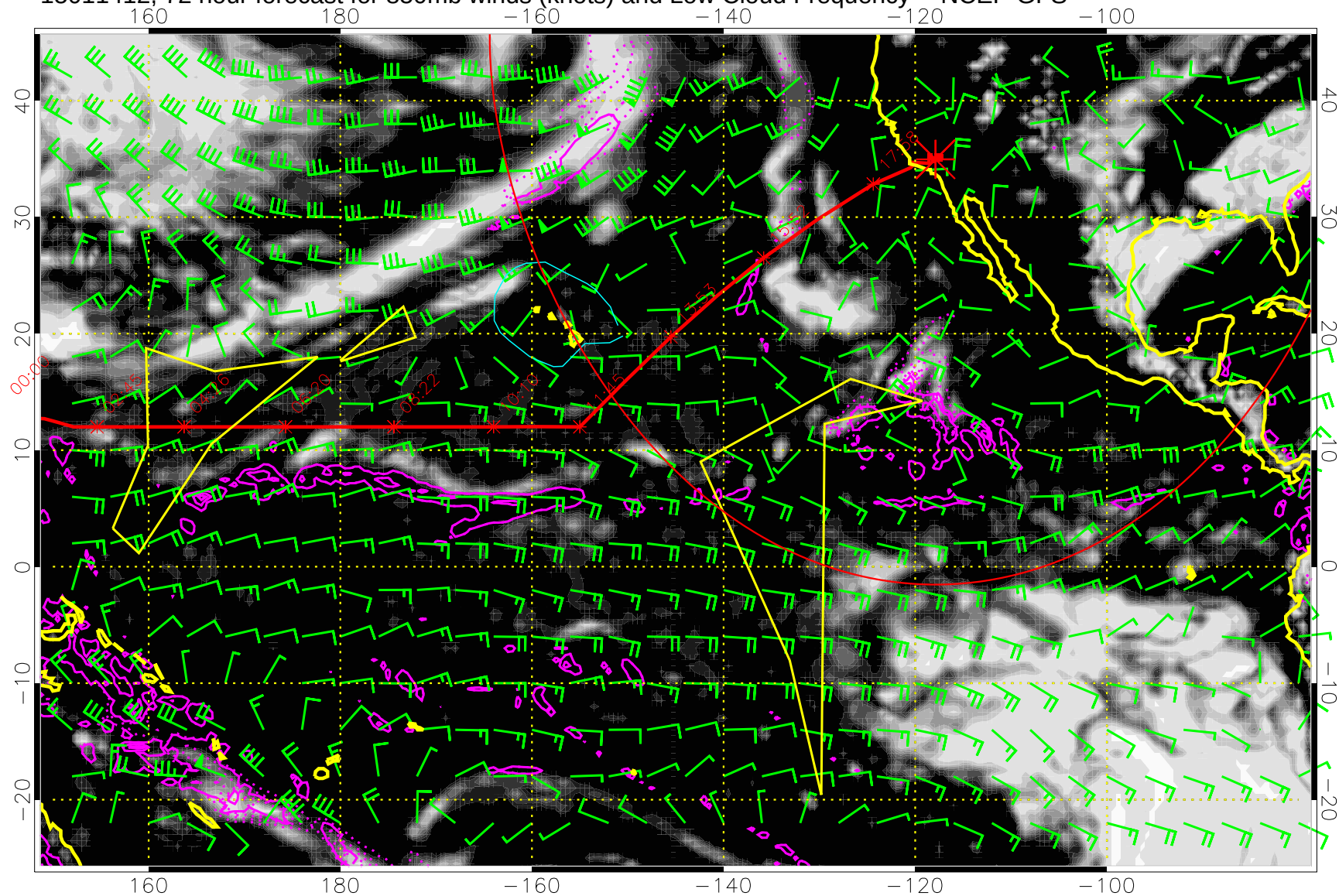
15011412, 72 hour forecast for 850mb winds (knots) and Low Cloud Frequency -- NCEP GFS
