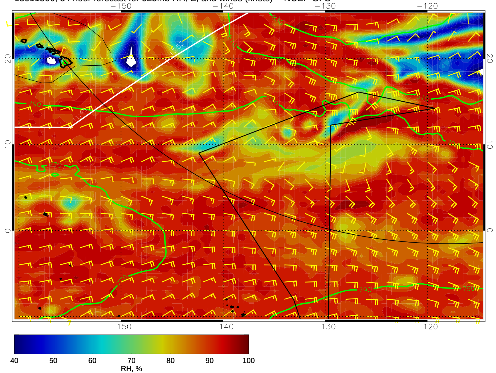
15011306, 54 hour forecast for 925mb RH, Z, and winds (knots) -- NCEP GFS
