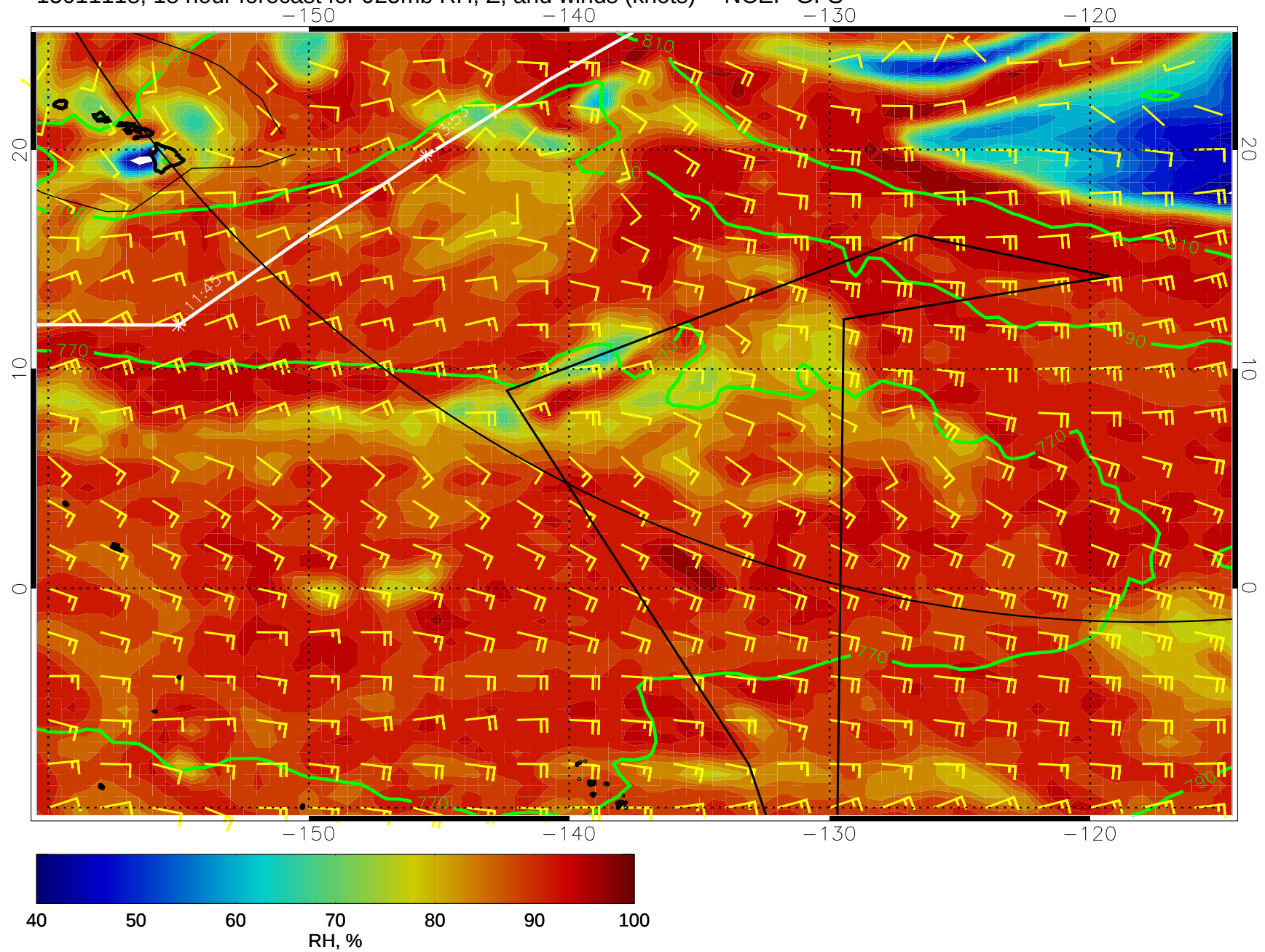
15011118, 18 hour forecast for 925mb RH, Z, and winds (knots) -- NCEP GFS
