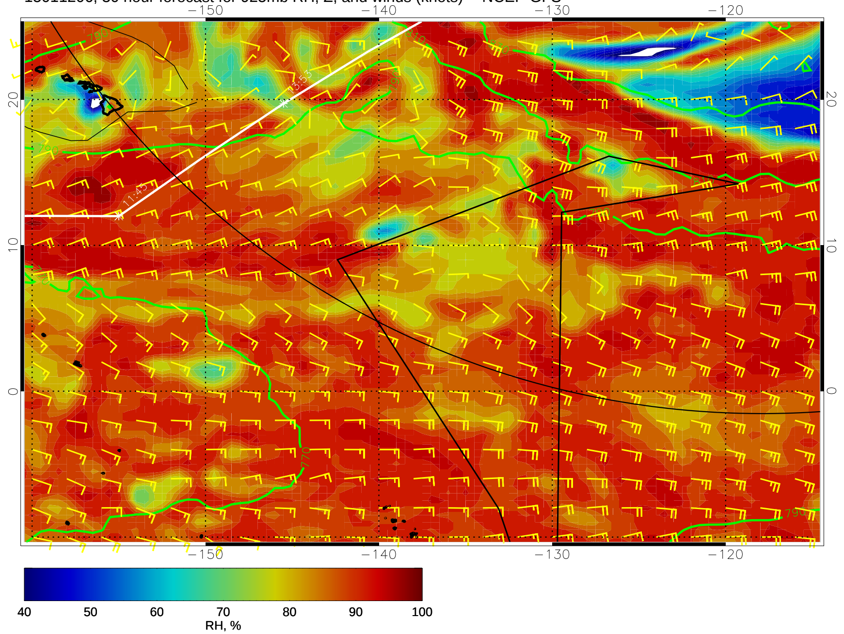
15011206, 30 hour forecast for 925mb RH, Z, and winds (knots) -- NCEP GFS
