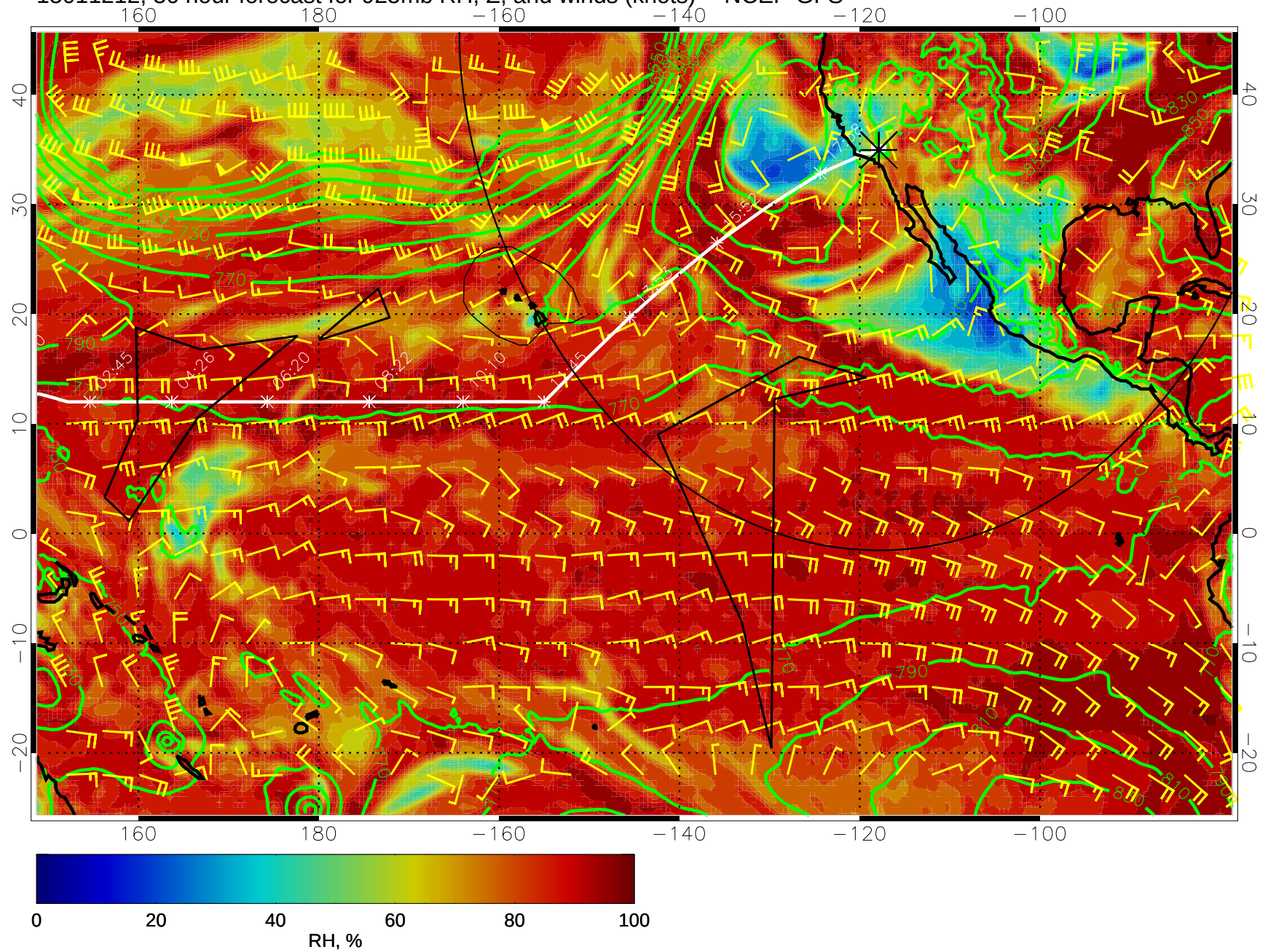
15011212, 36 hour forecast for 925mb RH, Z, and winds (knots) -- NCEP GFS
