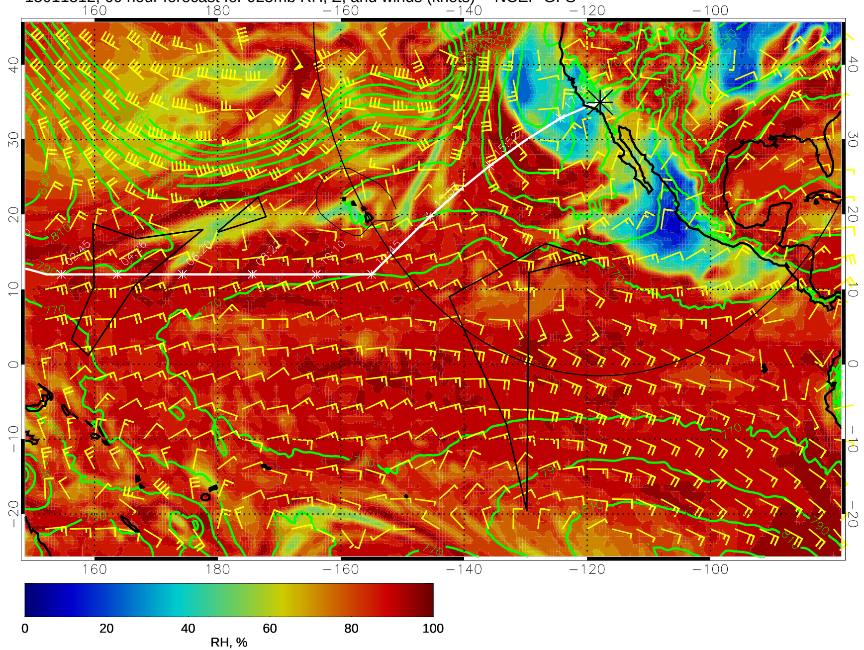
15011312, 60 hour forecast for 925mb RH, Z, and winds (knots) -- NCEP GFS
