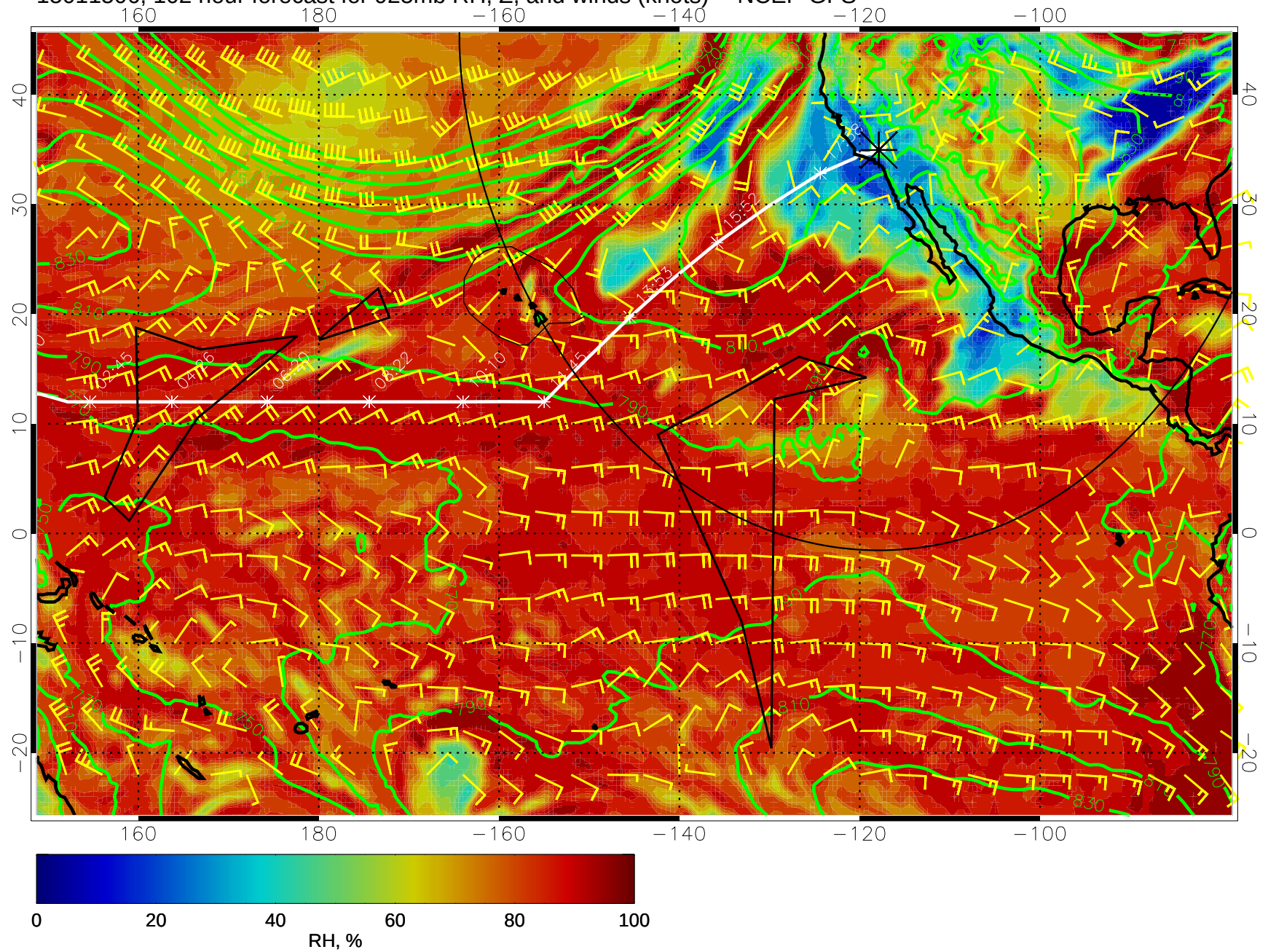
15011506, 102 hour forecast for 925mb RH, Z, and winds (knots) -- NCEP GFS
