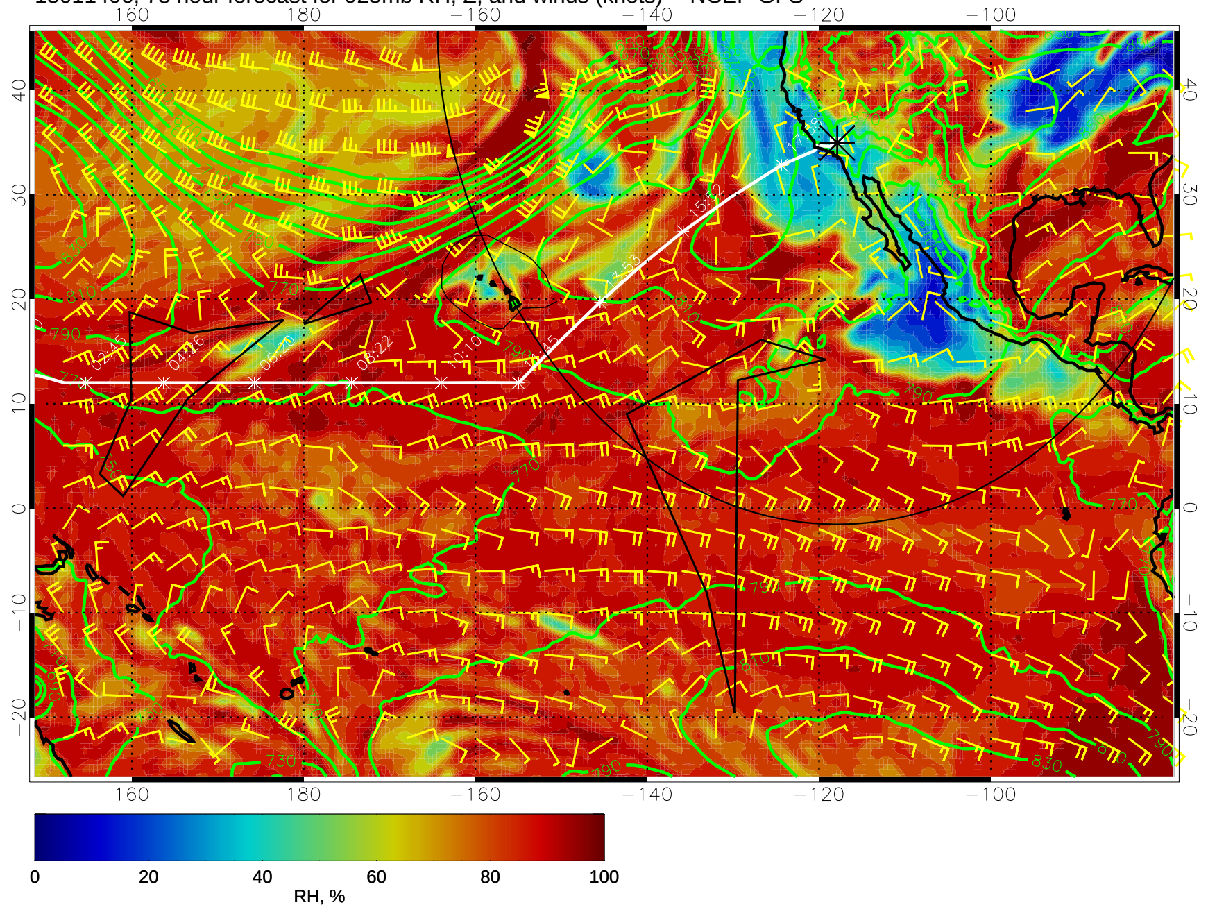
15011406, 78 hour forecast for 925mb RH, Z, and winds (knots) -- NCEP GFS
