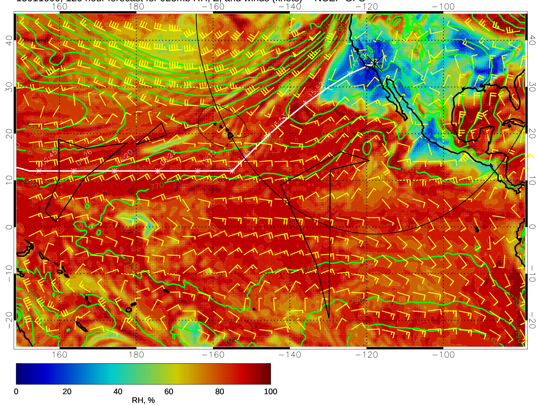
15011600, 120 hour forecast for 925mb RH, Z, and winds (knots) -- NCEP GFS
