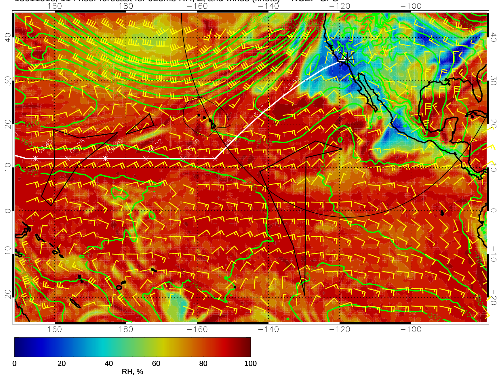
15011518, 114 hour forecast for 925mb RH, Z, and winds (knots) -- NCEP GFS
