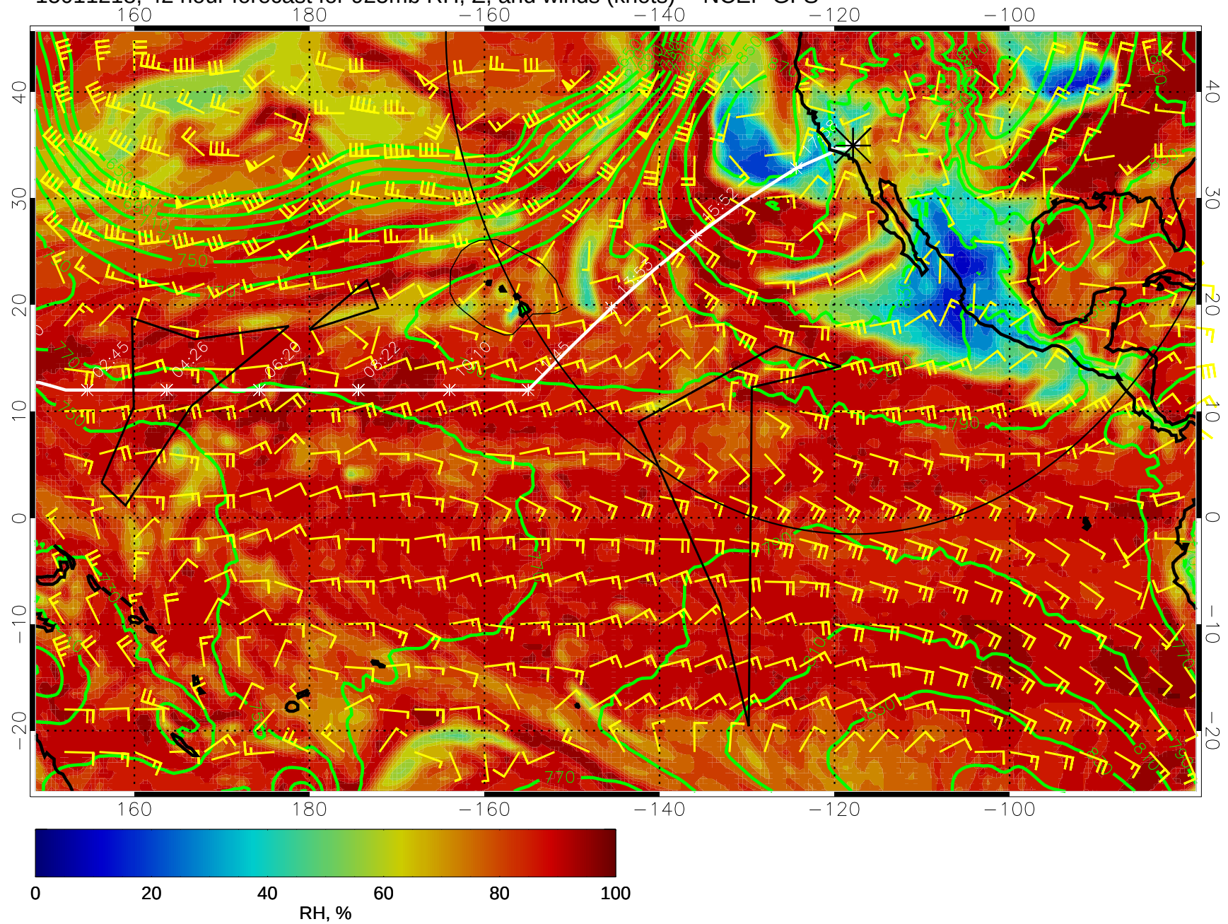
15011218, 42 hour forecast for 925mb RH, Z, and winds (knots) -- NCEP GFS
