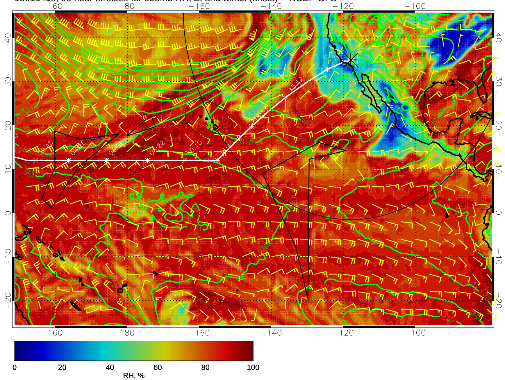
15011418, 90 hour forecast for 925mb RH, Z, and winds (knots) -- NCEP GFS
