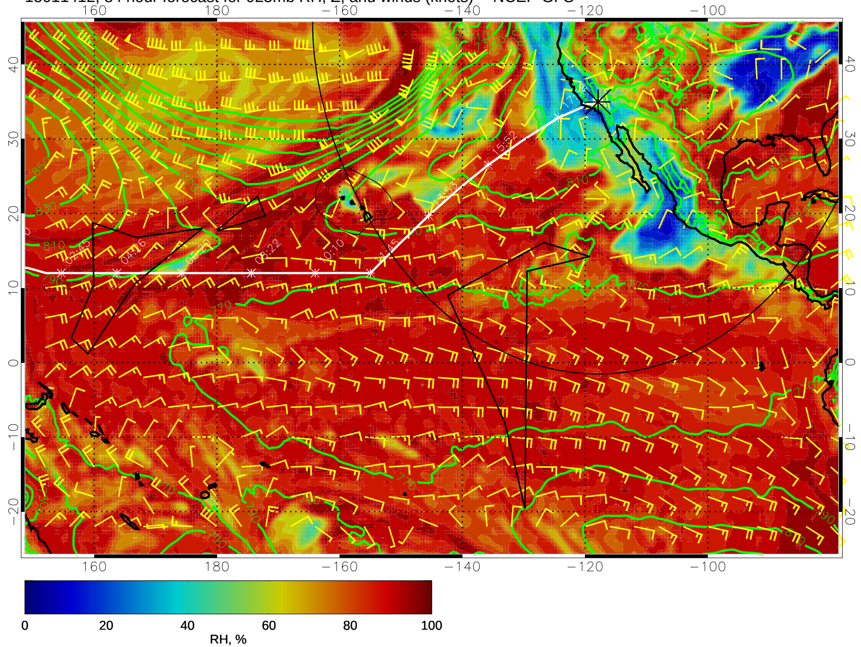
15011412, 84 hour forecast for 925mb RH, Z, and winds (knots) -- NCEP GFS
