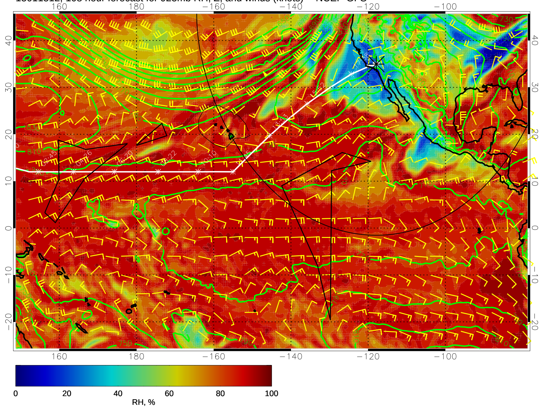
15011512, 108 hour forecast for 925mb RH, Z, and winds (knots) -- NCEP GFS
