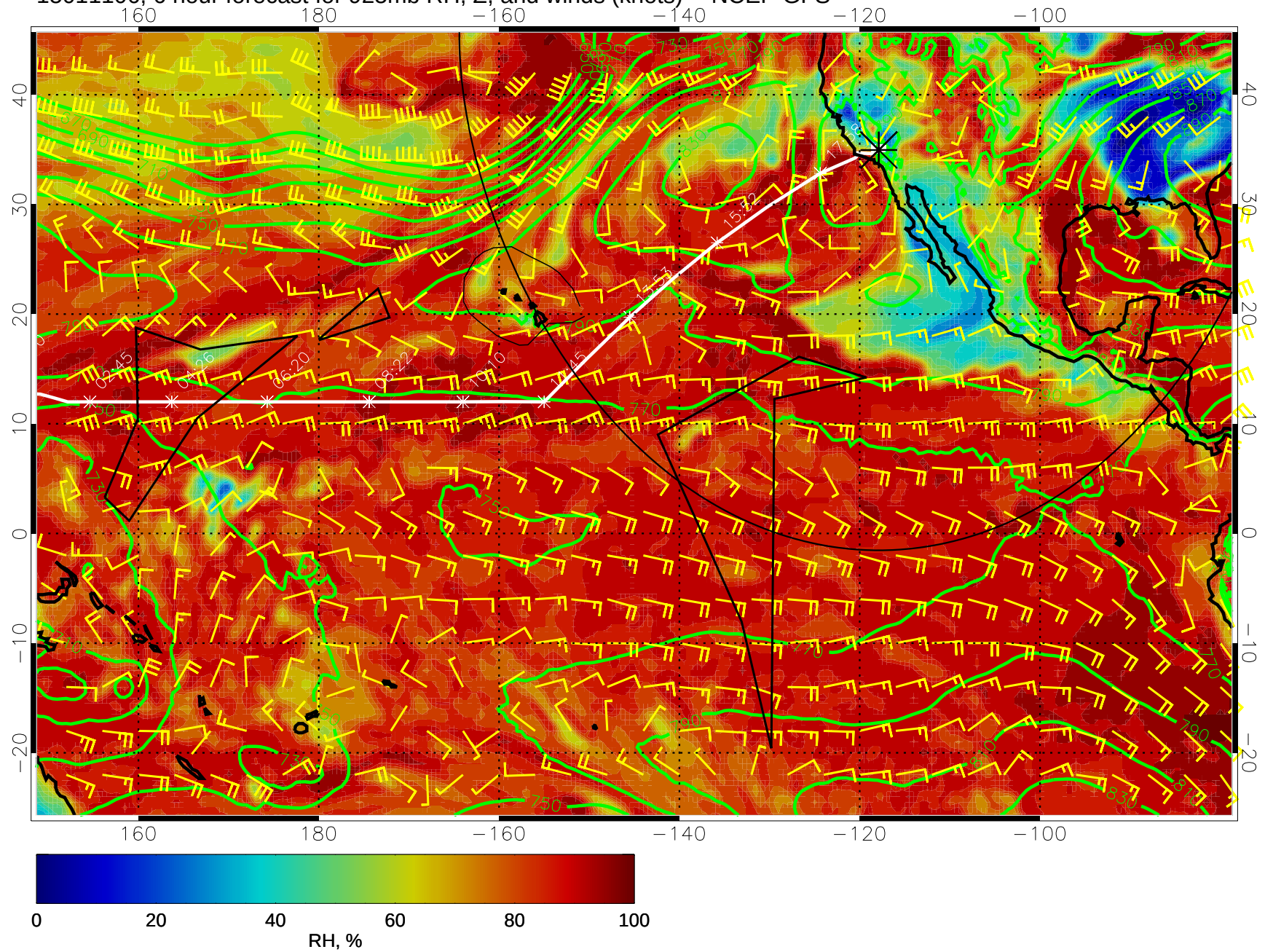
15011106, 6 hour forecast for 925mb RH, Z, and winds (knots) -- NCEP GFS
