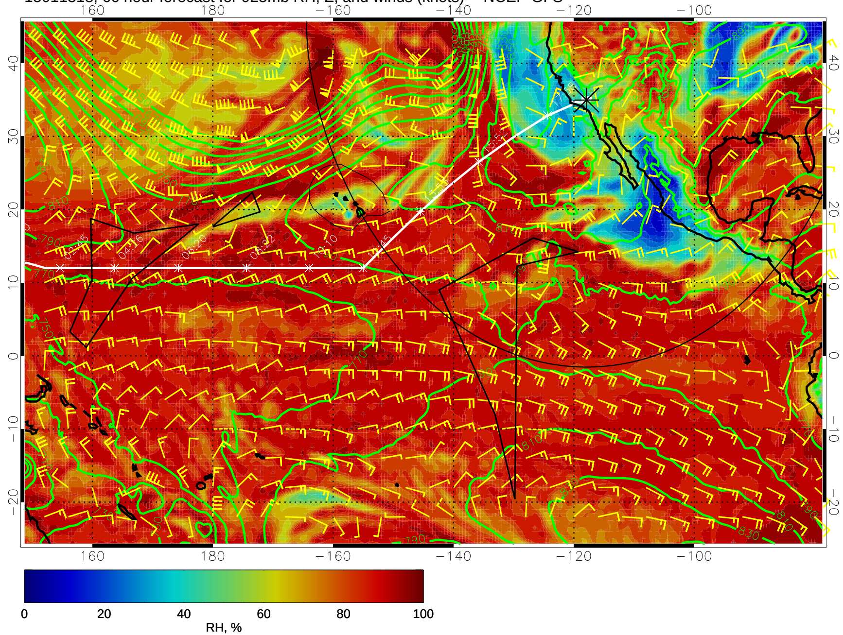
15011318, 66 hour forecast for 925mb RH, Z, and winds (knots) -- NCEP GFS
