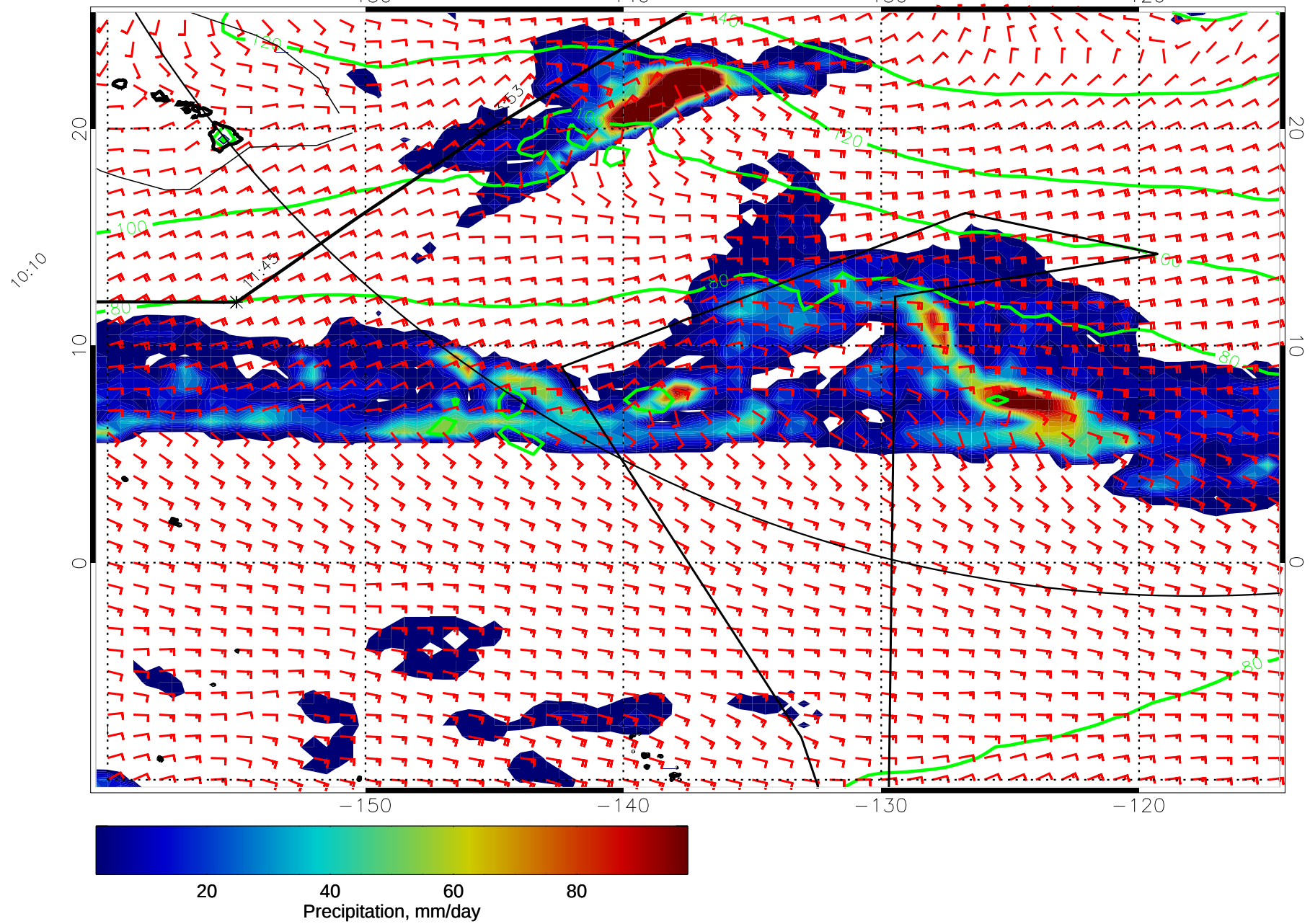
15011112, 12 hour forecast for precip, 1000mb Z, and winds (knots) -- NCEP GFS
