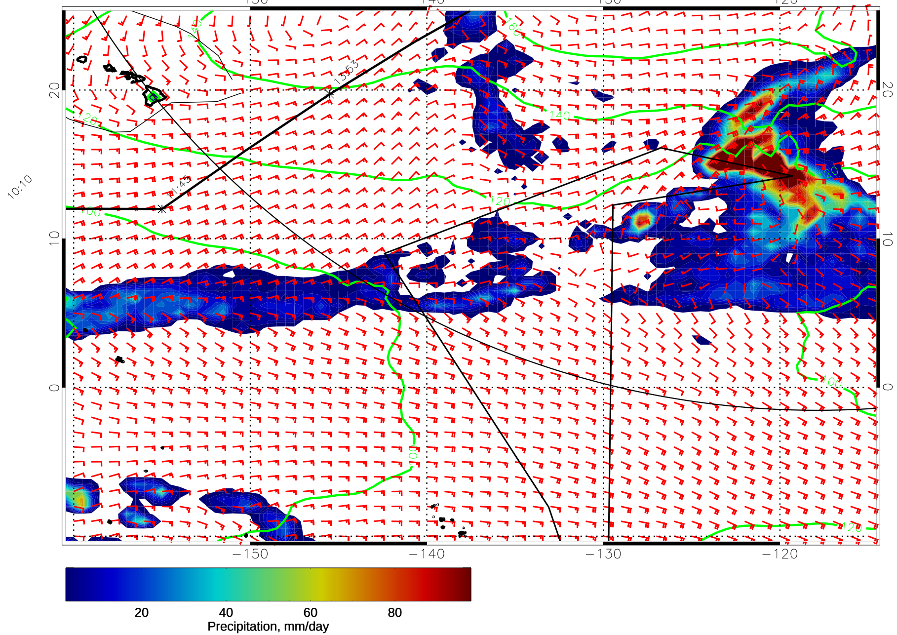
15011406, 78 hour forecast for precip, 1000mb Z, and winds (knots) -- NCEP GFS
