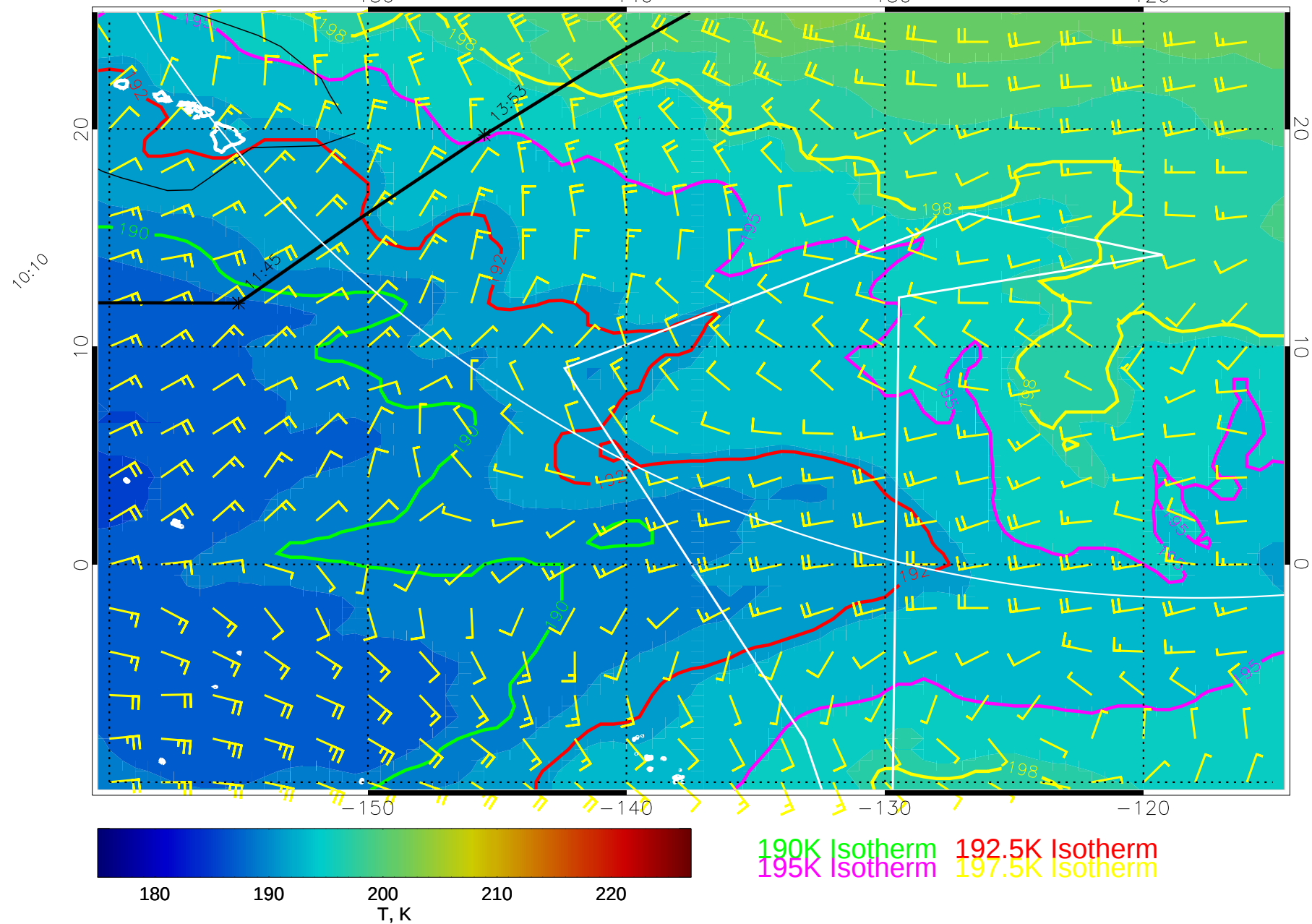
15011106, 6 hour forecast for 70mb T and winds (knots) -- NCEP GFS
