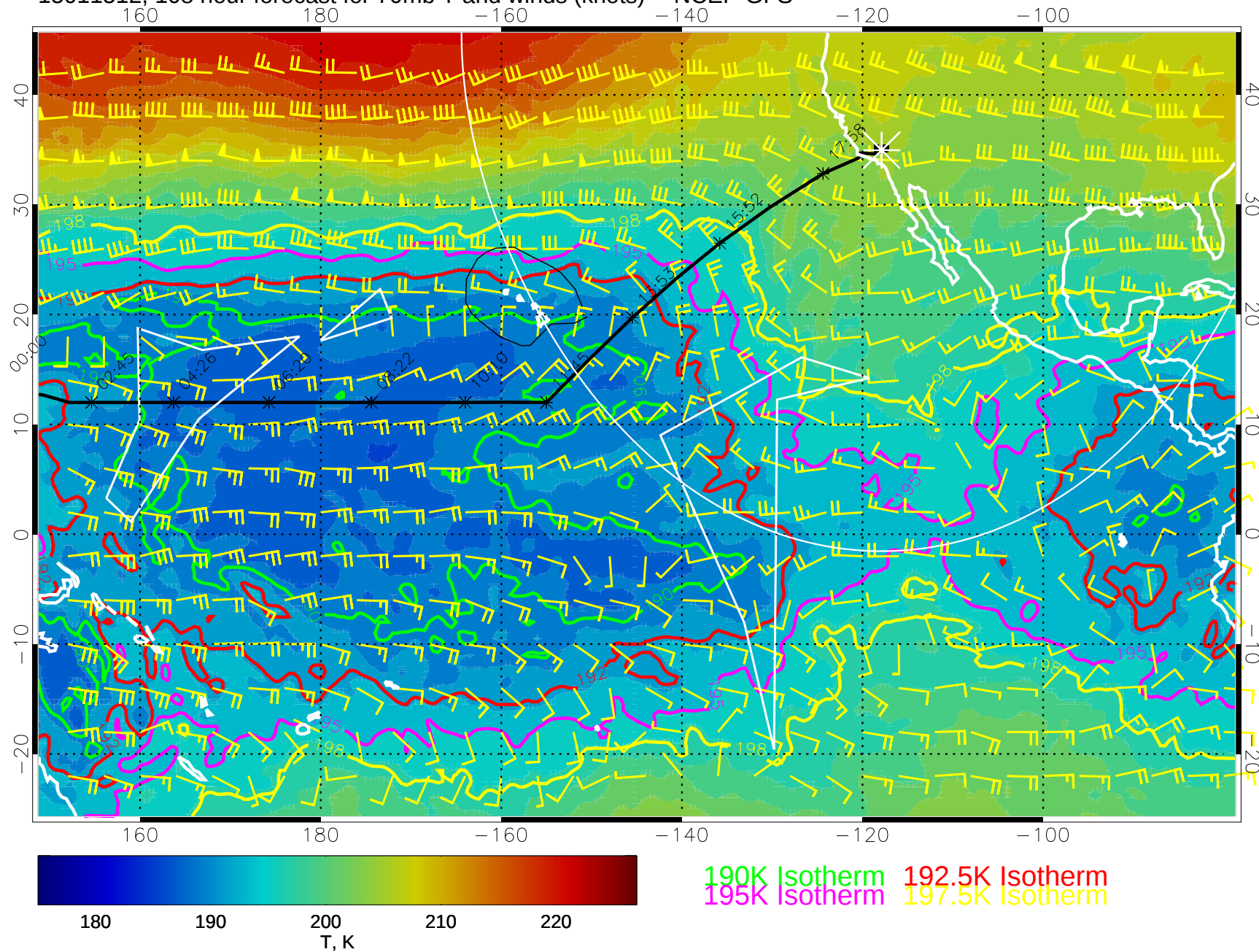
15011512, 108 hour forecast for 70mb T and winds (knots) -- NCEP GFS
