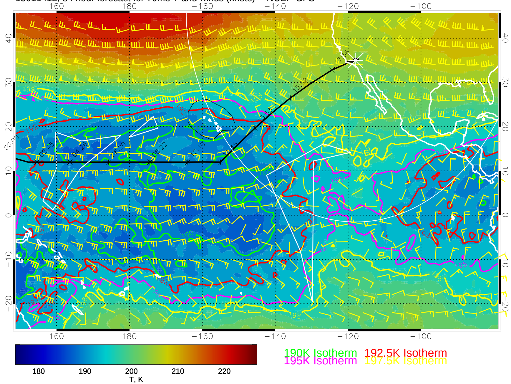
15011412, 84 hour forecast for 70mb T and winds (knots) -- NCEP GFS
