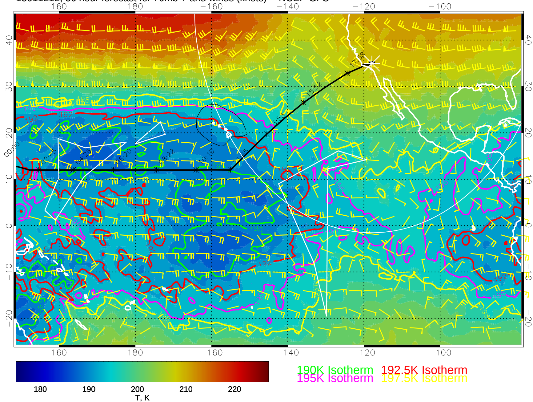
15011212, 36 hour forecast for 70mb T and winds (knots) -- NCEP GFS
