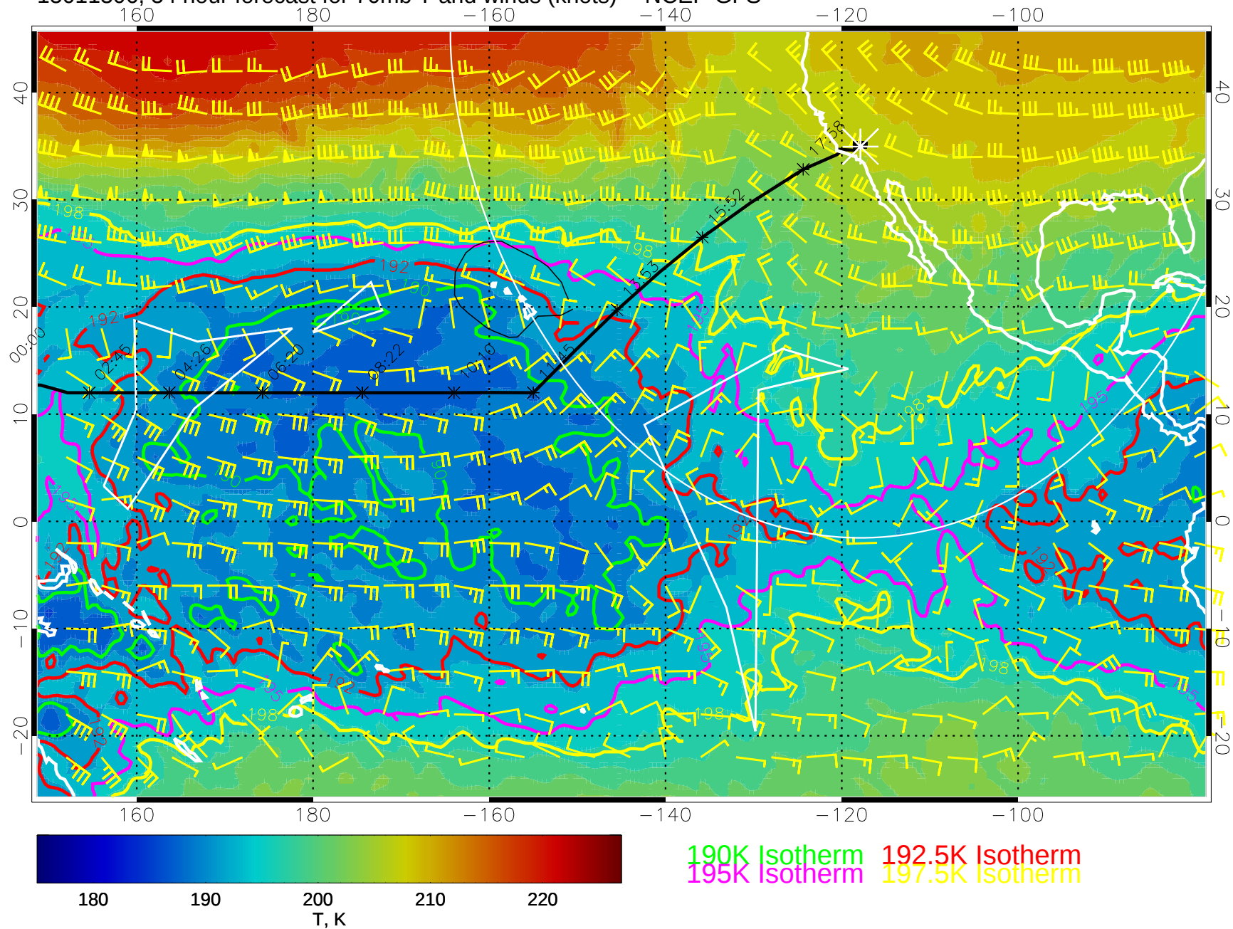
15011306, 54 hour forecast for 70mb T and winds (knots) -- NCEP GFS
