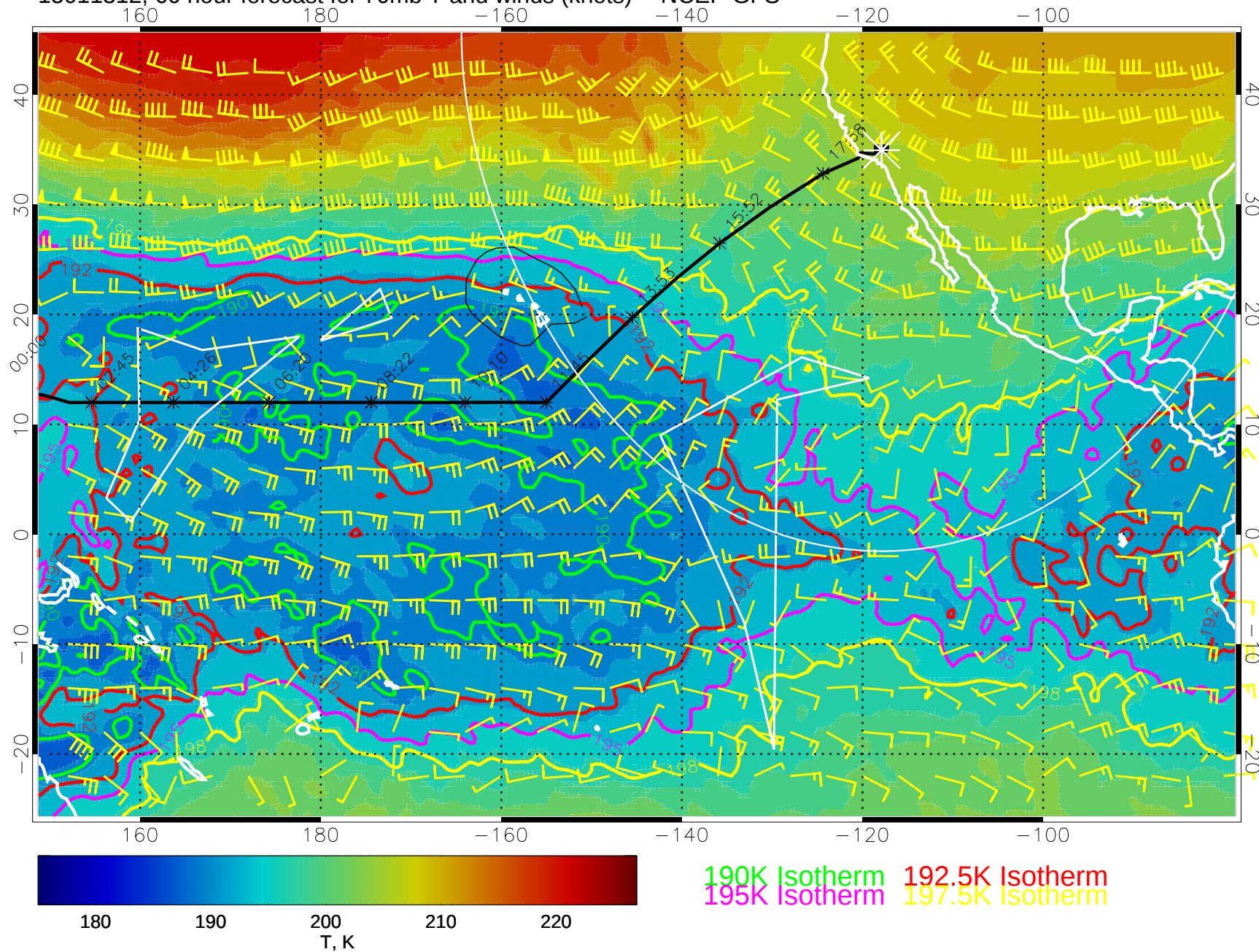
15011312, 60 hour forecast for 70mb T and winds (knots) -- NCEP GFS
