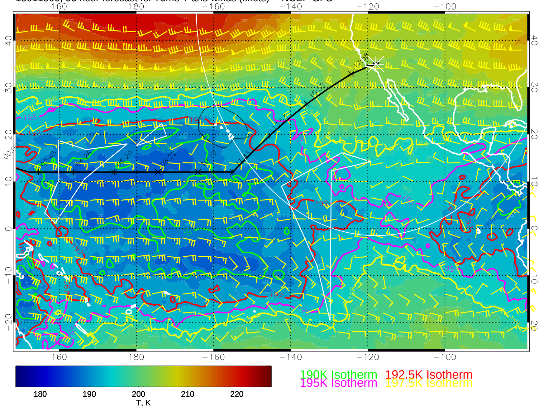
15011500, 96 hour forecast for 70mb T and winds (knots) -- NCEP GFS
