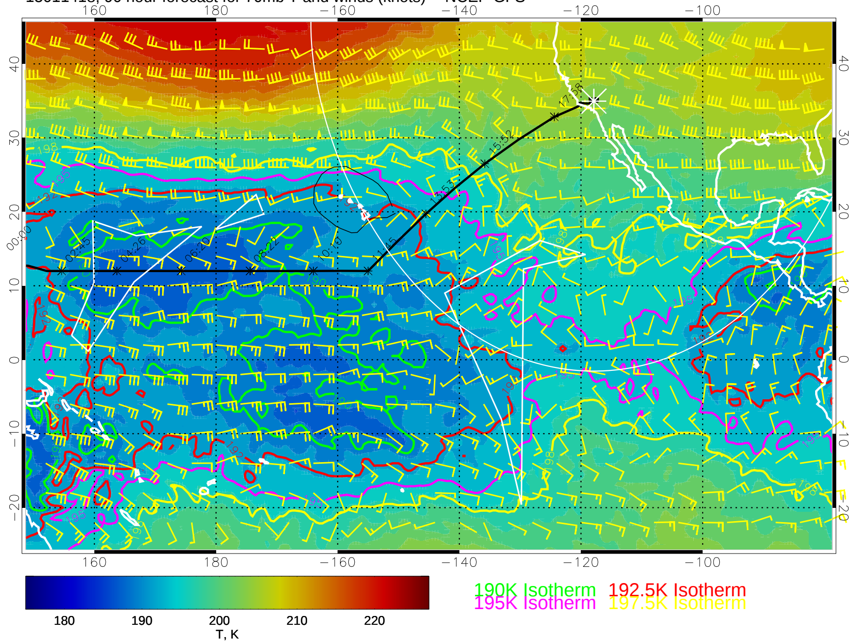
15011418, 90 hour forecast for 70mb T and winds (knots) -- NCEP GFS
