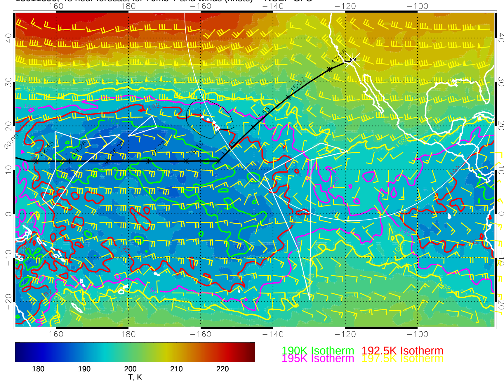
15011300, 48 hour forecast for 70mb T and winds (knots) -- NCEP GFS
