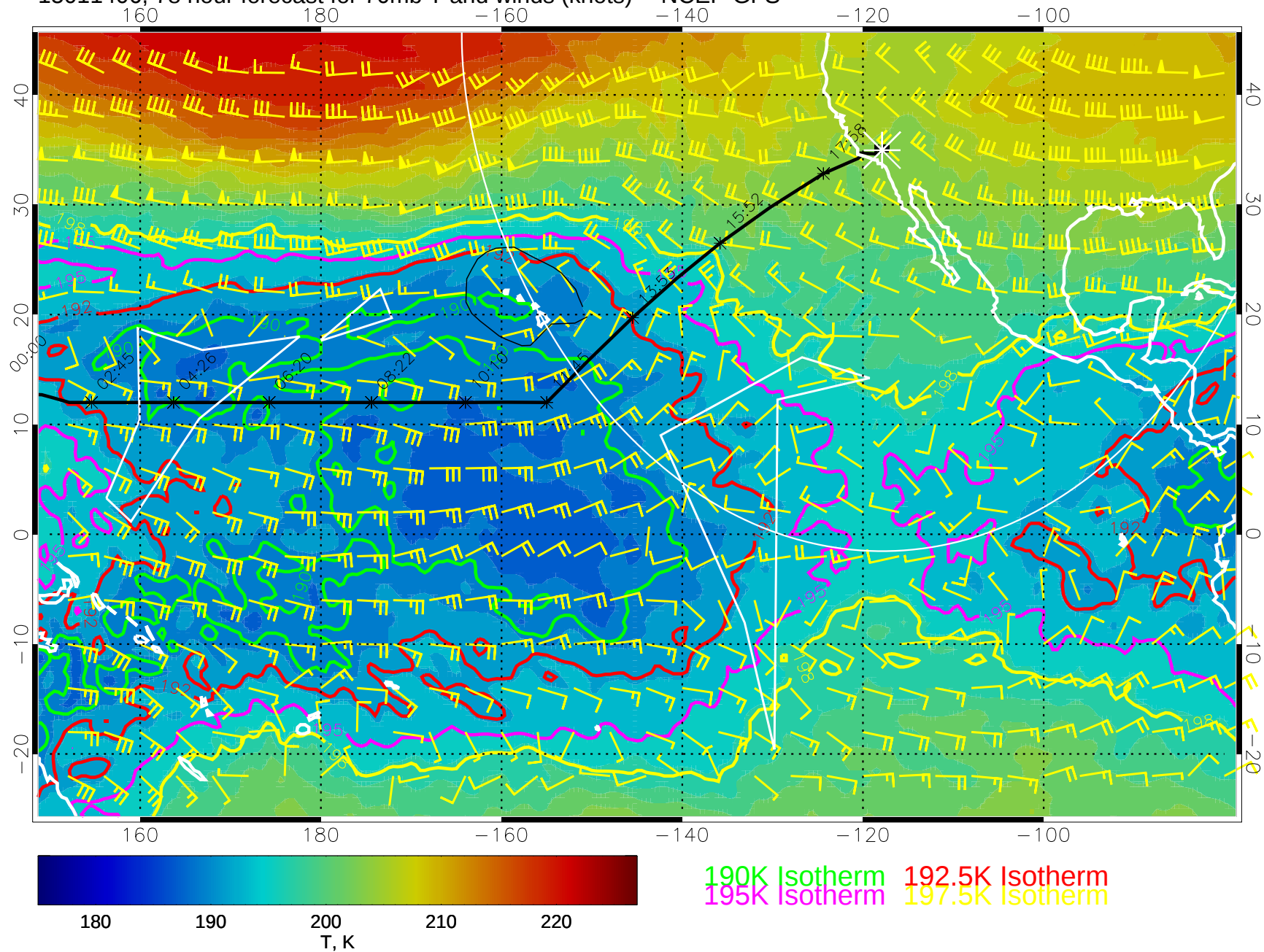
15011406, 78 hour forecast for 70mb T and winds (knots) -- NCEP GFS
