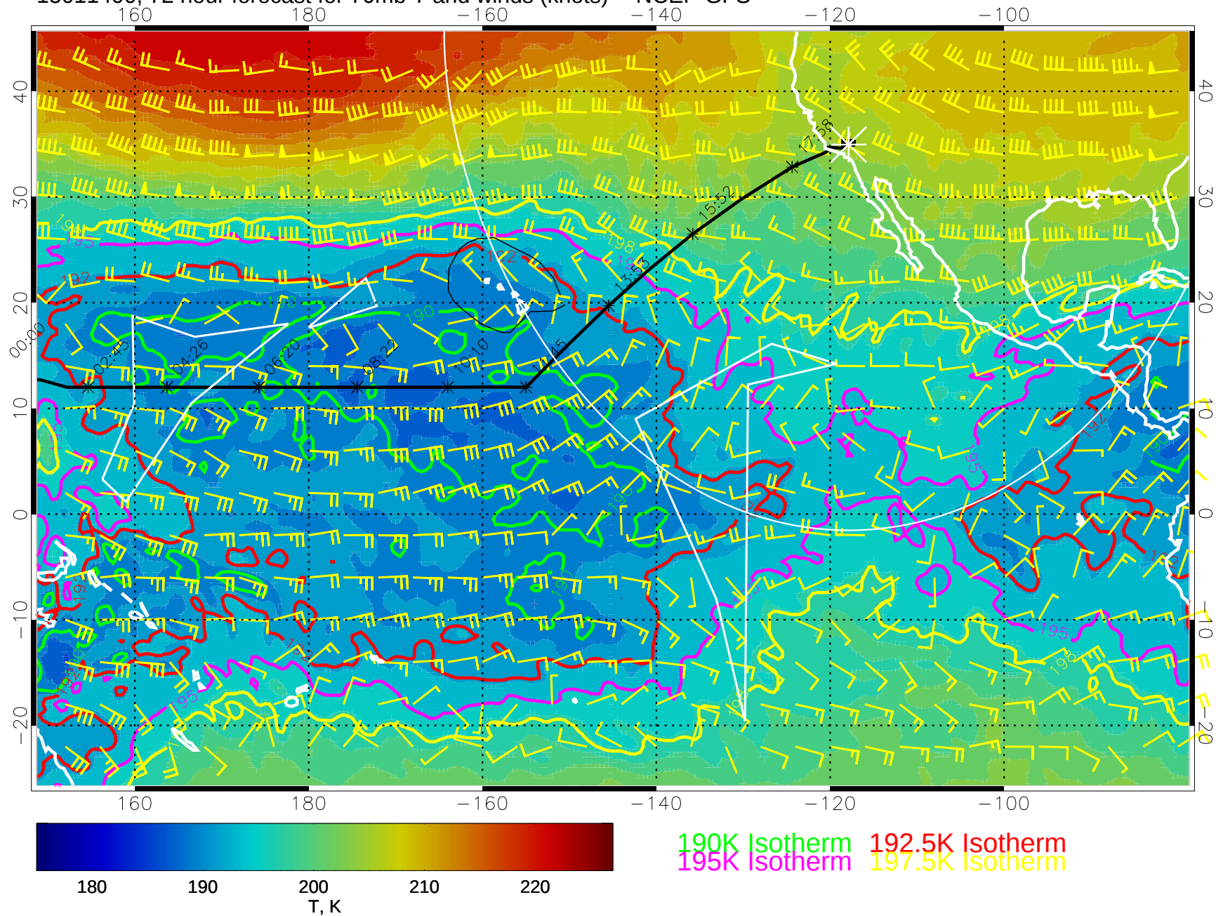
15011400, 72 hour forecast for 70mb T and winds (knots) -- NCEP GFS
