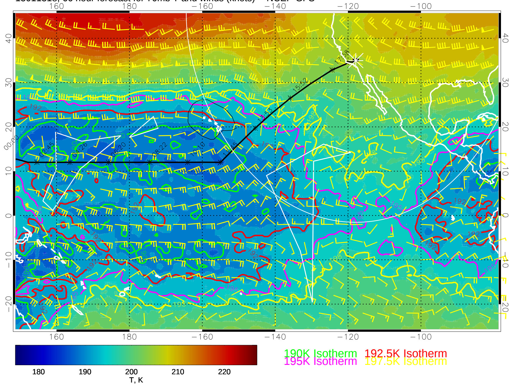
15011318, 66 hour forecast for 70mb T and winds (knots) -- NCEP GFS
