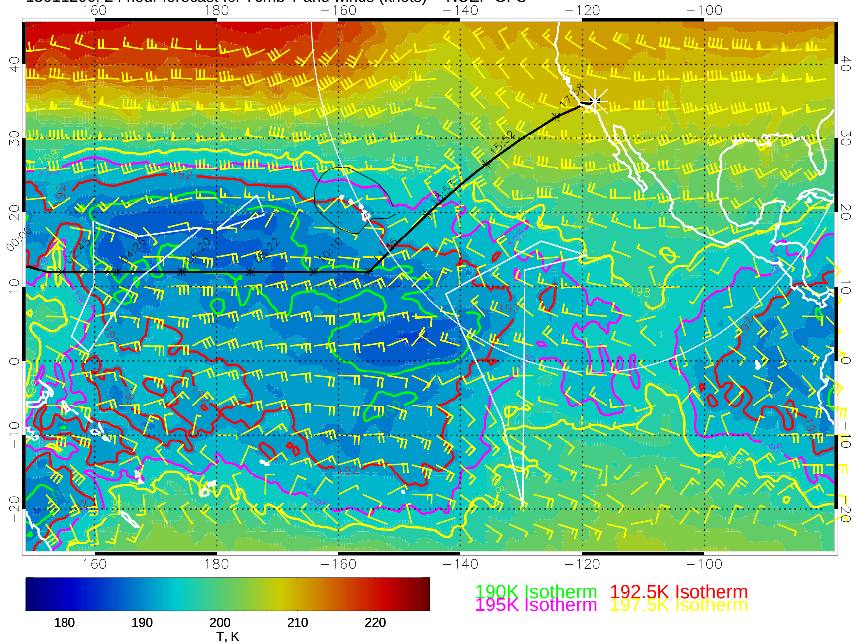
15011200, 24 hour forecast for 70mb T and winds (knots) -- NCEP GFS
