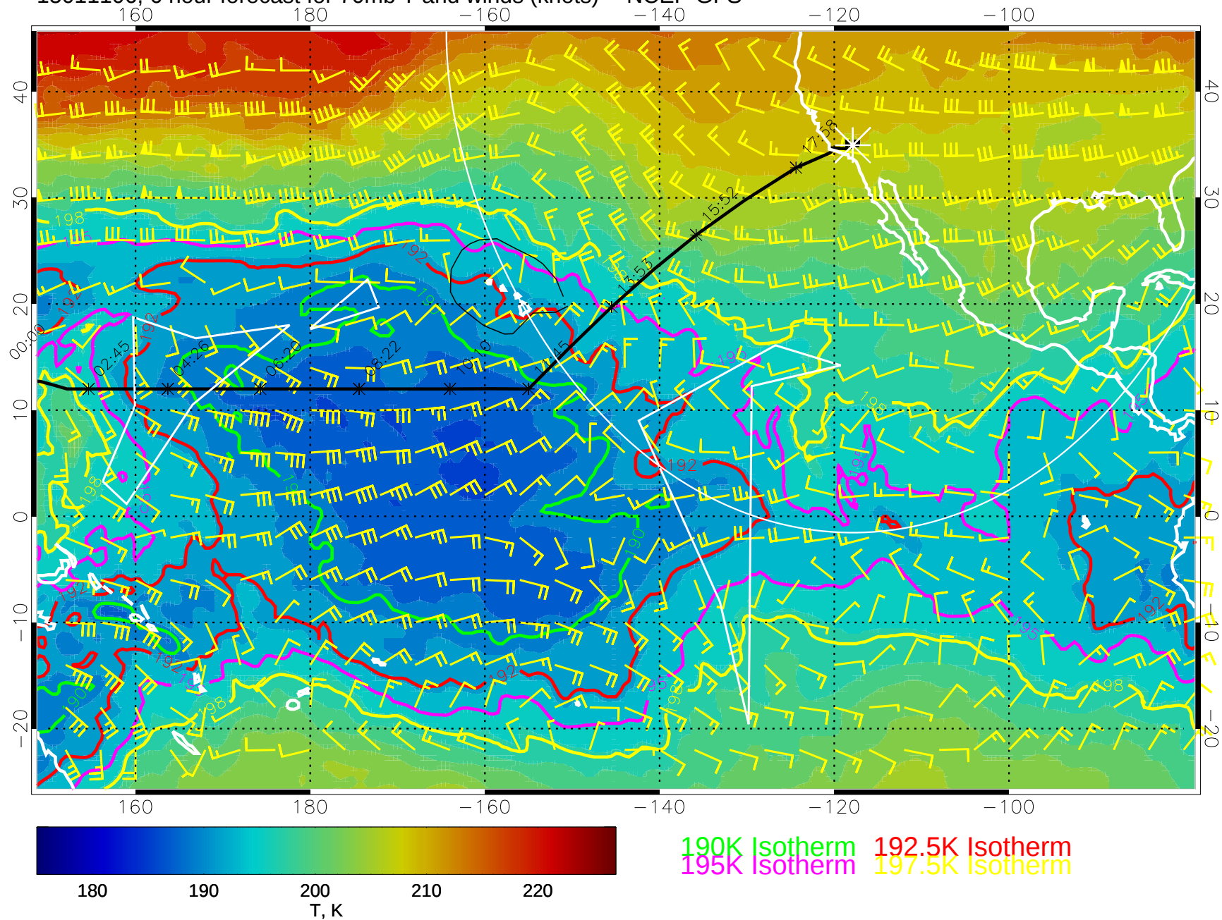
15011106, 6 hour forecast for 70mb T and winds (knots) -- NCEP GFS
