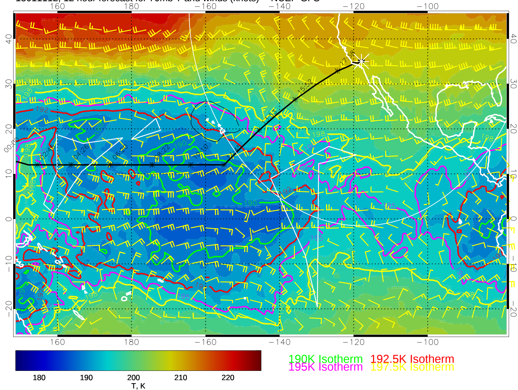
15011112, 12 hour forecast for 70mb T and winds (knots) -- NCEP GFS
