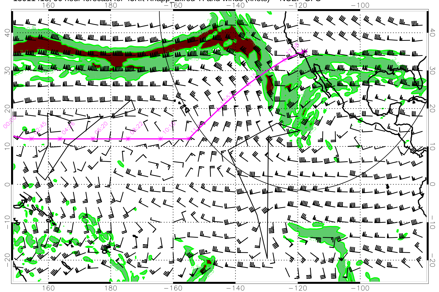
15011418, 90 hour forecast for 45Kft Knapp_Ellrod TI and winds (knots) -- NCEP GFS
