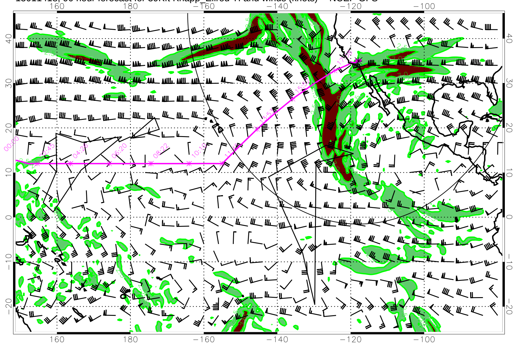
15011418, 90 hour forecast for 39Kft Knapp_Ellrod TI and winds (knots) -- NCEP GFS
