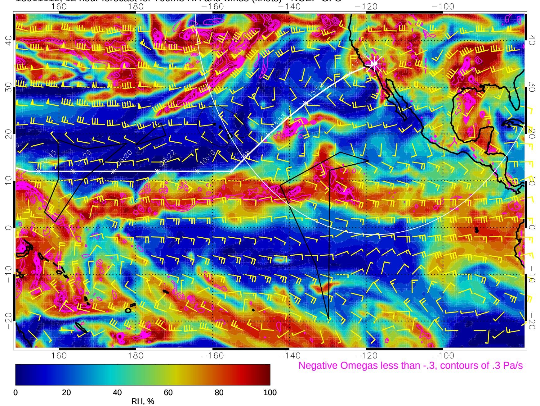
15011112, 12 hour forecast for 700mb RH and winds (knots) - NCEP GFS
