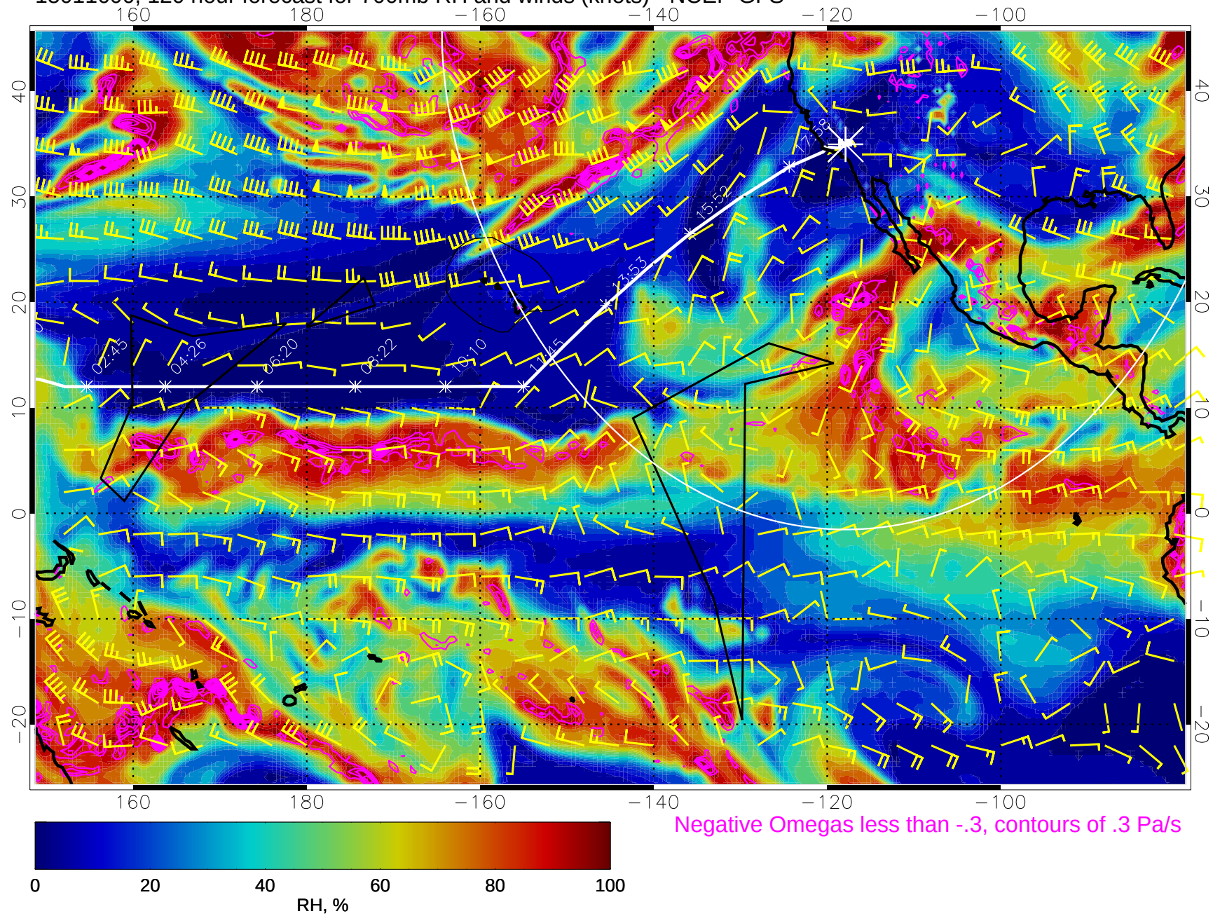
15011600, 120 hour forecast for 700mb RH and winds (knots) - NCEP GFS
