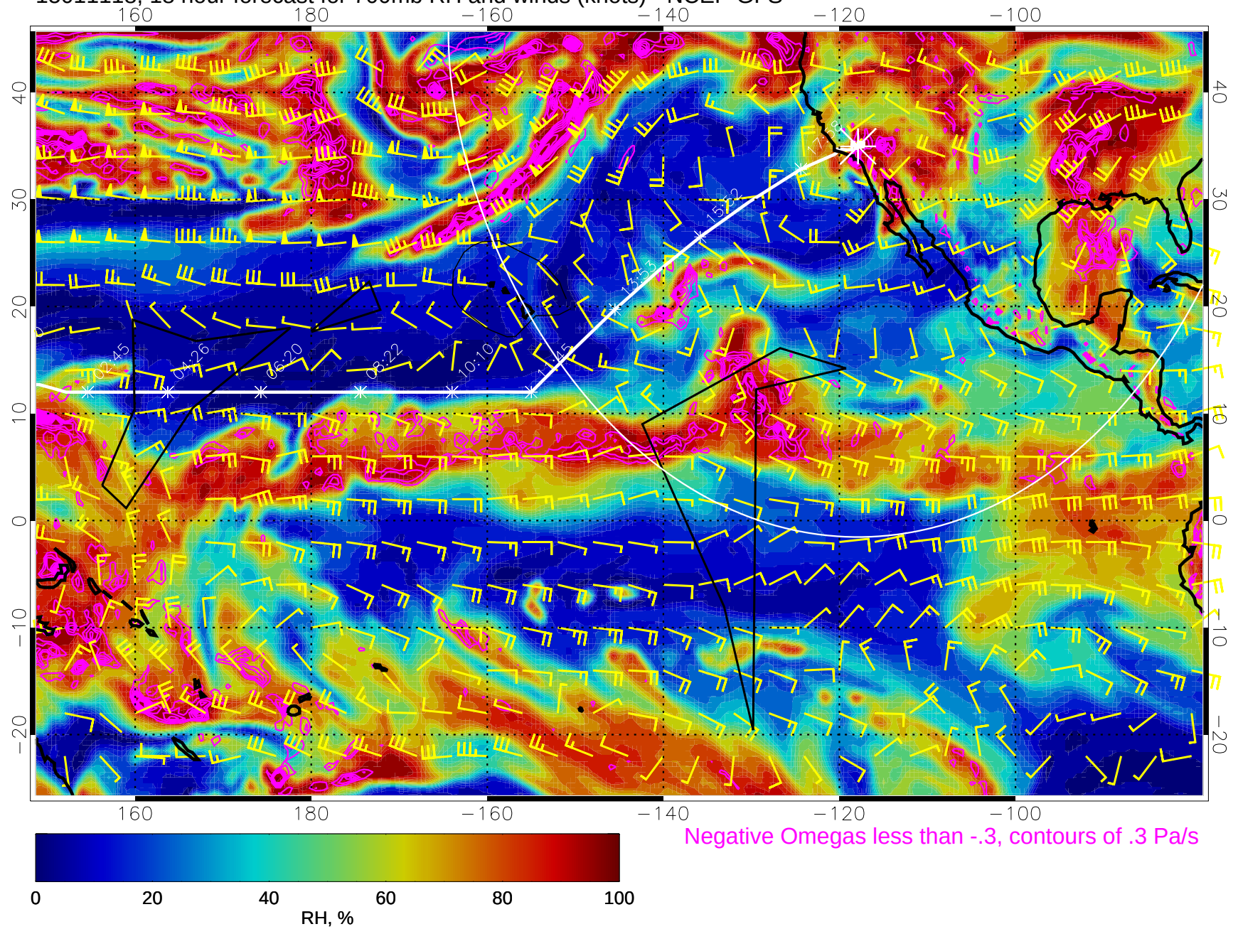
15011118, 18 hour forecast for 700mb RH and winds (knots) - NCEP GFS
