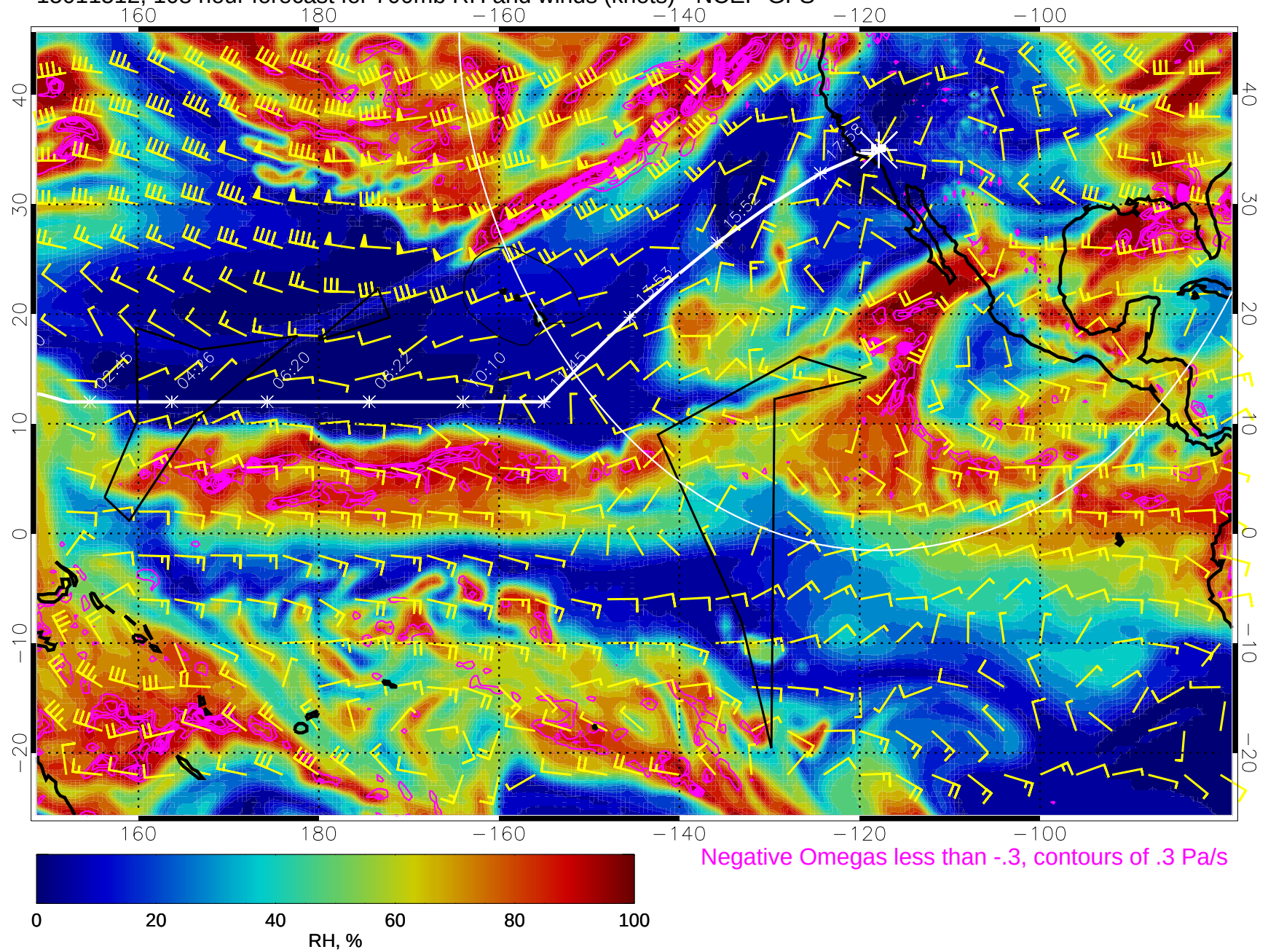
15011512, 108 hour forecast for 700mb RH and winds (knots) - NCEP GFS
