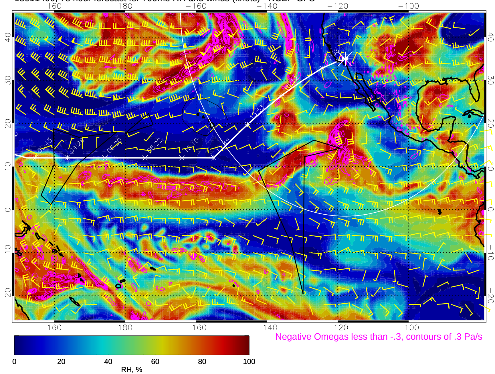
15011406, 78 hour forecast for 700mb RH and winds (knots) - NCEP GFS
