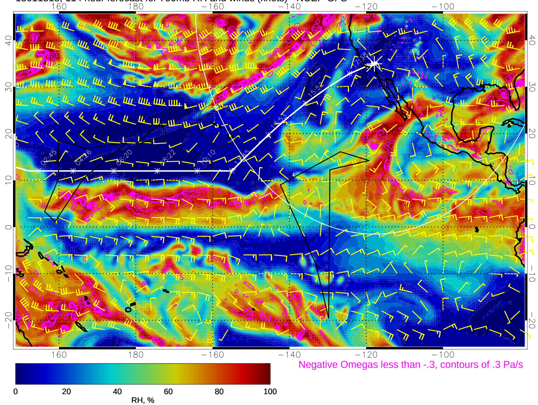
15011518, 114 hour forecast for 700mb RH and winds (knots) - NCEP GFS
