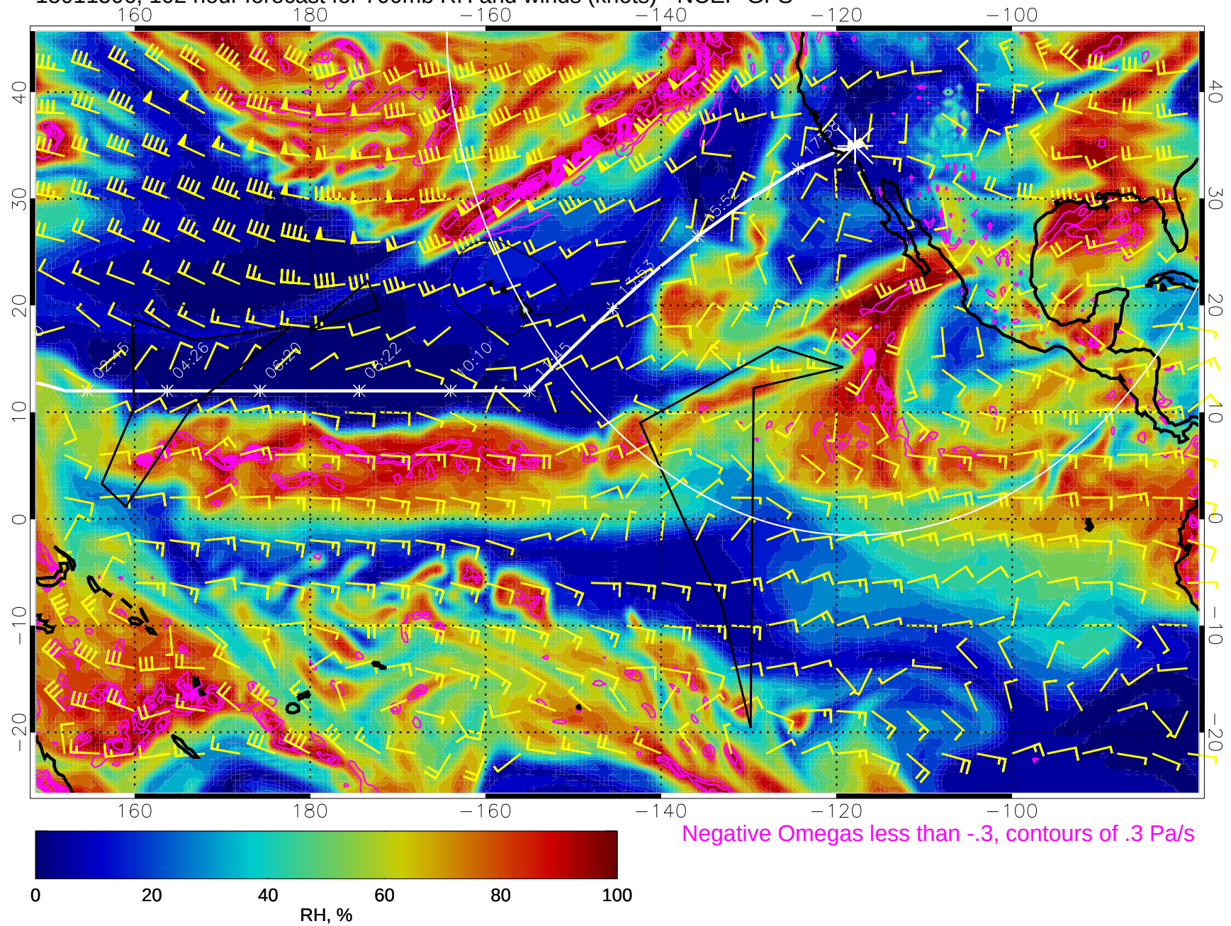
15011506, 102 hour forecast for 700mb RH and winds (knots) - NCEP GFS
