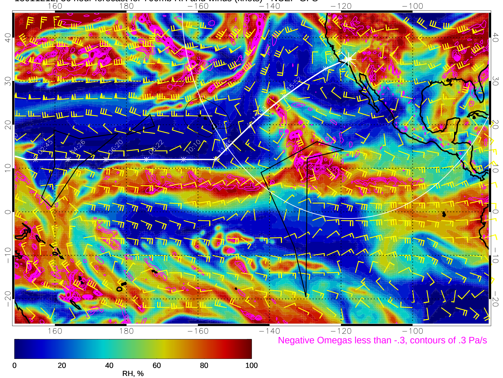
15011212, 36 hour forecast for 700mb RH and winds (knots) - NCEP GFS
