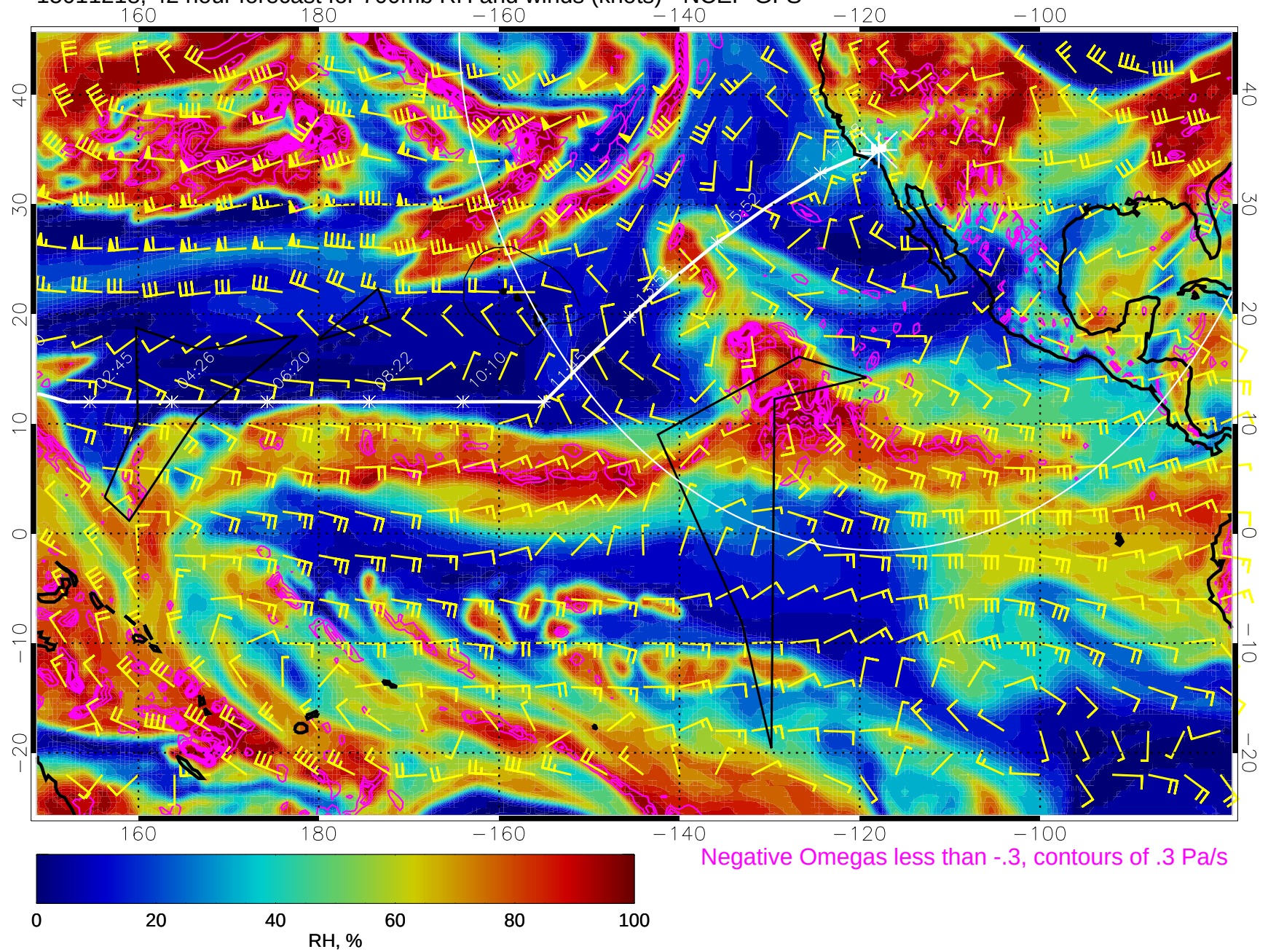
15011218, 42 hour forecast for 700mb RH and winds (knots) - NCEP GFS
