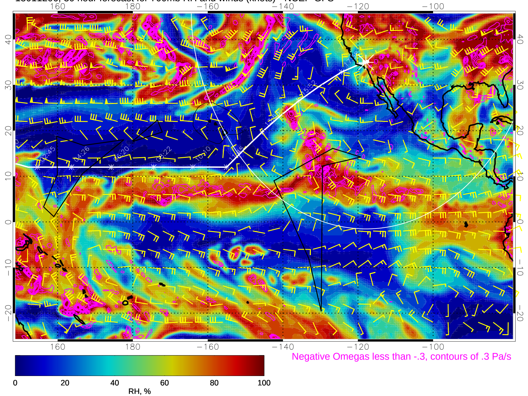
15011206, 30 hour forecast for 700mb RH and winds (knots) - NCEP GFS
