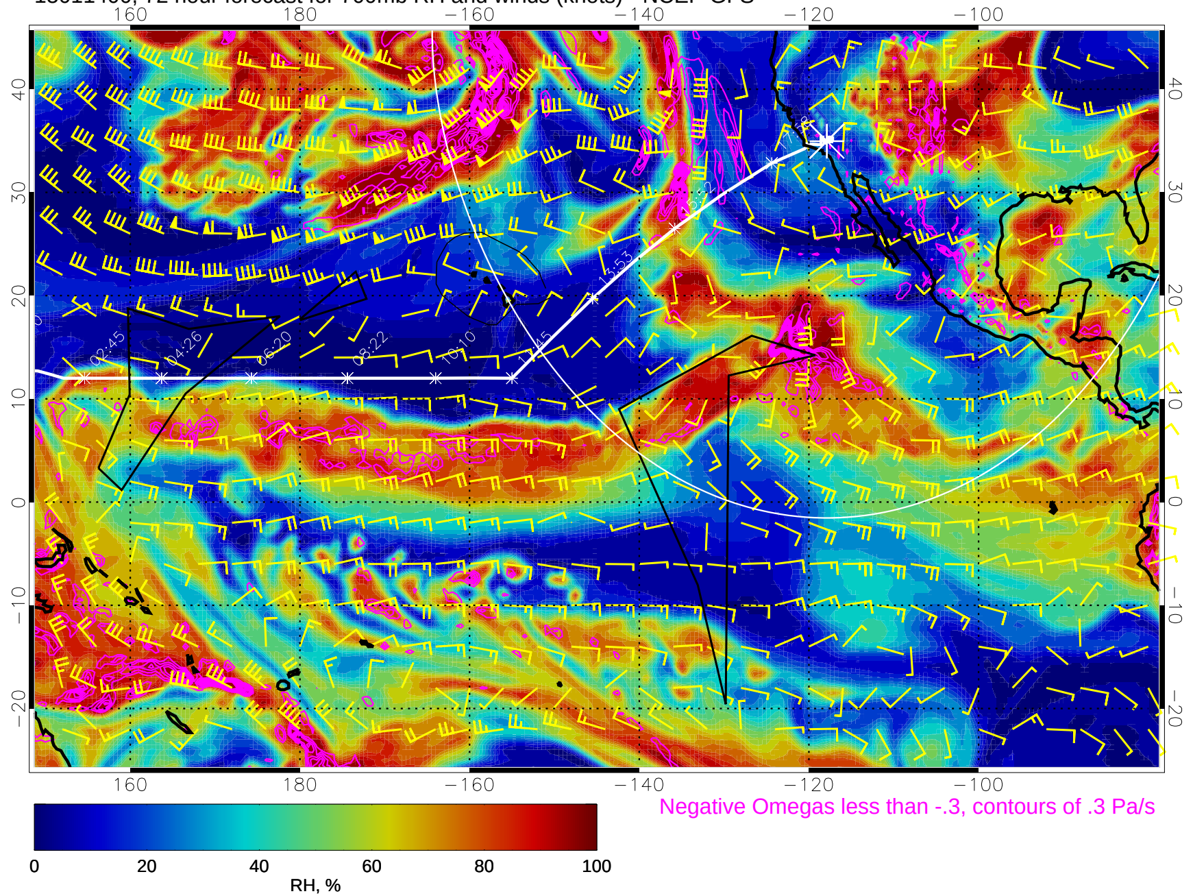
15011400, 72 hour forecast for 700mb RH and winds (knots) - NCEP GFS
