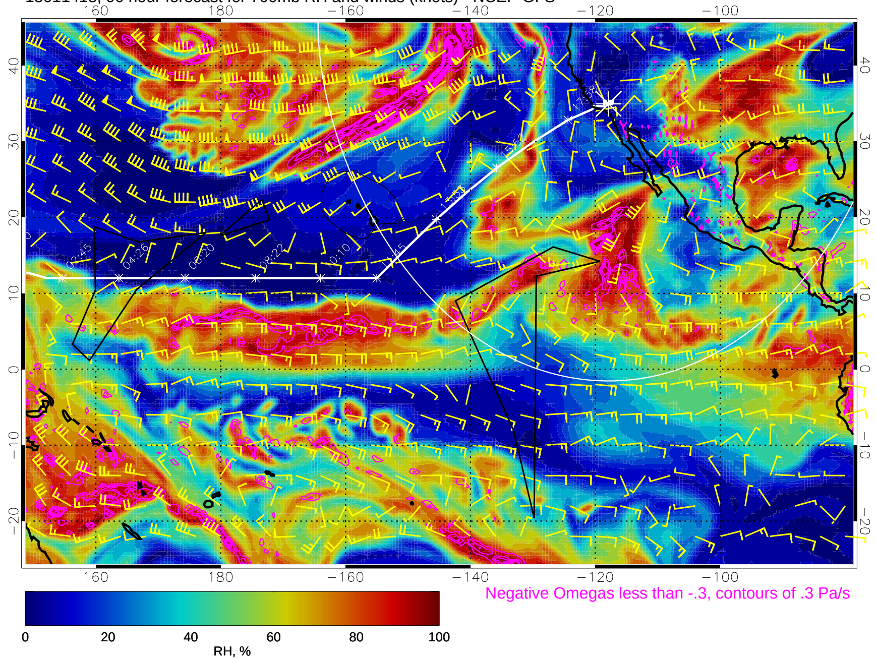
15011418, 90 hour forecast for 700mb RH and winds (knots) - NCEP GFS
