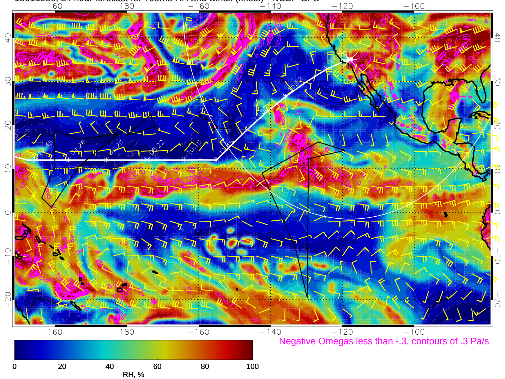
15011200, 24 hour forecast for 700mb RH and winds (knots) - NCEP GFS
