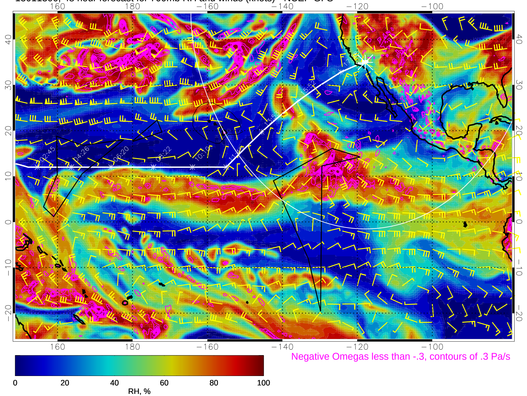
15011300, 48 hour forecast for 700mb RH and winds (knots) - NCEP GFS
