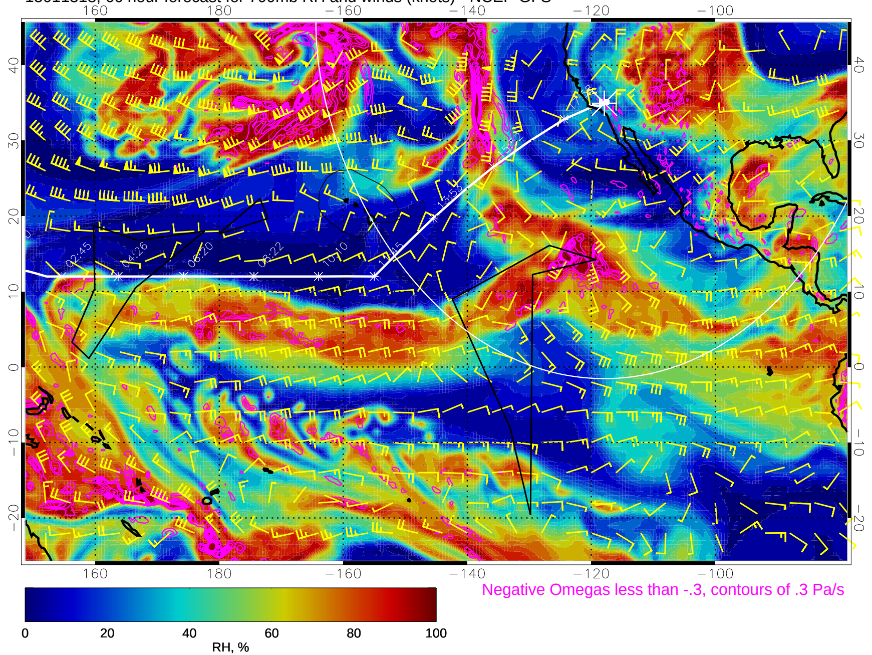
15011318, 66 hour forecast for 700mb RH and winds (knots) - NCEP GFS
