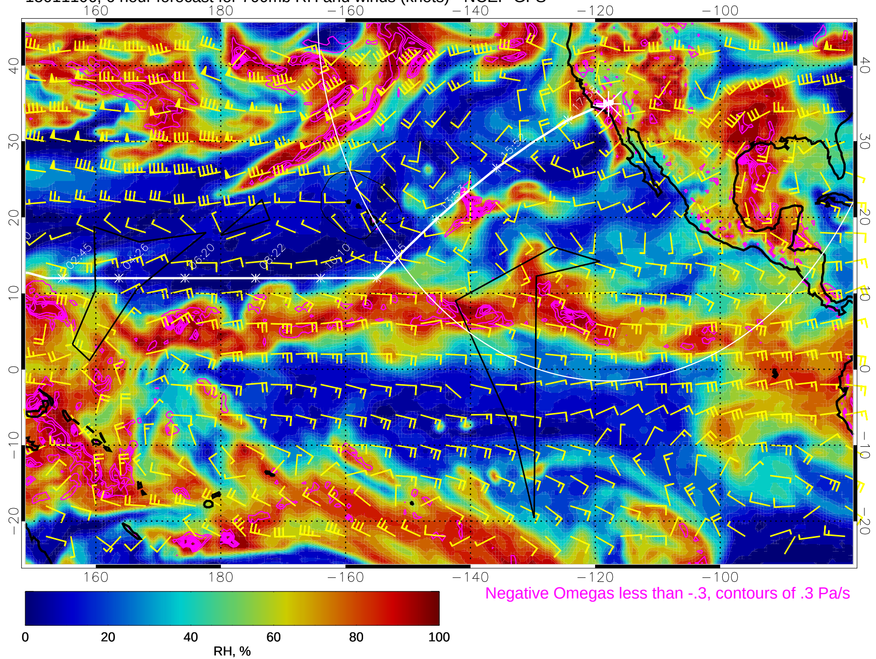
15011106, 6 hour forecast for 700mb RH and winds (knots) - NCEP GFS
