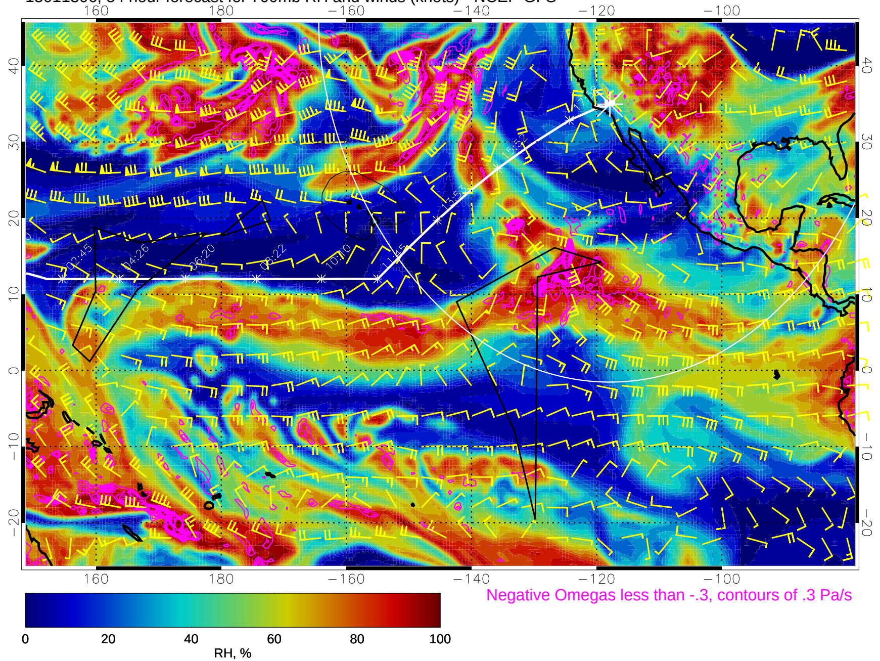
15011306, 54 hour forecast for 700mb RH and winds (knots) - NCEP GFS
