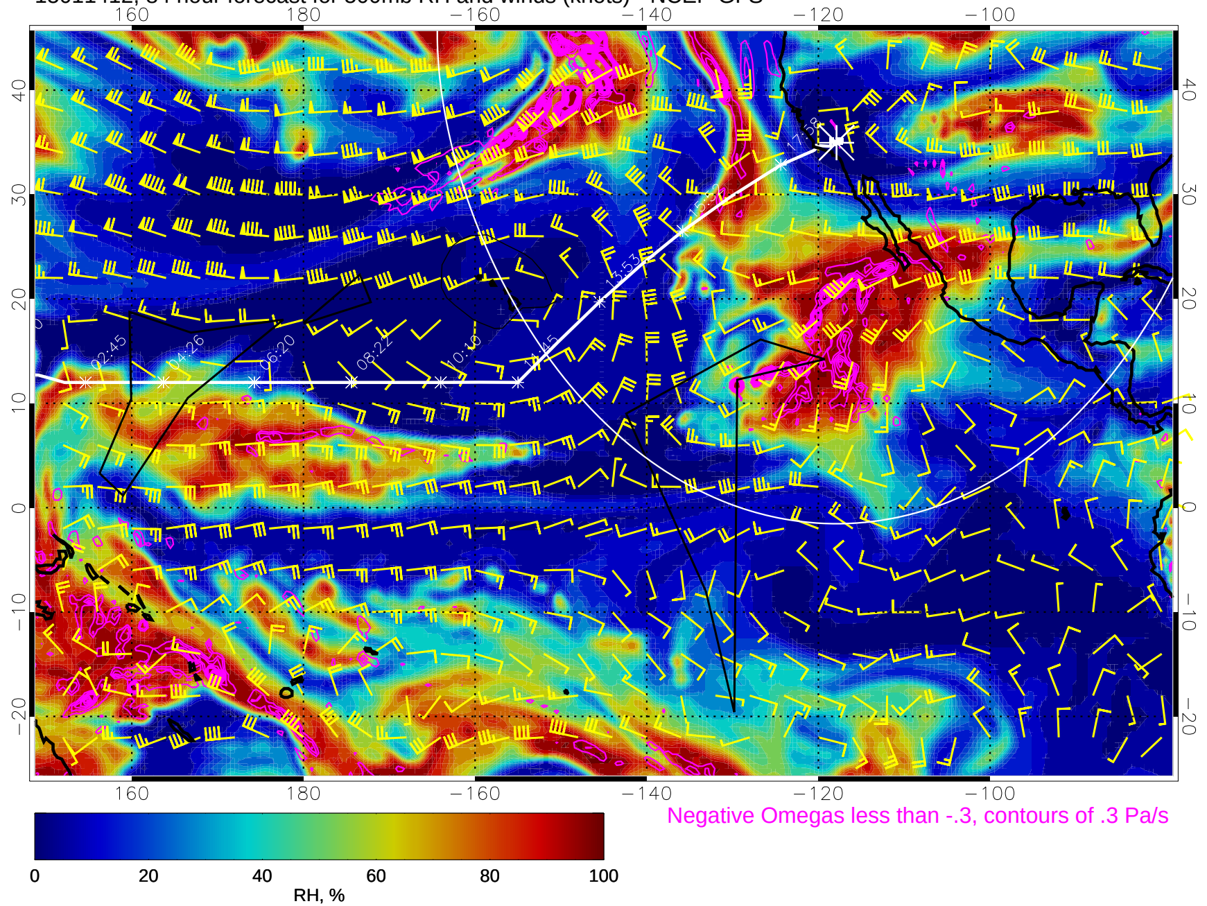
15011412, 84 hour forecast for 500mb RH and winds (knots) - NCEP GFS
