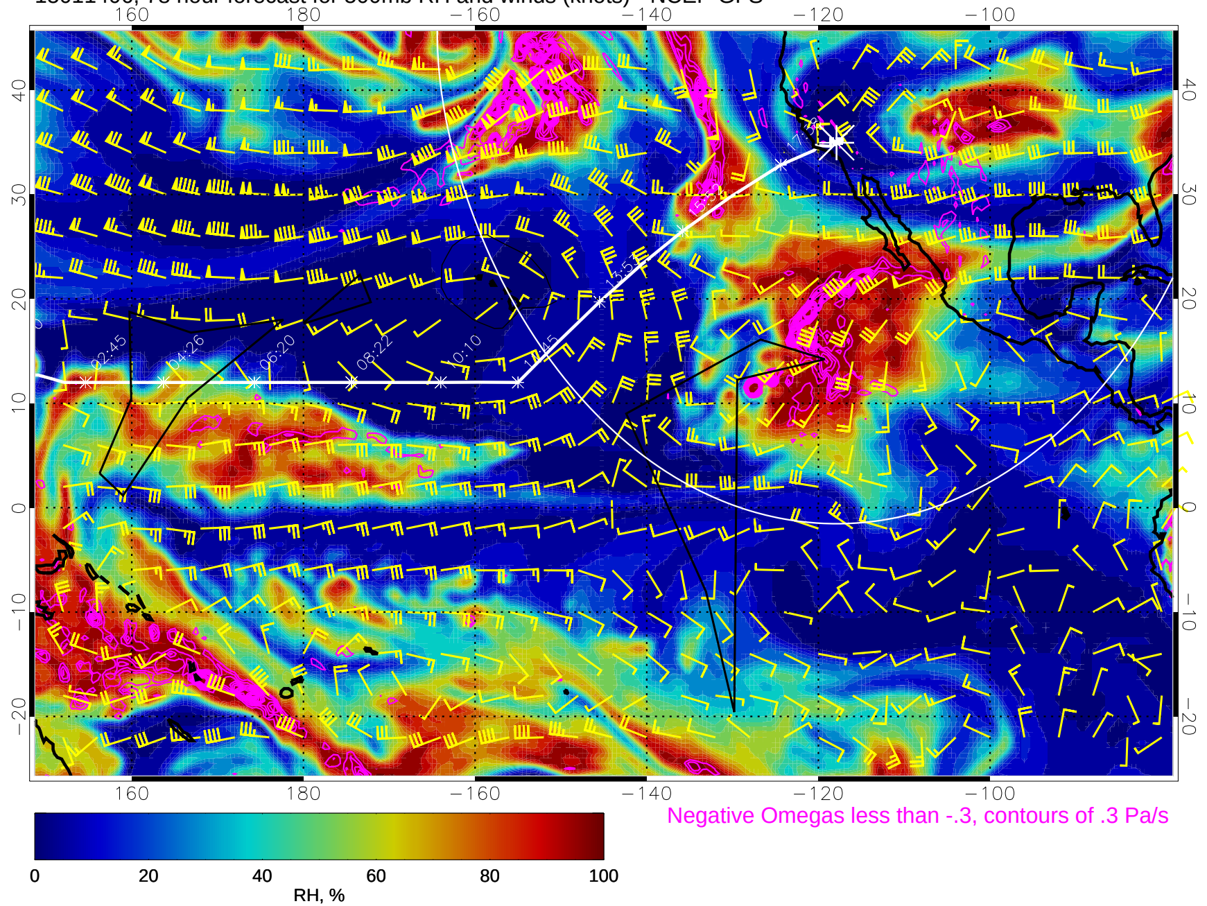
15011406, 78 hour forecast for 500mb RH and winds (knots) - NCEP GFS
