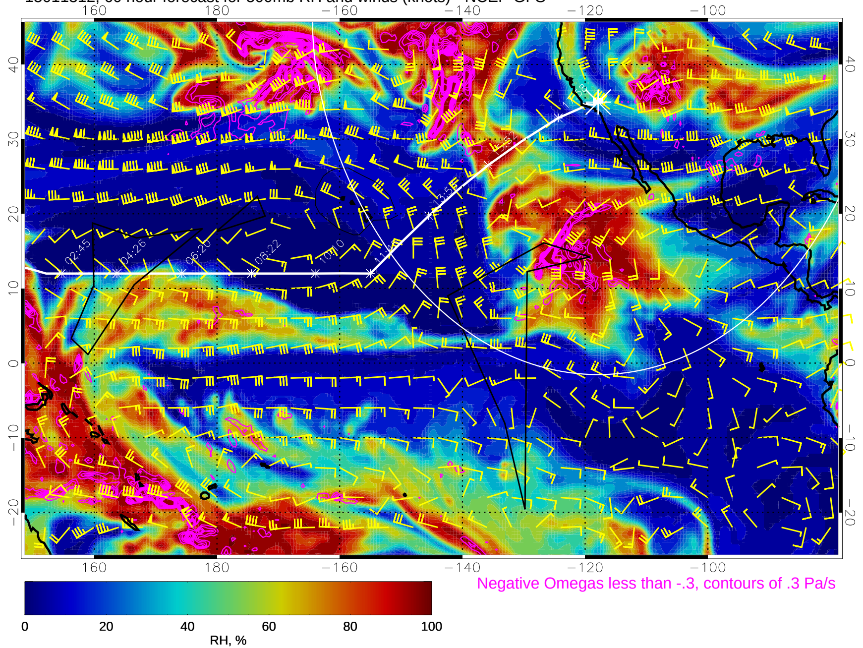
15011312, 60 hour forecast for 500mb RH and winds (knots) - NCEP GFS
