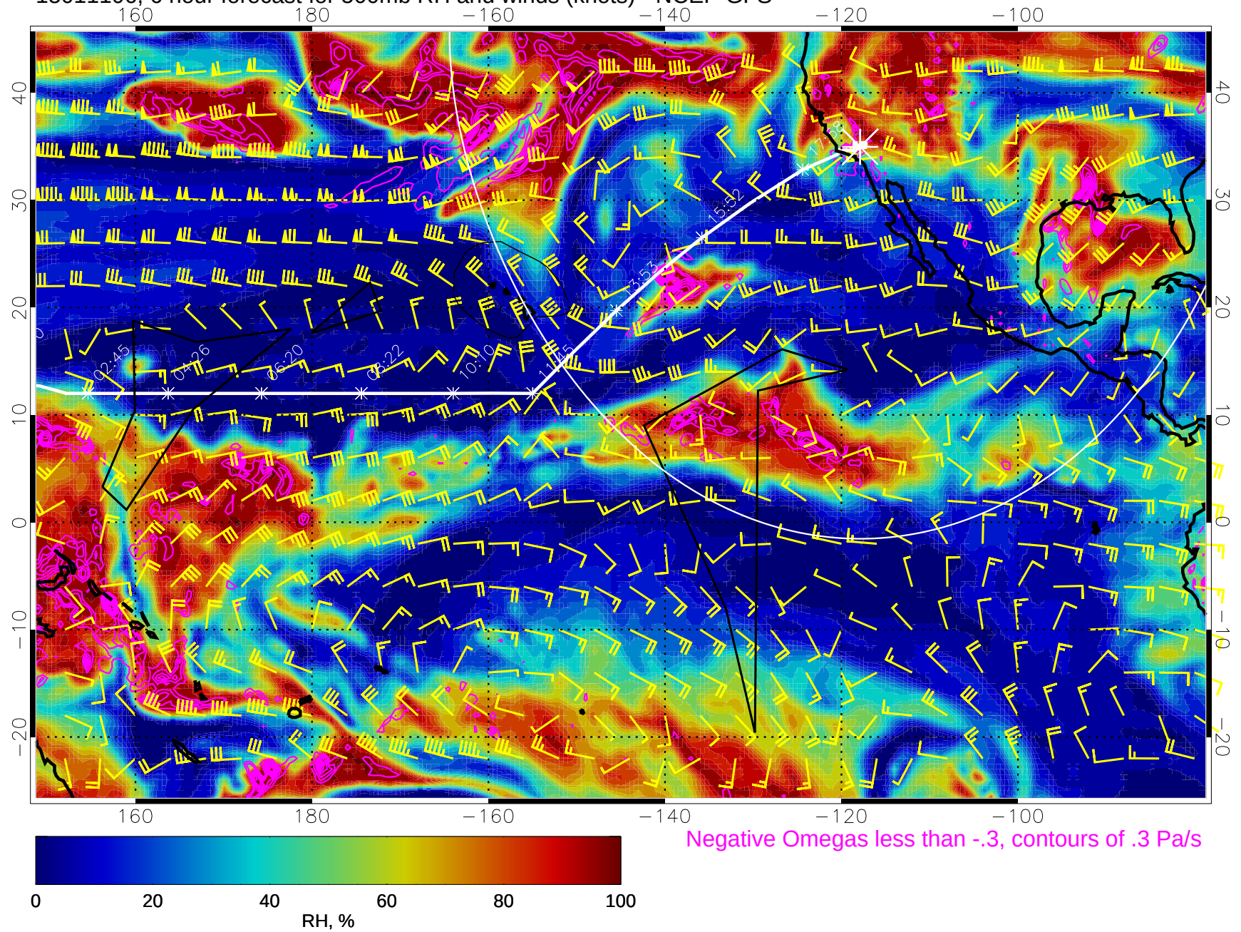
15011106, 6 hour forecast for 500mb RH and winds (knots) - NCEP GFS
