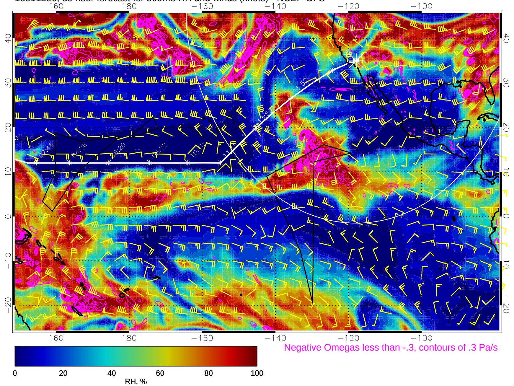
15011206, 30 hour forecast for 500mb RH and winds (knots) - NCEP GFS
