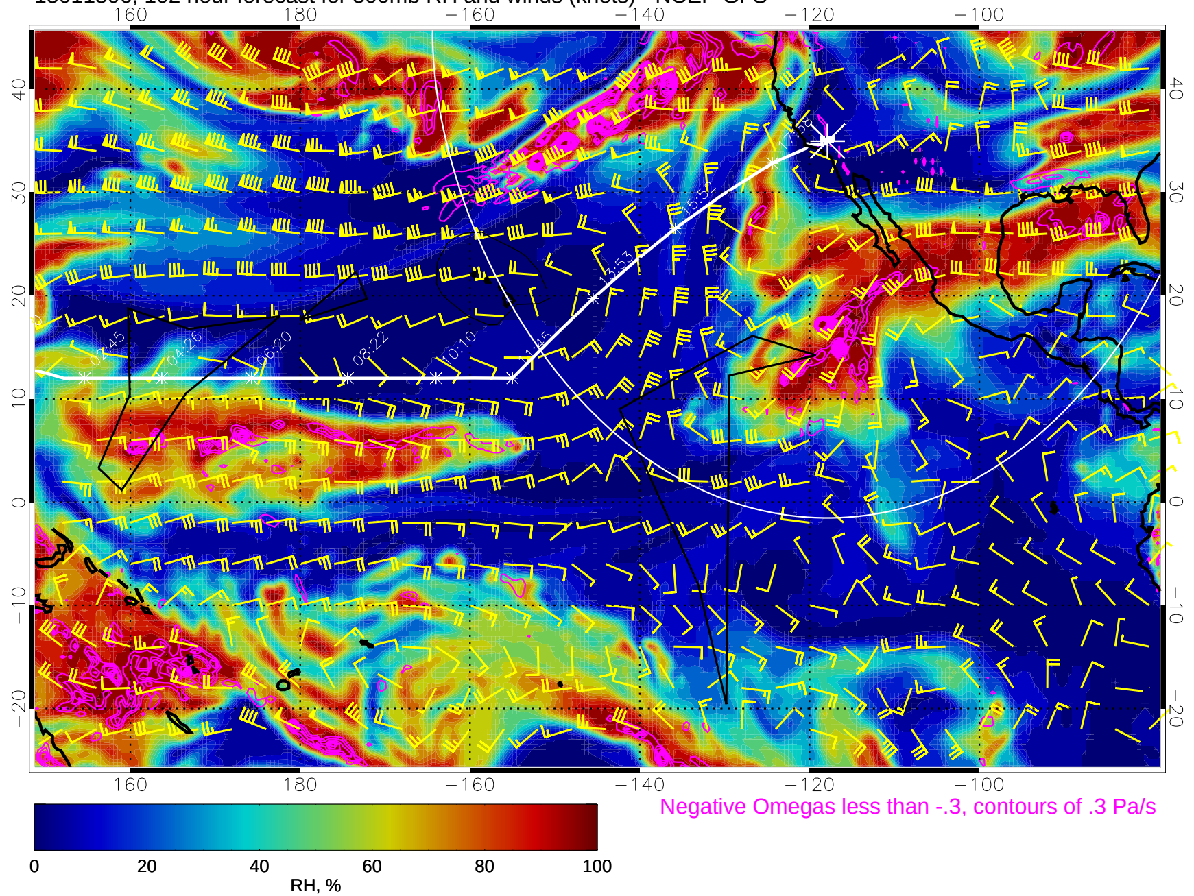
15011506, 102 hour forecast for 500mb RH and winds (knots) - NCEP GFS
