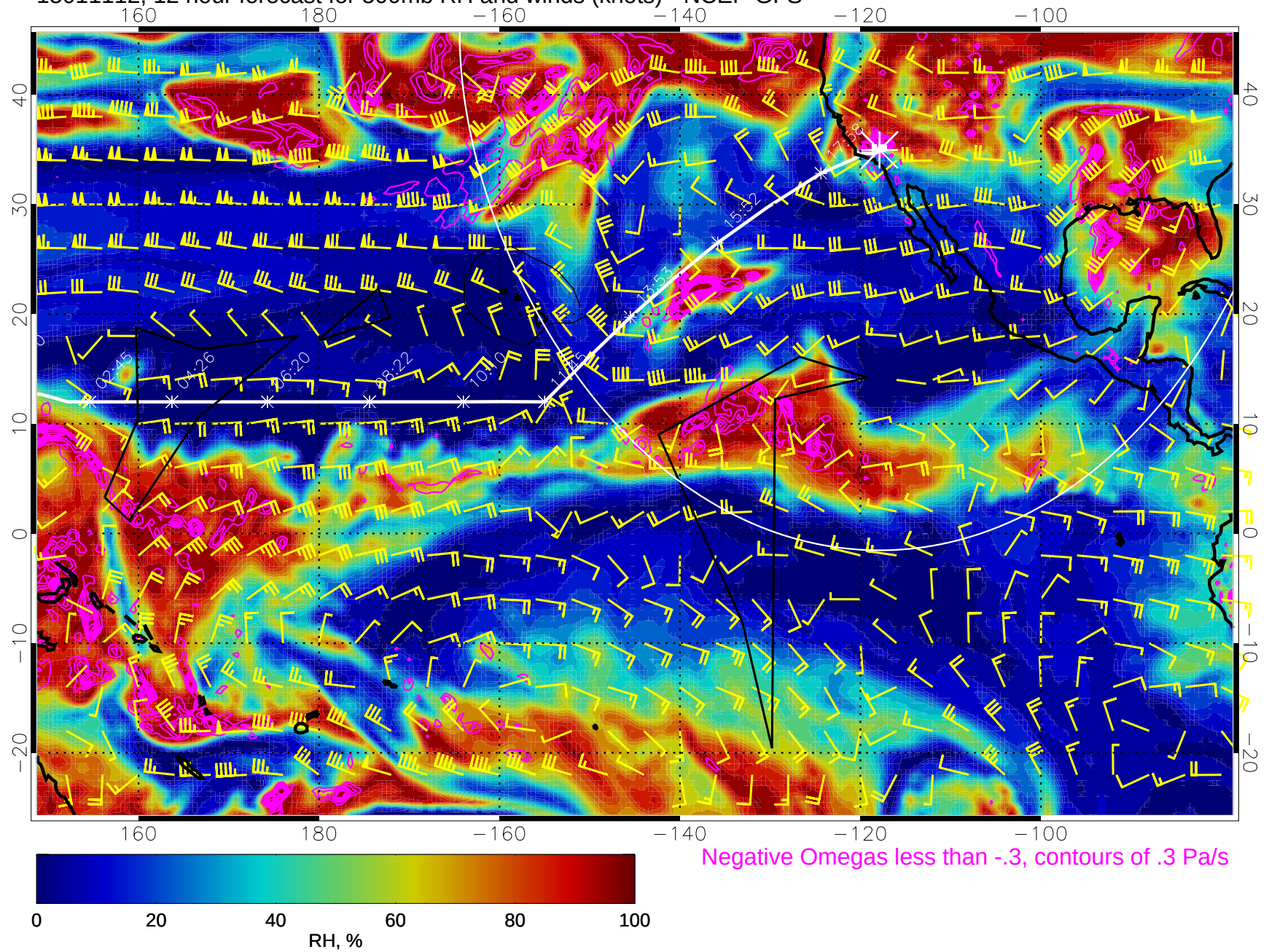
15011112, 12 hour forecast for 500mb RH and winds (knots) - NCEP GFS
