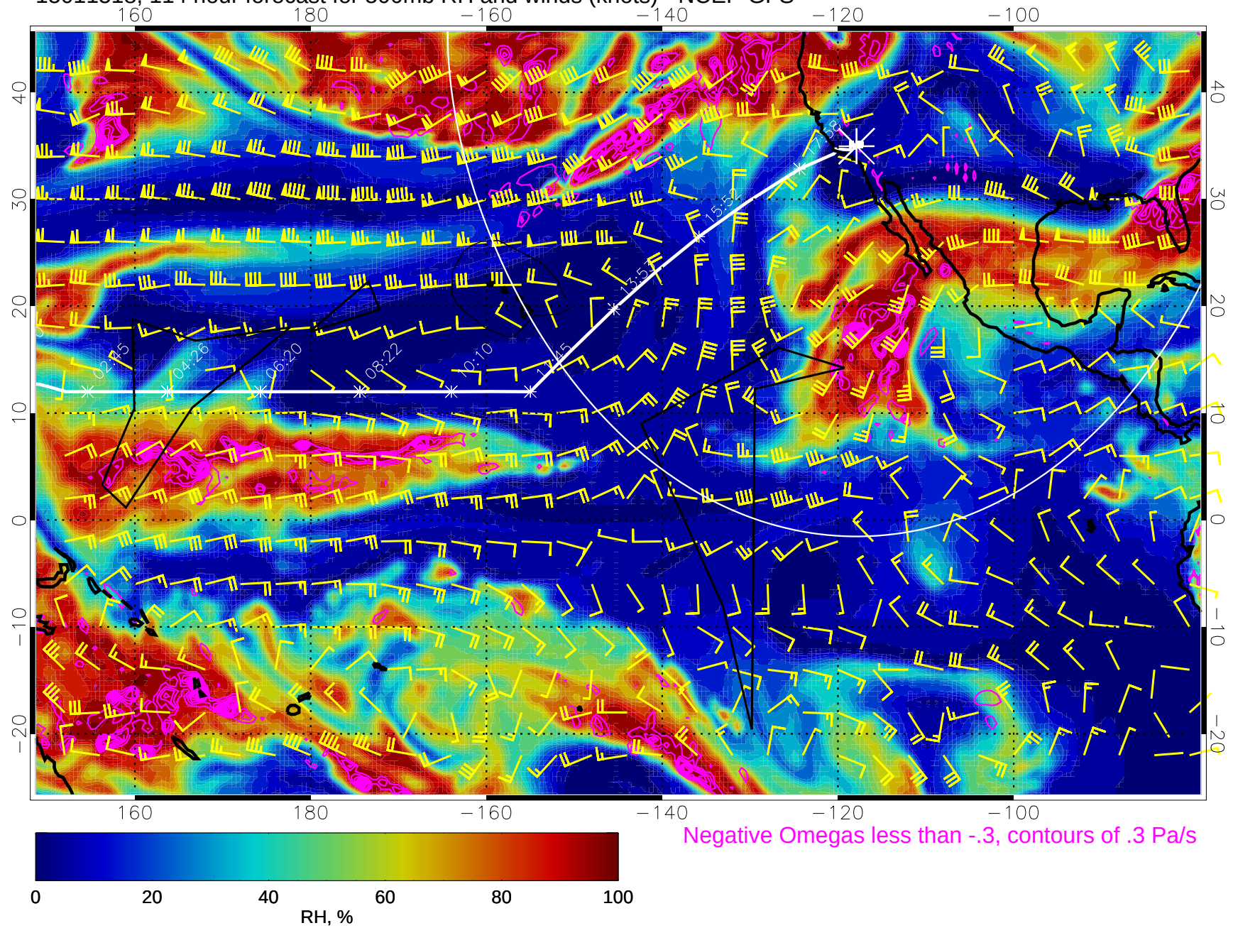
15011518, 114 hour forecast for 500mb RH and winds (knots) - NCEP GFS
