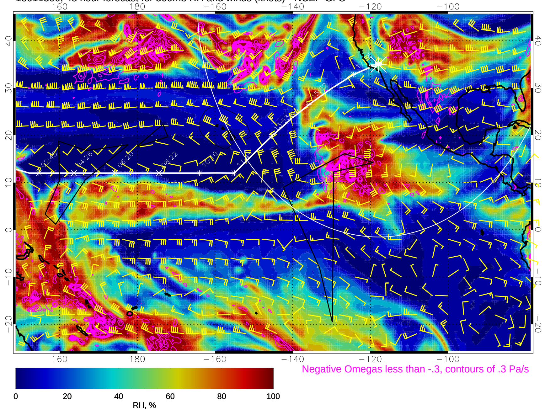
15011300, 48 hour forecast for 500mb RH and winds (knots) - NCEP GFS
