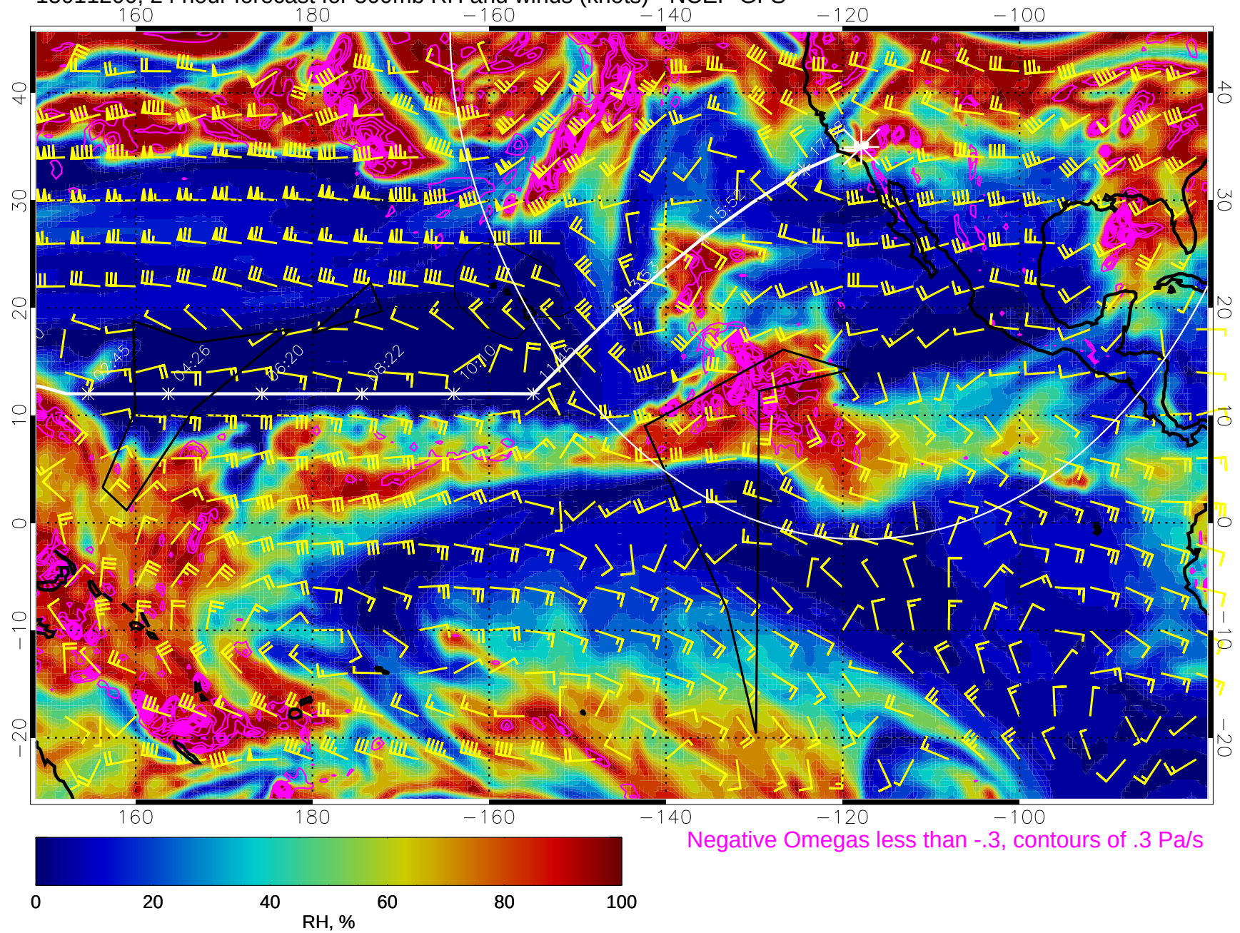
15011200, 24 hour forecast for 500mb RH and winds (knots) - NCEP GFS
