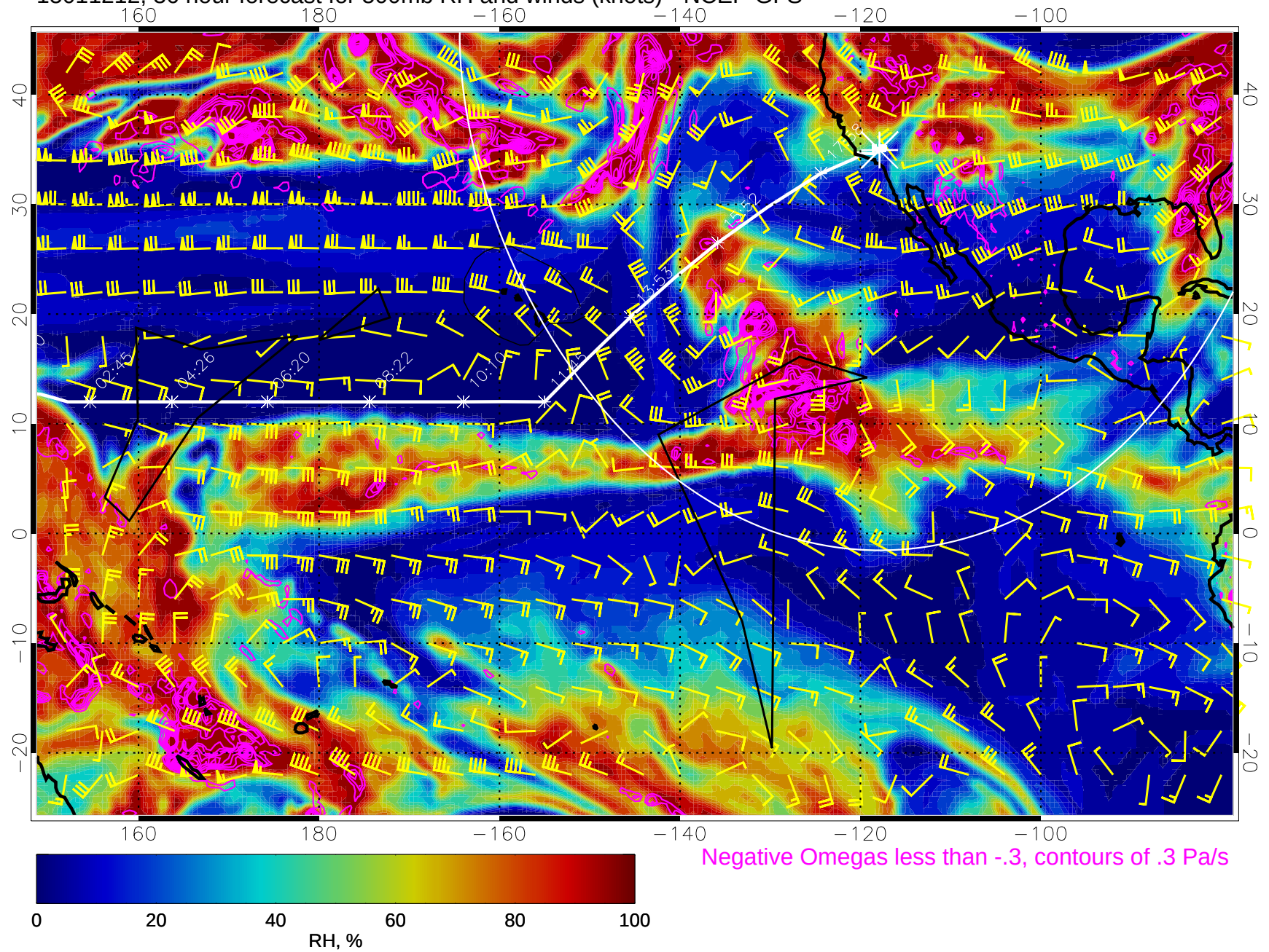
15011212, 36 hour forecast for 500mb RH and winds (knots) - NCEP GFS
