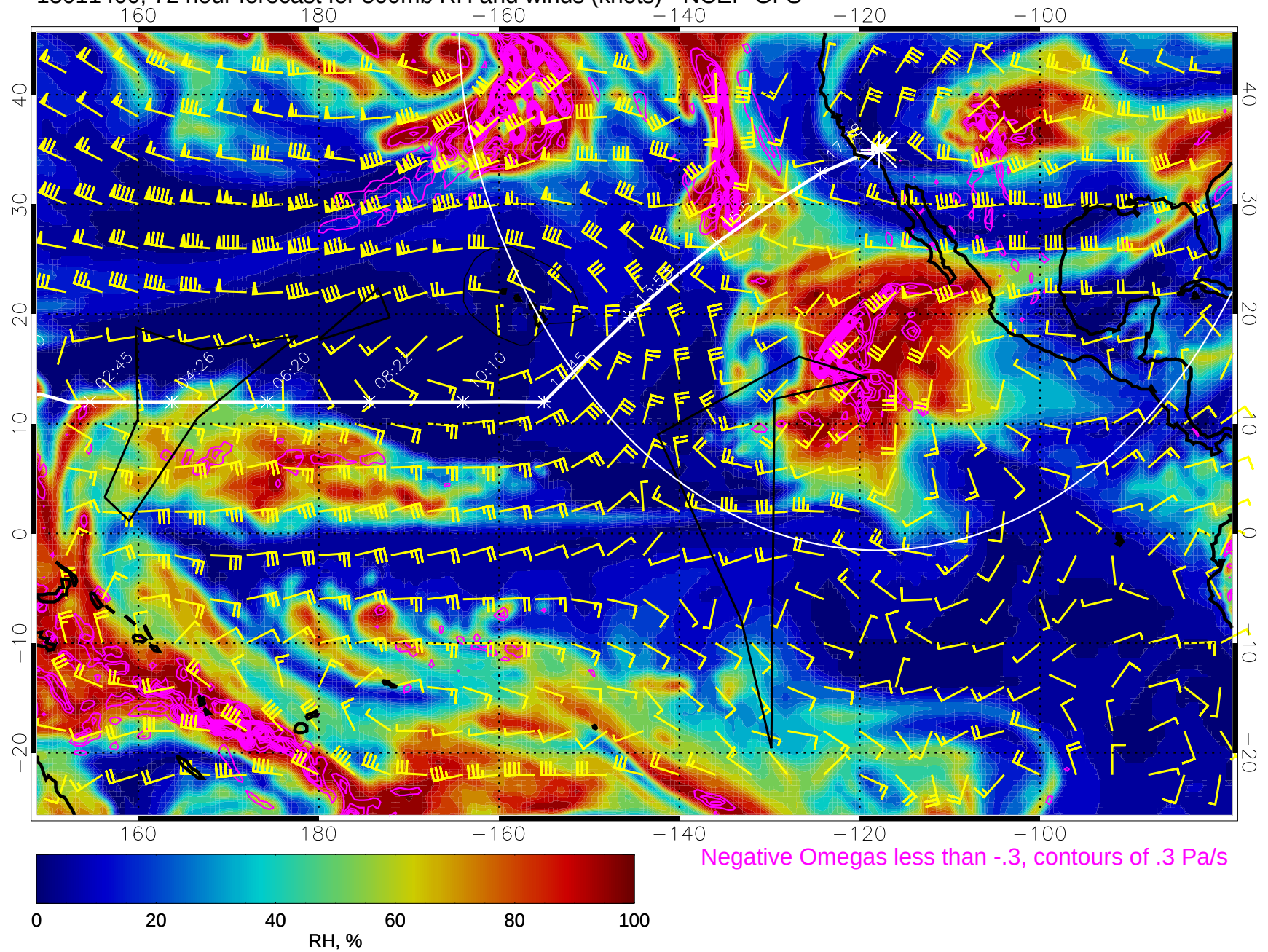
15011400, 72 hour forecast for 500mb RH and winds (knots) - NCEP GFS
