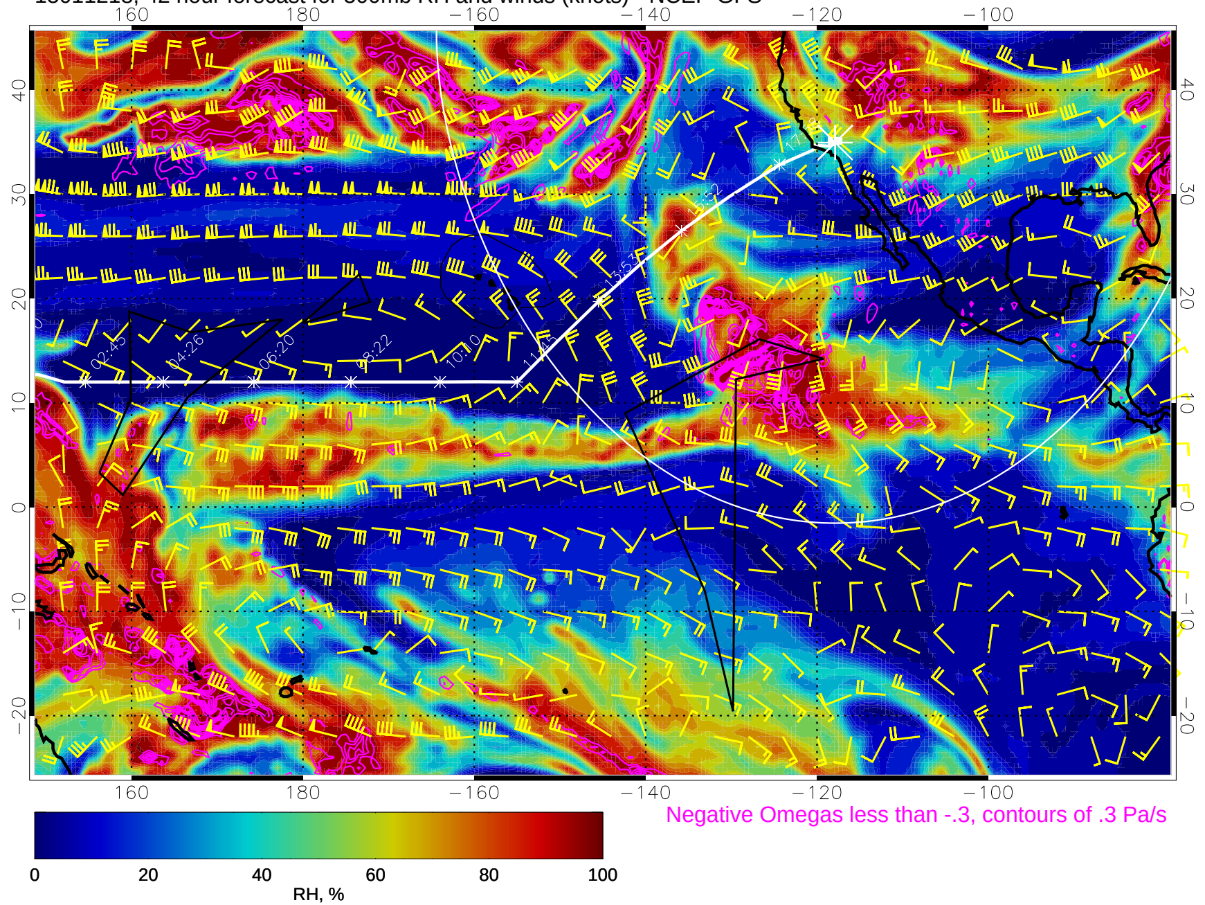
15011218, 42 hour forecast for 500mb RH and winds (knots) - NCEP GFS
