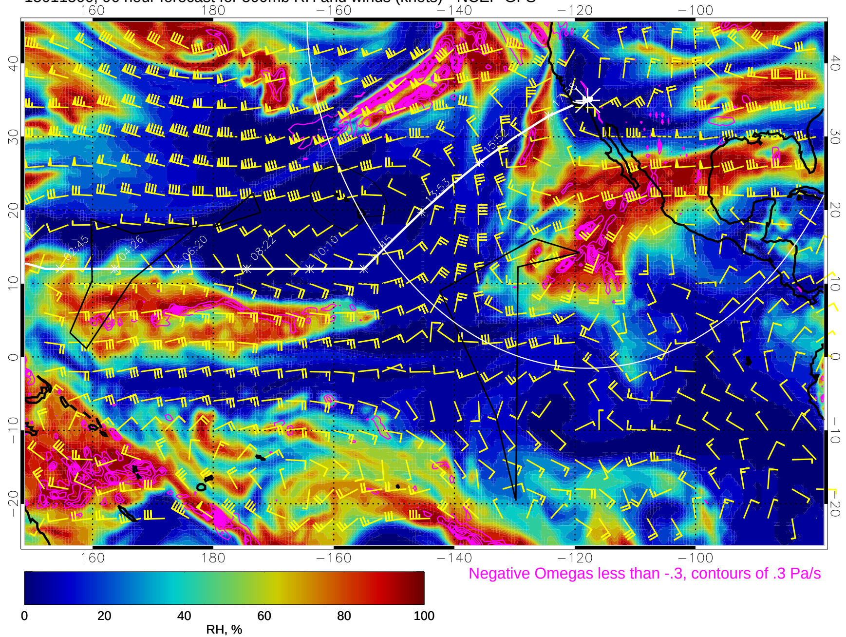
15011500, 96 hour forecast for 500mb RH and winds (knots) - NCEP GFS
