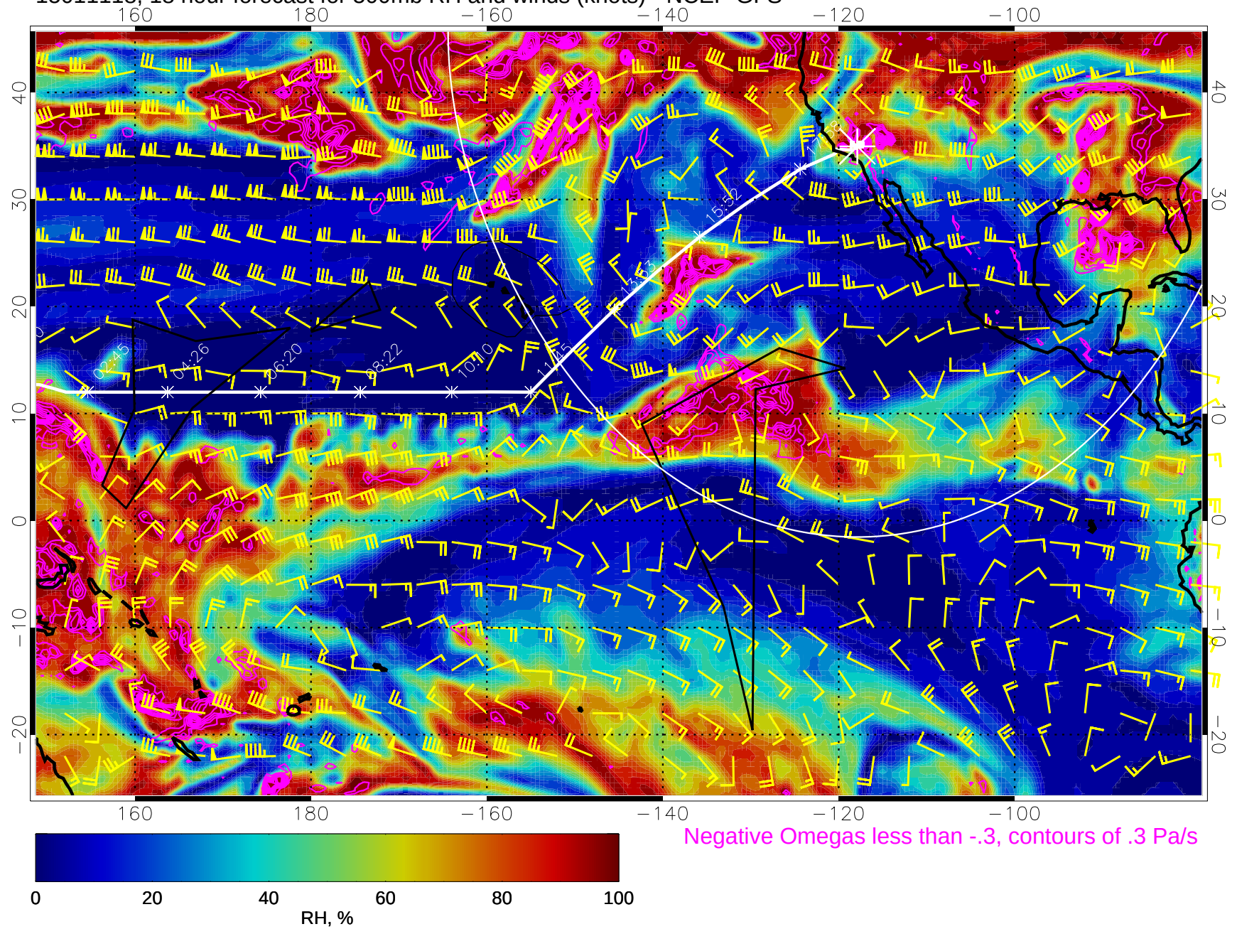
15011118, 18 hour forecast for 500mb RH and winds (knots) - NCEP GFS
