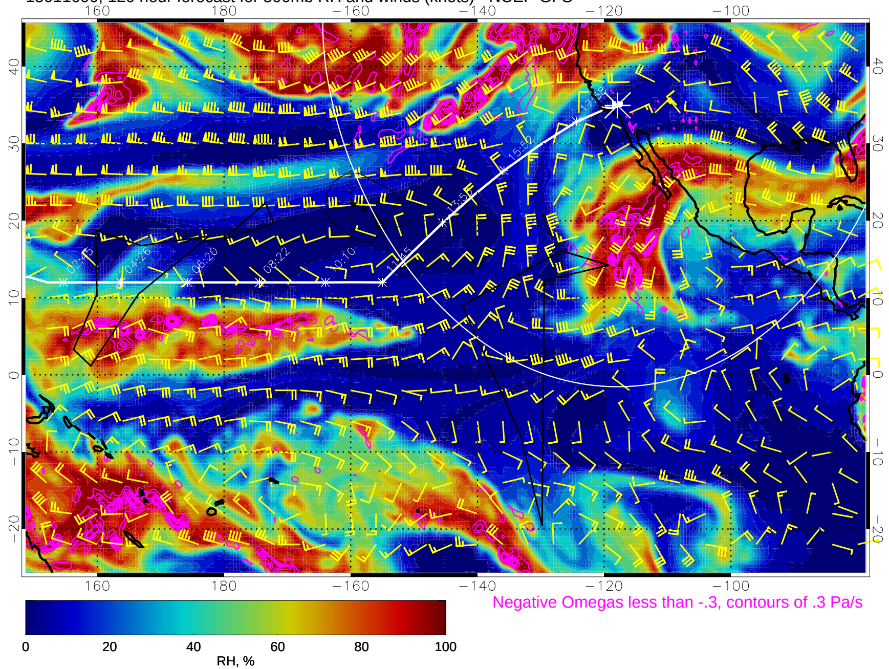
15011600, 120 hour forecast for 500mb RH and winds (knots) - NCEP GFS
