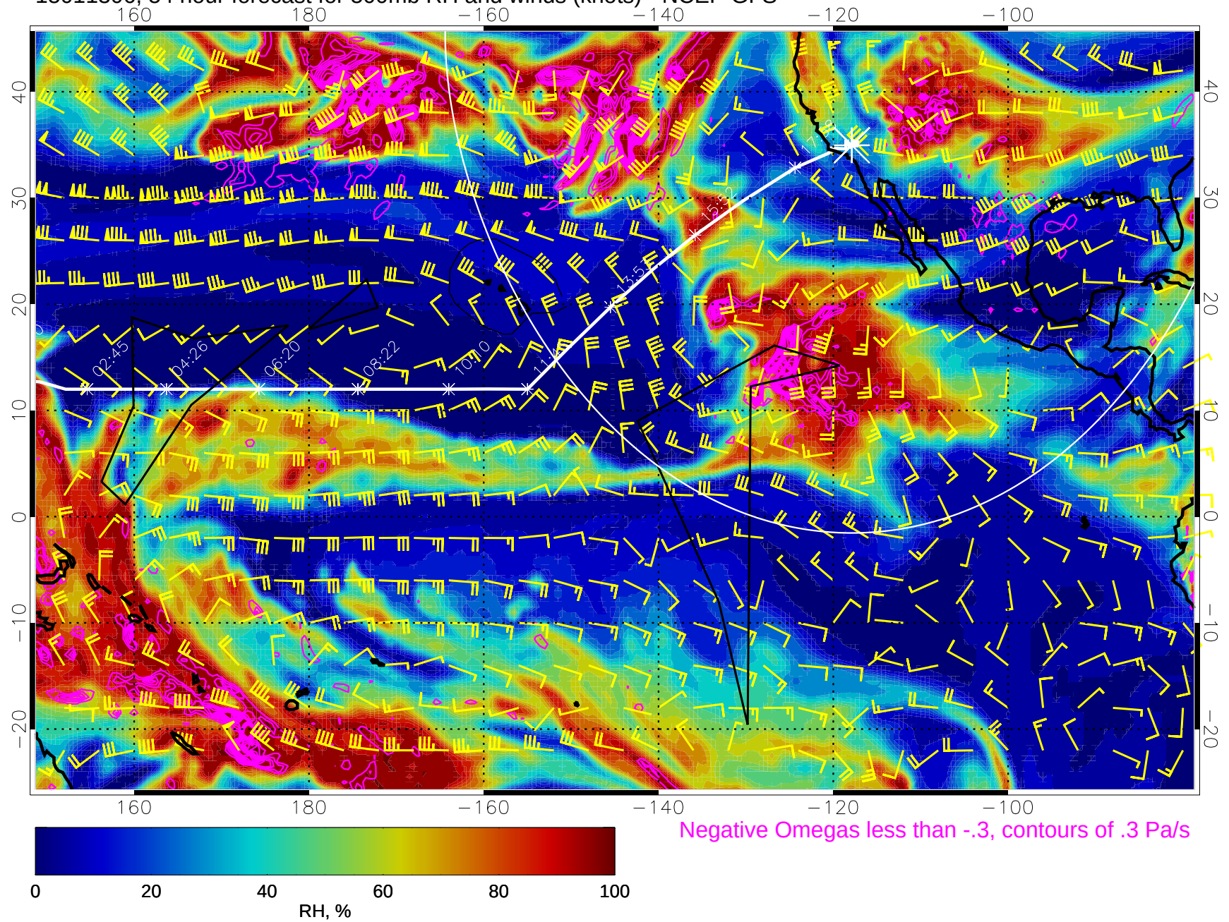
15011306, 54 hour forecast for 500mb RH and winds (knots) - NCEP GFS
