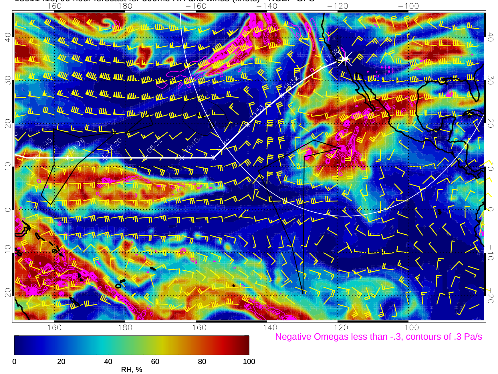
15011418, 90 hour forecast for 500mb RH and winds (knots) - NCEP GFS
