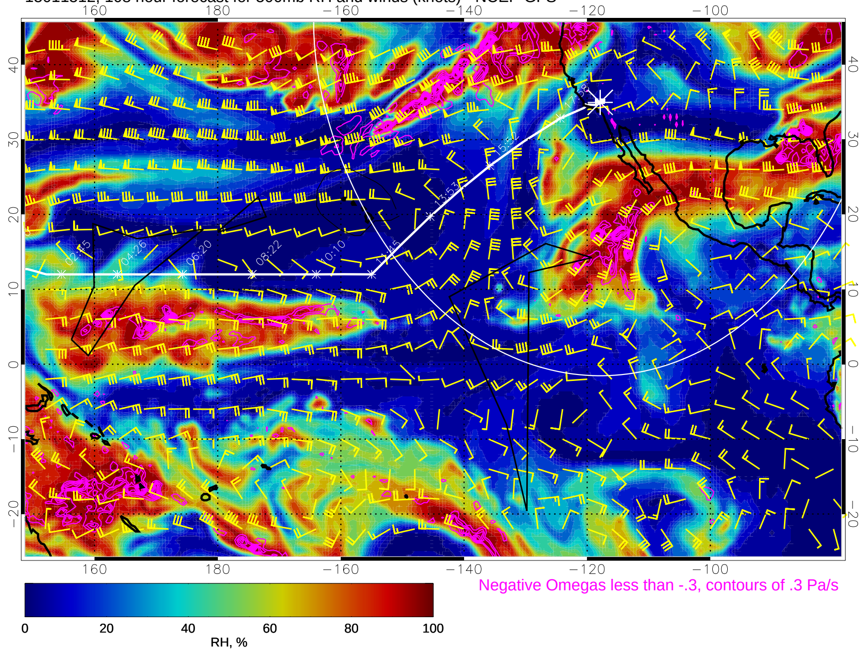
15011512, 108 hour forecast for 500mb RH and winds (knots) - NCEP GFS
