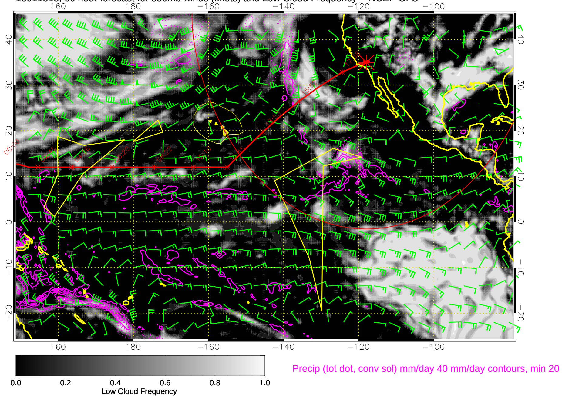
15011318, 66 hour forecast for 850mb winds (knots) and Low Cloud Frequency -- NCEP GFS
