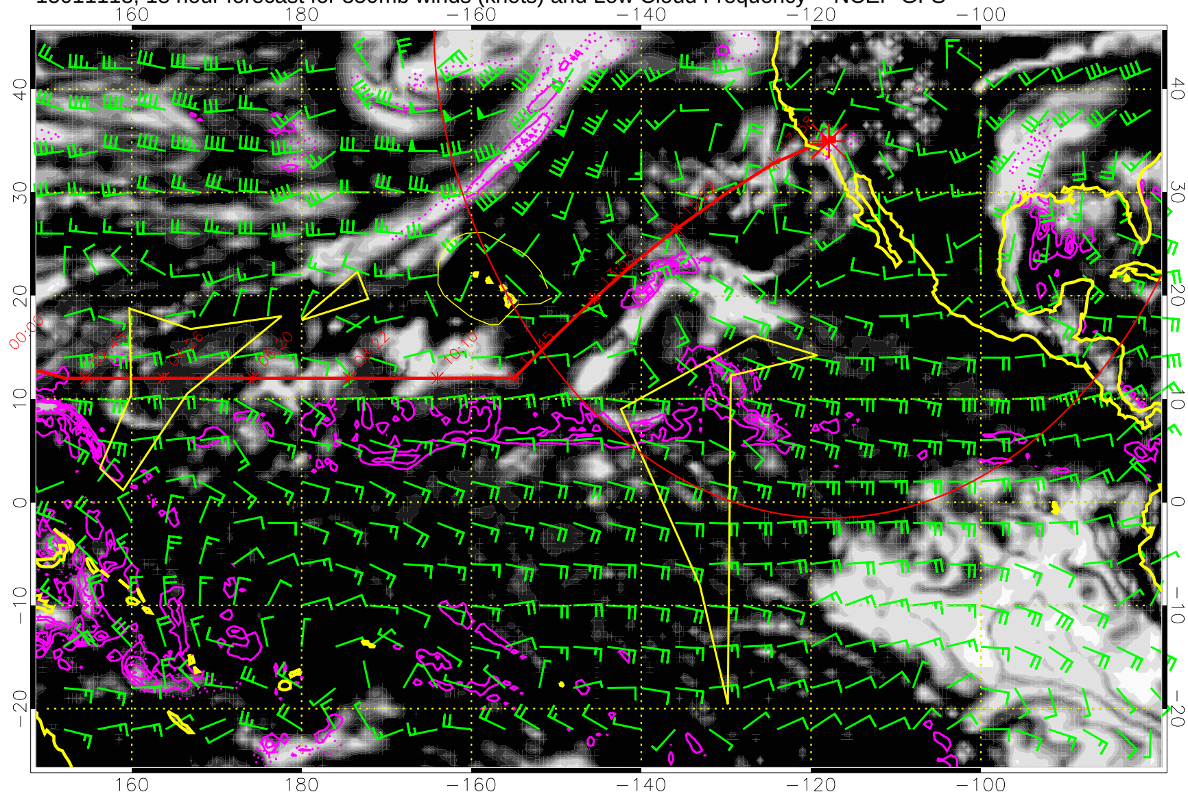
15011118, 18 hour forecast for 850mb winds (knots) and Low Cloud Frequency -- NCEP GFS
