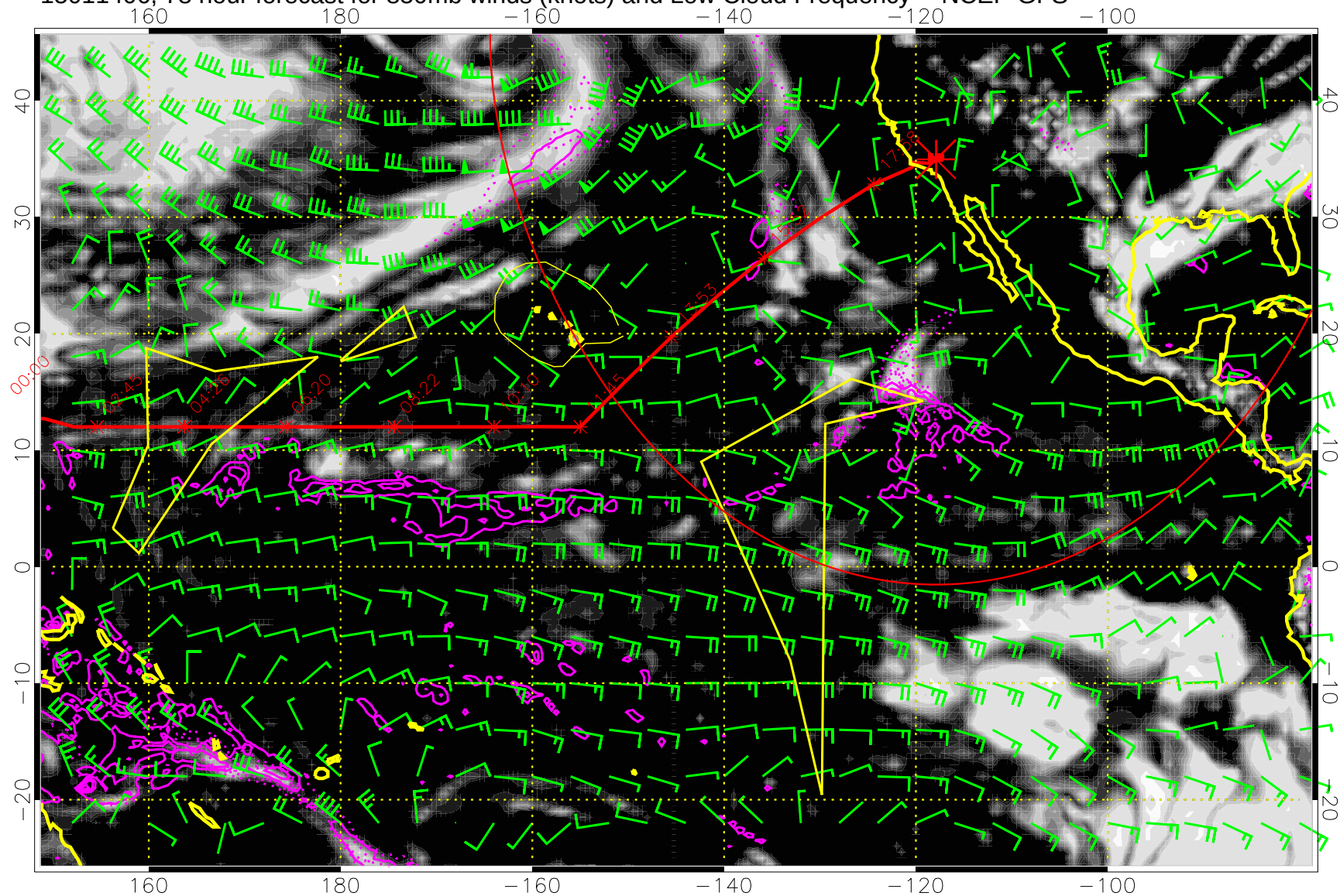
15011406, 78 hour forecast for 850mb winds (knots) and Low Cloud Frequency -- NCEP GFS
