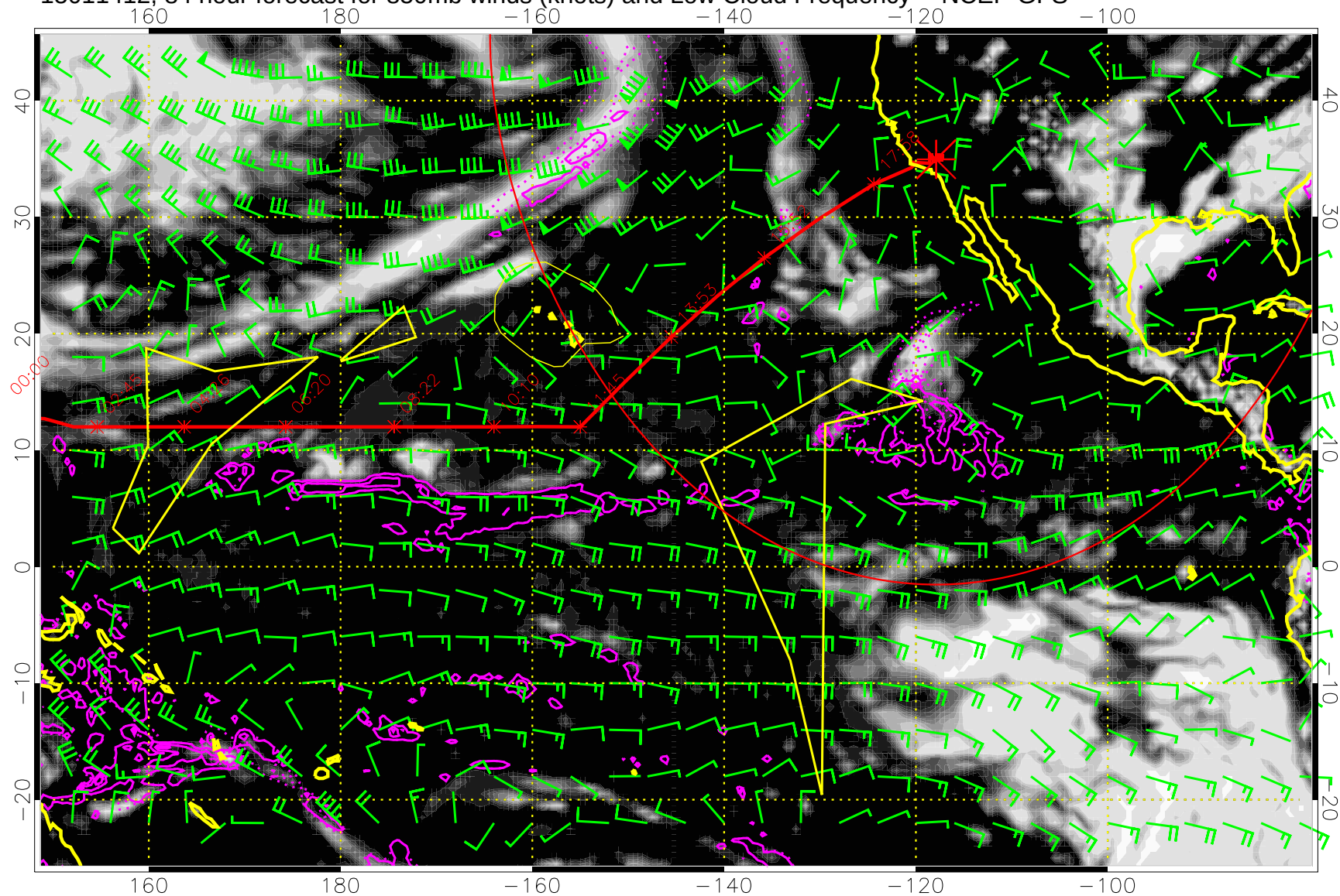
15011412, 84 hour forecast for 850mb winds (knots) and Low Cloud Frequency -- NCEP GFS
