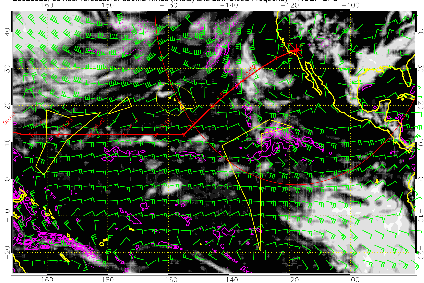
15011312, 60 hour forecast for 850mb winds (knots) and Low Cloud Frequency -- NCEP GFS
