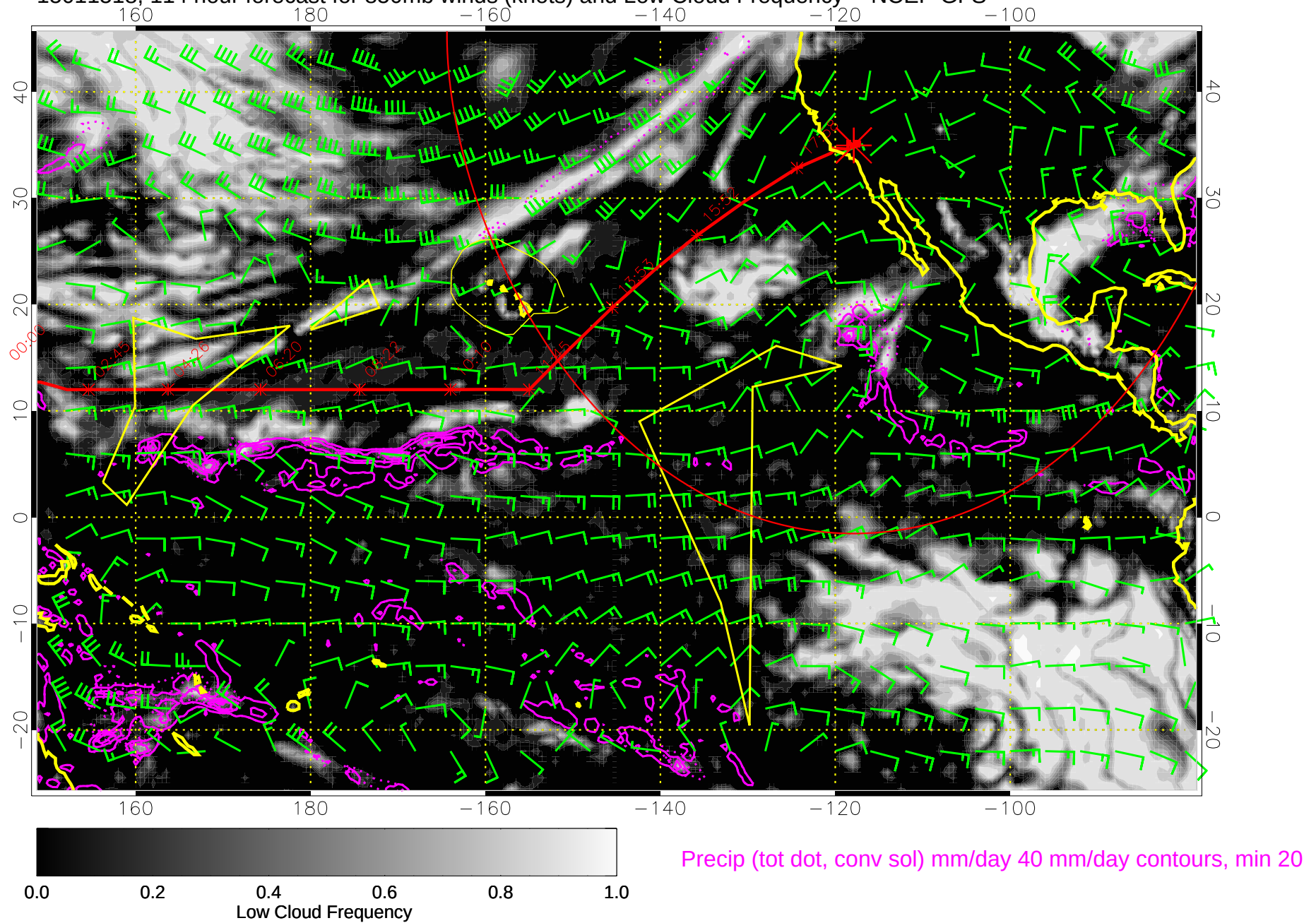
15011518, 114 hour forecast for 850mb winds (knots) and Low Cloud Frequency -- NCEP GFS
