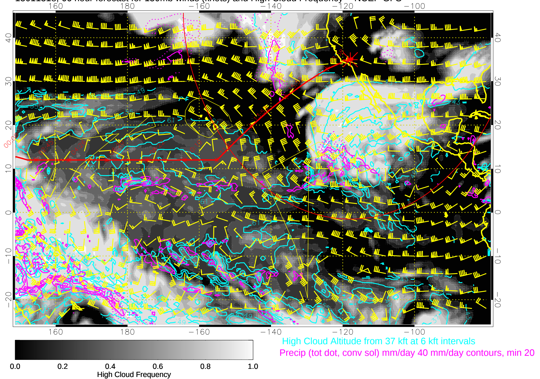
15011318, 66 hour forecast for 150mb winds (knots) and High Cloud Frequency -- NCEP GFS
