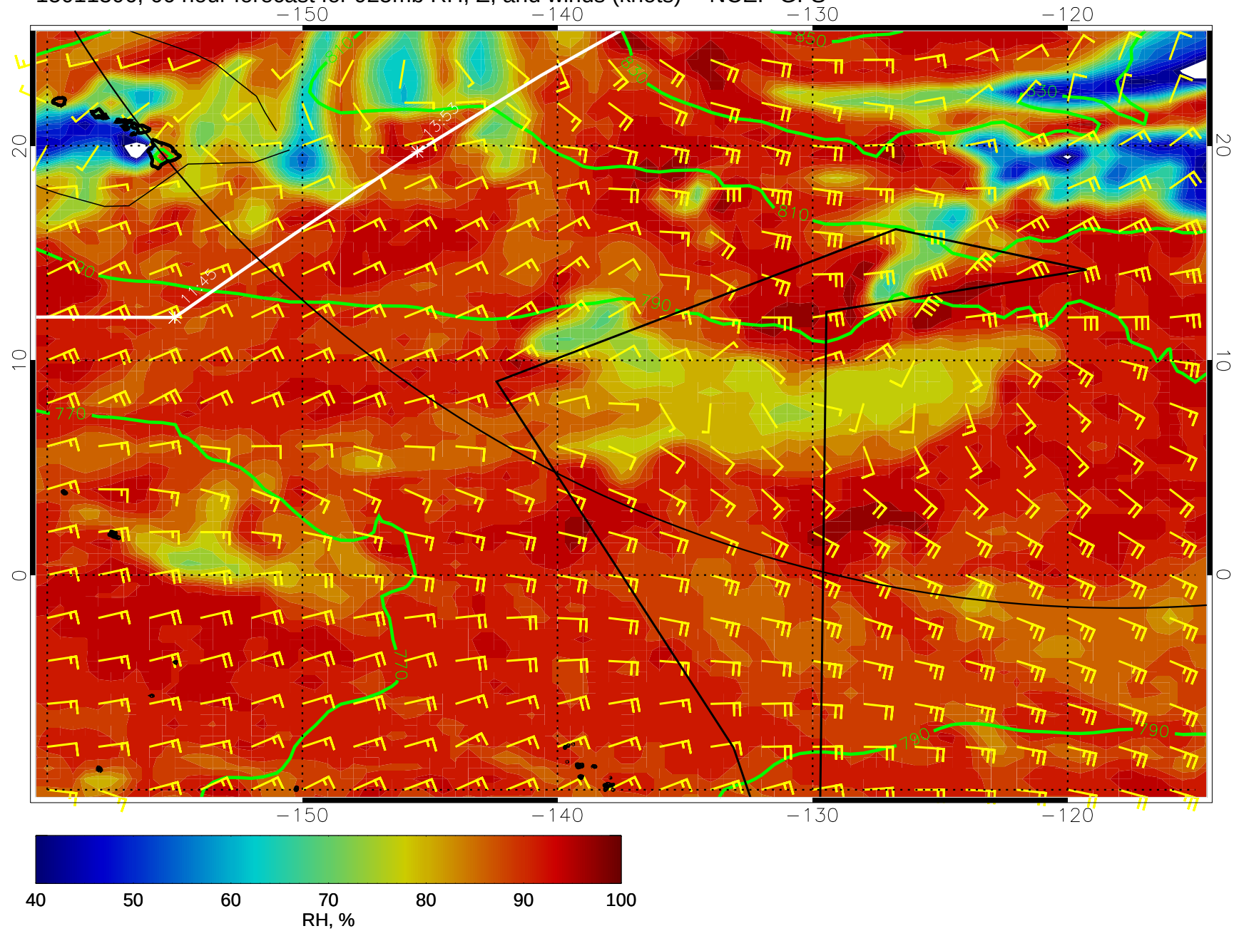
15011306, 66 hour forecast for 925mb RH, Z, and winds (knots) -- NCEP GFS
