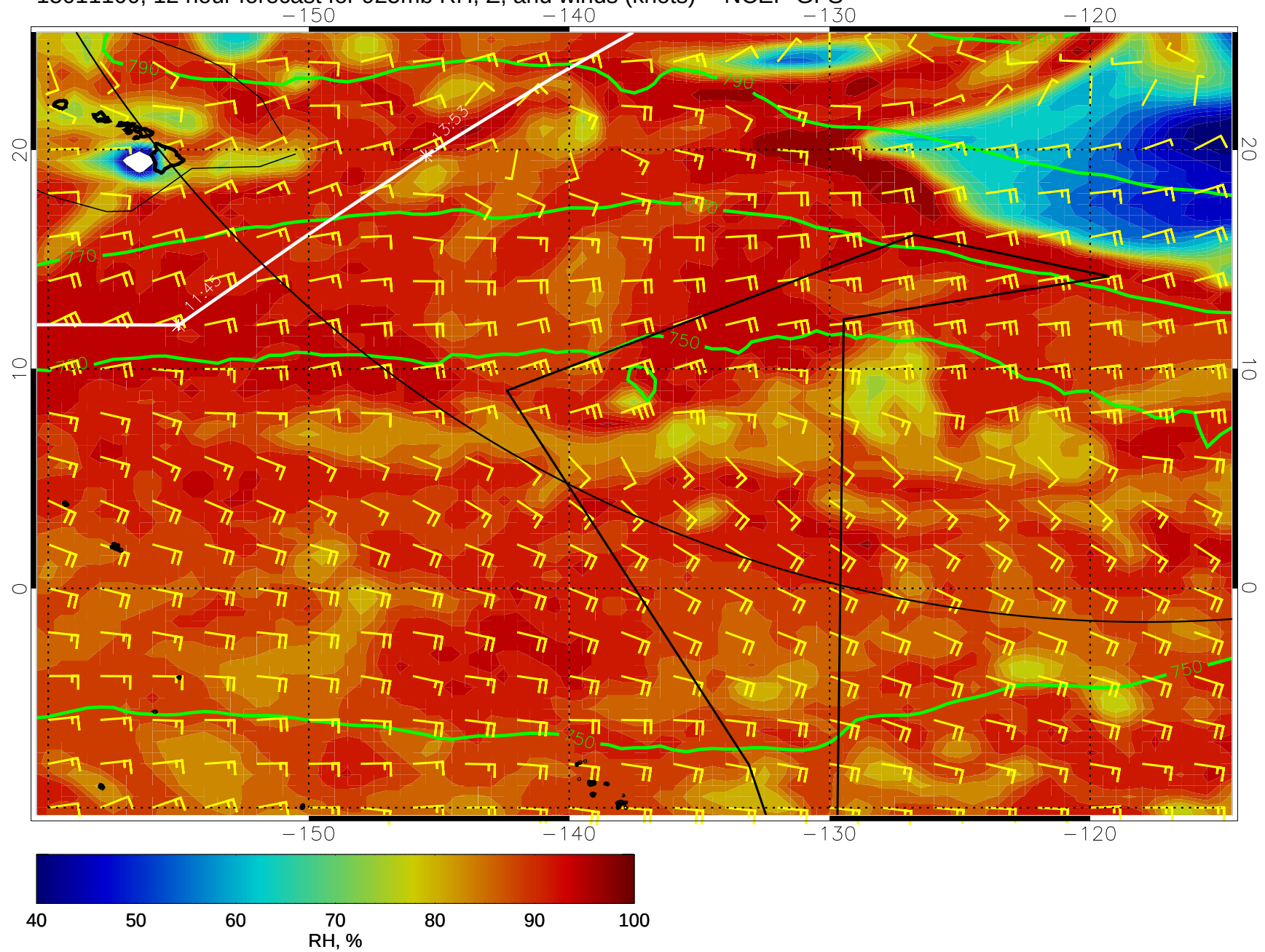
15011100, 12 hour forecast for 925mb RH, Z, and winds (knots) -- NCEP GFS
