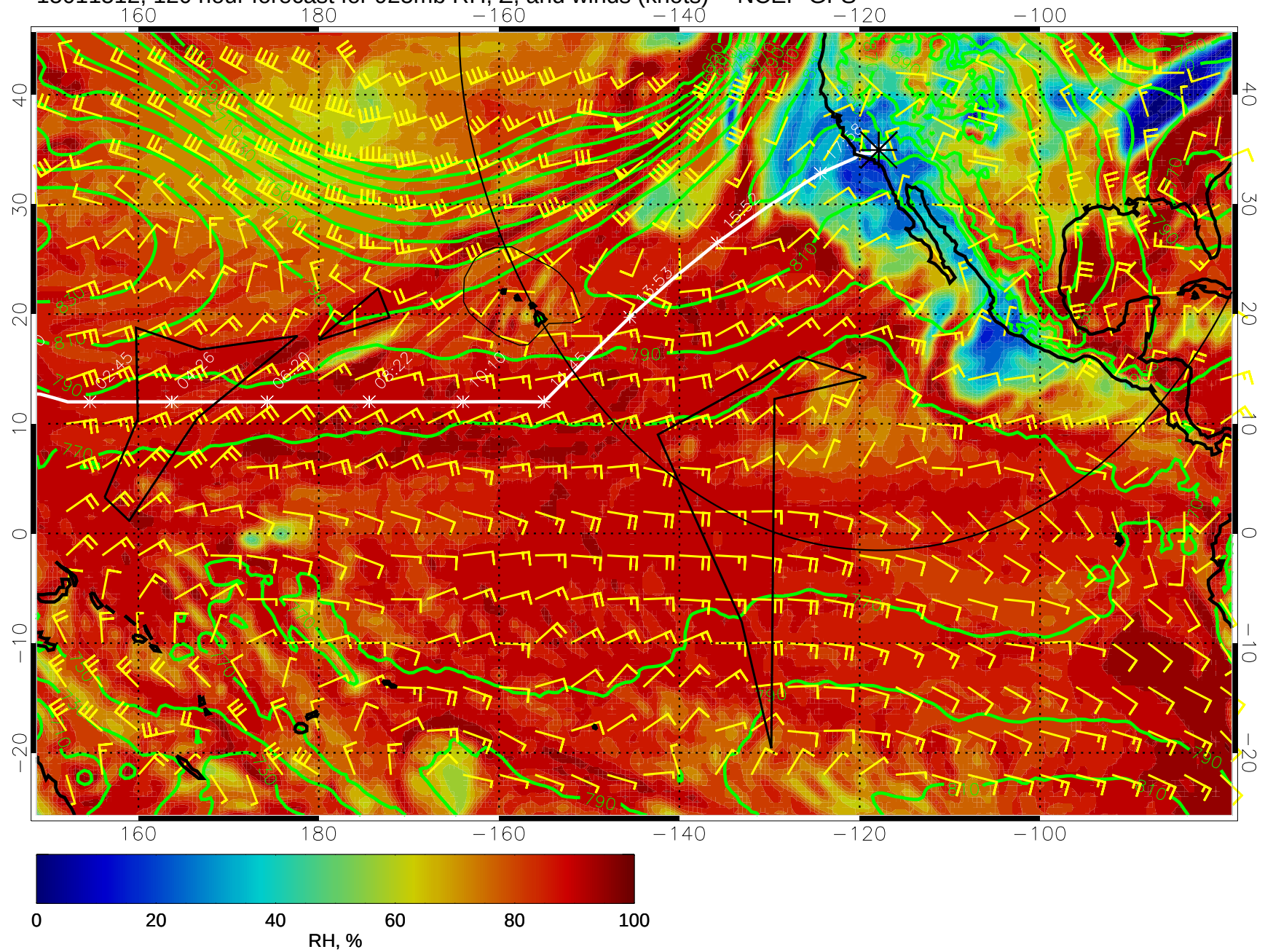
15011512, 120 hour forecast for 925mb RH, Z, and winds (knots) -- NCEP GFS
