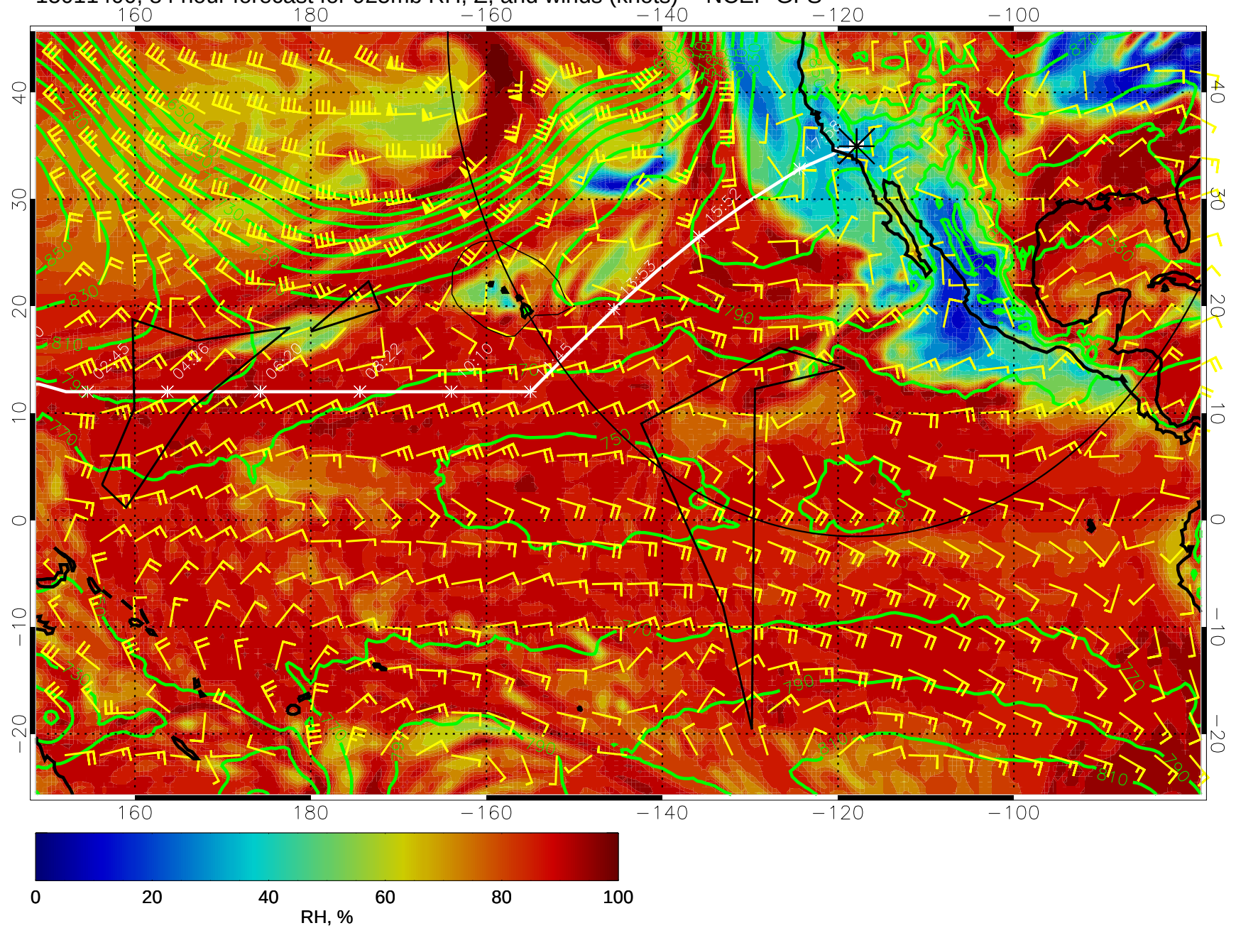
15011400, 84 hour forecast for 925mb RH, Z, and winds (knots) -- NCEP GFS
