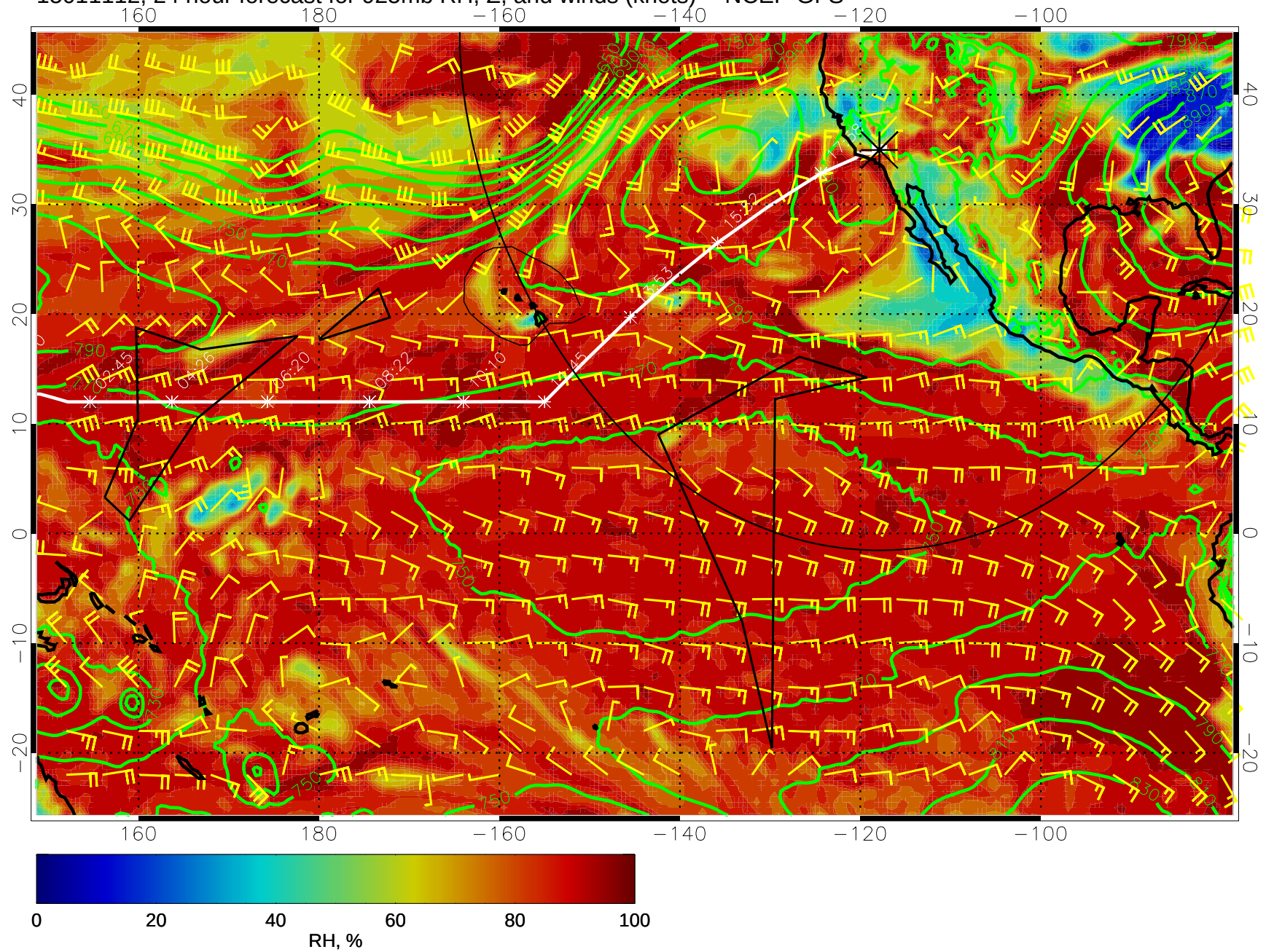
15011112, 24 hour forecast for 925mb RH, Z, and winds (knots) -- NCEP GFS
