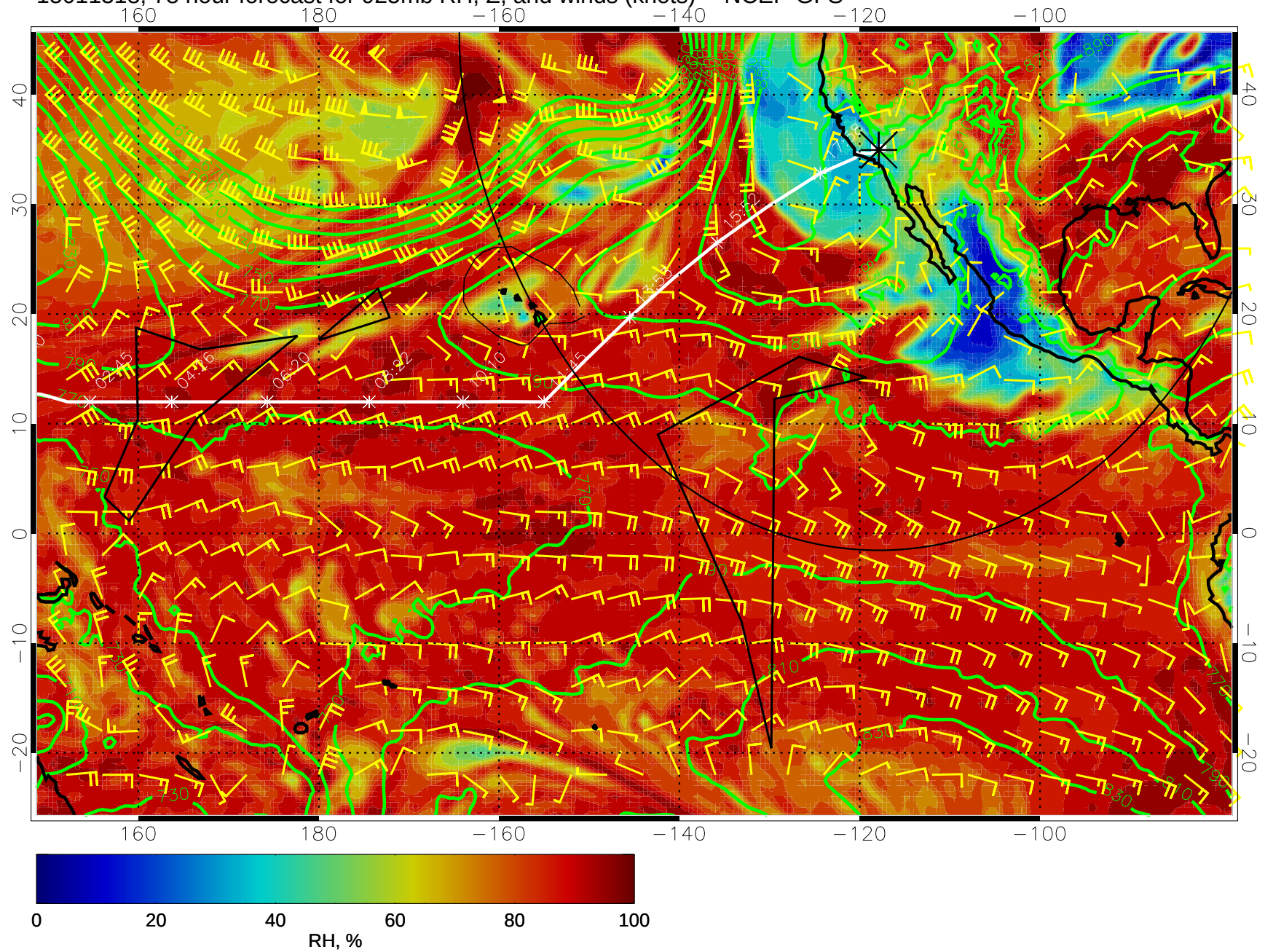
15011318, 78 hour forecast for 925mb RH, Z, and winds (knots) -- NCEP GFS
