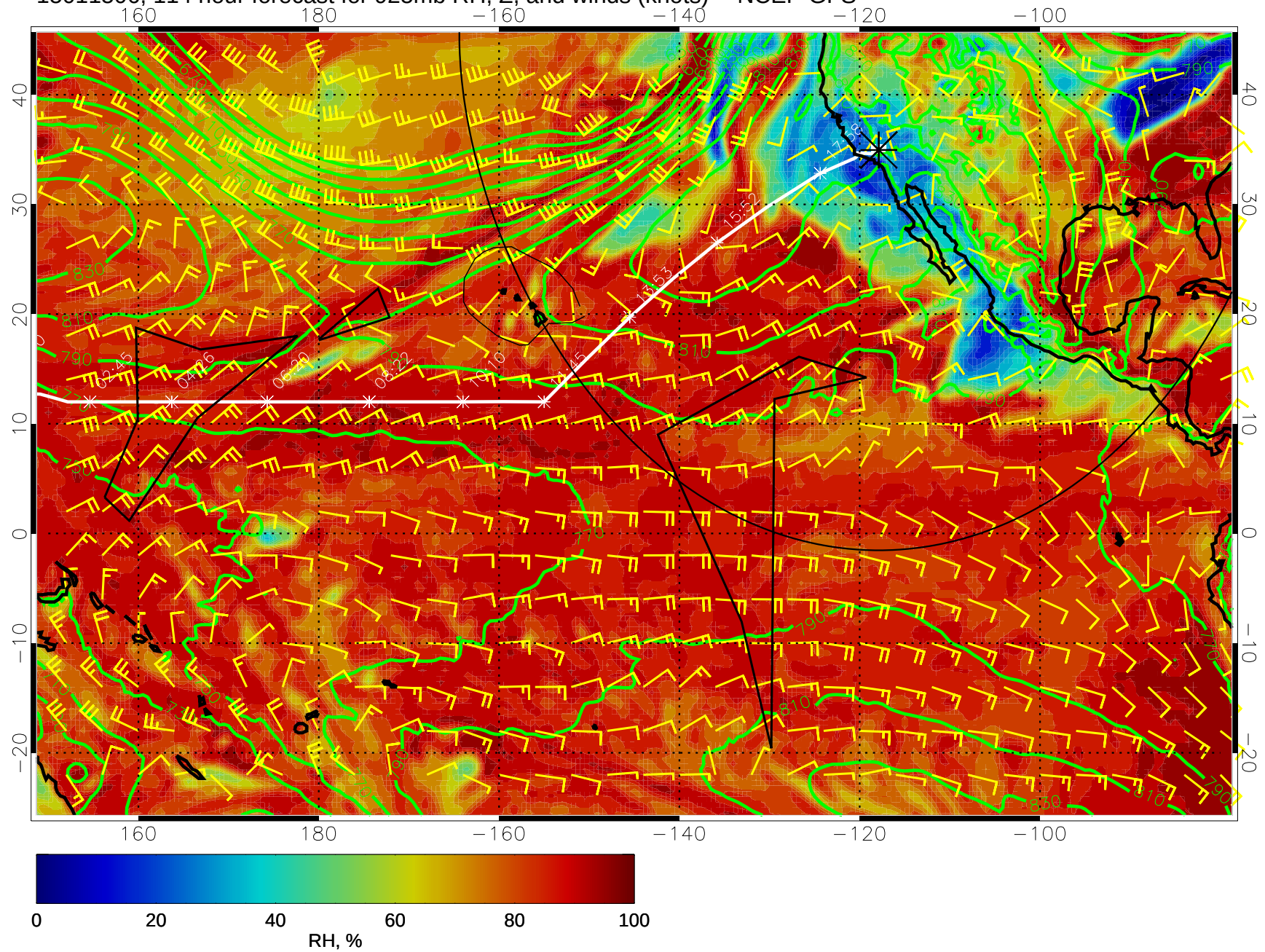
15011506, 114 hour forecast for 925mb RH, Z, and winds (knots) -- NCEP GFS
