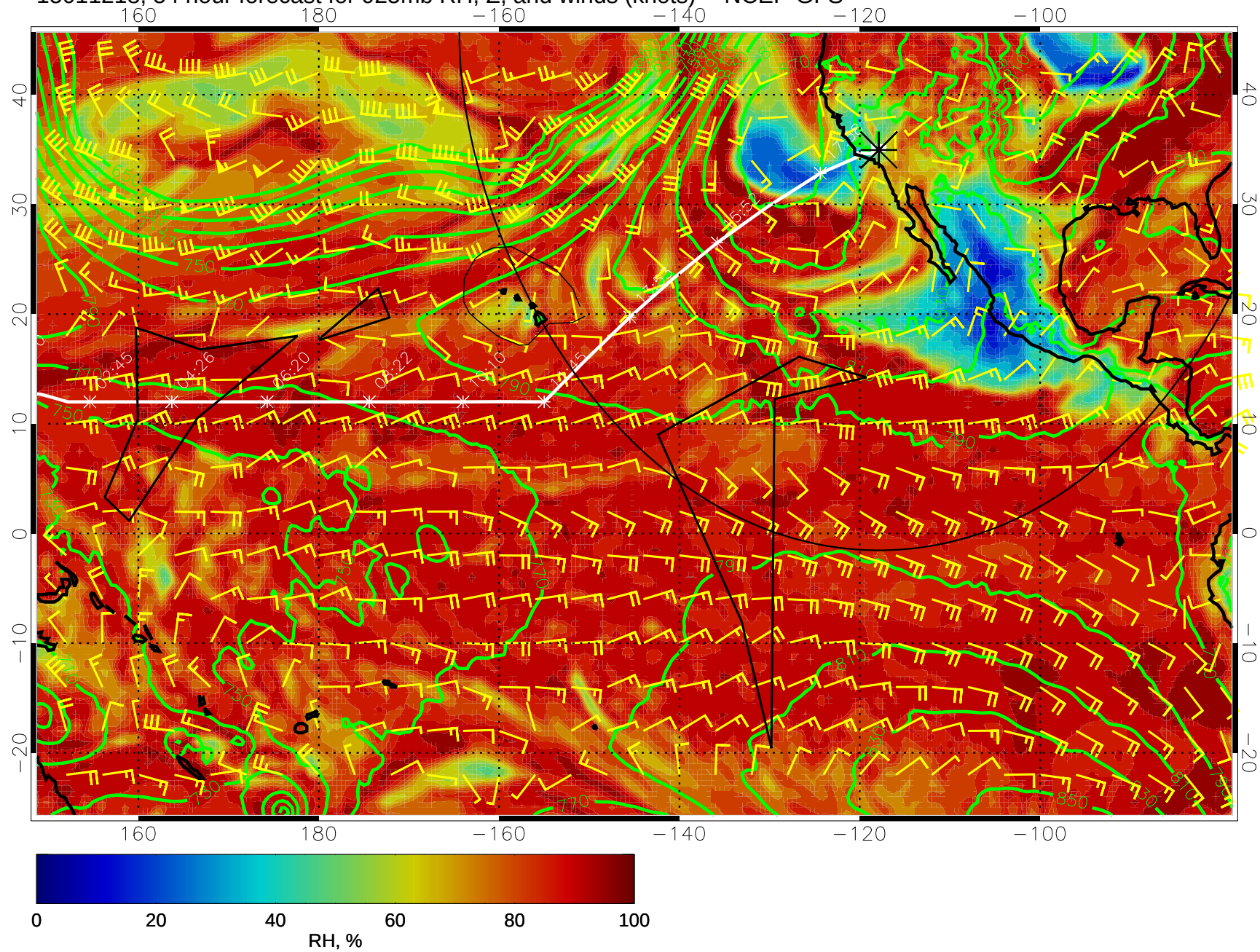
15011218, 54 hour forecast for 925mb RH, Z, and winds (knots) -- NCEP GFS
