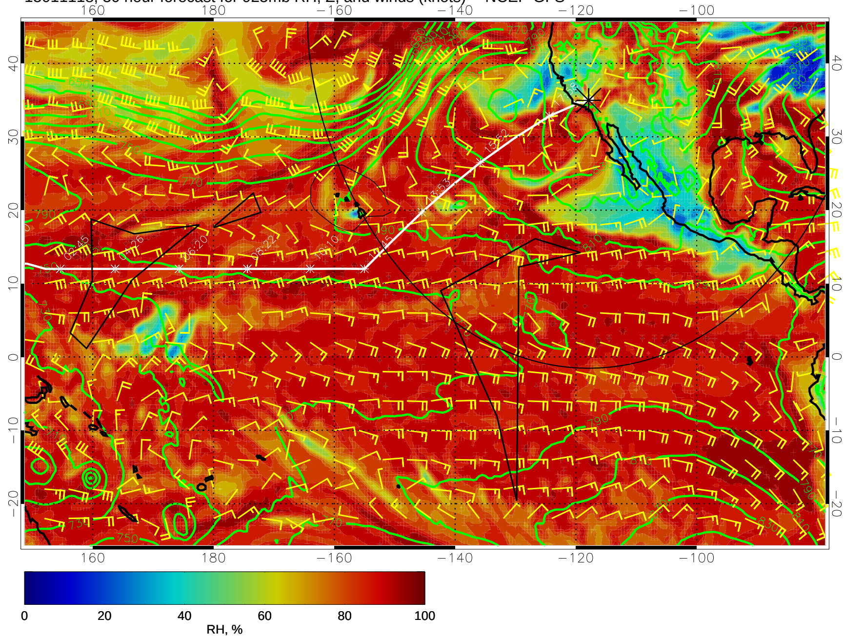
15011118, 30 hour forecast for 925mb RH, Z, and winds (knots) -- NCEP GFS
