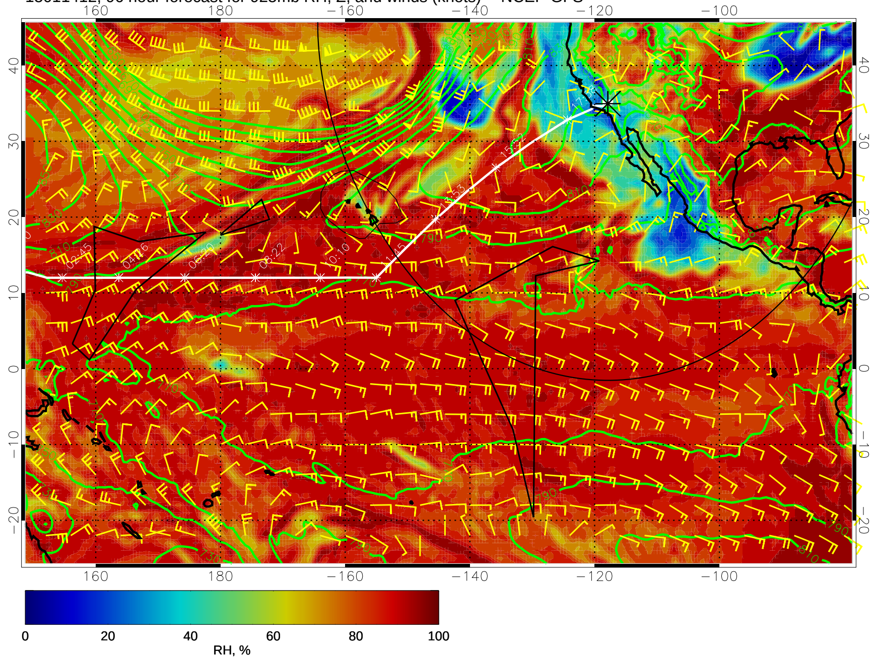
15011412, 96 hour forecast for 925mb RH, Z, and winds (knots) -- NCEP GFS
