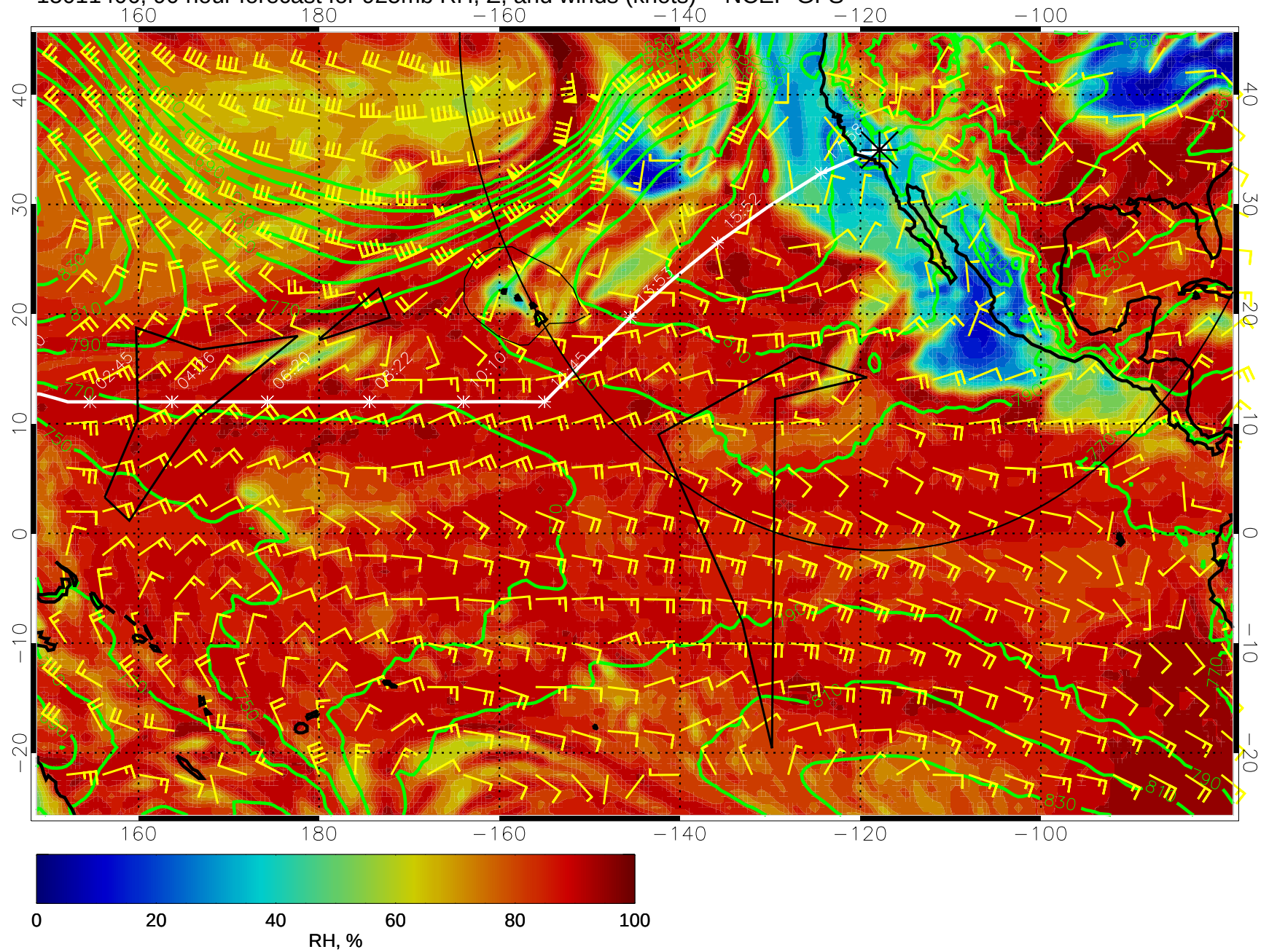
15011406, 90 hour forecast for 925mb RH, Z, and winds (knots) -- NCEP GFS
