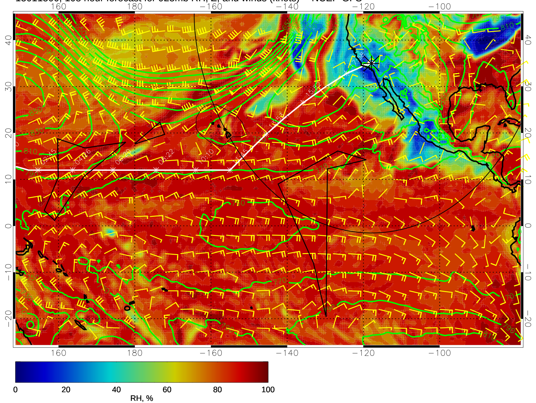
15011500, 108 hour forecast for 925mb RH, Z, and winds (knots) -- NCEP GFS
