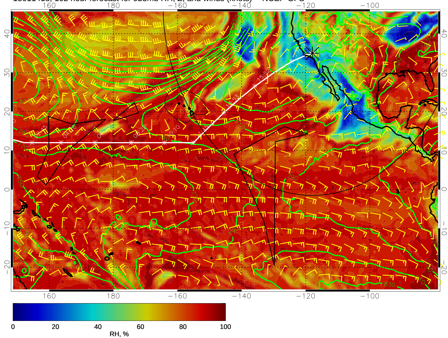
15011418, 102 hour forecast for 925mb RH, Z, and winds (knots) -- NCEP GFS
