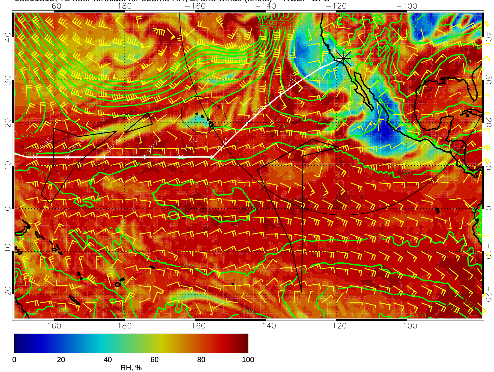
15011312, 72 hour forecast for 925mb RH, Z, and winds (knots) -- NCEP GFS
