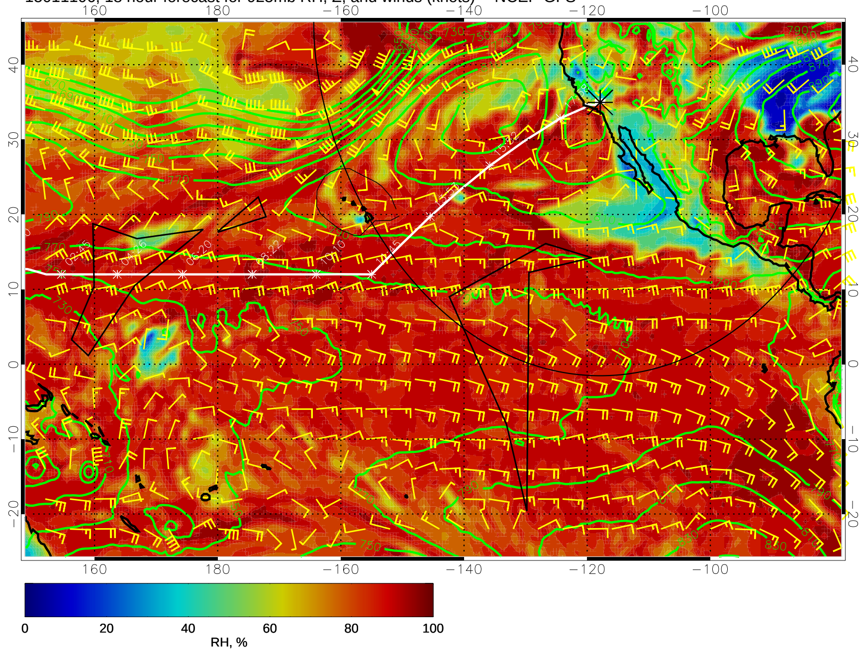
15011106, 18 hour forecast for 925mb RH, Z, and winds (knots) -- NCEP GFS
