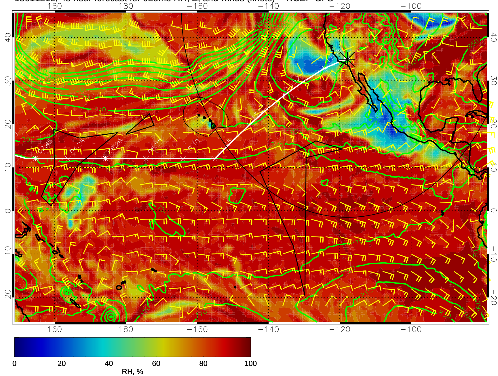
15011212, 48 hour forecast for 925mb RH, Z, and winds (knots) -- NCEP GFS
