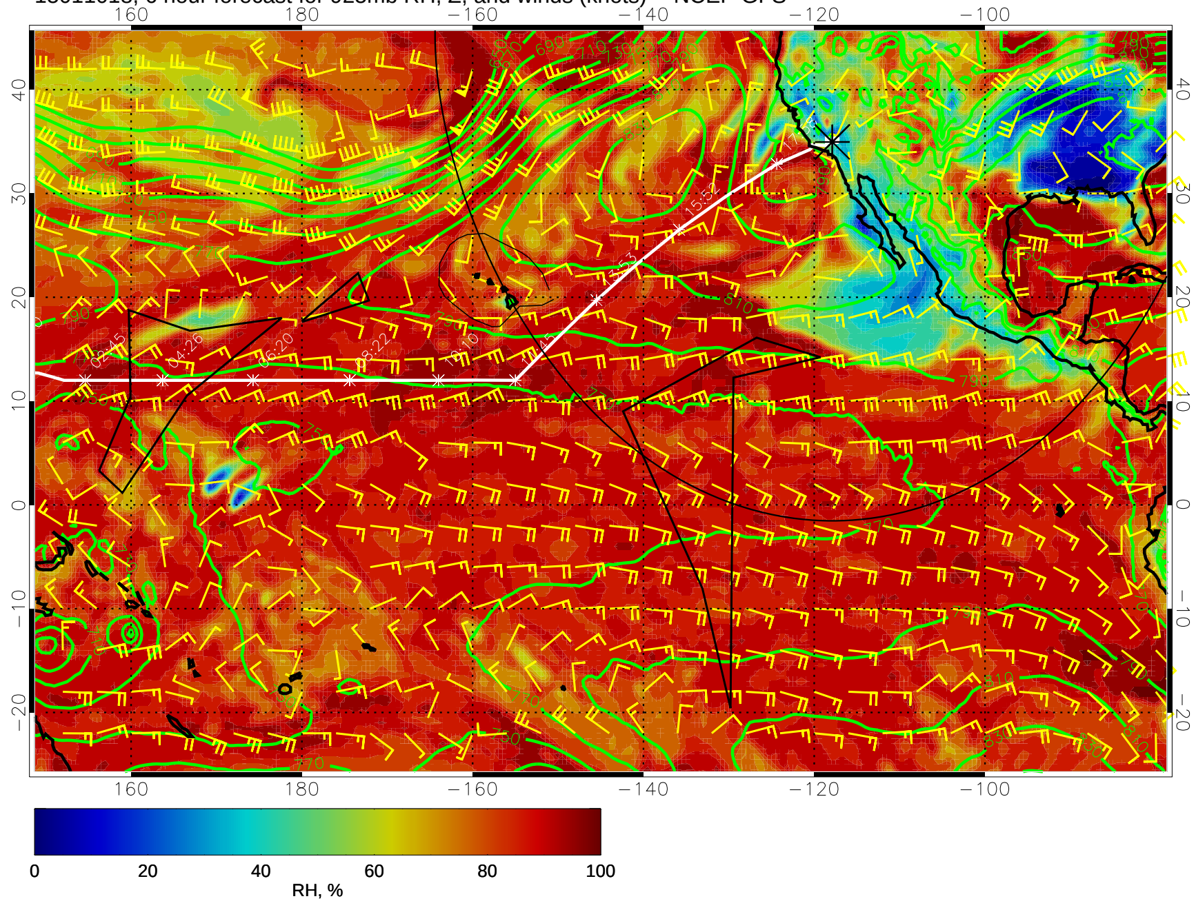
15011018, 6 hour forecast for 925mb RH, Z, and winds (knots) -- NCEP GFS
