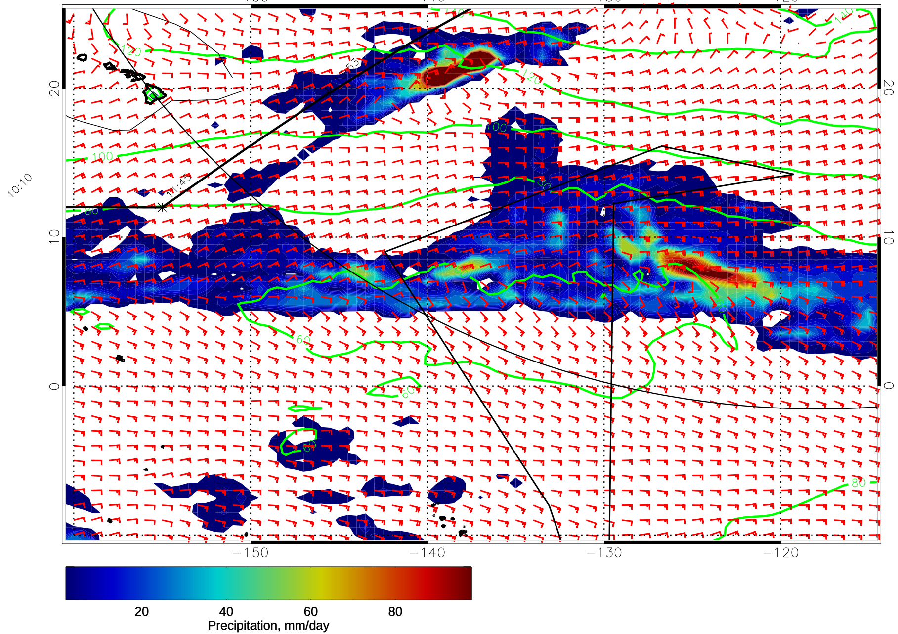
15011112, 24 hour forecast for precip, 1000mb Z, and winds (knots) -- NCEP GFS
