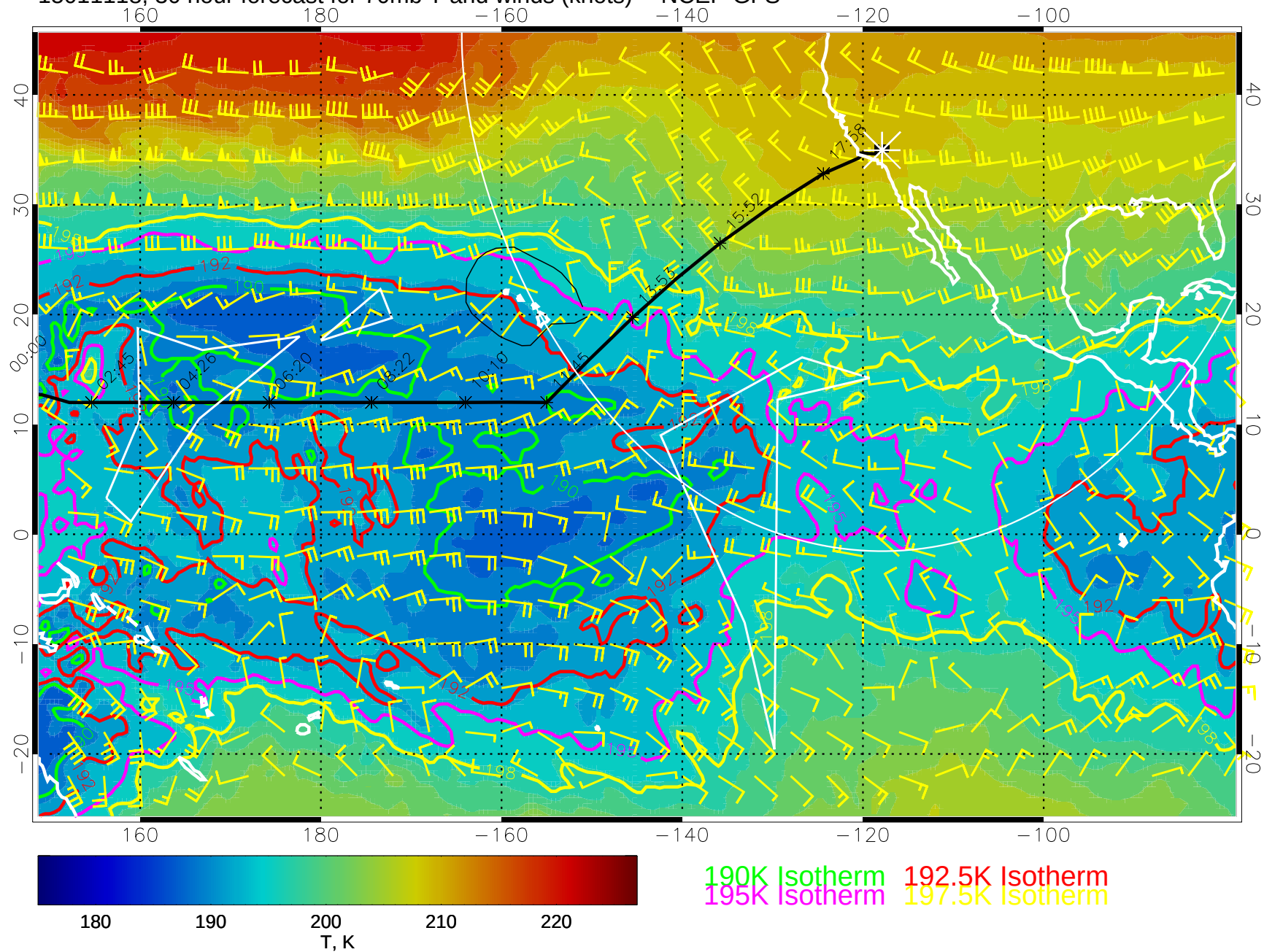
15011118, 30 hour forecast for 70mb T and winds (knots) -- NCEP GFS
