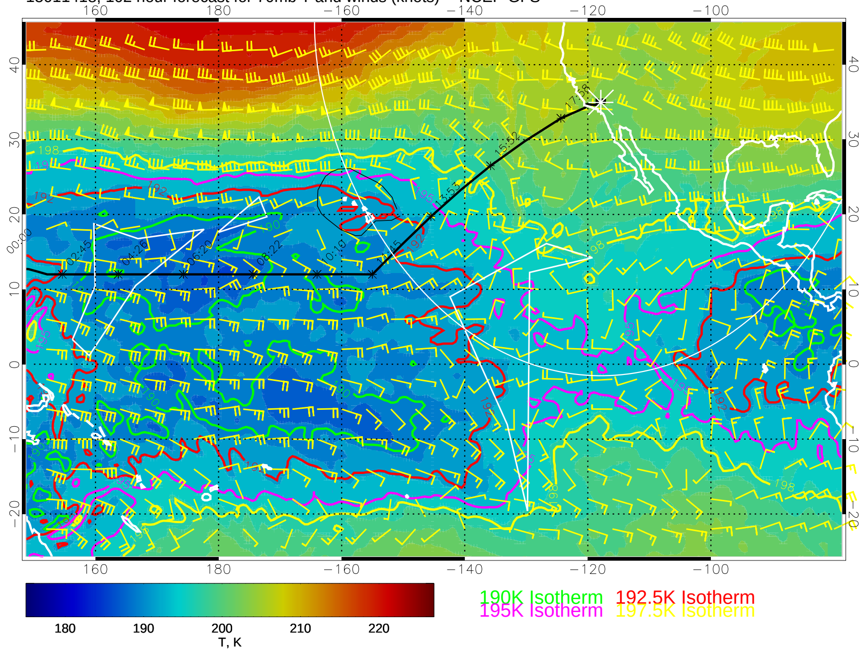
15011418, 102 hour forecast for 70mb T and winds (knots) -- NCEP GFS
