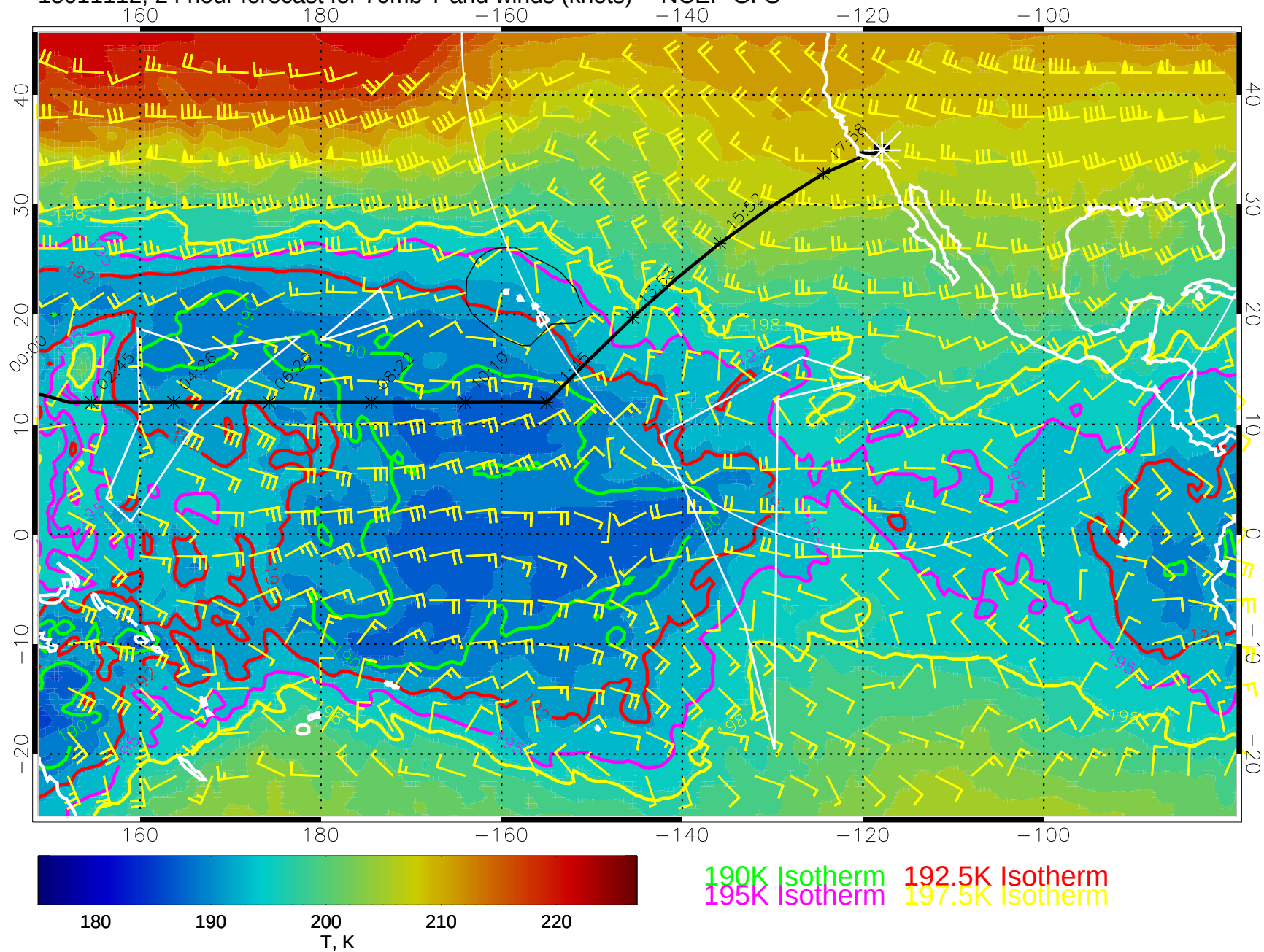
15011112, 24 hour forecast for 70mb T and winds (knots) -- NCEP GFS
