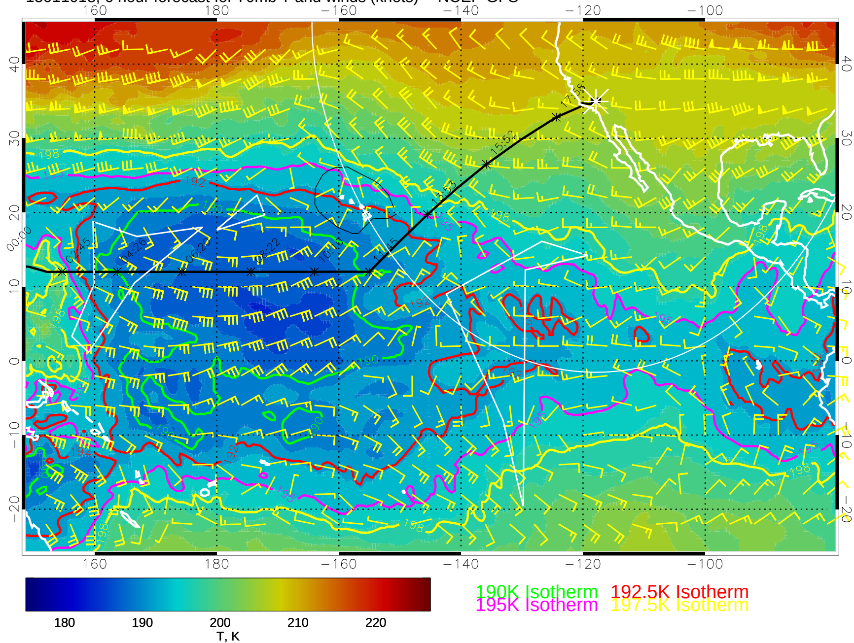
15011018, 6 hour forecast for 70mb T and winds (knots) -- NCEP GFS
