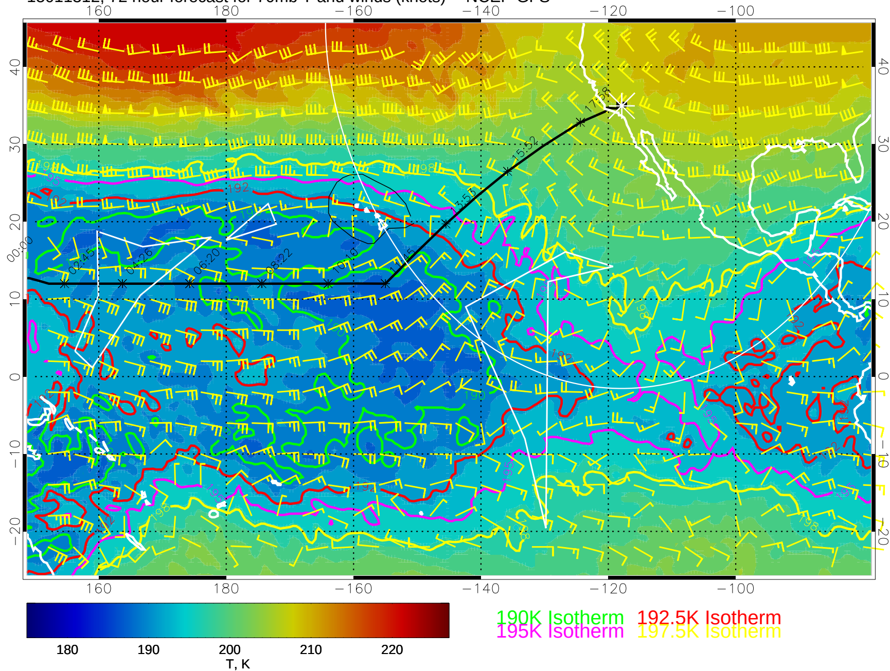
15011312, 72 hour forecast for 70mb T and winds (knots) -- NCEP GFS
