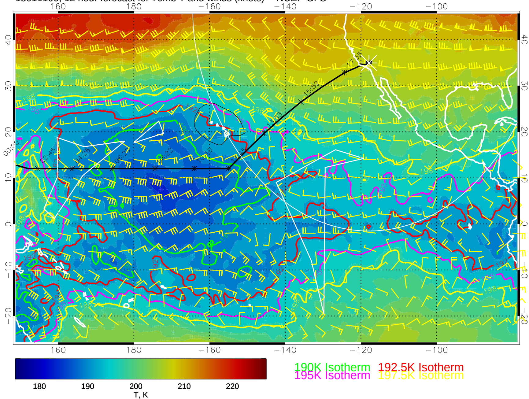
15011100, 12 hour forecast for 70mb T and winds (knots) -- NCEP GFS
