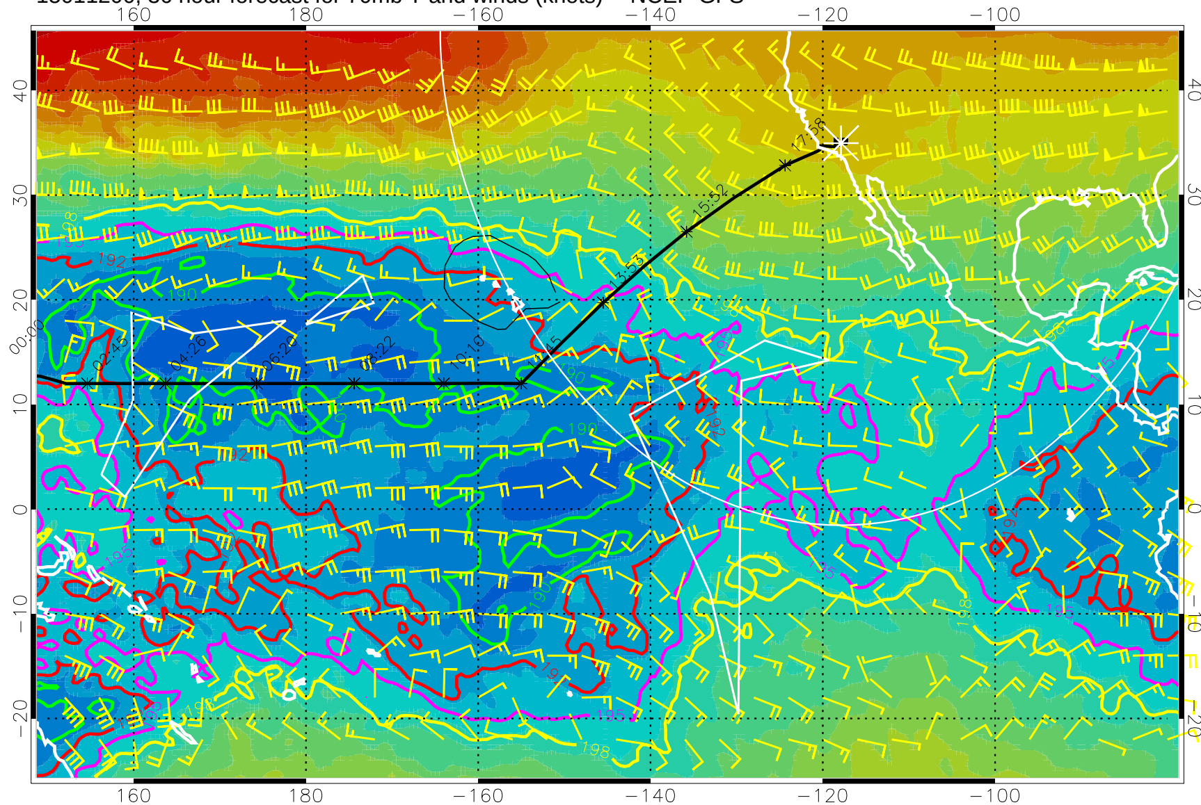
15011200, 36 hour forecast for 70mb T and winds (knots) -- NCEP GFS
