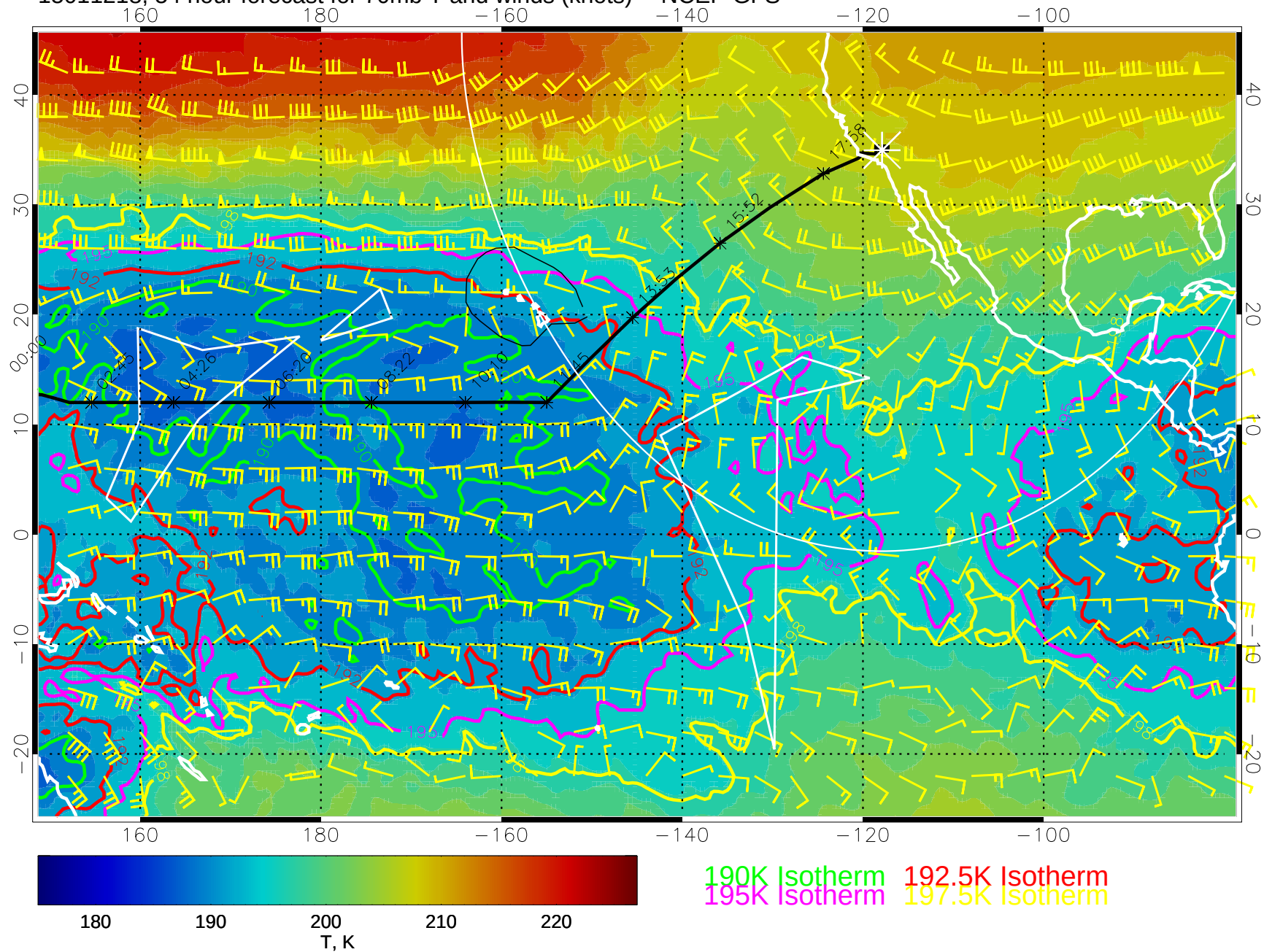
15011218, 54 hour forecast for 70mb T and winds (knots) -- NCEP GFS
