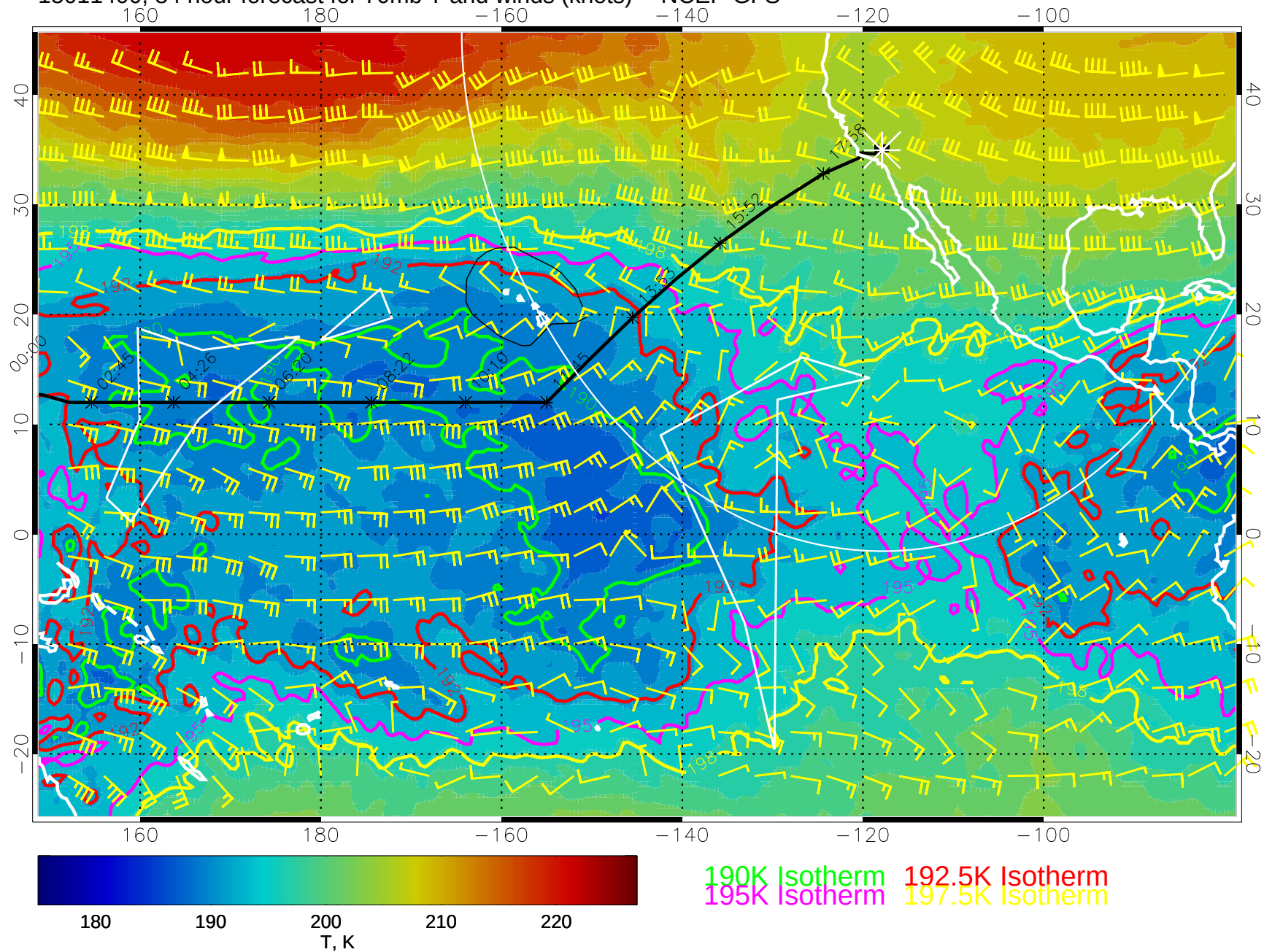
15011400, 84 hour forecast for 70mb T and winds (knots) -- NCEP GFS
