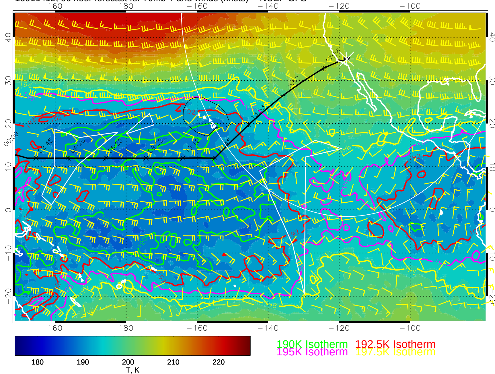
15011412, 96 hour forecast for 70mb T and winds (knots) -- NCEP GFS
