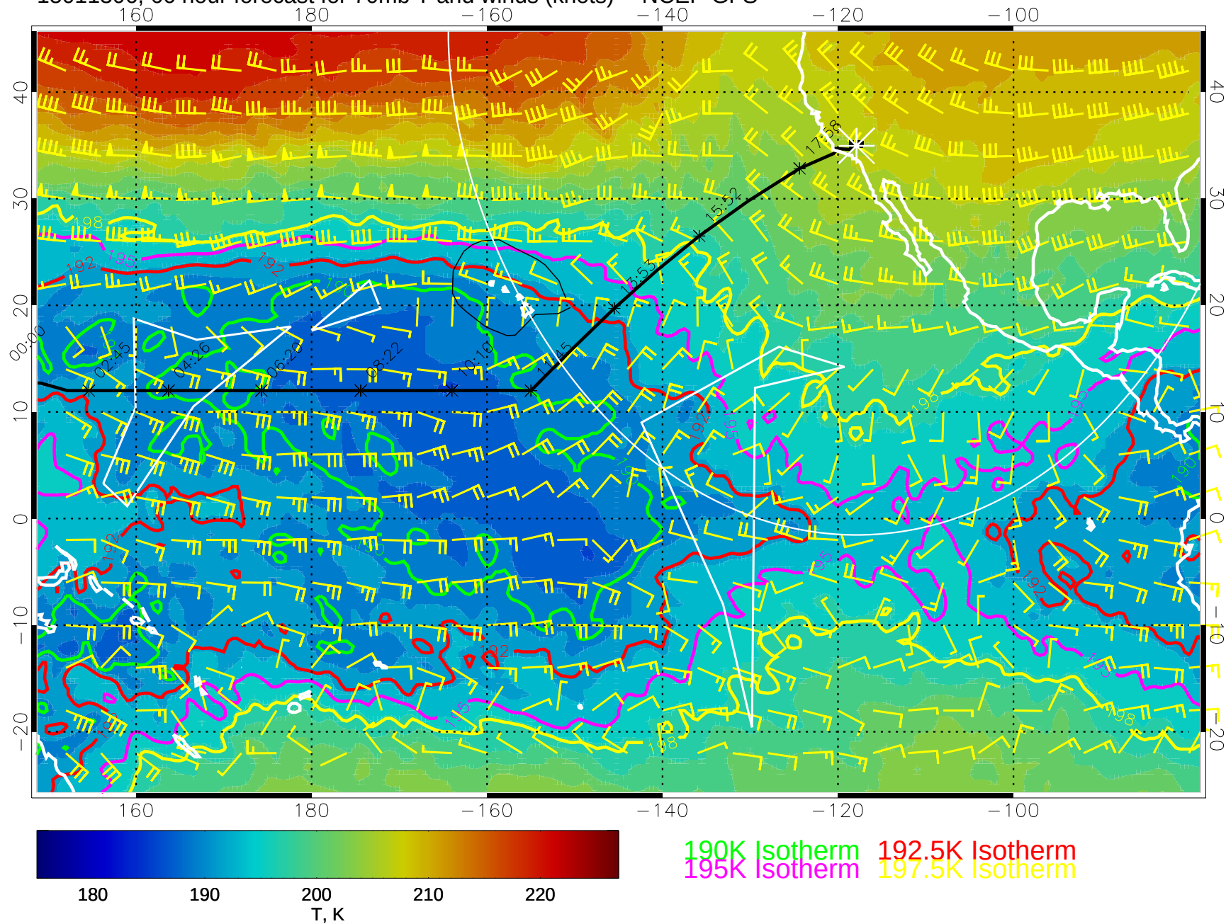
15011306, 66 hour forecast for 70mb T and winds (knots) -- NCEP GFS
