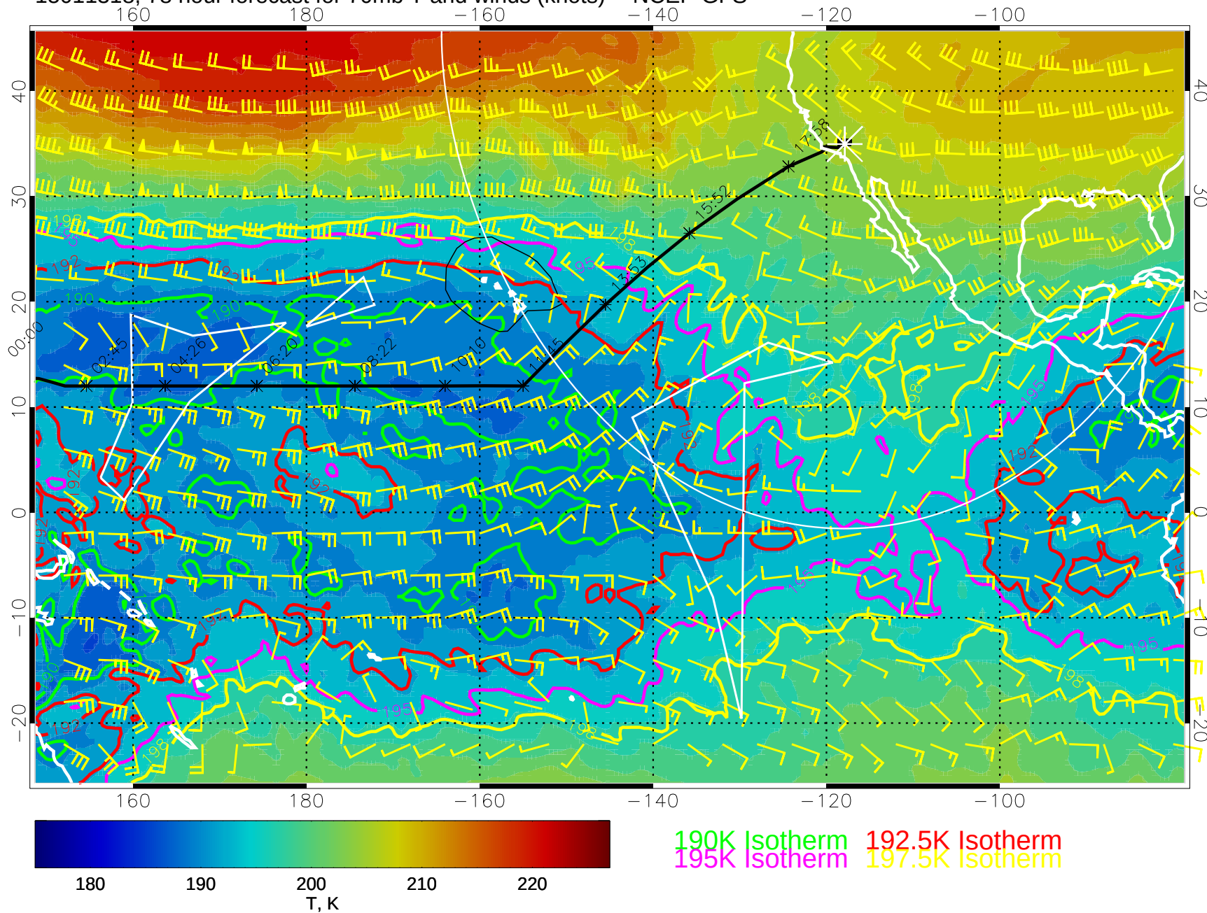
15011318, 78 hour forecast for 70mb T and winds (knots) -- NCEP GFS
