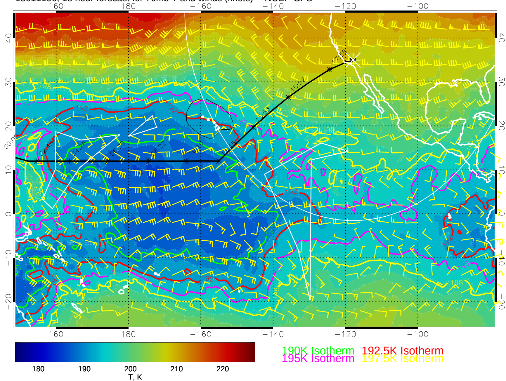
15011106, 18 hour forecast for 70mb T and winds (knots) -- NCEP GFS
