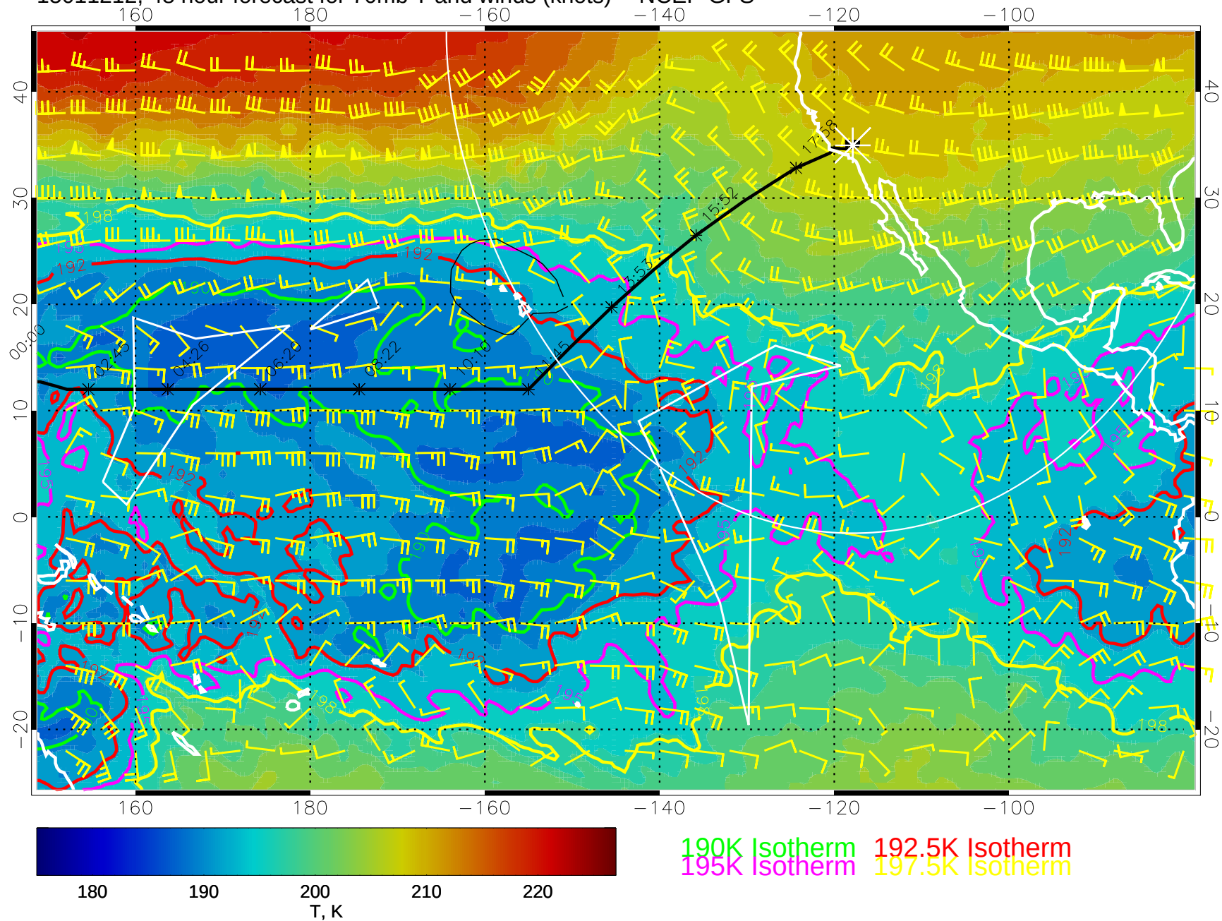
15011212, 48 hour forecast for 70mb T and winds (knots) -- NCEP GFS
