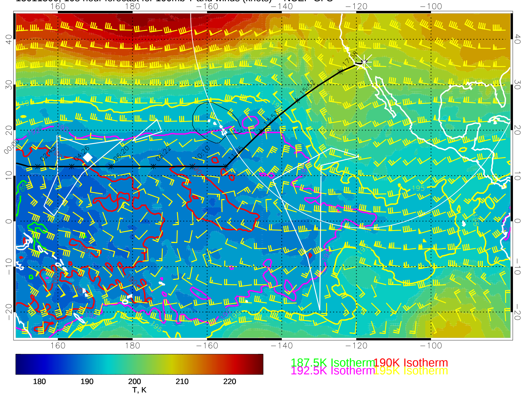
15011500, 108 hour forecast for 100mb T and winds (knots) -- NCEP GFS
