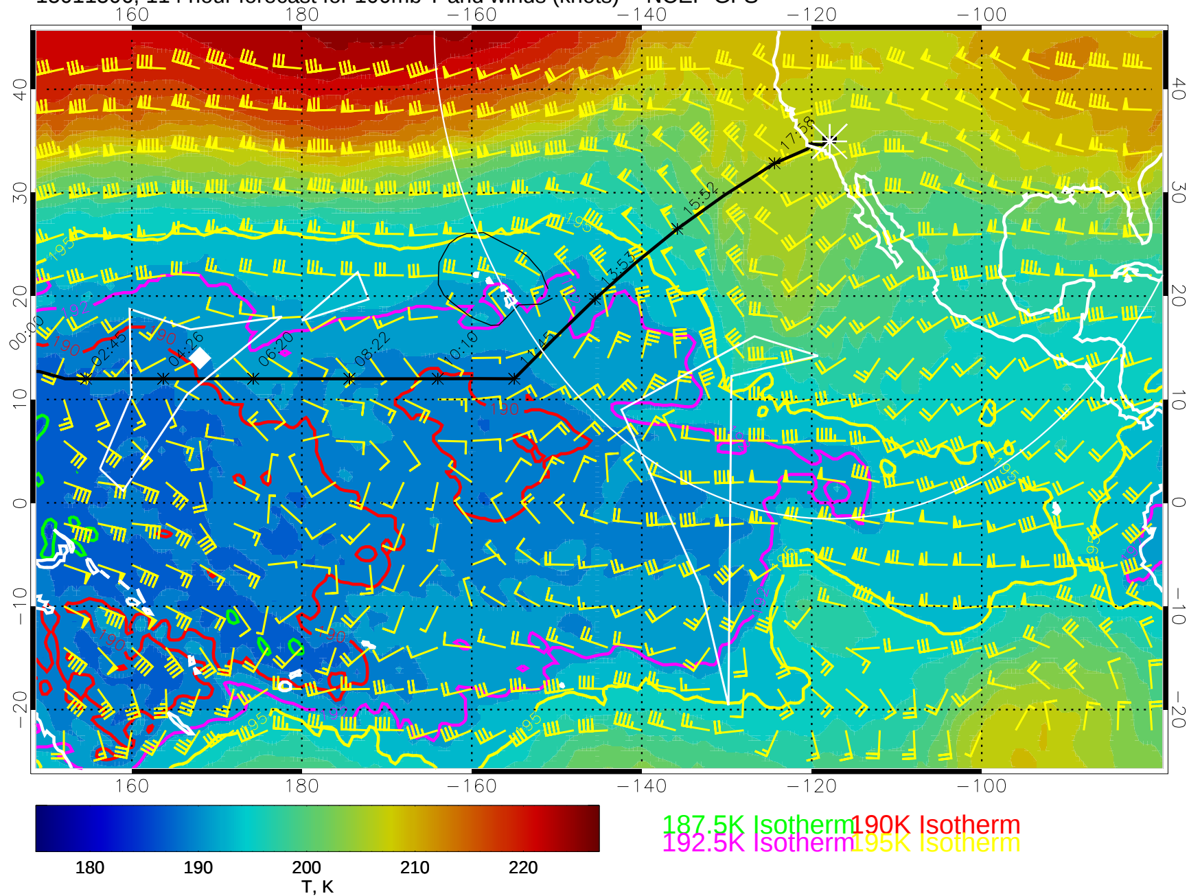
15011506, 114 hour forecast for 100mb T and winds (knots) -- NCEP GFS
