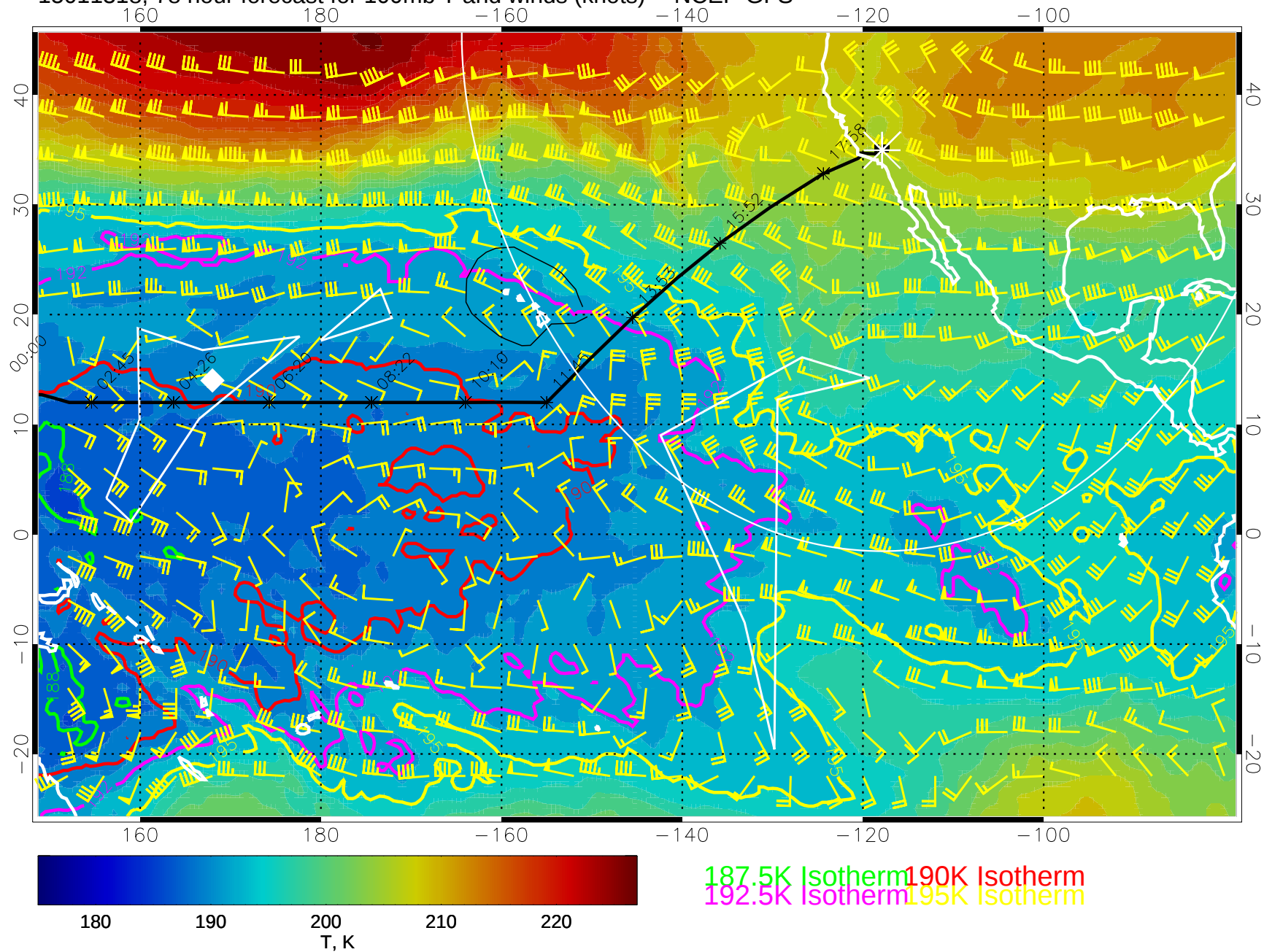
15011318, 78 hour forecast for 100mb T and winds (knots) -- NCEP GFS
