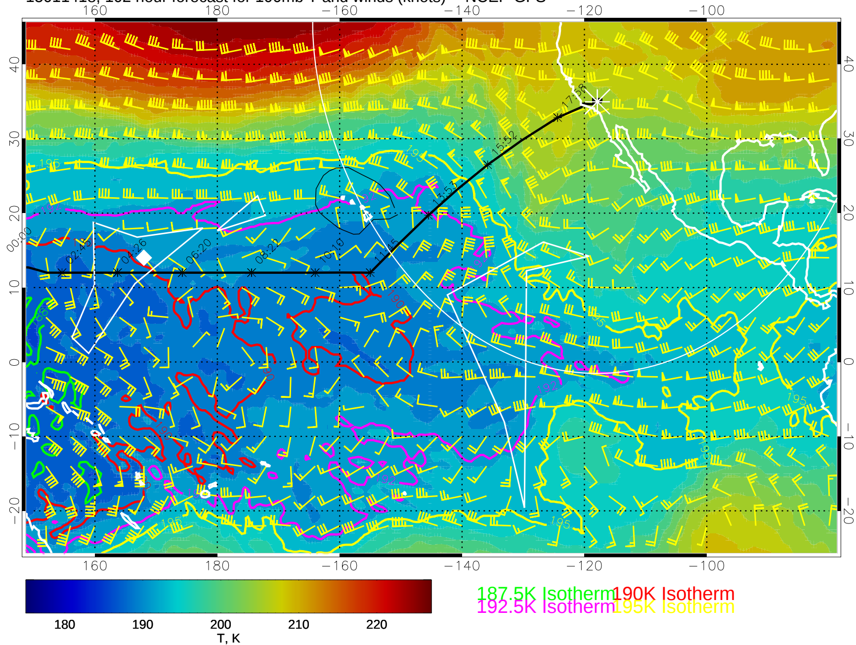
15011418, 102 hour forecast for 100mb T and winds (knots) -- NCEP GFS
