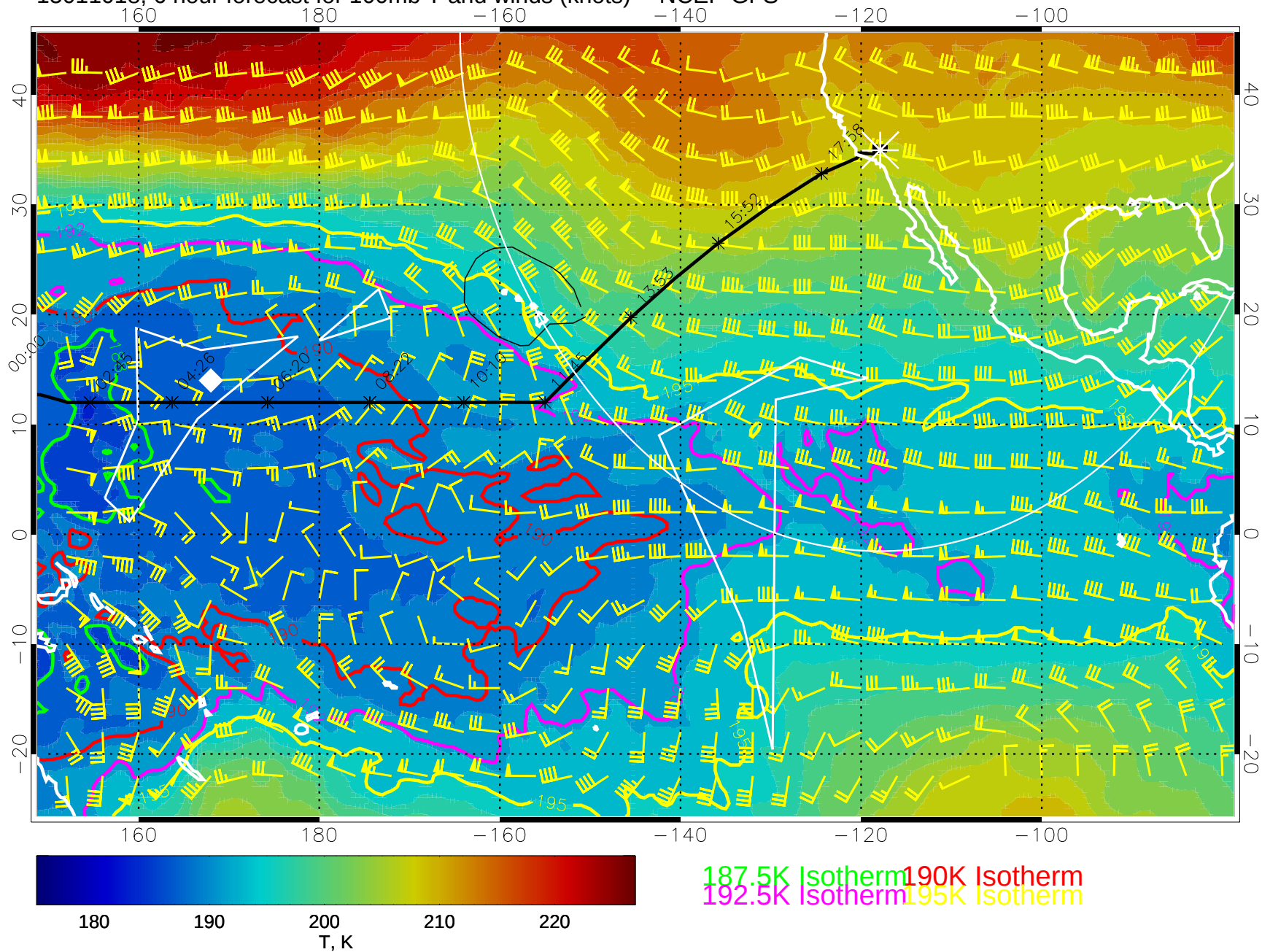
15011018, 6 hour forecast for 100mb T and winds (knots) -- NCEP GFS
