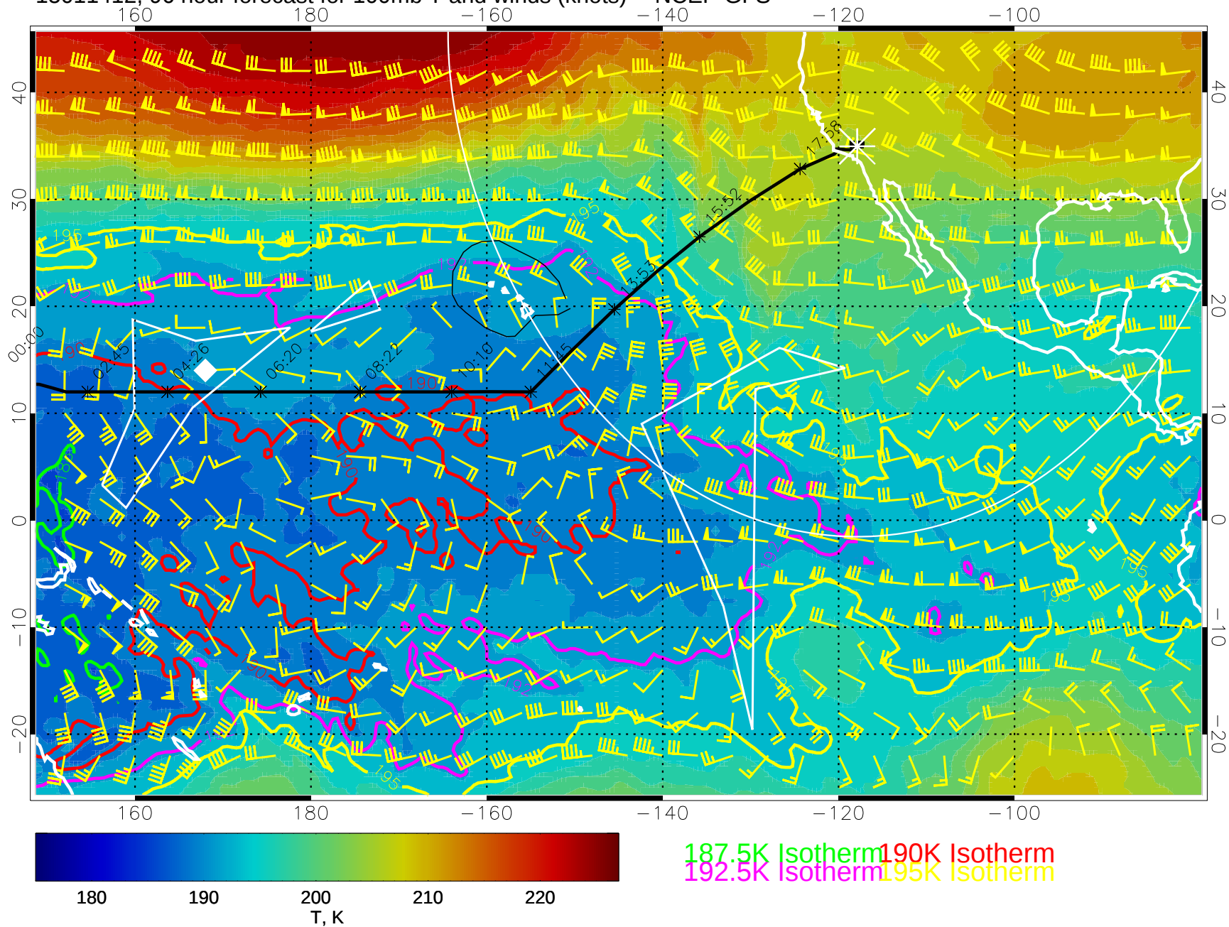
15011412, 96 hour forecast for 100mb T and winds (knots) -- NCEP GFS
