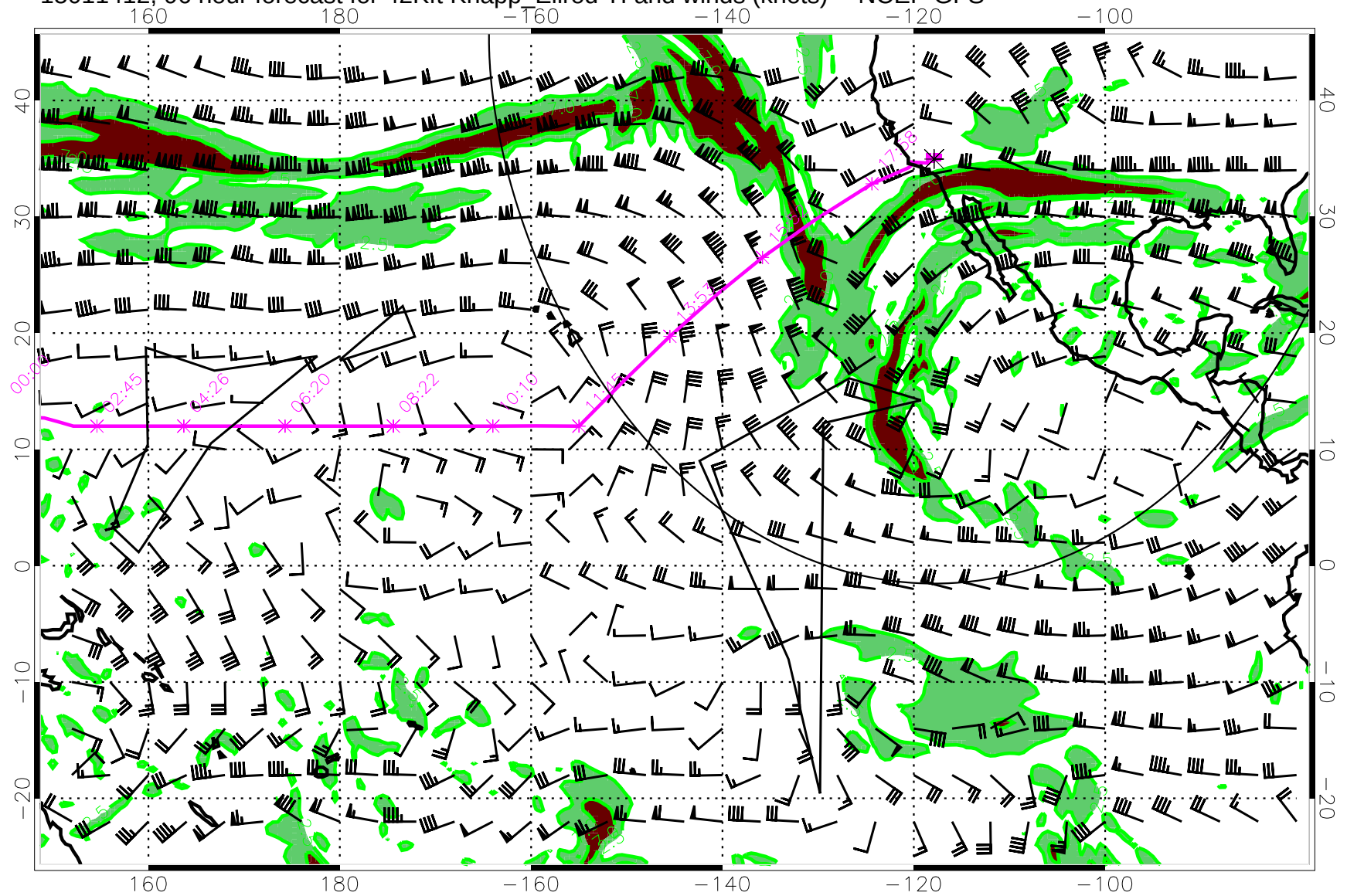
15011412, 96 hour forecast for 42Kft Knapp_Ellrod TI and winds (knots) -- NCEP GFS
