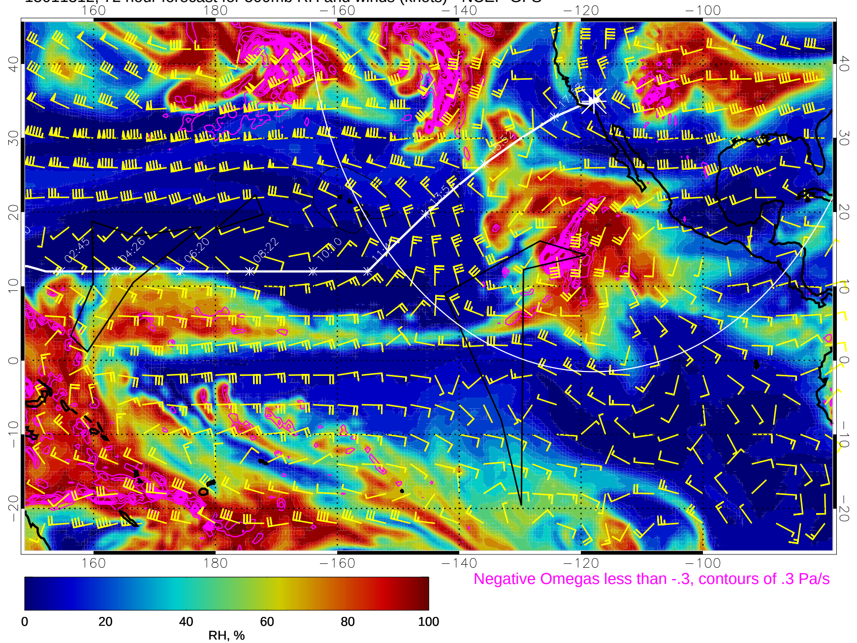
15011312, 72 hour forecast for 500mb RH and winds (knots) - NCEP GFS
