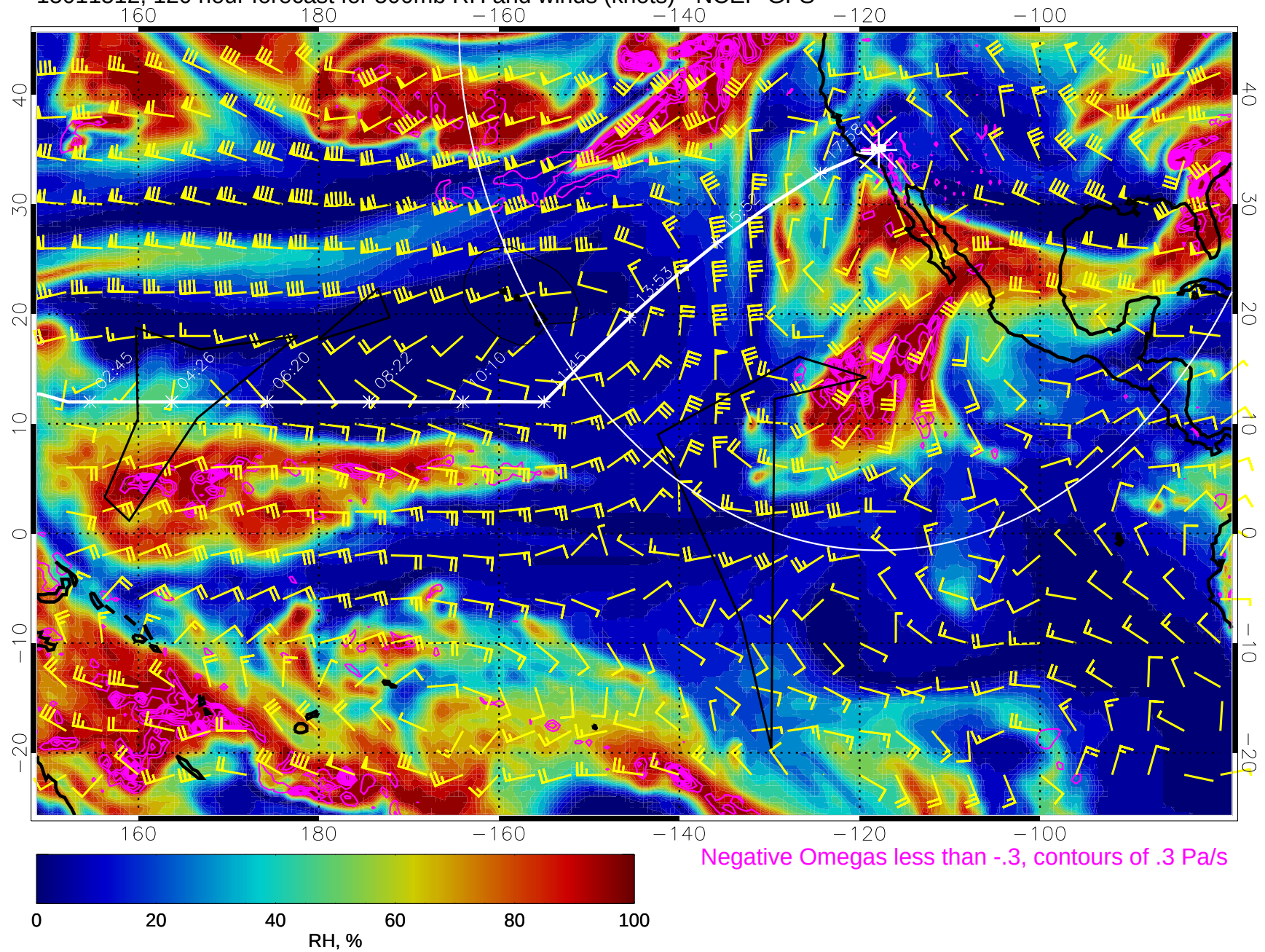
15011512, 120 hour forecast for 500mb RH and winds (knots) - NCEP GFS
