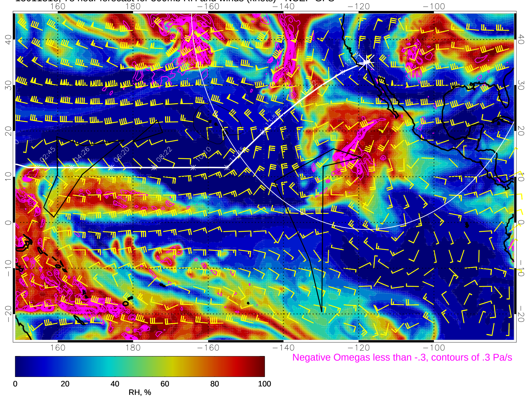
15011318, 78 hour forecast for 500mb RH and winds (knots) - NCEP GFS
