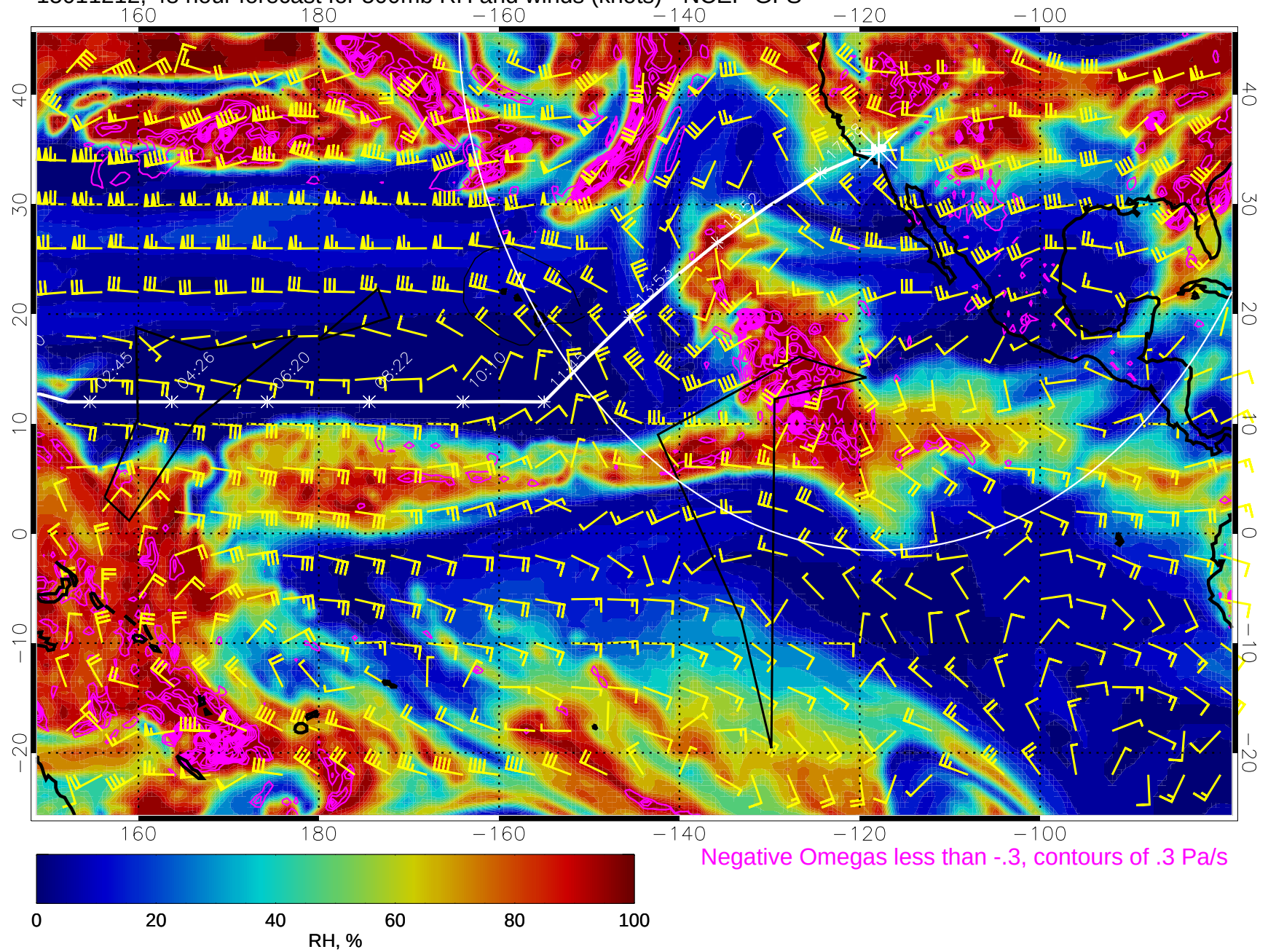
15011212, 48 hour forecast for 500mb RH and winds (knots) - NCEP GFS
