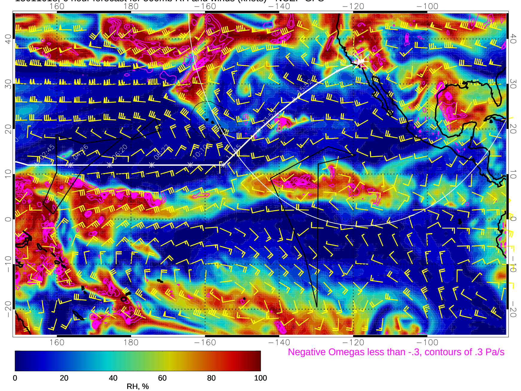
15011018, 6 hour forecast for 500mb RH and winds (knots) - NCEP GFS
