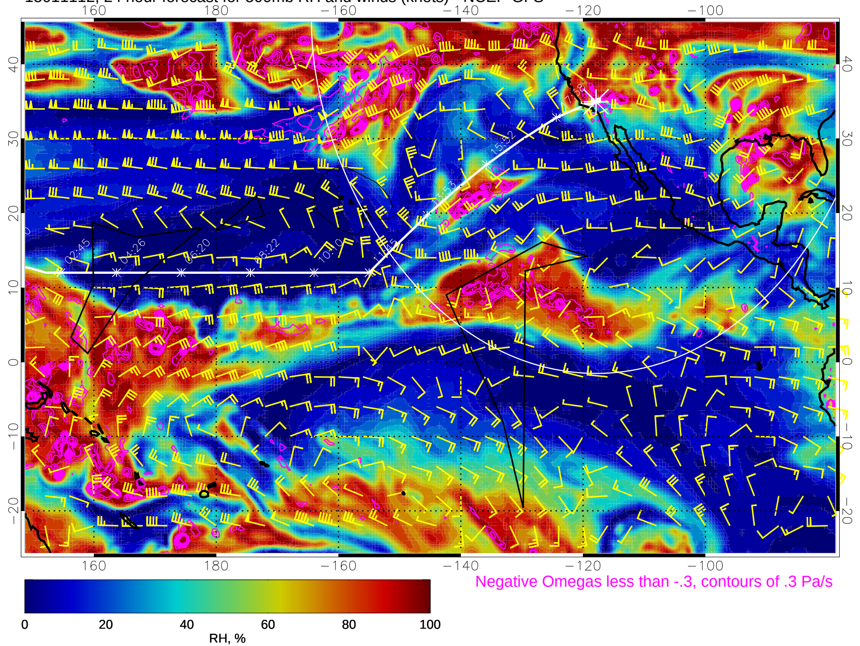
15011112, 24 hour forecast for 500mb RH and winds (knots) - NCEP GFS
