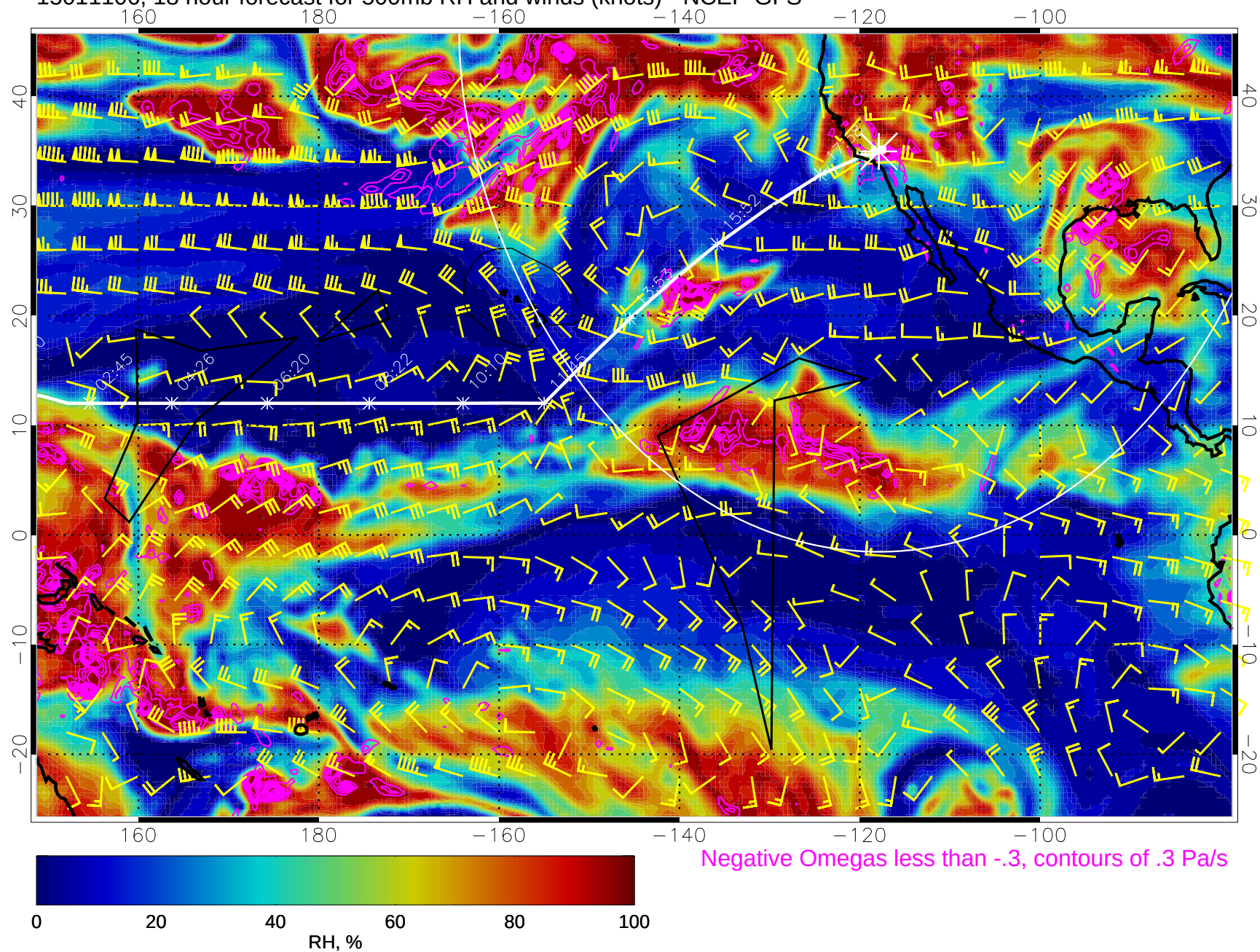
15011106, 18 hour forecast for 500mb RH and winds (knots) - NCEP GFS
