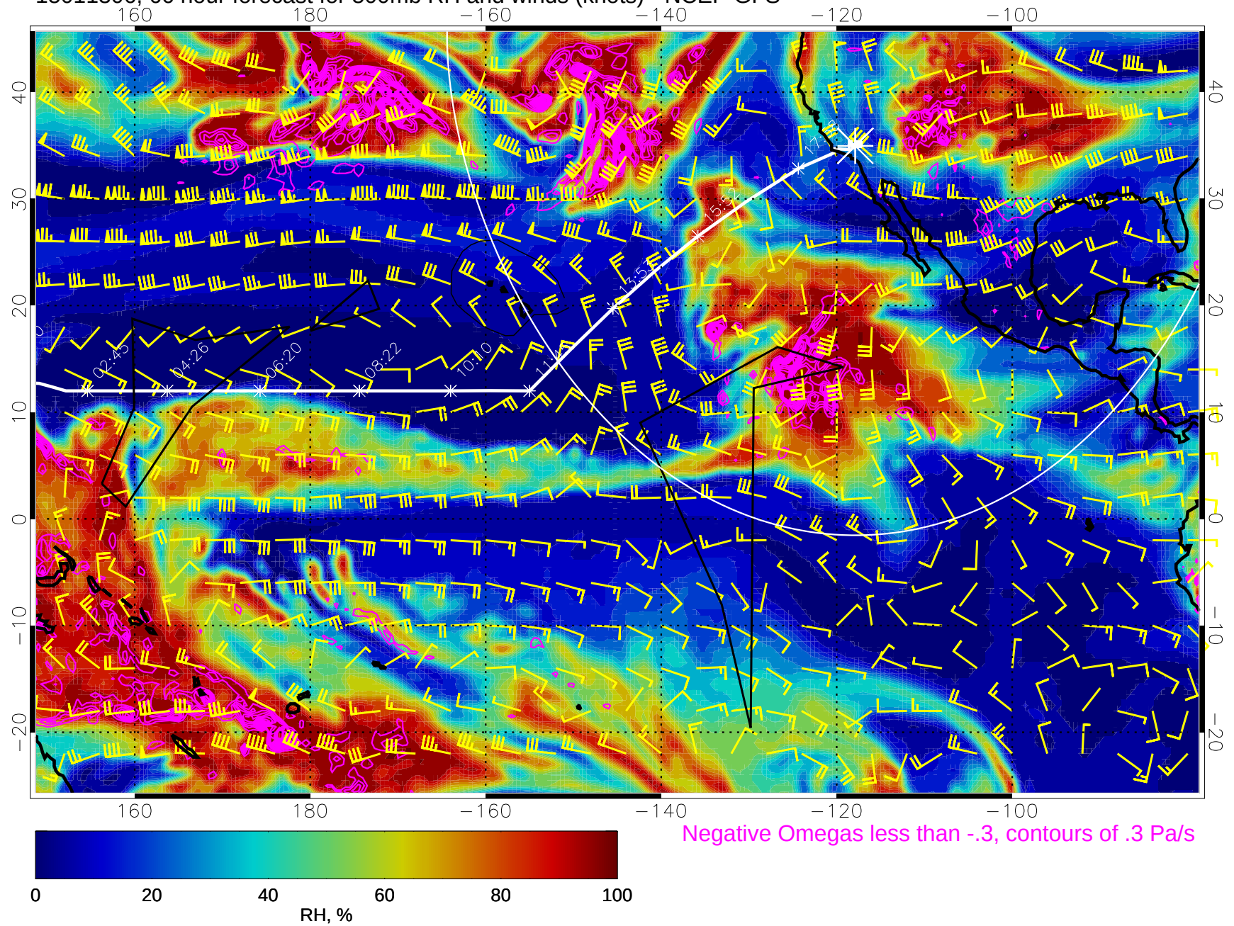
15011306, 66 hour forecast for 500mb RH and winds (knots) - NCEP GFS
