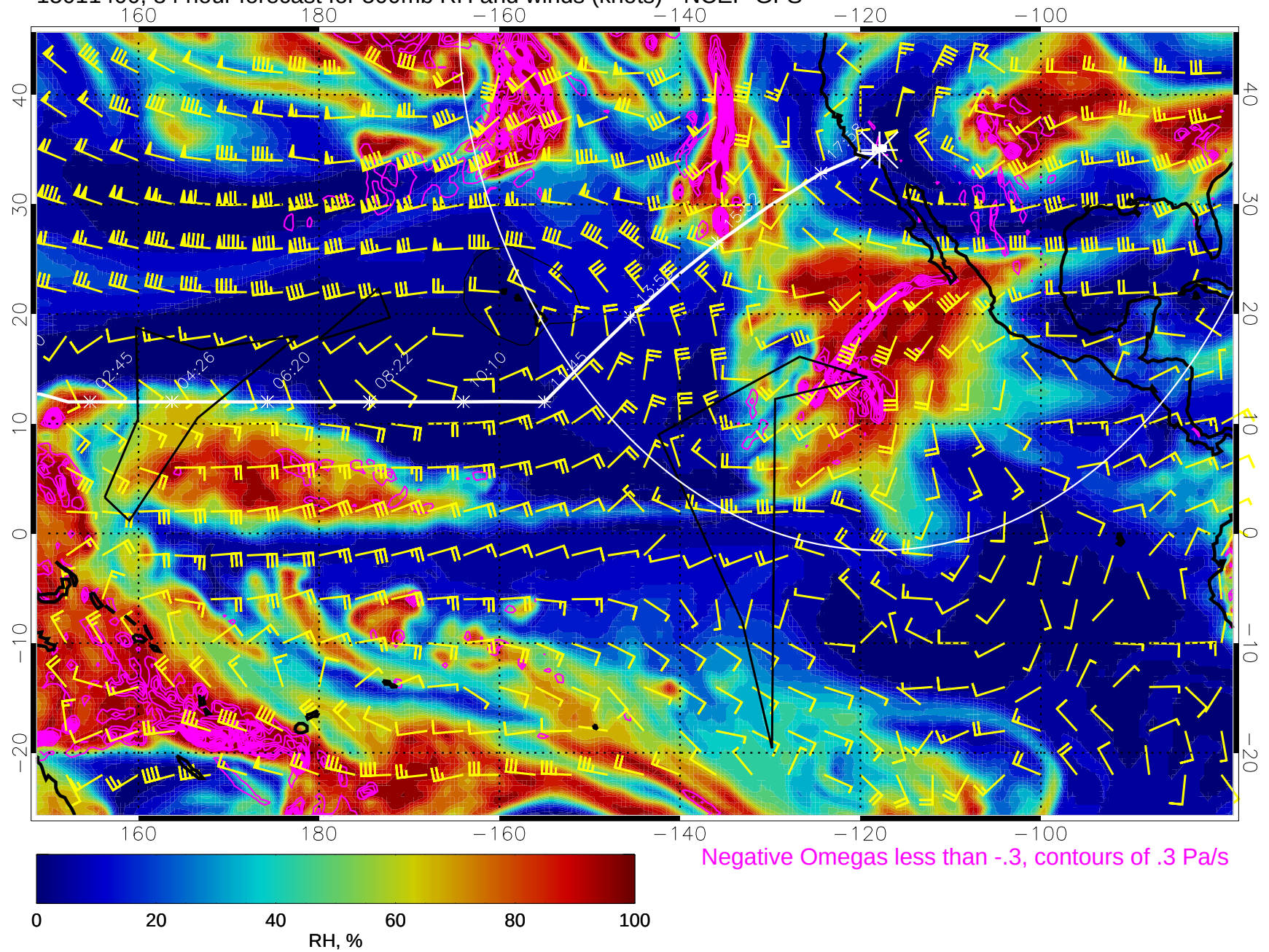
15011400, 84 hour forecast for 500mb RH and winds (knots) - NCEP GFS
