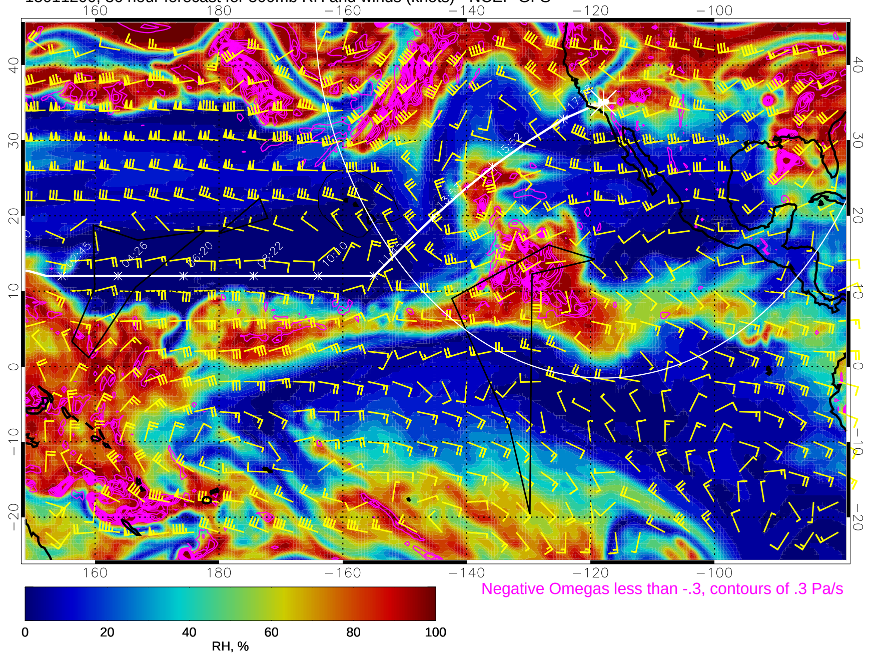
15011200, 36 hour forecast for 500mb RH and winds (knots) - NCEP GFS
