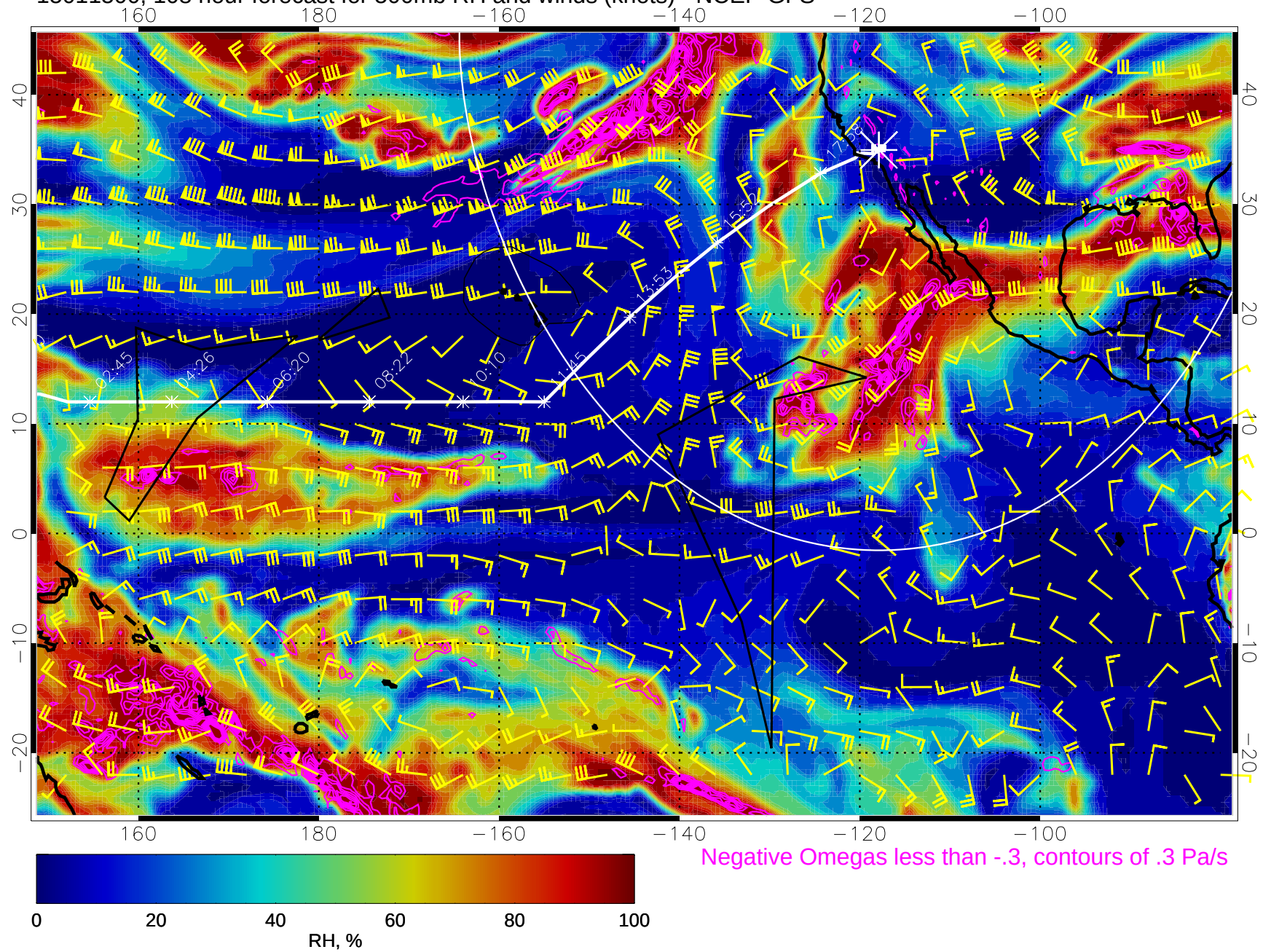
15011500, 108 hour forecast for 500mb RH and winds (knots) - NCEP GFS
