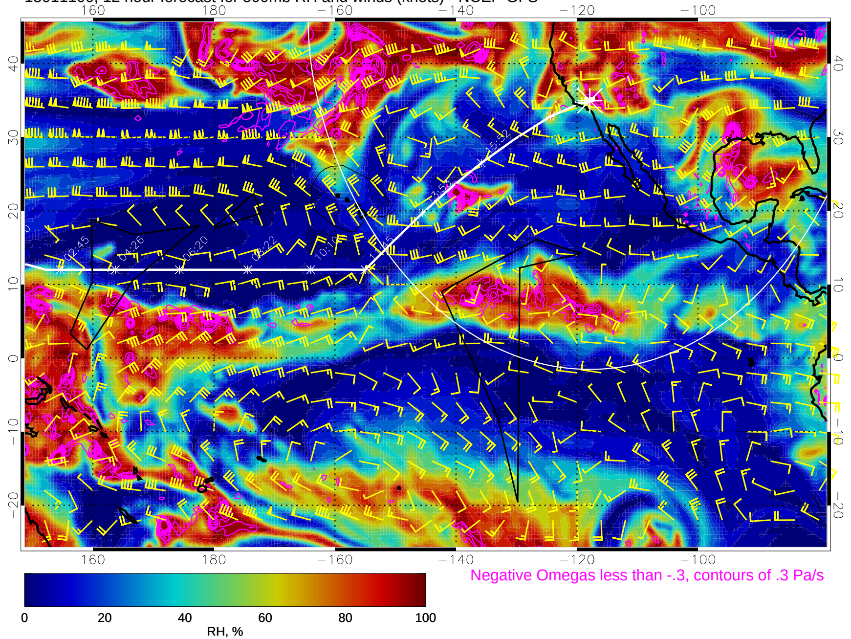
15011100, 12 hour forecast for 500mb RH and winds (knots) - NCEP GFS
