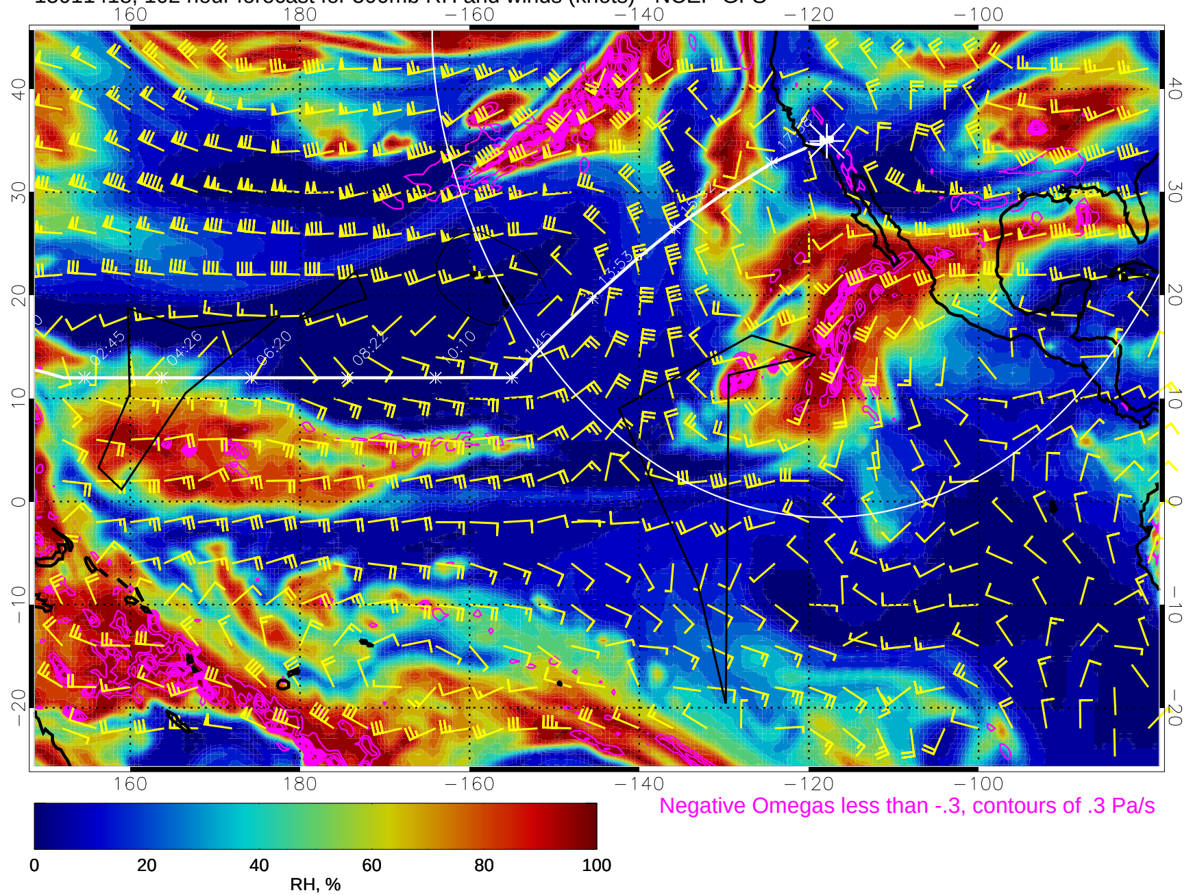
15011418, 102 hour forecast for 500mb RH and winds (knots) - NCEP GFS
