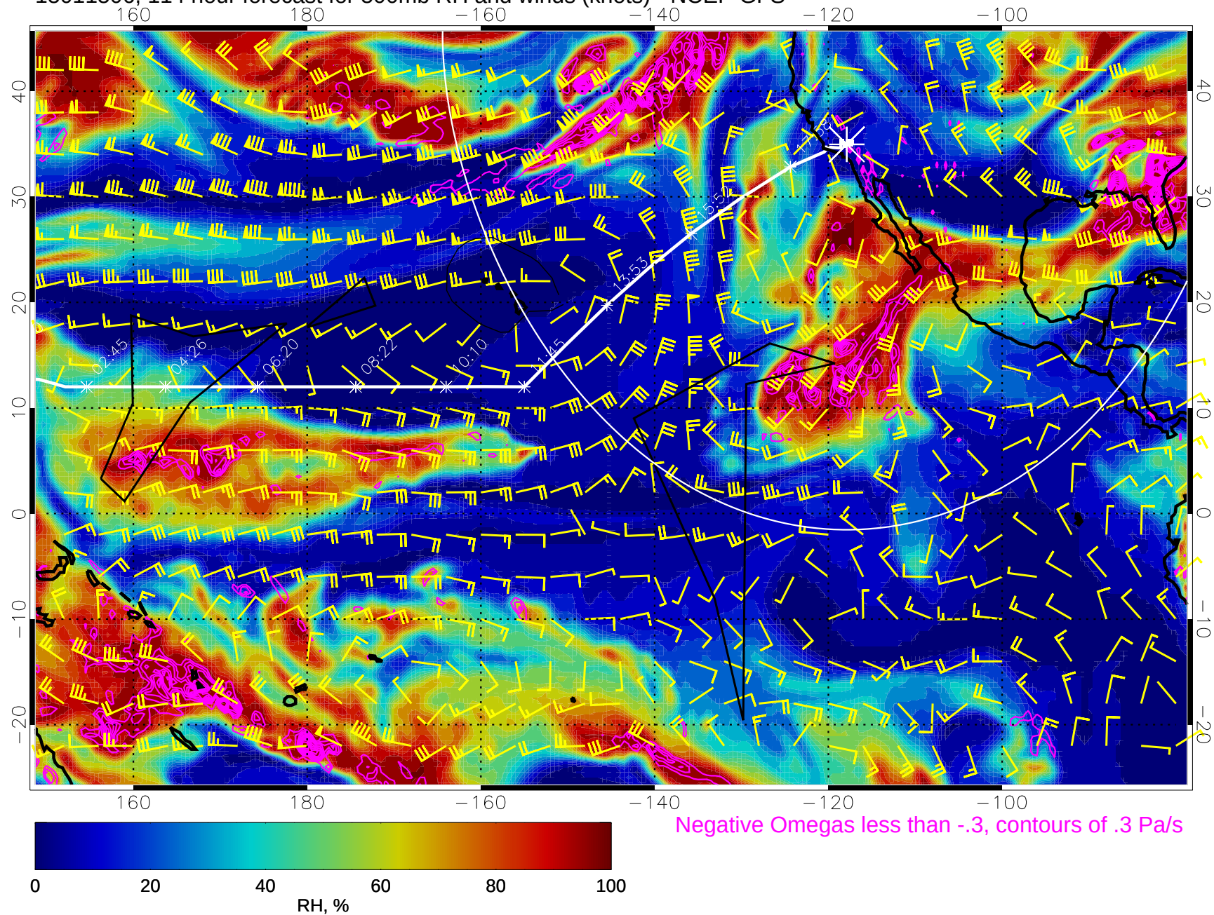
15011506, 114 hour forecast for 500mb RH and winds (knots) - NCEP GFS
