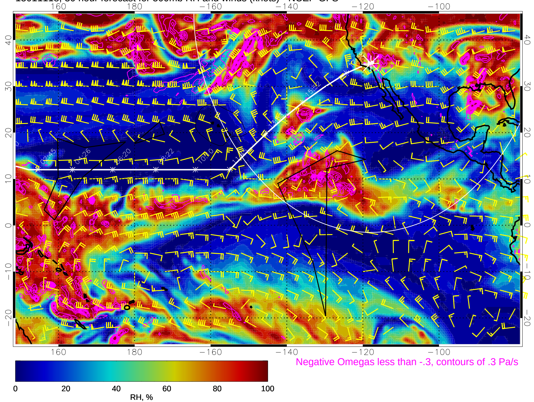
15011118, 30 hour forecast for 500mb RH and winds (knots) - NCEP GFS
