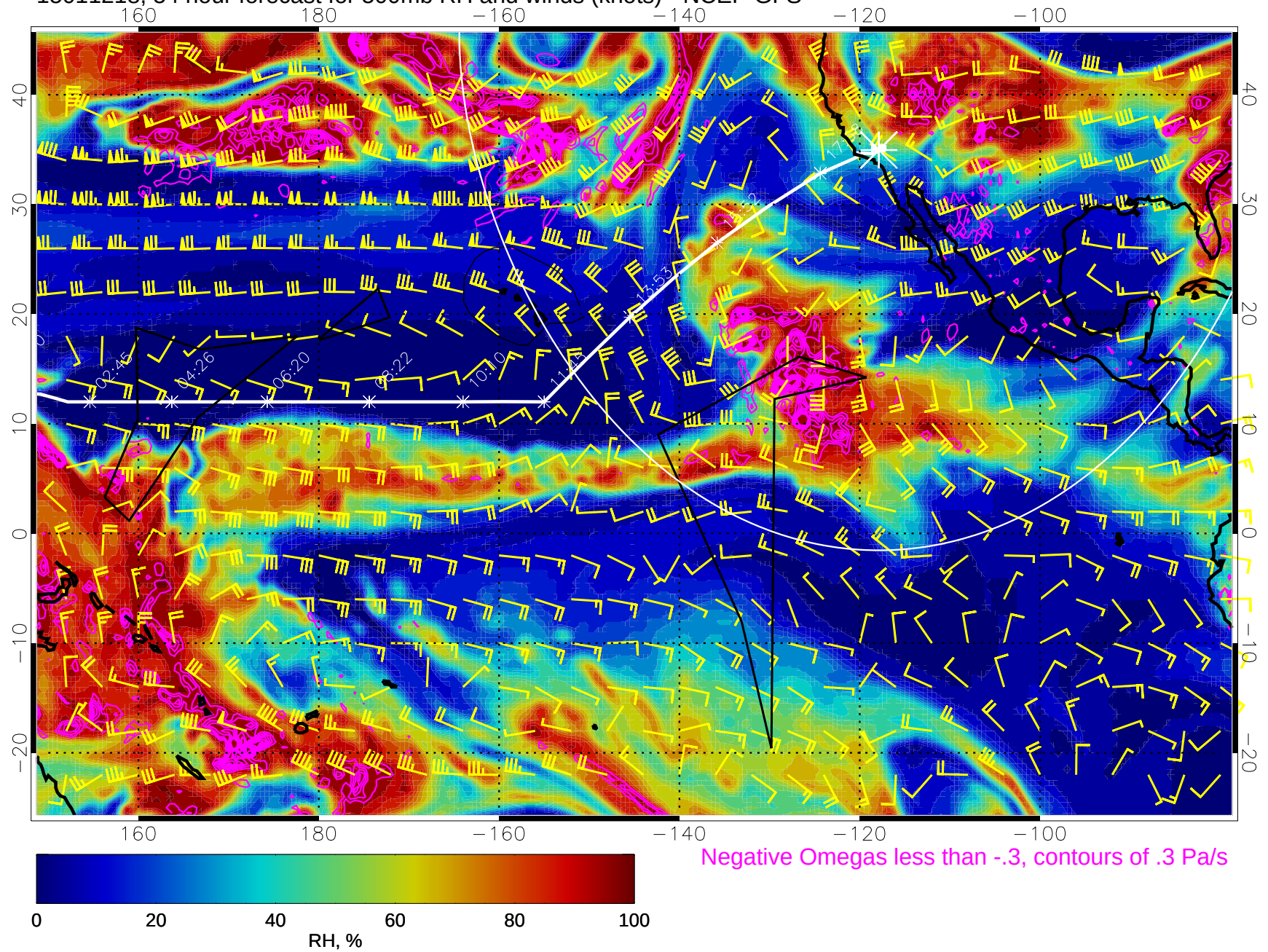
15011218, 54 hour forecast for 500mb RH and winds (knots) - NCEP GFS
