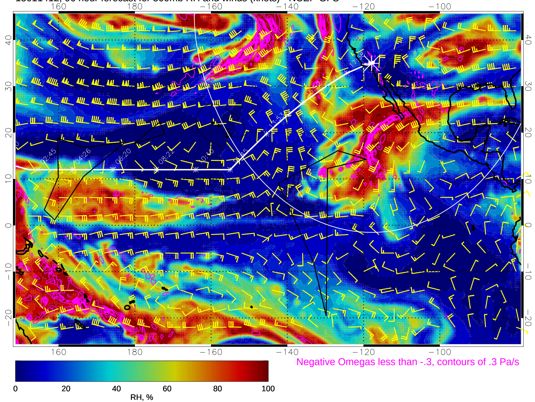
15011412, 96 hour forecast for 500mb RH and winds (knots) - NCEP GFS
