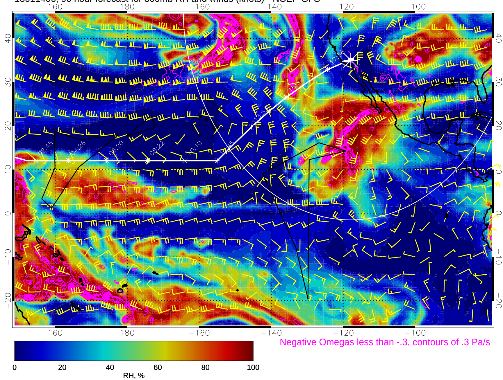
15011406, 90 hour forecast for 500mb RH and winds (knots) - NCEP GFS
