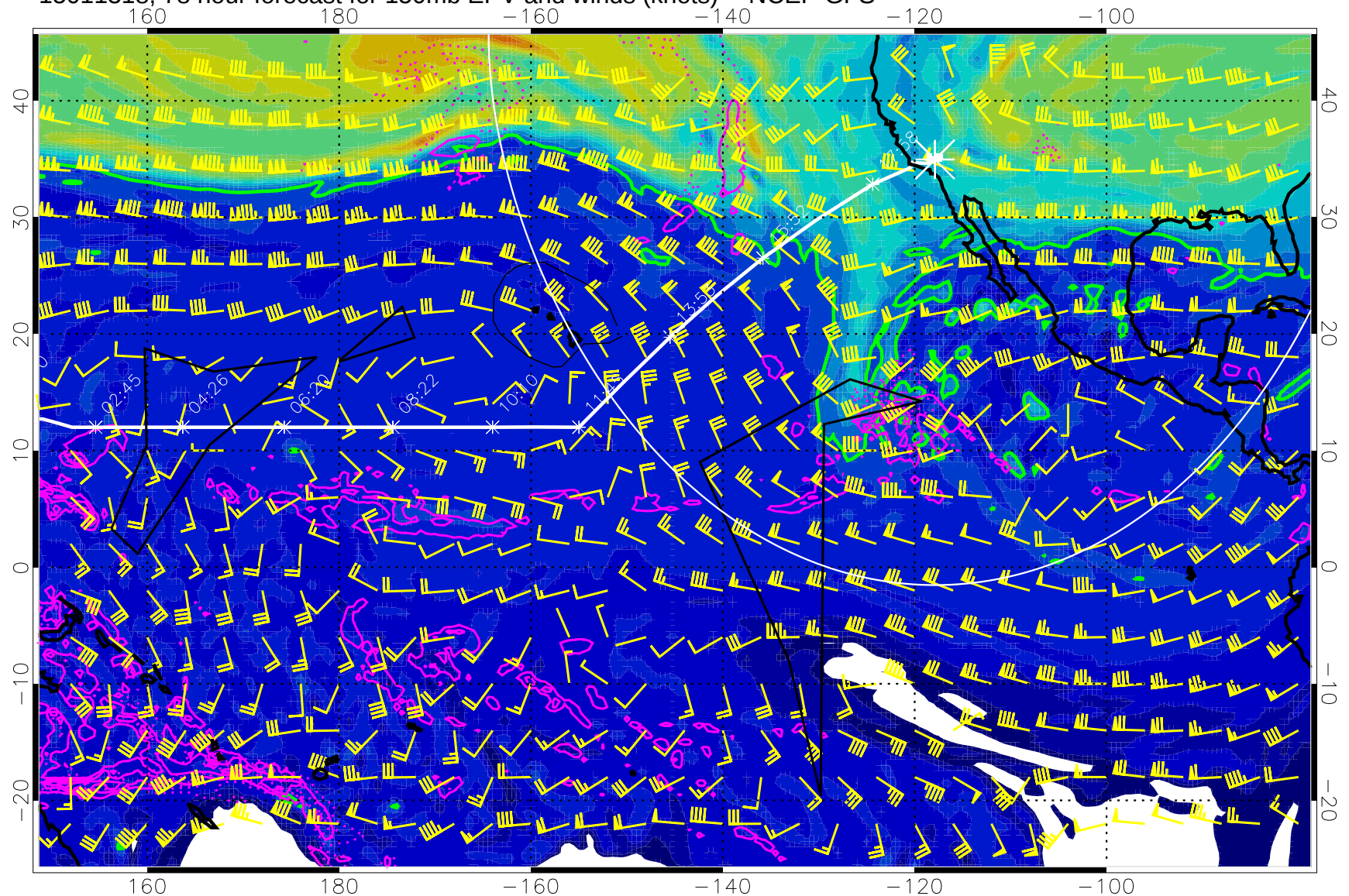
15011318, 78 hour forecast for 150mb EPV and winds (knots) -- NCEP GFS
