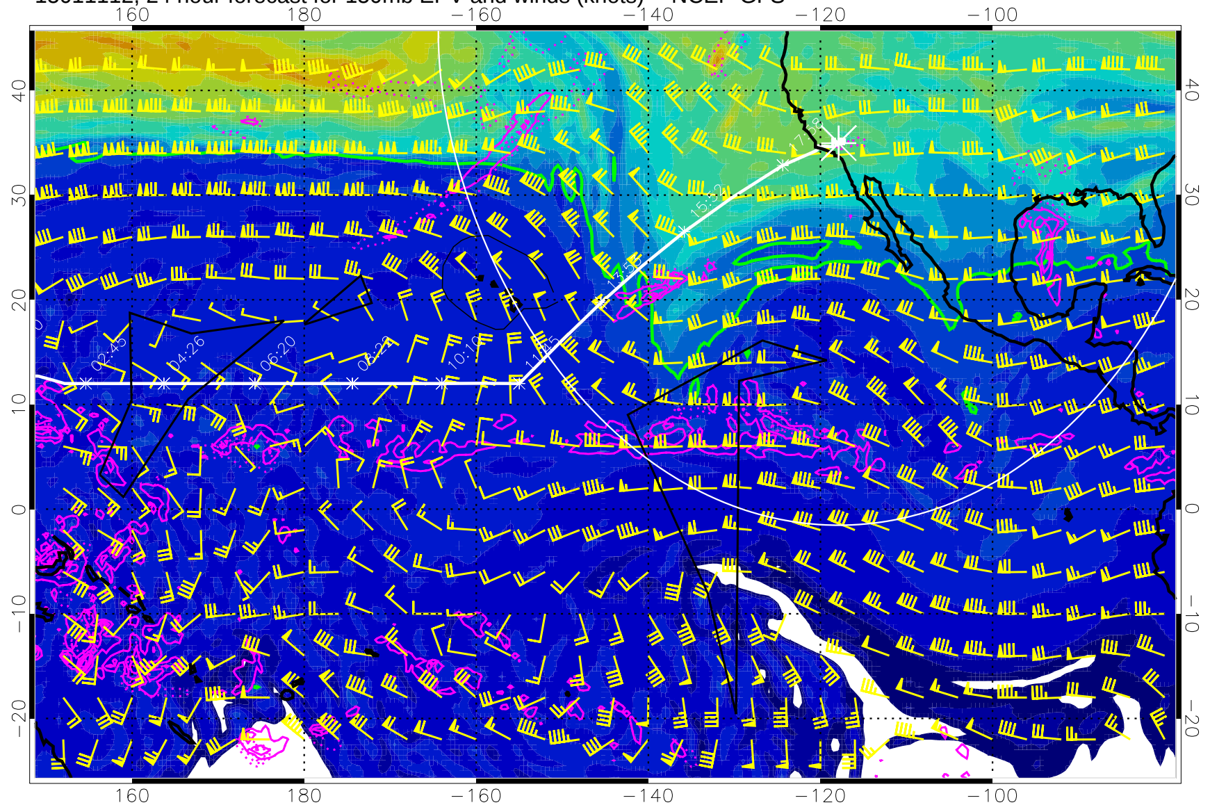
15011112, 24 hour forecast for 150mb EPV and winds (knots) -- NCEP GFS
