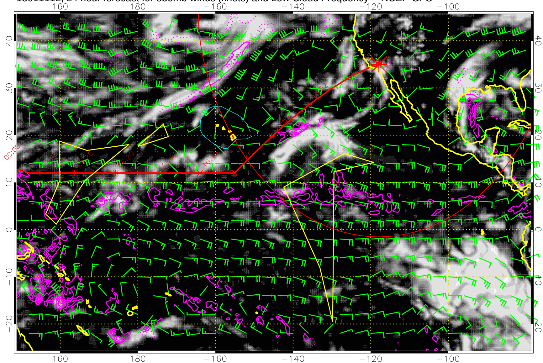
15011112, 24 hour forecast for 850mb winds (knots) and Low Cloud Frequency -- NCEP GFS
