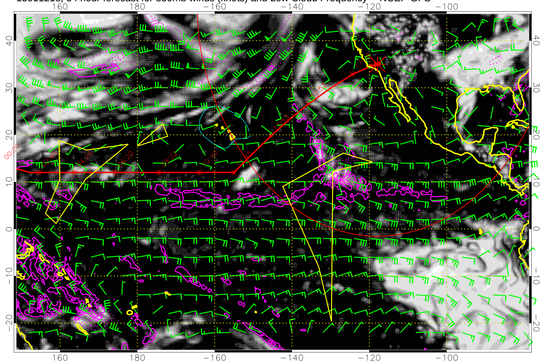
15011218, 54 hour forecast for 850mb winds (knots) and Low Cloud Frequency -- NCEP GFS
