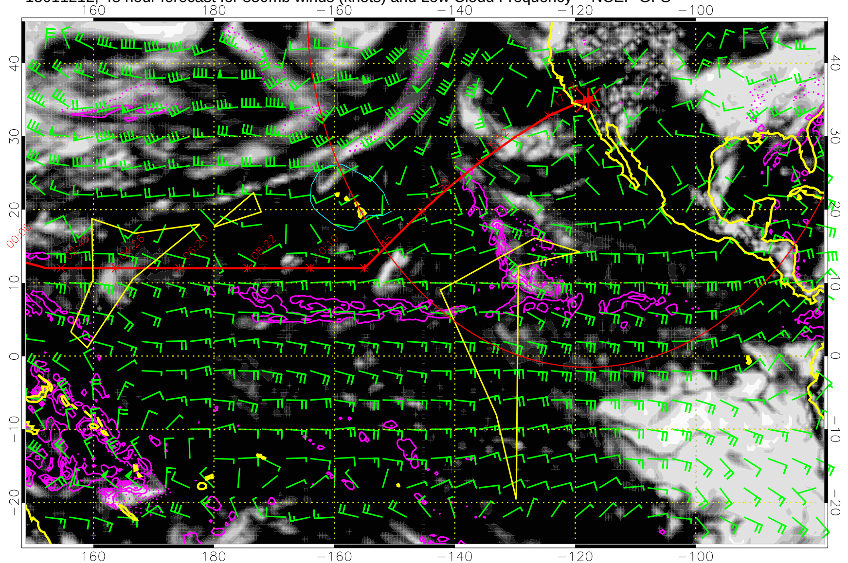
15011212, 48 hour forecast for 850mb winds (knots) and Low Cloud Frequency -- NCEP GFS
