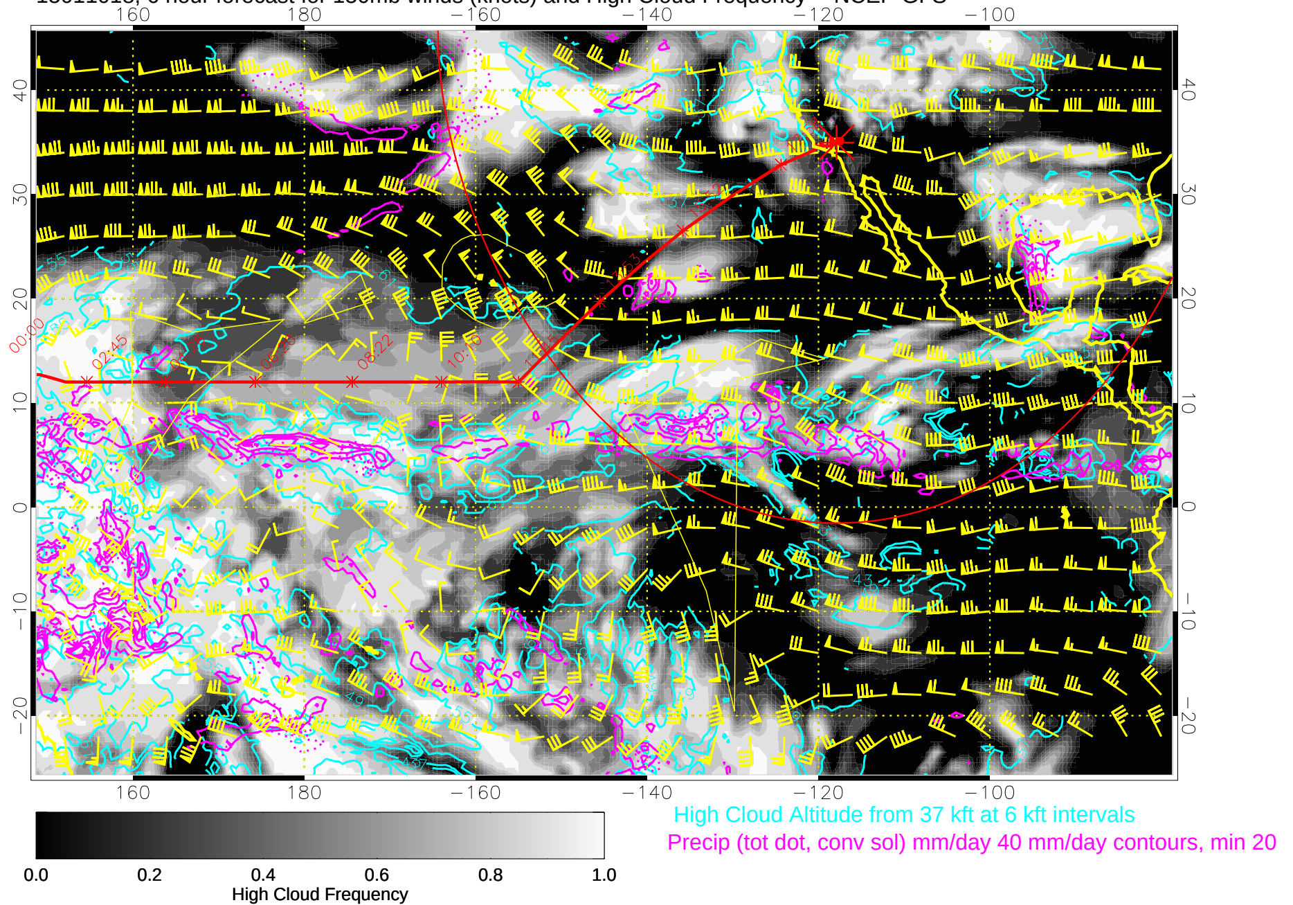
15011018, 6 hour forecast for 150mb winds (knots) and High Cloud Frequency -- NCEP GFS
